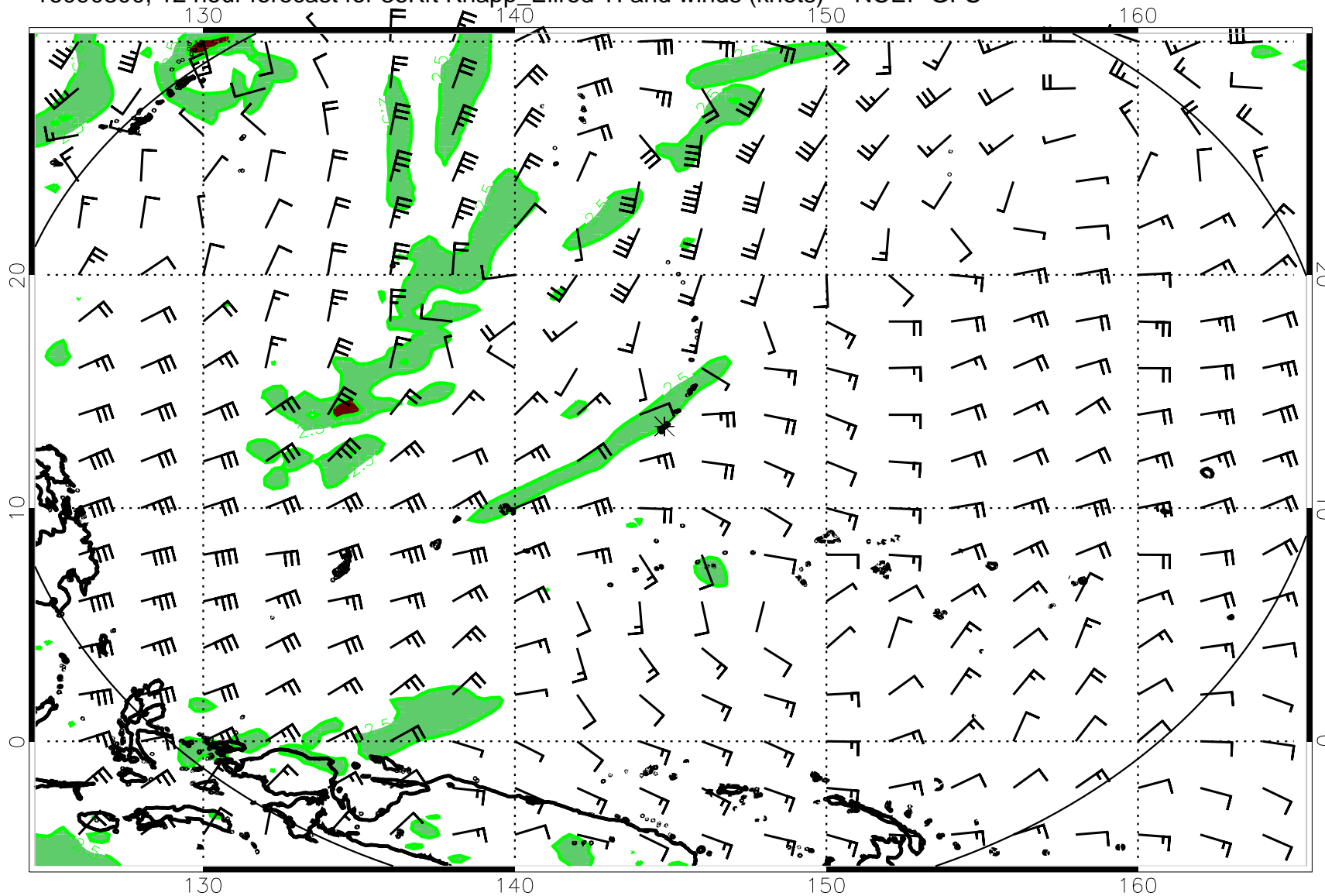
16090300, 12 hour forecast for 36Kft Knapp_Ellrod TI and winds (knots) -- NCEP GFS
