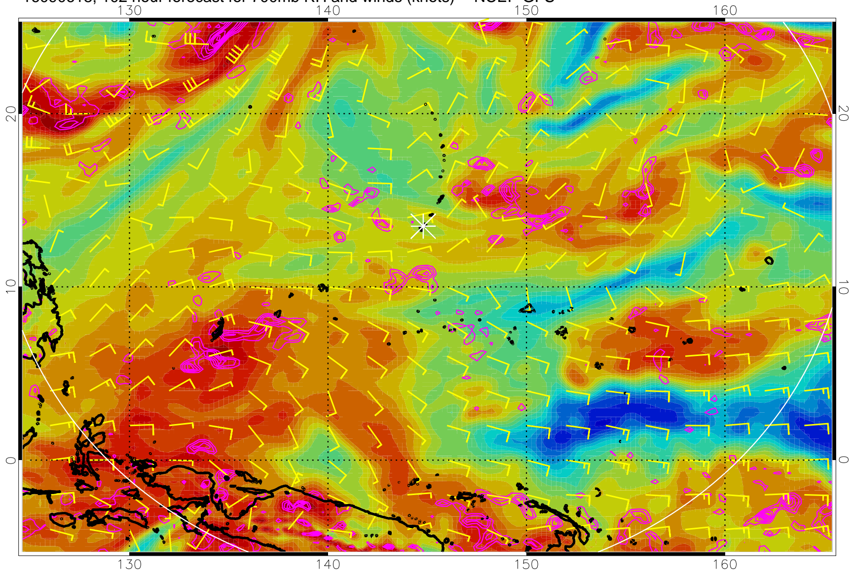
16090618, 102 hour forecast for 700mb RH and winds (knots) -- NCEP GFS
