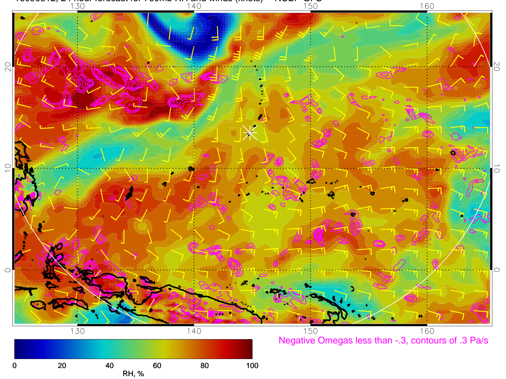
16090312, 24 hour forecast for 700mb RH and winds (knots) -- NCEP GFS
