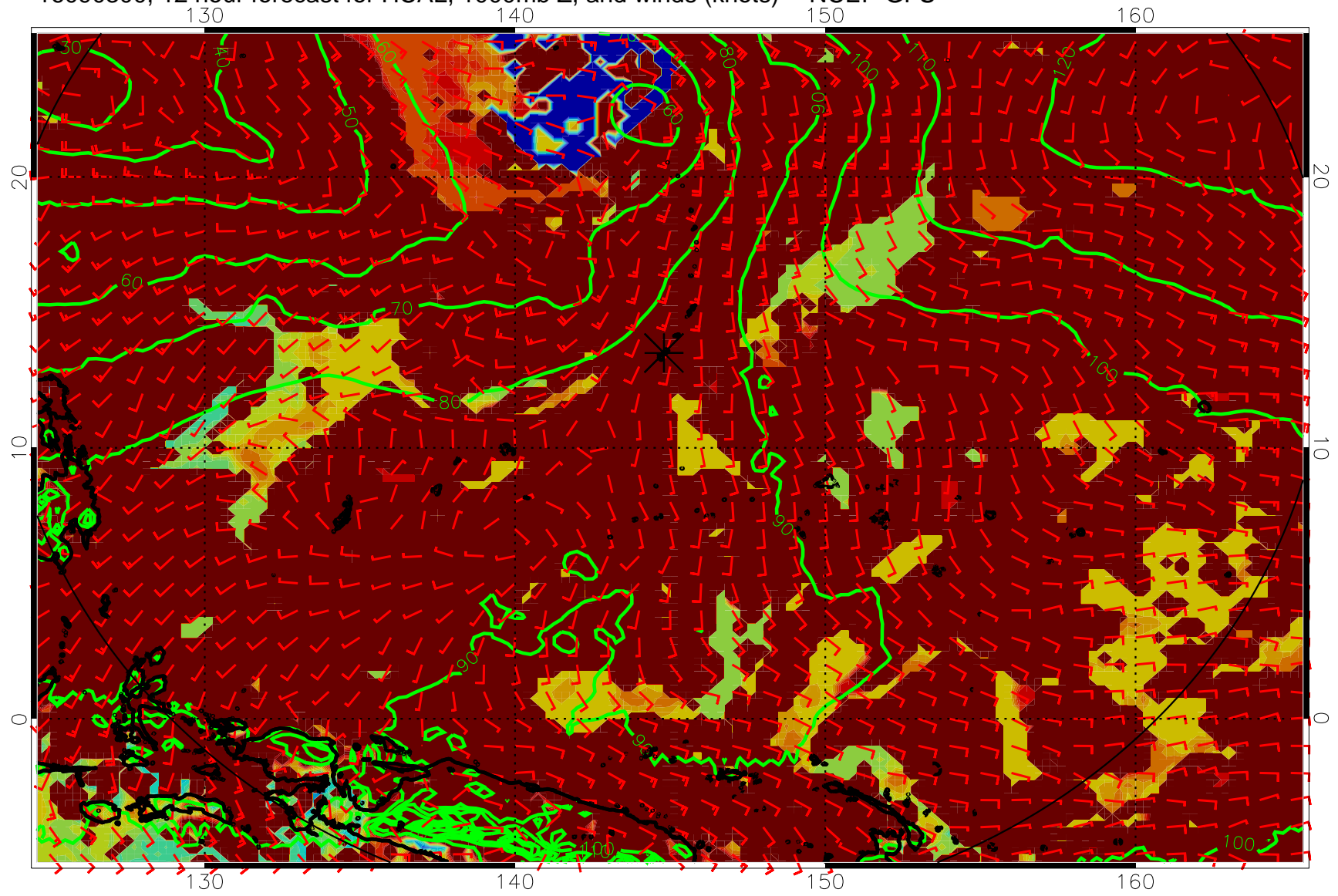
16090300, 12 hour forecast for HCAL, 1000mb Z, and winds (knots) -- NCEP GFS
