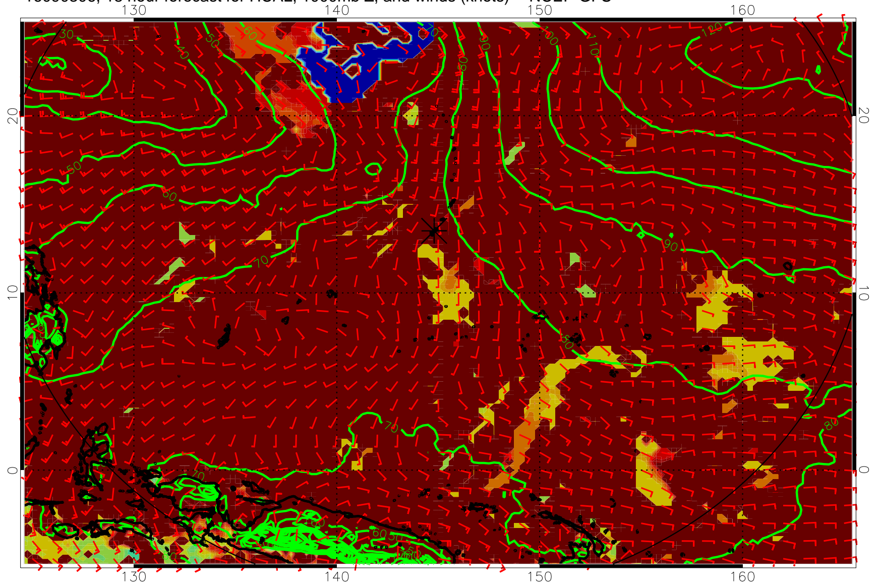
16090306, 18 hour forecast for HCAL, 1000mb Z, and winds (knots) -- NCEP GFS
