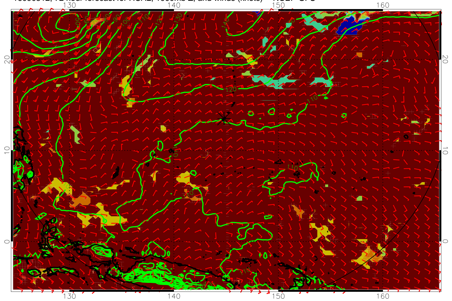
16090512, 72 hour forecast for HCAL, 1000mb Z, and winds (knots) -- NCEP GFS
