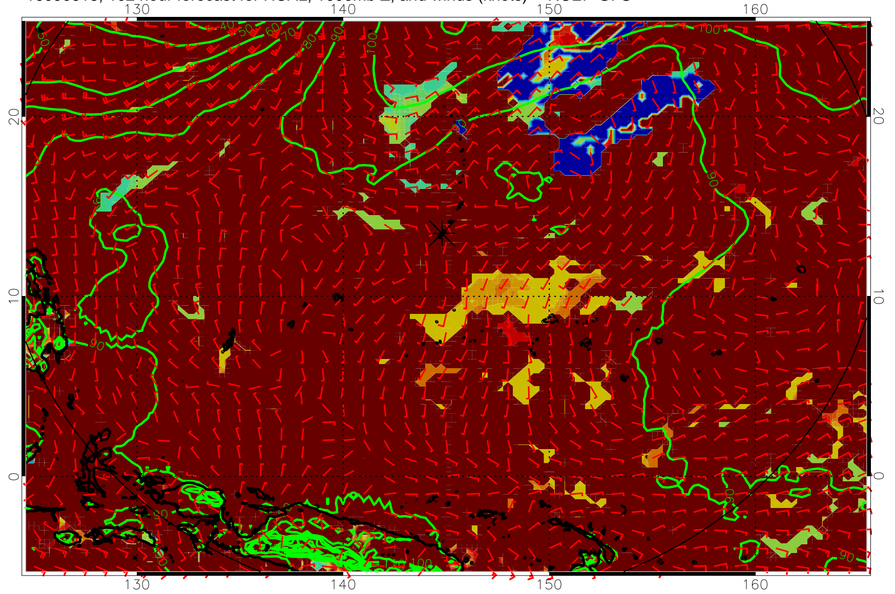
16090618, 102 hour forecast for HCAL, 1000mb Z, and winds (knots) -- NCEP GFS
