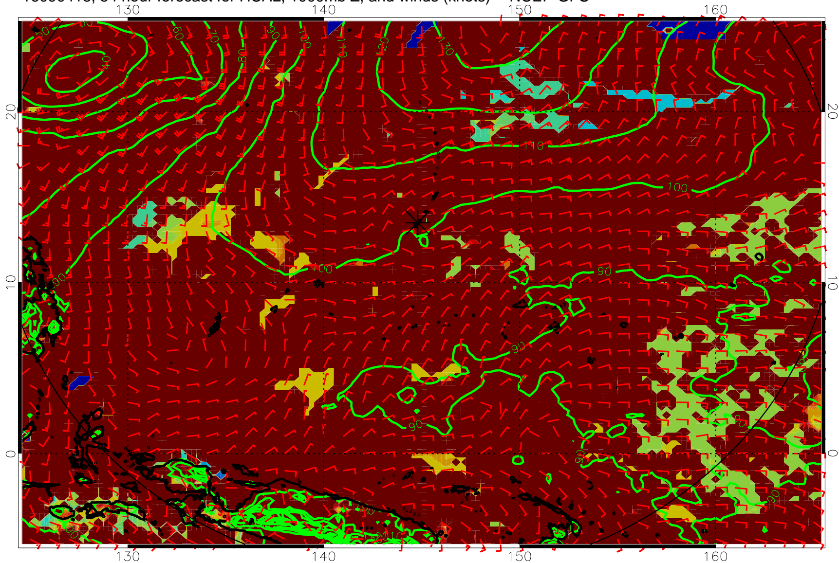
16090418, 54 hour forecast for HCAL, 1000mb Z, and winds (knots) -- NCEP GFS
