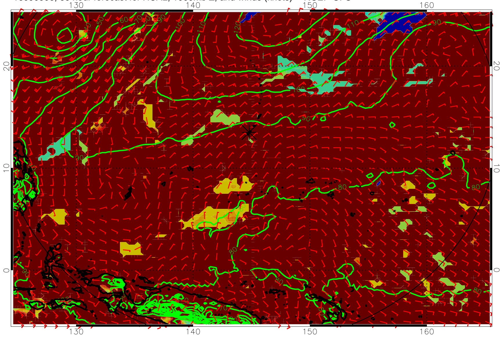
16090506, 66 hour forecast for HCAL, 1000mb Z, and winds (knots) -- NCEP GFS
