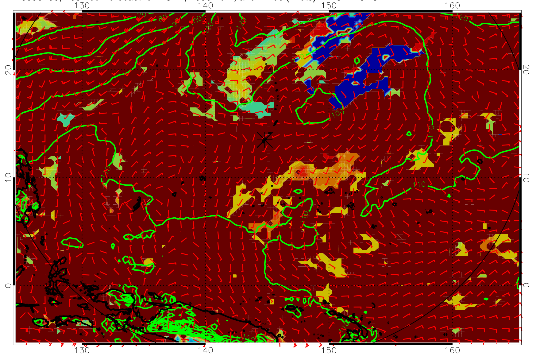
16090700, 108 hour forecast for HCAL, 1000mb Z, and winds (knots) -- NCEP GFS
