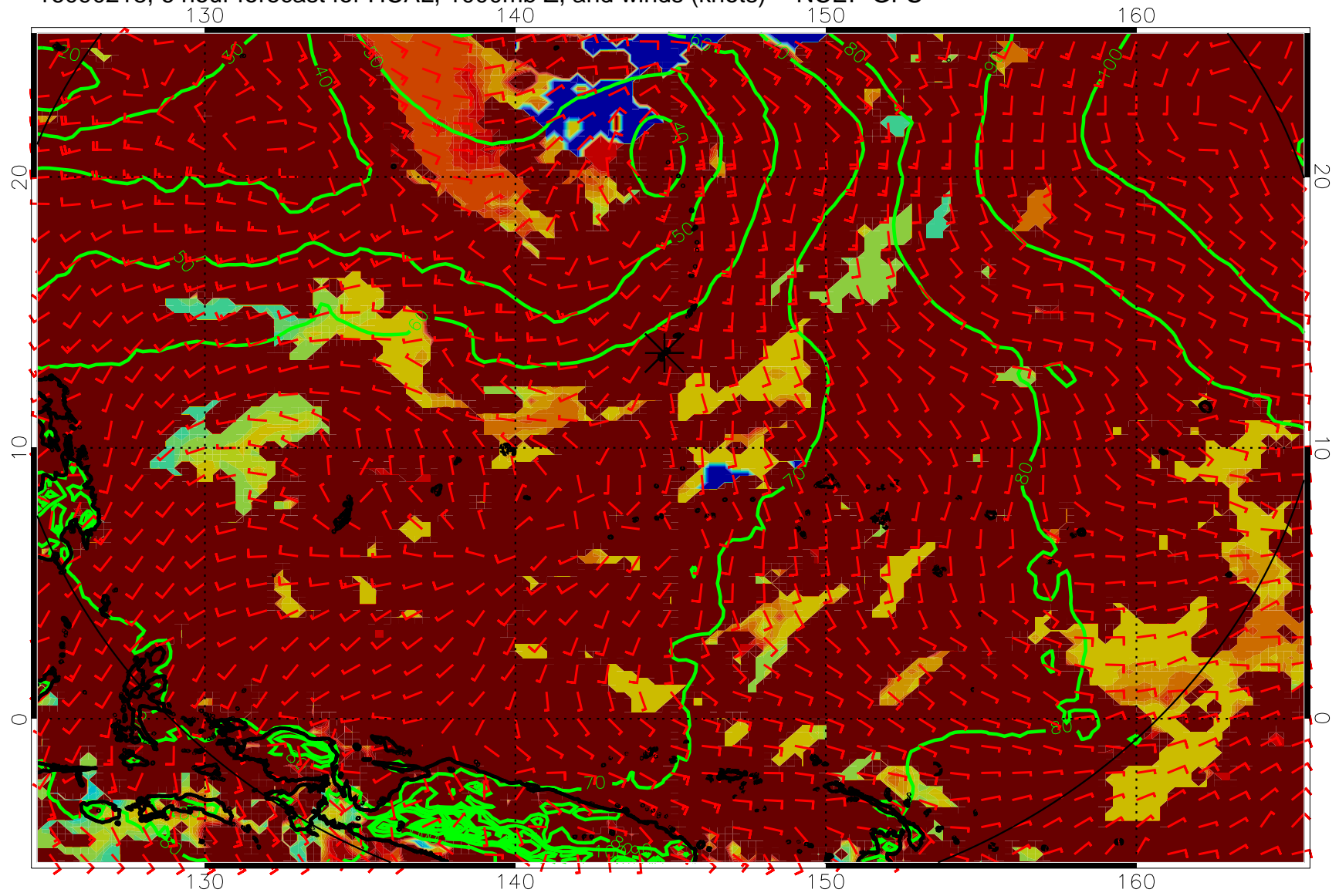
16090218, 6 hour forecast for HCAL, 1000mb Z, and winds (knots) -- NCEP GFS
