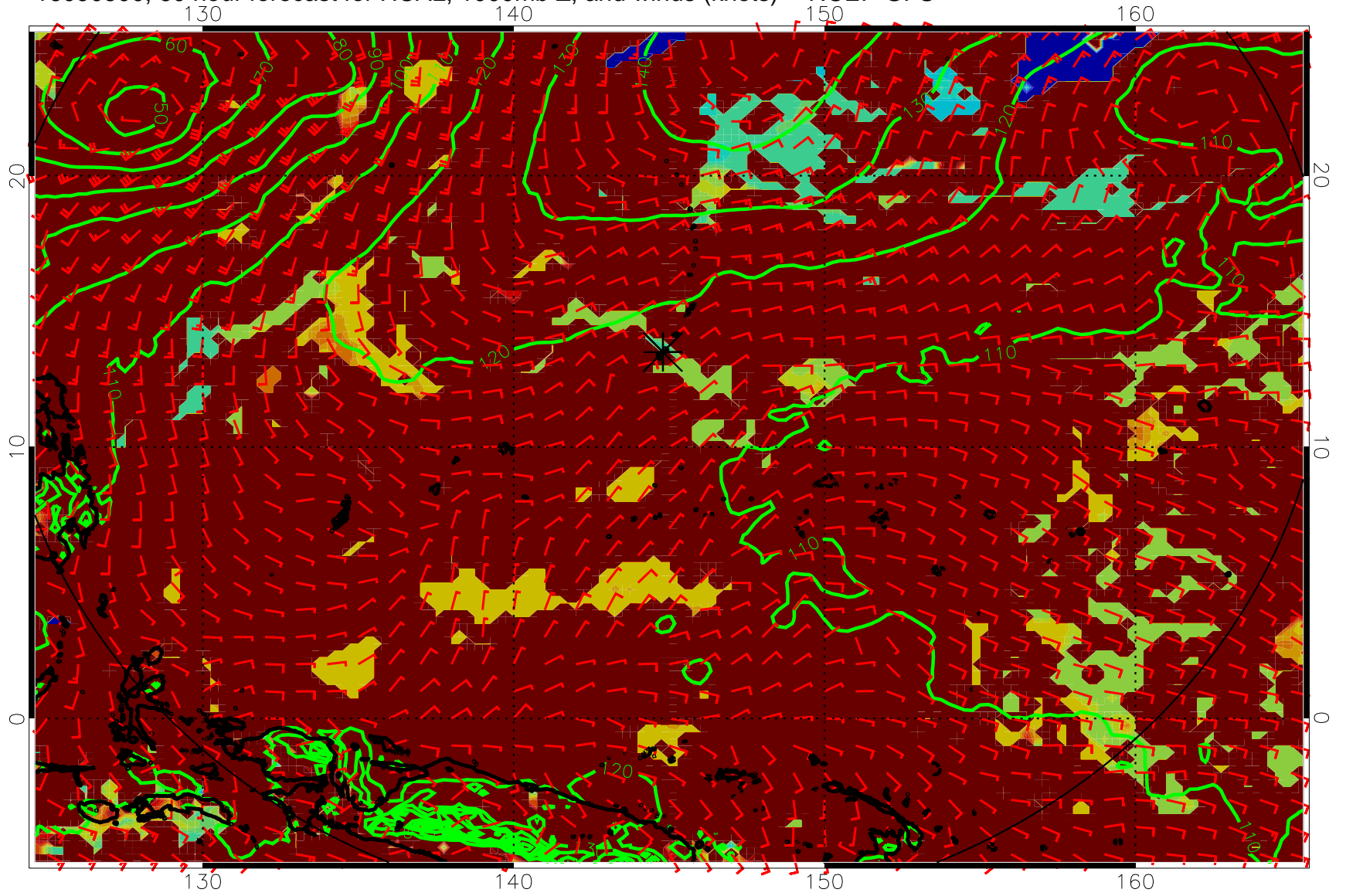
16090500, 60 hour forecast for HCAL, 1000mb Z, and winds (knots) -- NCEP GFS
