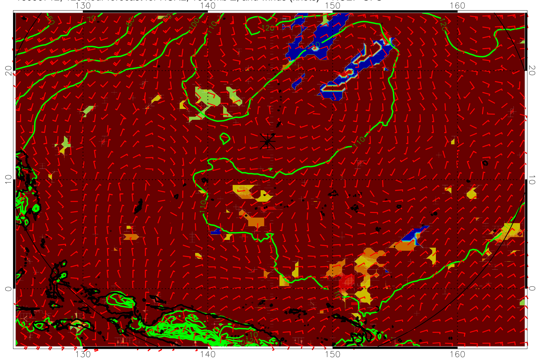
16090712, 120 hour forecast for HCAL, 1000mb Z, and winds (knots) -- NCEP GFS
