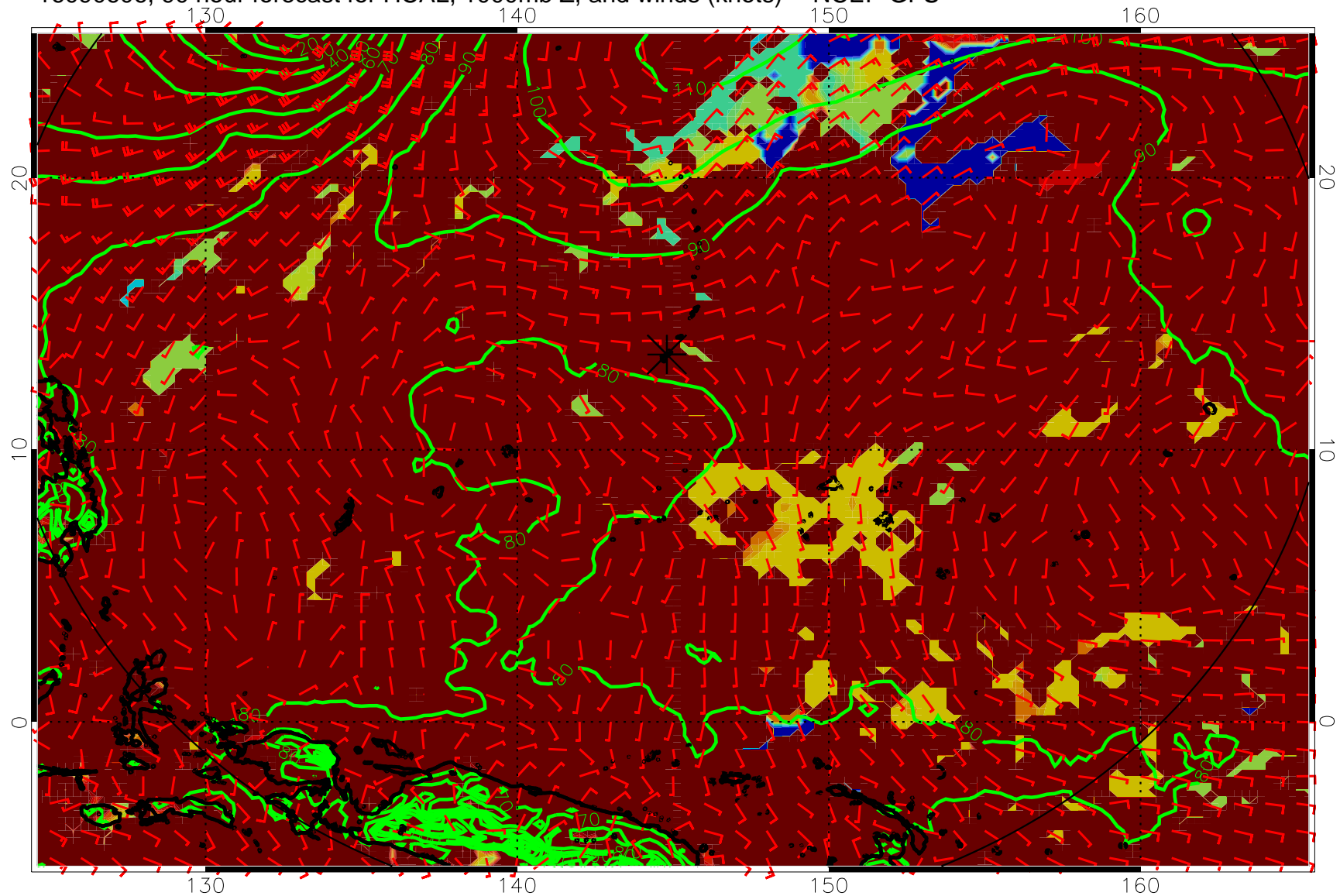
16090606, 90 hour forecast for HCAL, 1000mb Z, and winds (knots) -- NCEP GFS
