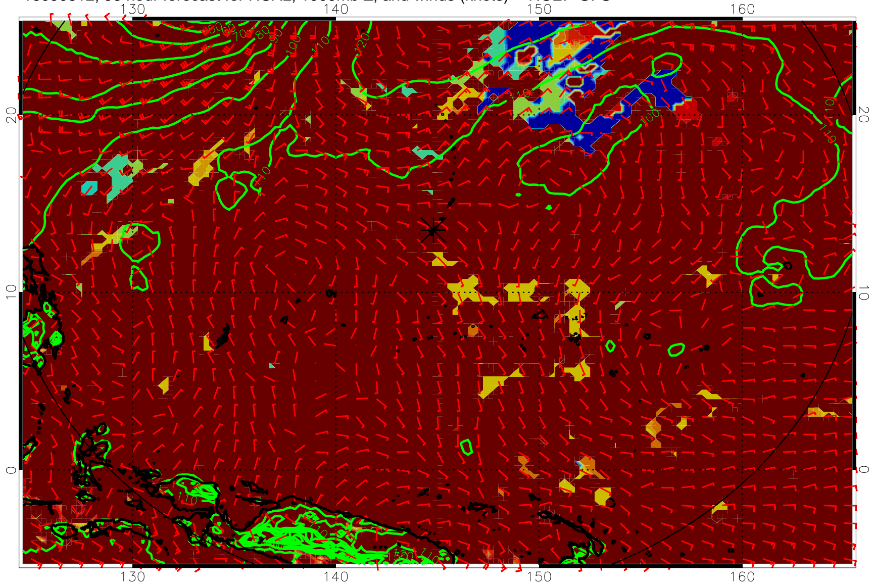
16090612, 96 hour forecast for HCAL, 1000mb Z, and winds (knots) -- NCEP GFS
