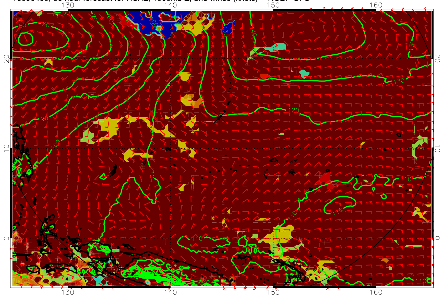
16090400, 36 hour forecast for HCAL, 1000mb Z, and winds (knots) -- NCEP GFS
