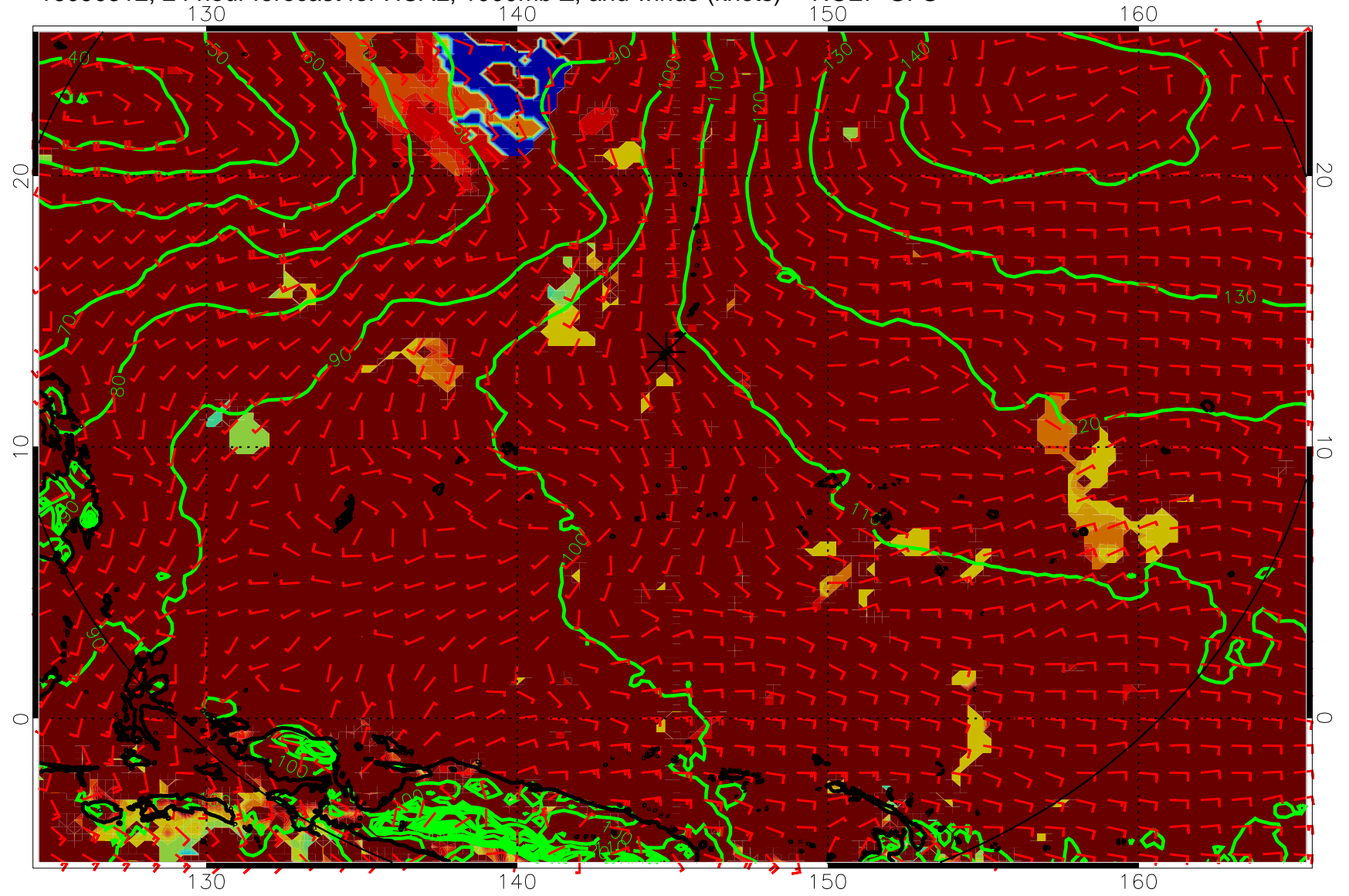
16090312, 24 hour forecast for HCAL, 1000mb Z, and winds (knots) -- NCEP GFS
