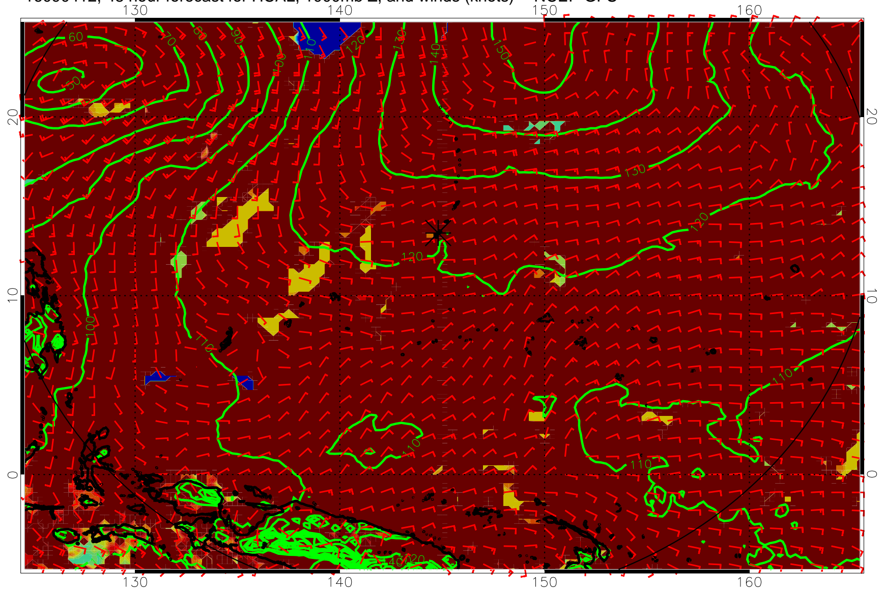
16090412, 48 hour forecast for HCAL, 1000mb Z, and winds (knots) -- NCEP GFS
