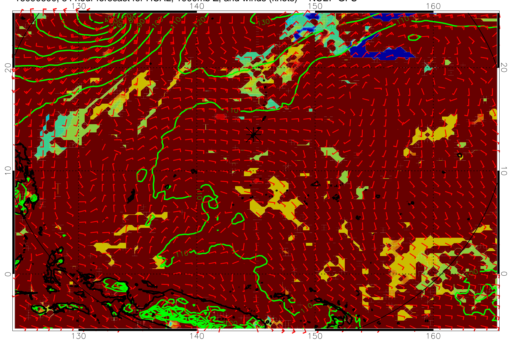
16090600, 84 hour forecast for HCAL, 1000mb Z, and winds (knots) -- NCEP GFS
