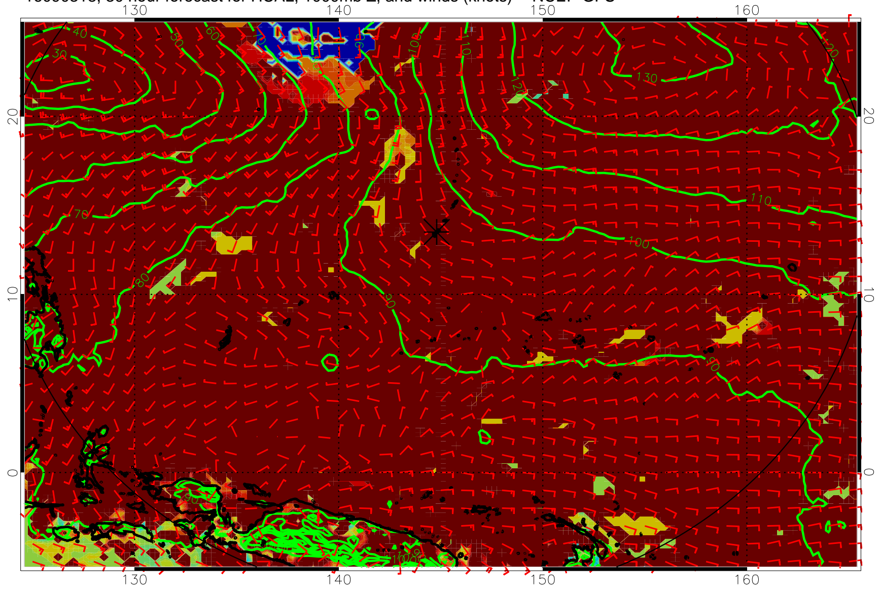
16090318, 30 hour forecast for HCAL, 1000mb Z, and winds (knots) -- NCEP GFS
