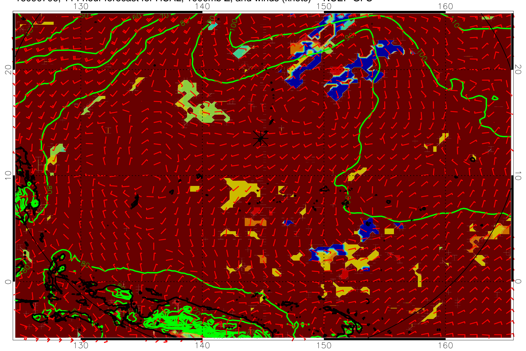
16090706, 114 hour forecast for HCAL, 1000mb Z, and winds (knots) -- NCEP GFS
