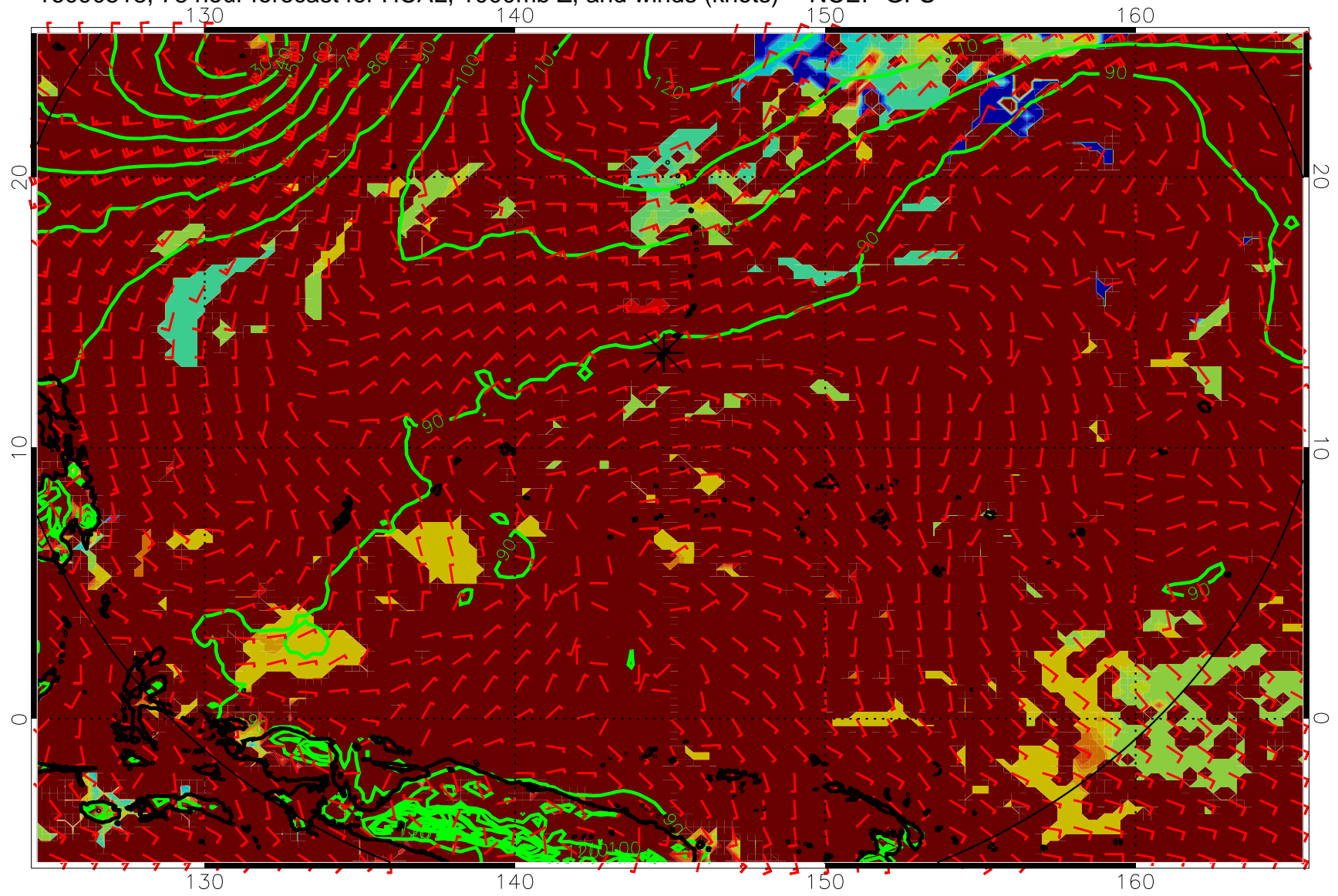
16090518, 78 hour forecast for HCAL, 1000mb Z, and winds (knots) -- NCEP GFS
