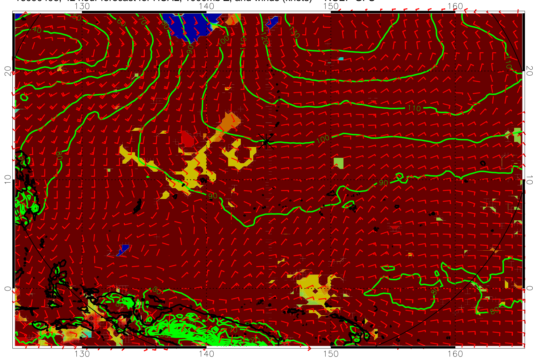
16090406, 42 hour forecast for HCAL, 1000mb Z, and winds (knots) -- NCEP GFS
