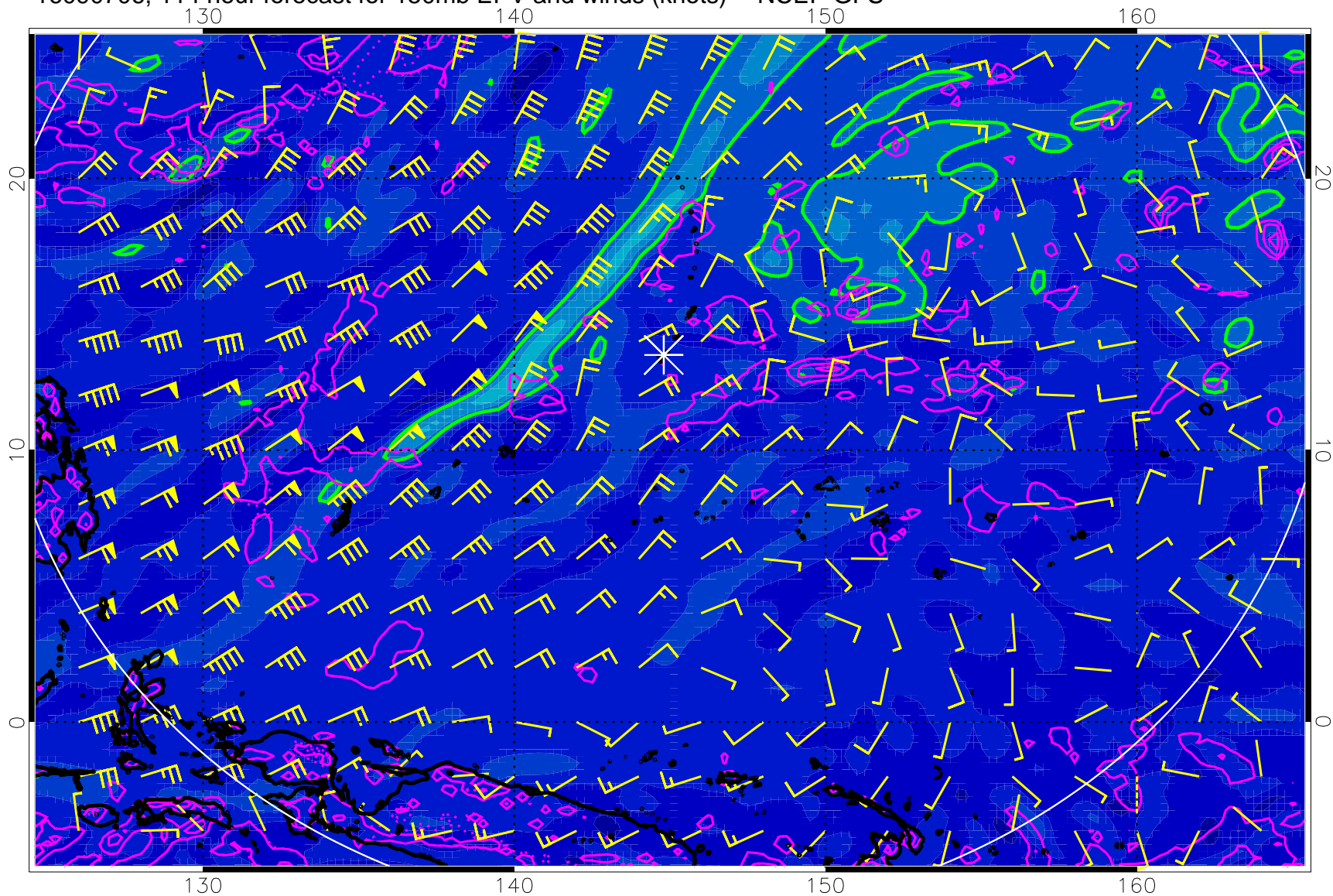
16090706, 114 hour forecast for 150mb EPV and winds (knots) -- NCEP GFS
