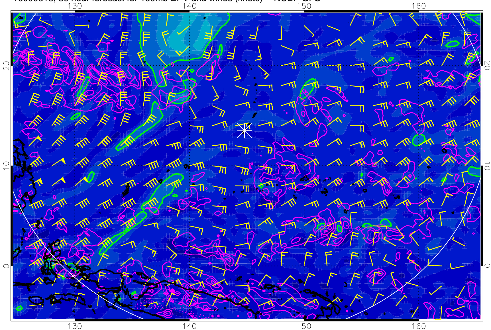
16090318, 30 hour forecast for 150mb EPV and winds (knots) -- NCEP GFS
