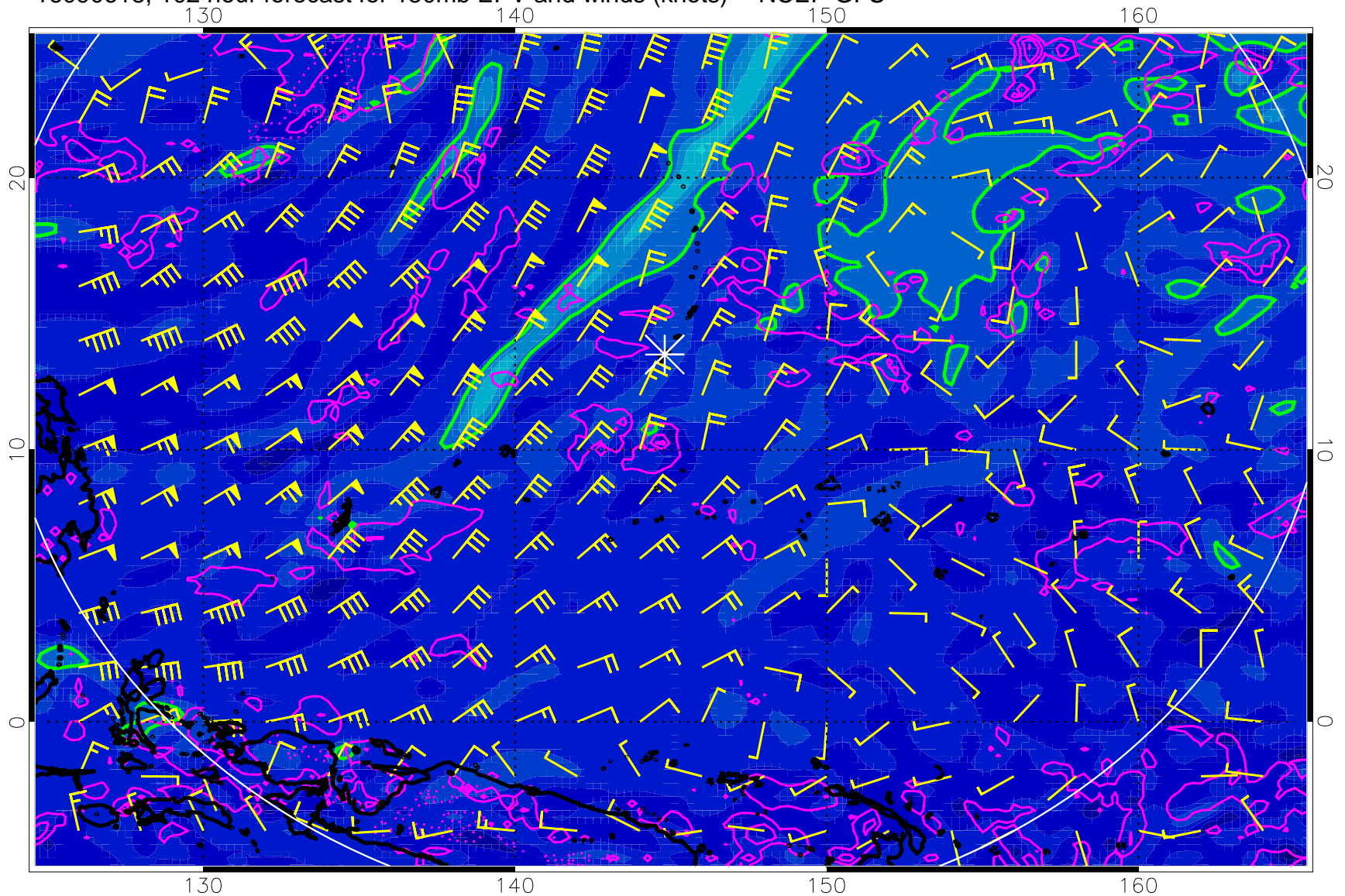
16090618, 102 hour forecast for 150mb EPV and winds (knots) -- NCEP GFS
