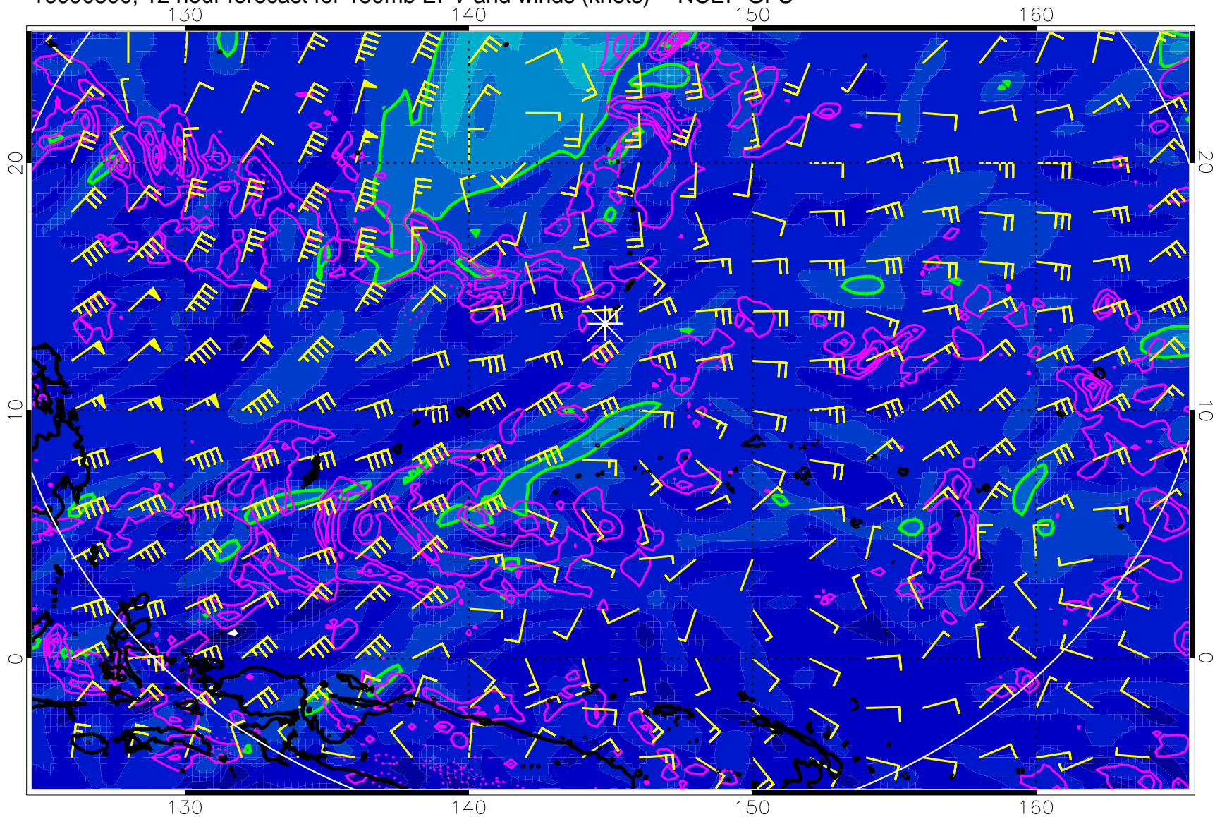
16090300, 12 hour forecast for 150mb EPV and winds (knots) -- NCEP GFS
