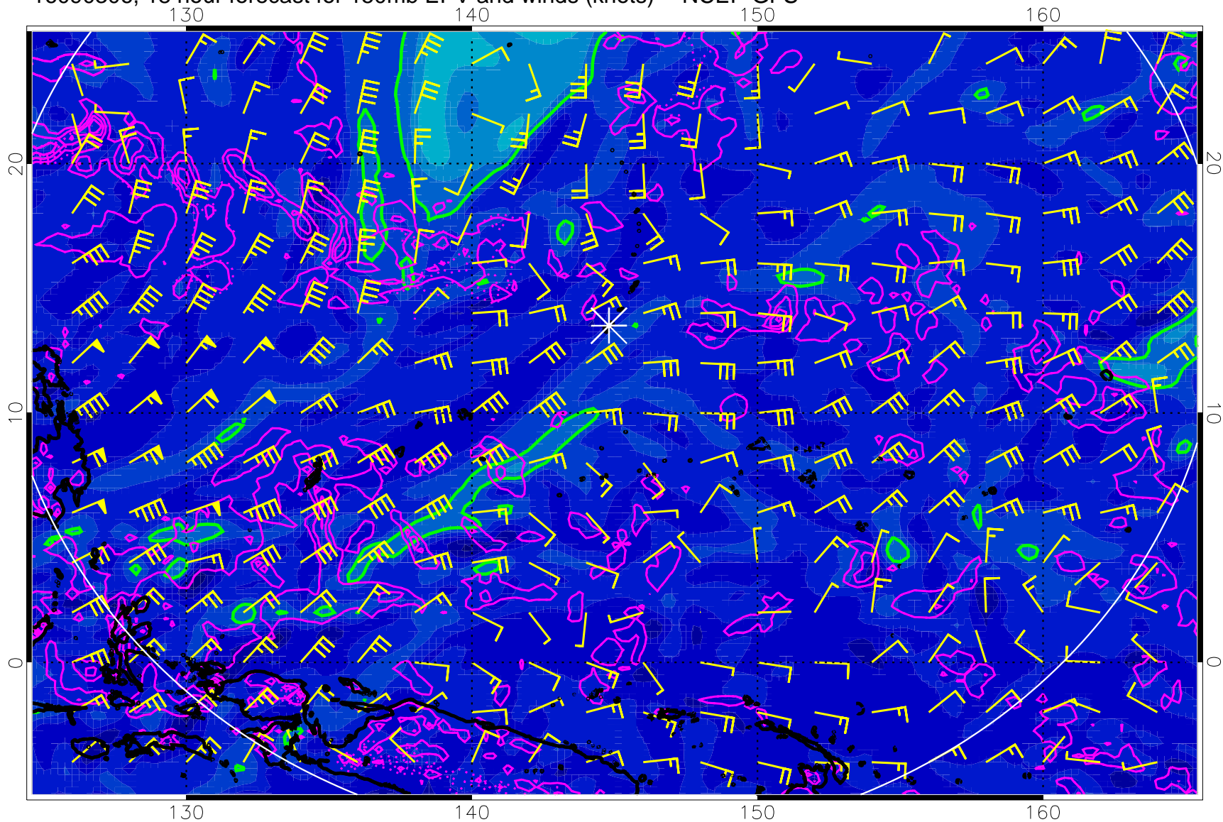
16090306, 18 hour forecast for 150mb EPV and winds (knots) -- NCEP GFS
