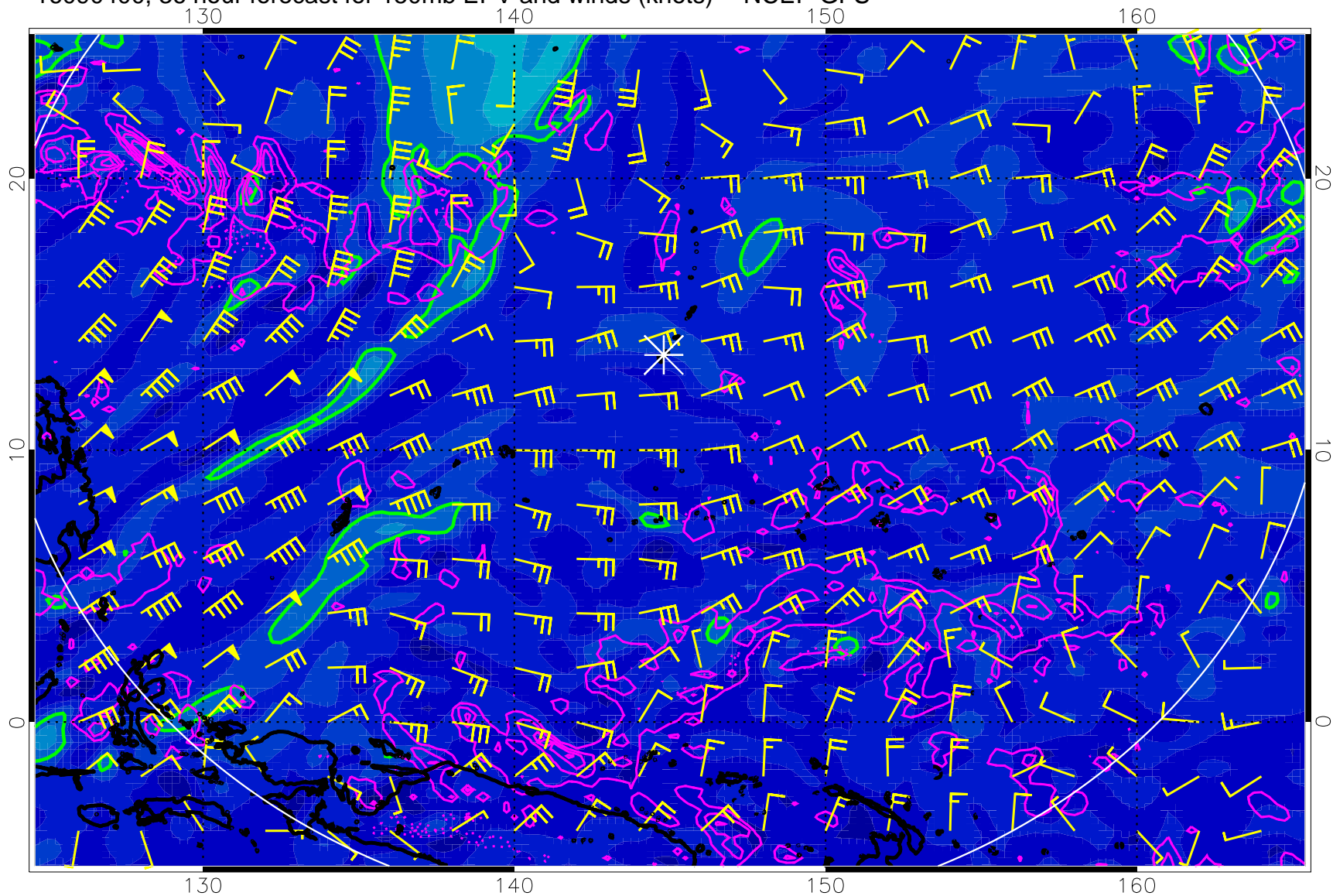
16090400, 36 hour forecast for 150mb EPV and winds (knots) -- NCEP GFS
