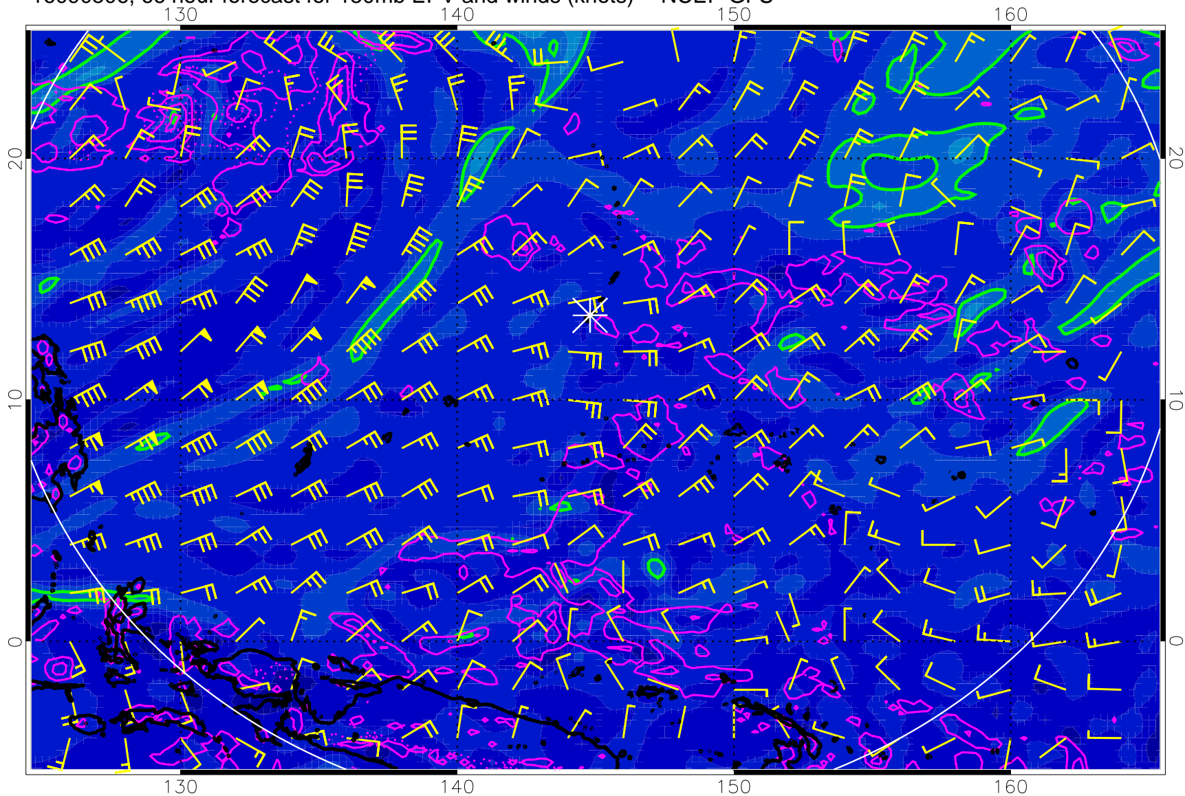
16090506, 66 hour forecast for 150mb EPV and winds (knots) -- NCEP GFS
