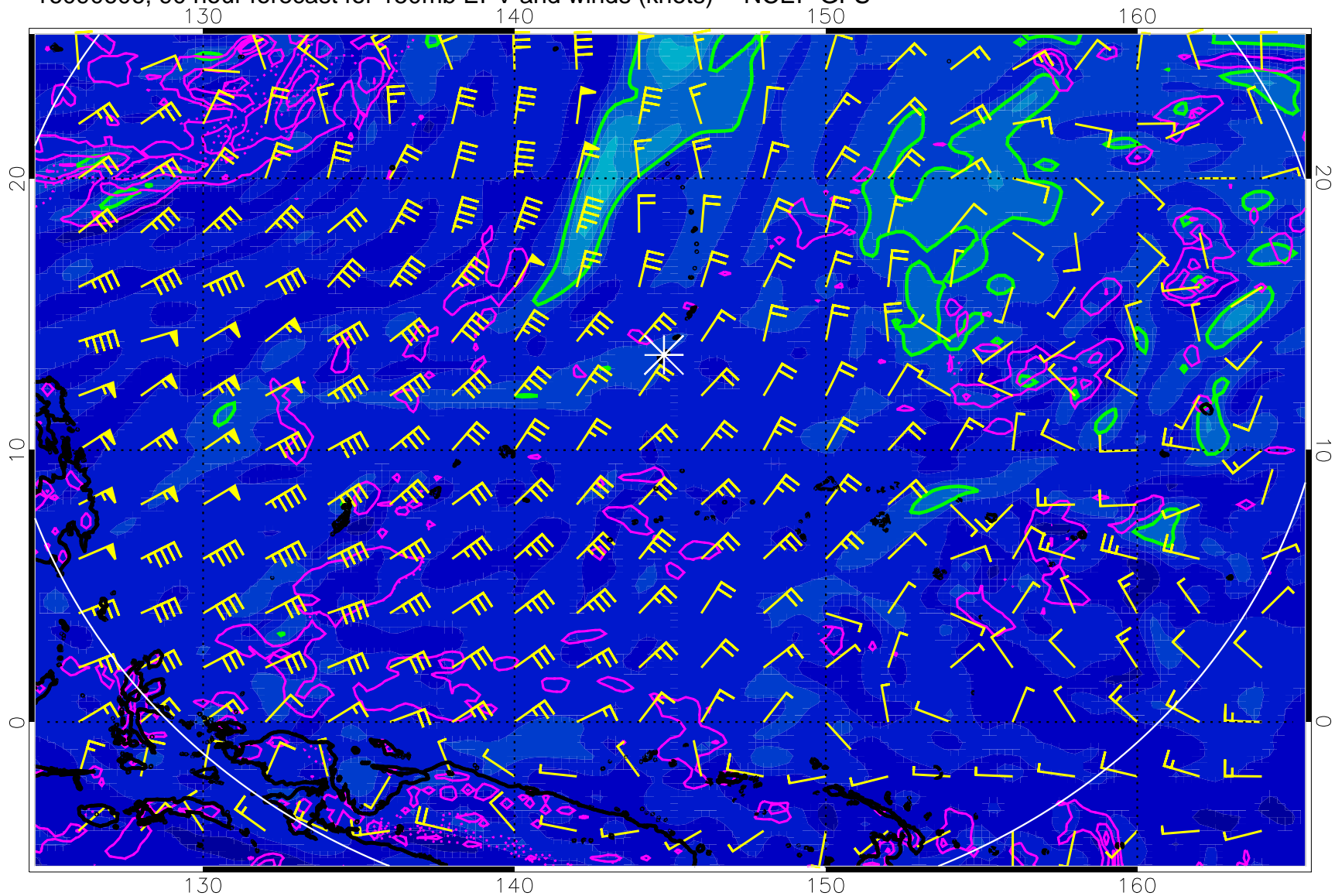
16090606, 90 hour forecast for 150mb EPV and winds (knots) -- NCEP GFS
