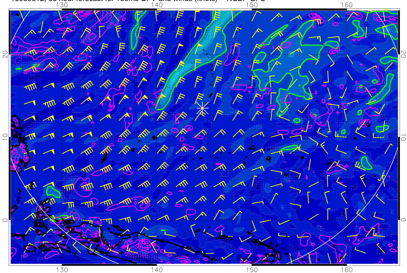
16090612, 96 hour forecast for 150mb EPV and winds (knots) -- NCEP GFS
