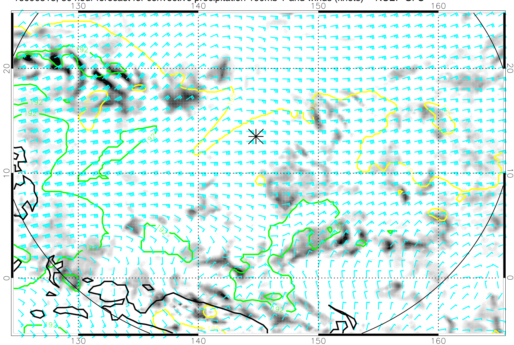
16090318, 30 hour forecast for convective precipitation 100mb T and winds (knots) -- NCEP GFS
