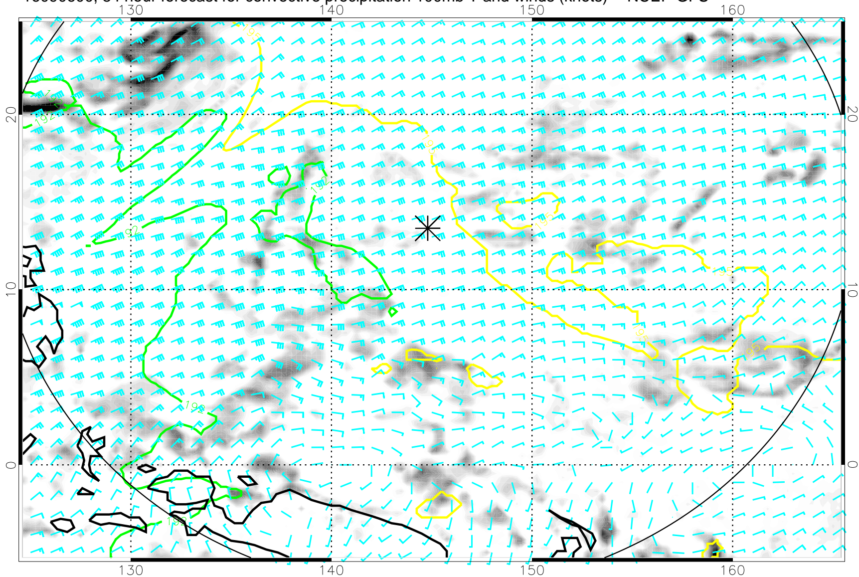
16090600, 84 hour forecast for convective precipitation 100mb T and winds (knots) -- NCEP GFS
