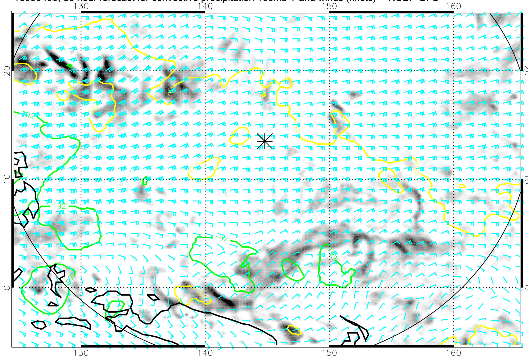
16090400, 36 hour forecast for convective precipitation 100mb T and winds (knots) -- NCEP GFS
