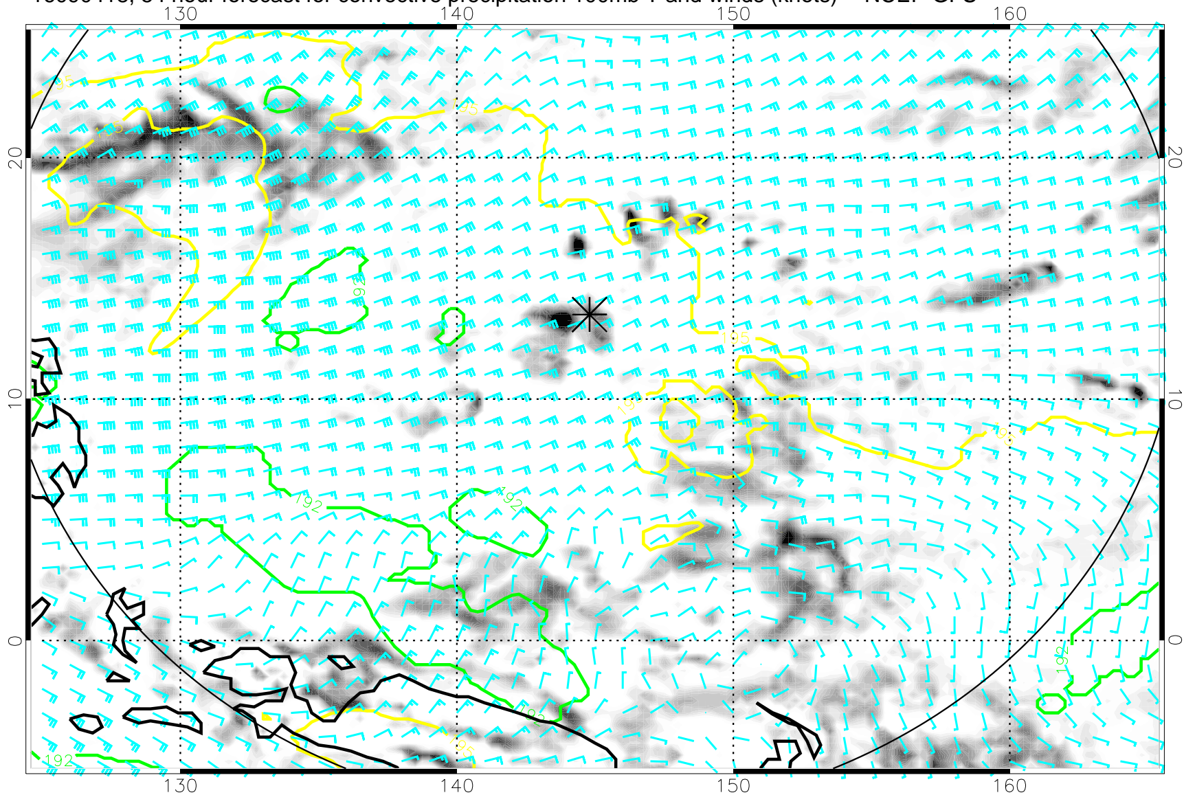
16090418, 54 hour forecast for convective precipitation 100mb T and winds (knots) -- NCEP GFS
