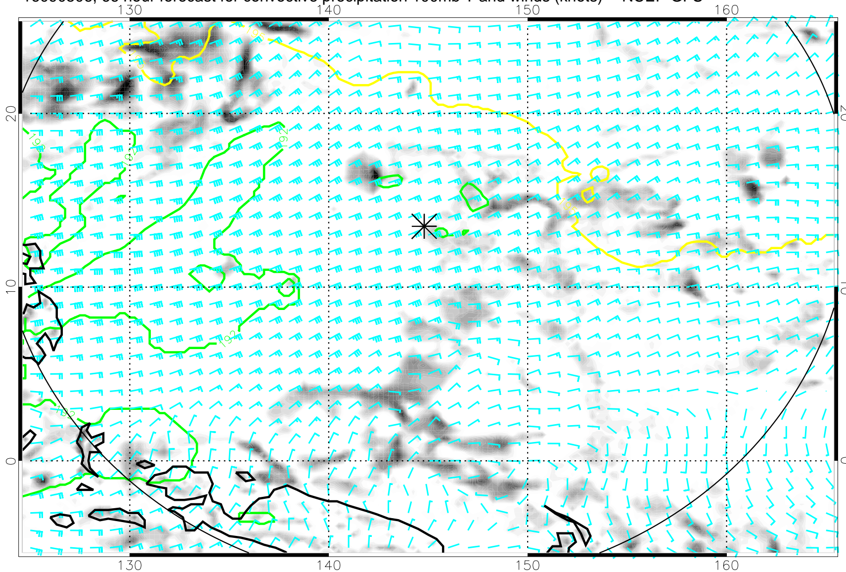
16090506, 66 hour forecast for convective precipitation 100mb T and winds (knots) -- NCEP GFS
