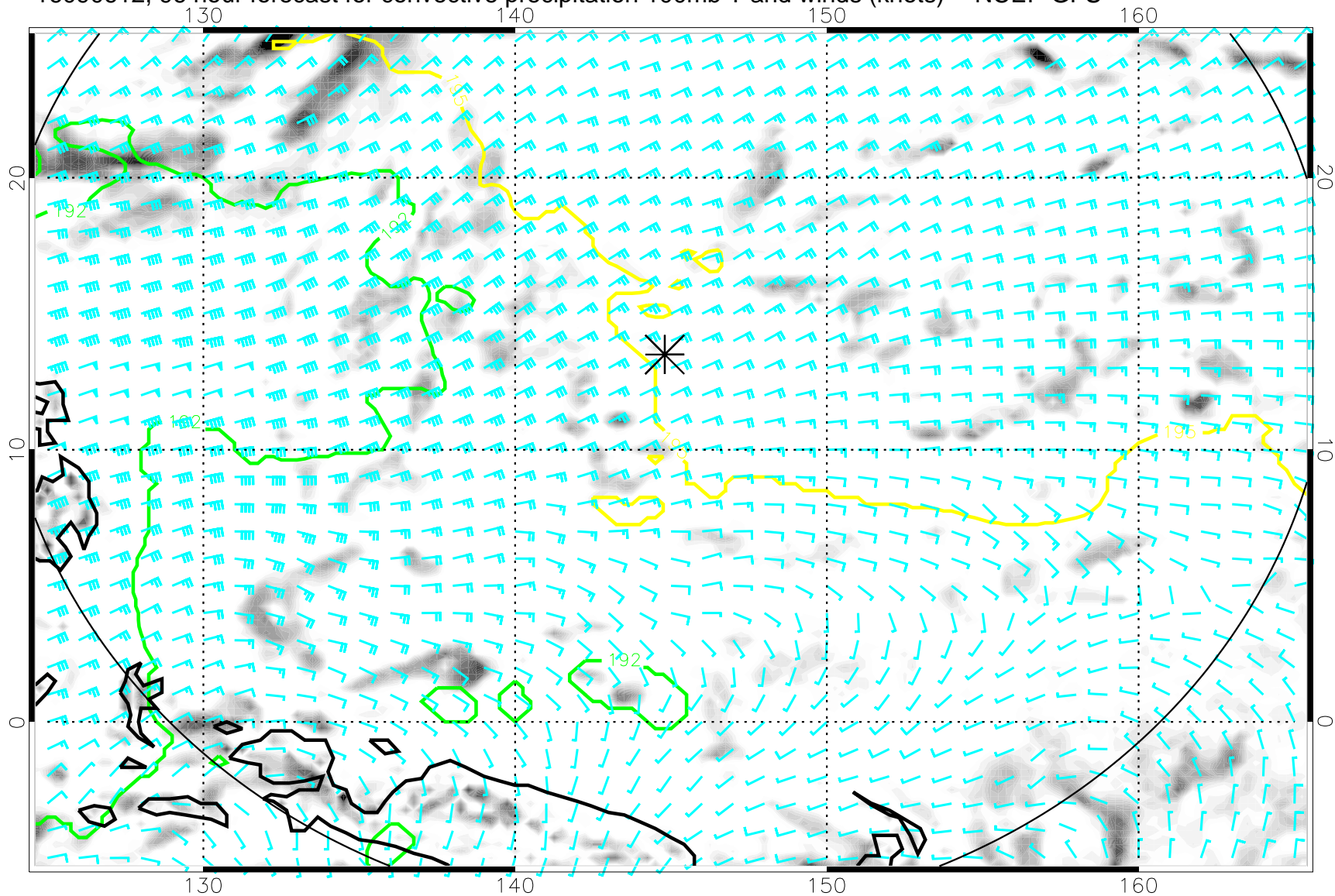
16090612, 96 hour forecast for convective precipitation 100mb T and winds (knots) -- NCEP GFS
