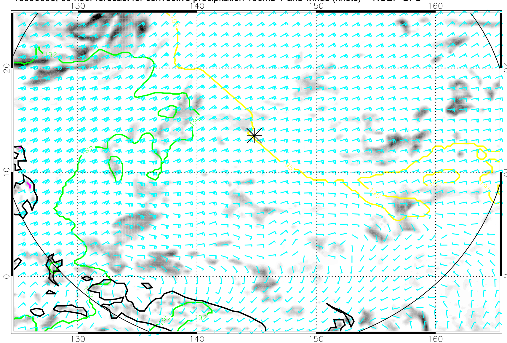
16090606, 90 hour forecast for convective precipitation 100mb T and winds (knots) -- NCEP GFS
