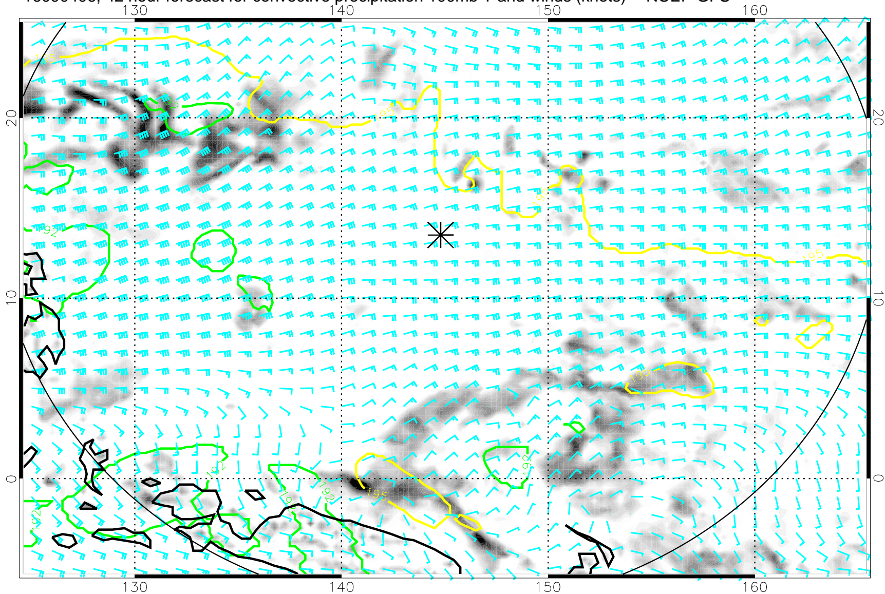
16090406, 42 hour forecast for convective precipitation 100mb T and winds (knots) -- NCEP GFS
