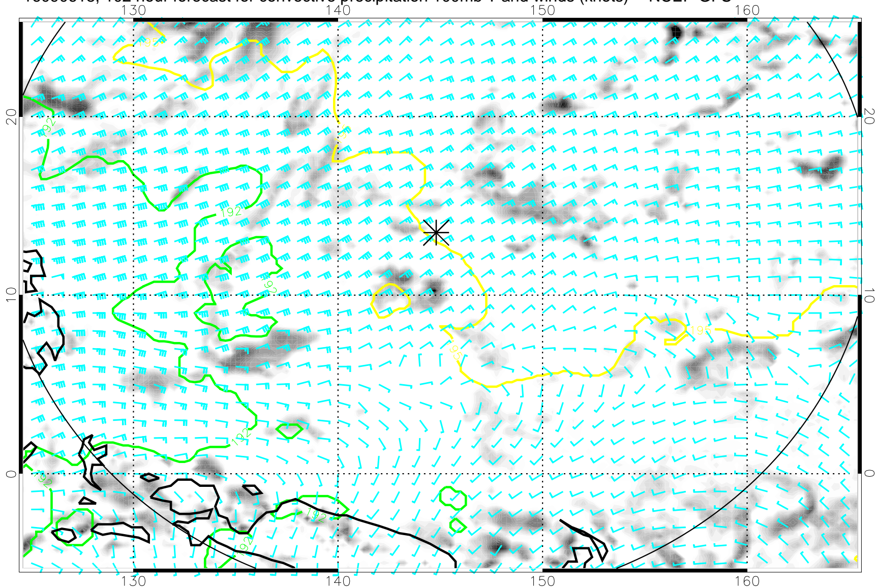
16090618, 102 hour forecast for convective precipitation 100mb T and winds (knots) -- NCEP GFS
