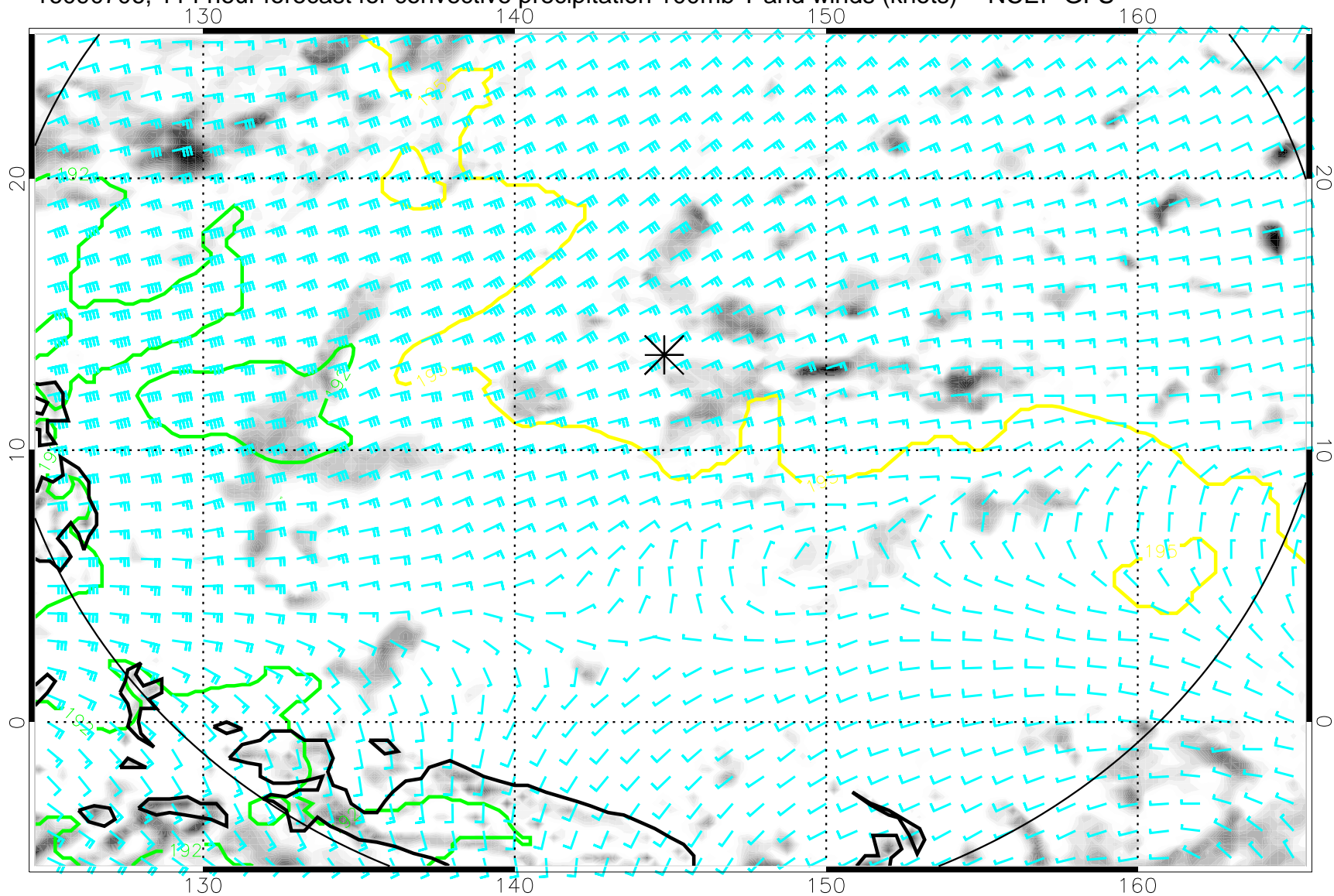
16090706, 114 hour forecast for convective precipitation 100mb T and winds (knots) -- NCEP GFS
