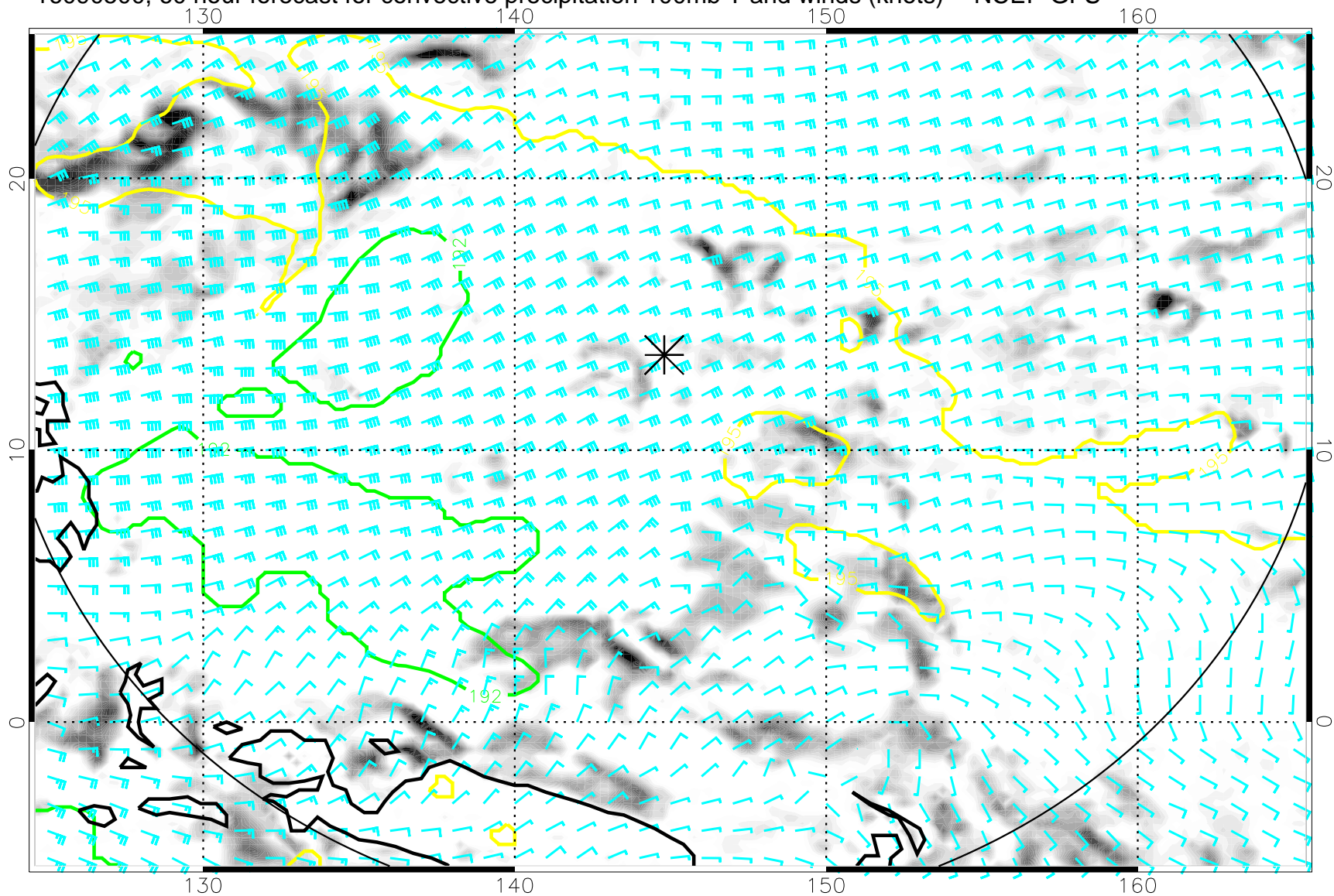
16090500, 60 hour forecast for convective precipitation 100mb T and winds (knots) -- NCEP GFS
