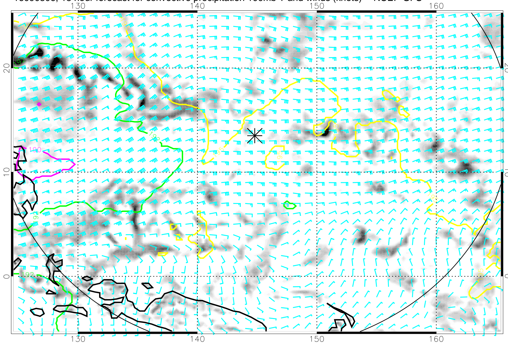
16090306, 18 hour forecast for convective precipitation 100mb T and winds (knots) -- NCEP GFS
