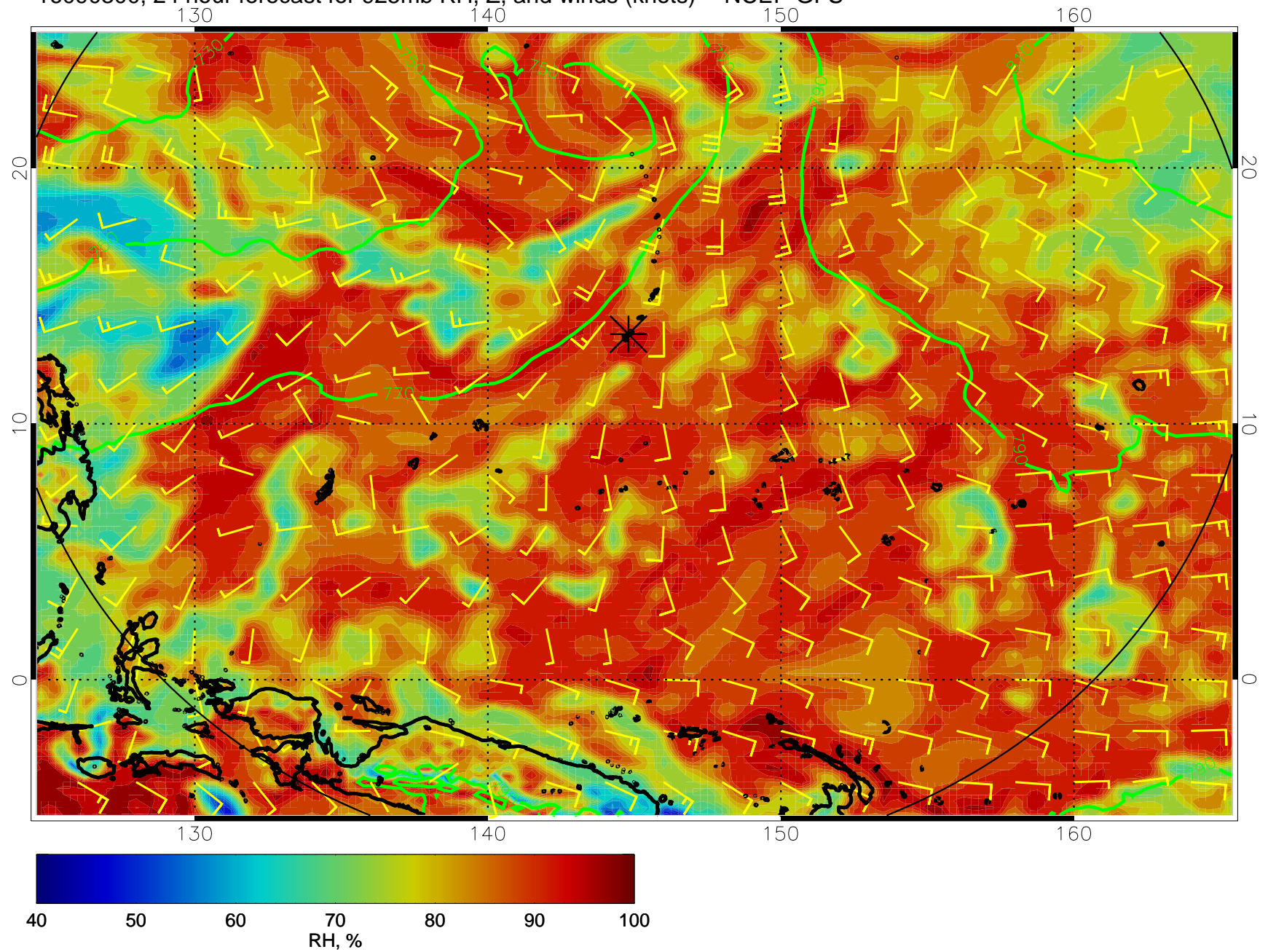
16090300, 24 hour forecast for 925mb RH, Z, and winds (knots) -- NCEP GFS
