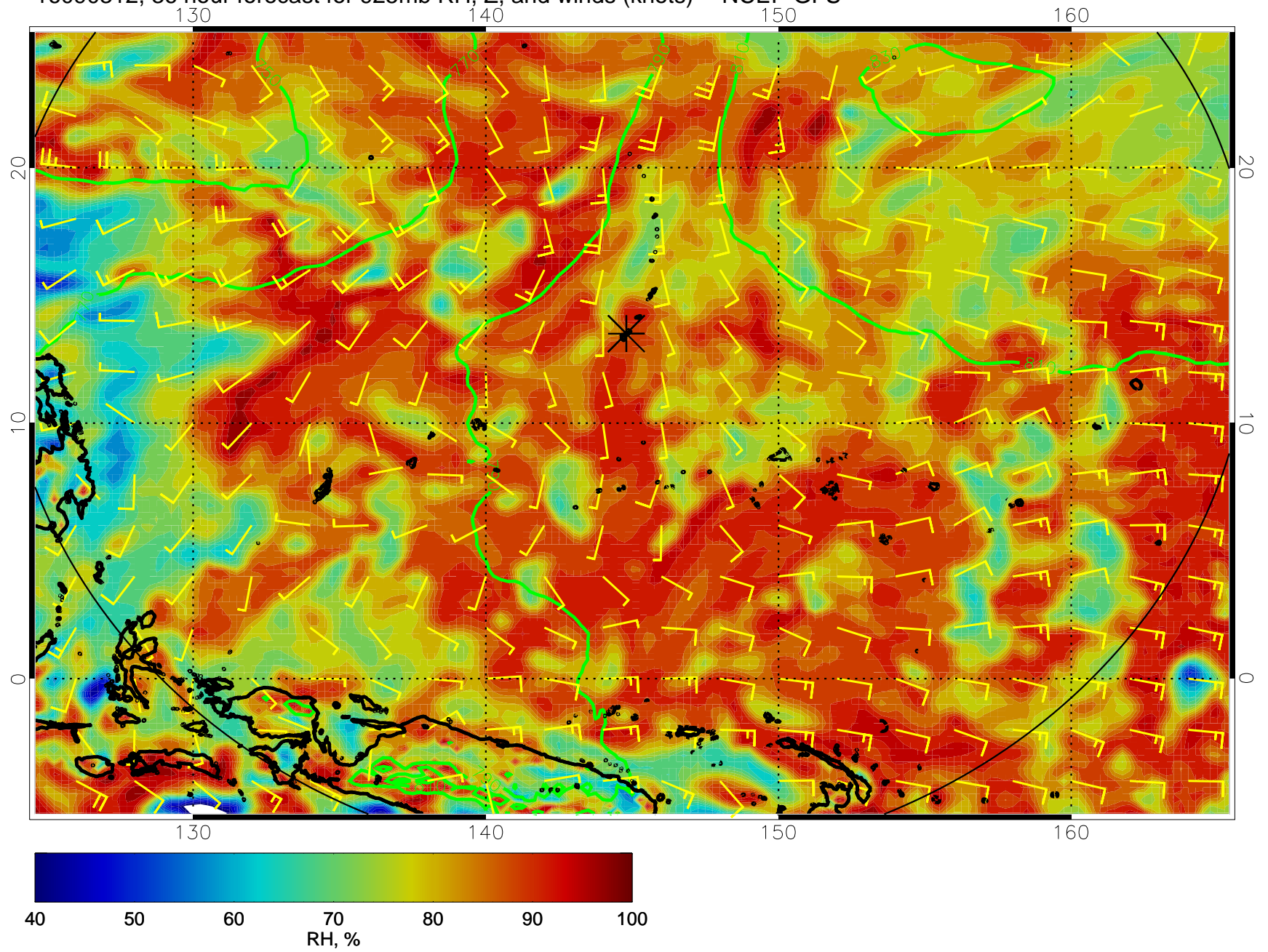
16090312, 36 hour forecast for 925mb RH, Z, and winds (knots) -- NCEP GFS
