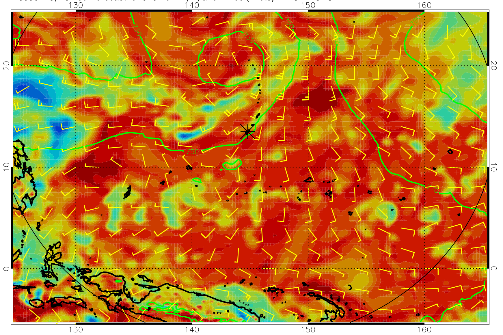
16090218, 18 hour forecast for 925mb RH, Z, and winds (knots) -- NCEP GFS
