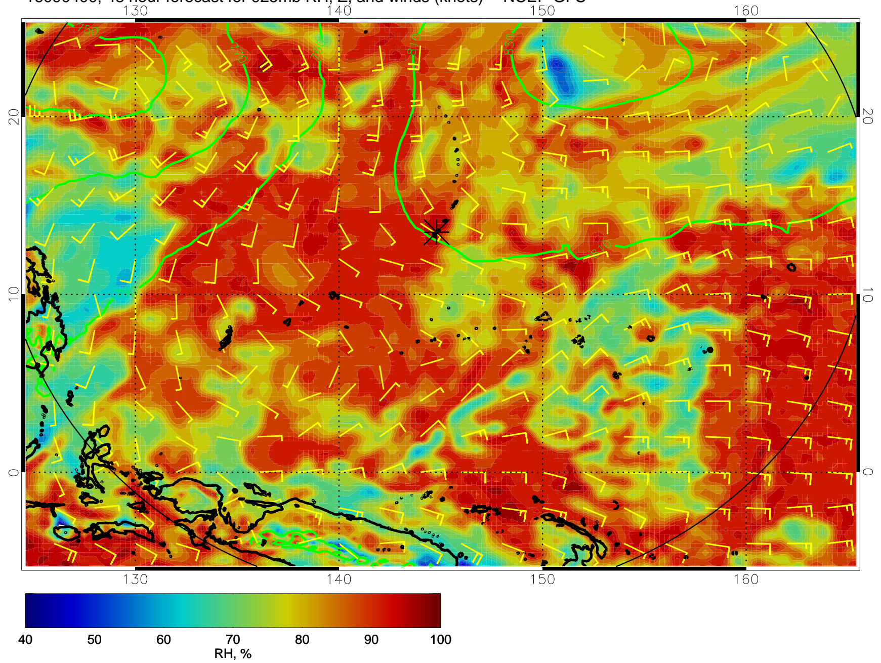
16090400, 48 hour forecast for 925mb RH, Z, and winds (knots) -- NCEP GFS
