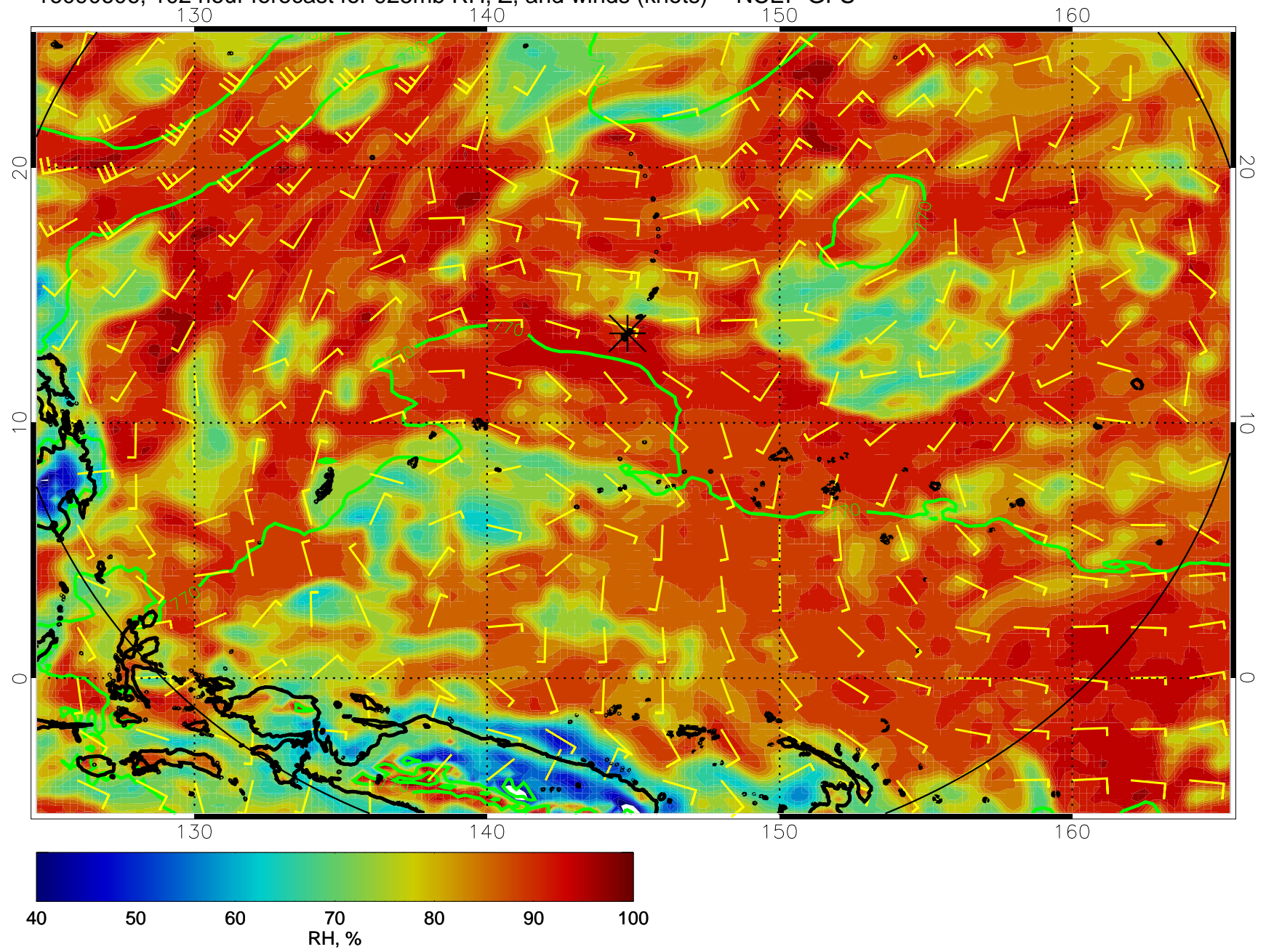
16090606, 102 hour forecast for 925mb RH, Z, and winds (knots) -- NCEP GFS
