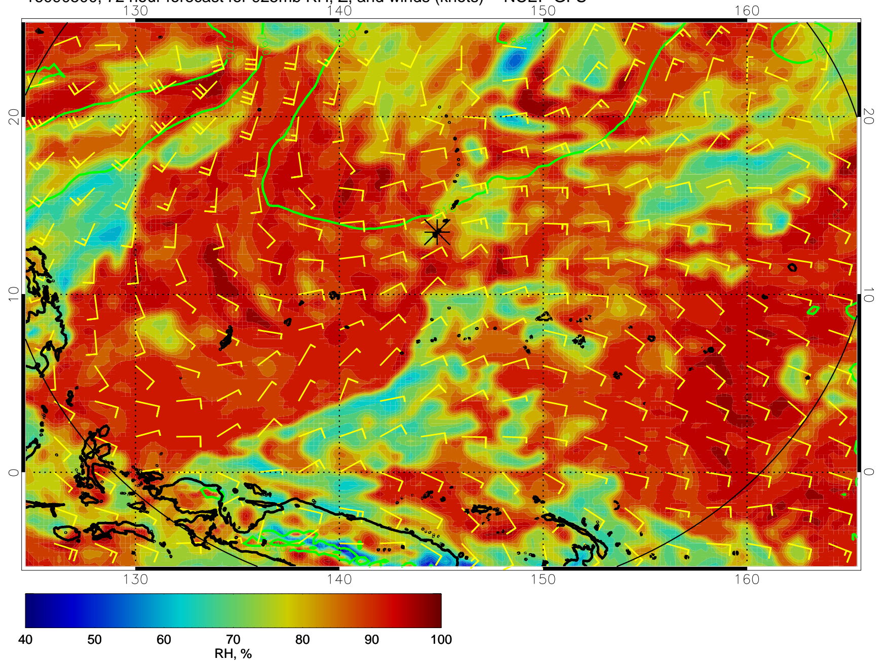
16090500, 72 hour forecast for 925mb RH, Z, and winds (knots) -- NCEP GFS
