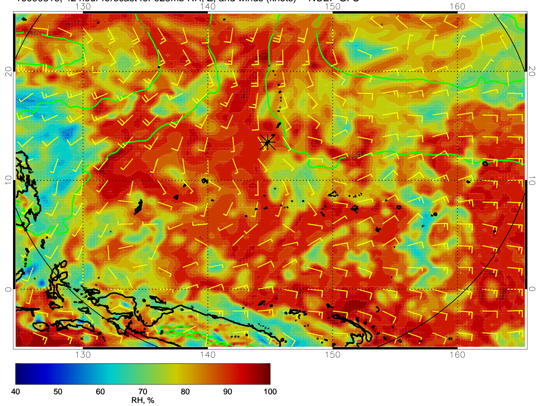
16090318, 42 hour forecast for 925mb RH, Z, and winds (knots) -- NCEP GFS
