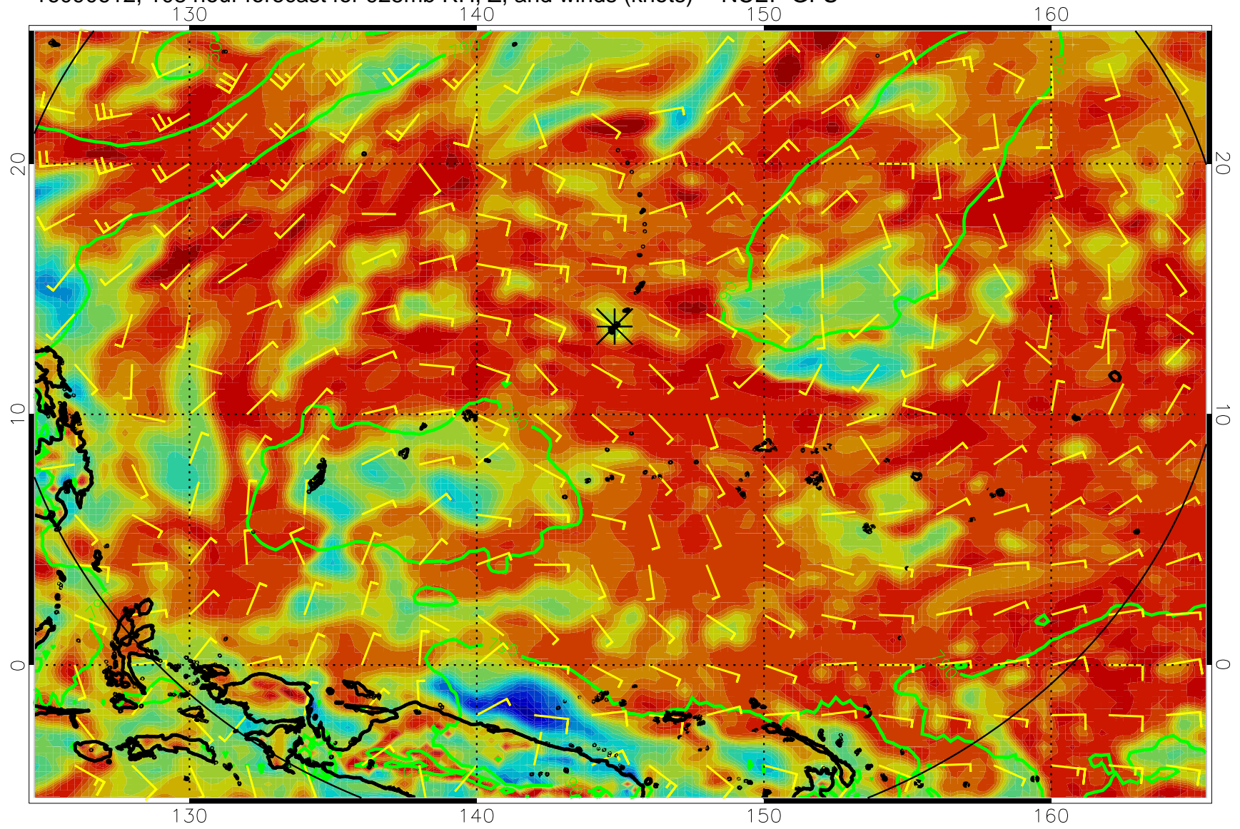
16090612, 108 hour forecast for 925mb RH, Z, and winds (knots) -- NCEP GFS
