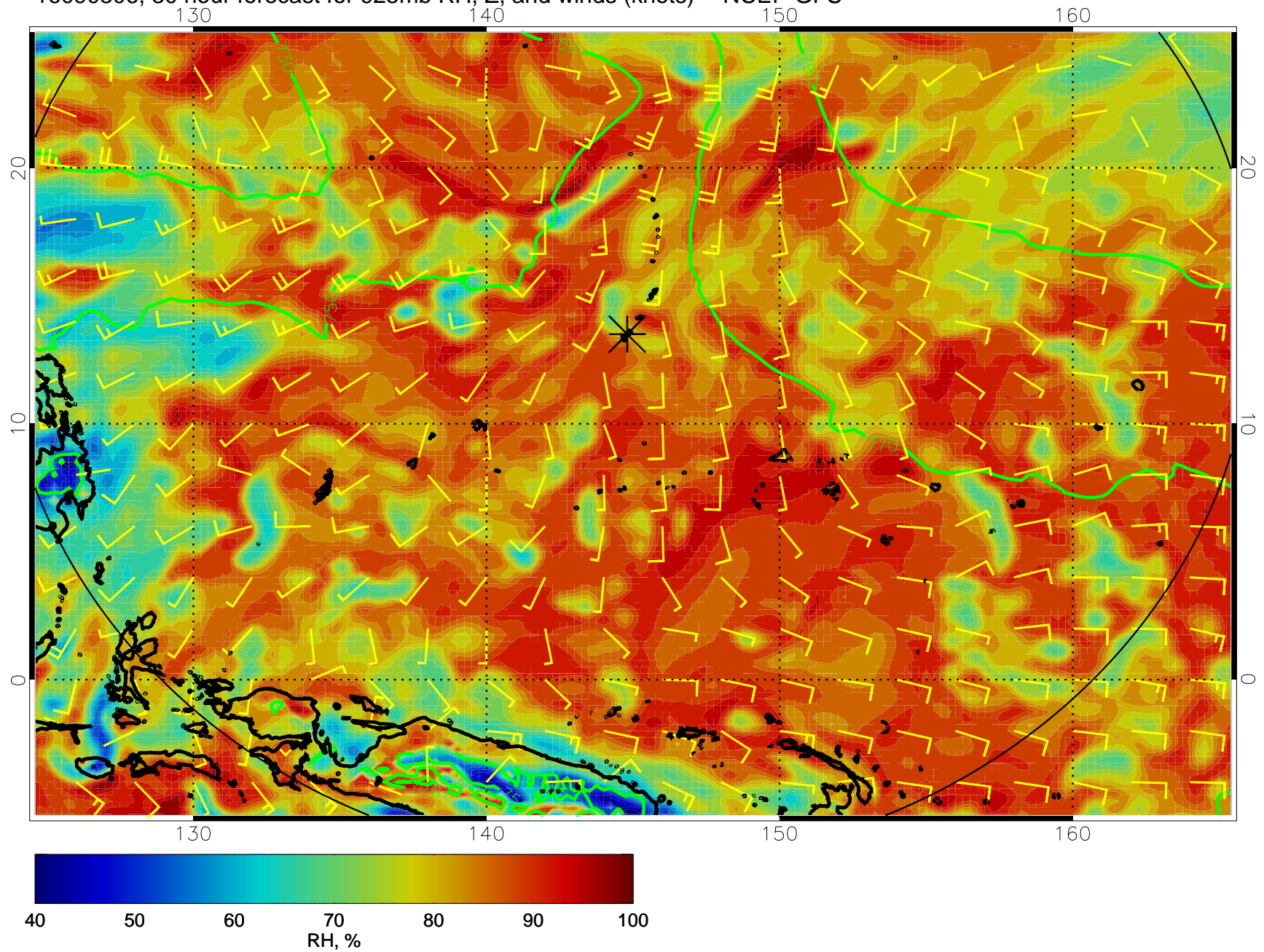
16090306, 30 hour forecast for 925mb RH, Z, and winds (knots) -- NCEP GFS
