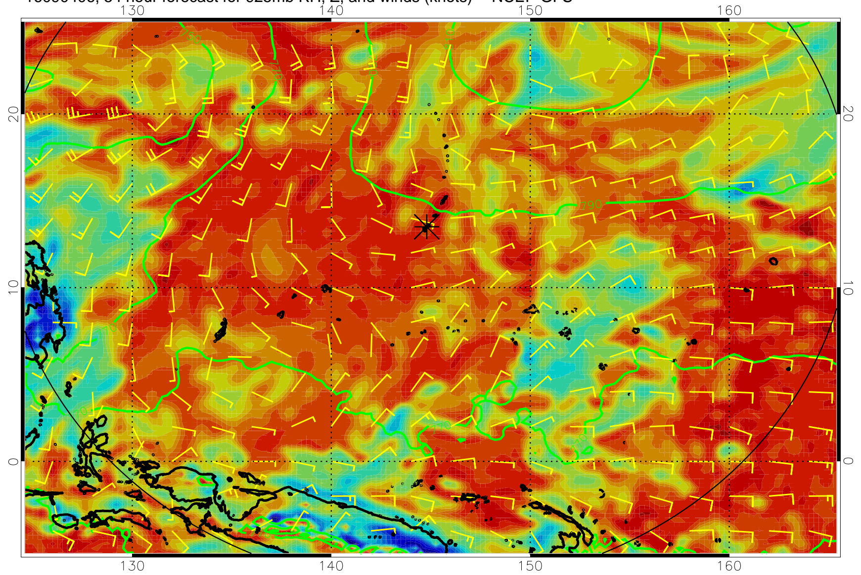
16090406, 54 hour forecast for 925mb RH, Z, and winds (knots) -- NCEP GFS
