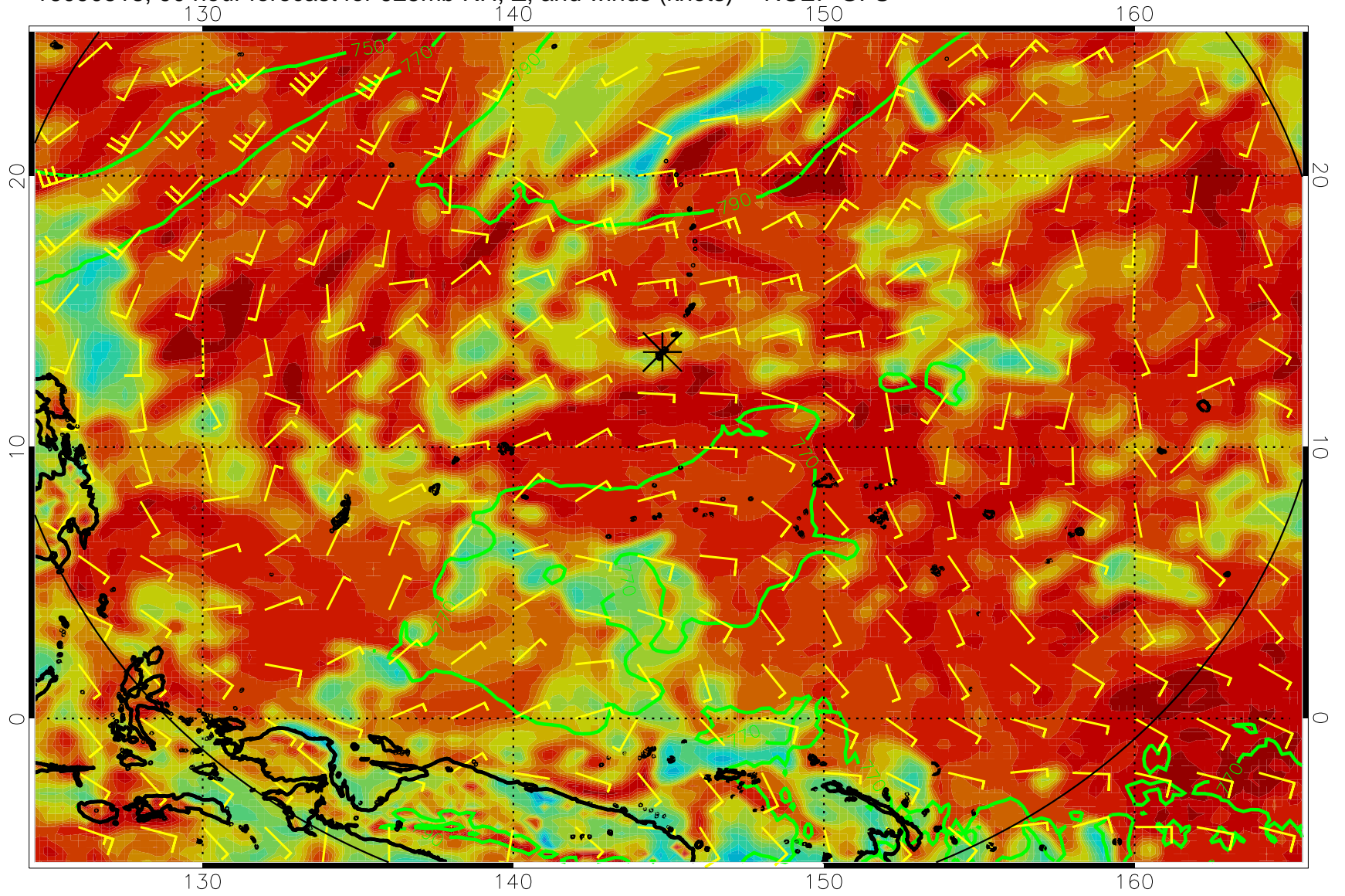
16090518, 90 hour forecast for 925mb RH, Z, and winds (knots) -- NCEP GFS
