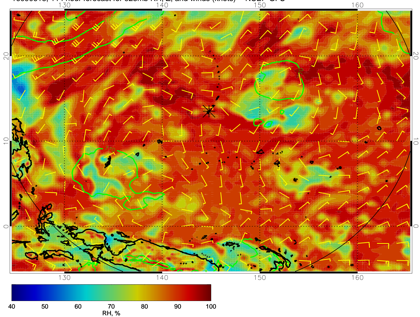
16090618, 114 hour forecast for 925mb RH, Z, and winds (knots) -- NCEP GFS
