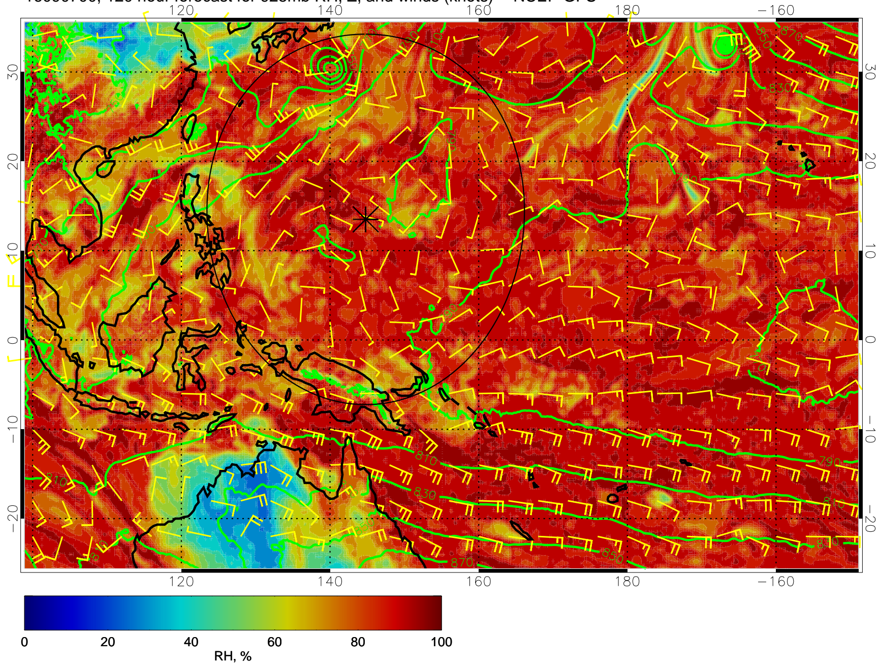
16090700, 120 hour forecast for 925mb RH, Z, and winds (knots) -- NCEP GFS
