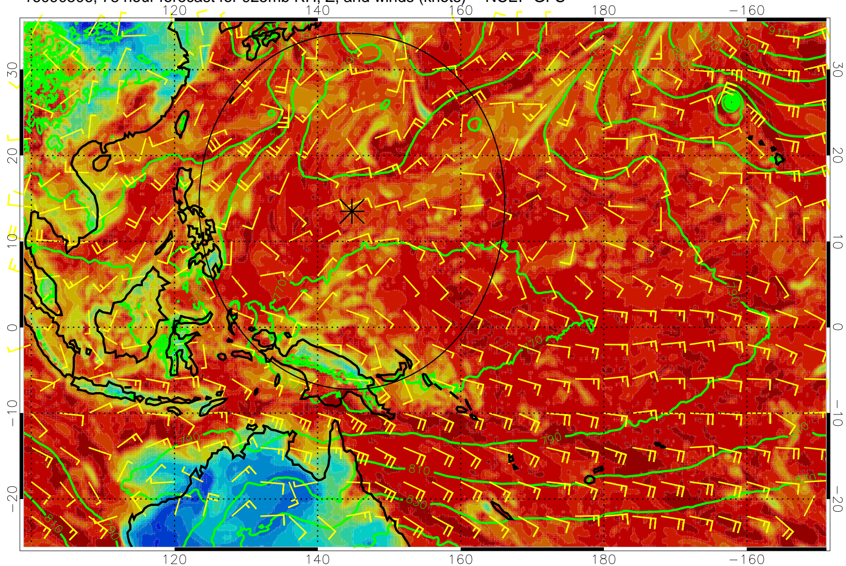
16090506, 78 hour forecast for 925mb RH, Z, and winds (knots) -- NCEP GFS
