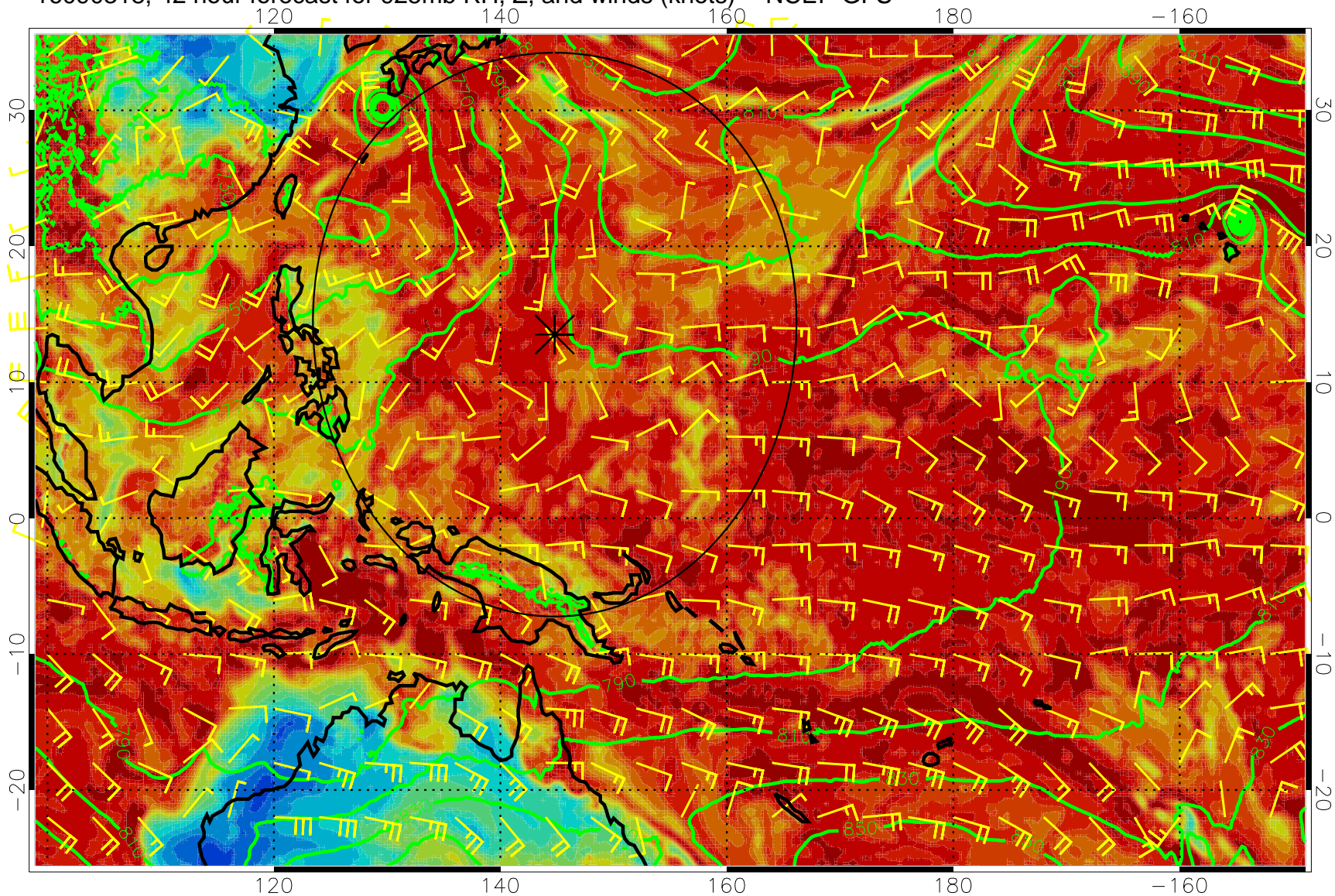
16090318, 42 hour forecast for 925mb RH, Z, and winds (knots) -- NCEP GFS
