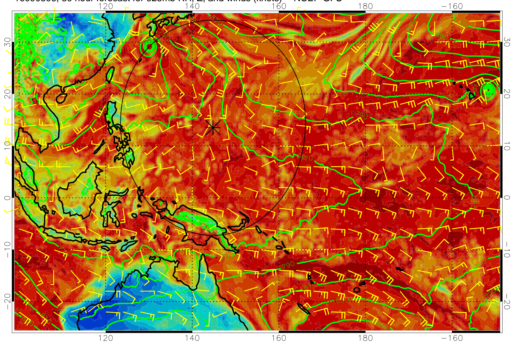
16090306, 30 hour forecast for 925mb RH, Z, and winds (knots) -- NCEP GFS
