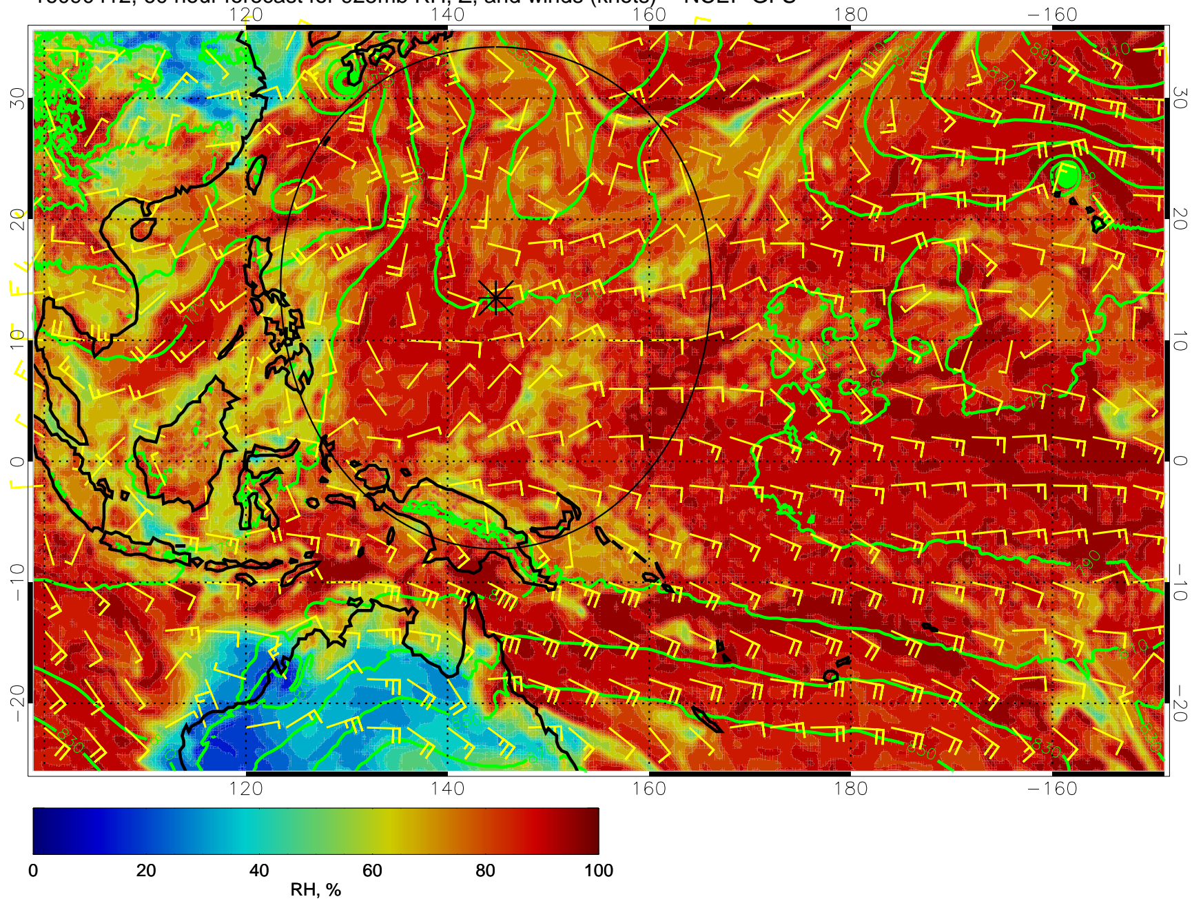
16090412, 60 hour forecast for 925mb RH, Z, and winds (knots) -- NCEP GFS
