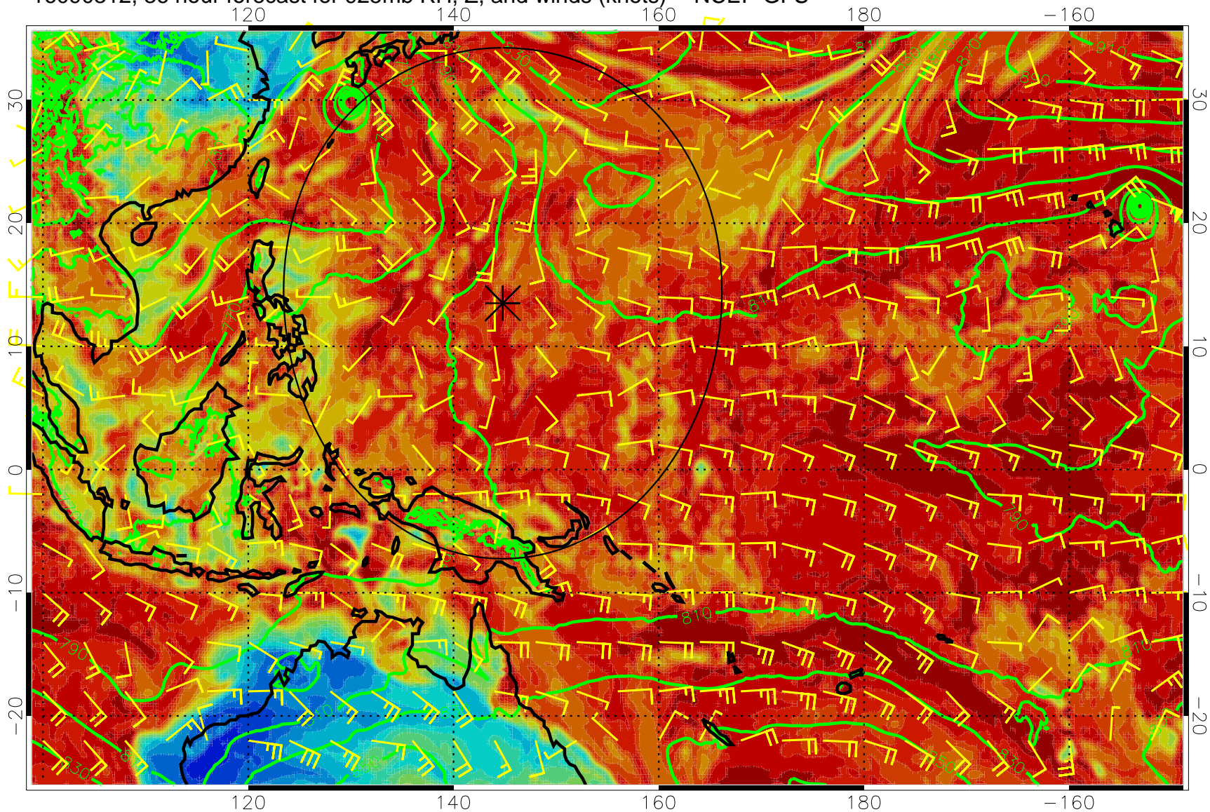
16090312, 36 hour forecast for 925mb RH, Z, and winds (knots) -- NCEP GFS
