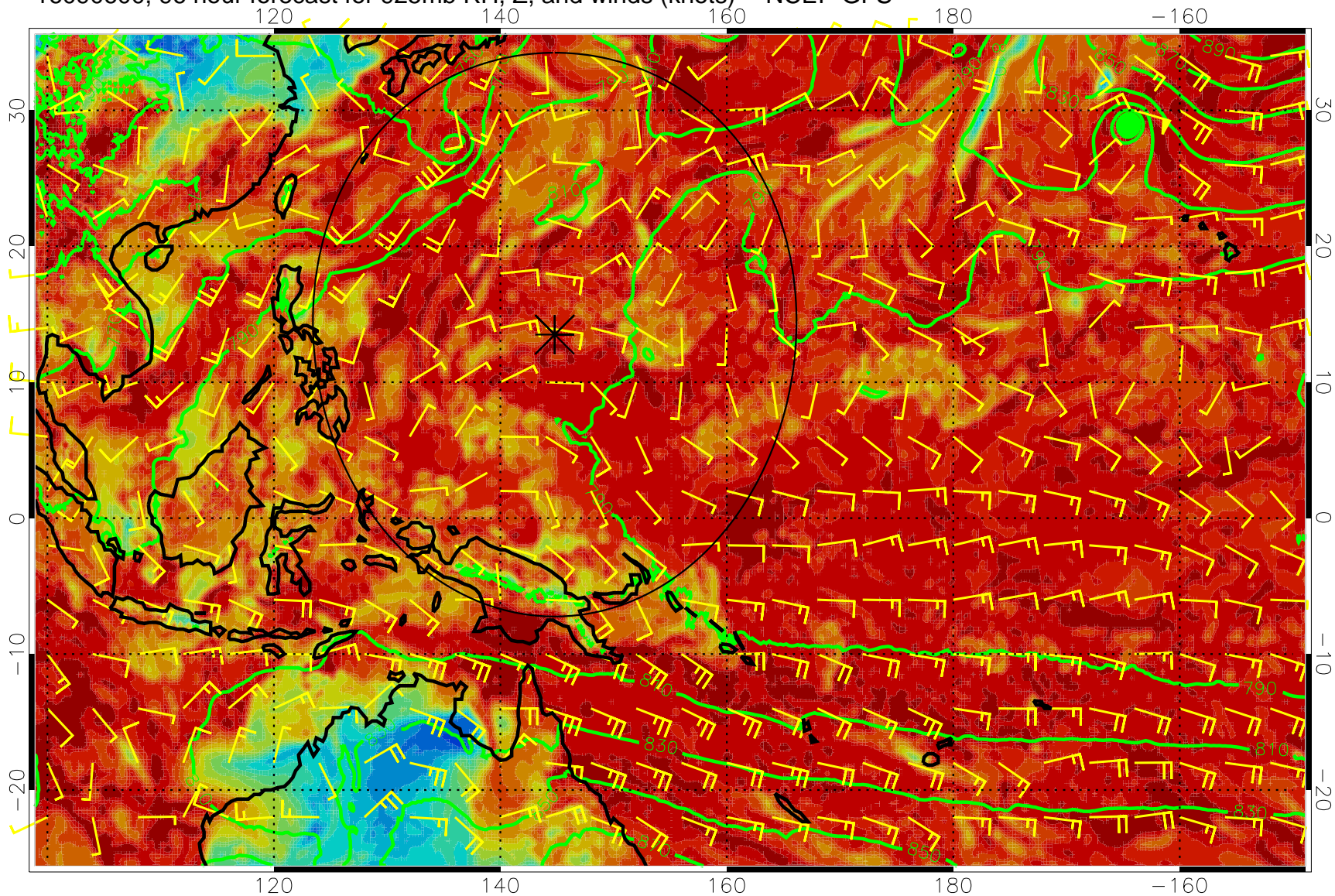
16090600, 96 hour forecast for 925mb RH, Z, and winds (knots) -- NCEP GFS
