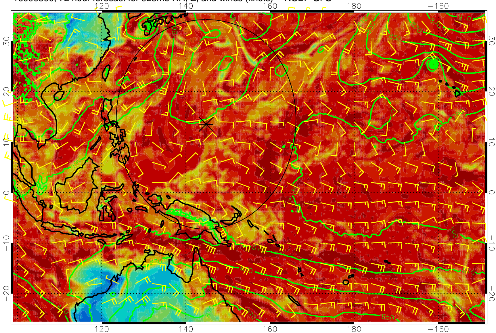
16090500, 72 hour forecast for 925mb RH, Z, and winds (knots) -- NCEP GFS
