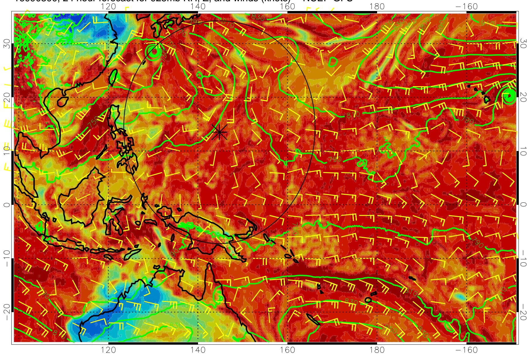
16090300, 24 hour forecast for 925mb RH, Z, and winds (knots) -- NCEP GFS
