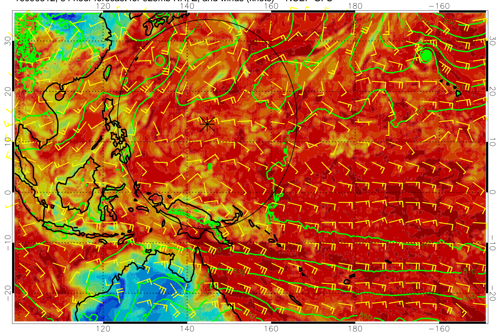
16090512, 84 hour forecast for 925mb RH, Z, and winds (knots) -- NCEP GFS
