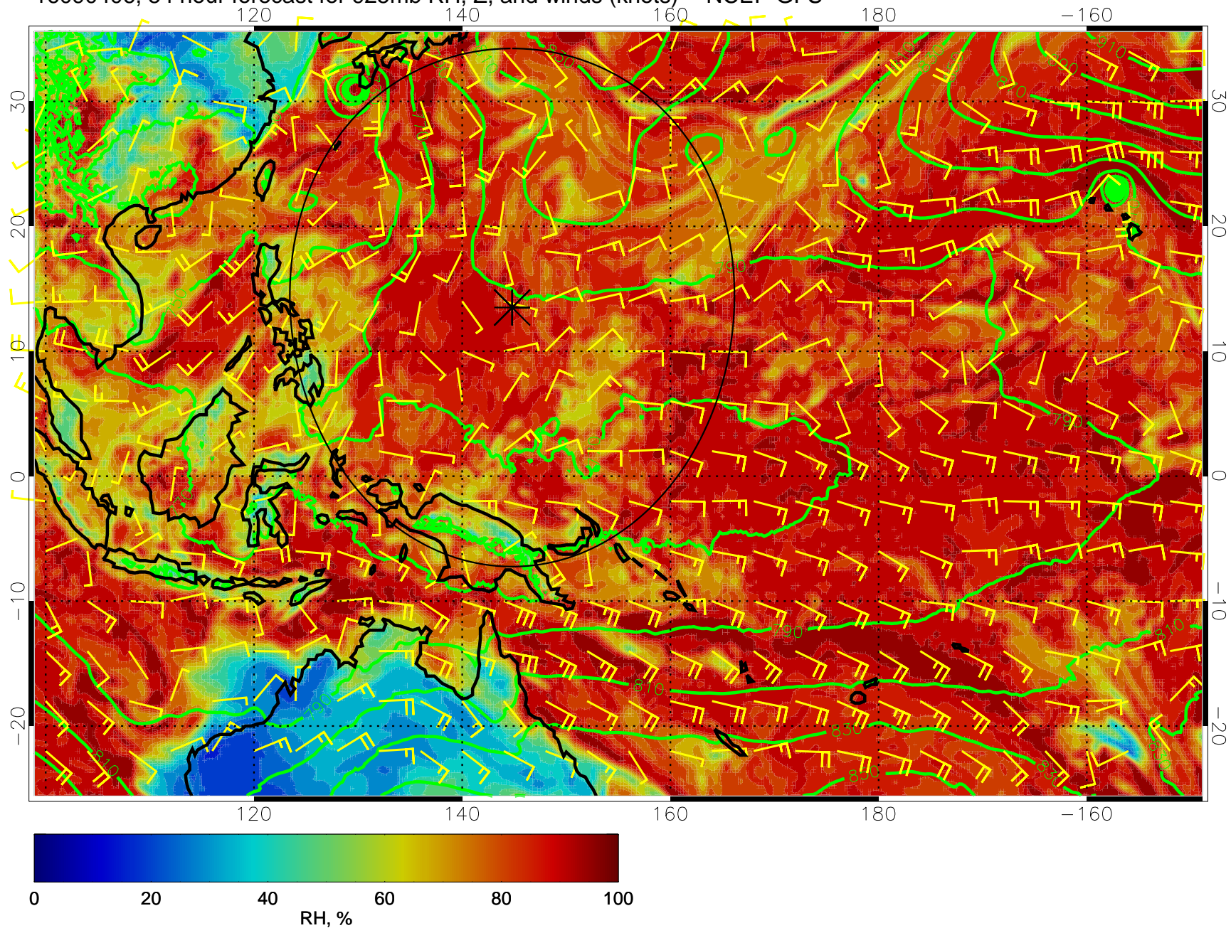
16090406, 54 hour forecast for 925mb RH, Z, and winds (knots) -- NCEP GFS
