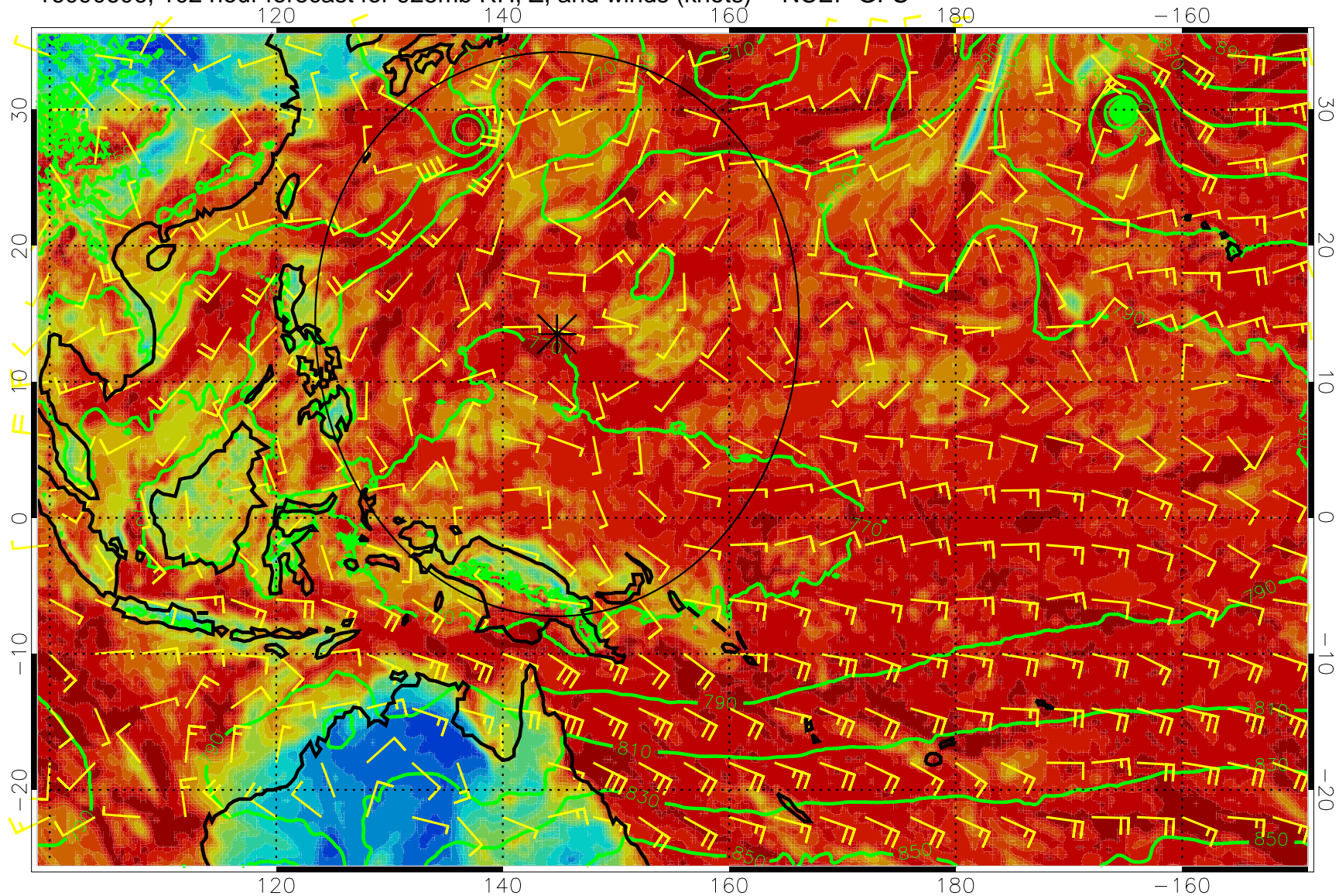
16090606, 102 hour forecast for 925mb RH, Z, and winds (knots) -- NCEP GFS
