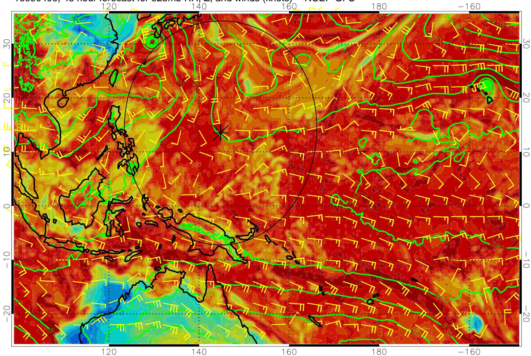
16090400, 48 hour forecast for 925mb RH, Z, and winds (knots) -- NCEP GFS
