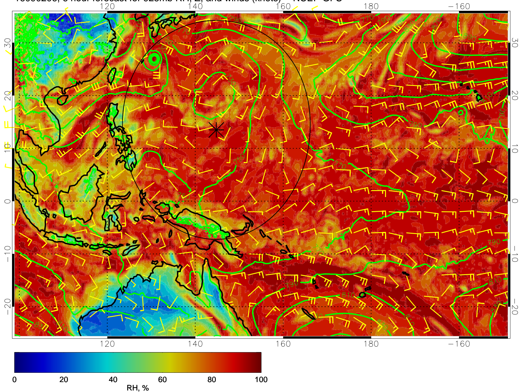
16090206, 6 hour forecast for 925mb RH, Z, and winds (knots) -- NCEP GFS
