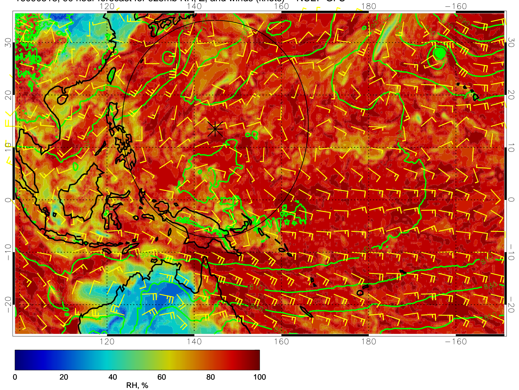
16090518, 90 hour forecast for 925mb RH, Z, and winds (knots) -- NCEP GFS
