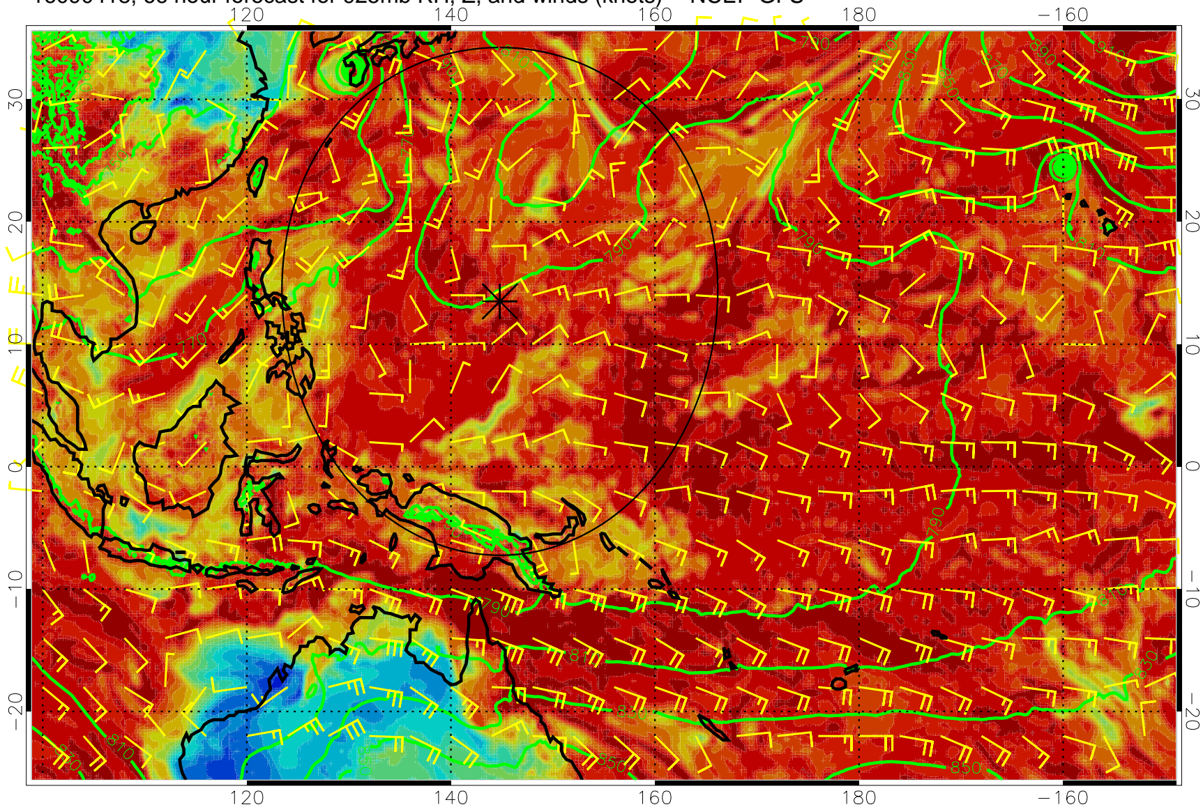
16090418, 66 hour forecast for 925mb RH, Z, and winds (knots) -- NCEP GFS
