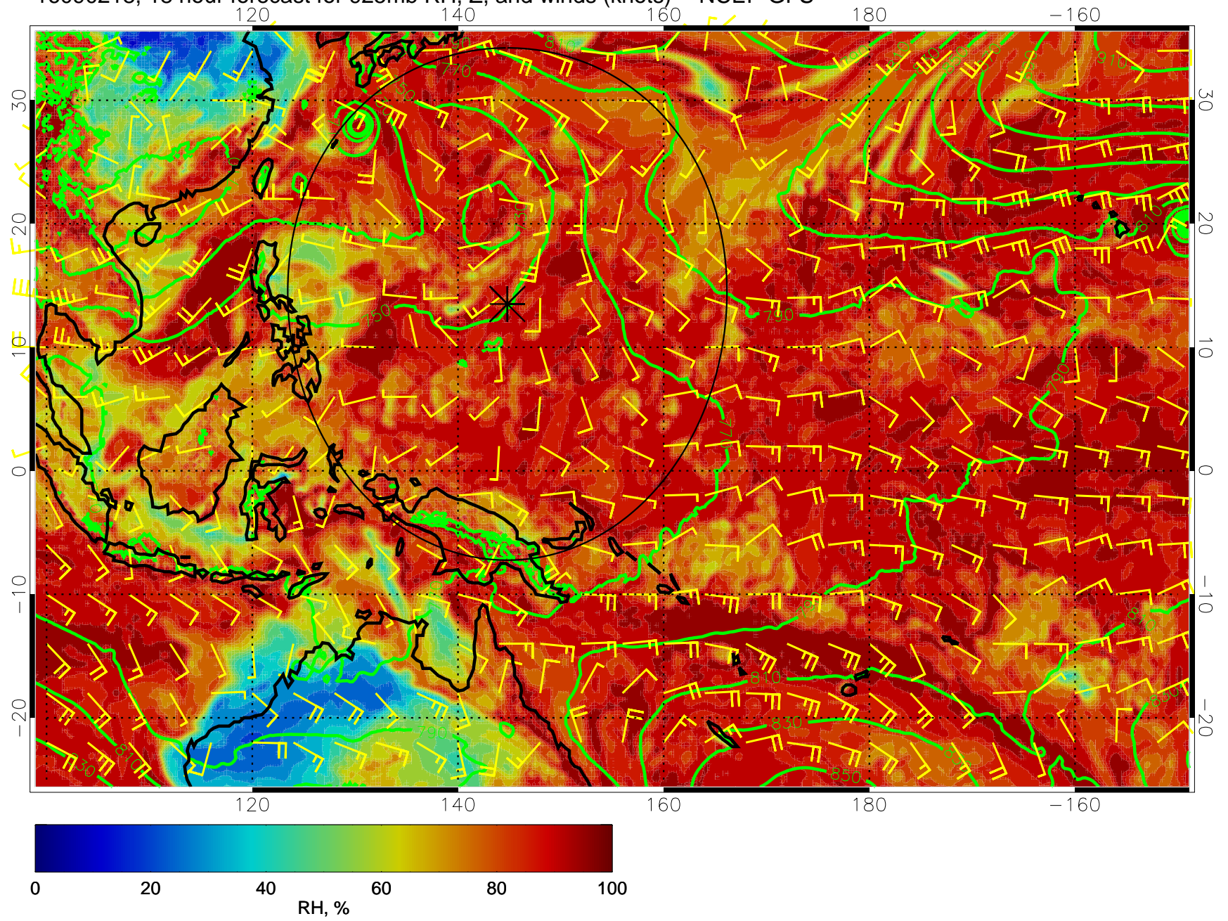
16090218, 18 hour forecast for 925mb RH, Z, and winds (knots) -- NCEP GFS
