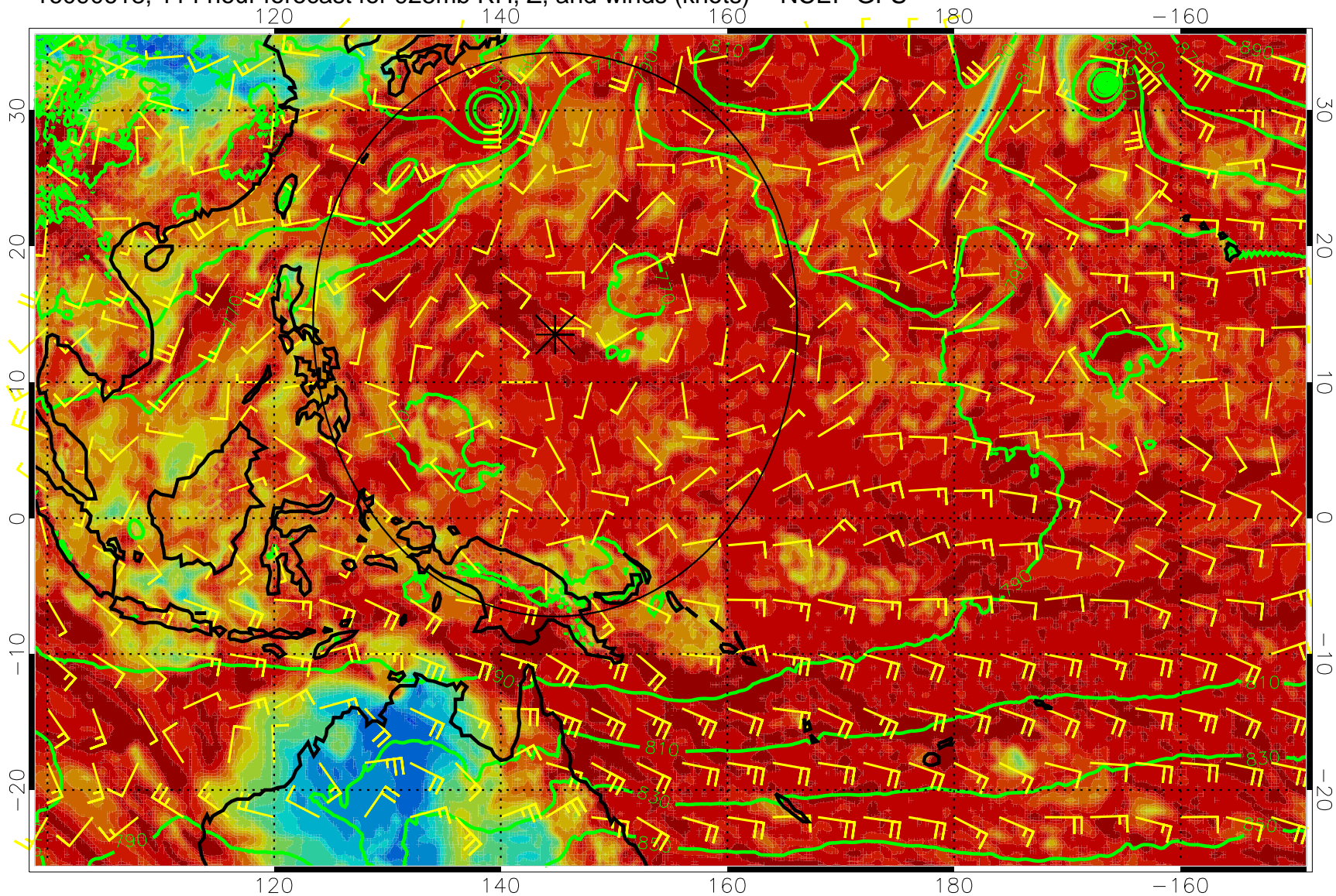
16090618, 114 hour forecast for 925mb RH, Z, and winds (knots) -- NCEP GFS
