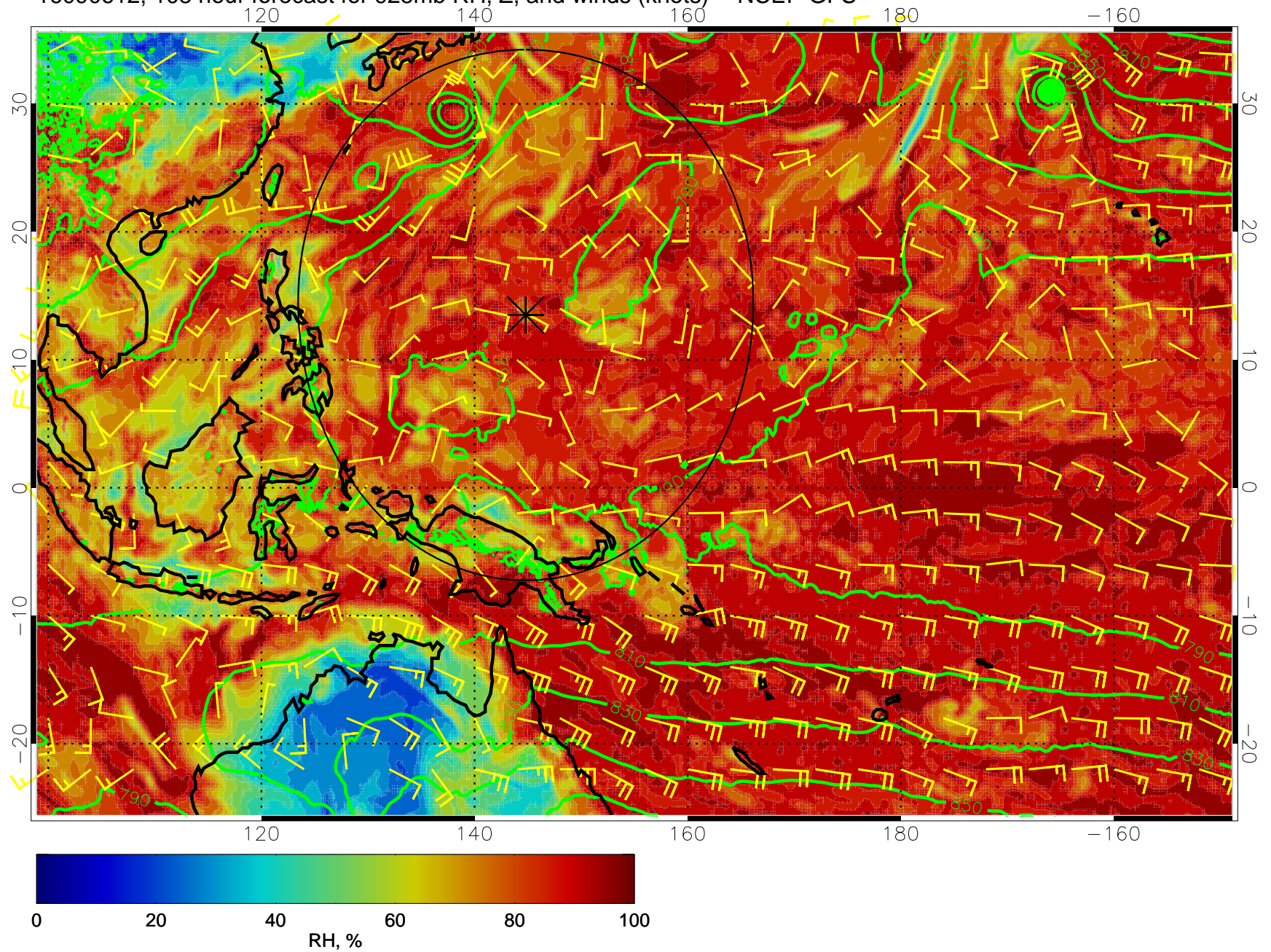
16090612, 108 hour forecast for 925mb RH, Z, and winds (knots) -- NCEP GFS
