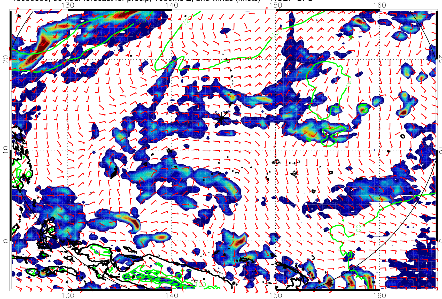
16090600, 96 hour forecast for precip, 1000mb Z, and winds (knots) -- NCEP GFS
