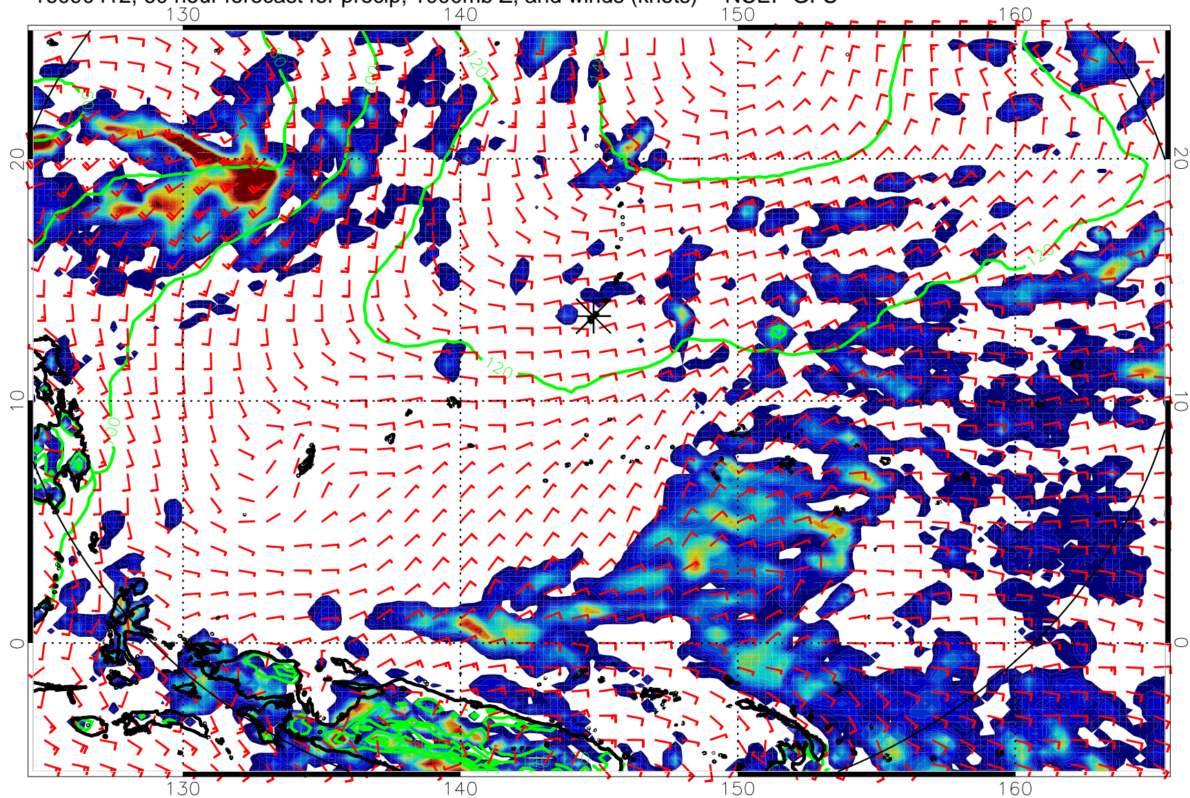
16090412, 60 hour forecast for precip, 1000mb Z, and winds (knots) -- NCEP GFS
