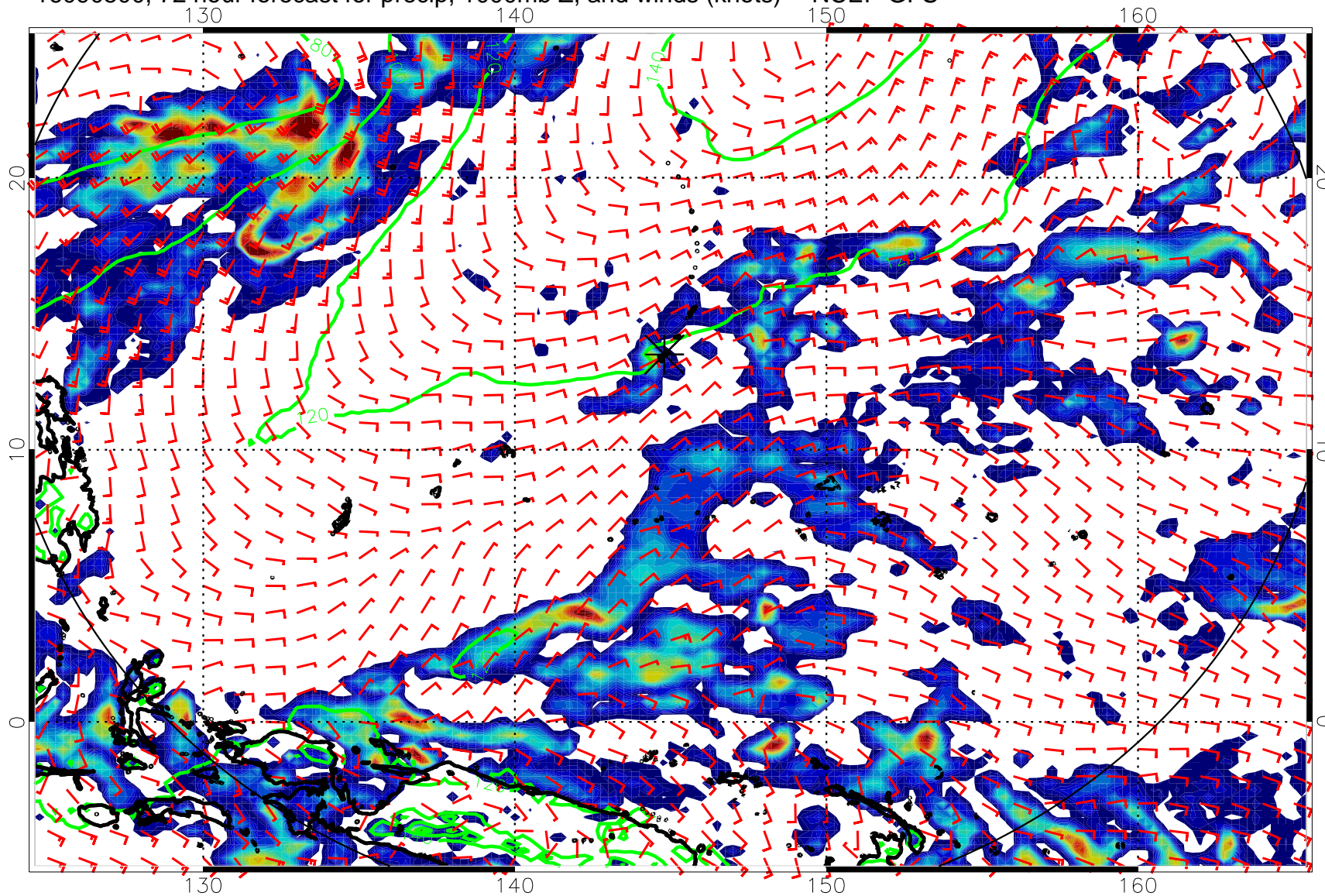
16090500, 72 hour forecast for precip, 1000mb Z, and winds (knots) -- NCEP GFS
