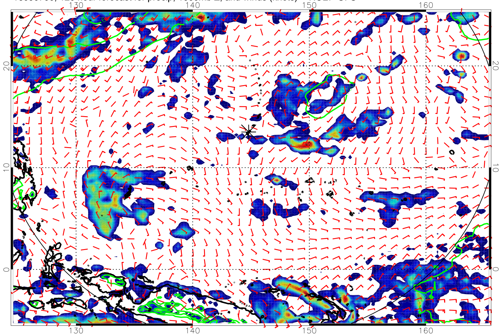
16090700, 120 hour forecast for precip, 1000mb Z, and winds (knots) -- NCEP GFS
