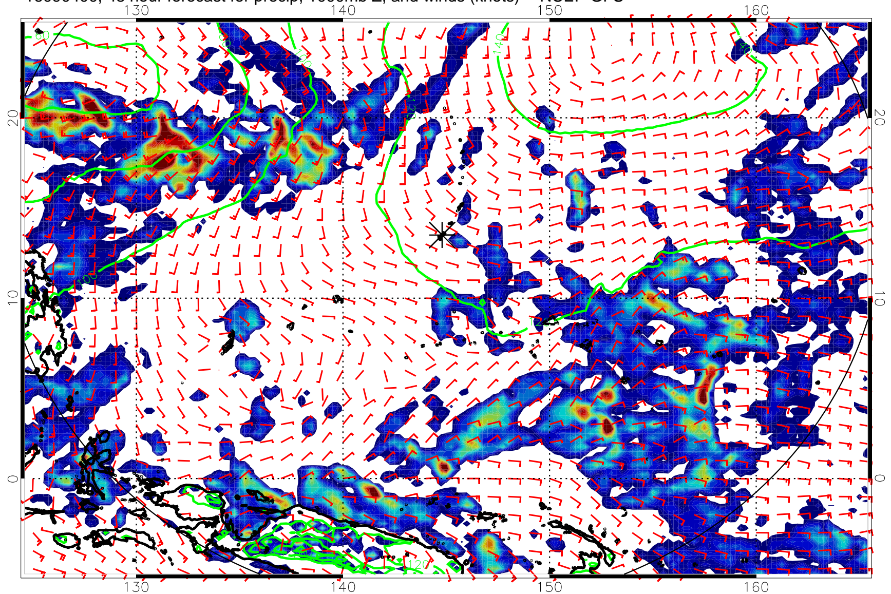
16090400, 48 hour forecast for precip, 1000mb Z, and winds (knots) -- NCEP GFS
