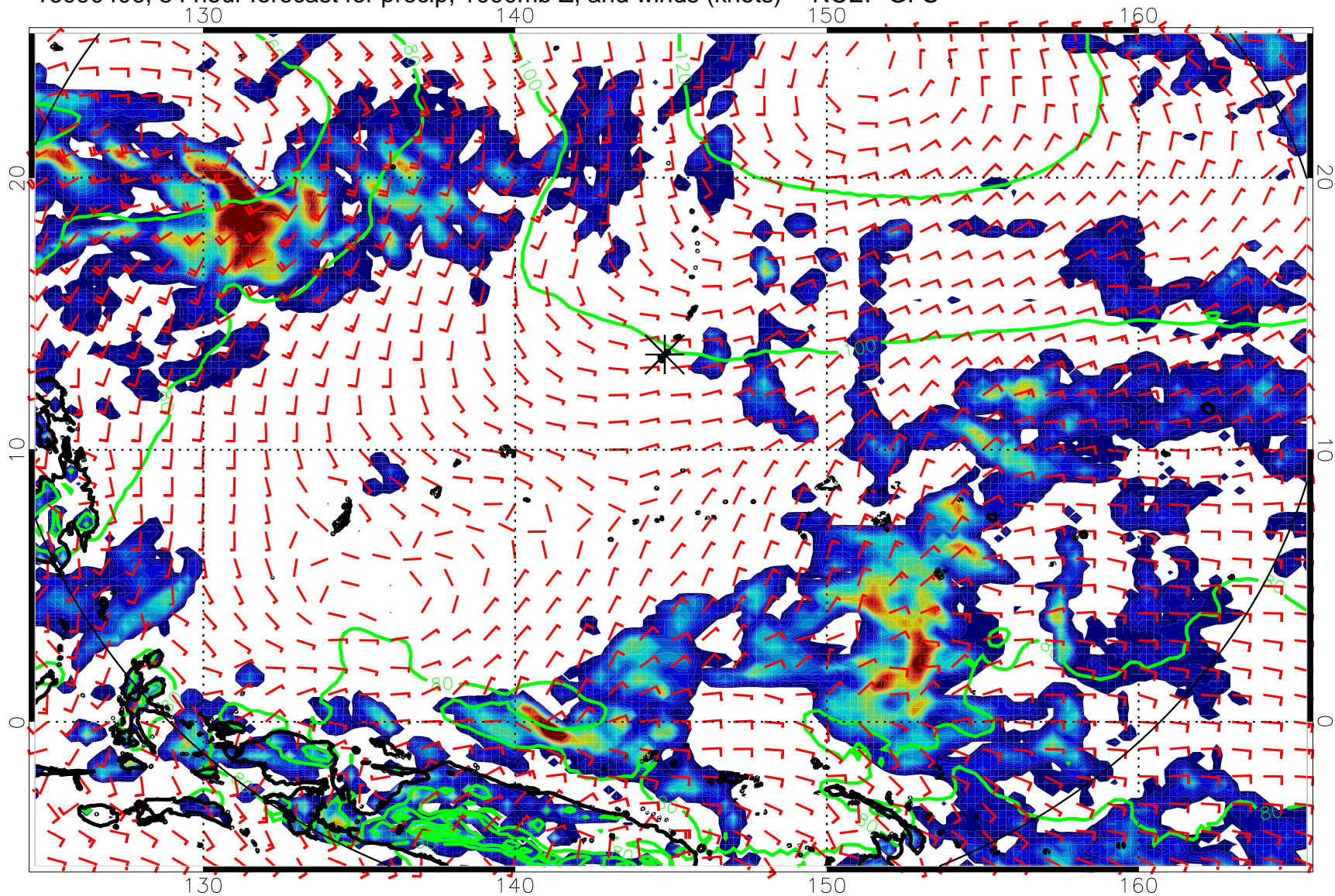
16090406, 54 hour forecast for precip, 1000mb Z, and winds (knots) -- NCEP GFS
