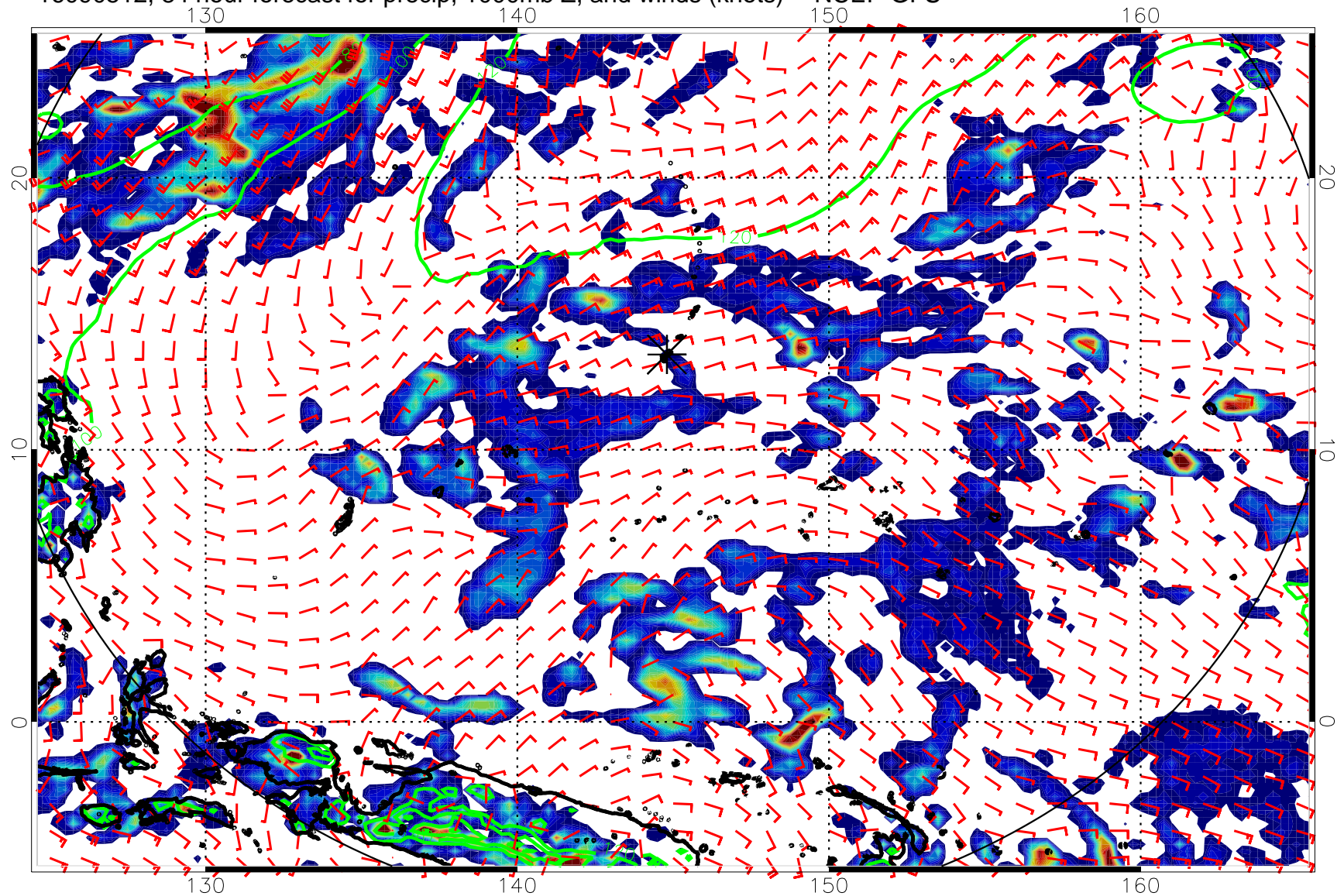
16090512, 84 hour forecast for precip, 1000mb Z, and winds (knots) -- NCEP GFS
