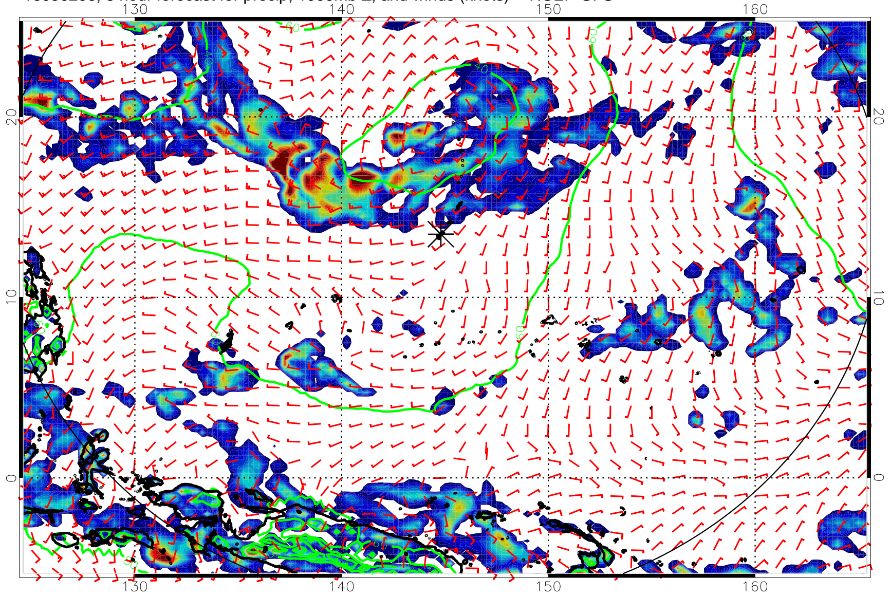
16090206, 6 hour forecast for precip, 1000mb Z, and winds (knots) -- NCEP GFS
