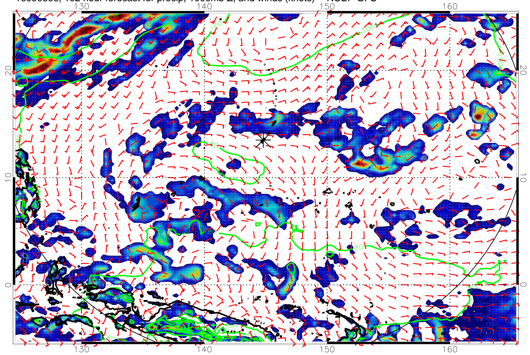
16090606, 102 hour forecast for precip, 1000mb Z, and winds (knots) -- NCEP GFS
