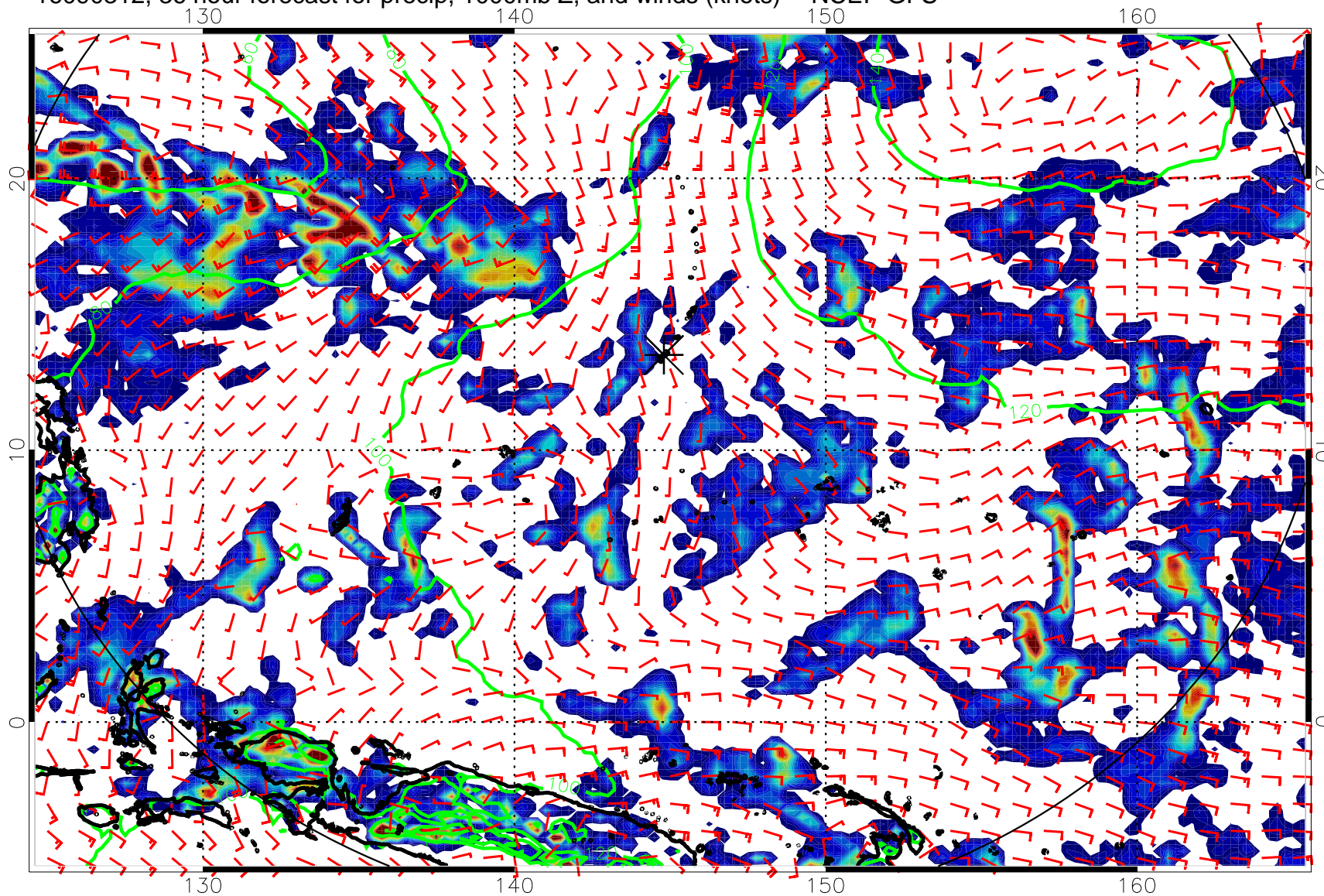
16090312, 36 hour forecast for precip, 1000mb Z, and winds (knots) -- NCEP GFS
