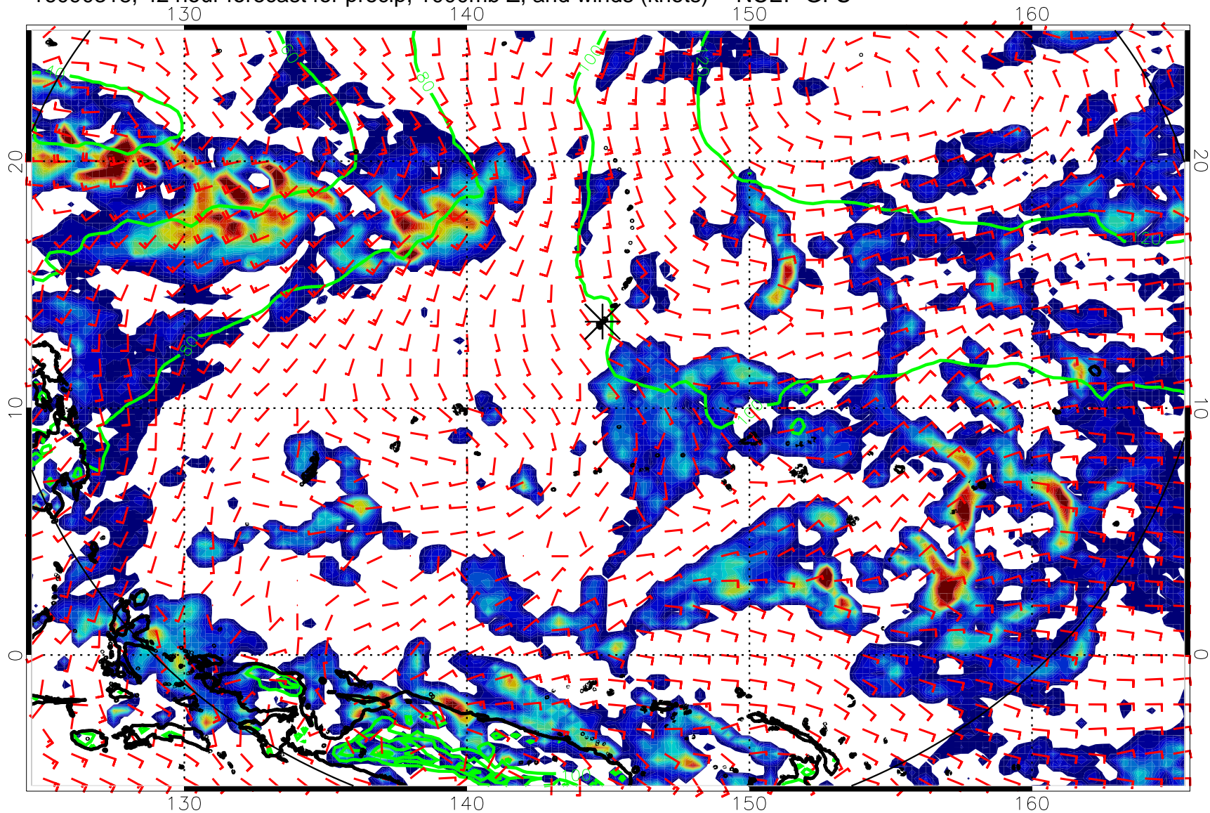
16090318, 42 hour forecast for precip, 1000mb Z, and winds (knots) -- NCEP GFS
