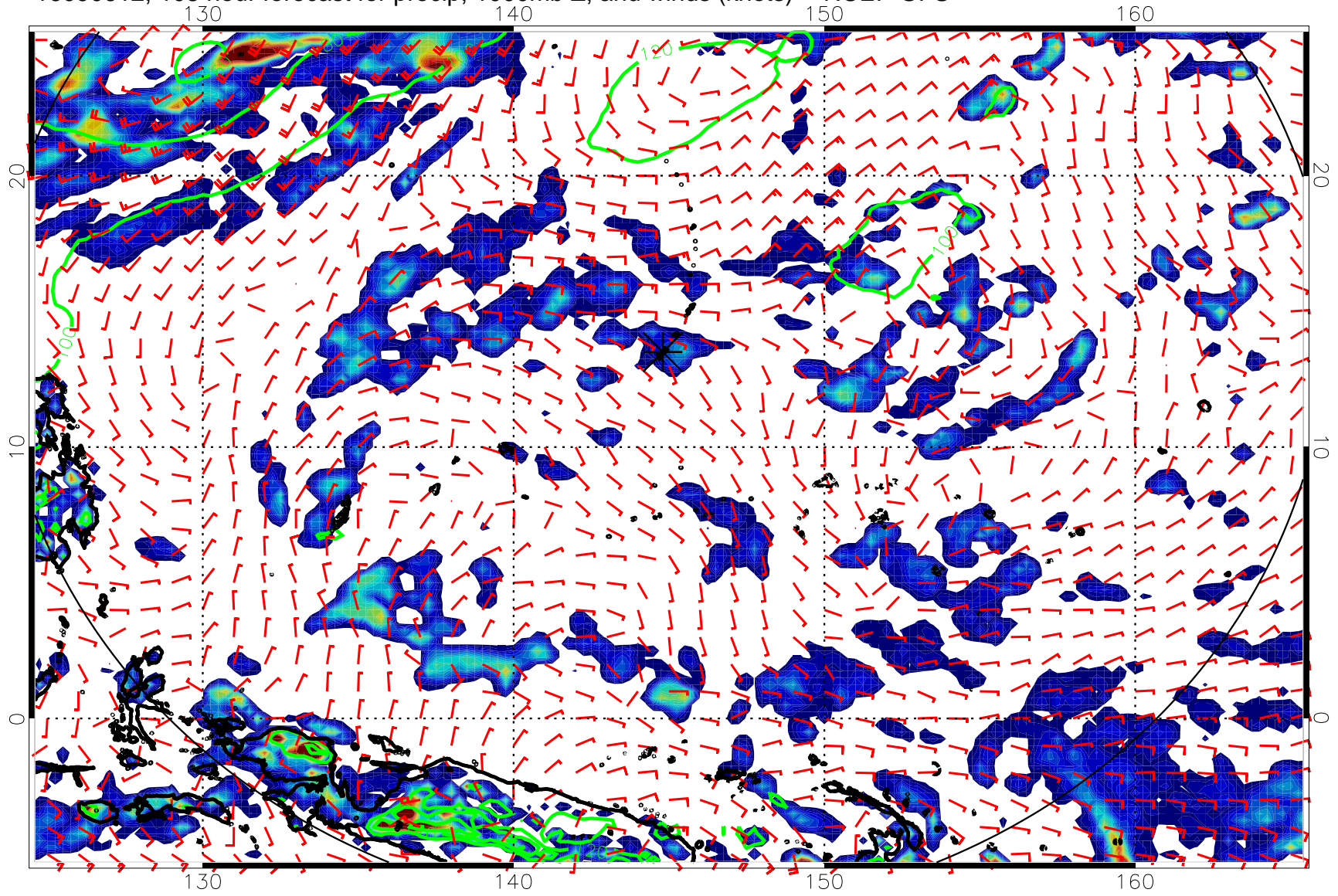
16090612, 108 hour forecast for precip, 1000mb Z, and winds (knots) -- NCEP GFS
