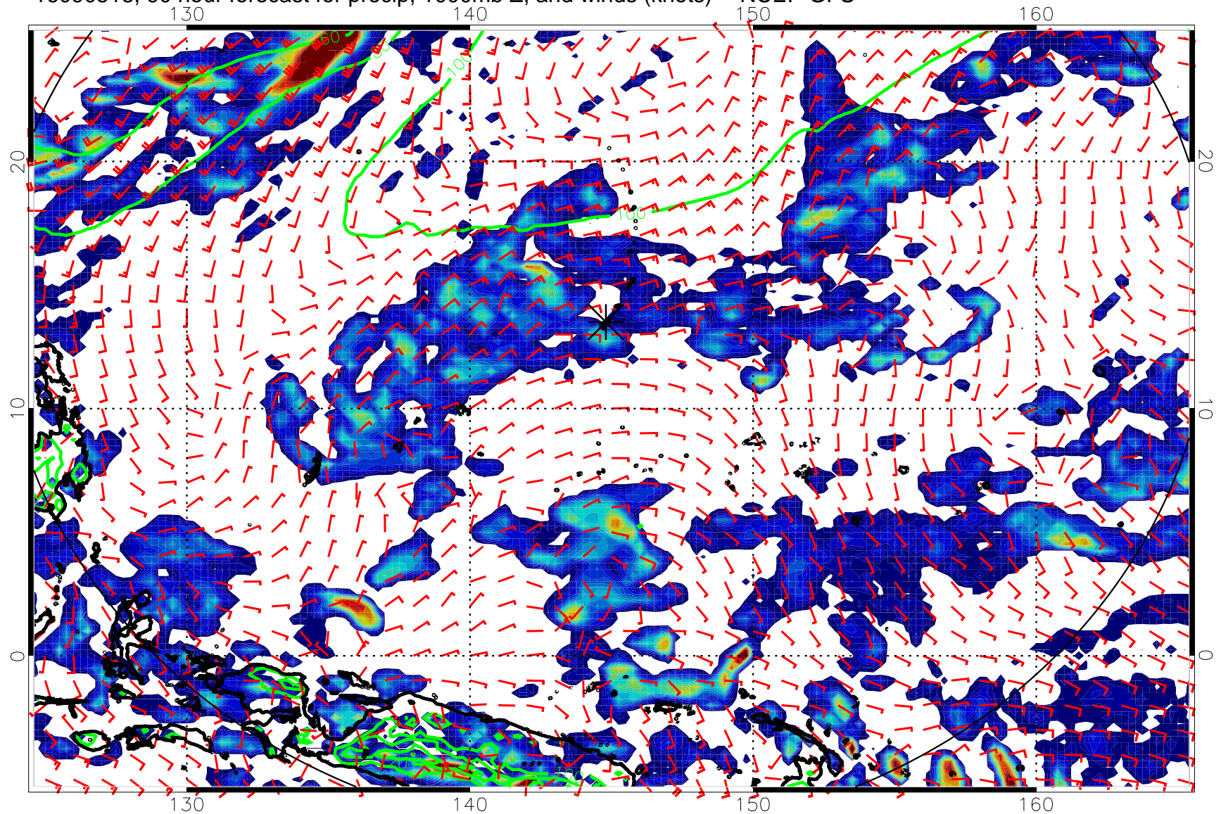
16090518, 90 hour forecast for precip, 1000mb Z, and winds (knots) -- NCEP GFS
