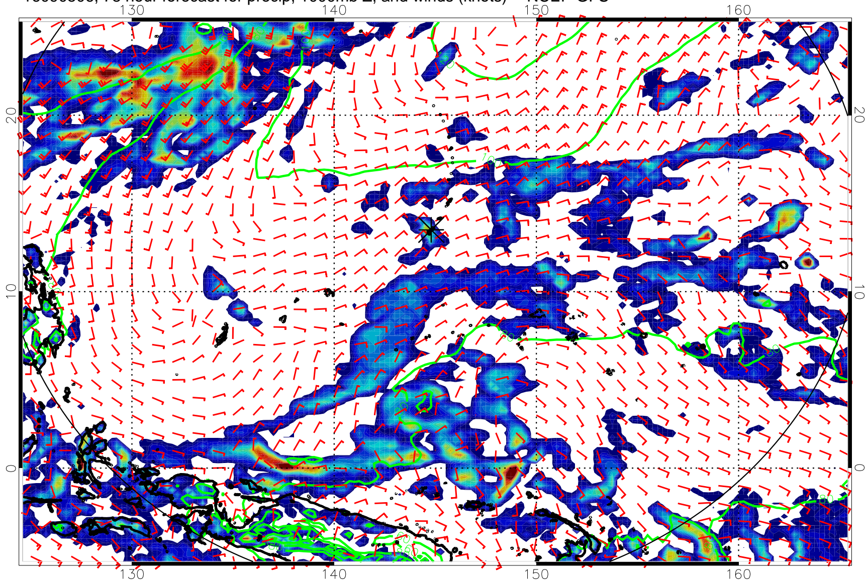
16090506, 78 hour forecast for precip, 1000mb Z, and winds (knots) -- NCEP GFS
