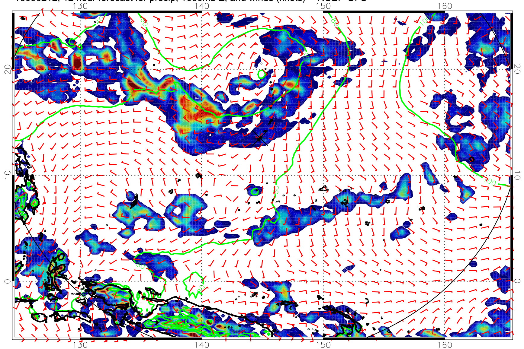
16090212, 12 hour forecast for precip, 1000mb Z, and winds (knots) -- NCEP GFS
