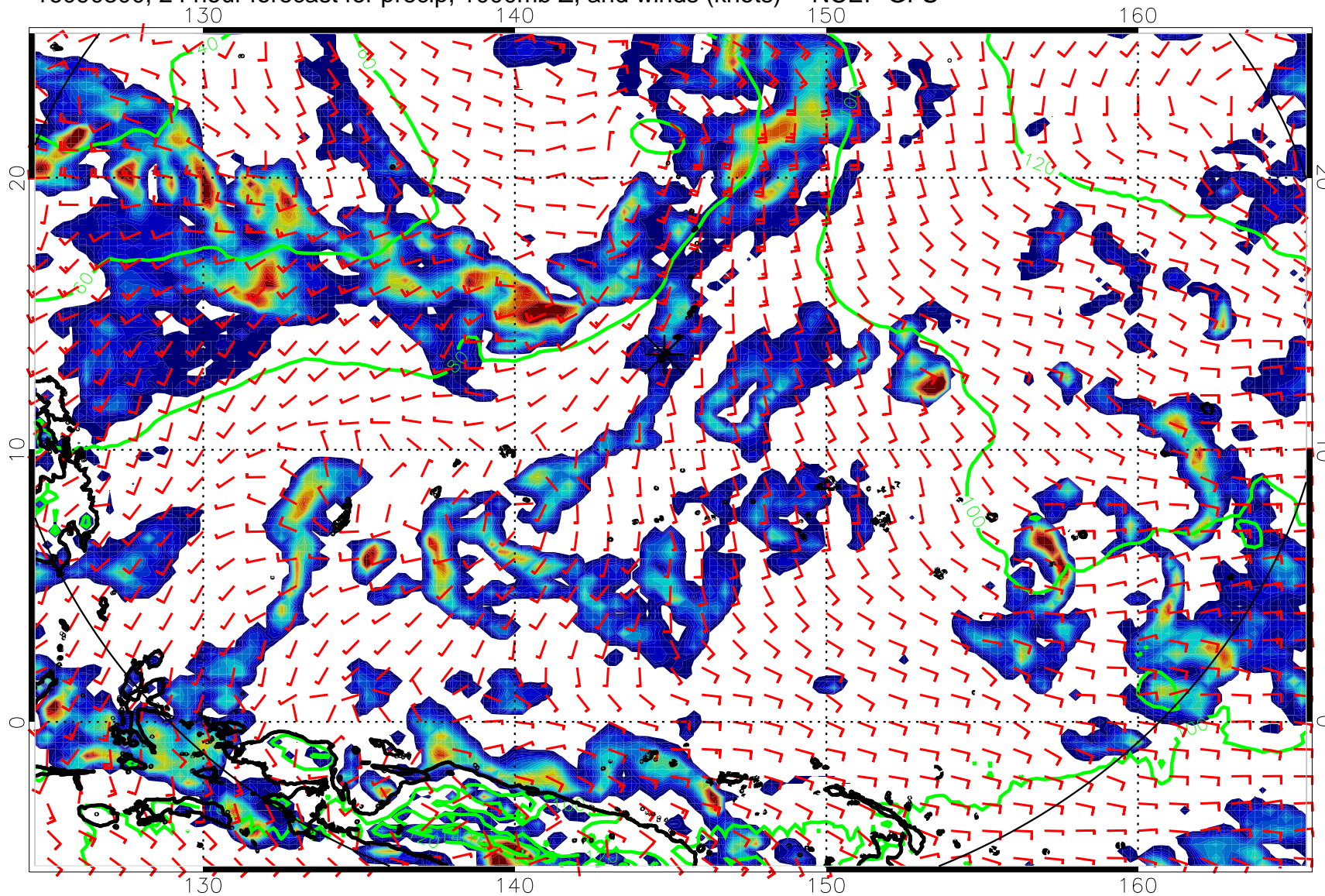
16090300, 24 hour forecast for precip, 1000mb Z, and winds (knots) -- NCEP GFS
