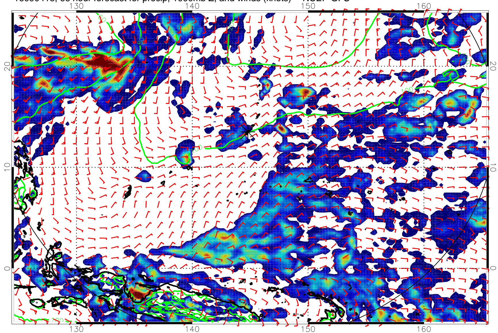
16090418, 66 hour forecast for precip, 1000mb Z, and winds (knots) -- NCEP GFS
