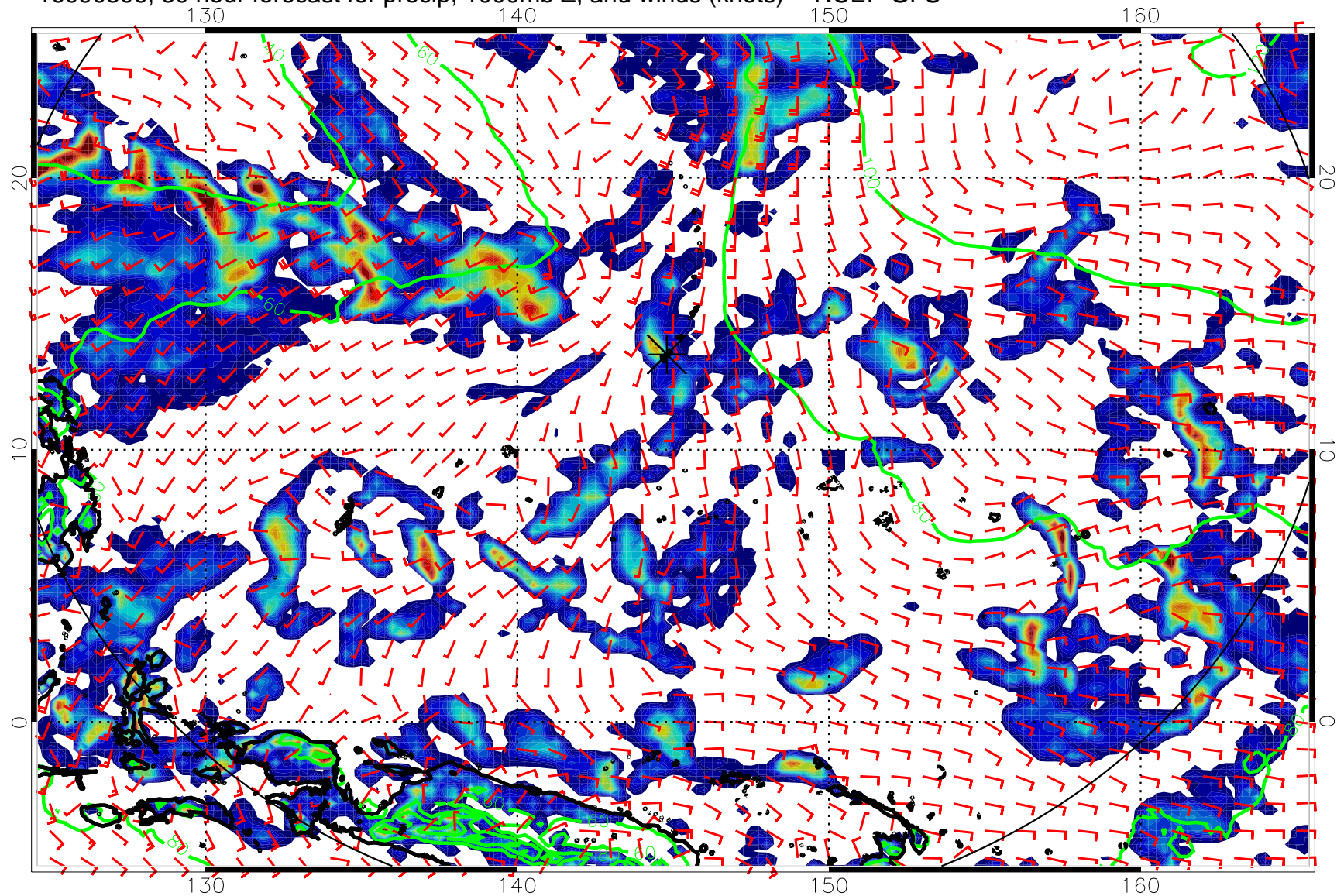
16090306, 30 hour forecast for precip, 1000mb Z, and winds (knots) -- NCEP GFS
