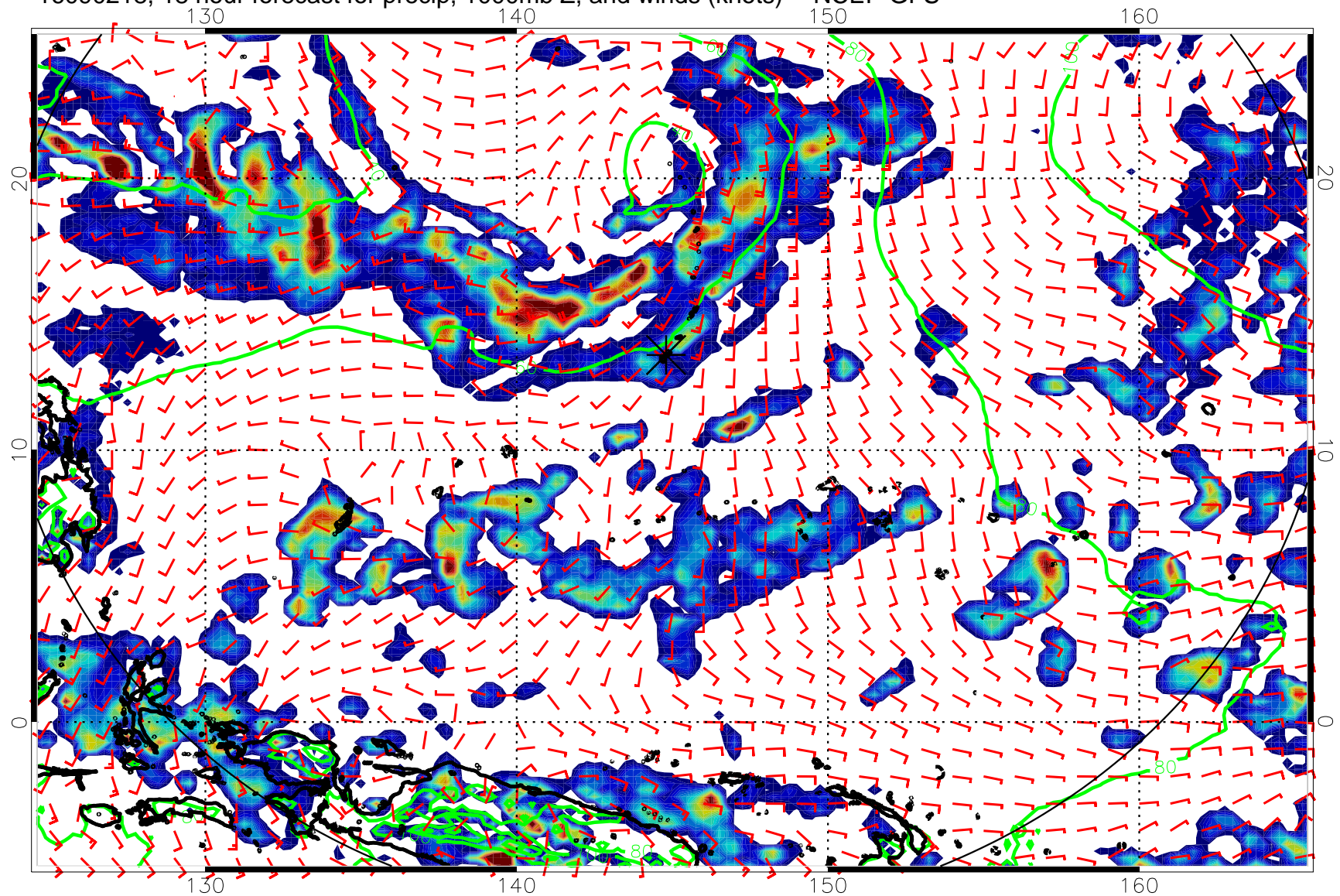
16090218, 18 hour forecast for precip, 1000mb Z, and winds (knots) -- NCEP GFS
