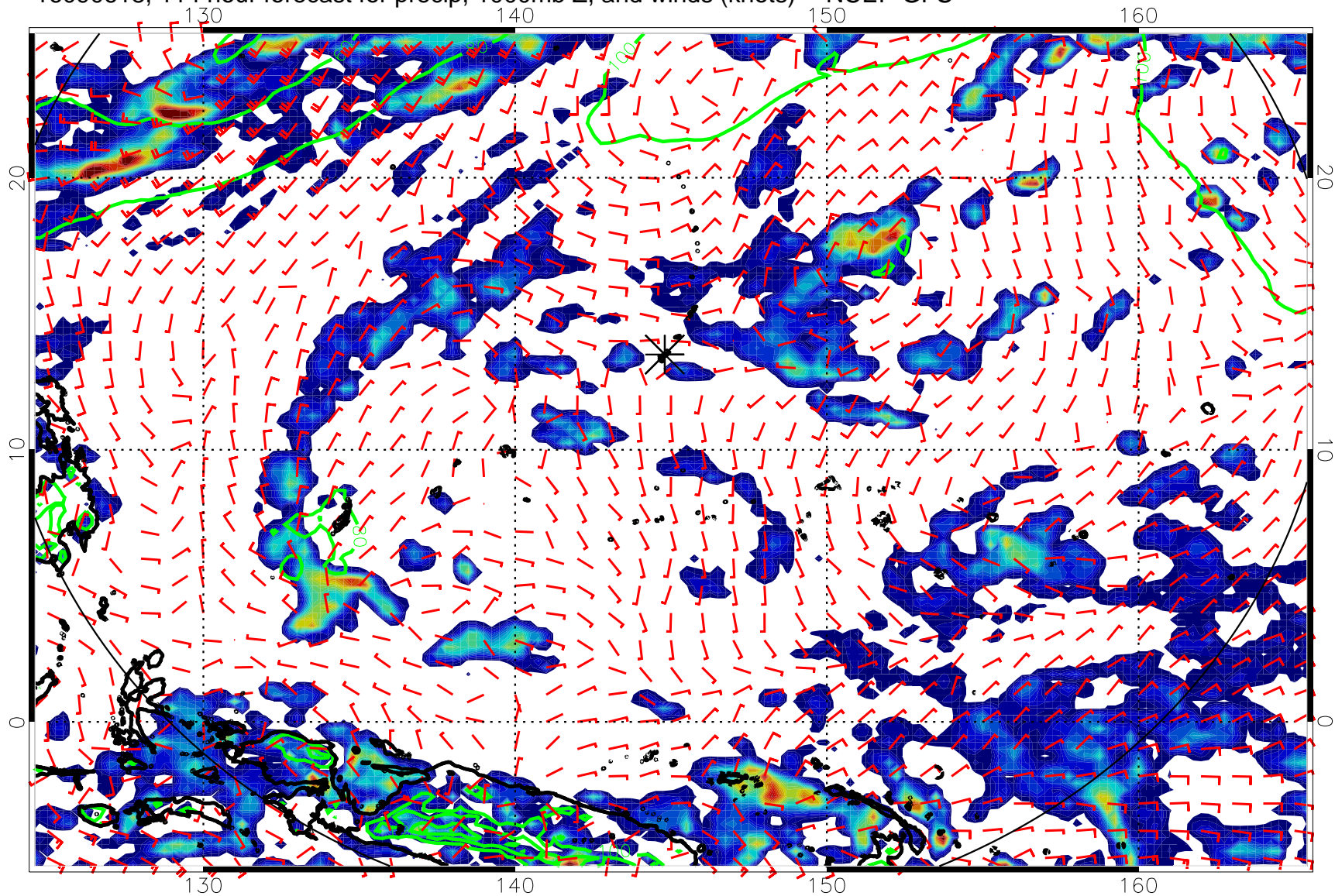
16090618, 114 hour forecast for precip, 1000mb Z, and winds (knots) -- NCEP GFS
