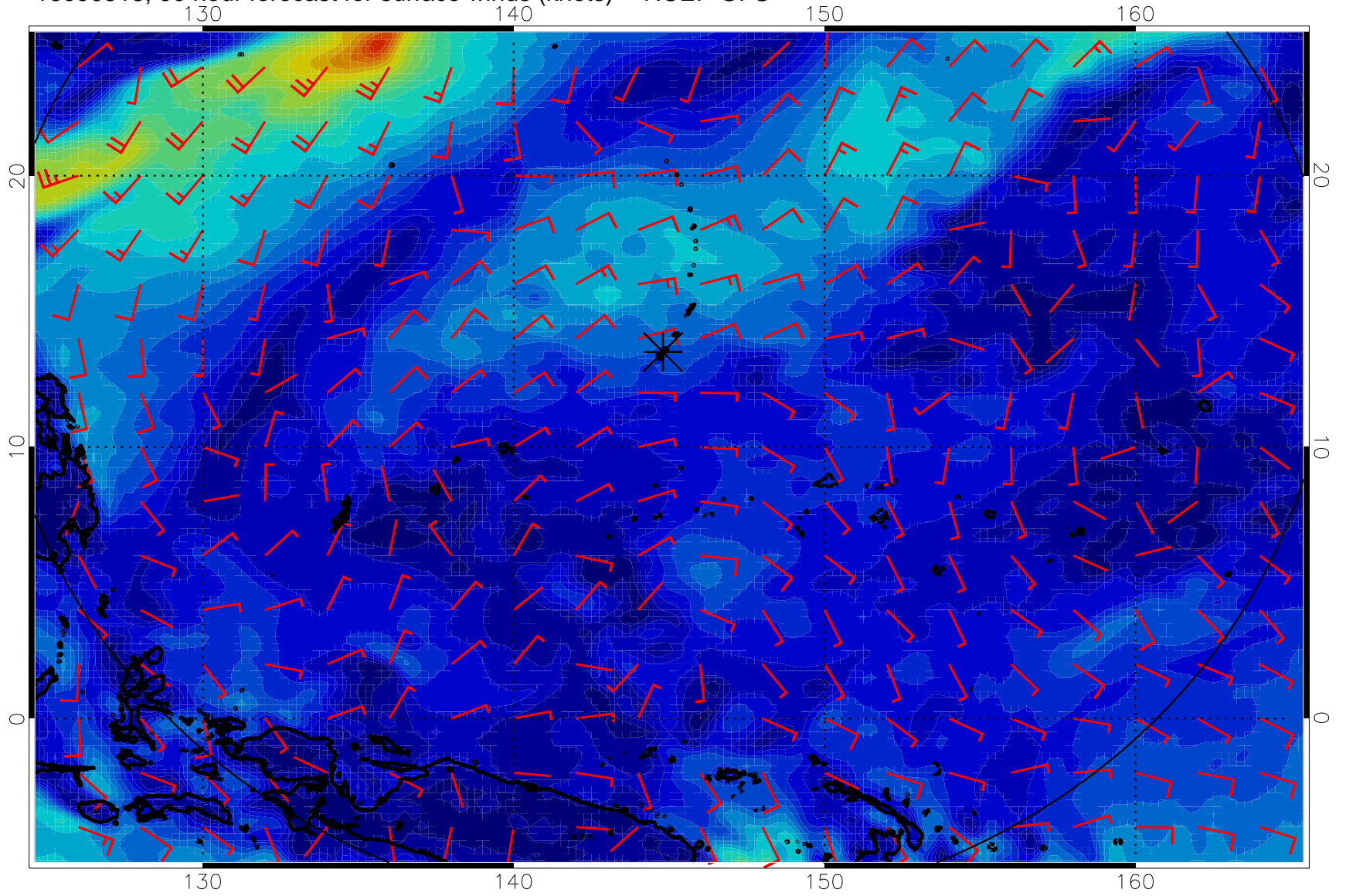
16090518, 90 hour forecast for surface winds (knots) -- NCEP GFS
