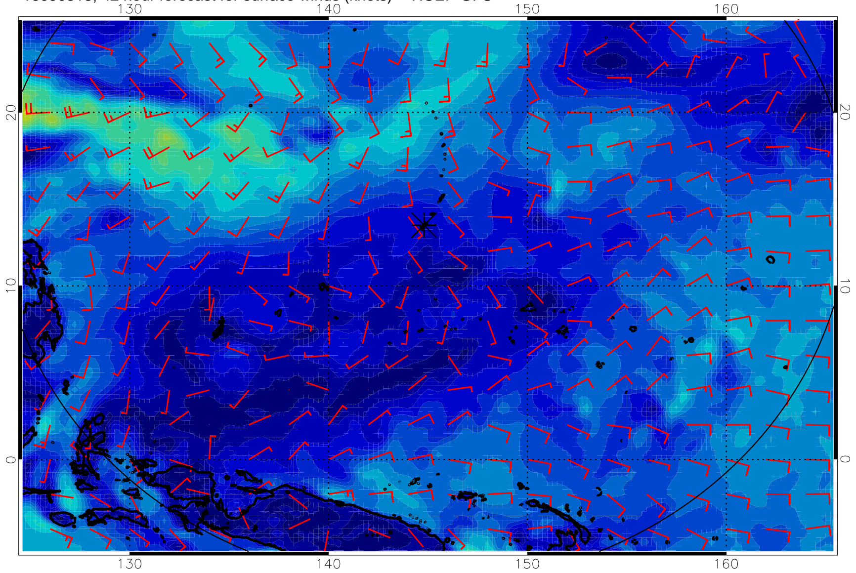
16090318, 42 hour forecast for surface winds (knots) -- NCEP GFS
