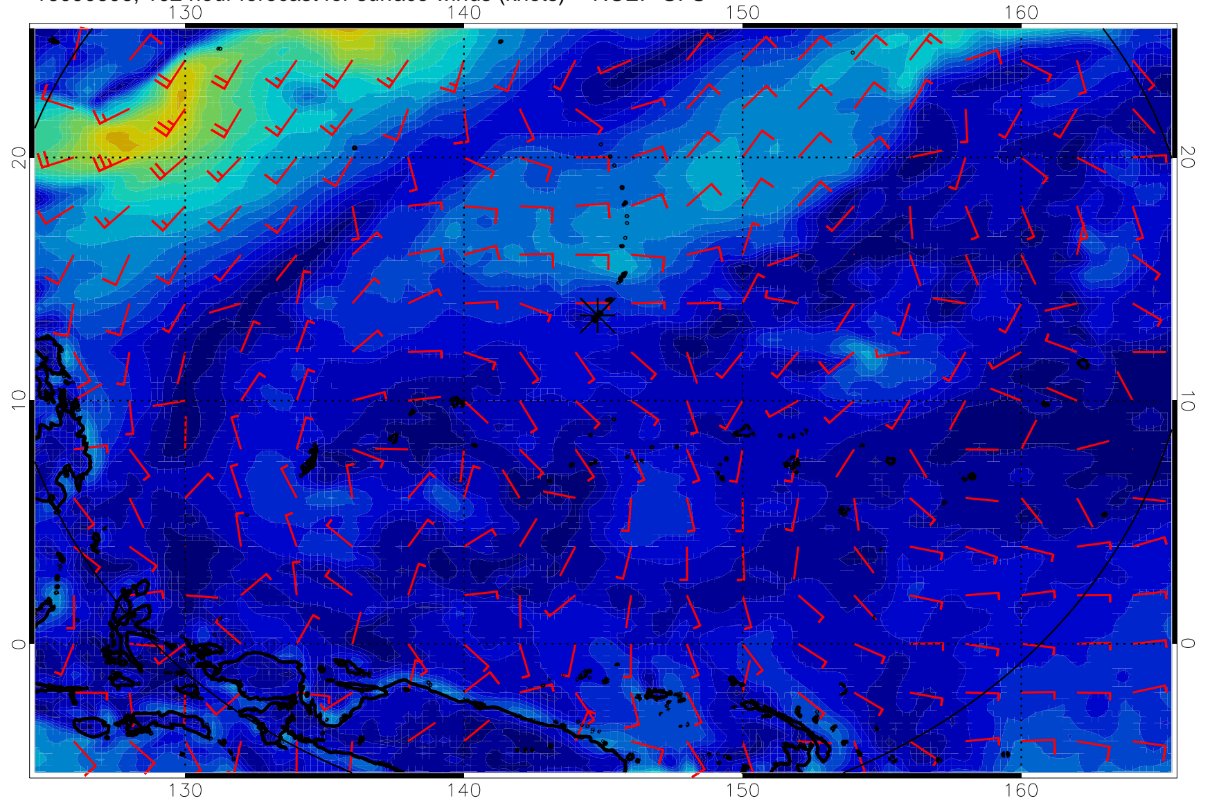
16090606, 102 hour forecast for surface winds (knots) -- NCEP GFS
