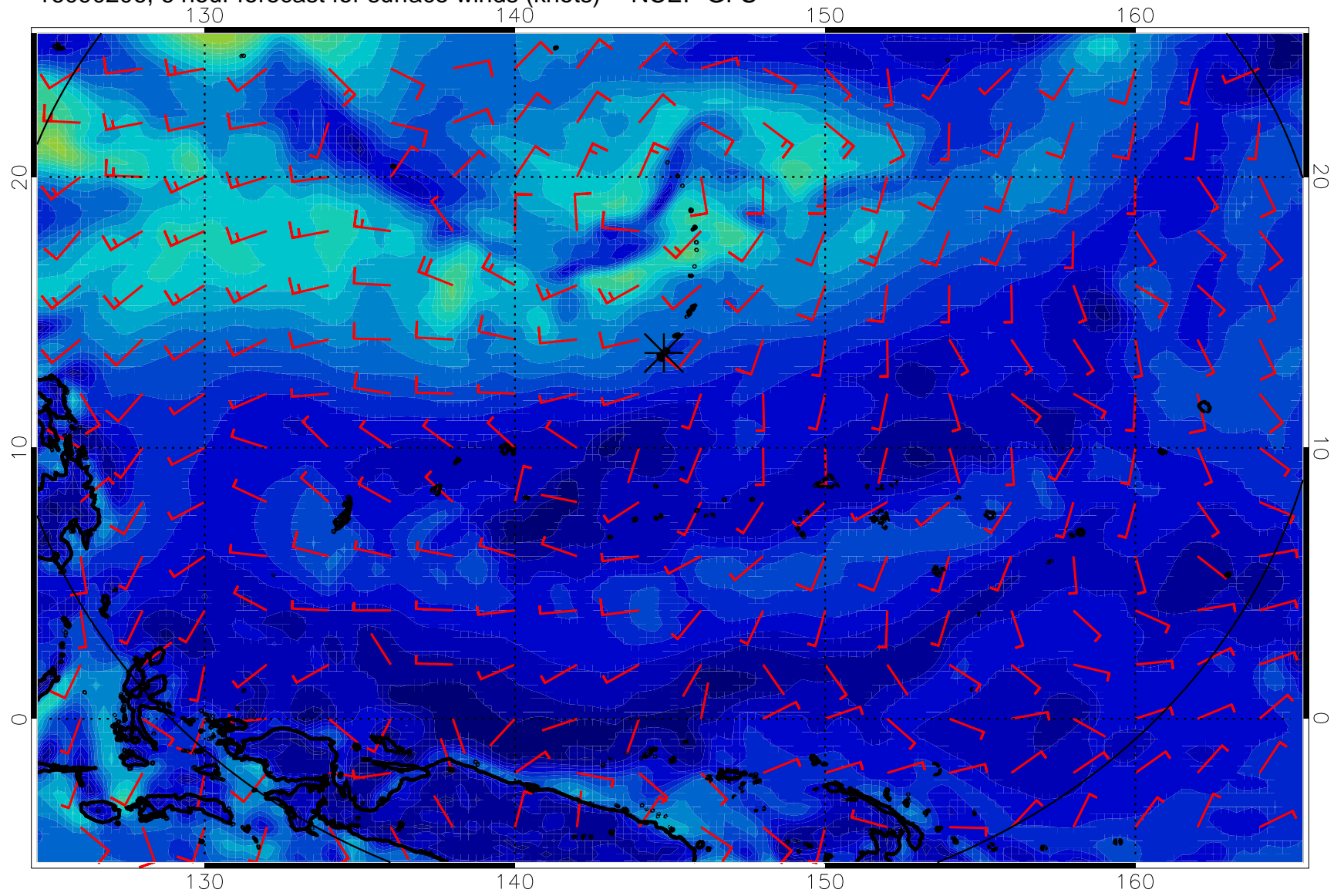
16090206, 6 hour forecast for surface winds (knots) -- NCEP GFS
