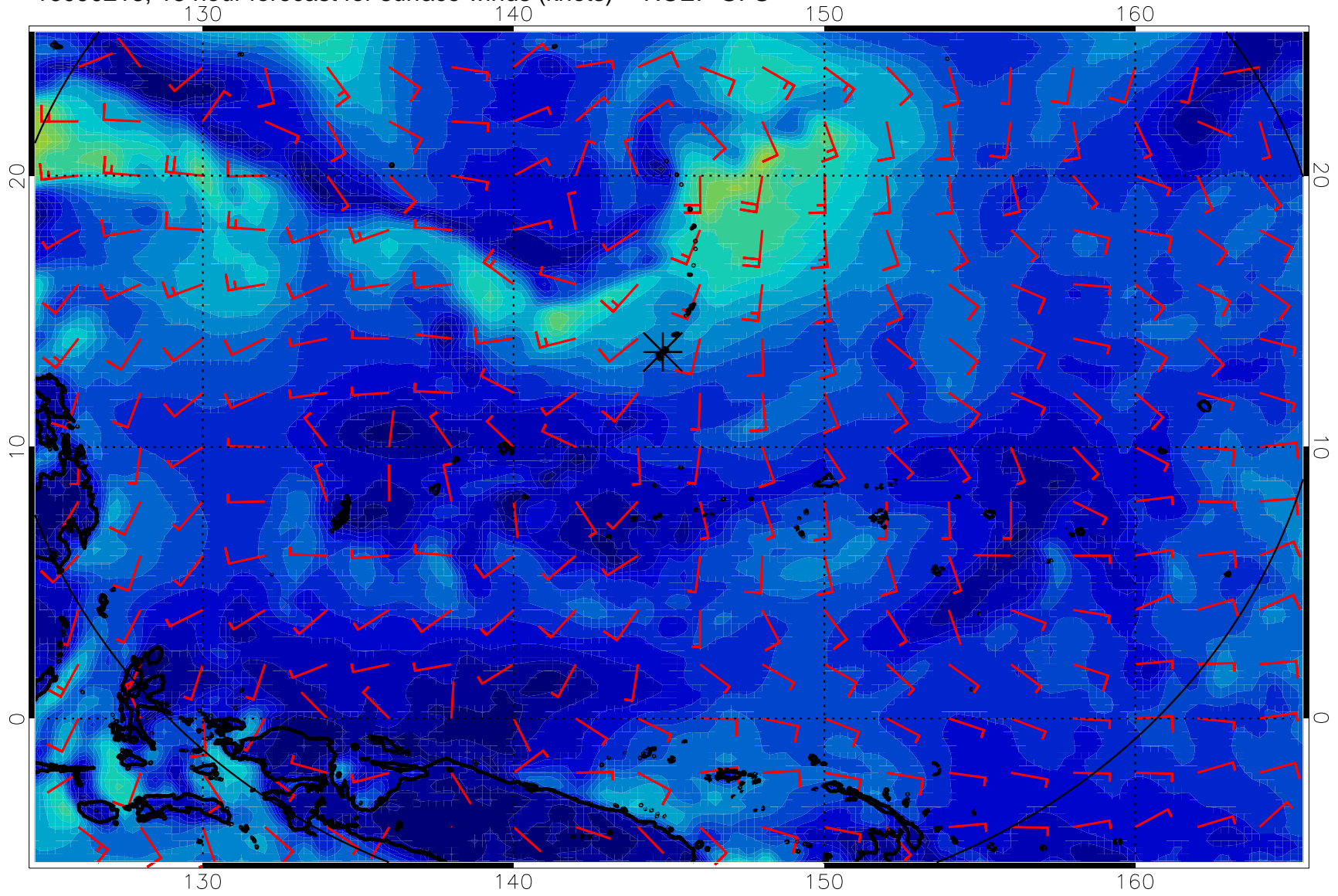
16090218, 18 hour forecast for surface winds (knots) -- NCEP GFS
