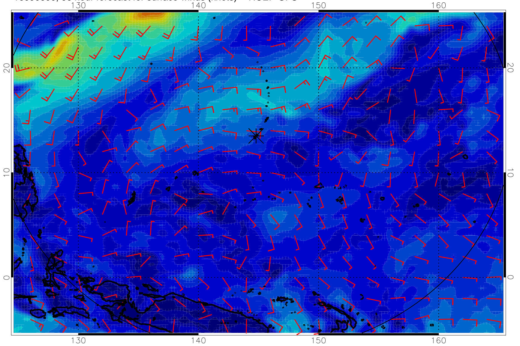
16090600, 96 hour forecast for surface winds (knots) -- NCEP GFS
