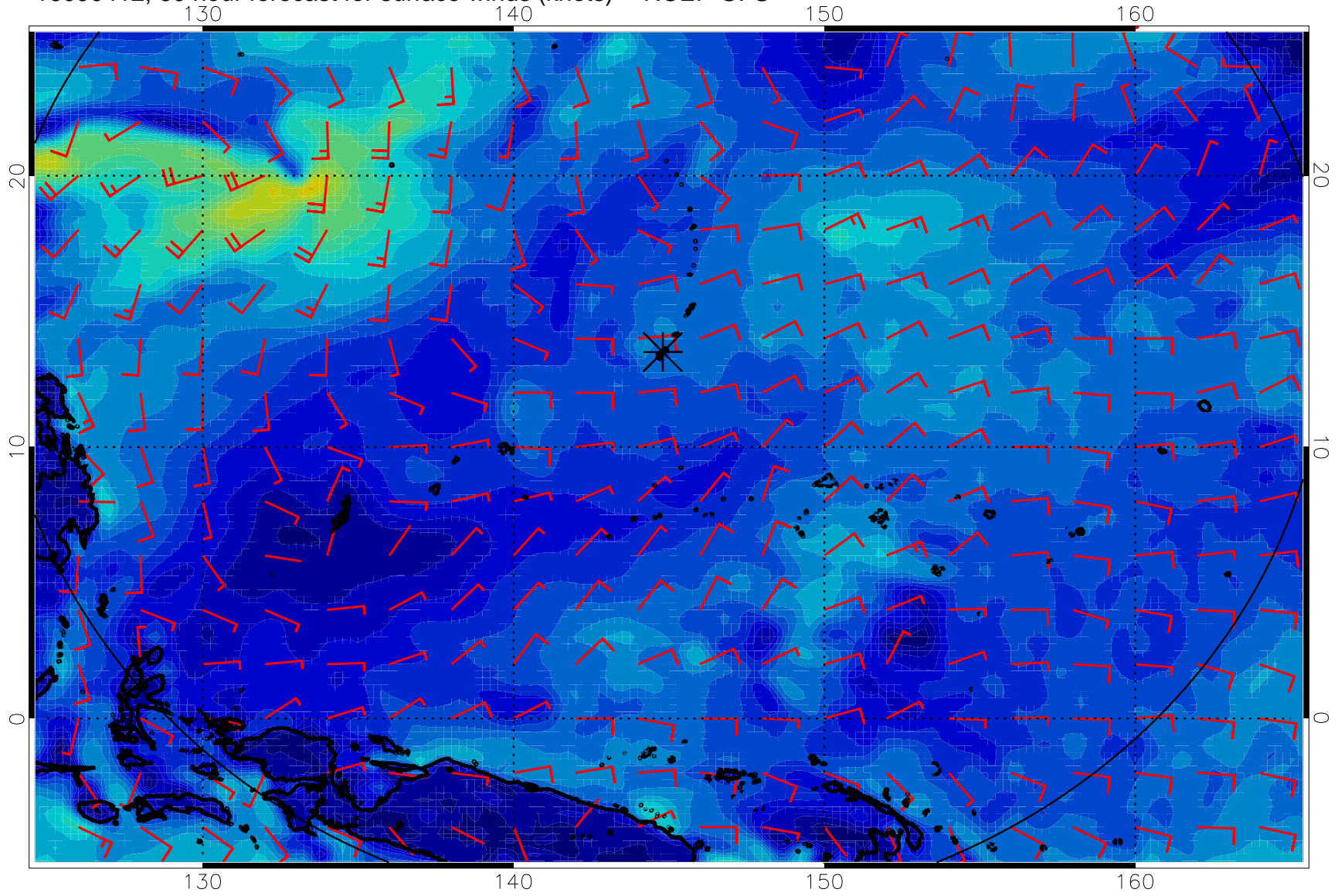
16090412, 60 hour forecast for surface winds (knots) -- NCEP GFS
