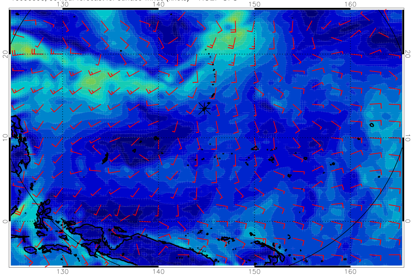
16090306, 30 hour forecast for surface winds (knots) -- NCEP GFS
