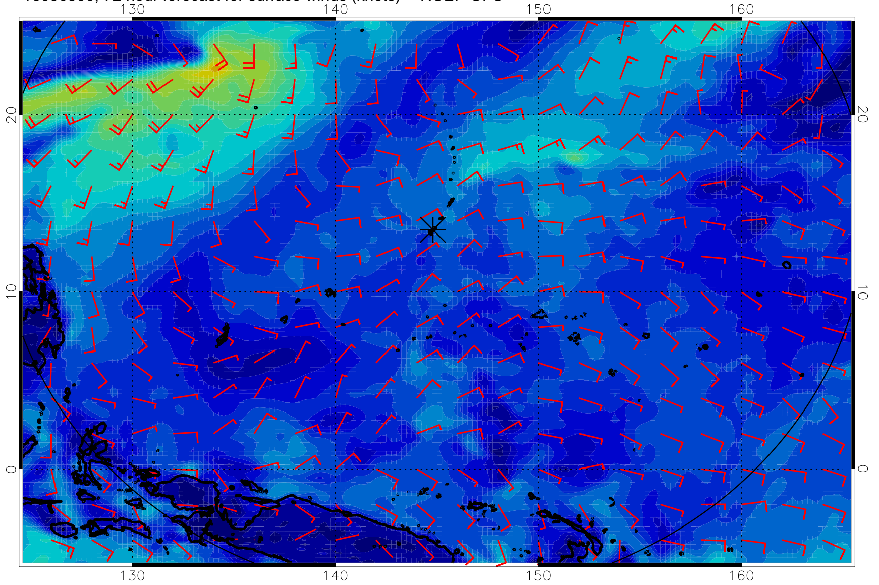
16090500, 72 hour forecast for surface winds (knots) -- NCEP GFS
