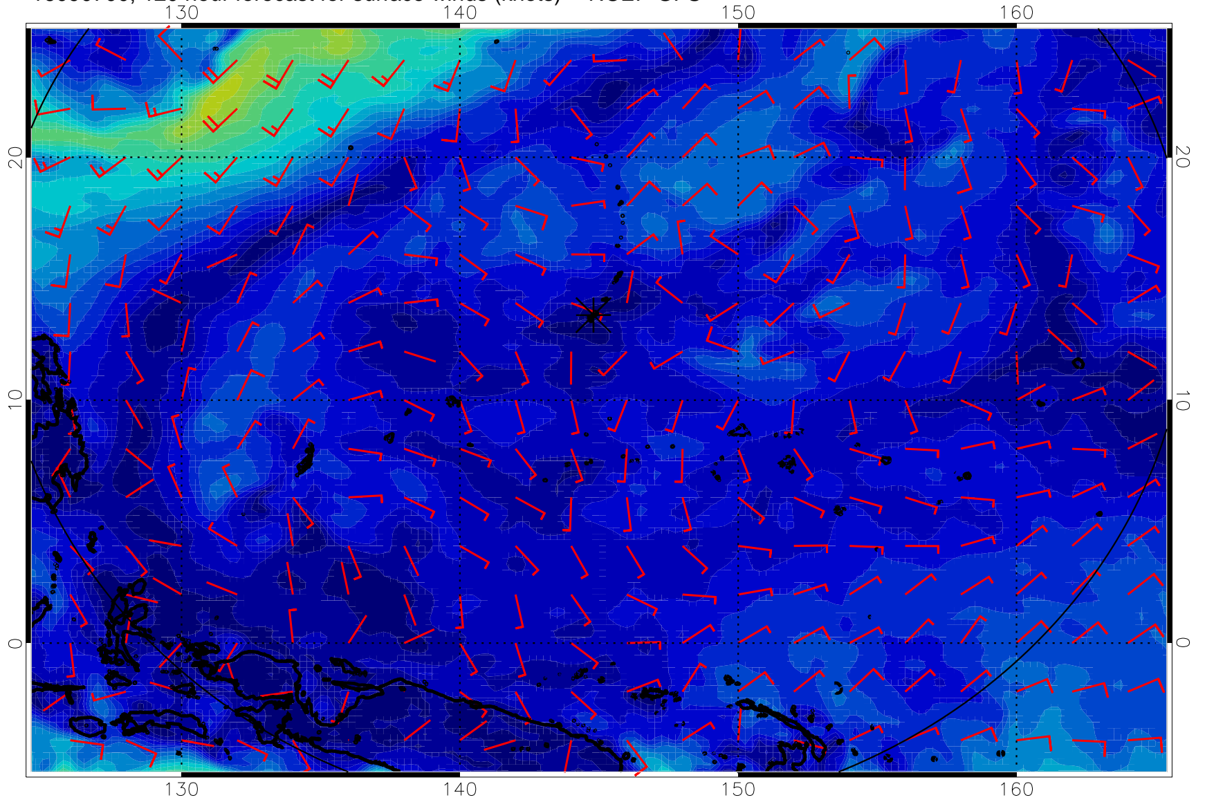
16090700, 120 hour forecast for surface winds (knots) -- NCEP GFS
