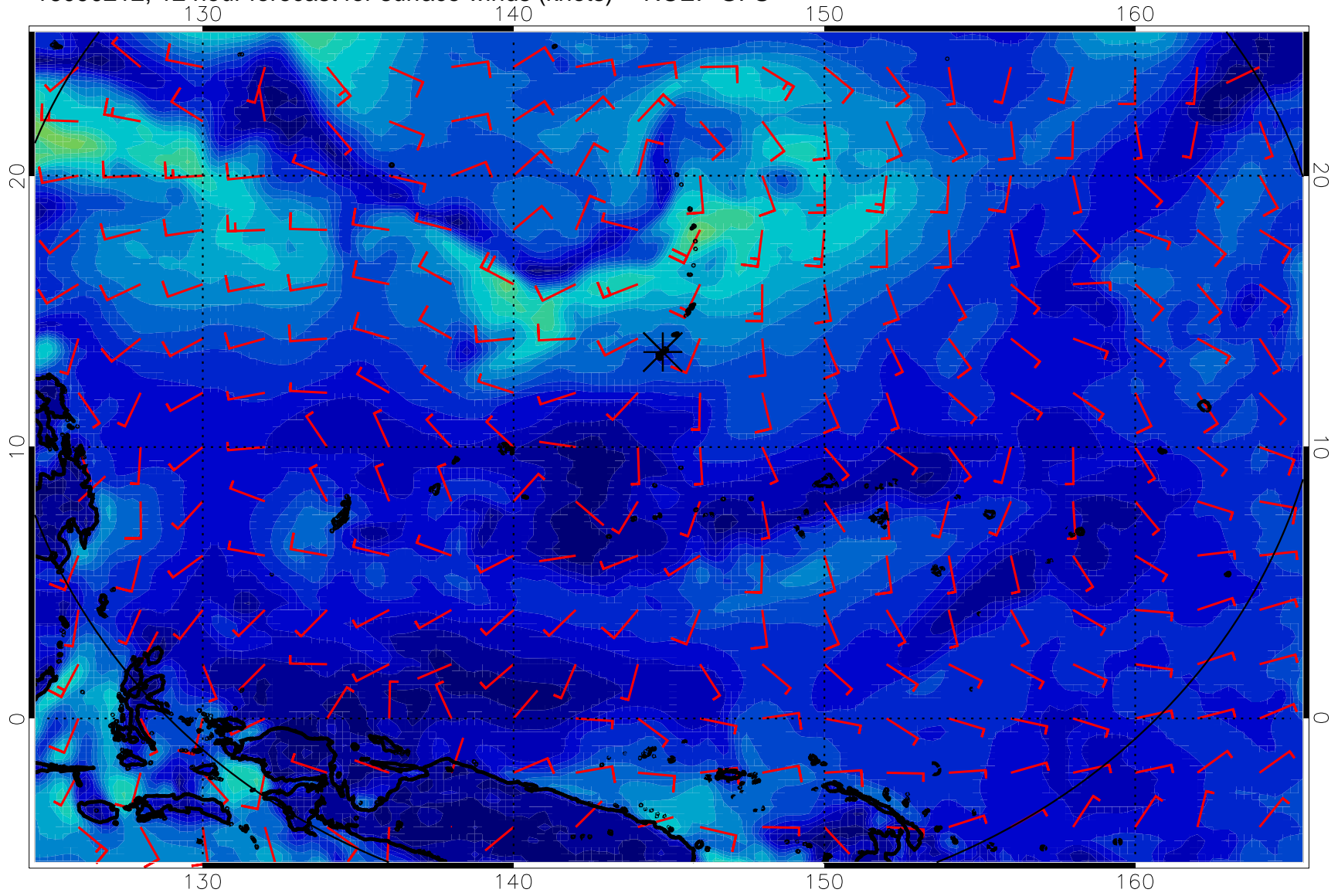
16090212, 12 hour forecast for surface winds (knots) -- NCEP GFS
