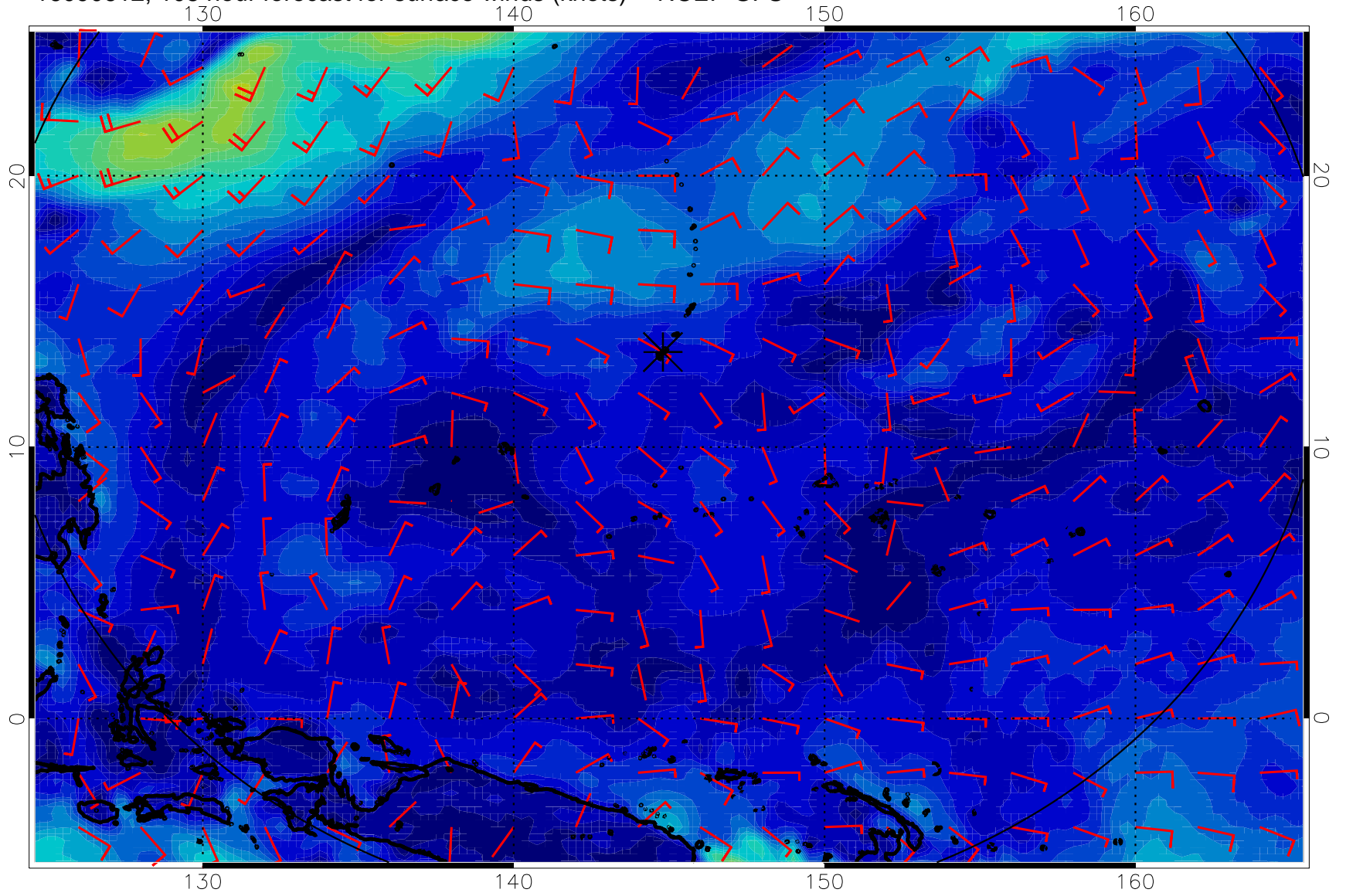
16090612, 108 hour forecast for surface winds (knots) -- NCEP GFS
