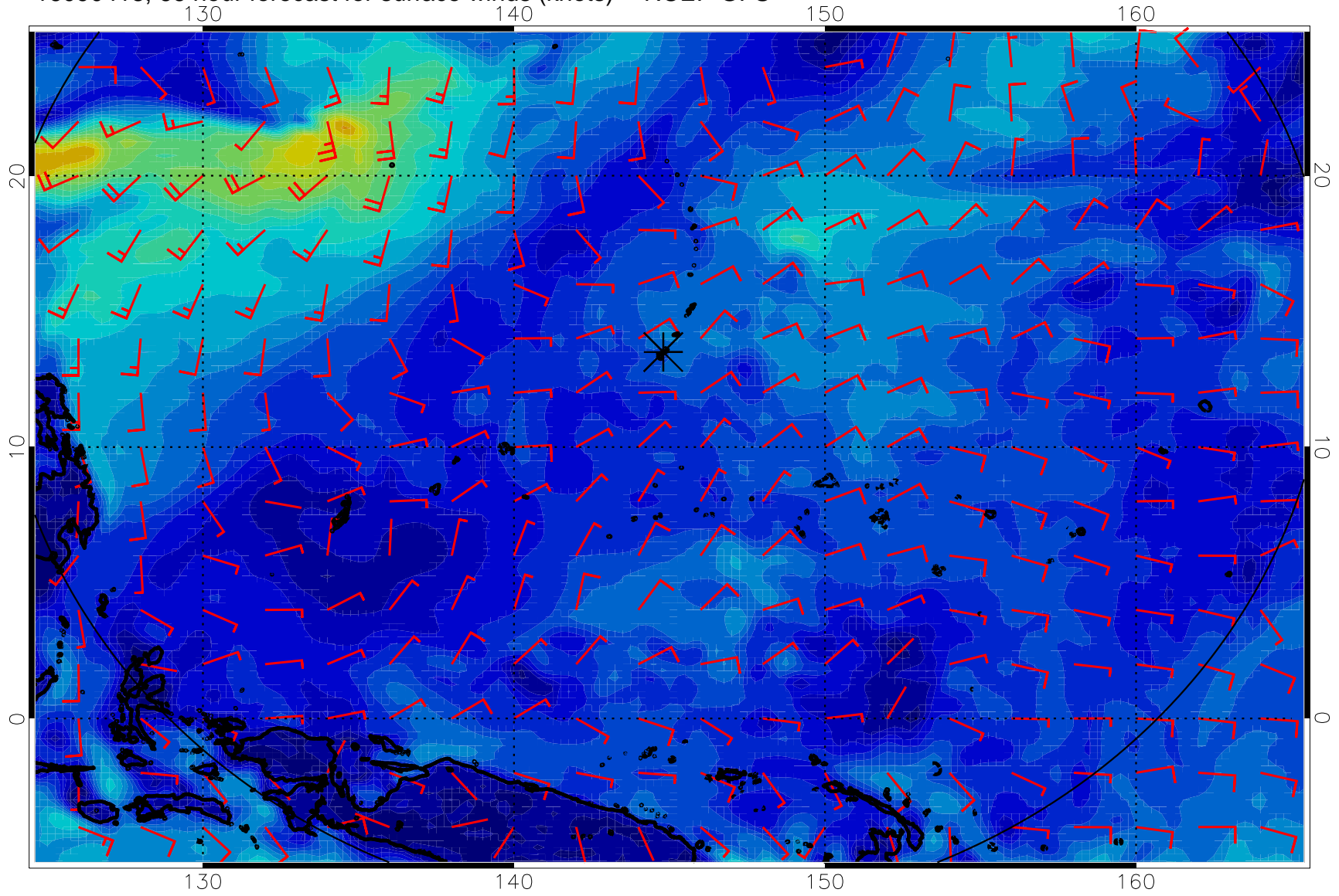
16090418, 66 hour forecast for surface winds (knots) -- NCEP GFS
