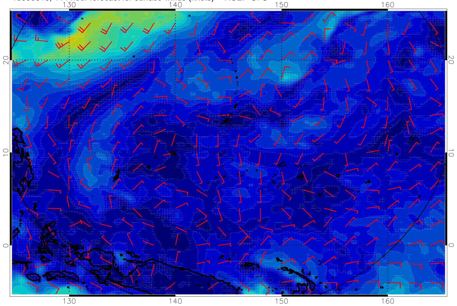
16090618, 114 hour forecast for surface winds (knots) -- NCEP GFS
