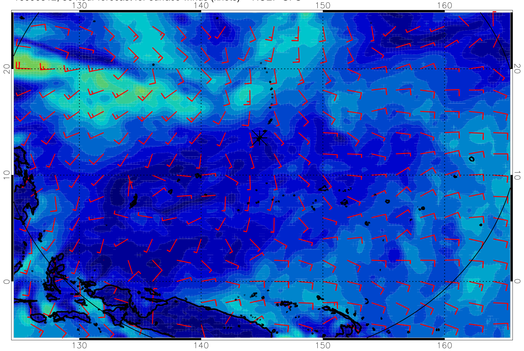
16090312, 36 hour forecast for surface winds (knots) -- NCEP GFS
