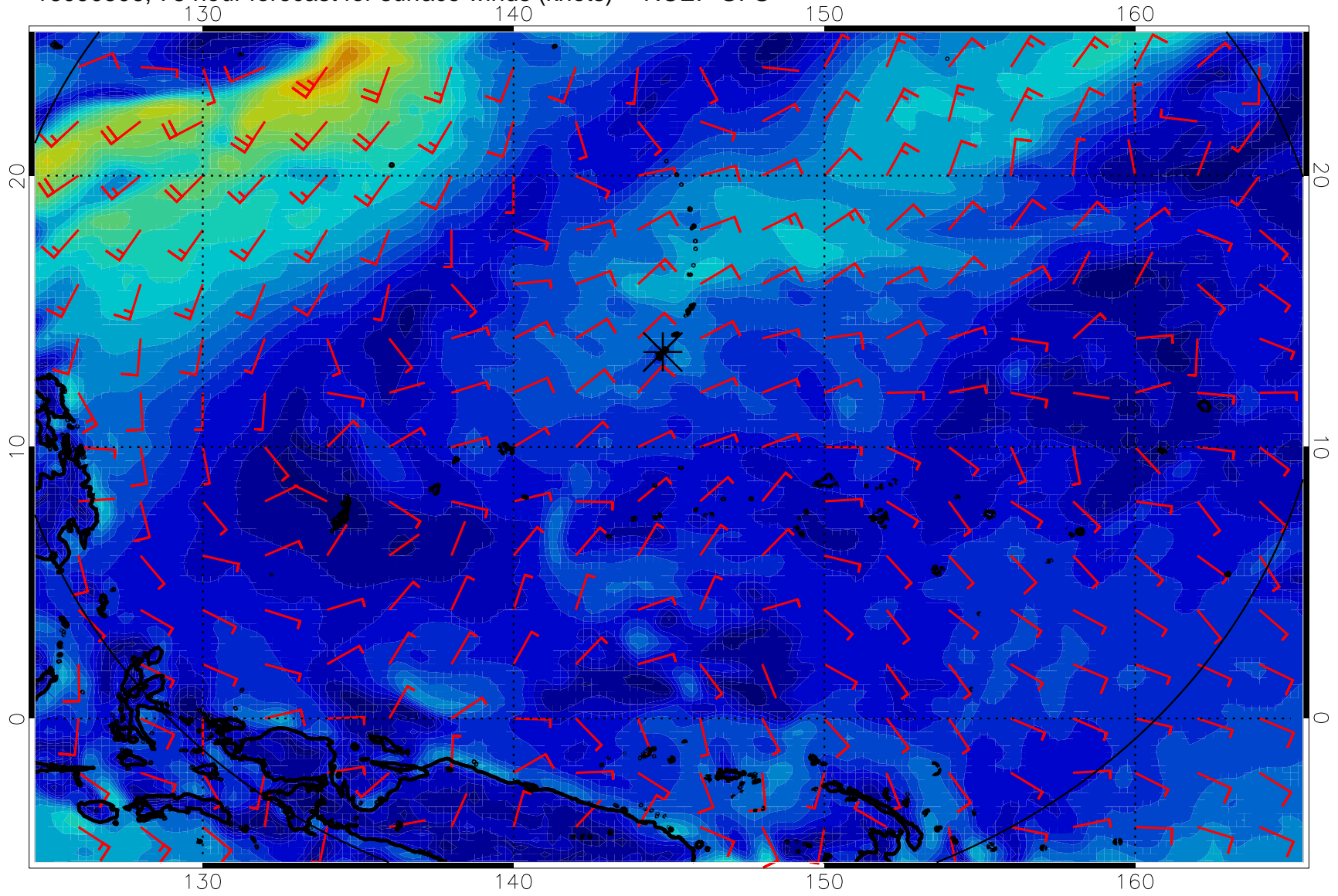
16090506, 78 hour forecast for surface winds (knots) -- NCEP GFS
