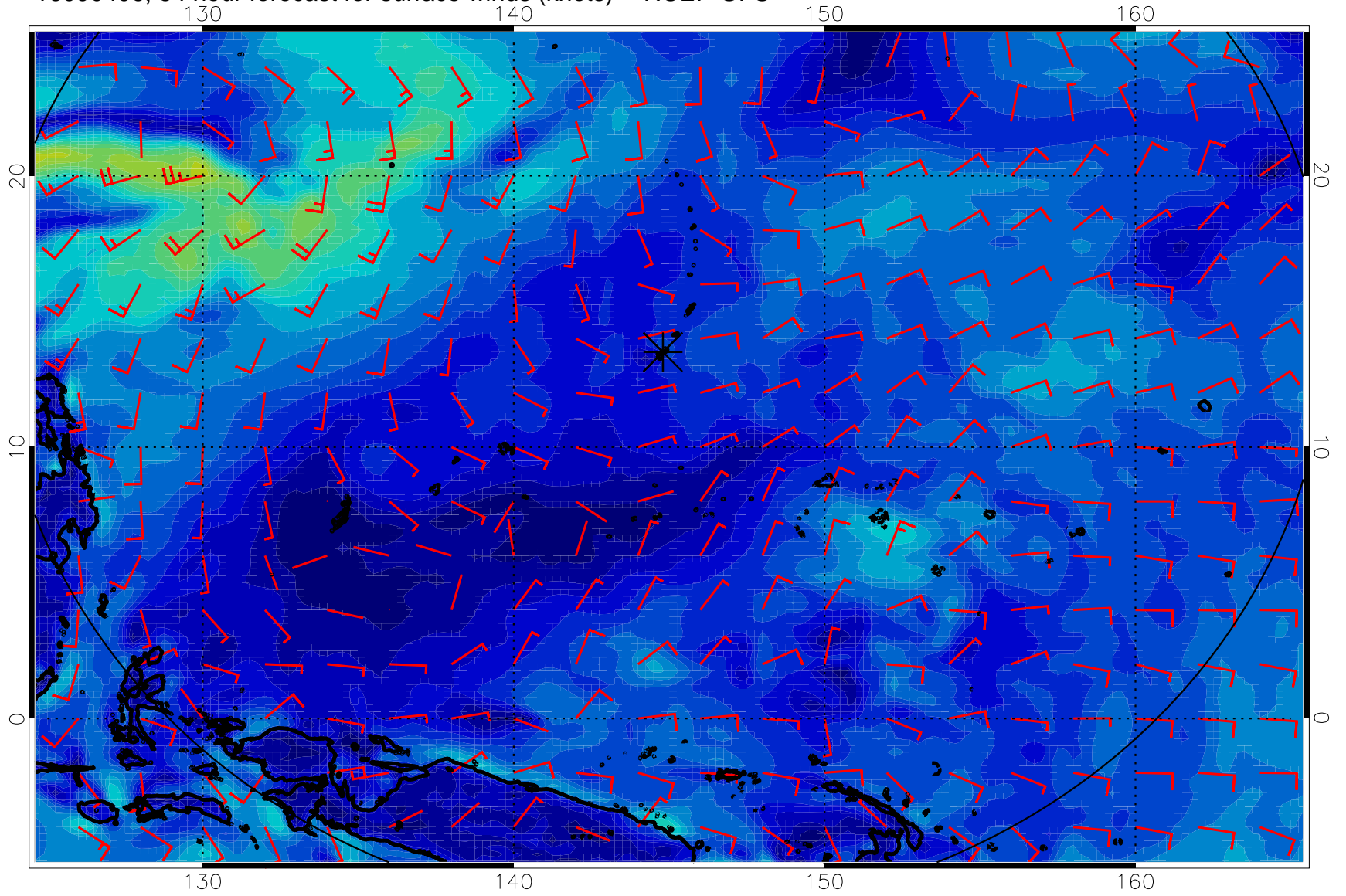
16090406, 54 hour forecast for surface winds (knots) -- NCEP GFS
