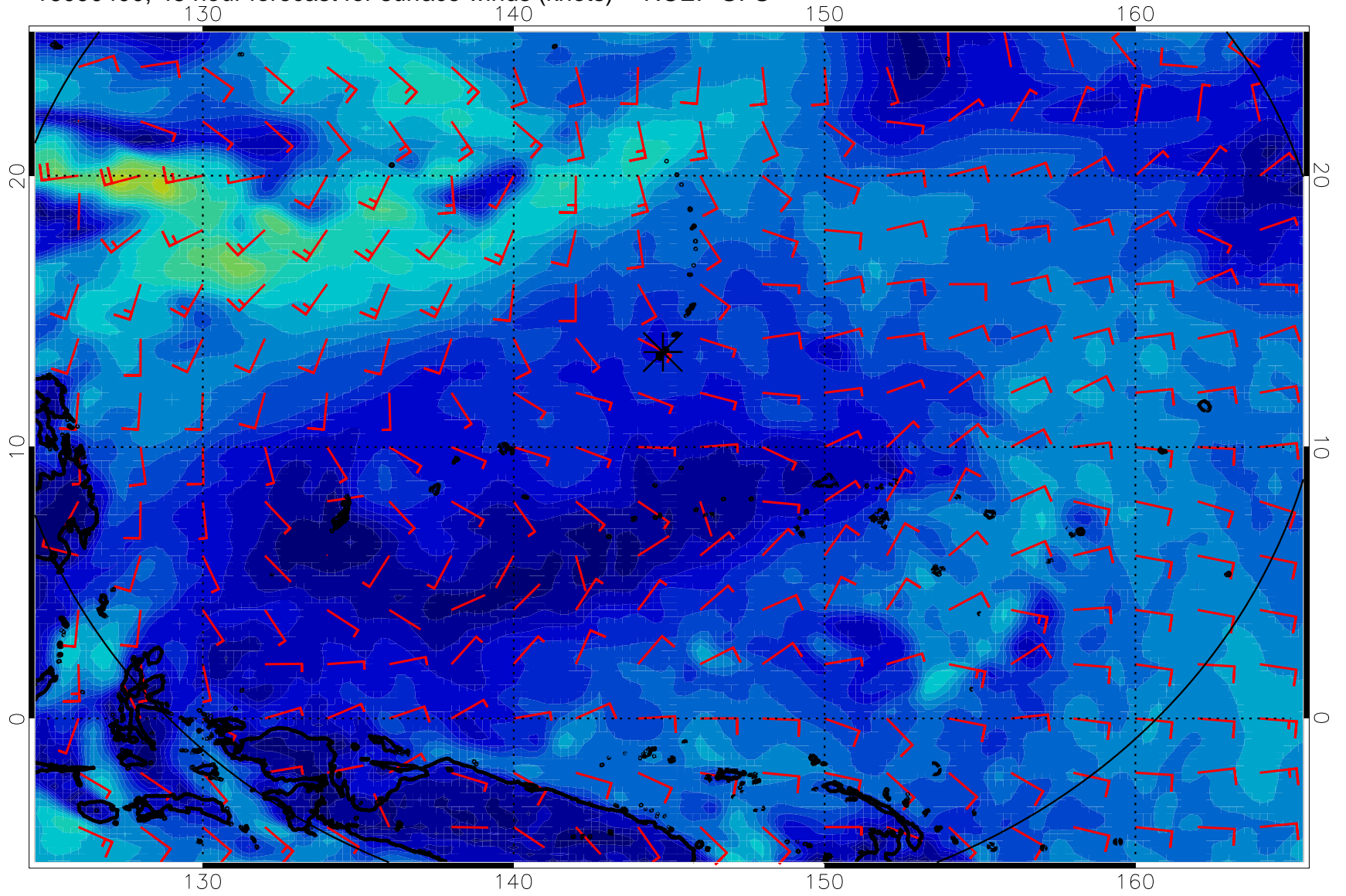
16090400, 48 hour forecast for surface winds (knots) -- NCEP GFS
