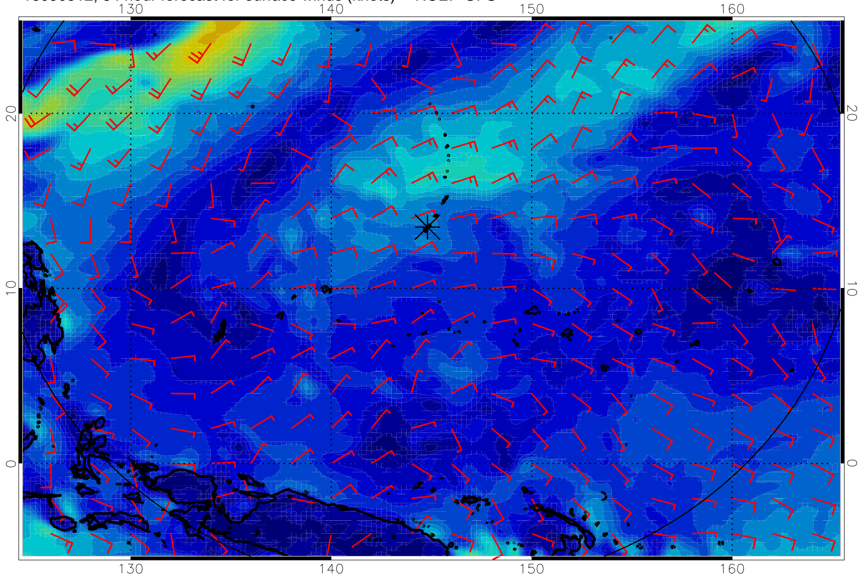
16090512, 84 hour forecast for surface winds (knots) -- NCEP GFS
