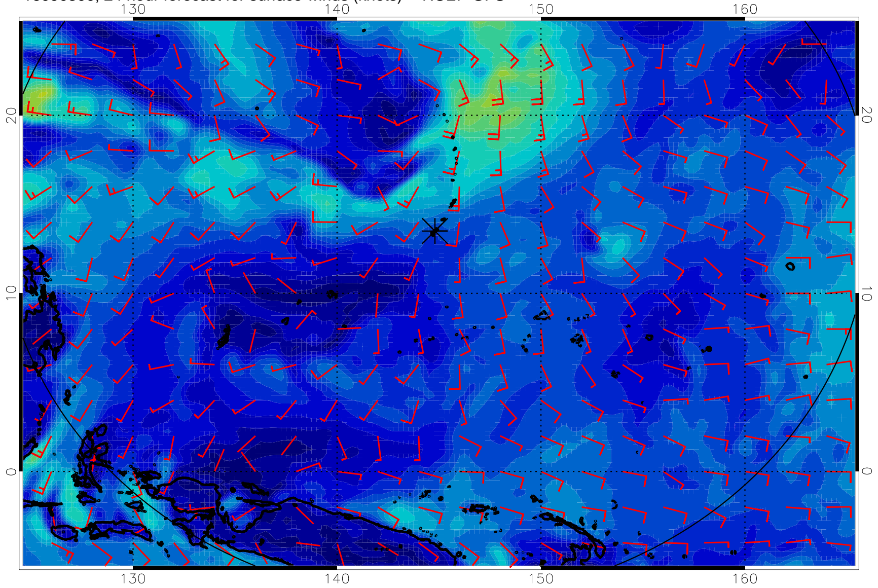
16090300, 24 hour forecast for surface winds (knots) -- NCEP GFS
