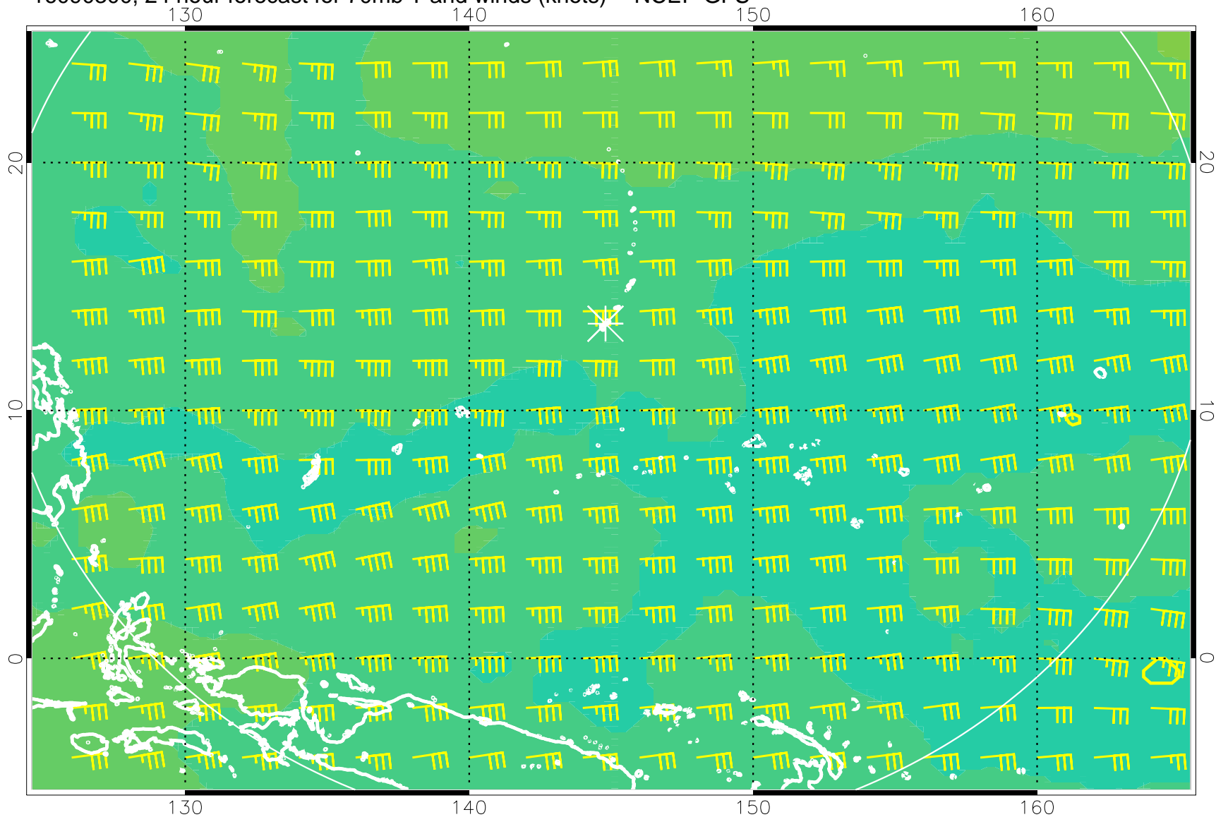
16090300, 24 hour forecast for 70mb T and winds (knots) -- NCEP GFS
