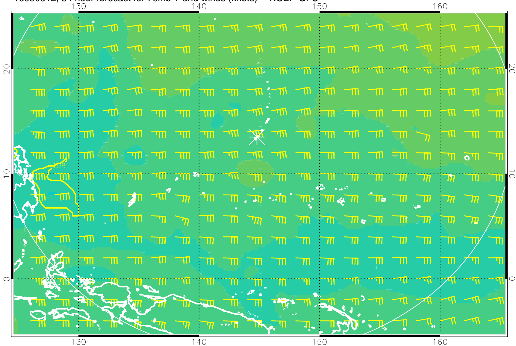
16090512, 84 hour forecast for 70mb T and winds (knots) -- NCEP GFS
