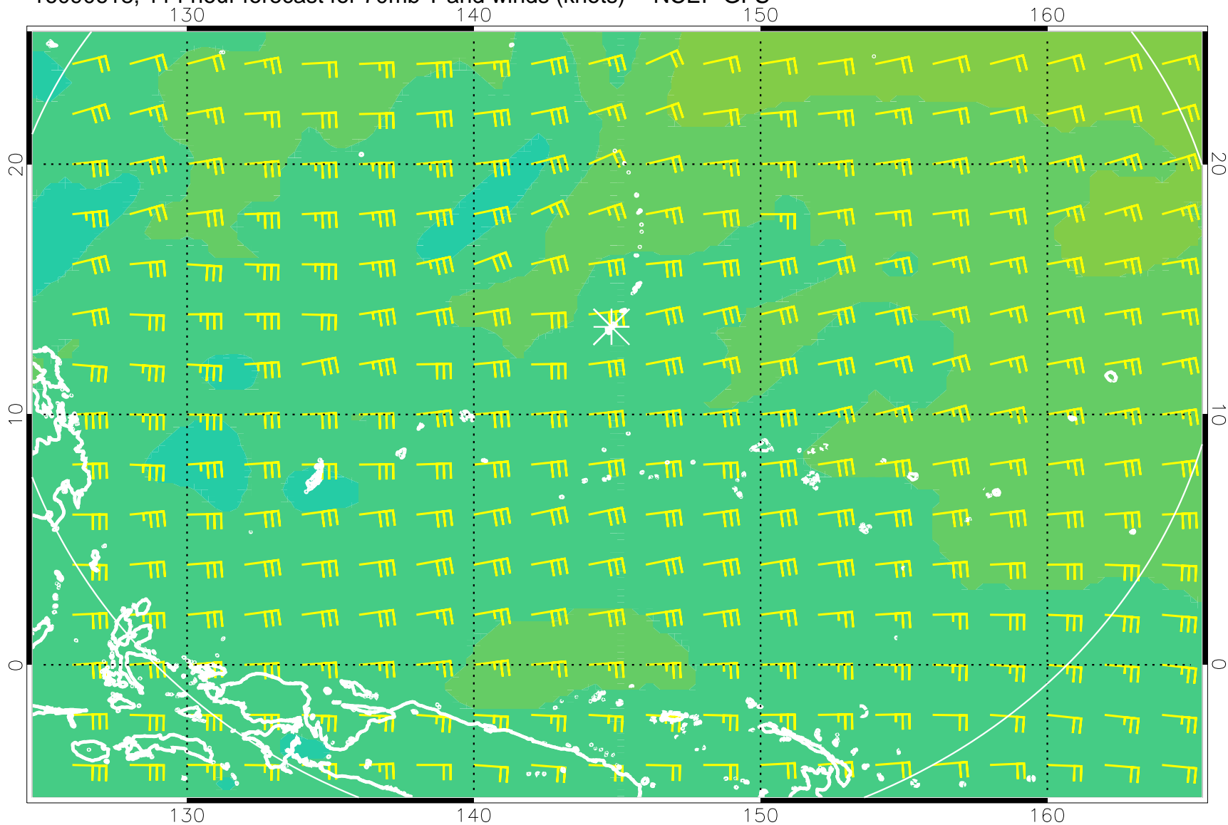
16090618, 114 hour forecast for 70mb T and winds (knots) -- NCEP GFS
