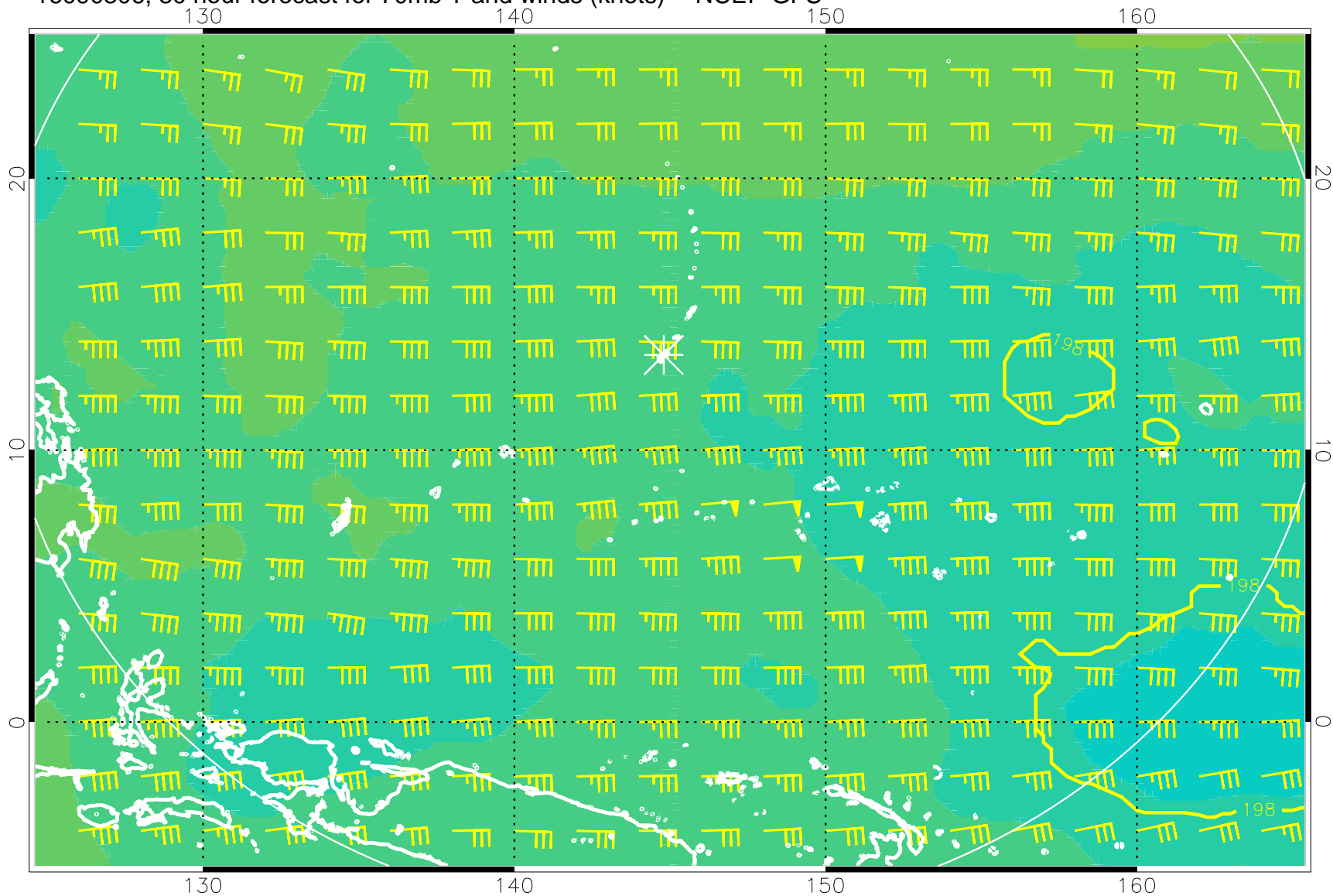
16090306, 30 hour forecast for 70mb T and winds (knots) -- NCEP GFS
