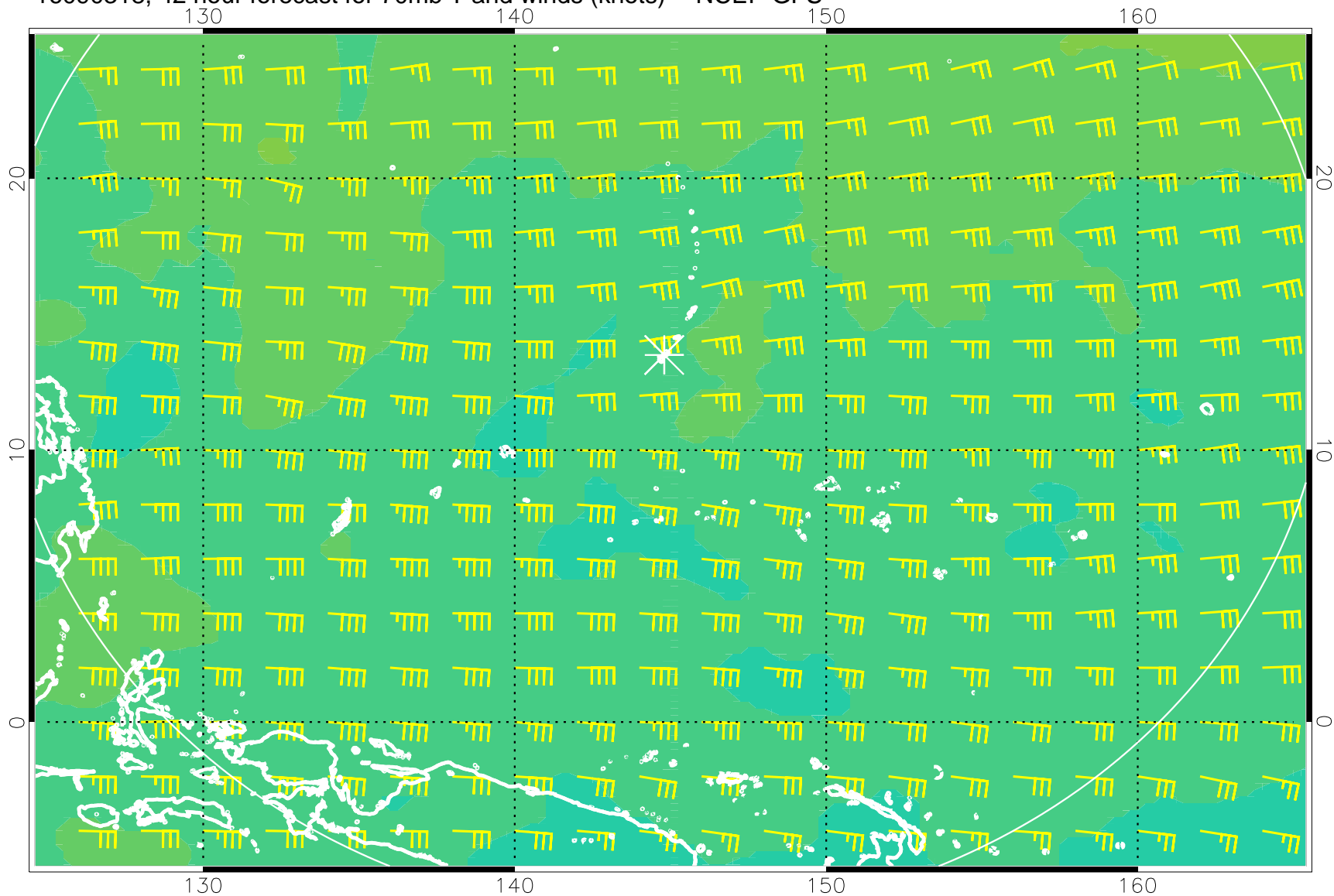
16090318, 42 hour forecast for 70mb T and winds (knots) -- NCEP GFS
