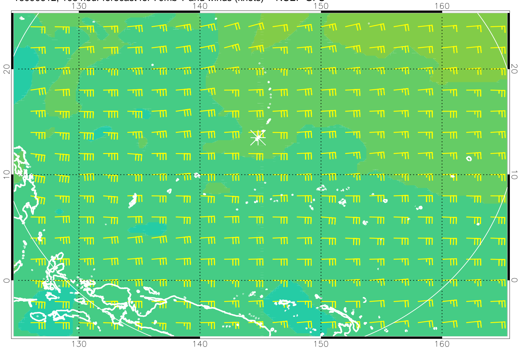
16090612, 108 hour forecast for 70mb T and winds (knots) -- NCEP GFS
