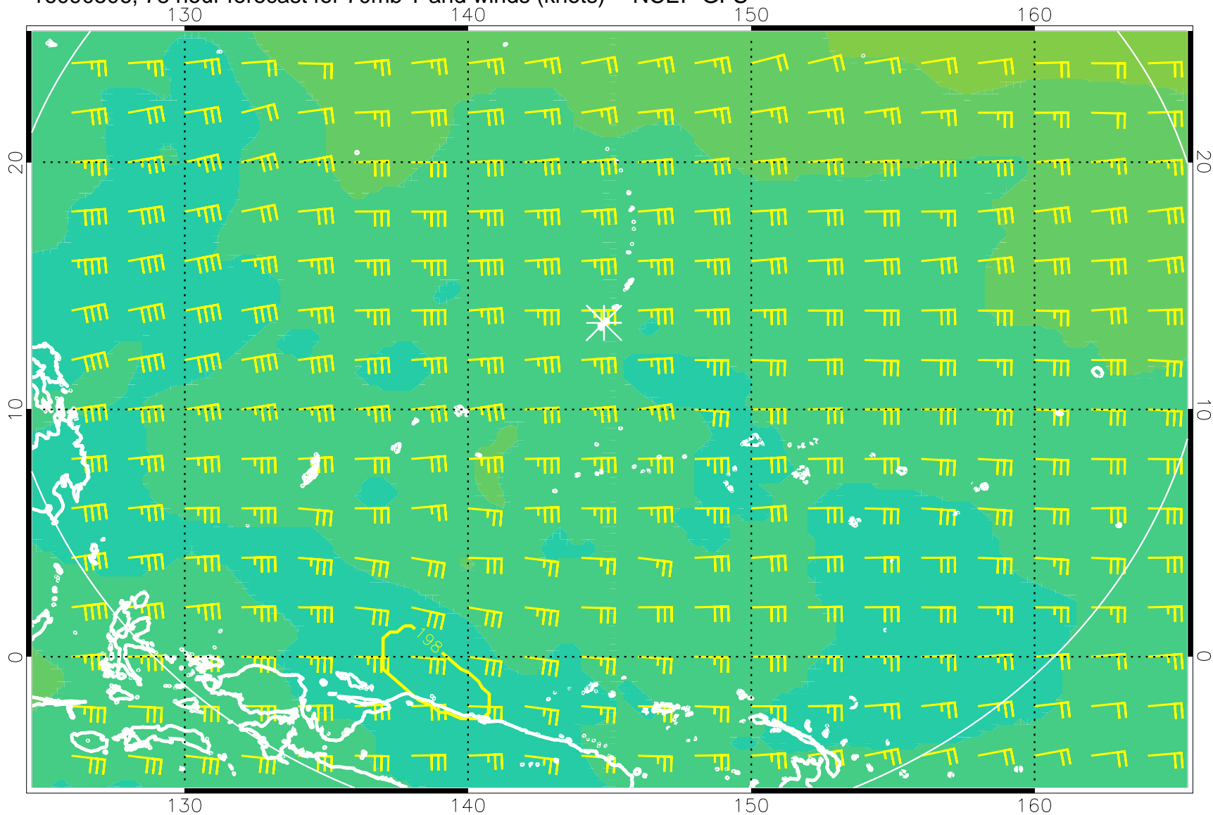
16090506, 78 hour forecast for 70mb T and winds (knots) -- NCEP GFS
