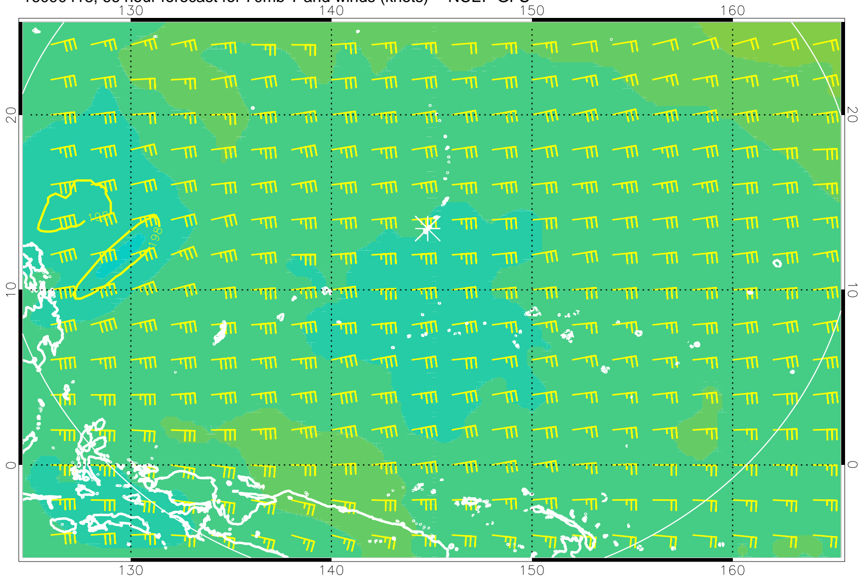
16090418, 66 hour forecast for 70mb T and winds (knots) -- NCEP GFS
