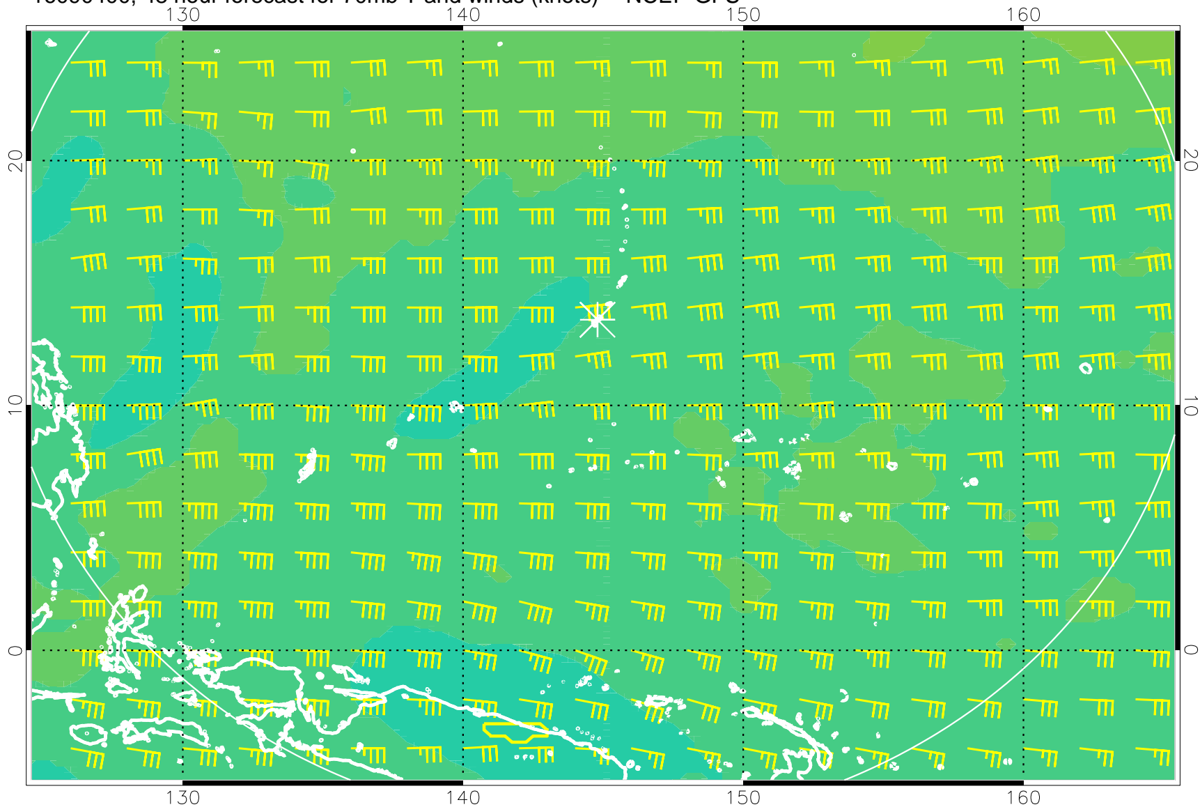
16090400, 48 hour forecast for 70mb T and winds (knots) -- NCEP GFS
