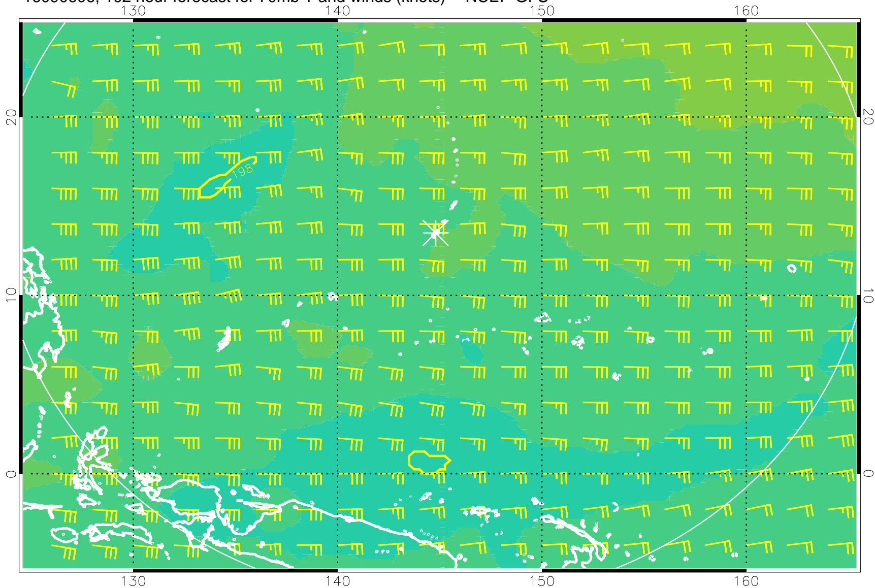
16090606, 102 hour forecast for 70mb T and winds (knots) -- NCEP GFS
