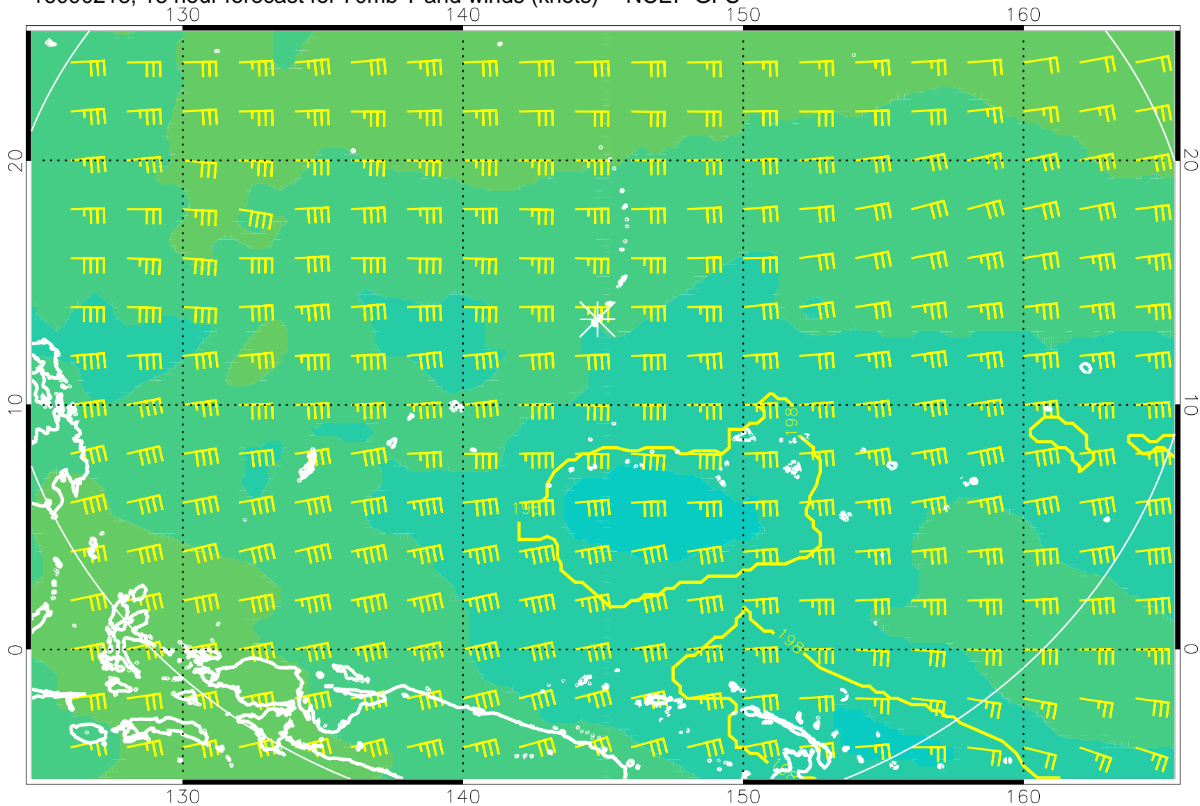
16090218, 18 hour forecast for 70mb T and winds (knots) -- NCEP GFS
