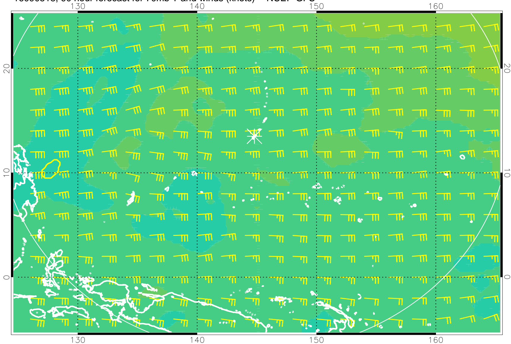
16090518, 90 hour forecast for 70mb T and winds (knots) -- NCEP GFS
