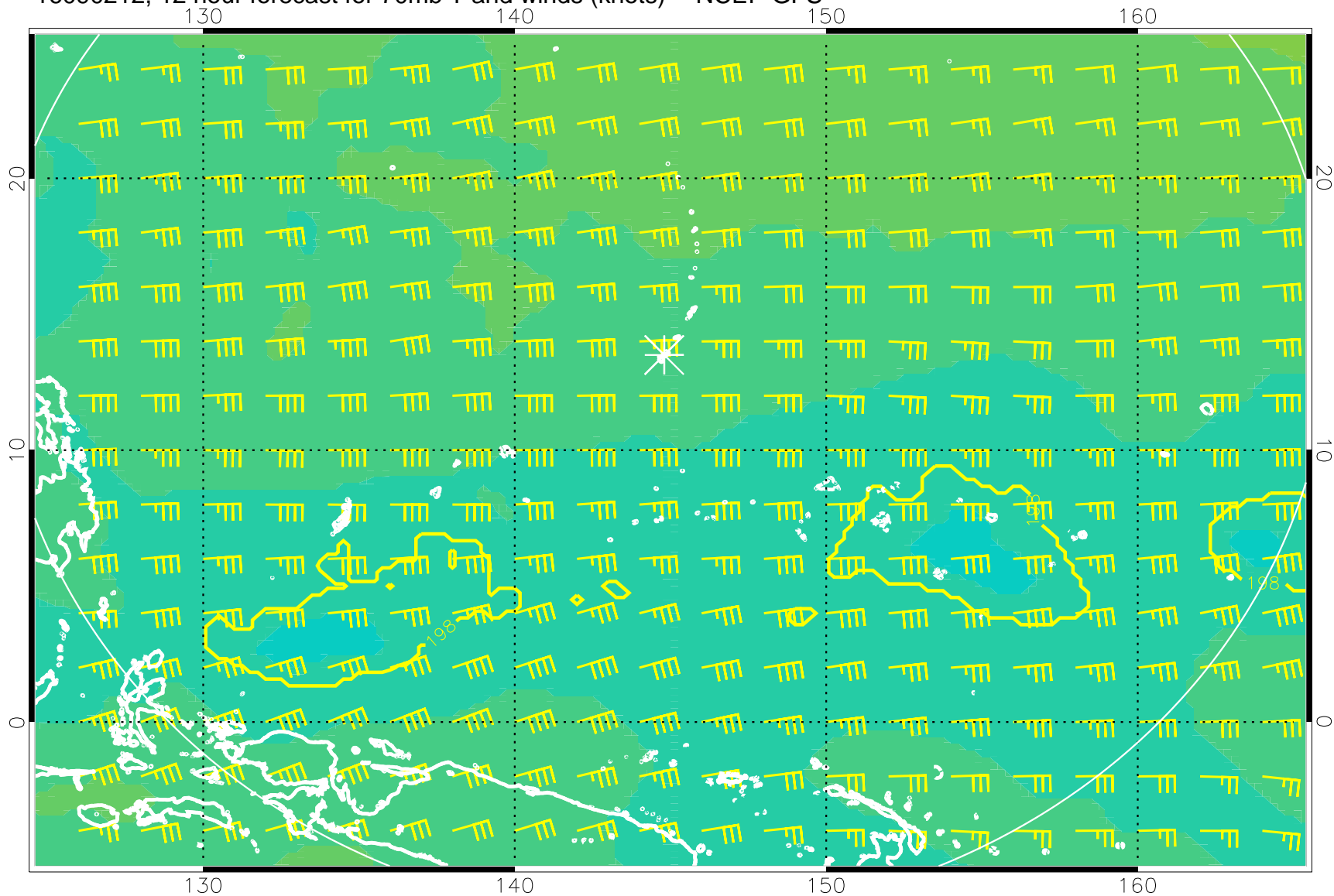
16090212, 12 hour forecast for 70mb T and winds (knots) -- NCEP GFS
