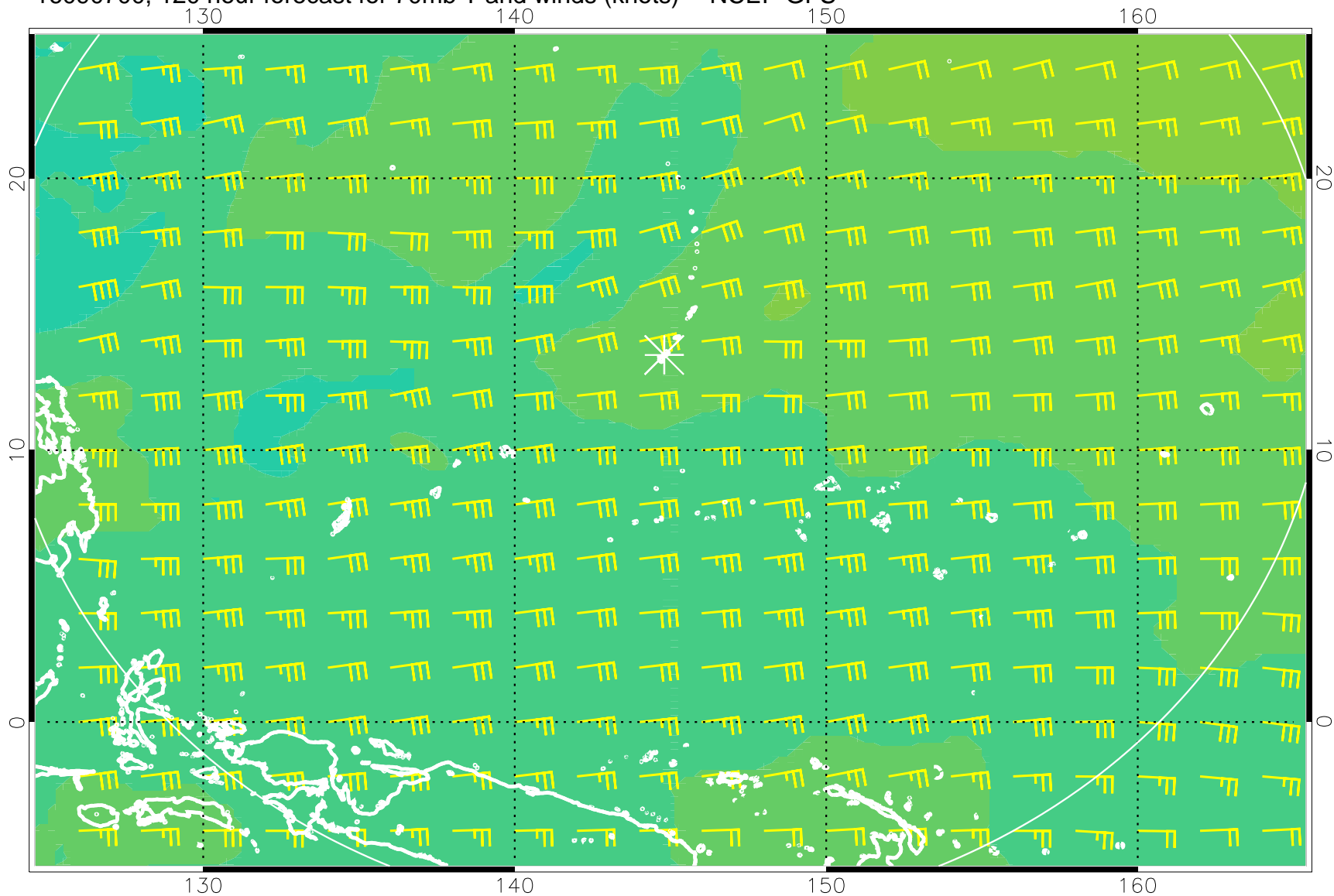
16090700, 120 hour forecast for 70mb T and winds (knots) -- NCEP GFS
