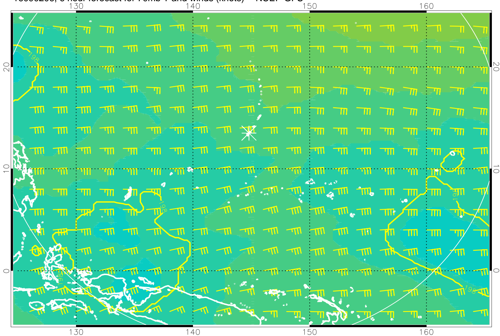
16090206, 6 hour forecast for 70mb T and winds (knots) -- NCEP GFS
