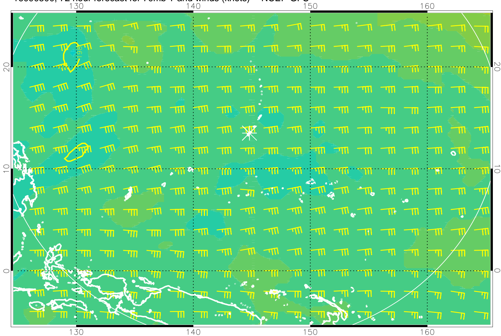
16090500, 72 hour forecast for 70mb T and winds (knots) -- NCEP GFS
