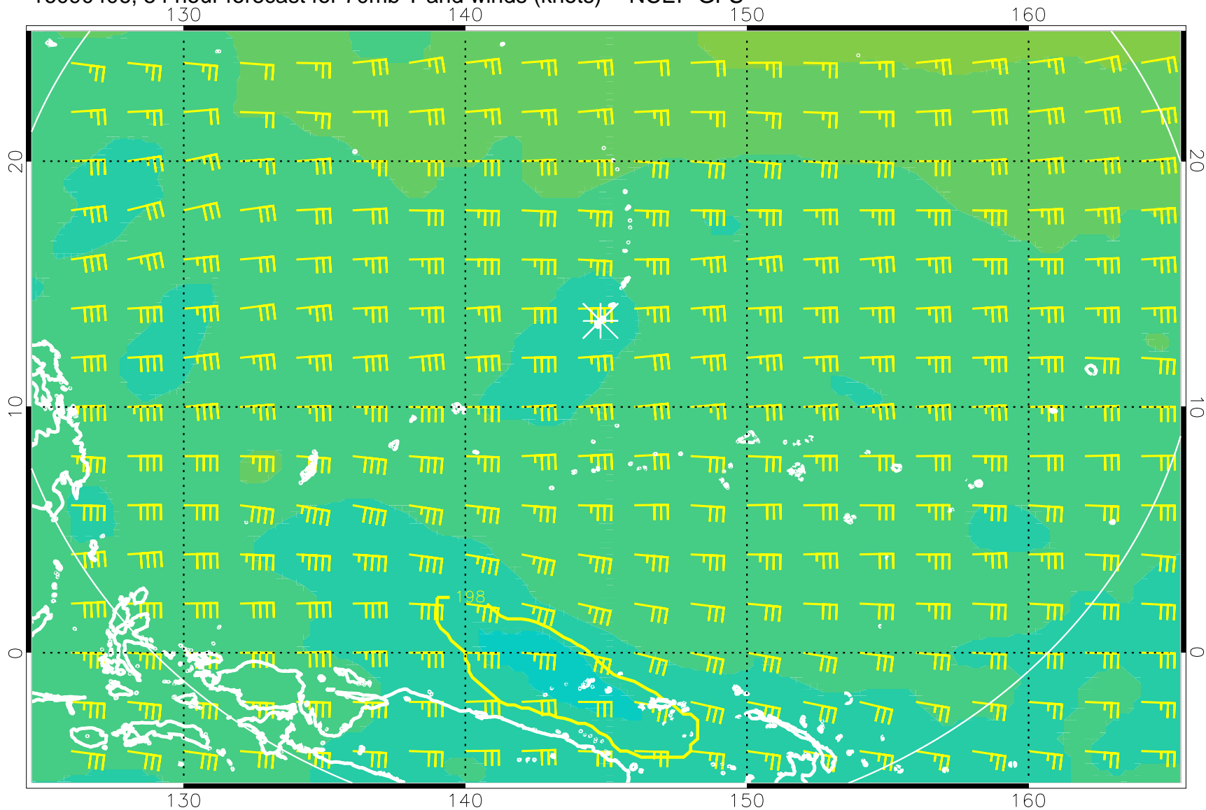
16090406, 54 hour forecast for 70mb T and winds (knots) -- NCEP GFS
