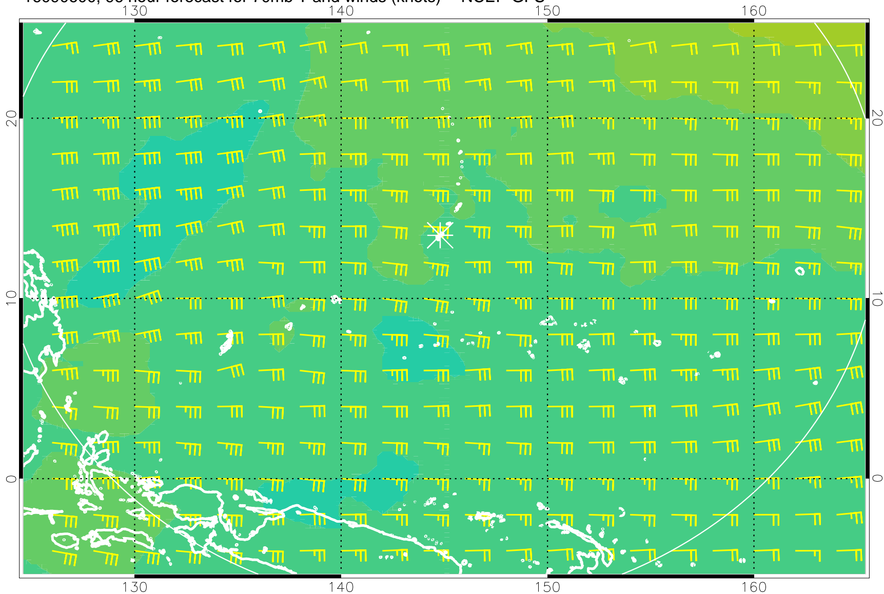
16090600, 96 hour forecast for 70mb T and winds (knots) -- NCEP GFS
