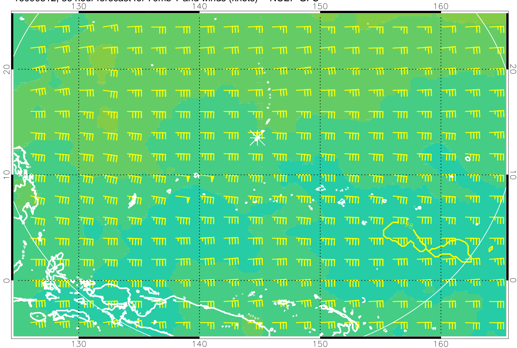
16090312, 36 hour forecast for 70mb T and winds (knots) -- NCEP GFS
