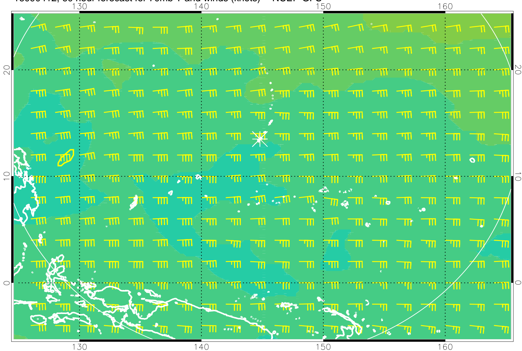
16090412, 60 hour forecast for 70mb T and winds (knots) -- NCEP GFS
