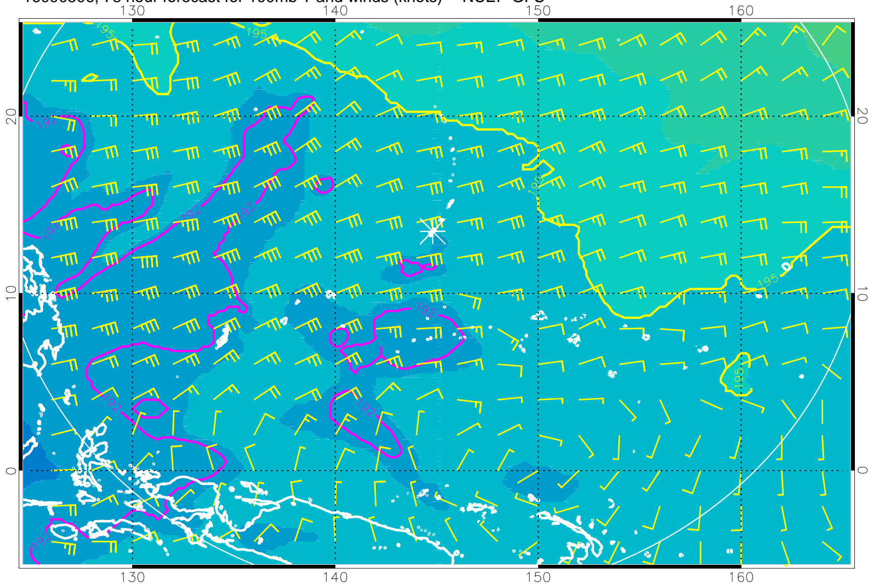
16090506, 78 hour forecast for 100mb T and winds (knots) -- NCEP GFS
