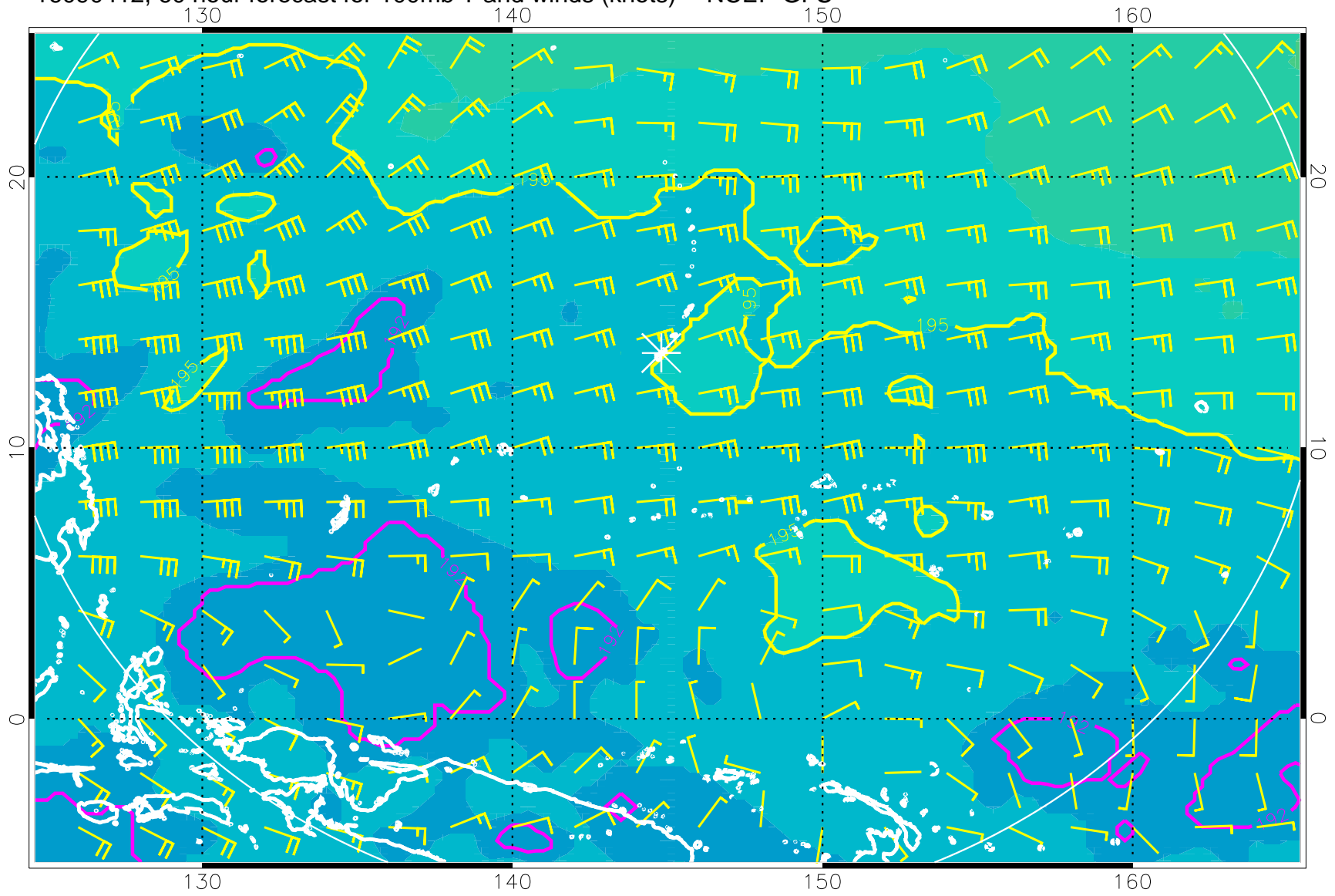
16090412, 60 hour forecast for 100mb T and winds (knots) -- NCEP GFS
