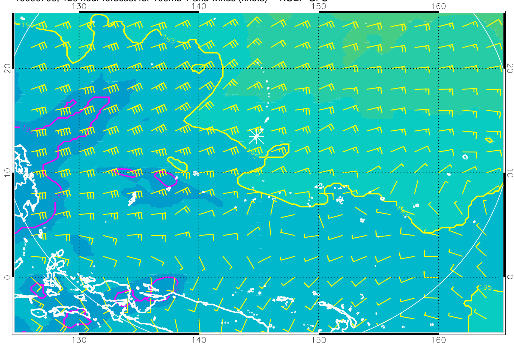
16090700, 120 hour forecast for 100mb T and winds (knots) -- NCEP GFS
