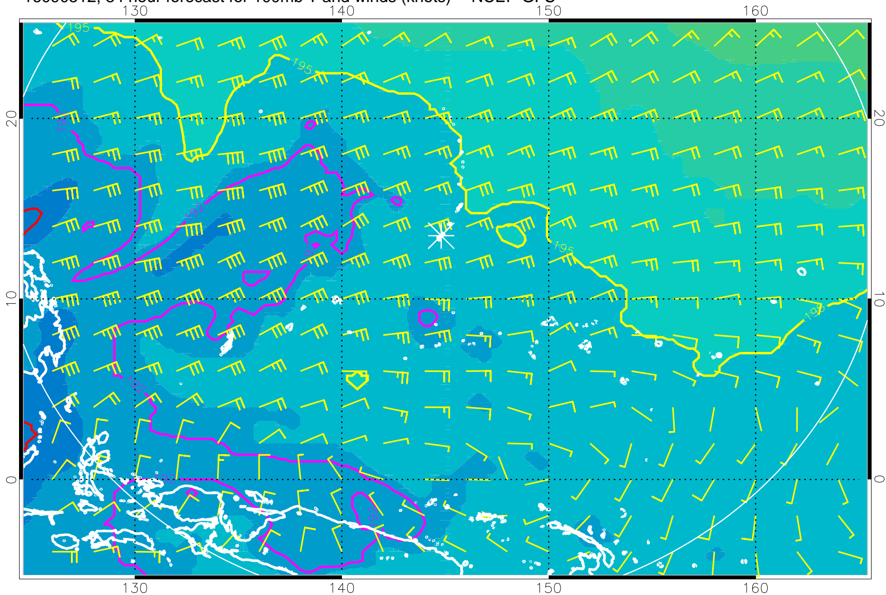
16090512, 84 hour forecast for 100mb T and winds (knots) -- NCEP GFS
