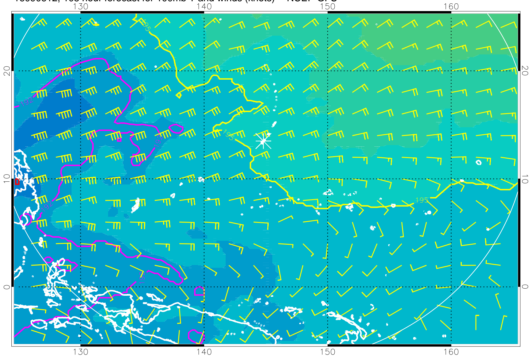
16090612, 108 hour forecast for 100mb T and winds (knots) -- NCEP GFS
