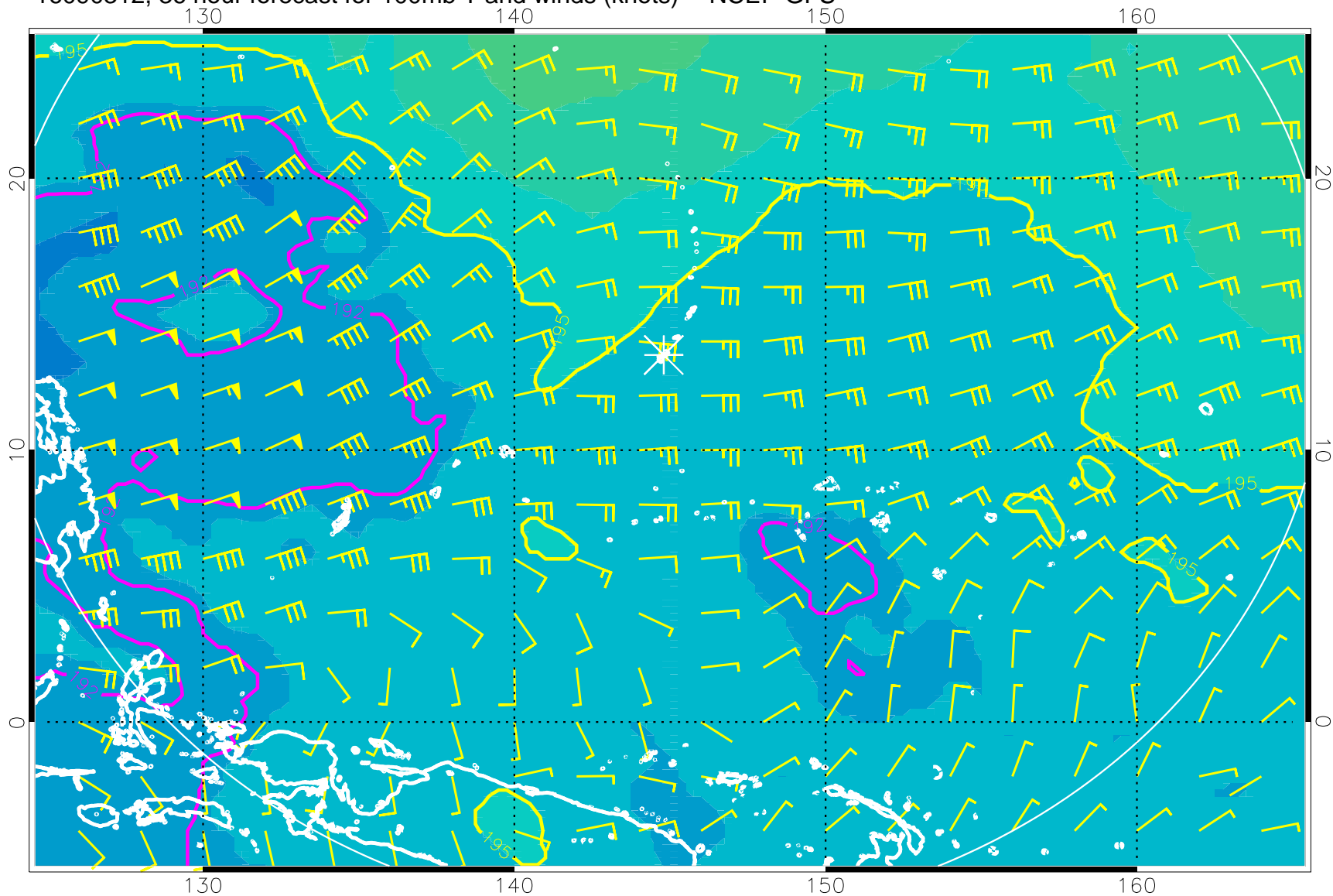
16090312, 36 hour forecast for 100mb T and winds (knots) -- NCEP GFS
