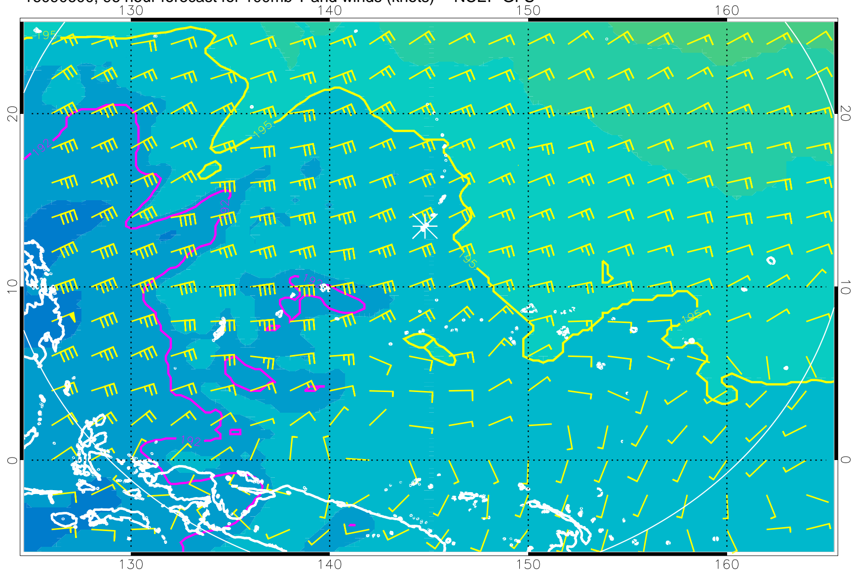
16090600, 96 hour forecast for 100mb T and winds (knots) -- NCEP GFS
