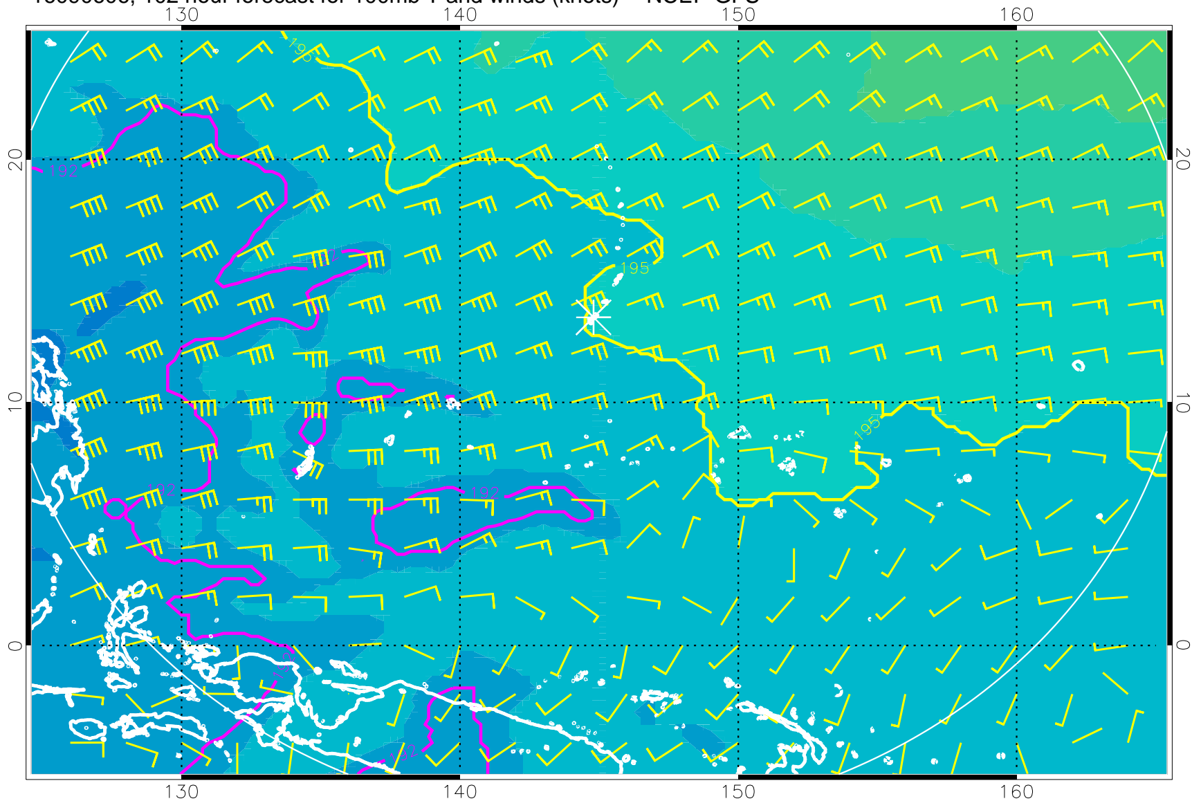
16090606, 102 hour forecast for 100mb T and winds (knots) -- NCEP GFS
