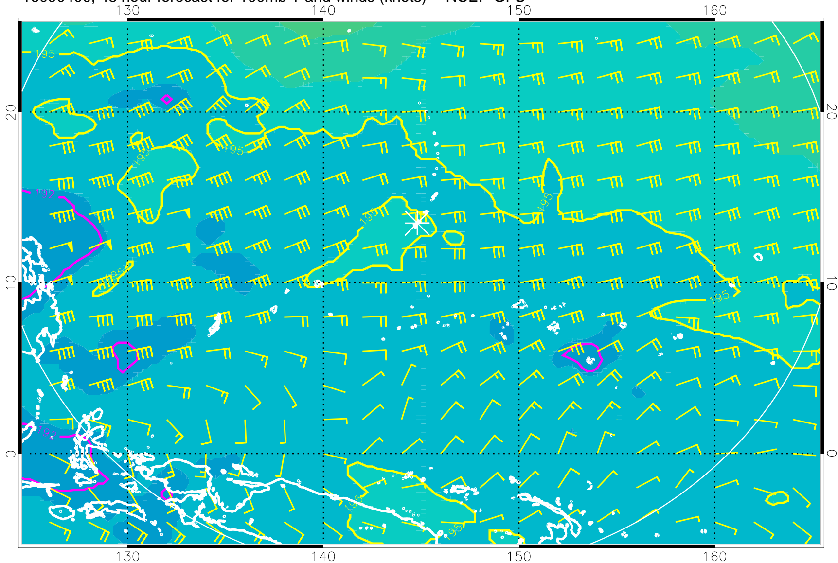
16090400, 48 hour forecast for 100mb T and winds (knots) -- NCEP GFS
