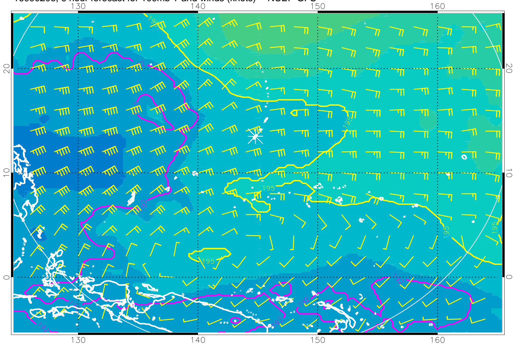
16090206, 6 hour forecast for 100mb T and winds (knots) -- NCEP GFS
