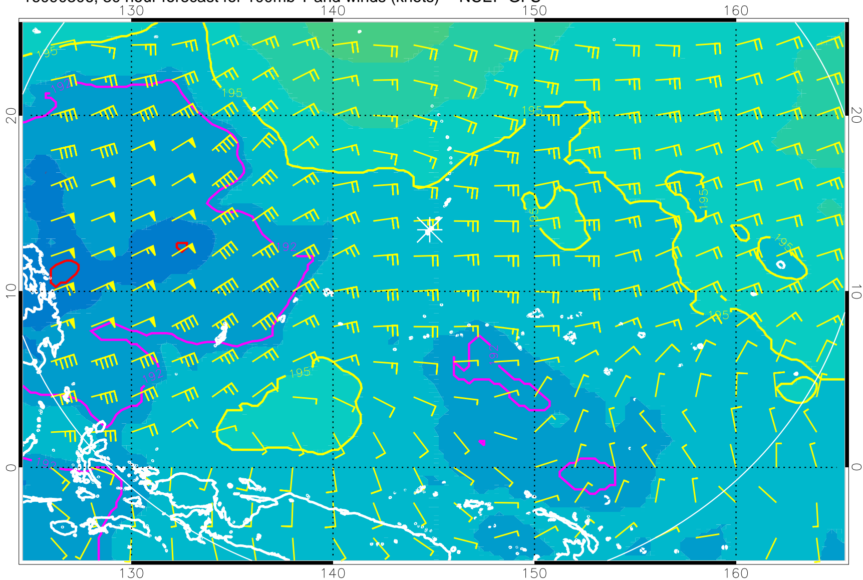
16090306, 30 hour forecast for 100mb T and winds (knots) -- NCEP GFS
