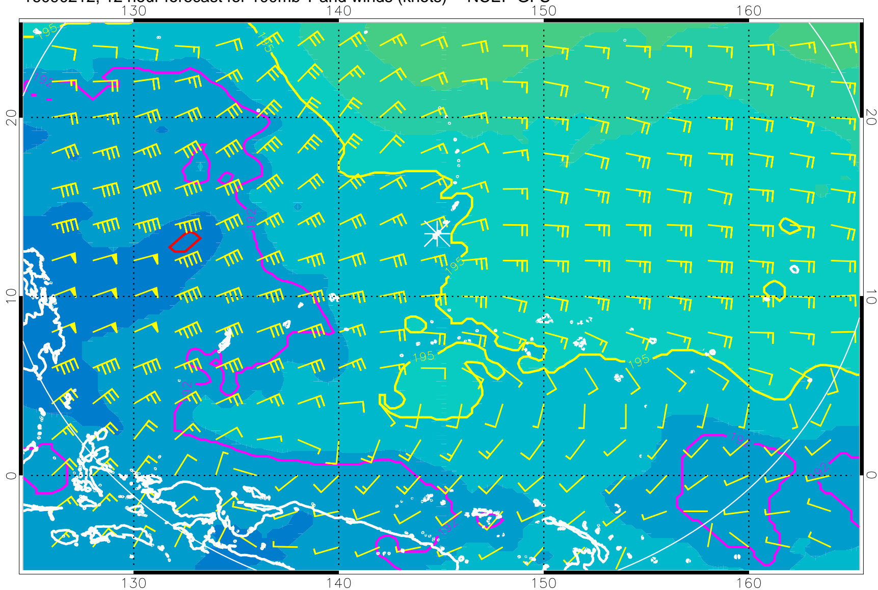
16090212, 12 hour forecast for 100mb T and winds (knots) -- NCEP GFS
