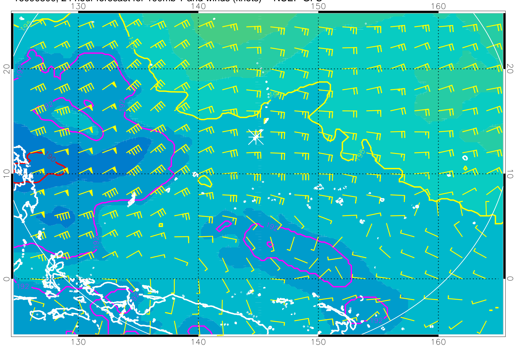
16090300, 24 hour forecast for 100mb T and winds (knots) -- NCEP GFS
