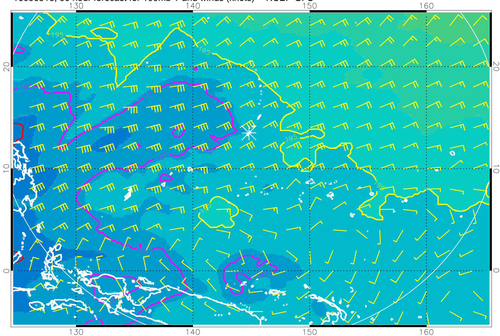
16090518, 90 hour forecast for 100mb T and winds (knots) -- NCEP GFS
