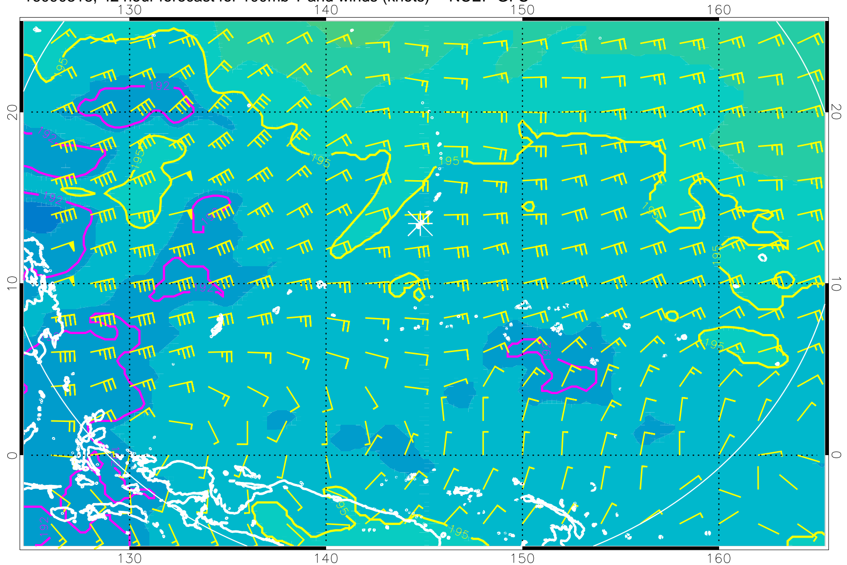
16090318, 42 hour forecast for 100mb T and winds (knots) -- NCEP GFS
