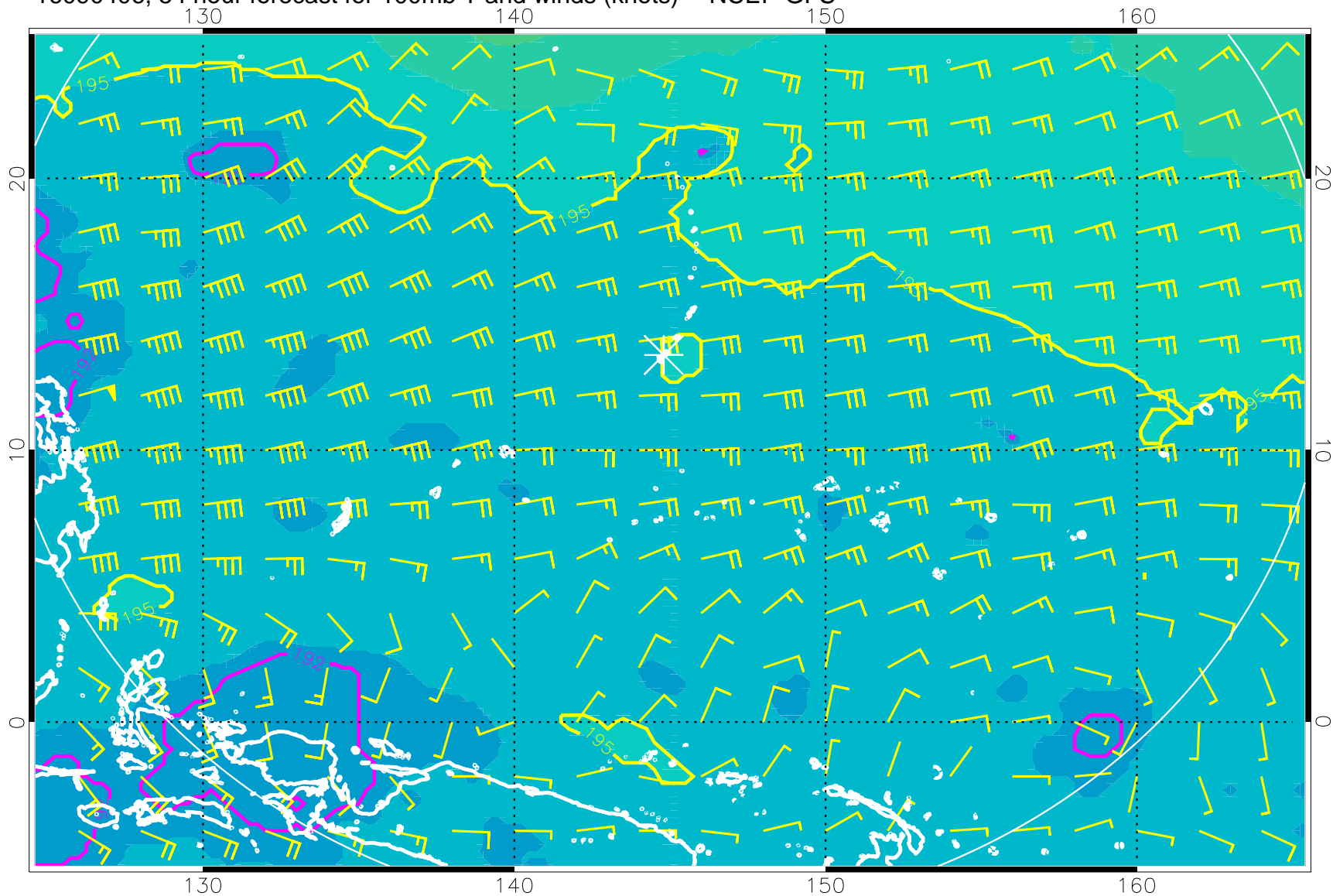
16090406, 54 hour forecast for 100mb T and winds (knots) -- NCEP GFS
