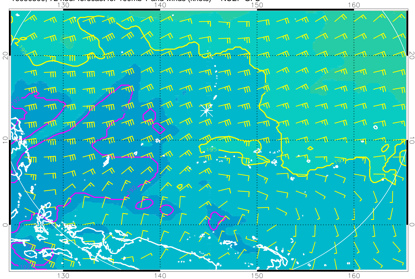
16090500, 72 hour forecast for 100mb T and winds (knots) -- NCEP GFS
