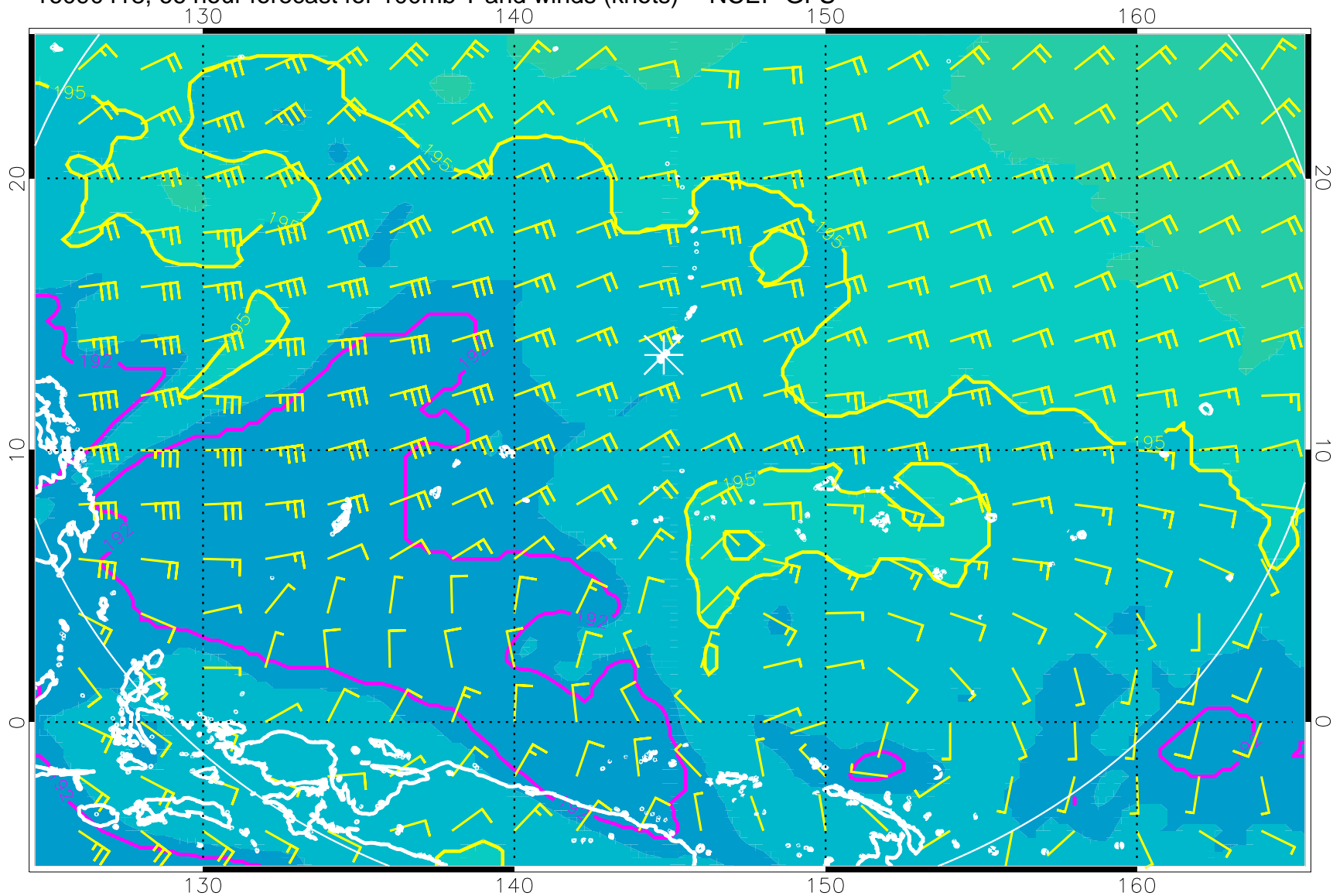
16090418, 66 hour forecast for 100mb T and winds (knots) -- NCEP GFS
