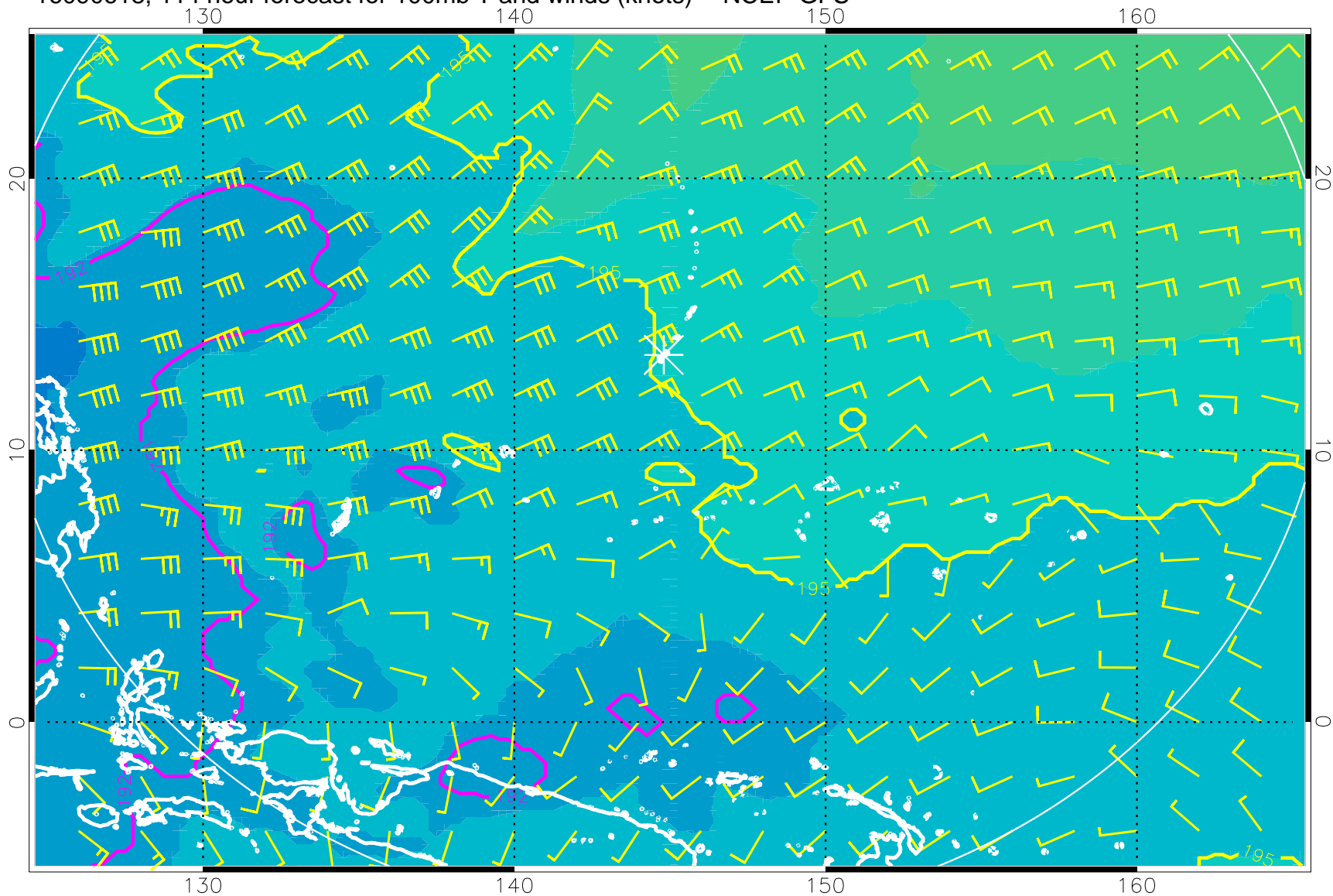
16090618, 114 hour forecast for 100mb T and winds (knots) -- NCEP GFS
