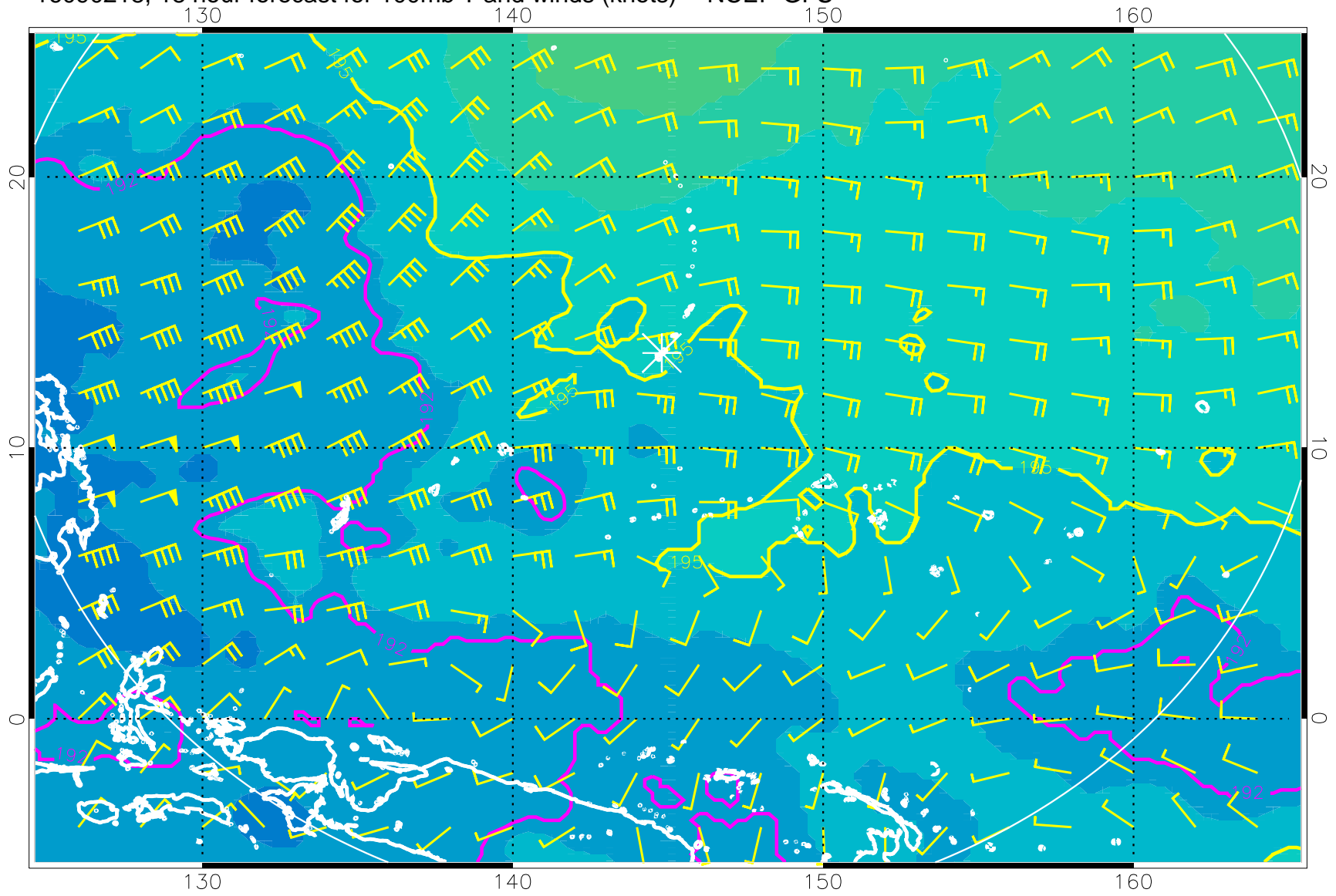
16090218, 18 hour forecast for 100mb T and winds (knots) -- NCEP GFS
