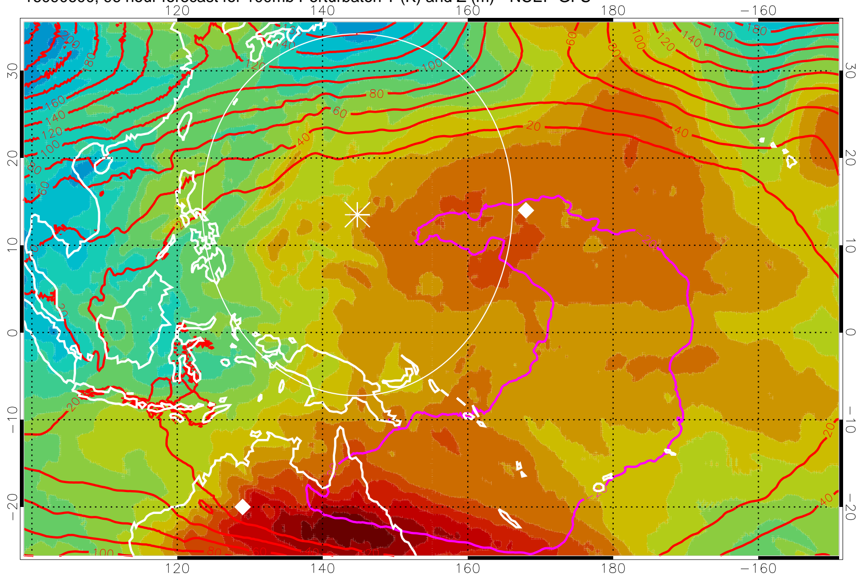
16090600, 96 hour forecast for 100mb Perturbaton T (K) and Z (m)-- NCEP GFS
