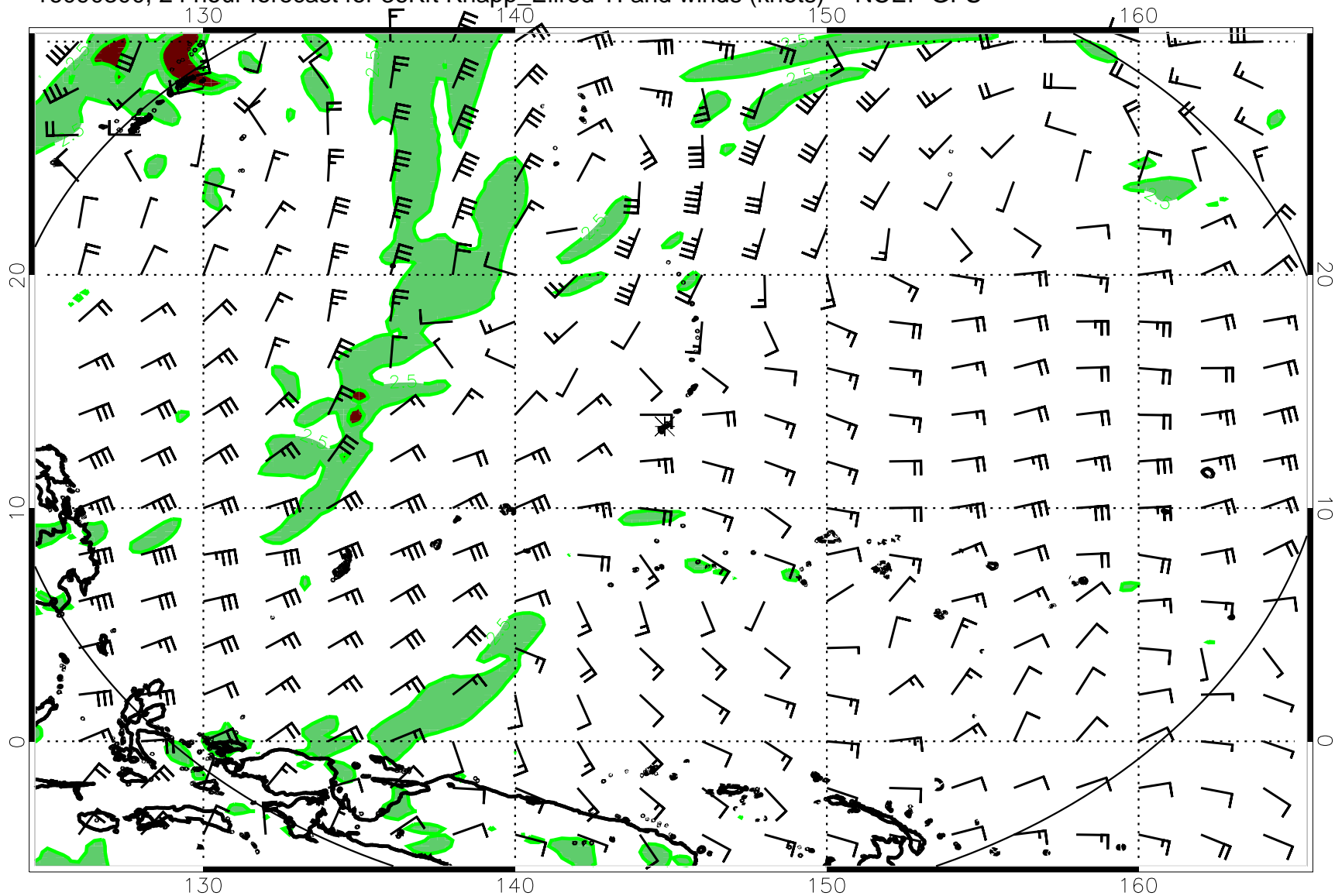
16090300, 24 hour forecast for 36Kft Knapp_Ellrod TI and winds (knots) -- NCEP GFS
