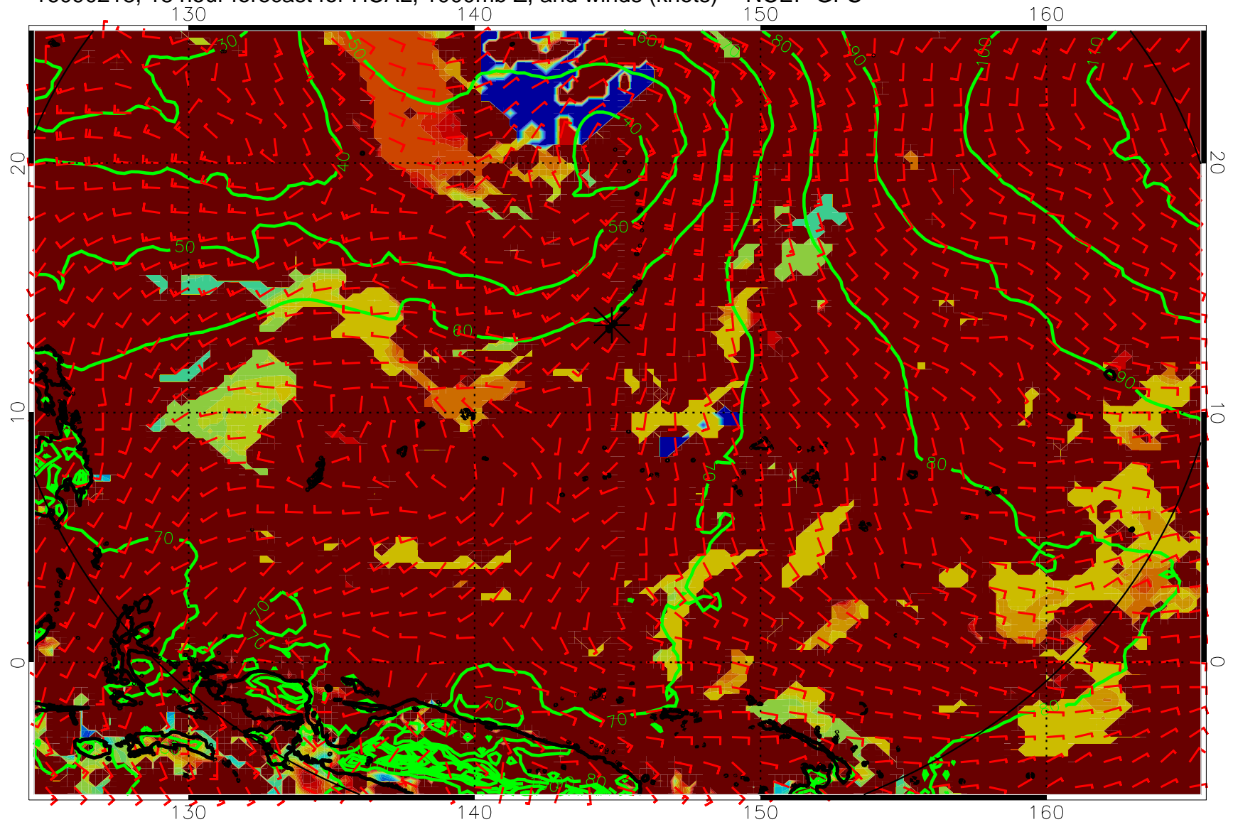
16090218, 18 hour forecast for HCAL, 1000mb Z, and winds (knots) -- NCEP GFS
