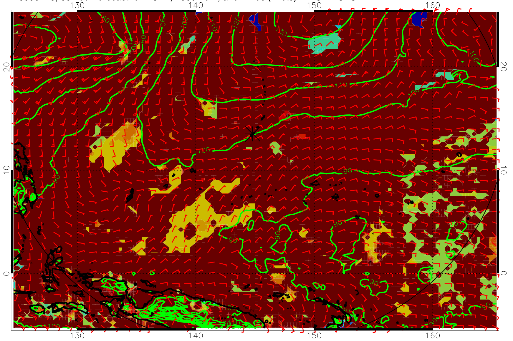
16090418, 66 hour forecast for HCAL, 1000mb Z, and winds (knots) -- NCEP GFS
