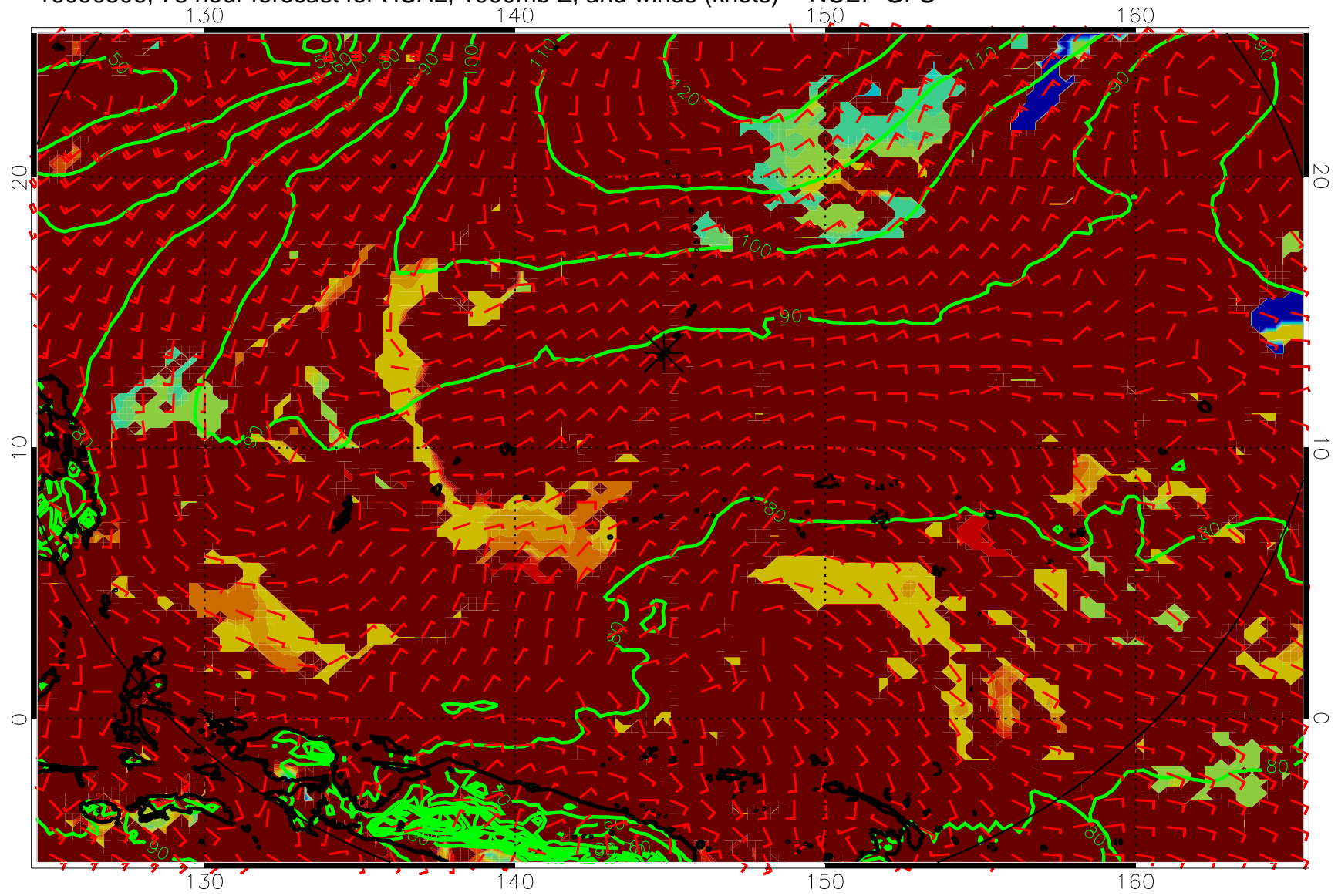
16090506, 78 hour forecast for HCAL, 1000mb Z, and winds (knots) -- NCEP GFS
