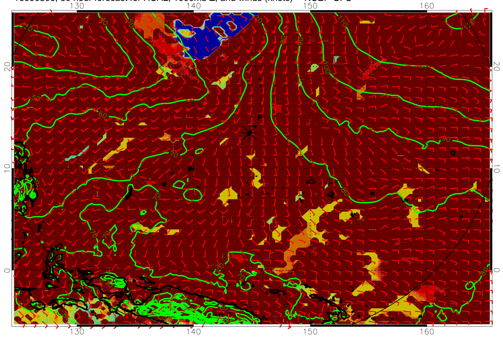
16090306, 30 hour forecast for HCAL, 1000mb Z, and winds (knots) -- NCEP GFS
