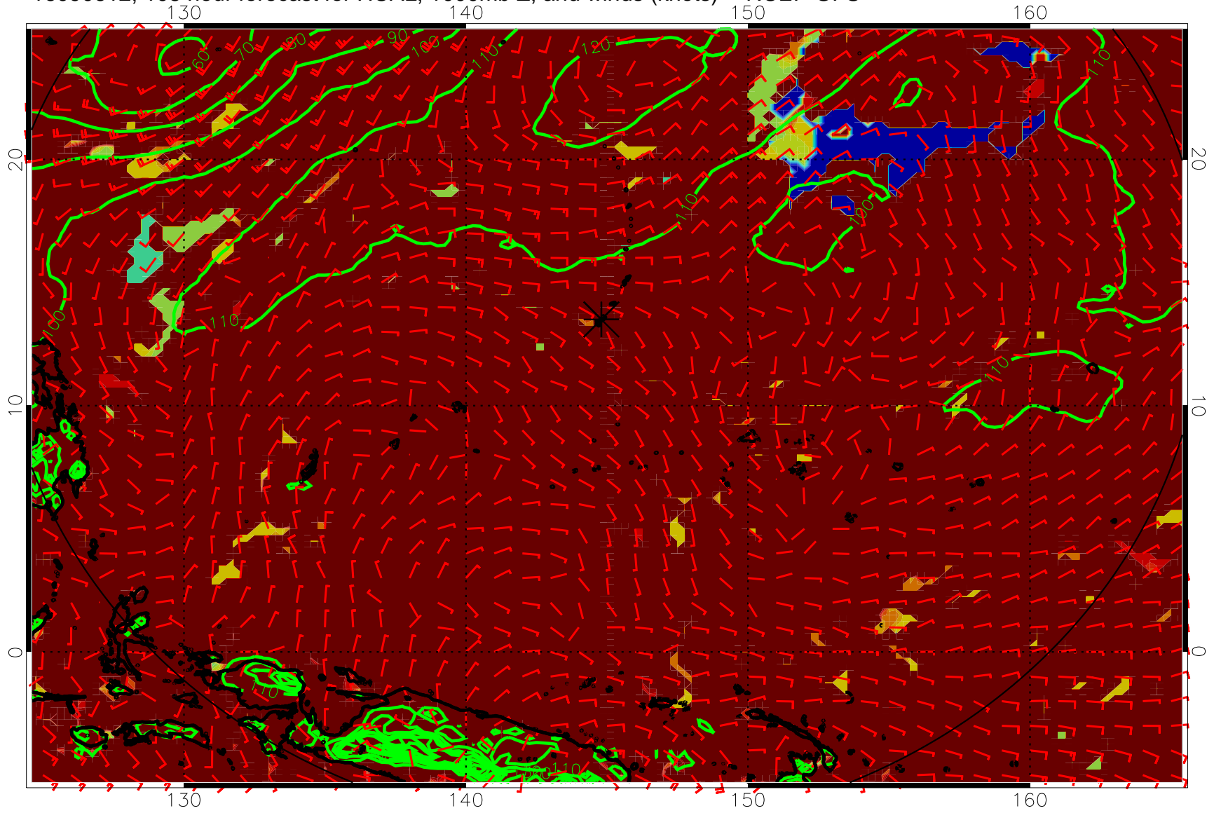
16090612, 108 hour forecast for HCAL, 1000mb Z, and winds (knots) -- NCEP GFS
