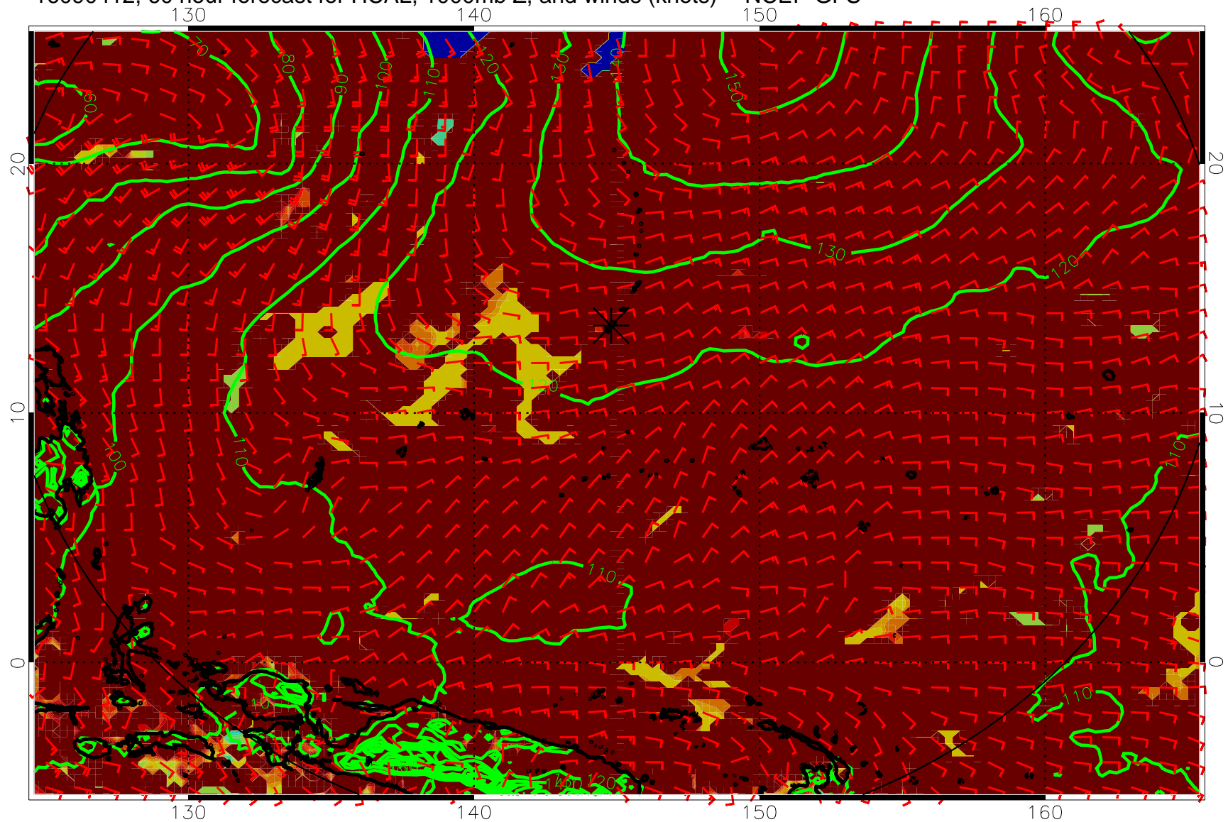
16090412, 60 hour forecast for HCAL, 1000mb Z, and winds (knots) -- NCEP GFS
