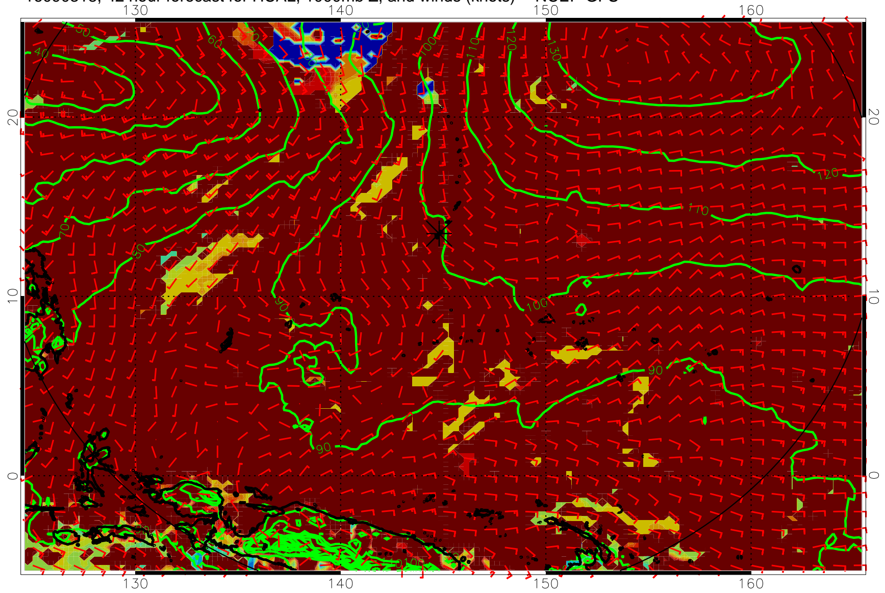
16090318, 42 hour forecast for HCAL, 1000mb Z, and winds (knots) -- NCEP GFS
