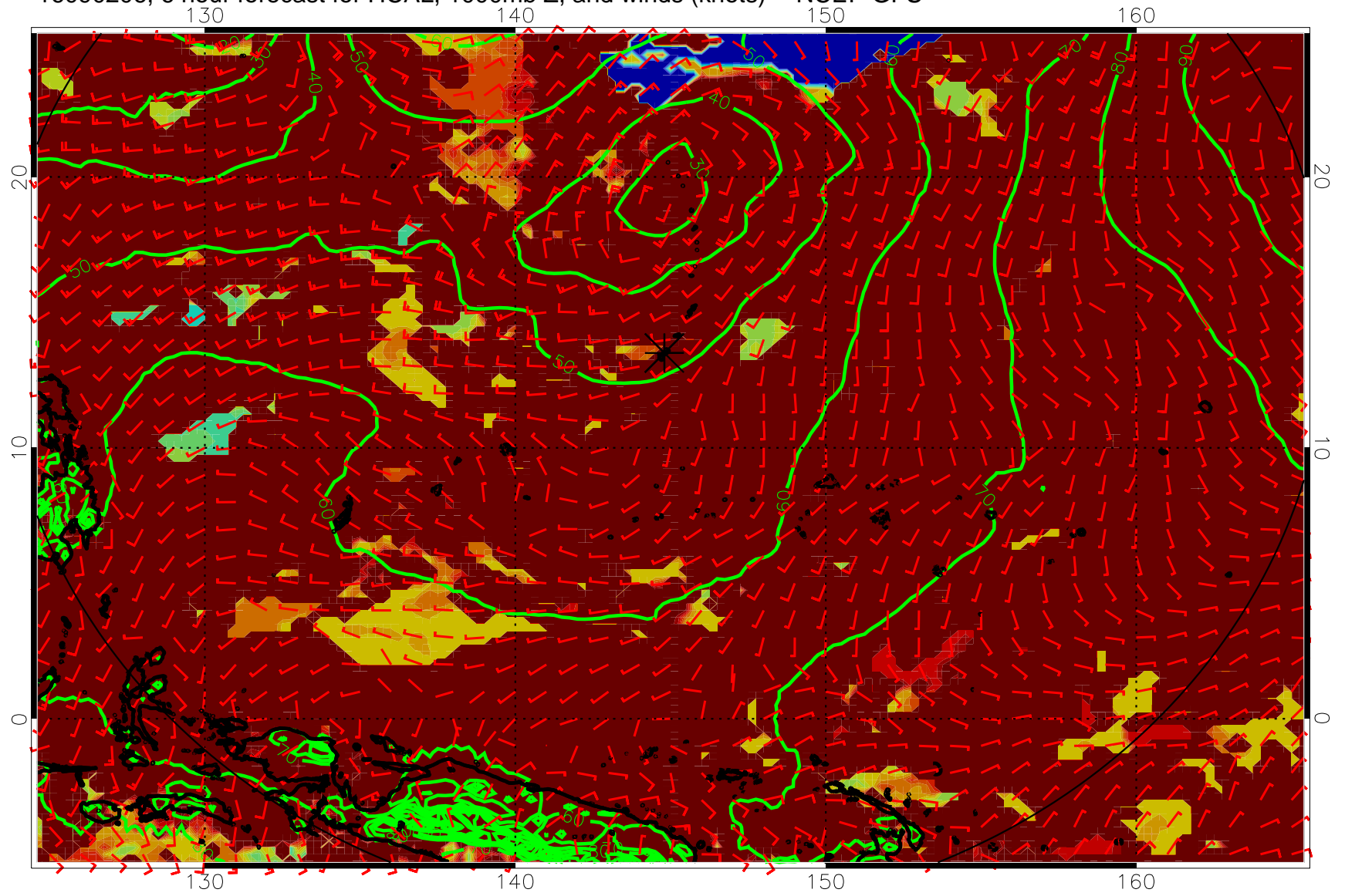
16090206, 6 hour forecast for HCAL, 1000mb Z, and winds (knots) -- NCEP GFS
