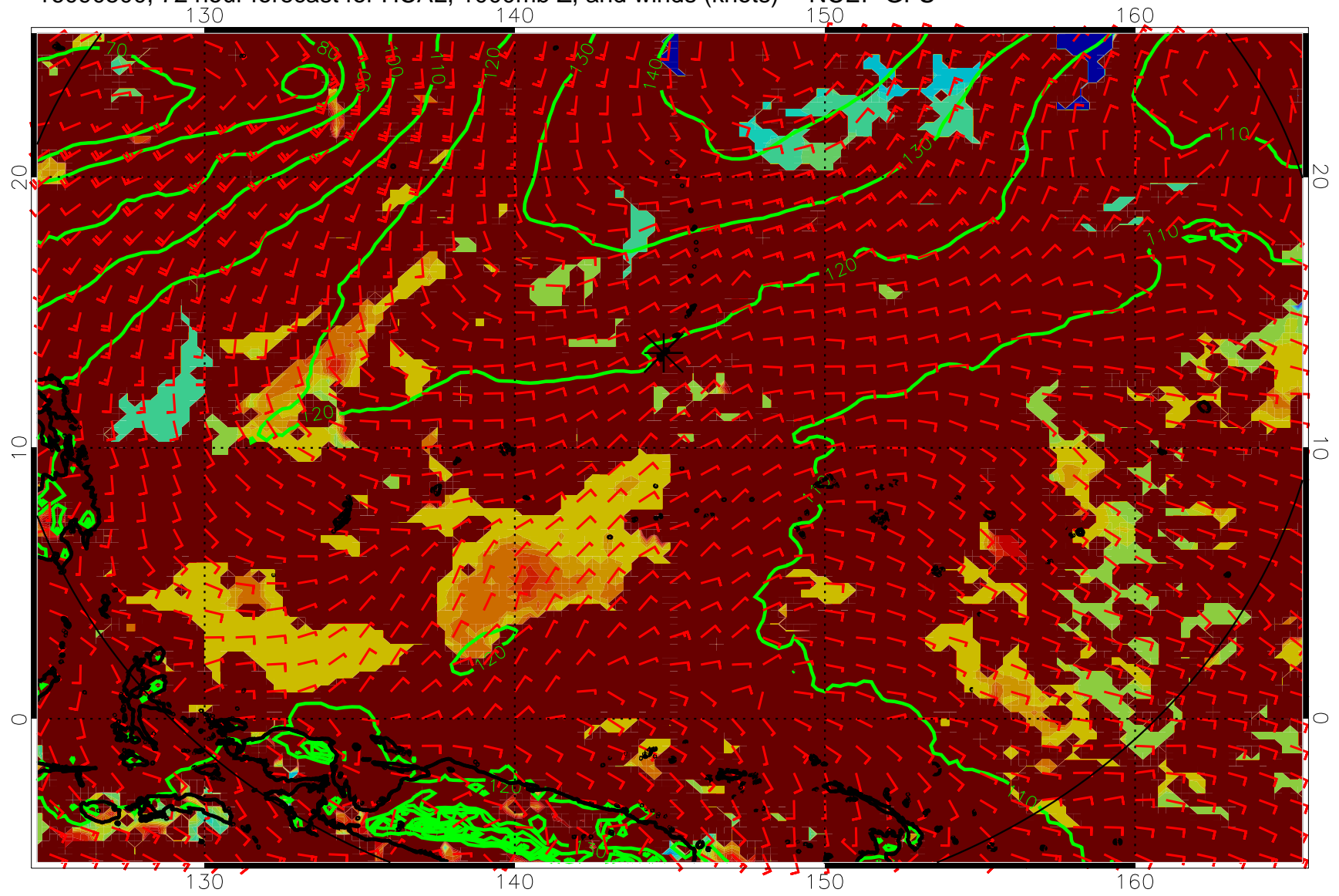
16090500, 72 hour forecast for HCAL, 1000mb Z, and winds (knots) -- NCEP GFS
