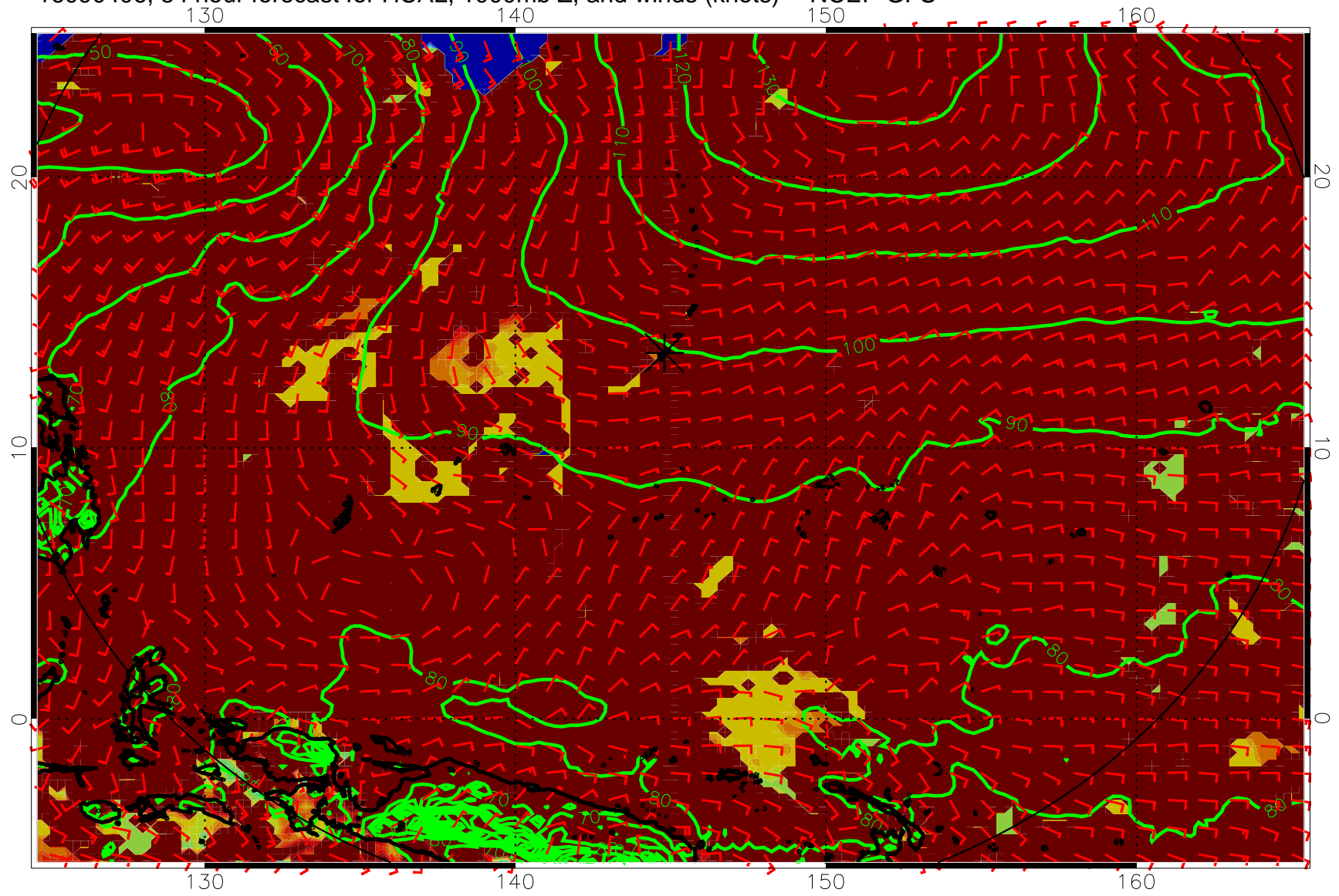
16090406, 54 hour forecast for HCAL, 1000mb Z, and winds (knots) -- NCEP GFS
