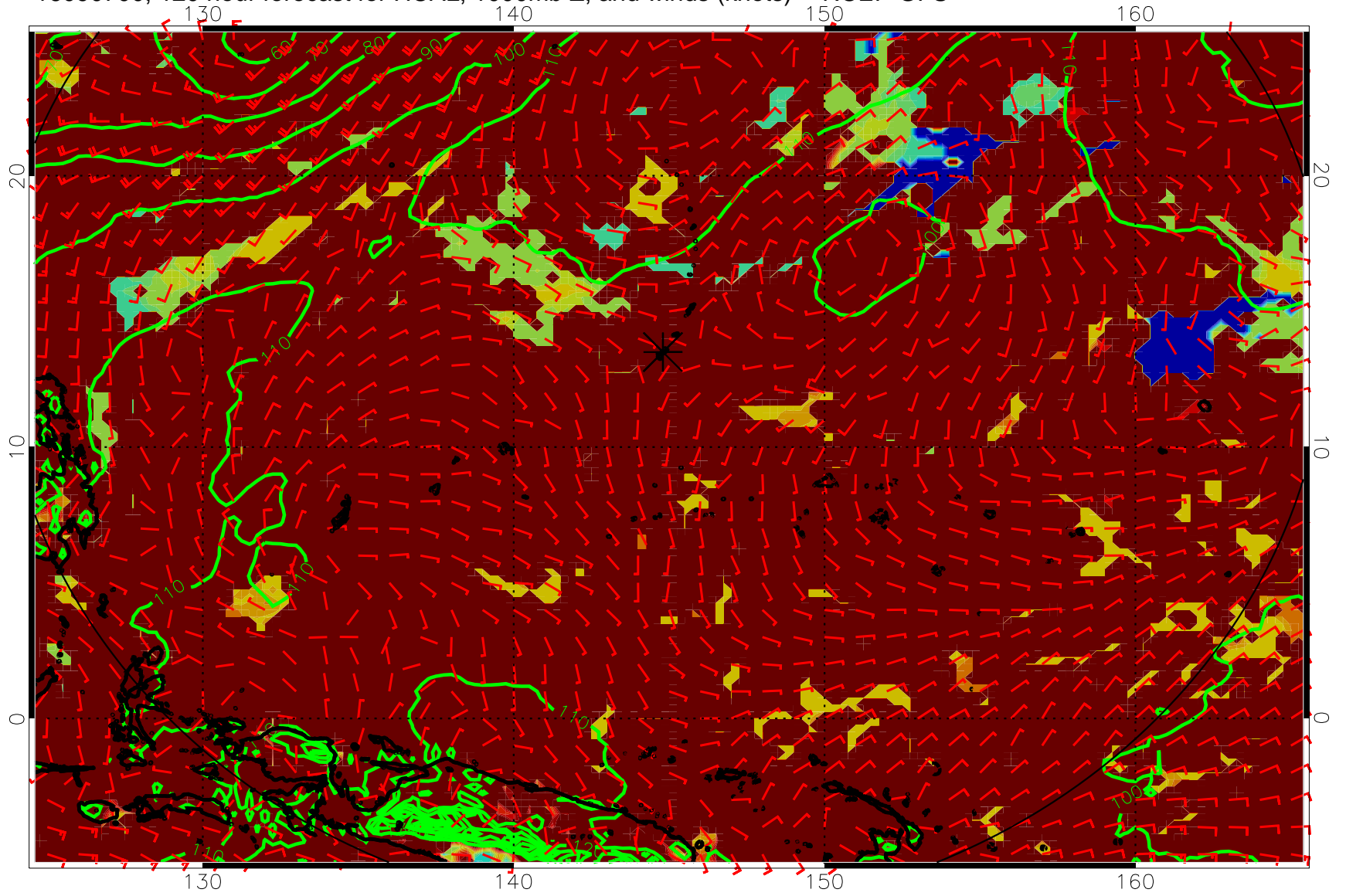
16090700, 120 hour forecast for HCAL, 1000mb Z, and winds (knots) -- NCEP GFS
