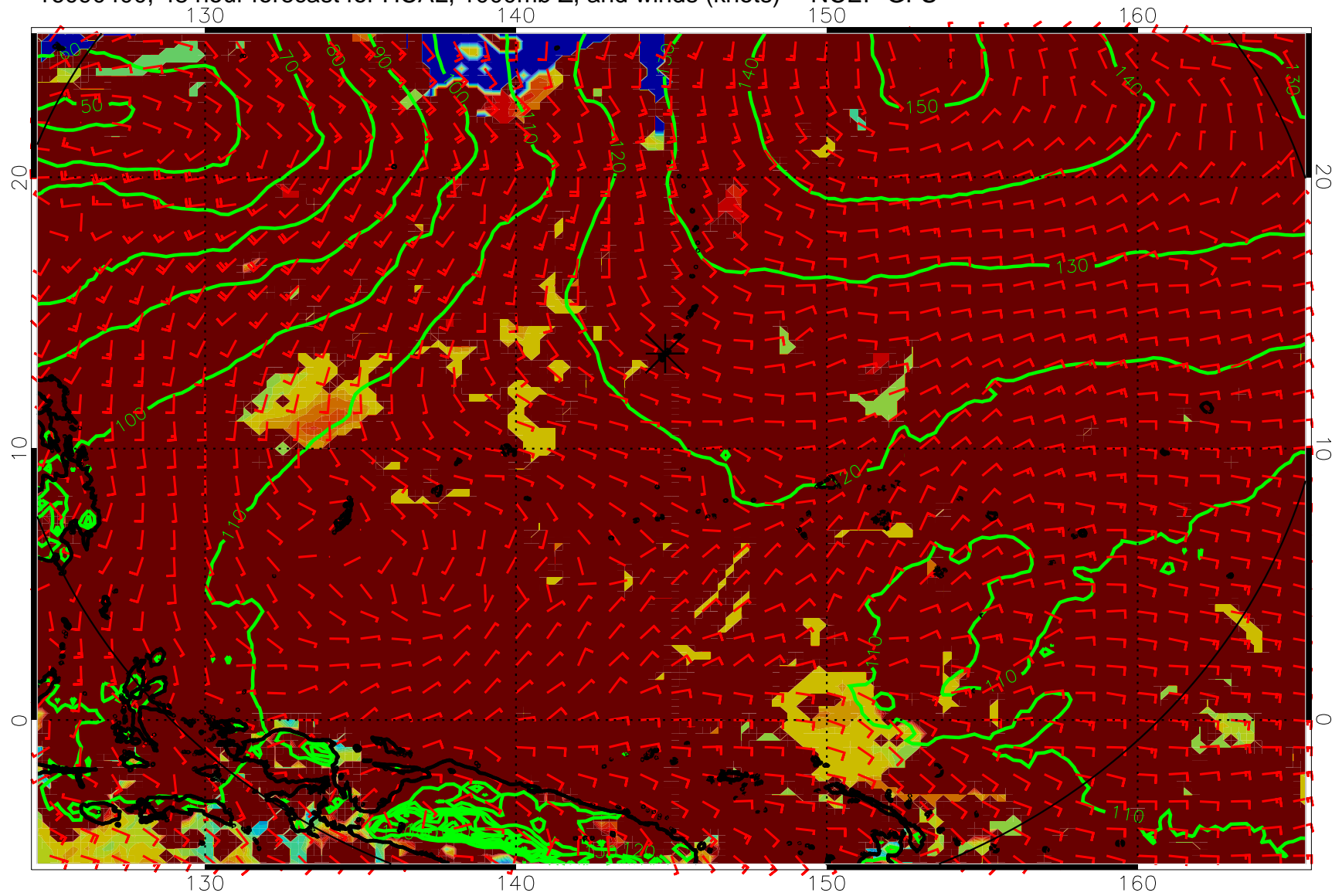
16090400, 48 hour forecast for HCAL, 1000mb Z, and winds (knots) -- NCEP GFS
