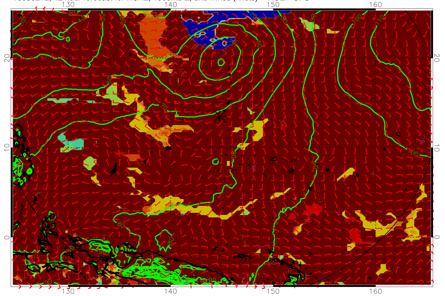
16090212, 12 hour forecast for HCAL, 1000mb Z, and winds (knots) -- NCEP GFS
