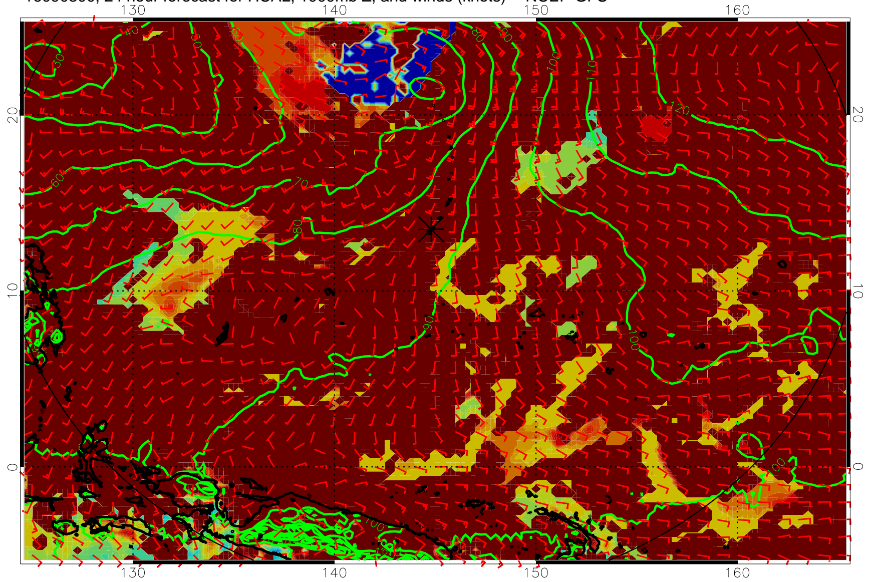
16090300, 24 hour forecast for HCAL, 1000mb Z, and winds (knots) -- NCEP GFS
