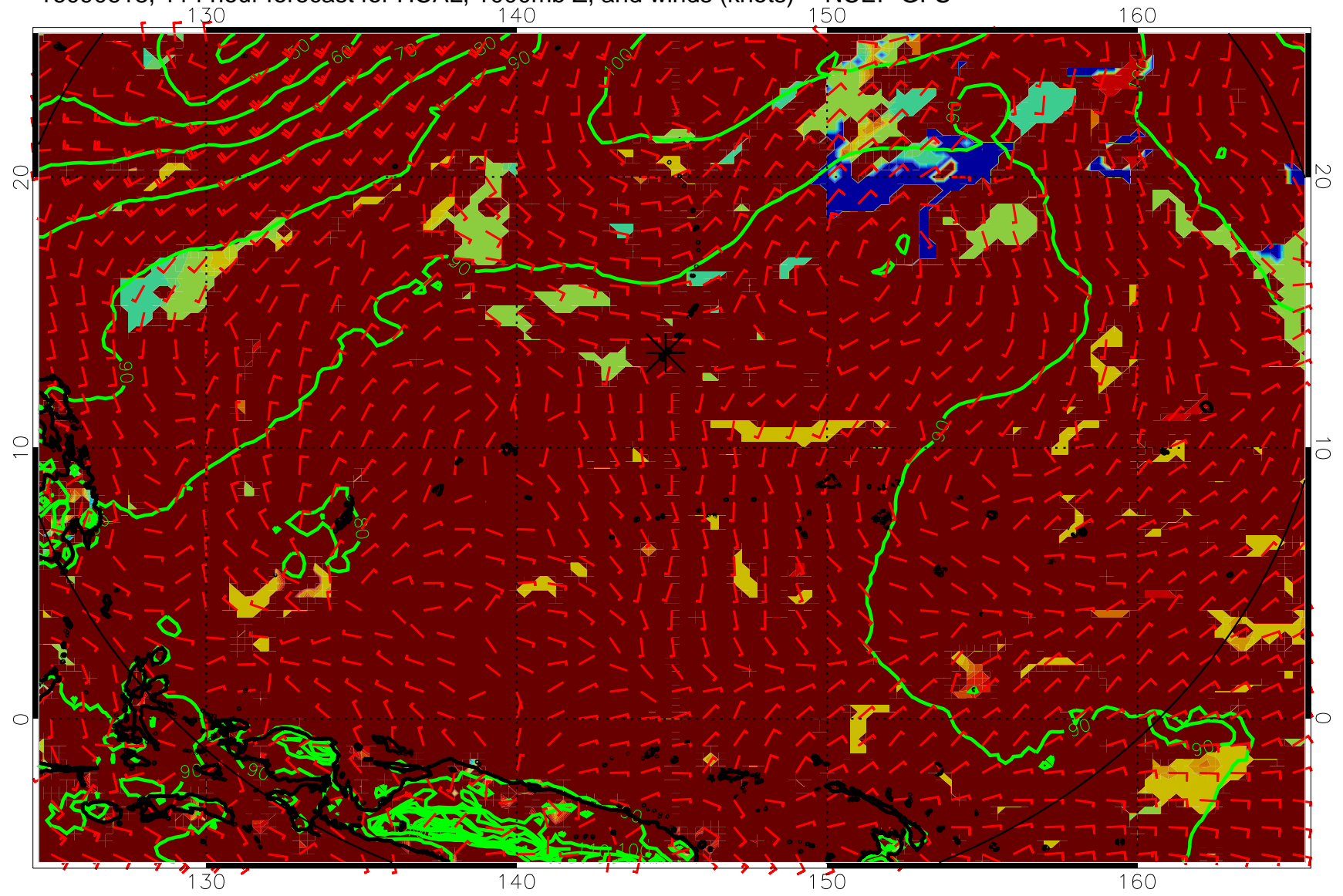
16090618, 114 hour forecast for HCAL, 1000mb Z, and winds (knots) -- NCEP GFS
