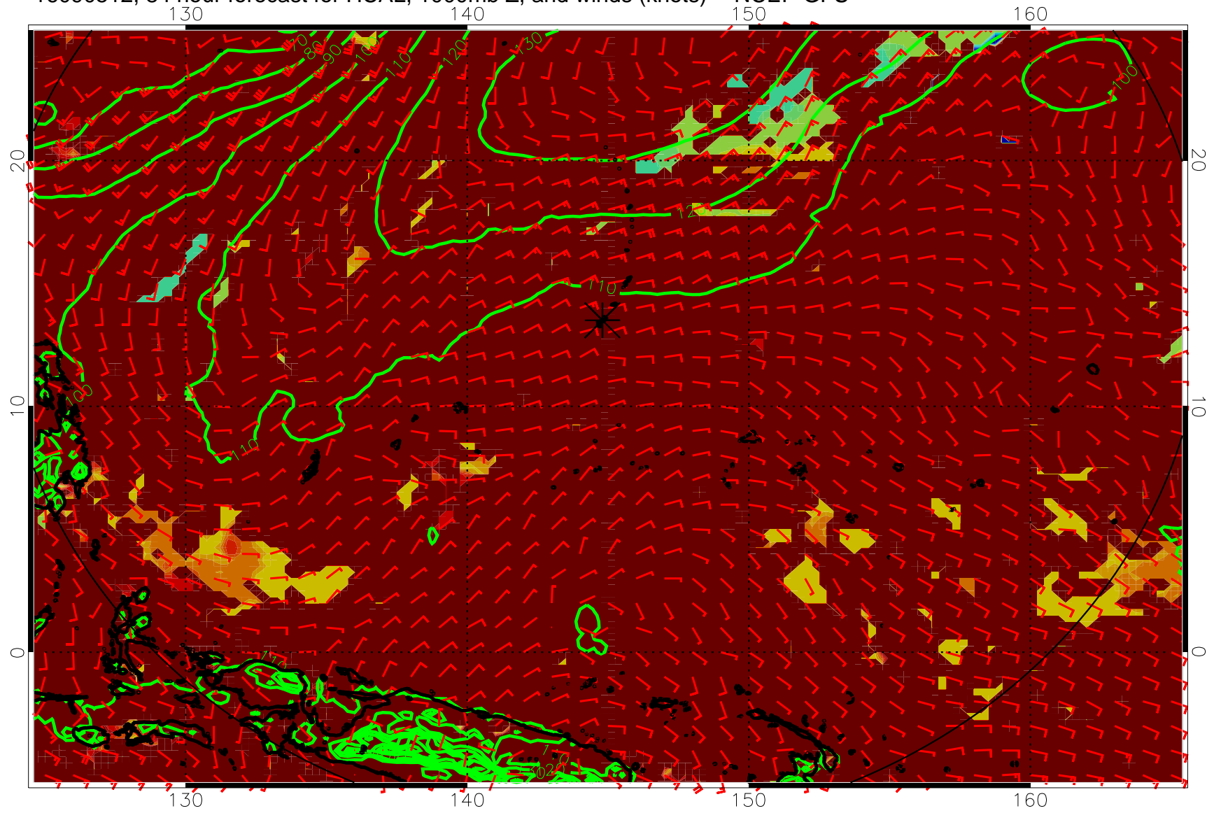
16090512, 84 hour forecast for HCAL, 1000mb Z, and winds (knots) -- NCEP GFS
