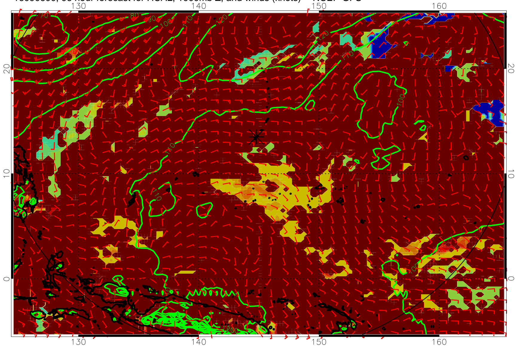
16090600, 96 hour forecast for HCAL, 1000mb Z, and winds (knots) -- NCEP GFS
