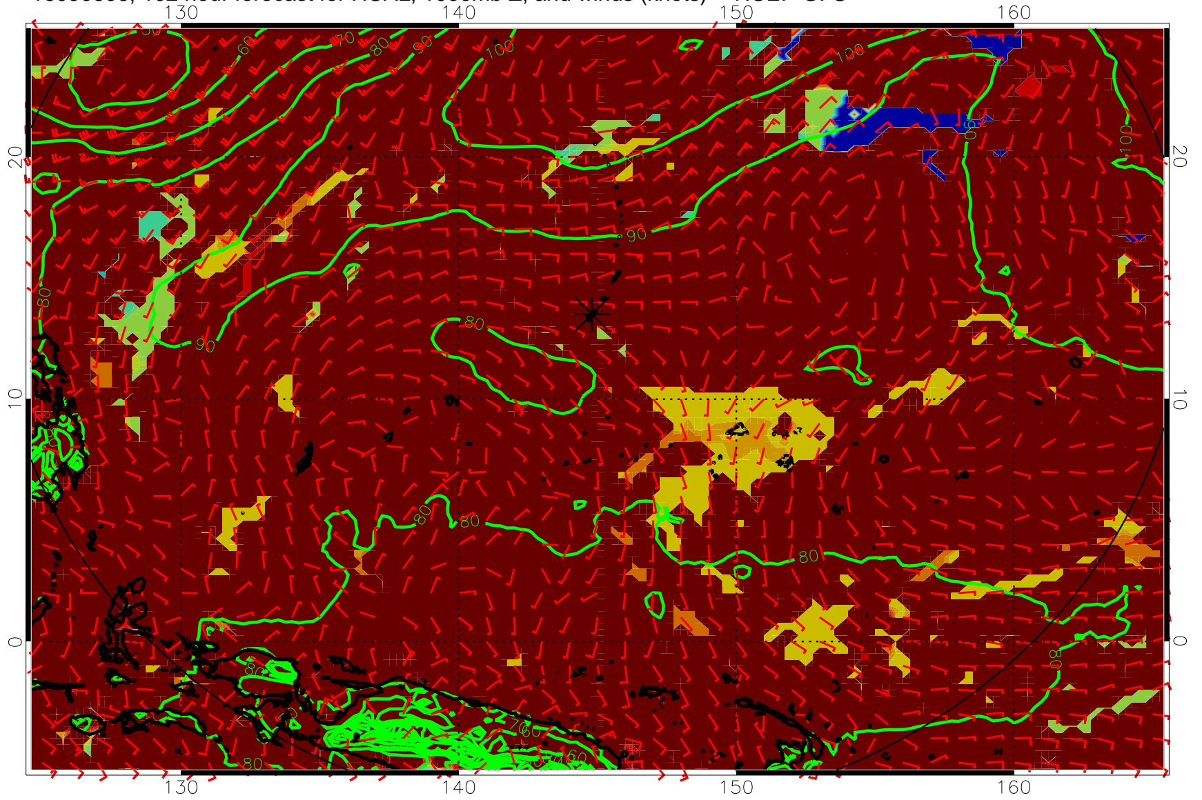
16090606, 102 hour forecast for HCAL, 1000mb Z, and winds (knots) -- NCEP GFS
