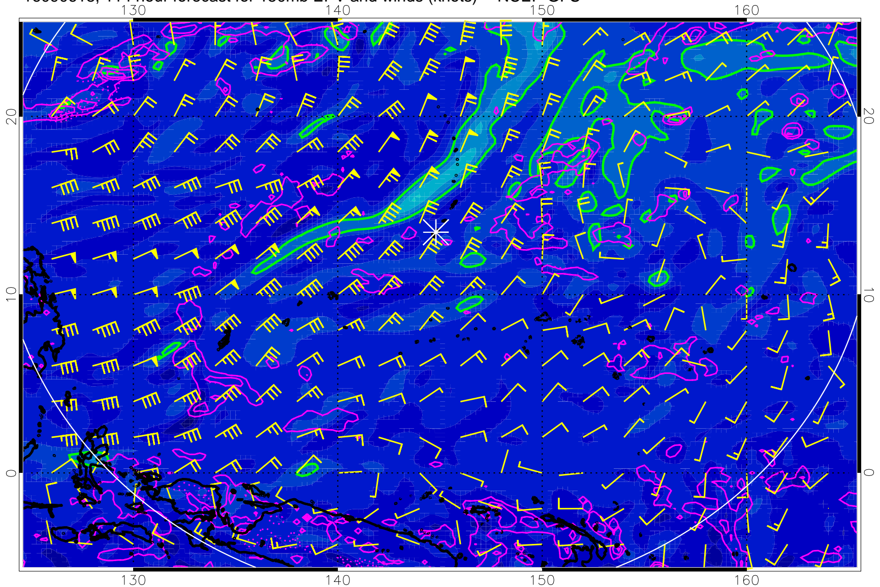
16090618, 114 hour forecast for 150mb EPV and winds (knots) -- NCEP GFS
