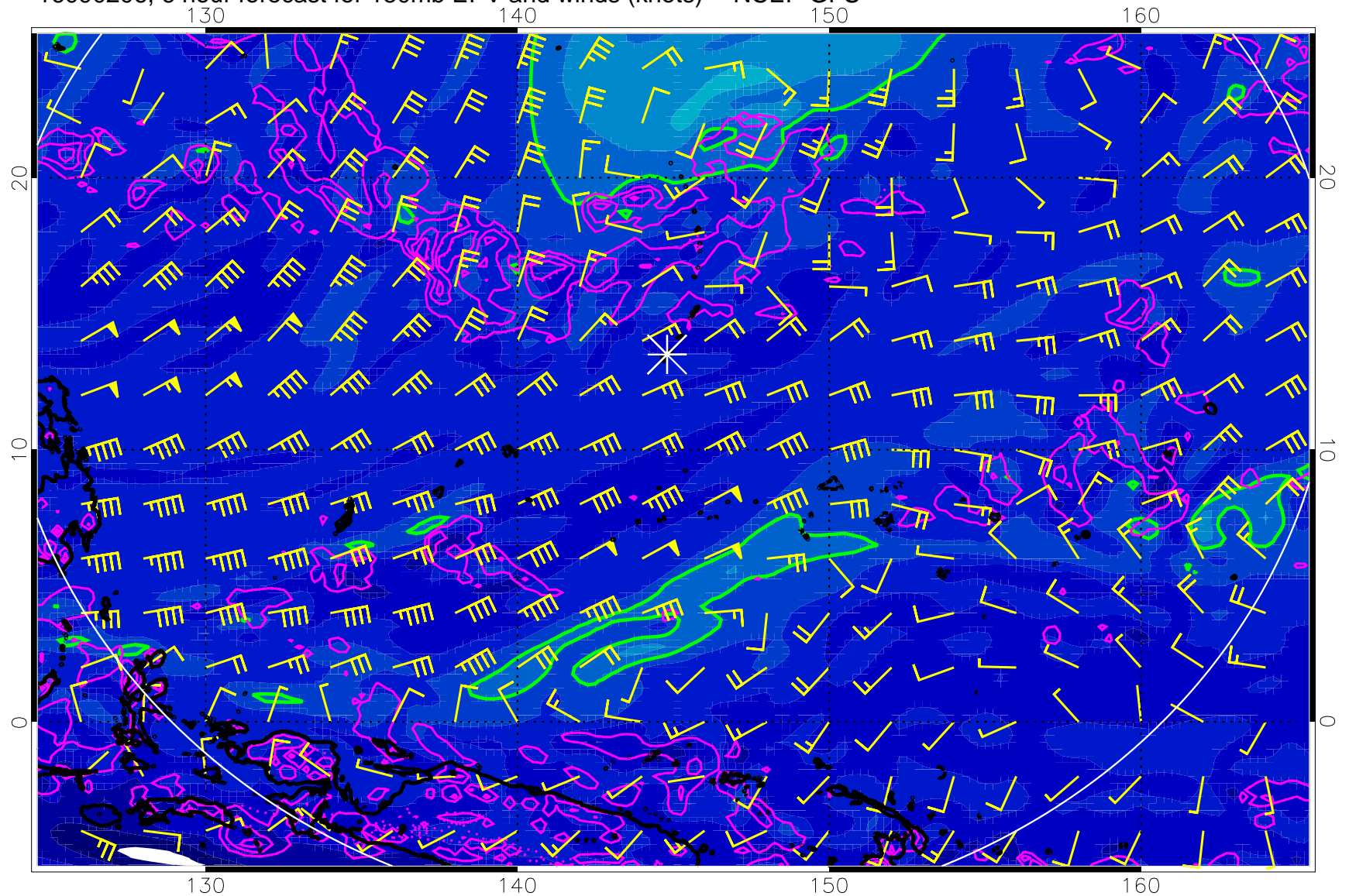
16090206, 6 hour forecast for 150mb EPV and winds (knots) -- NCEP GFS
