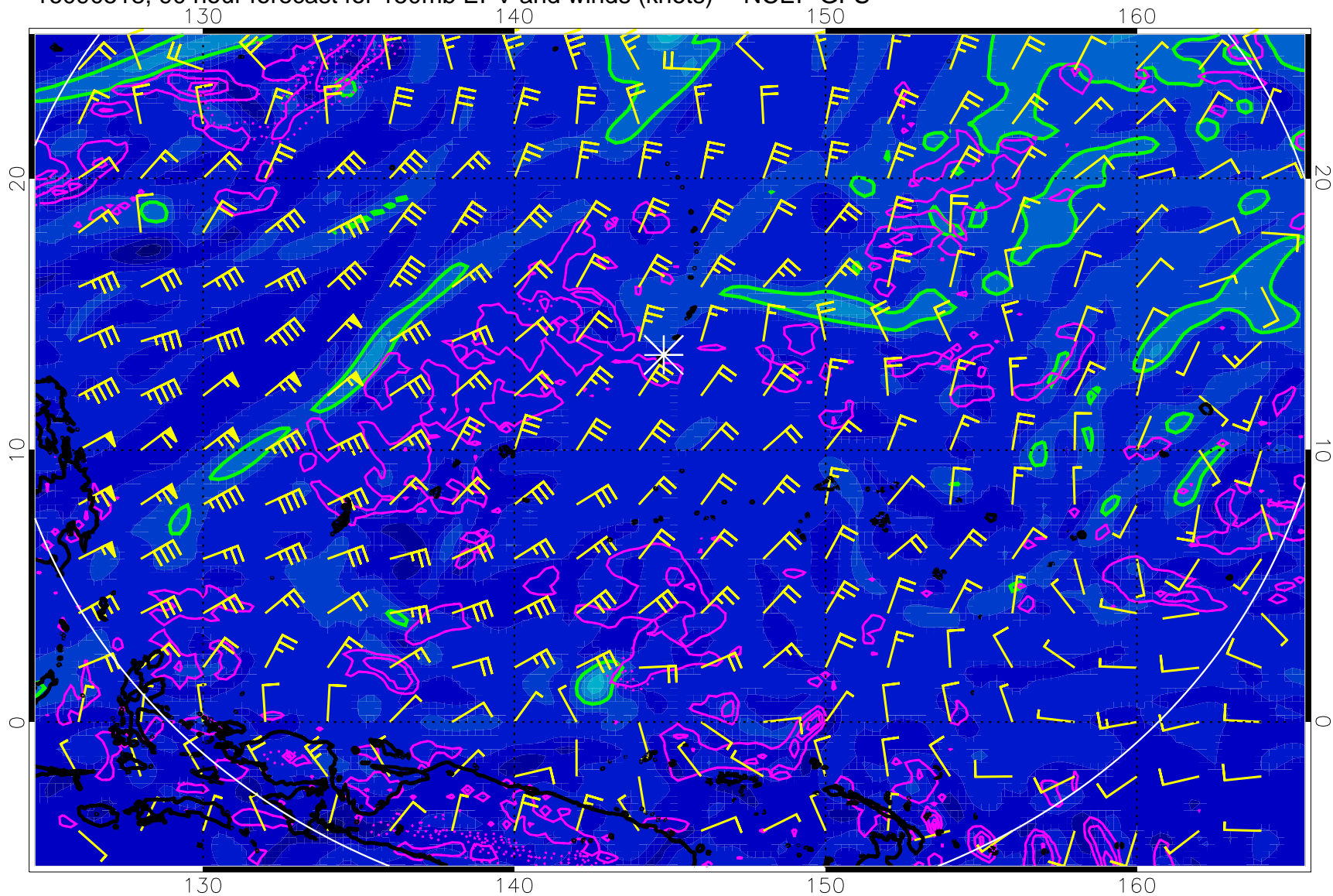
16090518, 90 hour forecast for 150mb EPV and winds (knots) -- NCEP GFS
