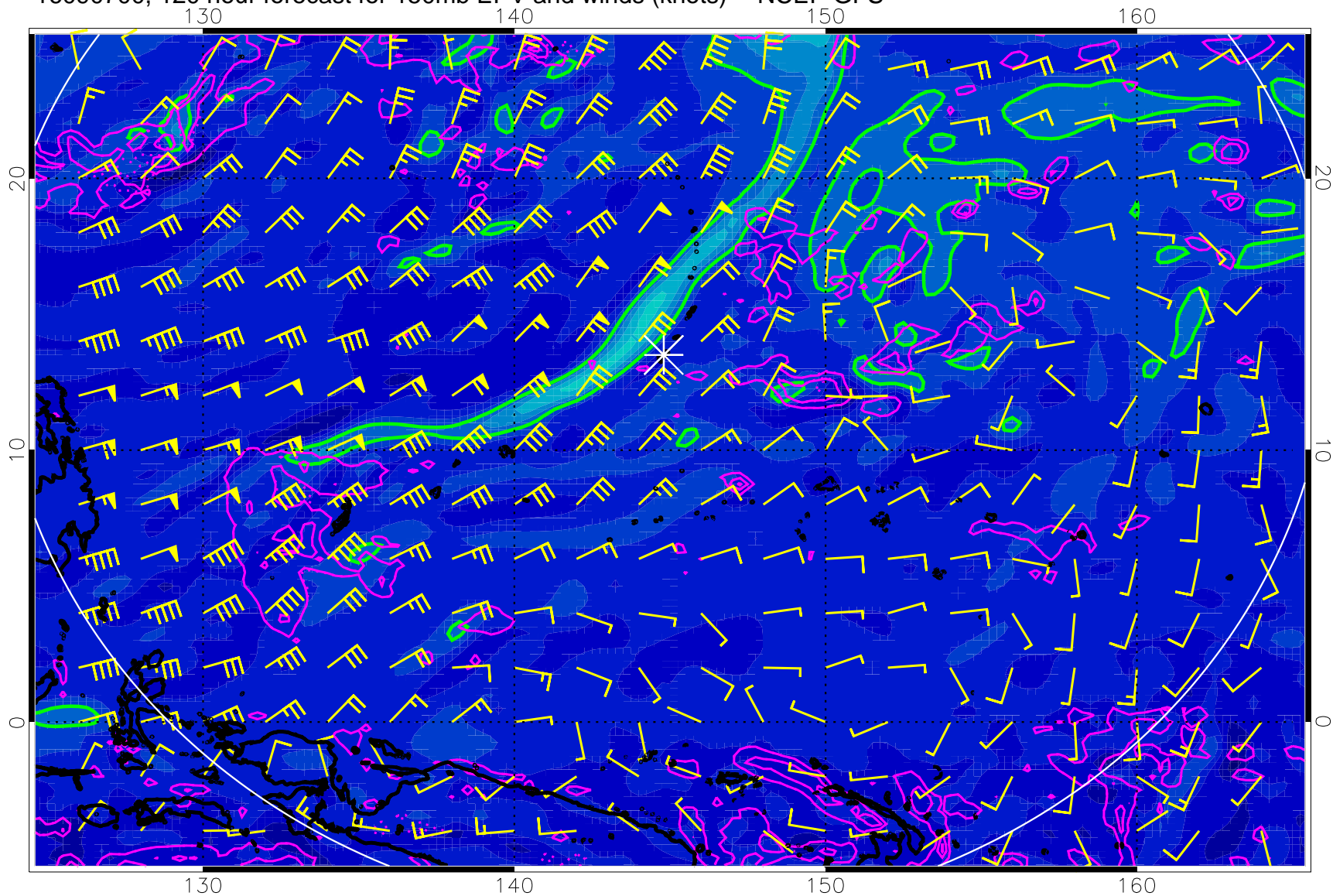
16090700, 120 hour forecast for 150mb EPV and winds (knots) -- NCEP GFS
