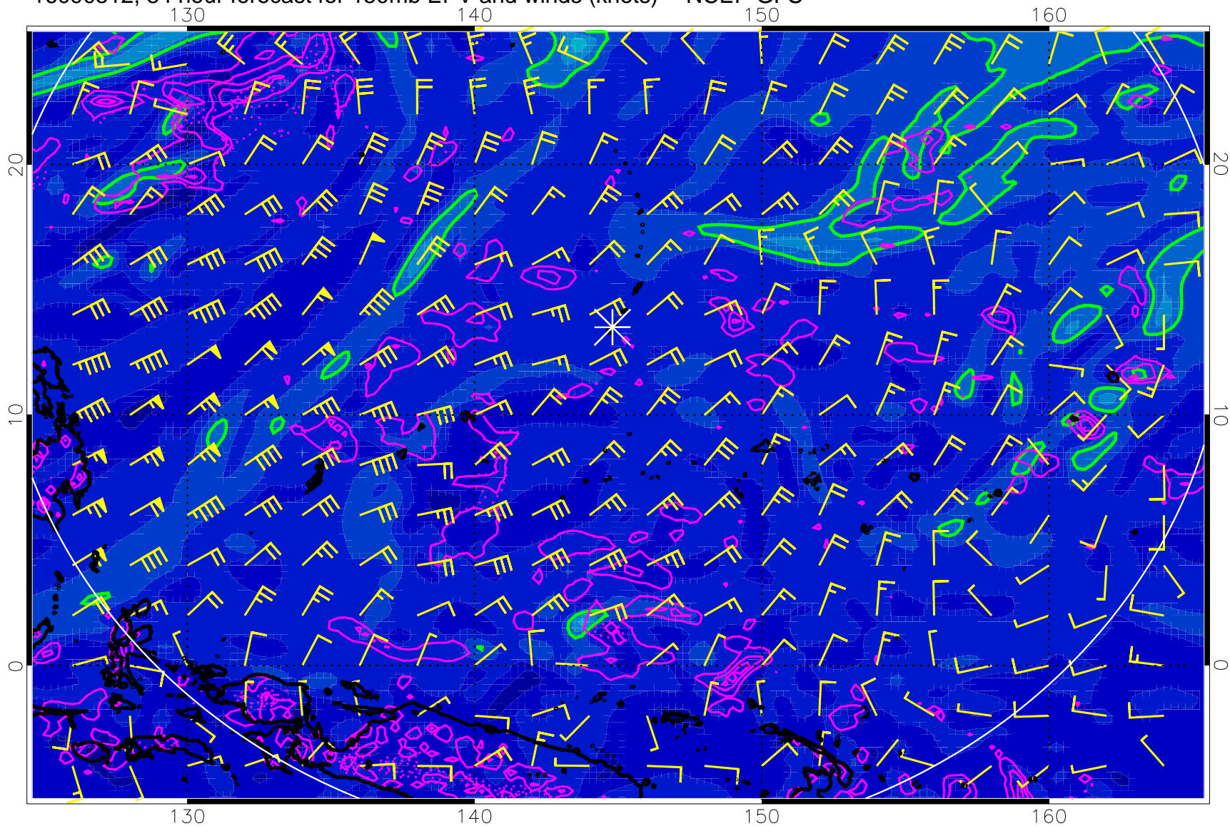
16090512, 84 hour forecast for 150mb EPV and winds (knots) -- NCEP GFS
