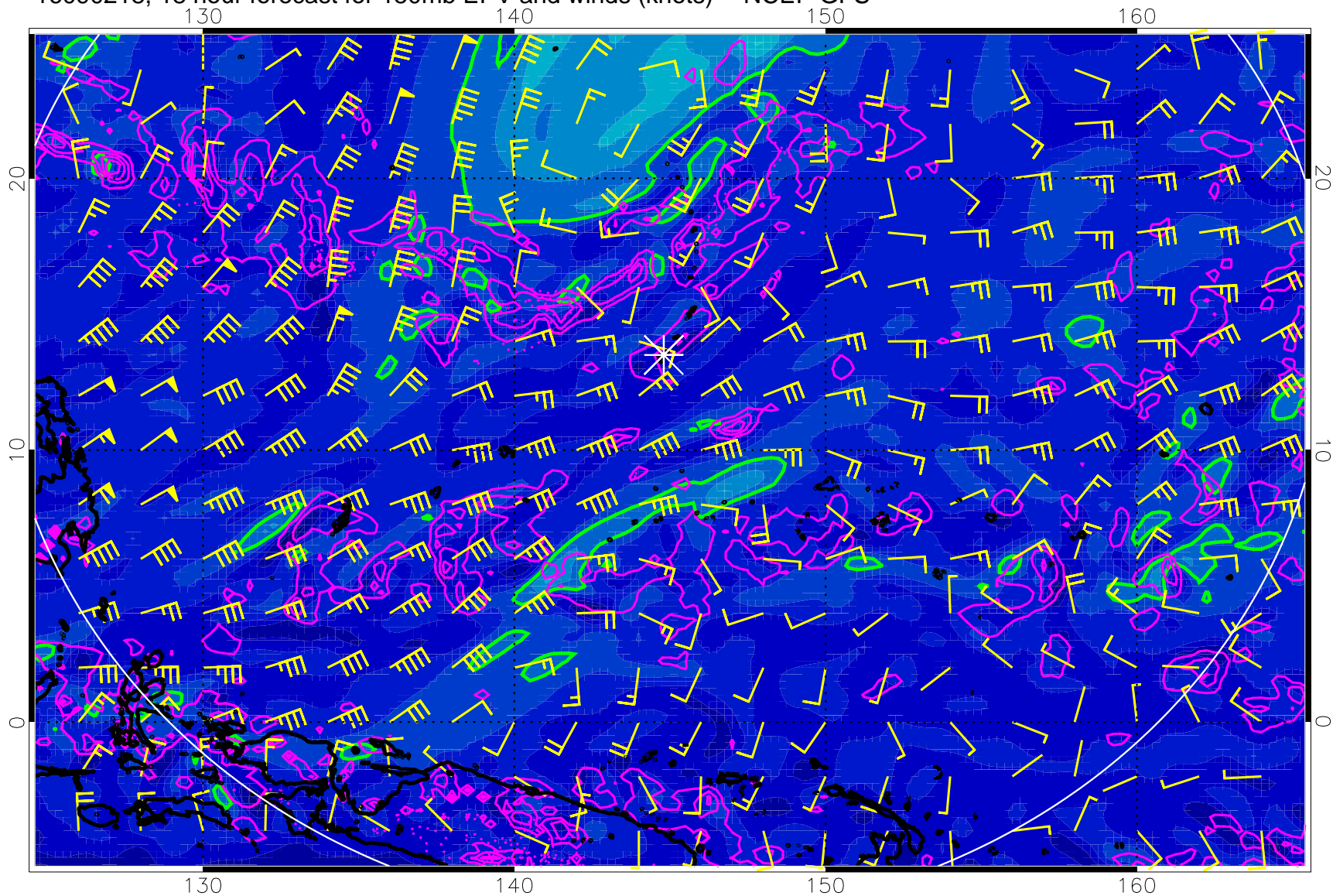
16090218, 18 hour forecast for 150mb EPV and winds (knots) -- NCEP GFS
