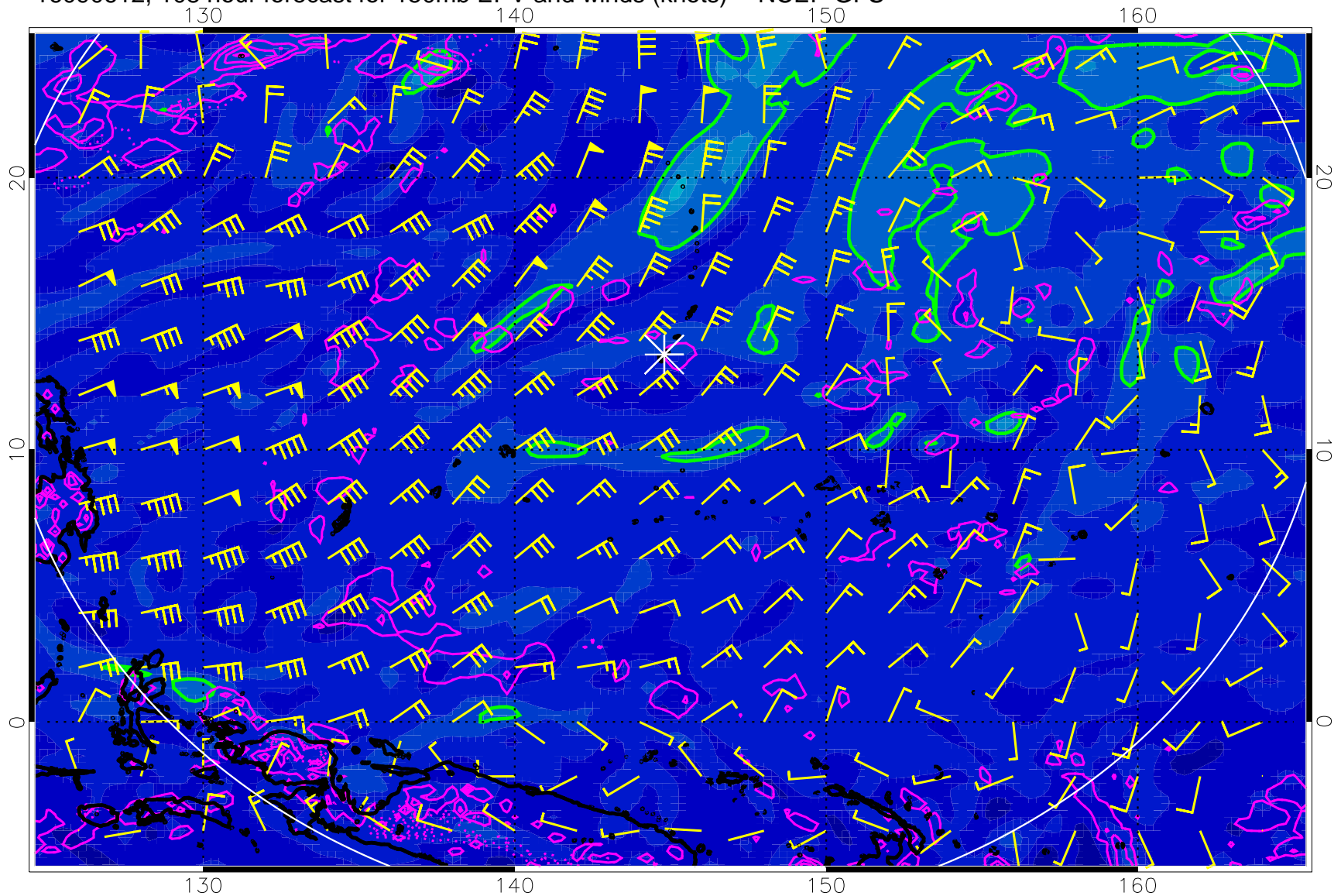
16090612, 108 hour forecast for 150mb EPV and winds (knots) -- NCEP GFS
