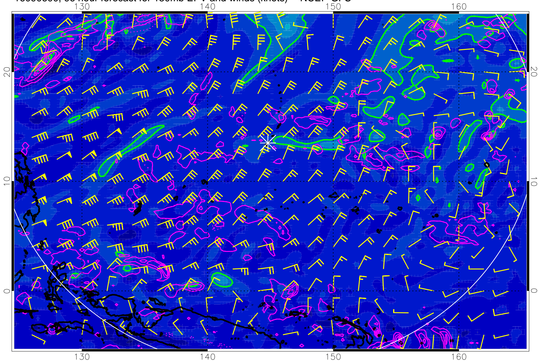
16090600, 96 hour forecast for 150mb EPV and winds (knots) -- NCEP GFS
