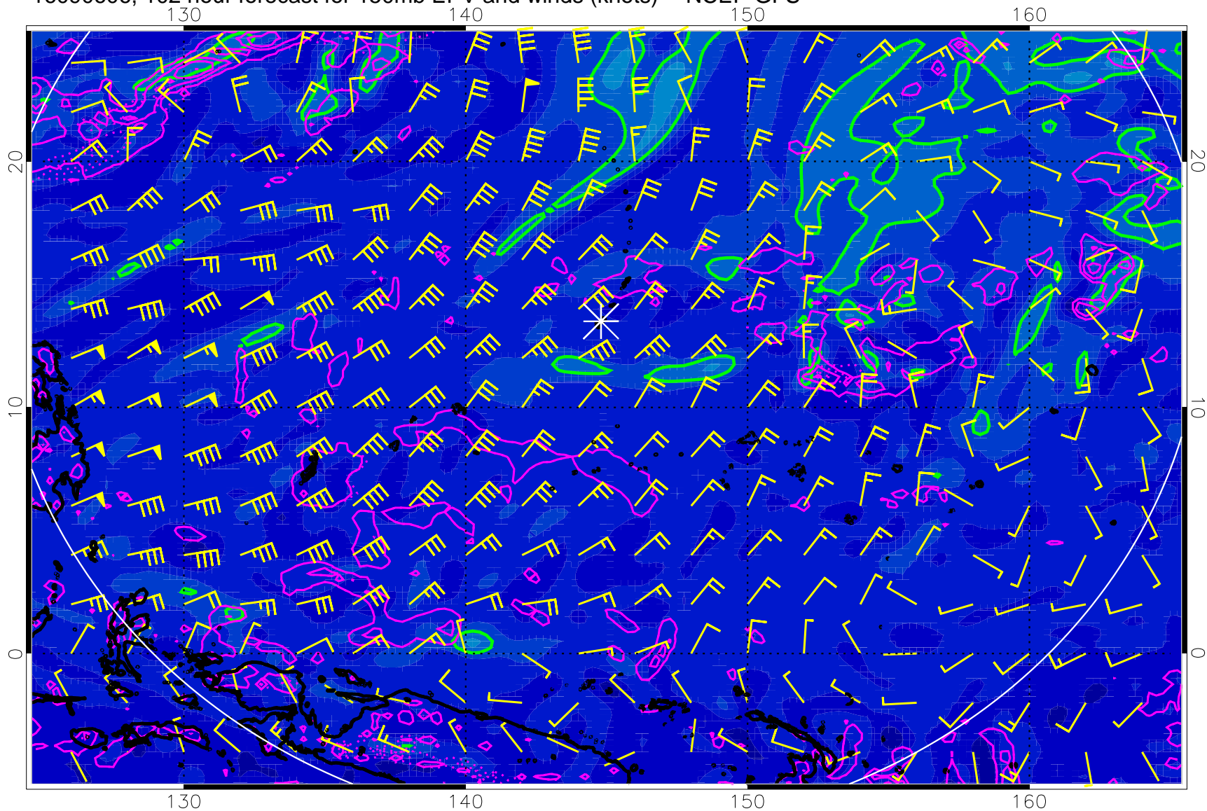
16090606, 102 hour forecast for 150mb EPV and winds (knots) -- NCEP GFS
