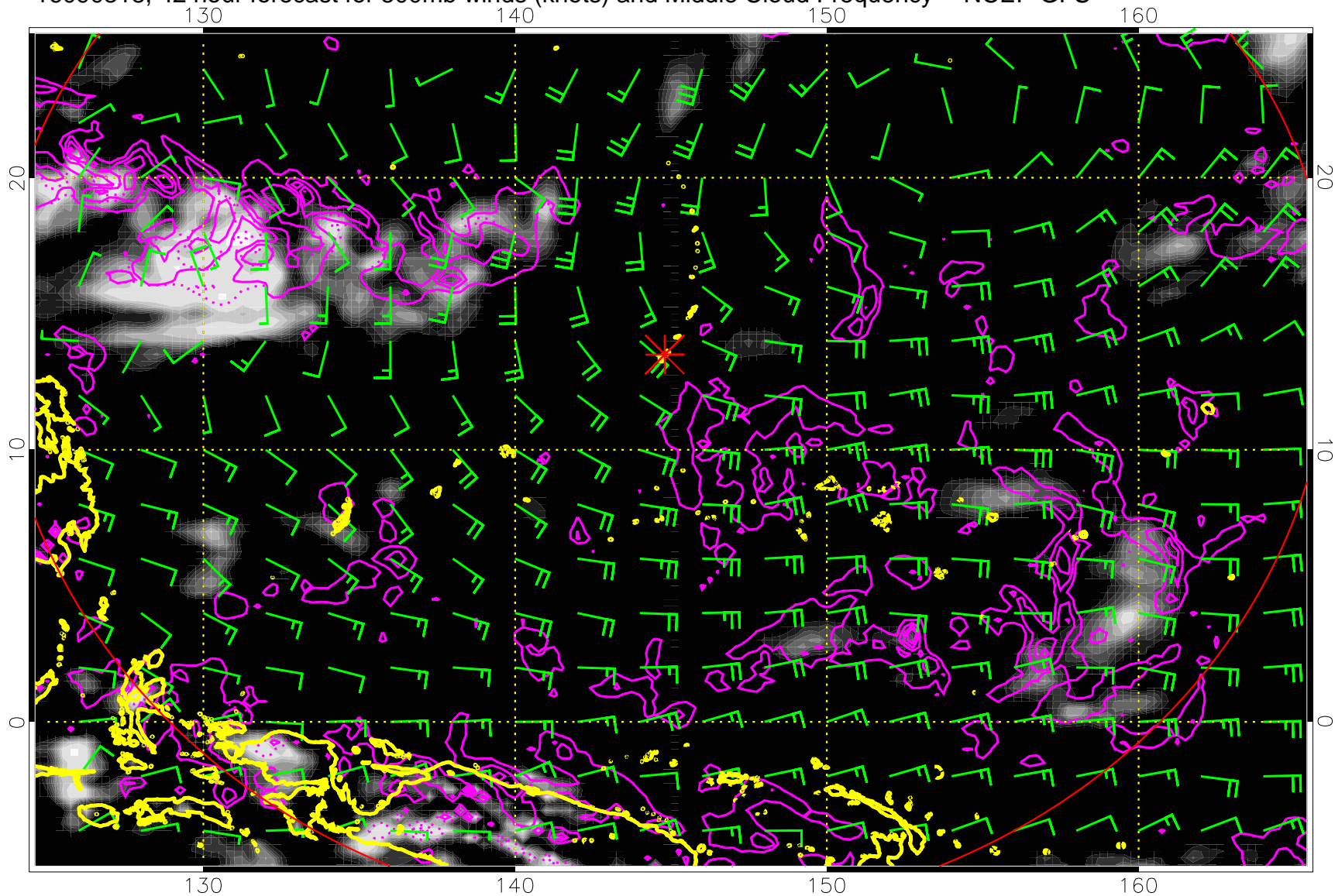
16090318, 42 hour forecast for 500mb winds (knots) and Middle Cloud Frequency -- NCEP GFS
