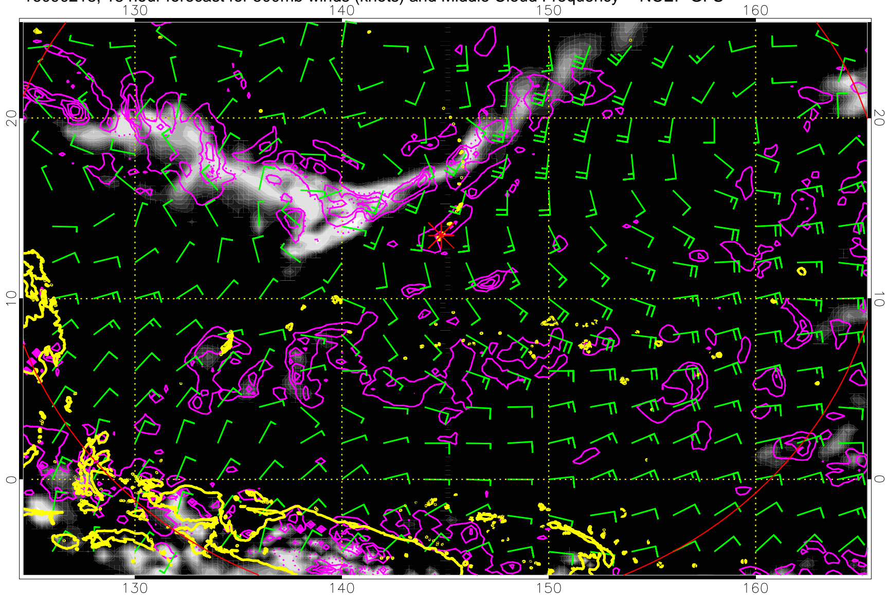
16090218, 18 hour forecast for 500mb winds (knots) and Middle Cloud Frequency -- NCEP GFS
