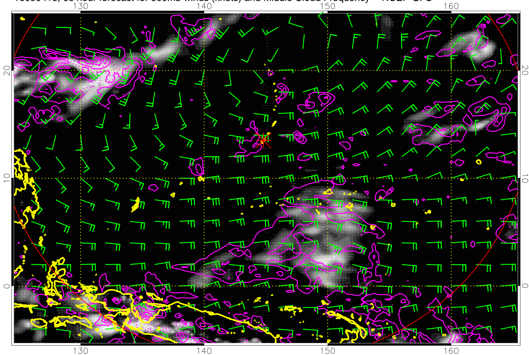
16090418, 66 hour forecast for 500mb winds (knots) and Middle Cloud Frequency -- NCEP GFS
