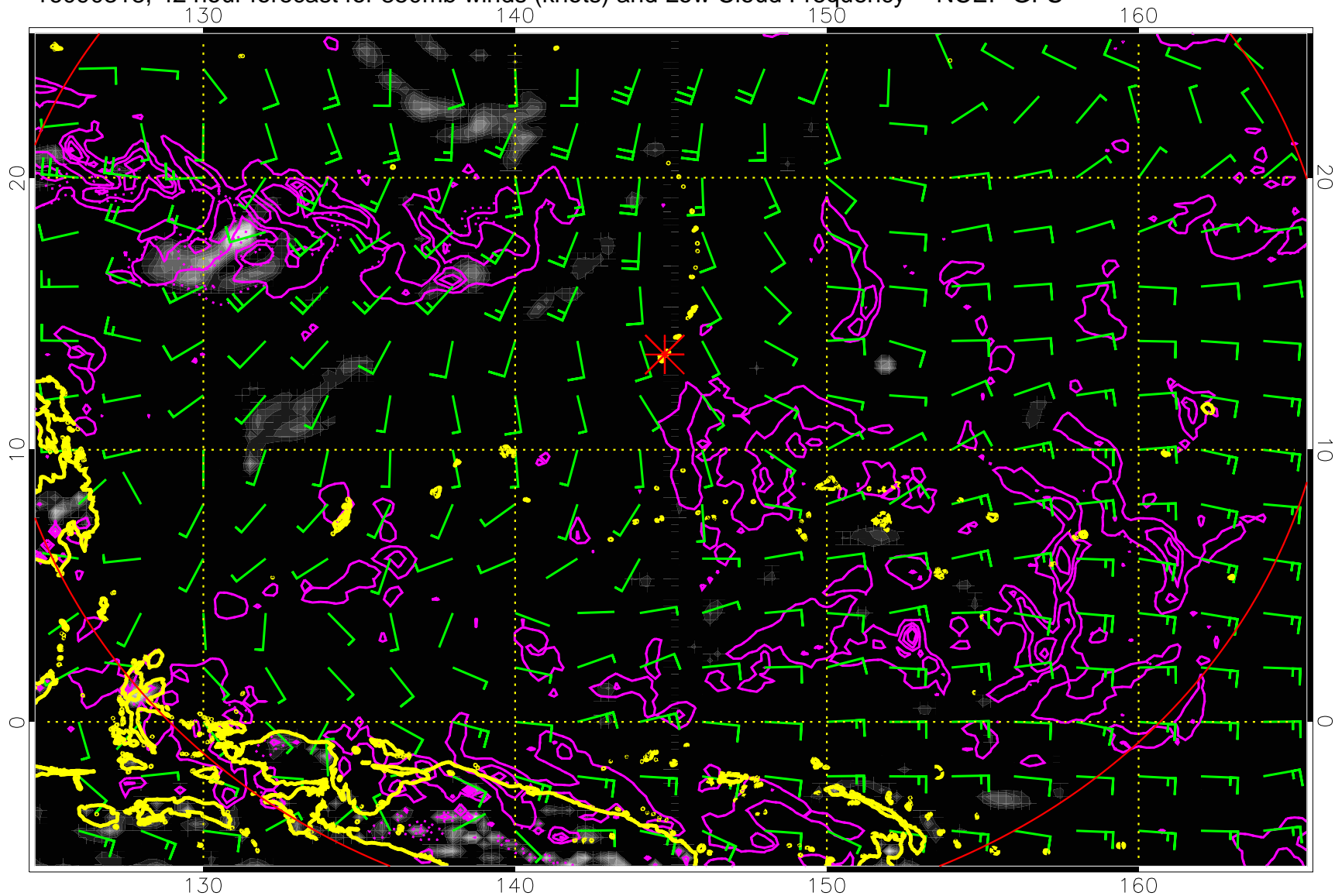
16090318, 42 hour forecast for 850mb winds (knots) and Low Cloud Frequency -- NCEP GFS
