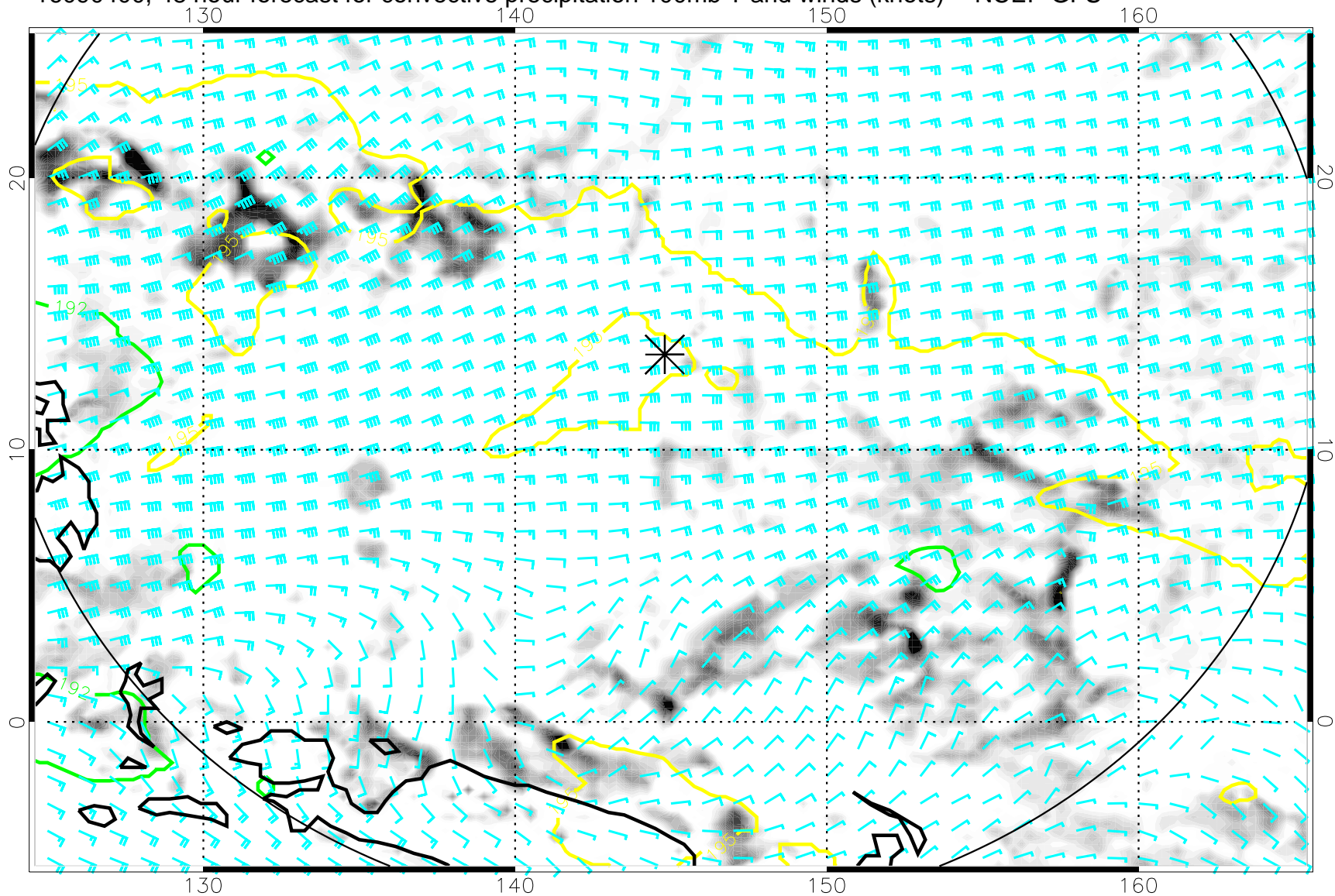
16090400, 48 hour forecast for convective precipitation 100mb T and winds (knots) -- NCEP GFS
