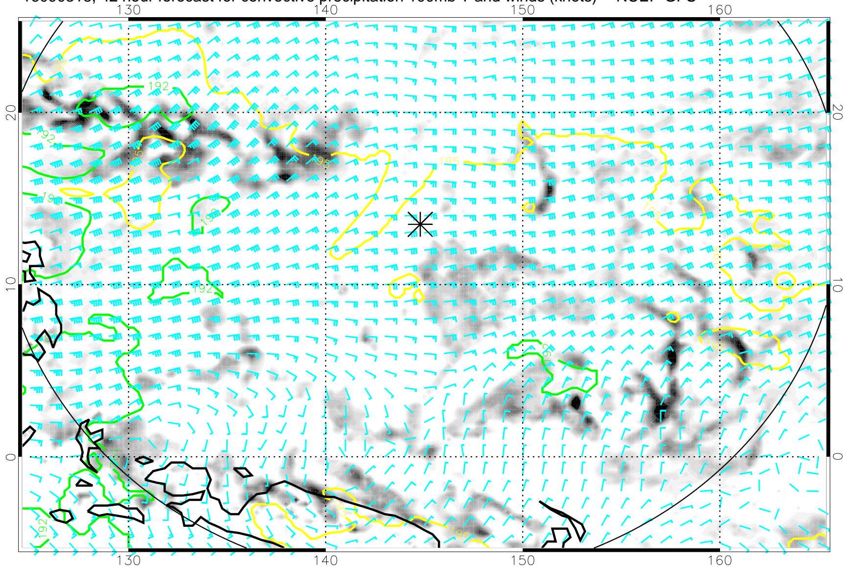
16090318, 42 hour forecast for convective precipitation 100mb T and winds (knots) -- NCEP GFS
