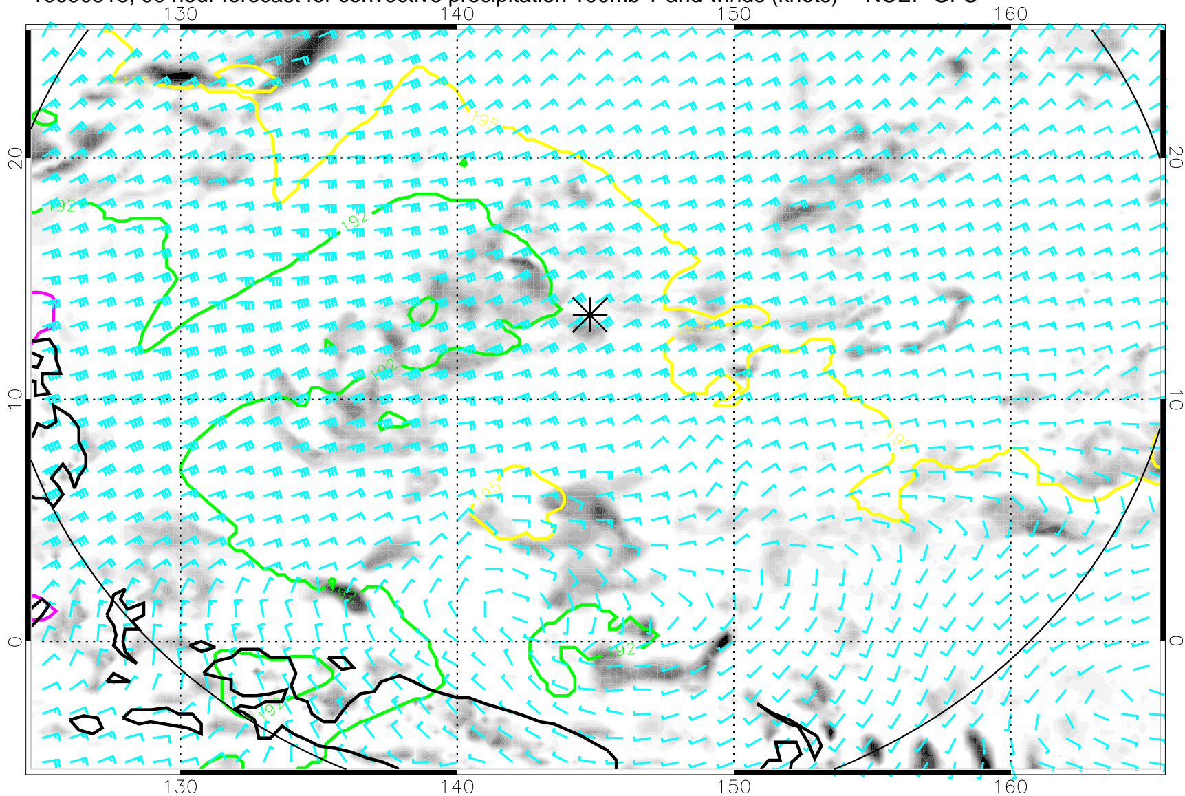
16090518, 90 hour forecast for convective precipitation 100mb T and winds (knots) -- NCEP GFS
