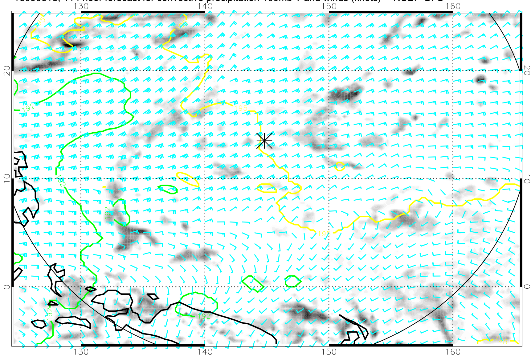
16090618, 114 hour forecast for convective precipitation 100mb T and winds (knots) -- NCEP GFS
