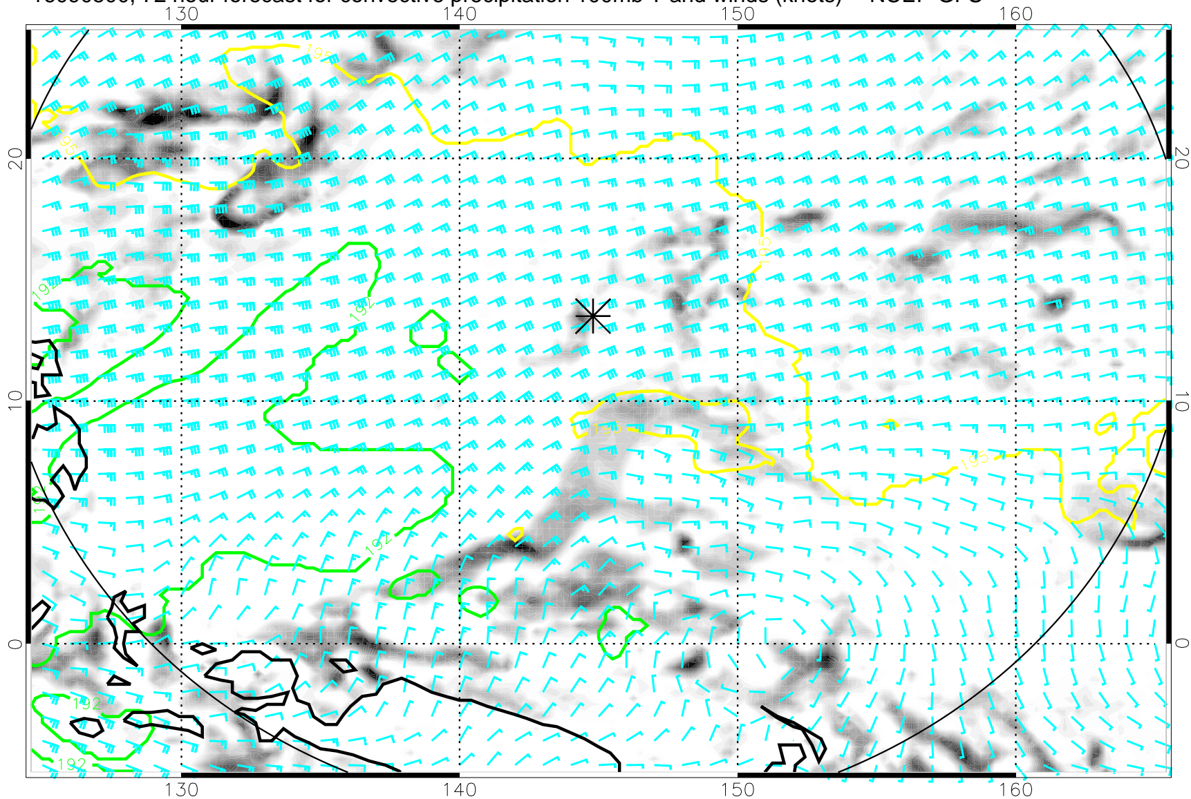
16090500, 72 hour forecast for convective precipitation 100mb T and winds (knots) -- NCEP GFS
