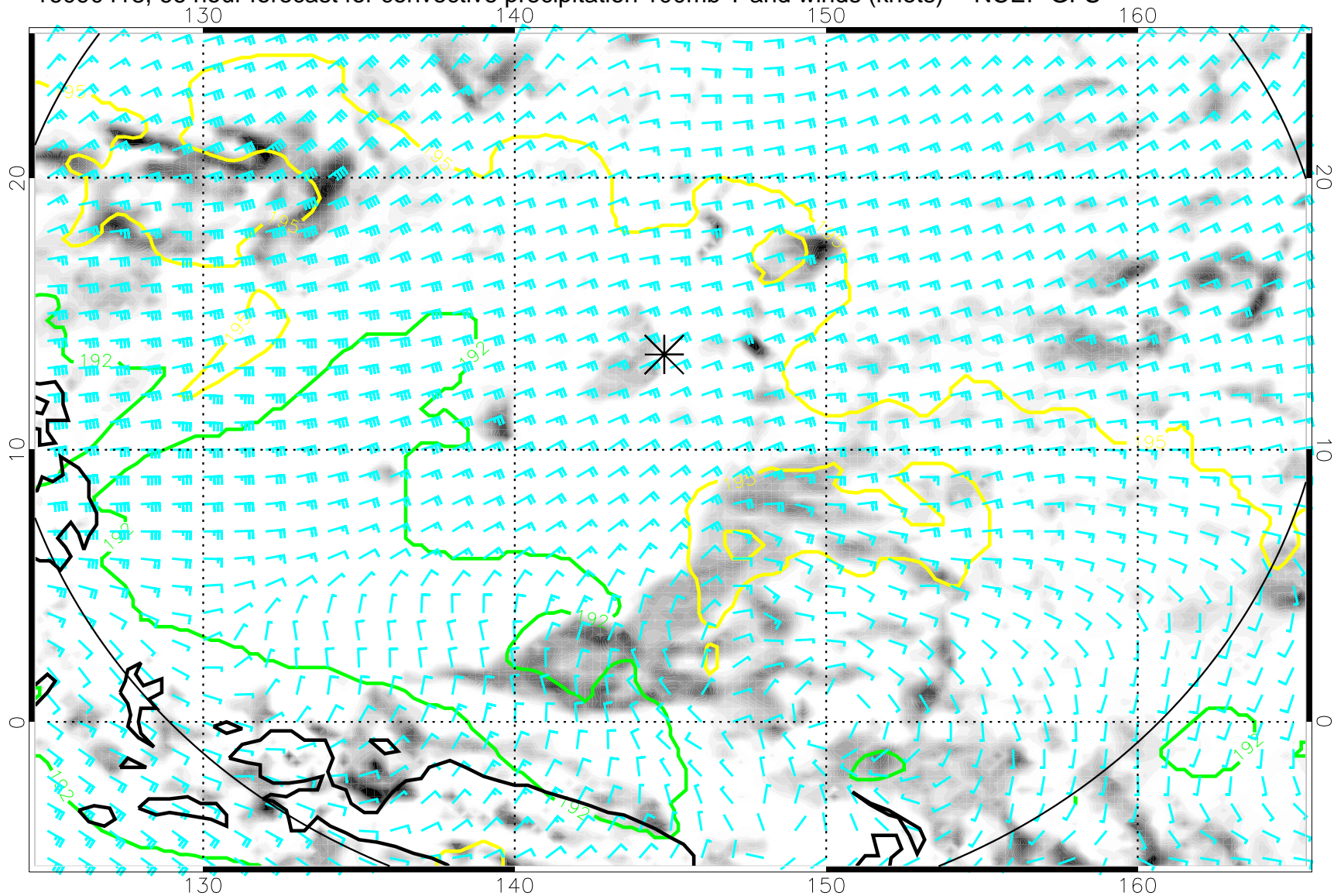
16090418, 66 hour forecast for convective precipitation 100mb T and winds (knots) -- NCEP GFS
