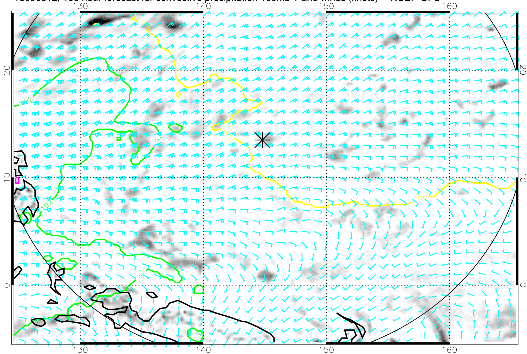
16090612, 108 hour forecast for convective precipitation 100mb T and winds (knots) -- NCEP GFS
