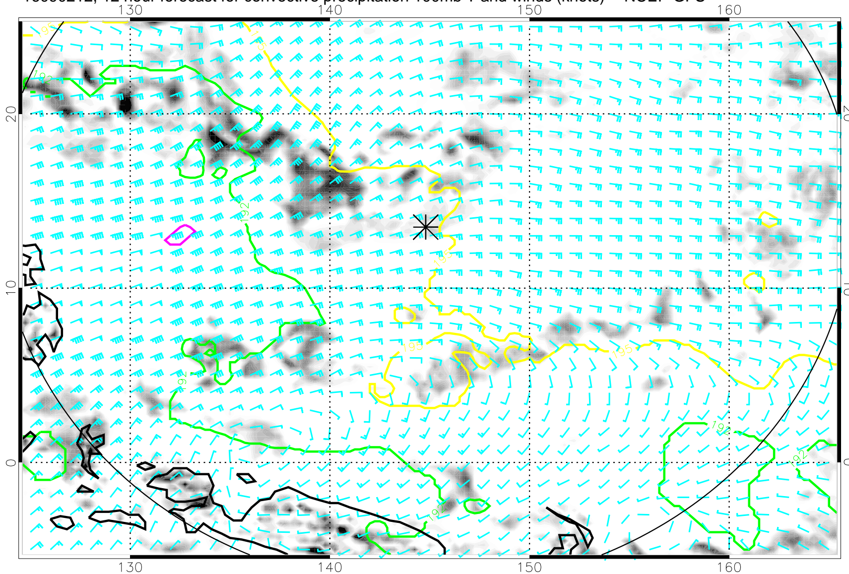
16090212, 12 hour forecast for convective precipitation 100mb T and winds (knots) -- NCEP GFS
