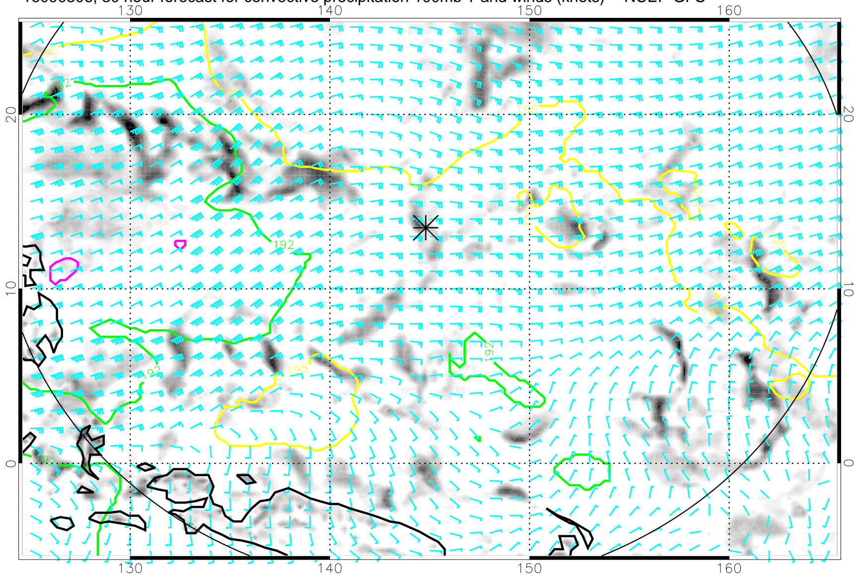
16090306, 30 hour forecast for convective precipitation 100mb T and winds (knots) -- NCEP GFS
