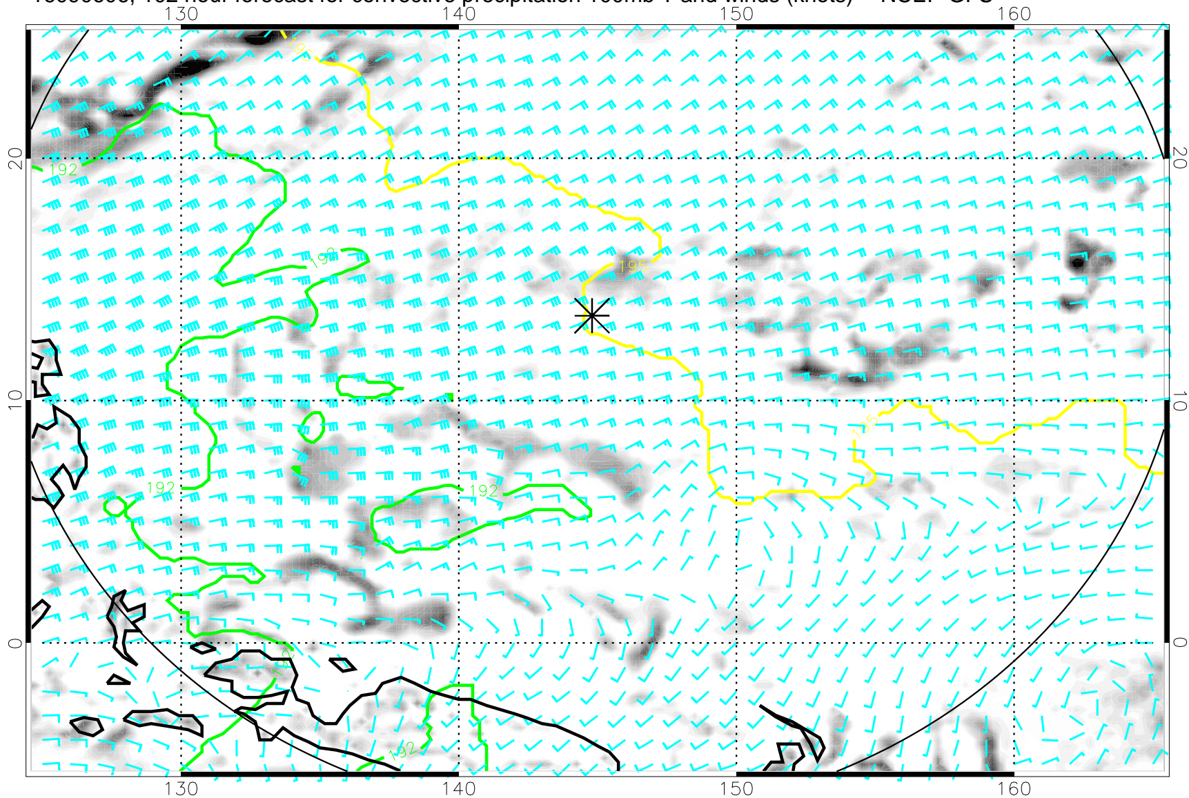
16090606, 102 hour forecast for convective precipitation 100mb T and winds (knots) -- NCEP GFS
