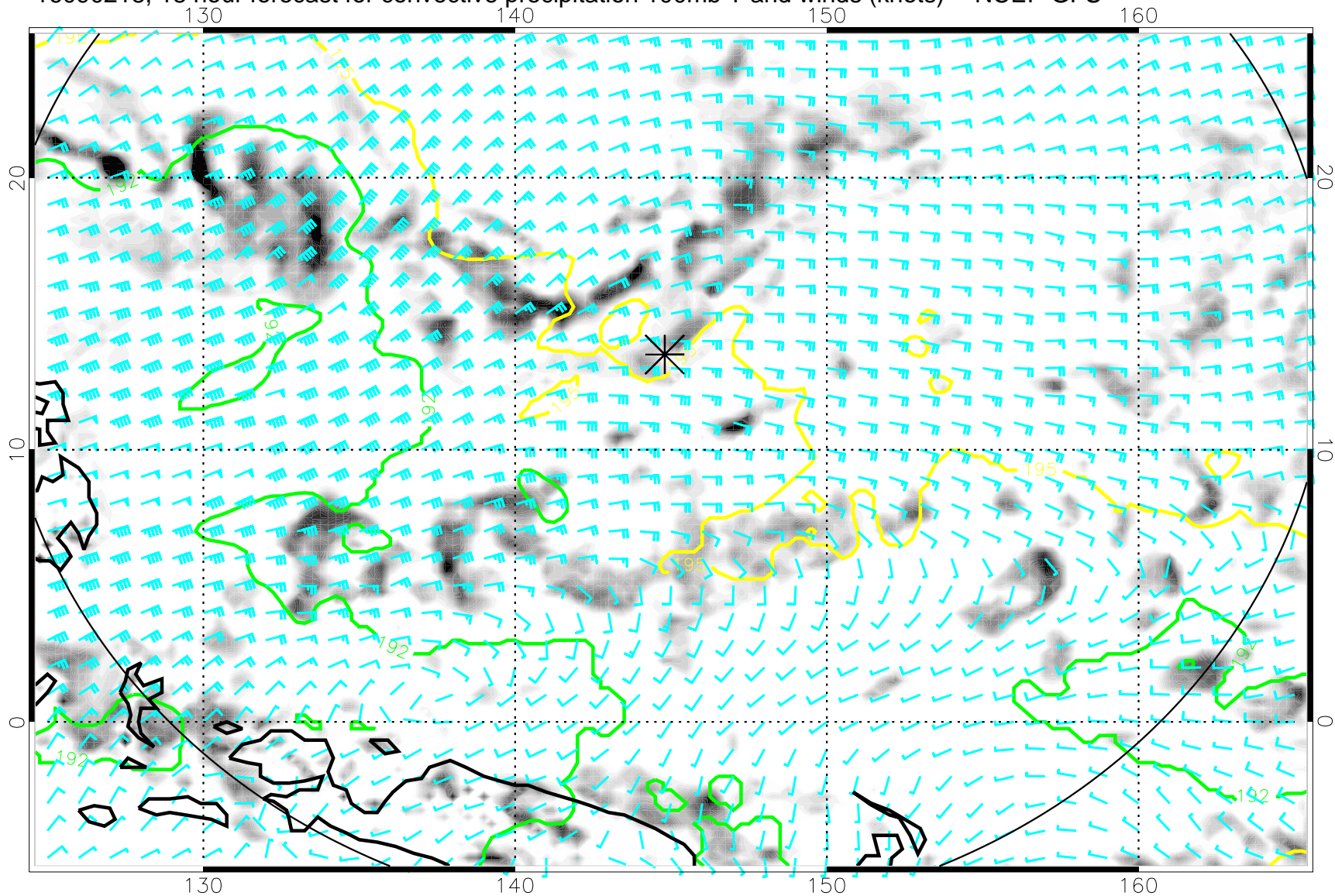
16090218, 18 hour forecast for convective precipitation 100mb T and winds (knots) -- NCEP GFS
