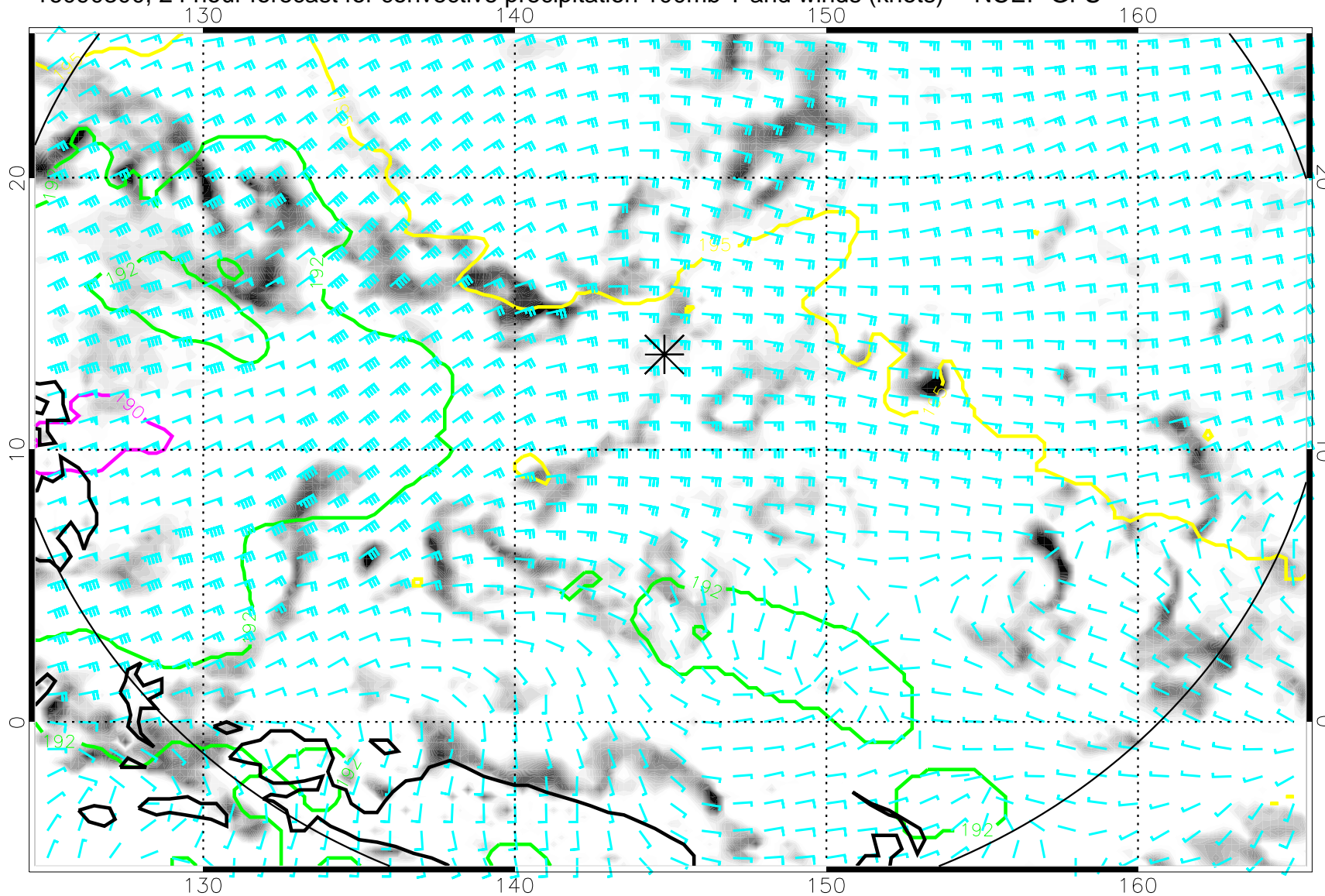
16090300, 24 hour forecast for convective precipitation 100mb T and winds (knots) -- NCEP GFS
