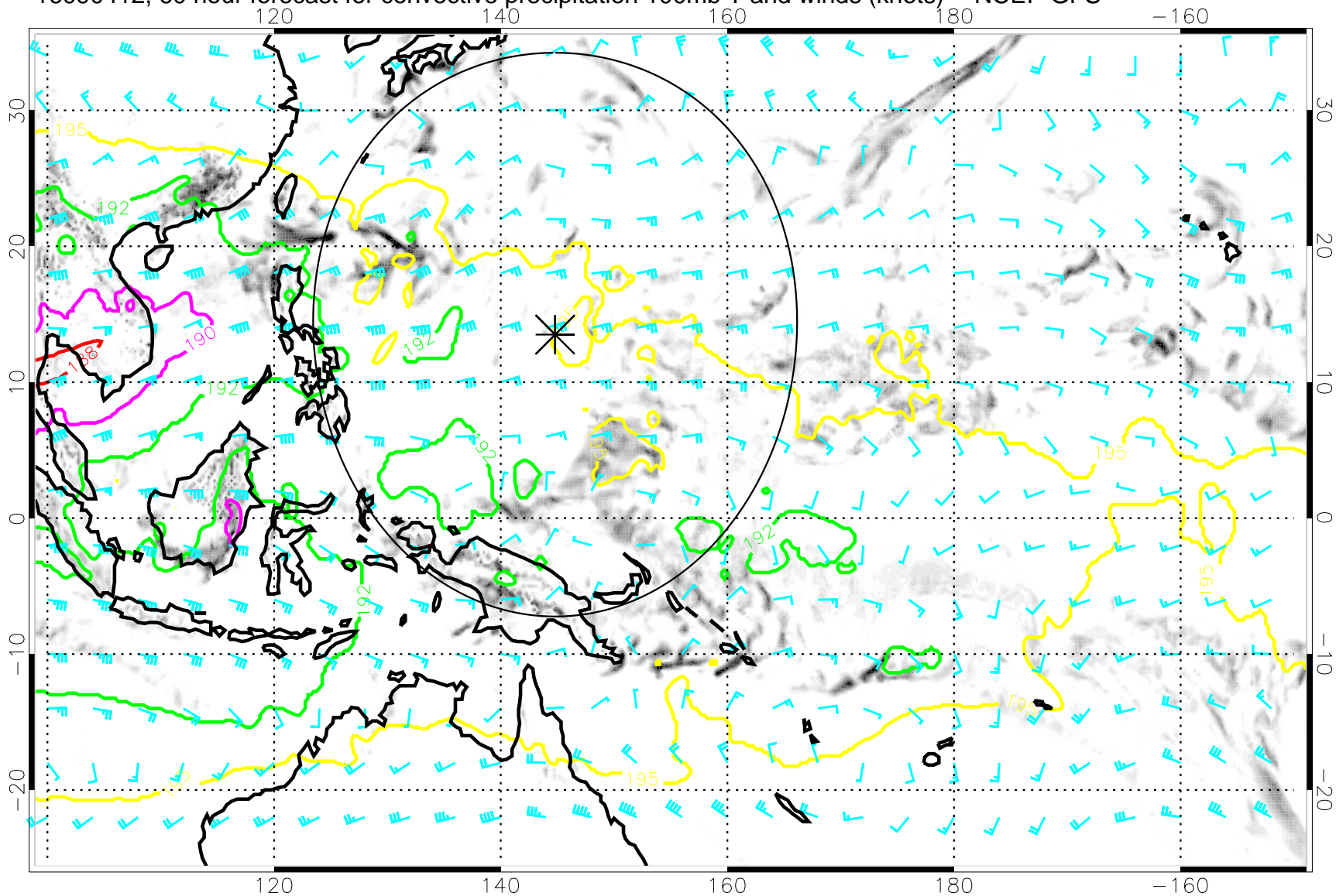
16090412, 60 hour forecast for convective precipitation 100mb T and winds (knots) -- NCEP GFS
