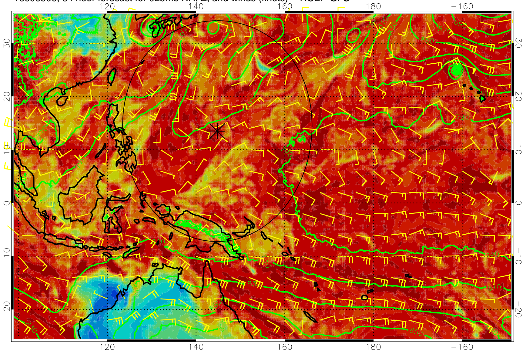
16090500, 84 hour forecast for 925mb RH, Z, and winds (knots) -- NCEP GFS
