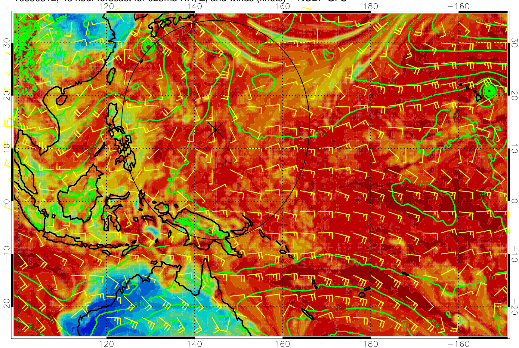
16090312, 48 hour forecast for 925mb RH, Z, and winds (knots) -- NCEP GFS
