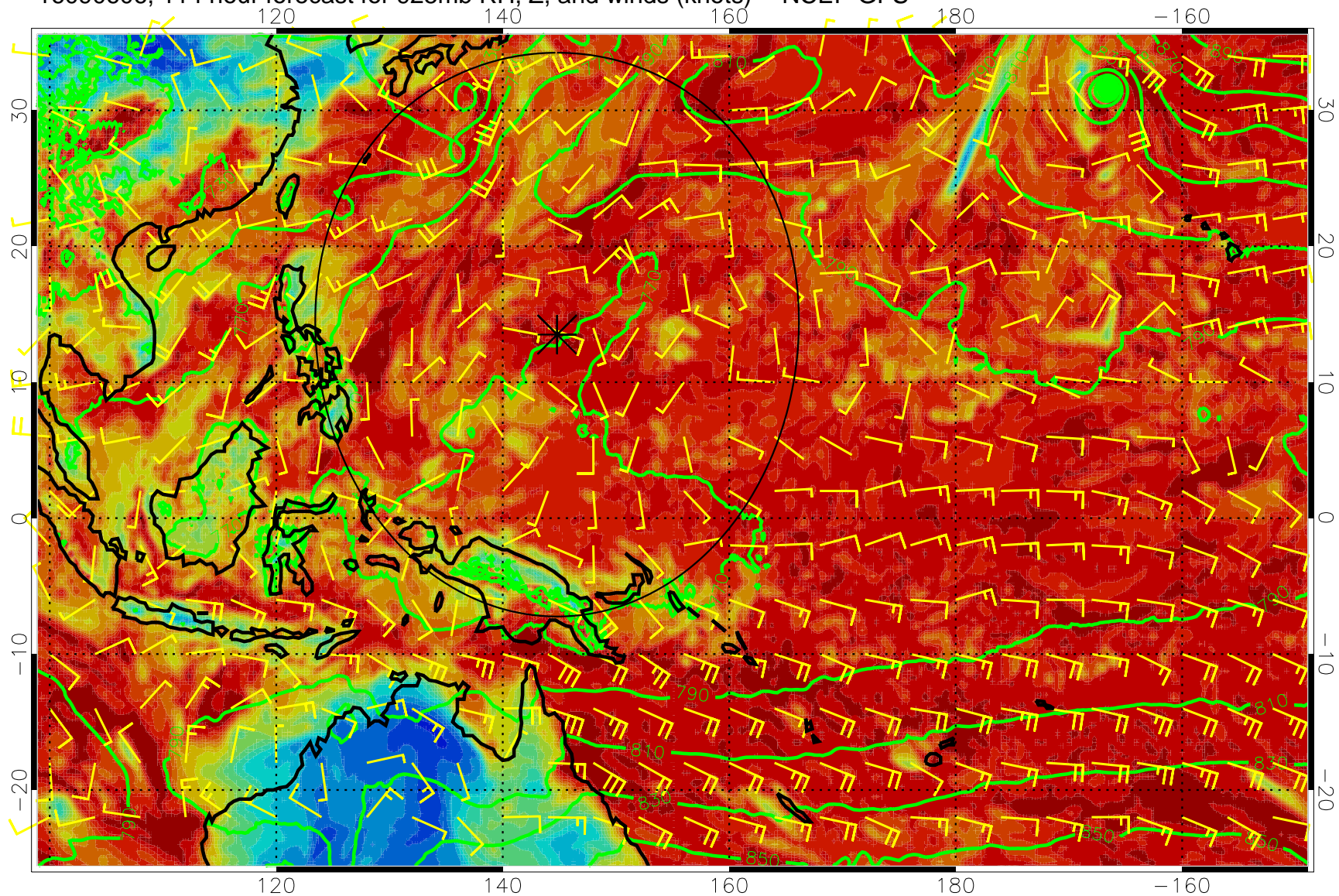
16090606, 114 hour forecast for 925mb RH, Z, and winds (knots) -- NCEP GFS
