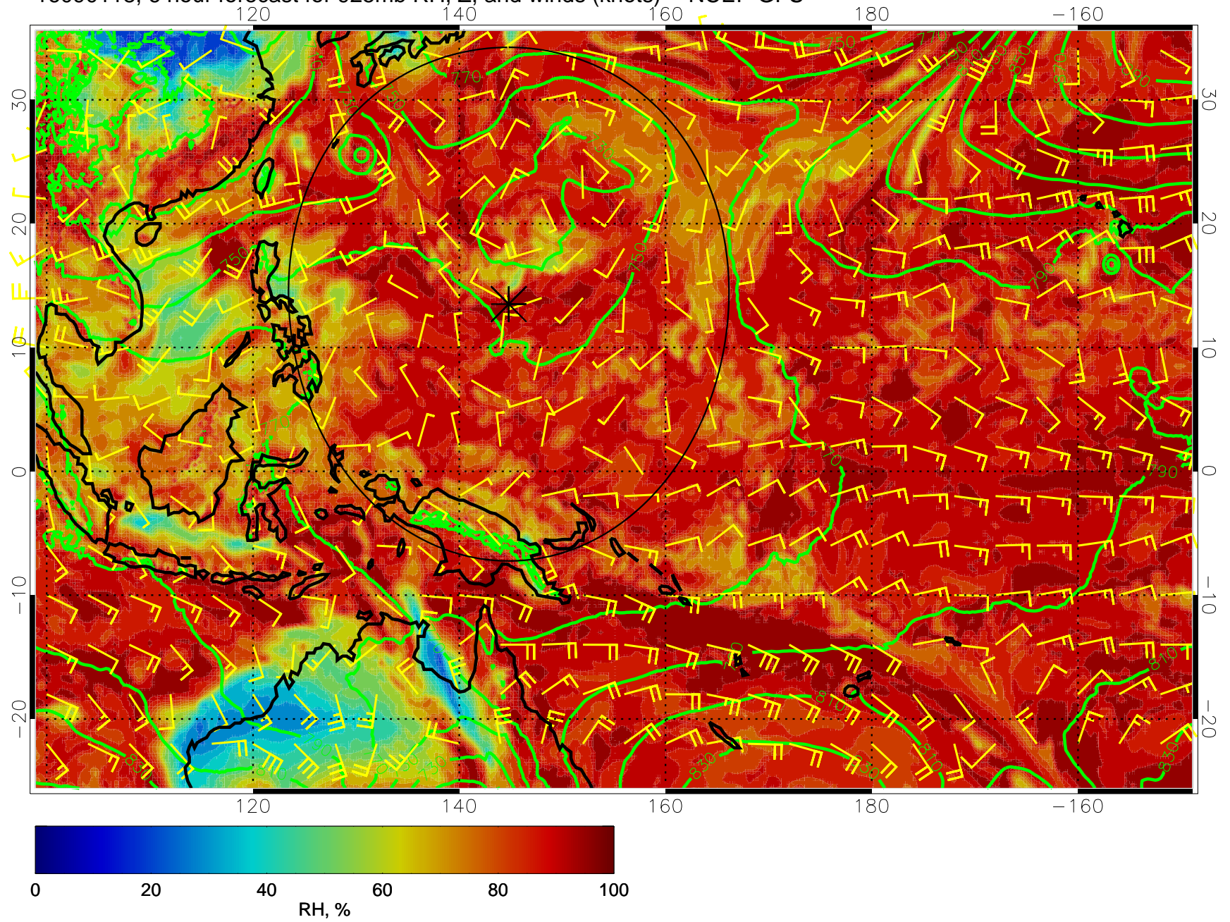
16090118, 6 hour forecast for 925mb RH, Z, and winds (knots) -- NCEP GFS
