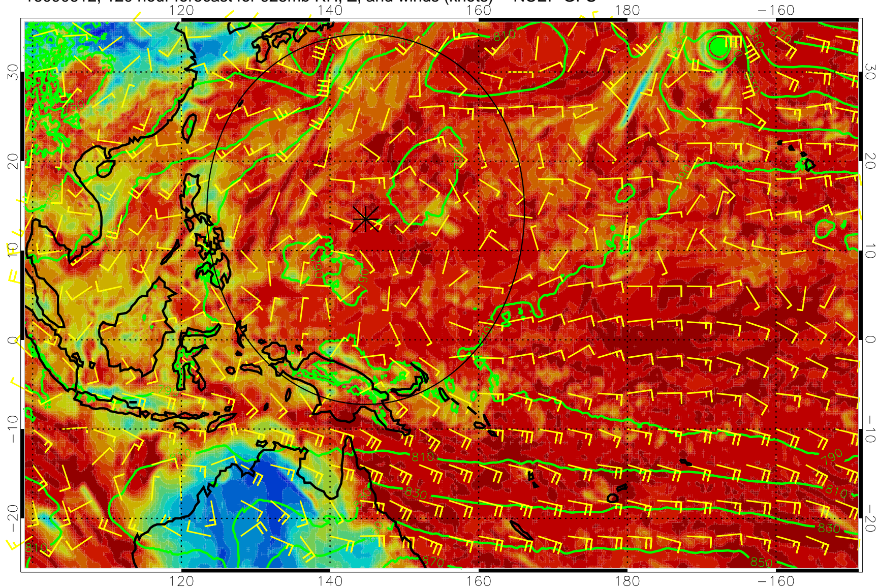
16090612, 120 hour forecast for 925mb RH, Z, and winds (knots) -- NCEP GFS
