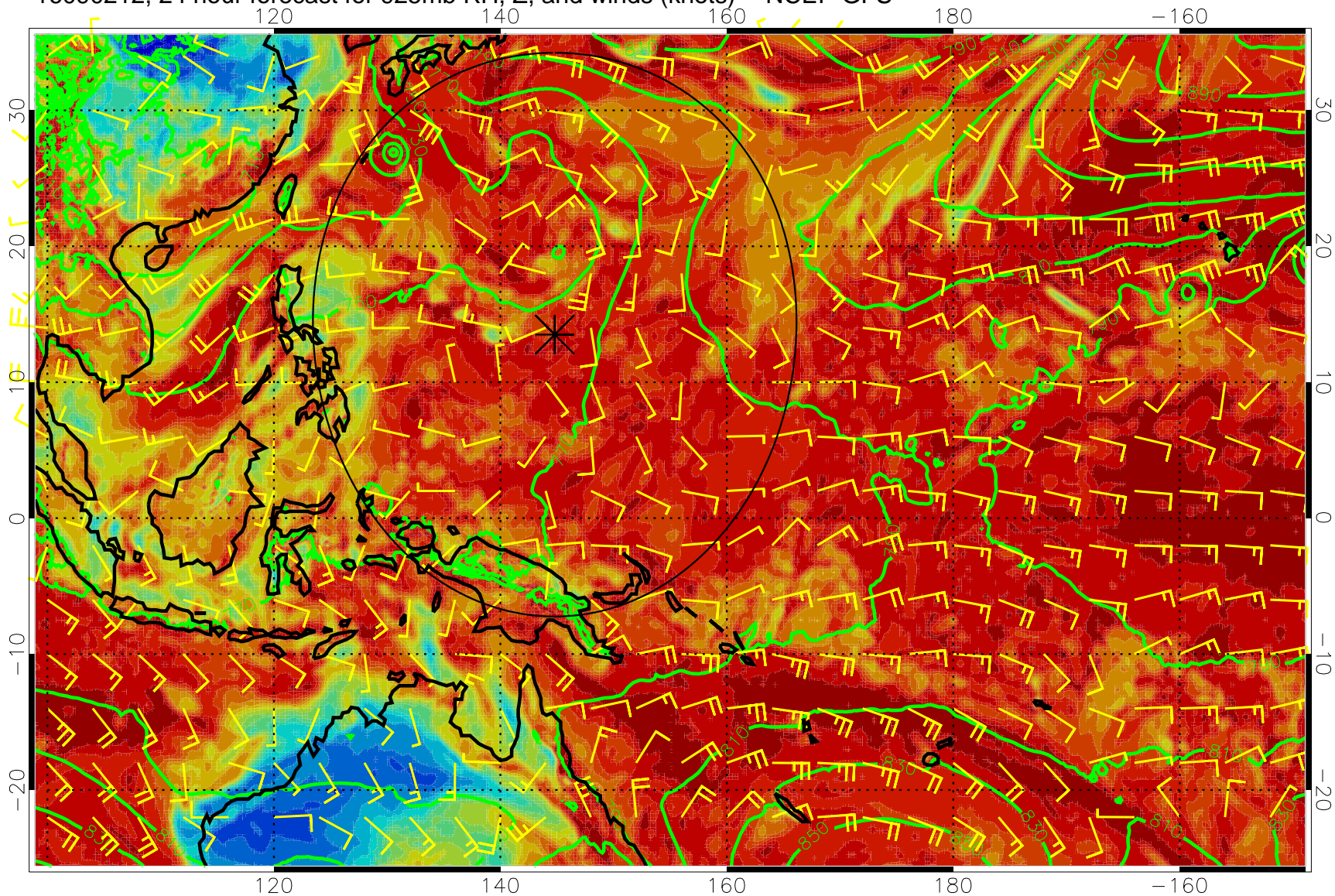
16090212, 24 hour forecast for 925mb RH, Z, and winds (knots) -- NCEP GFS
