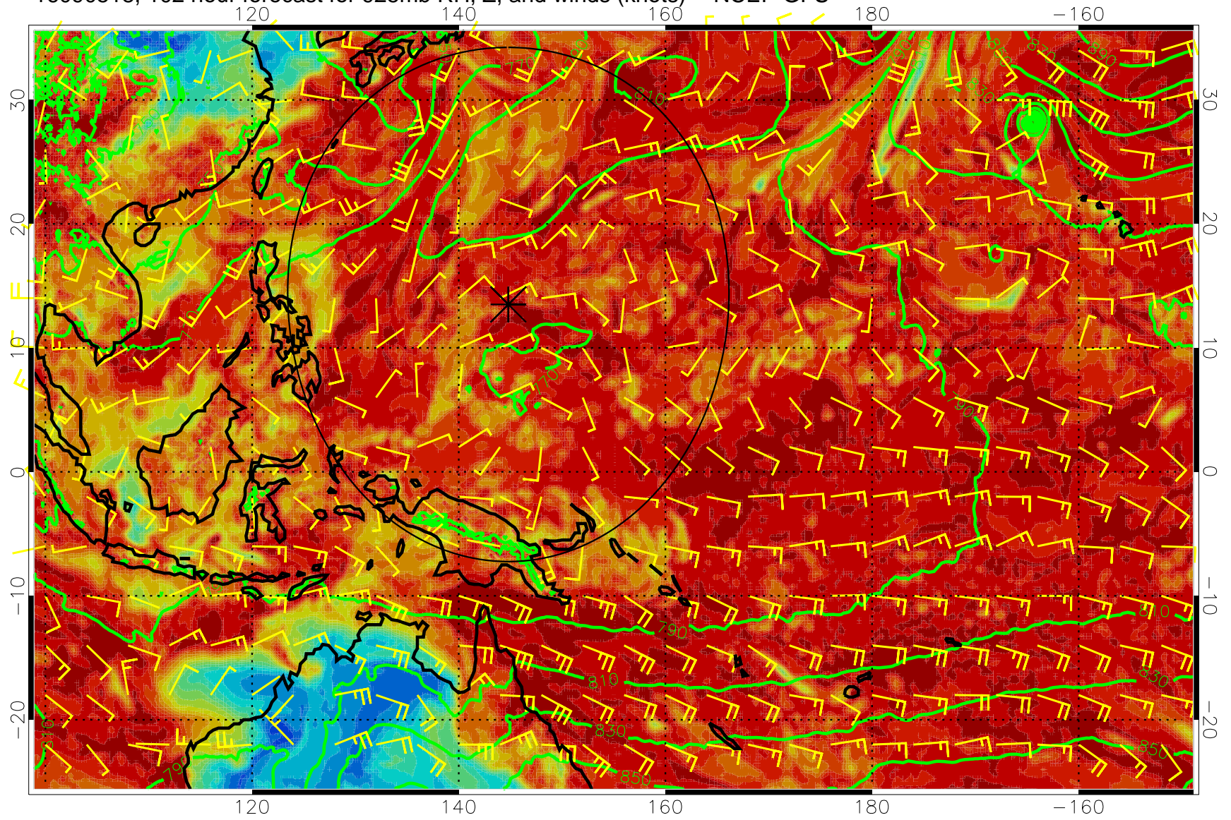
16090518, 102 hour forecast for 925mb RH, Z, and winds (knots) -- NCEP GFS
