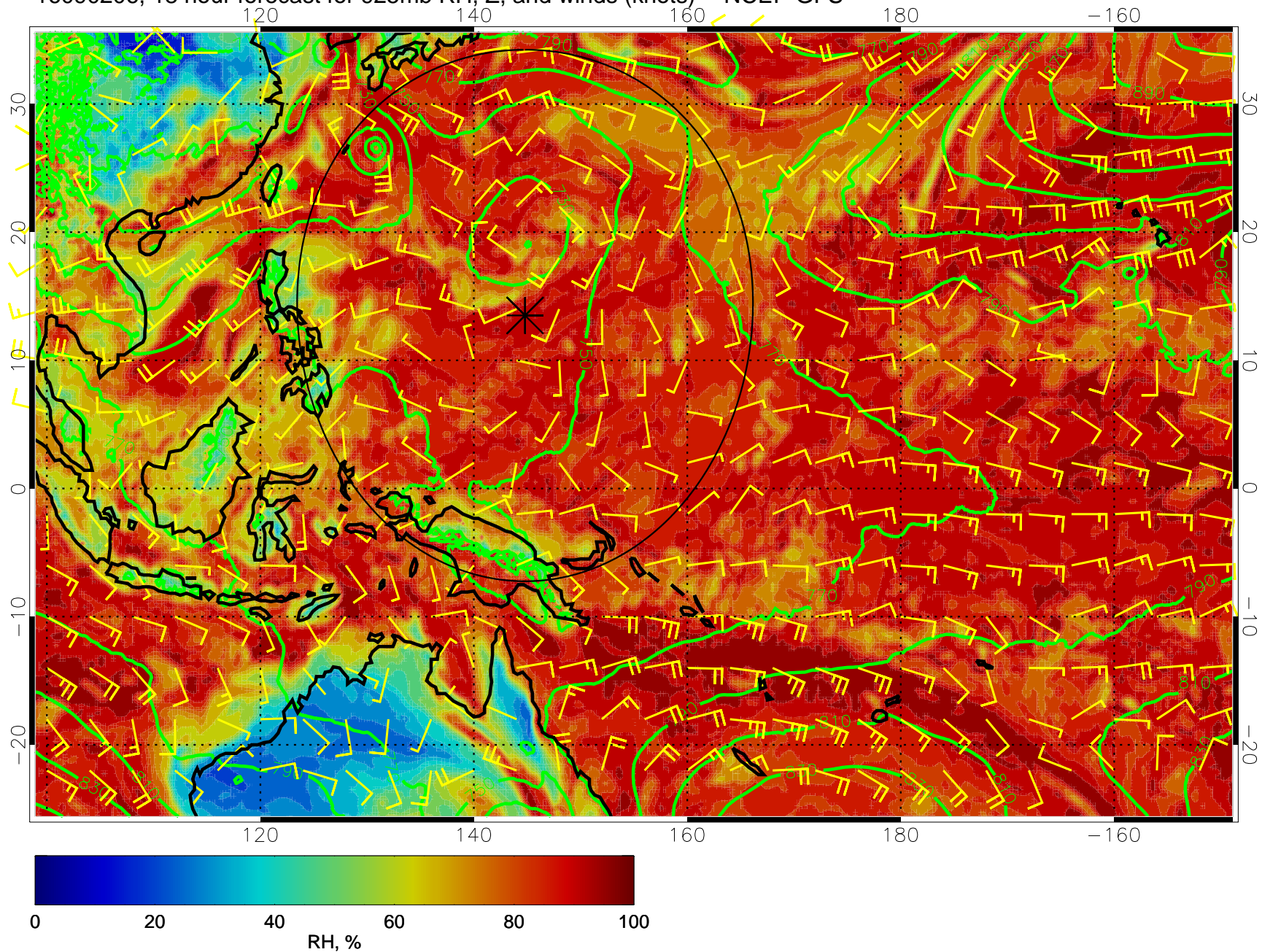
16090206, 18 hour forecast for 925mb RH, Z, and winds (knots) -- NCEP GFS
