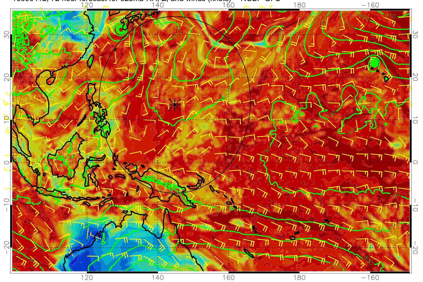
16090412, 72 hour forecast for 925mb RH, Z, and winds (knots) -- NCEP GFS
