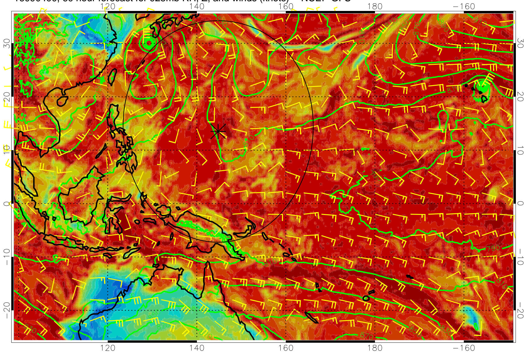
16090400, 60 hour forecast for 925mb RH, Z, and winds (knots) -- NCEP GFS
