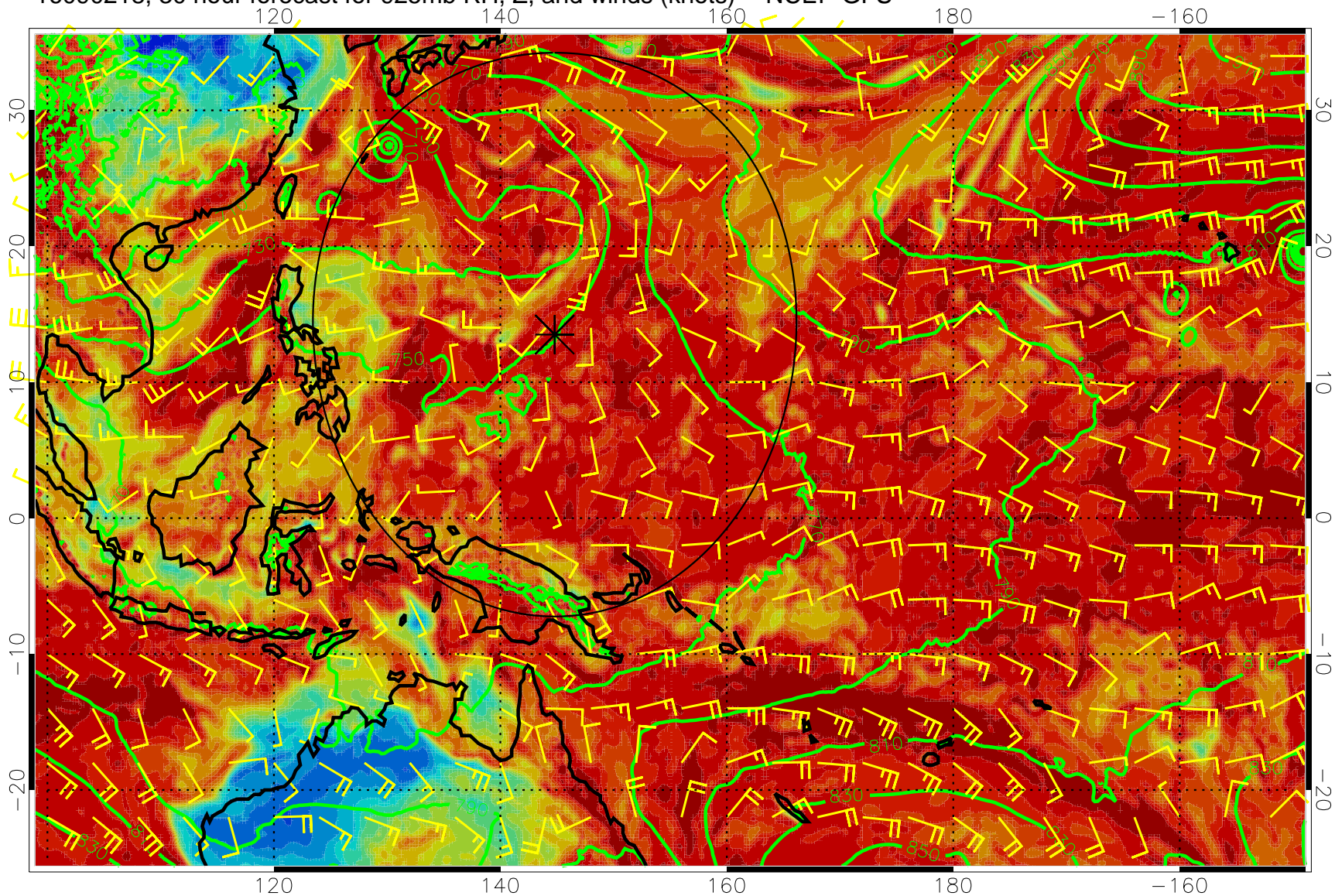
16090218, 30 hour forecast for 925mb RH, Z, and winds (knots) -- NCEP GFS
