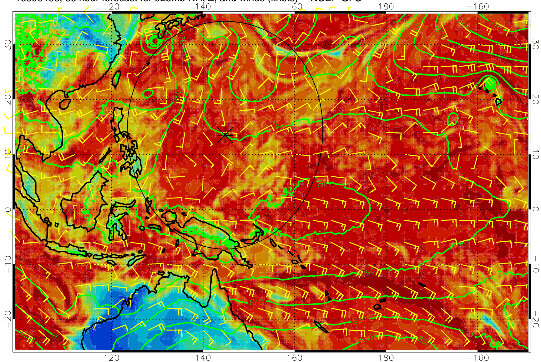
16090406, 66 hour forecast for 925mb RH, Z, and winds (knots) -- NCEP GFS
