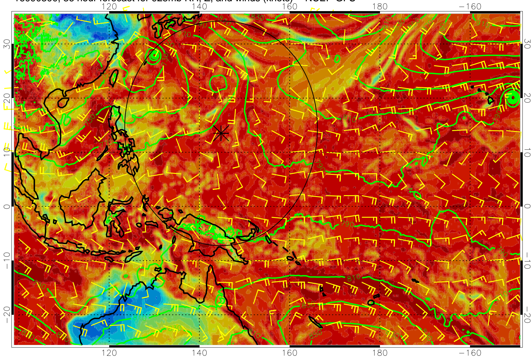
16090300, 36 hour forecast for 925mb RH, Z, and winds (knots) -- NCEP GFS
