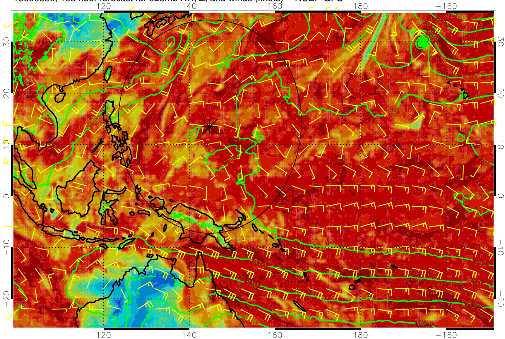
16090600, 108 hour forecast for 925mb RH, Z, and winds (knots) -- NCEP GFS
