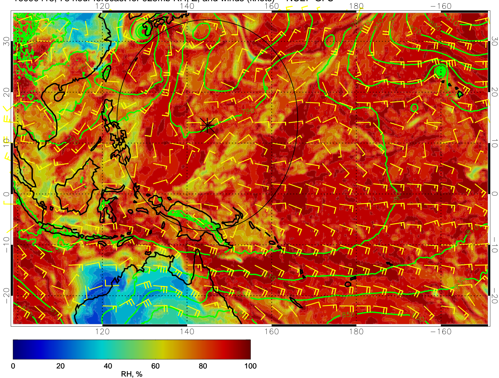
16090418, 78 hour forecast for 925mb RH, Z, and winds (knots) -- NCEP GFS
