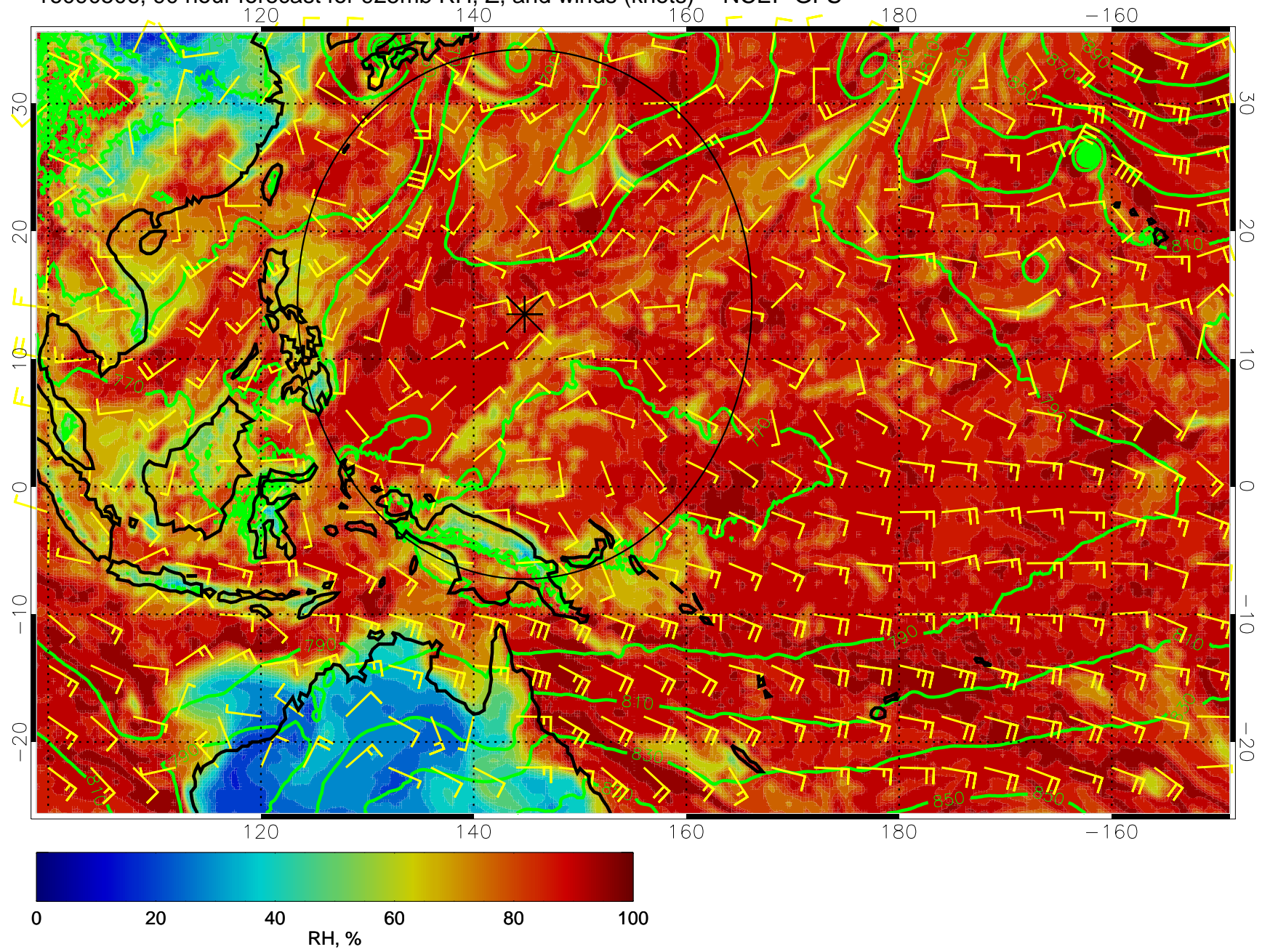
16090506, 90 hour forecast for 925mb RH, Z, and winds (knots) -- NCEP GFS
