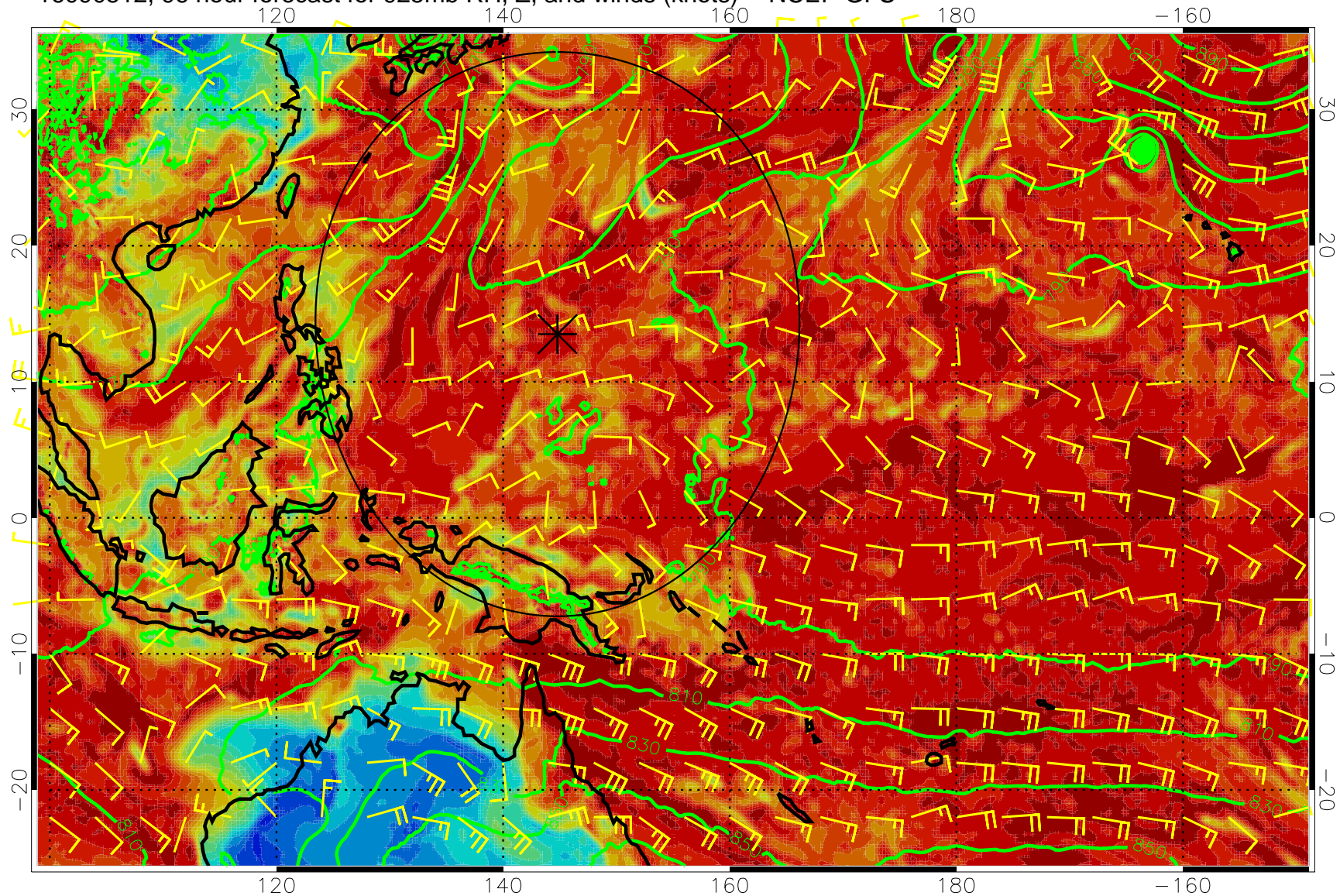
16090512, 96 hour forecast for 925mb RH, Z, and winds (knots) -- NCEP GFS
