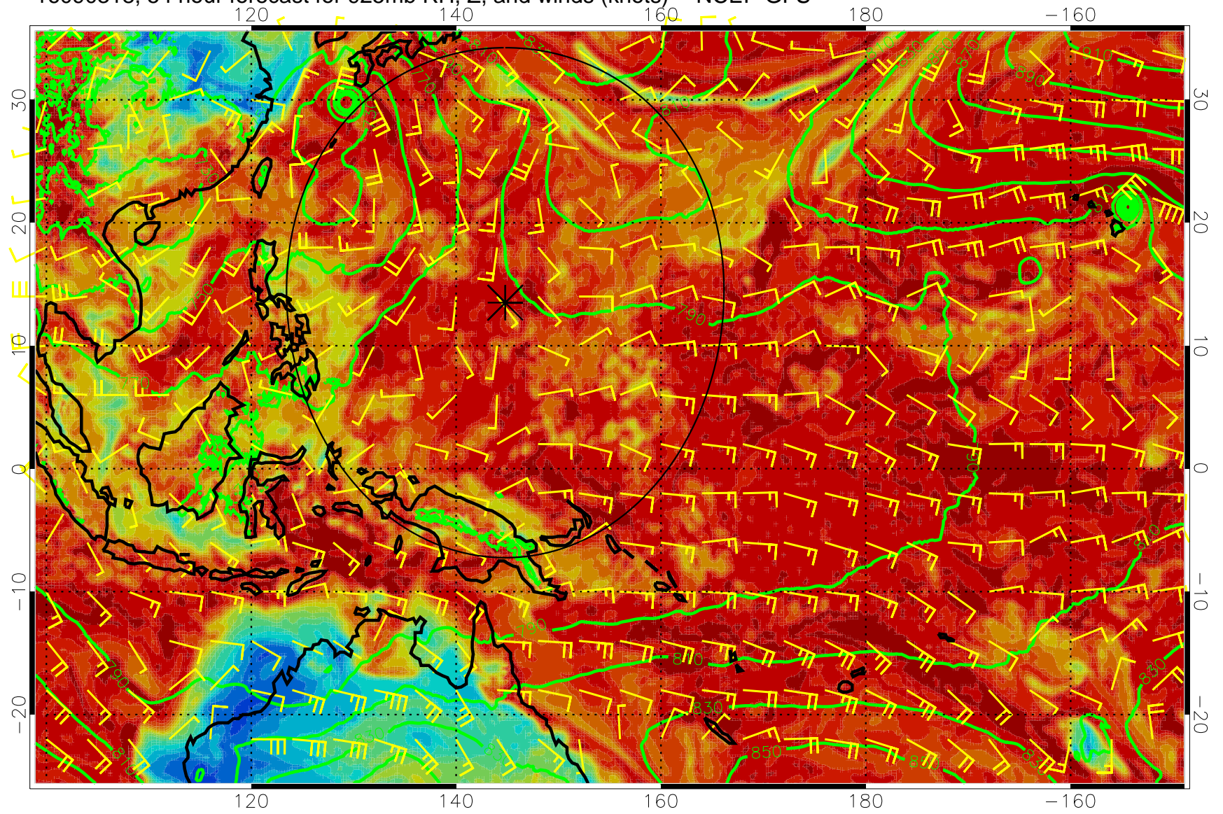
16090318, 54 hour forecast for 925mb RH, Z, and winds (knots) -- NCEP GFS
