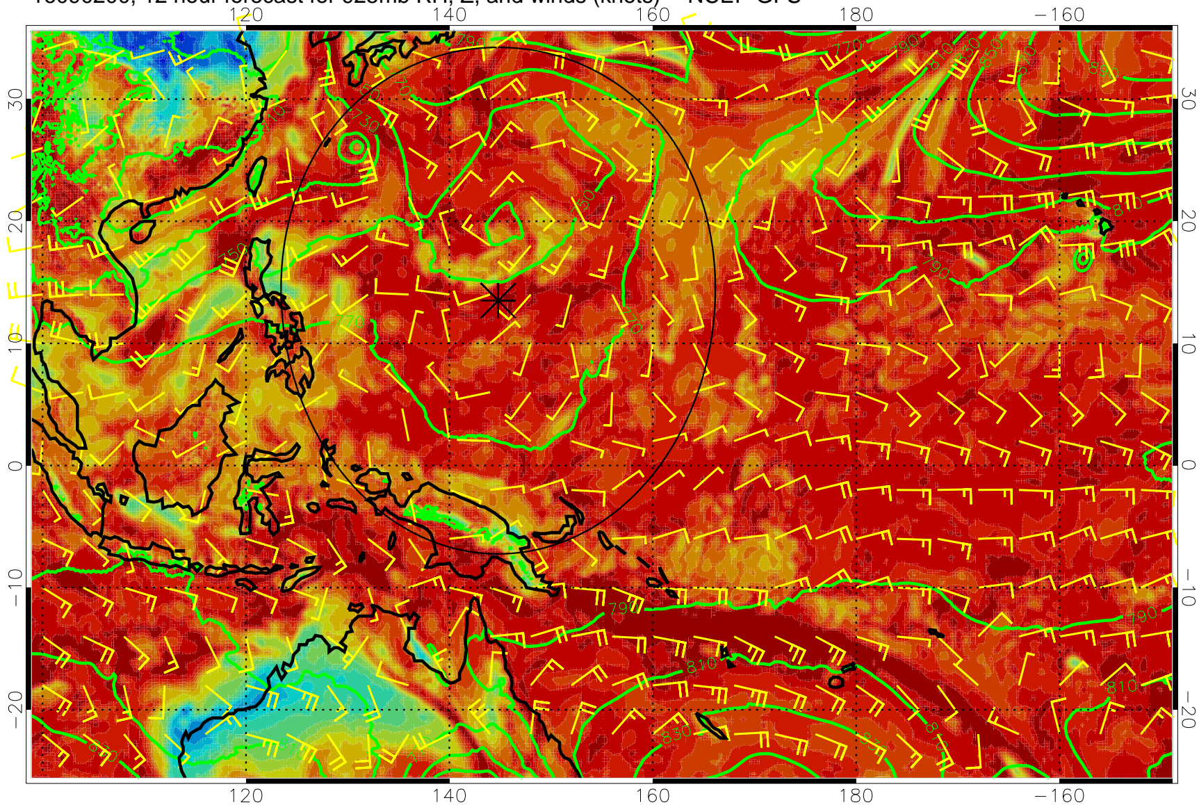
16090200, 12 hour forecast for 925mb RH, Z, and winds (knots) -- NCEP GFS
