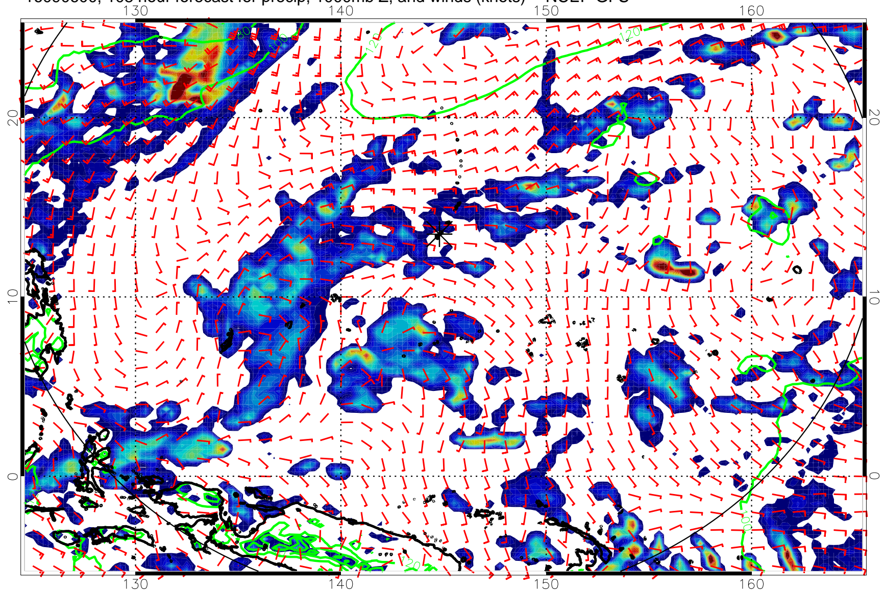
16090600, 108 hour forecast for precip, 1000mb Z, and winds (knots) -- NCEP GFS
