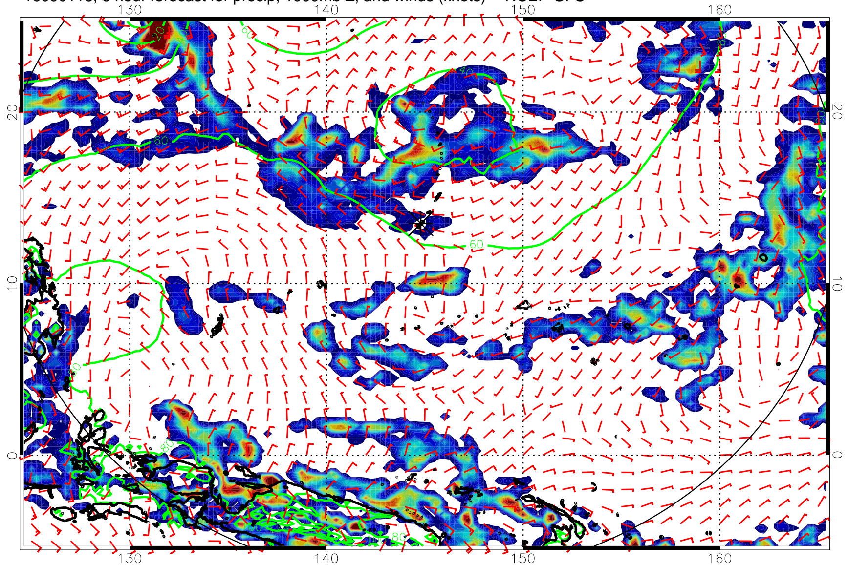
16090118, 6 hour forecast for precip, 1000mb Z, and winds (knots) -- NCEP GFS
