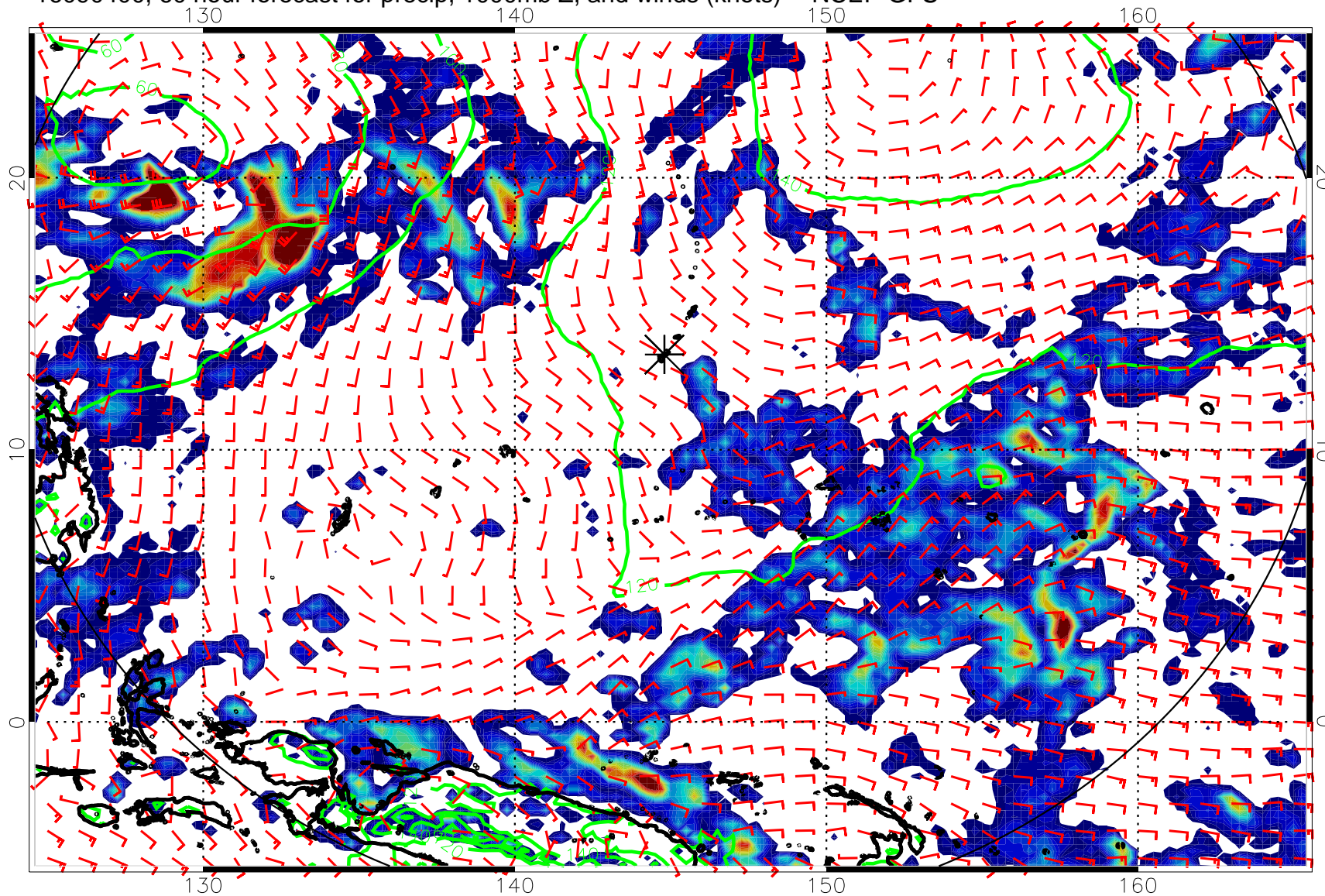
16090400, 60 hour forecast for precip, 1000mb Z, and winds (knots) -- NCEP GFS
