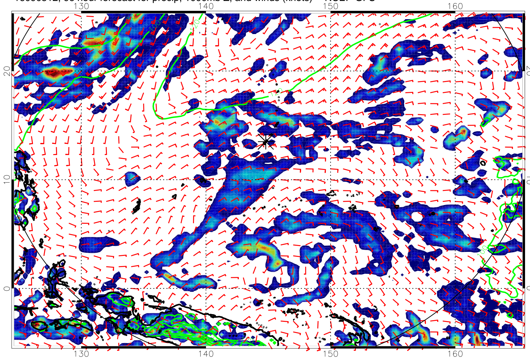
16090512, 96 hour forecast for precip, 1000mb Z, and winds (knots) -- NCEP GFS
