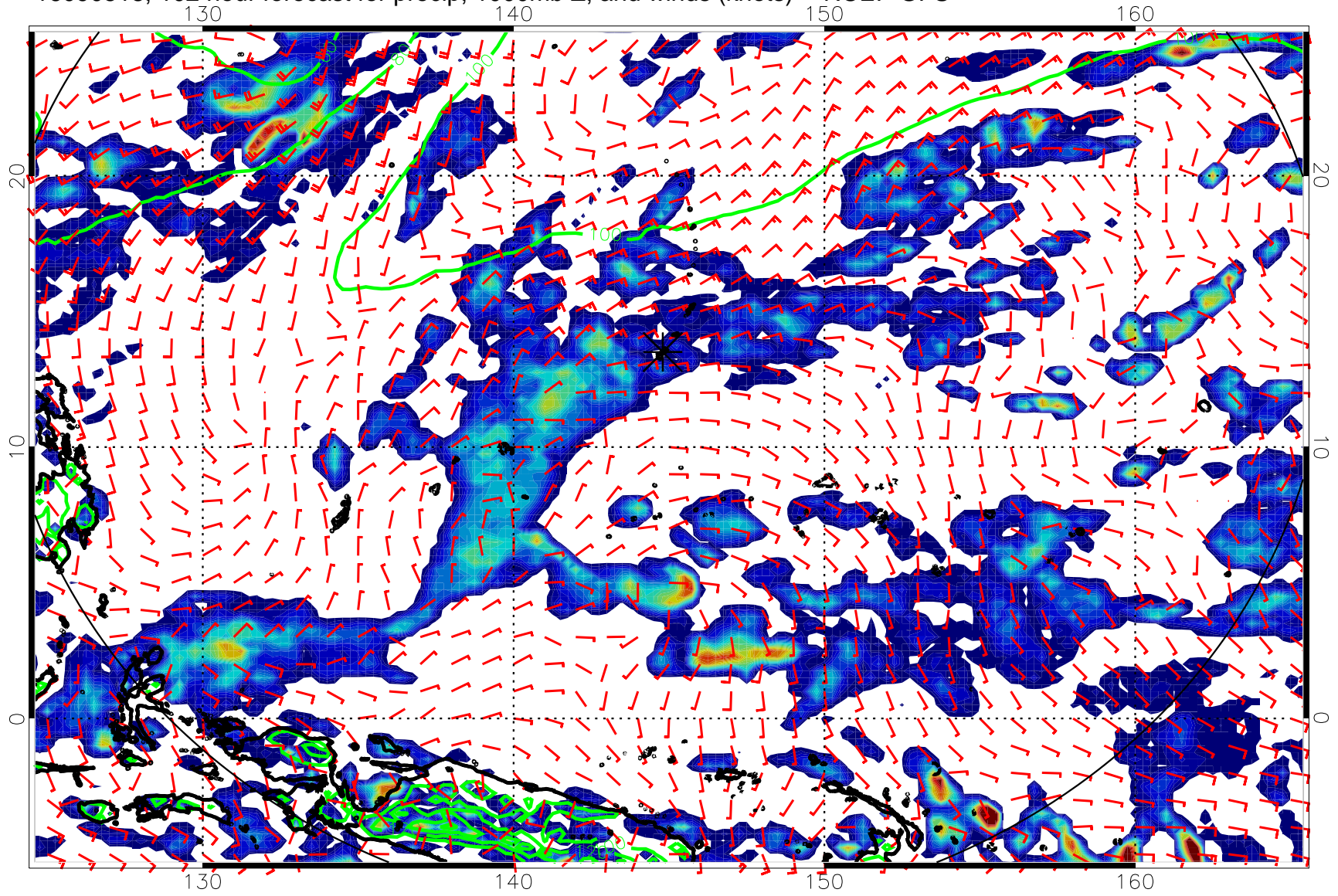
16090518, 102 hour forecast for precip, 1000mb Z, and winds (knots) -- NCEP GFS
