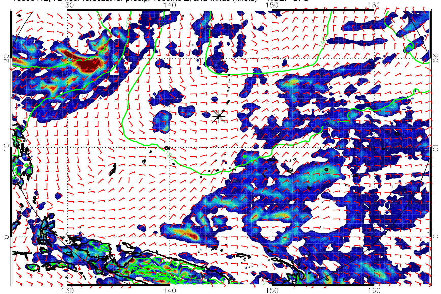
16090412, 72 hour forecast for precip, 1000mb Z, and winds (knots) -- NCEP GFS
