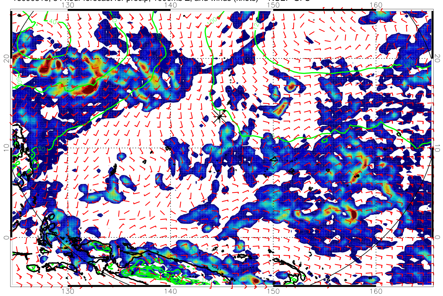
16090318, 54 hour forecast for precip, 1000mb Z, and winds (knots) -- NCEP GFS
