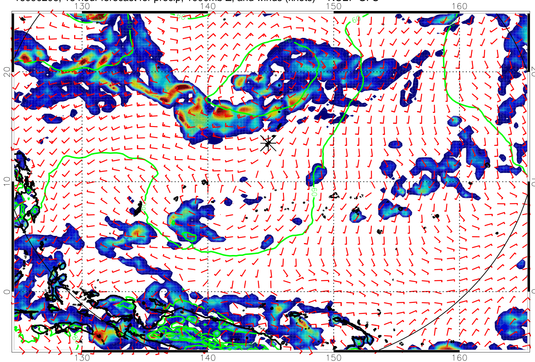
16090206, 18 hour forecast for precip, 1000mb Z, and winds (knots) -- NCEP GFS
