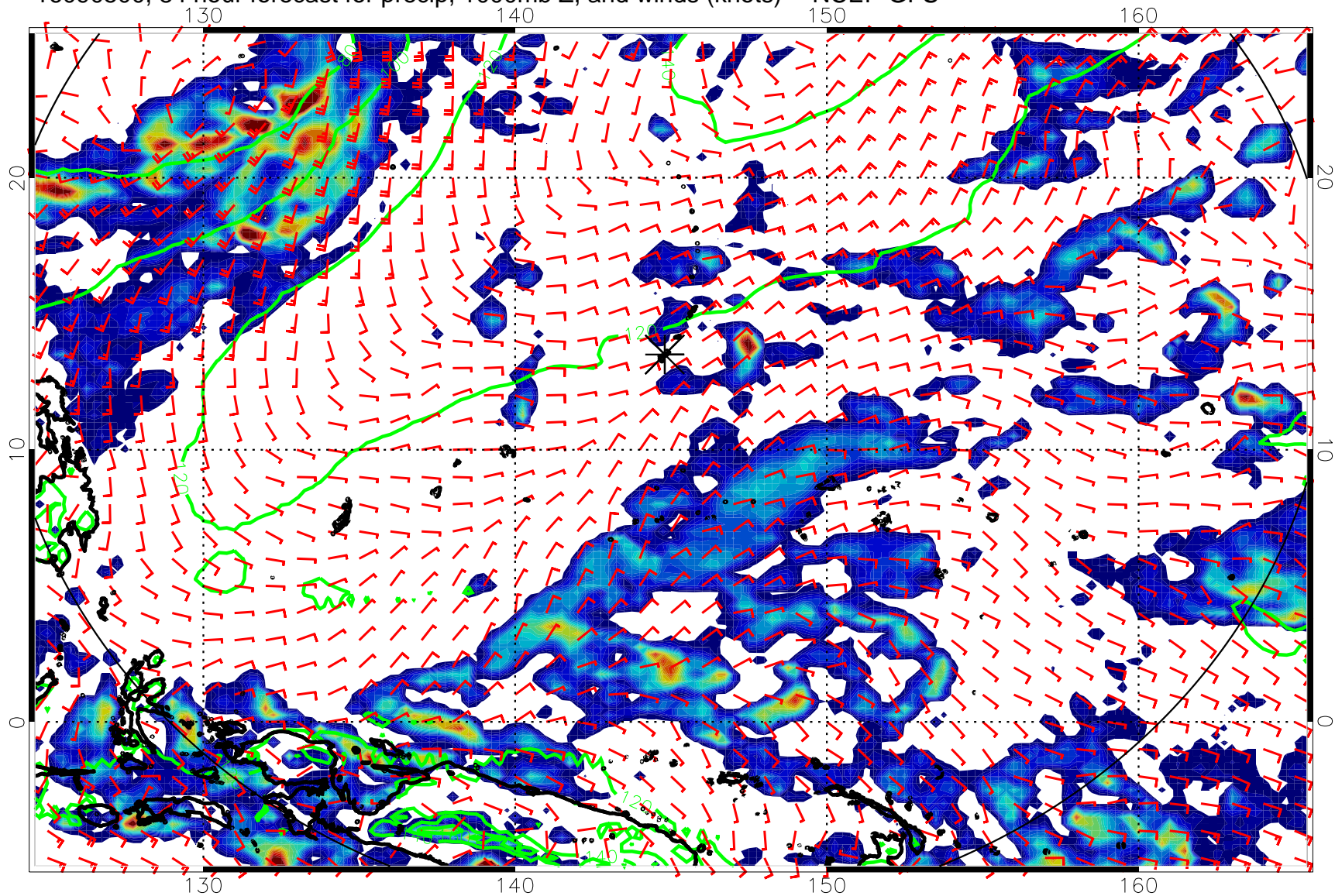
16090500, 84 hour forecast for precip, 1000mb Z, and winds (knots) -- NCEP GFS
