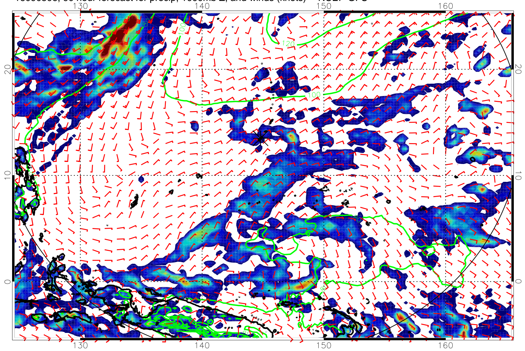
16090506, 90 hour forecast for precip, 1000mb Z, and winds (knots) -- NCEP GFS
