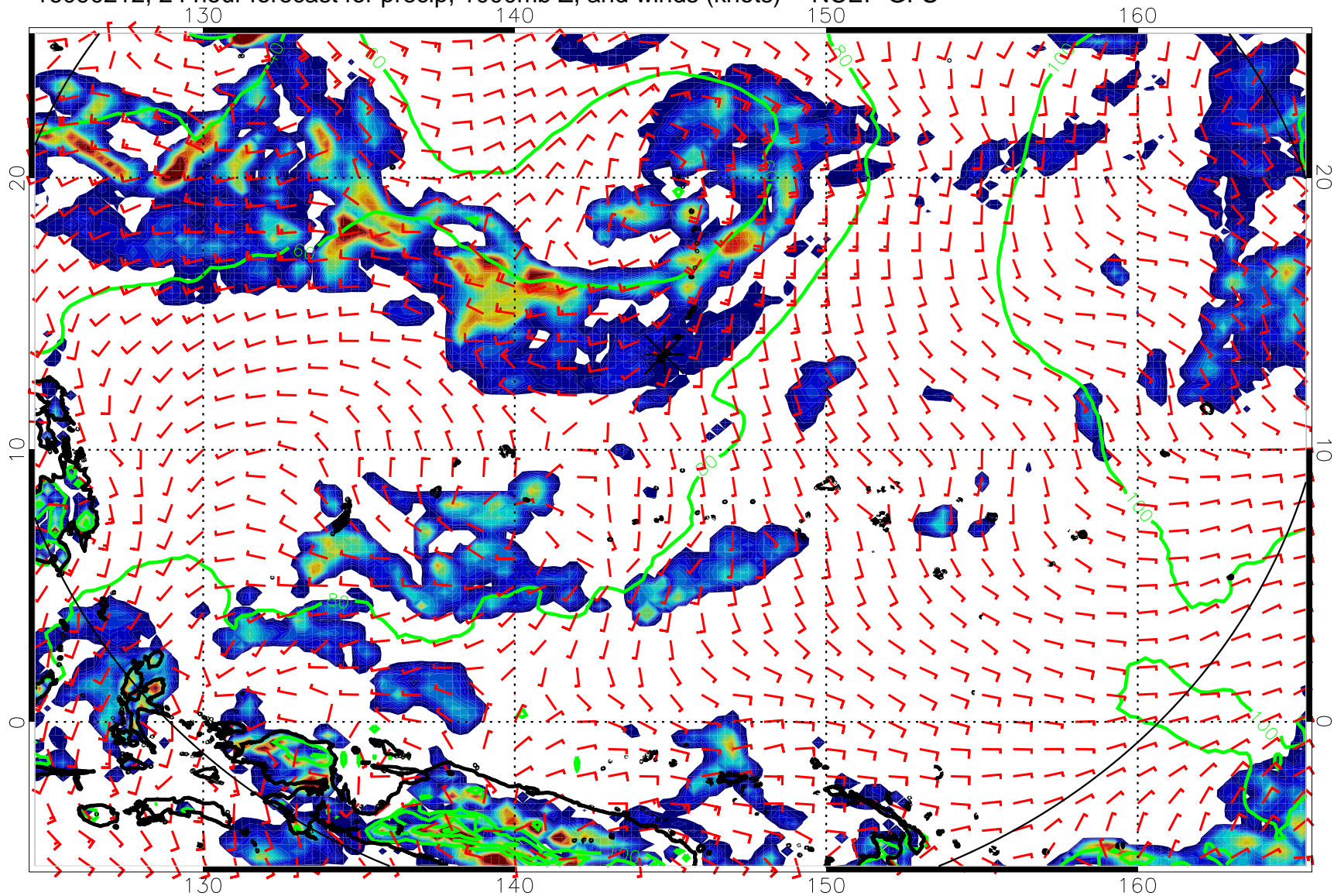
16090212, 24 hour forecast for precip, 1000mb Z, and winds (knots) -- NCEP GFS
