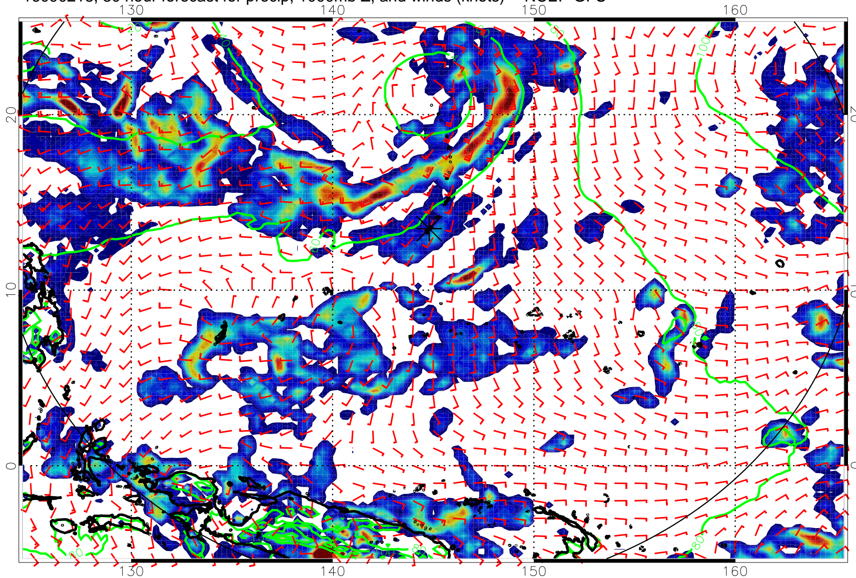
16090218, 30 hour forecast for precip, 1000mb Z, and winds (knots) -- NCEP GFS
