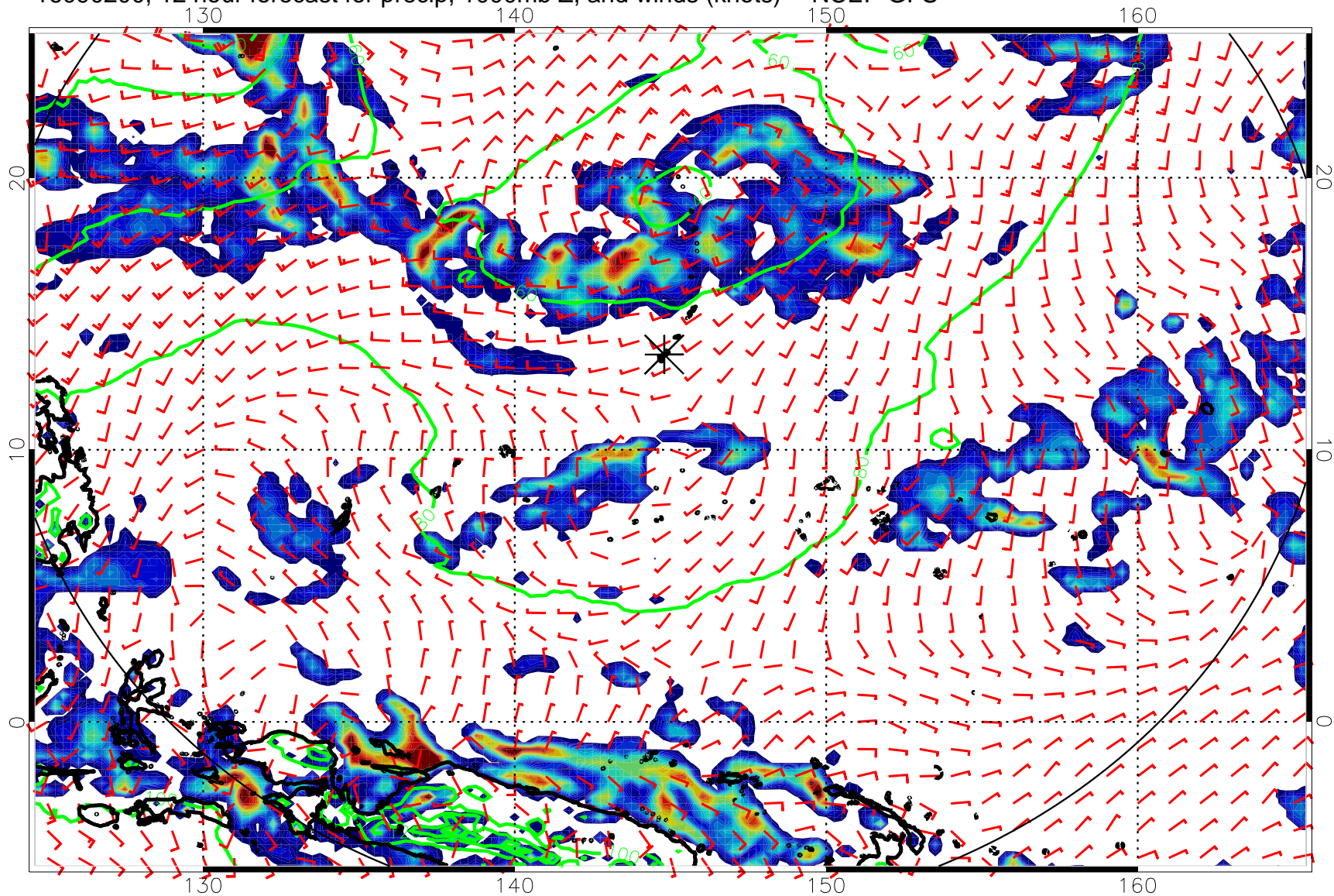
16090200, 12 hour forecast for precip, 1000mb Z, and winds (knots) -- NCEP GFS
