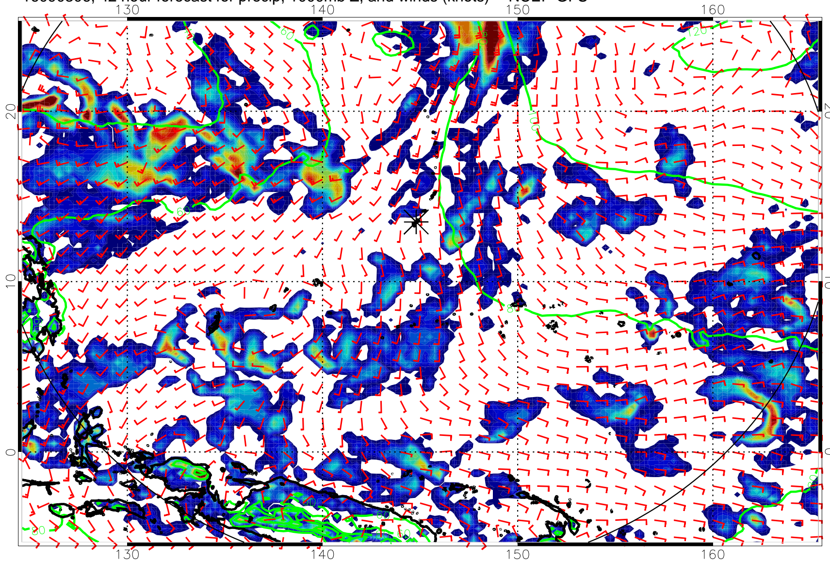
16090306, 42 hour forecast for precip, 1000mb Z, and winds (knots) -- NCEP GFS
