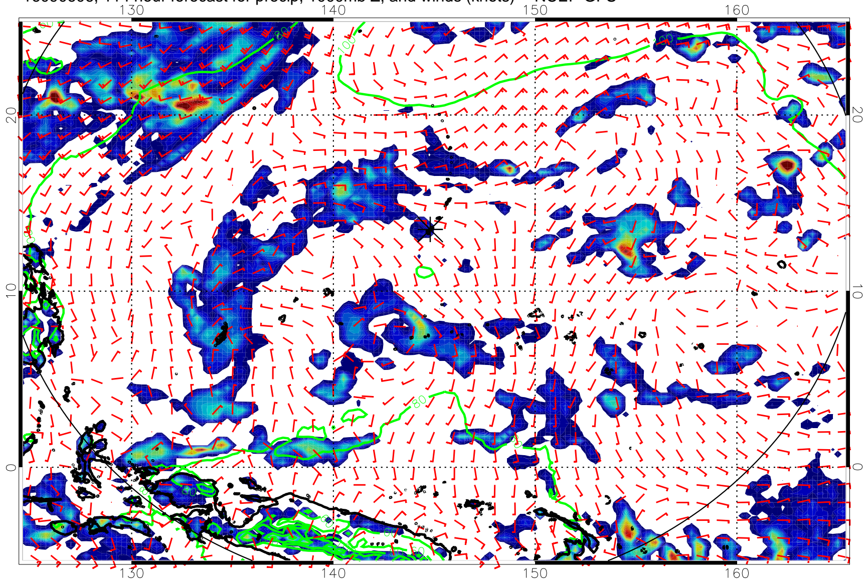
16090606, 114 hour forecast for precip, 1000mb Z, and winds (knots) -- NCEP GFS
