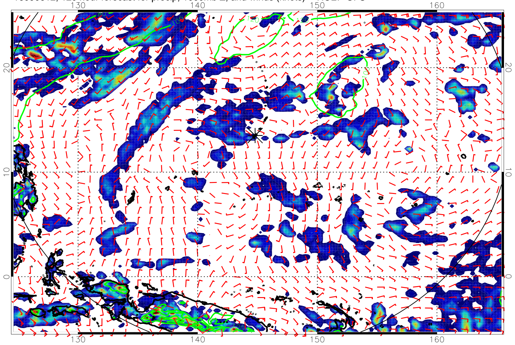
16090612, 120 hour forecast for precip, 1000mb Z, and winds (knots) -- NCEP GFS
