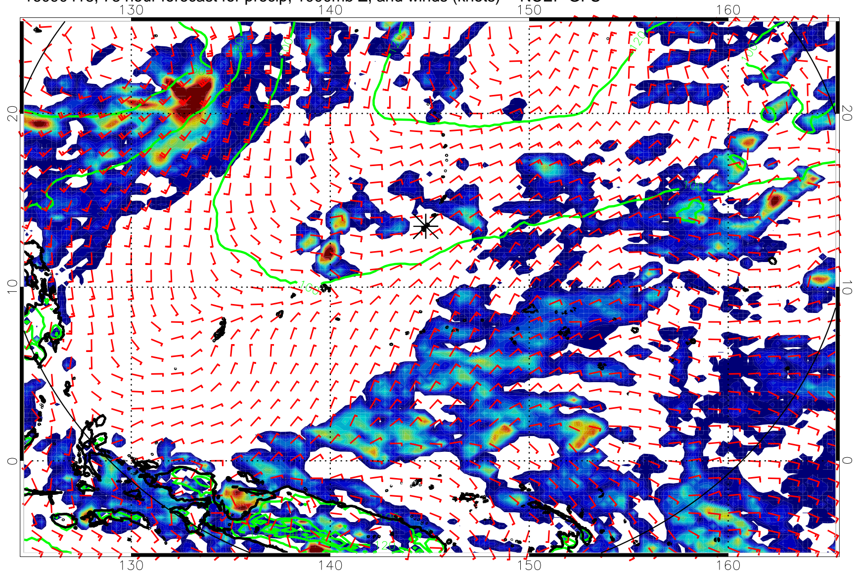
16090418, 78 hour forecast for precip, 1000mb Z, and winds (knots) -- NCEP GFS
