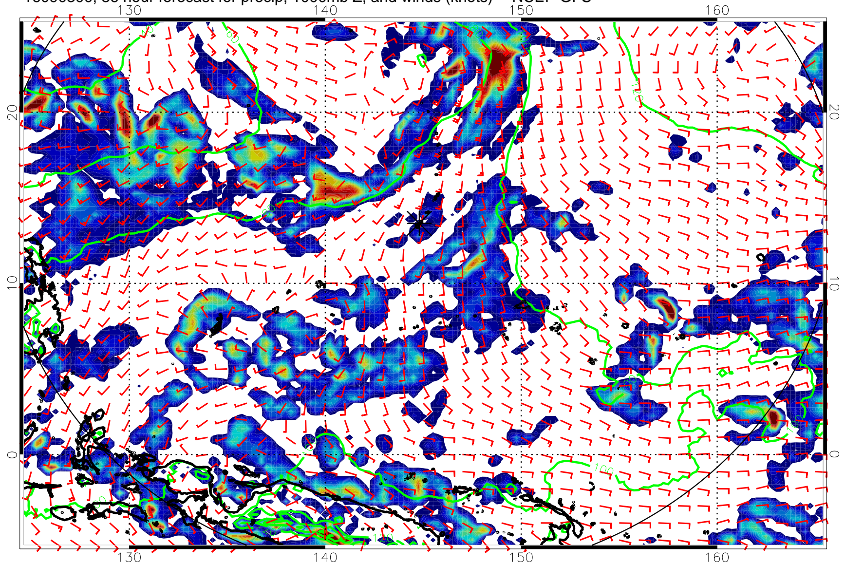
16090300, 36 hour forecast for precip, 1000mb Z, and winds (knots) -- NCEP GFS
