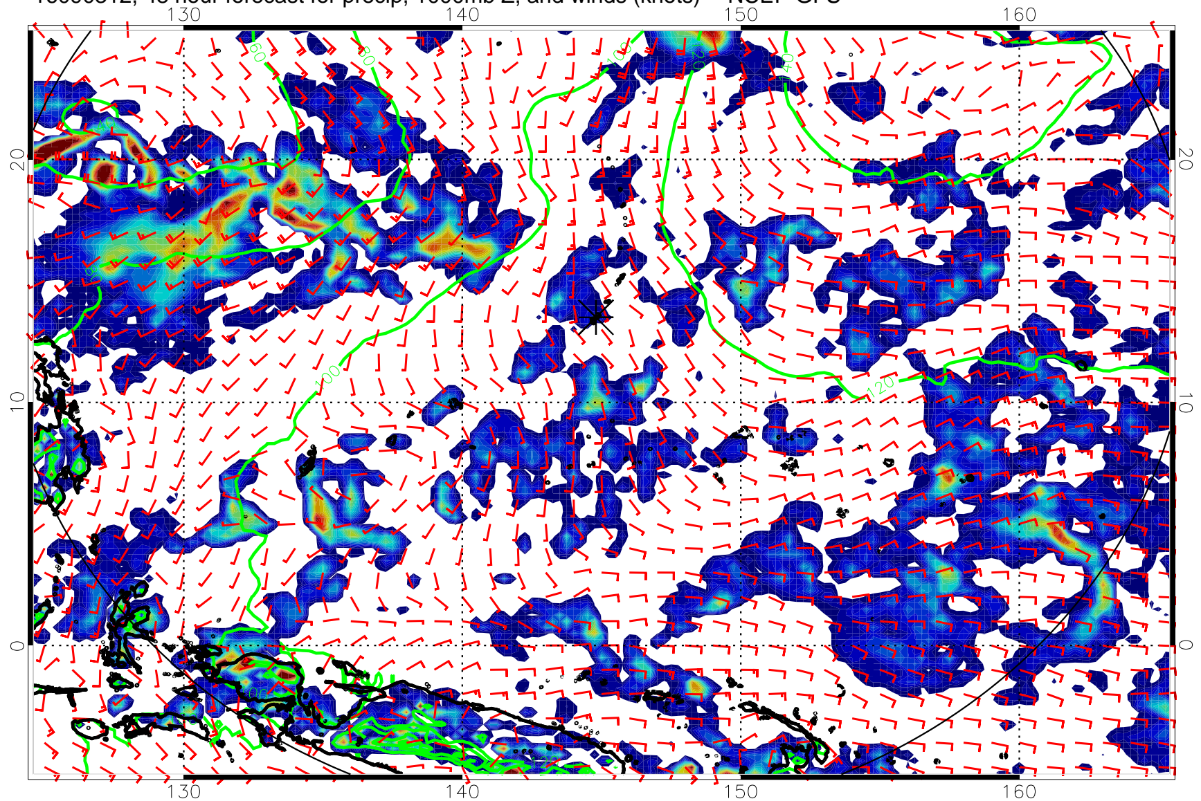
16090312, 48 hour forecast for precip, 1000mb Z, and winds (knots) -- NCEP GFS
