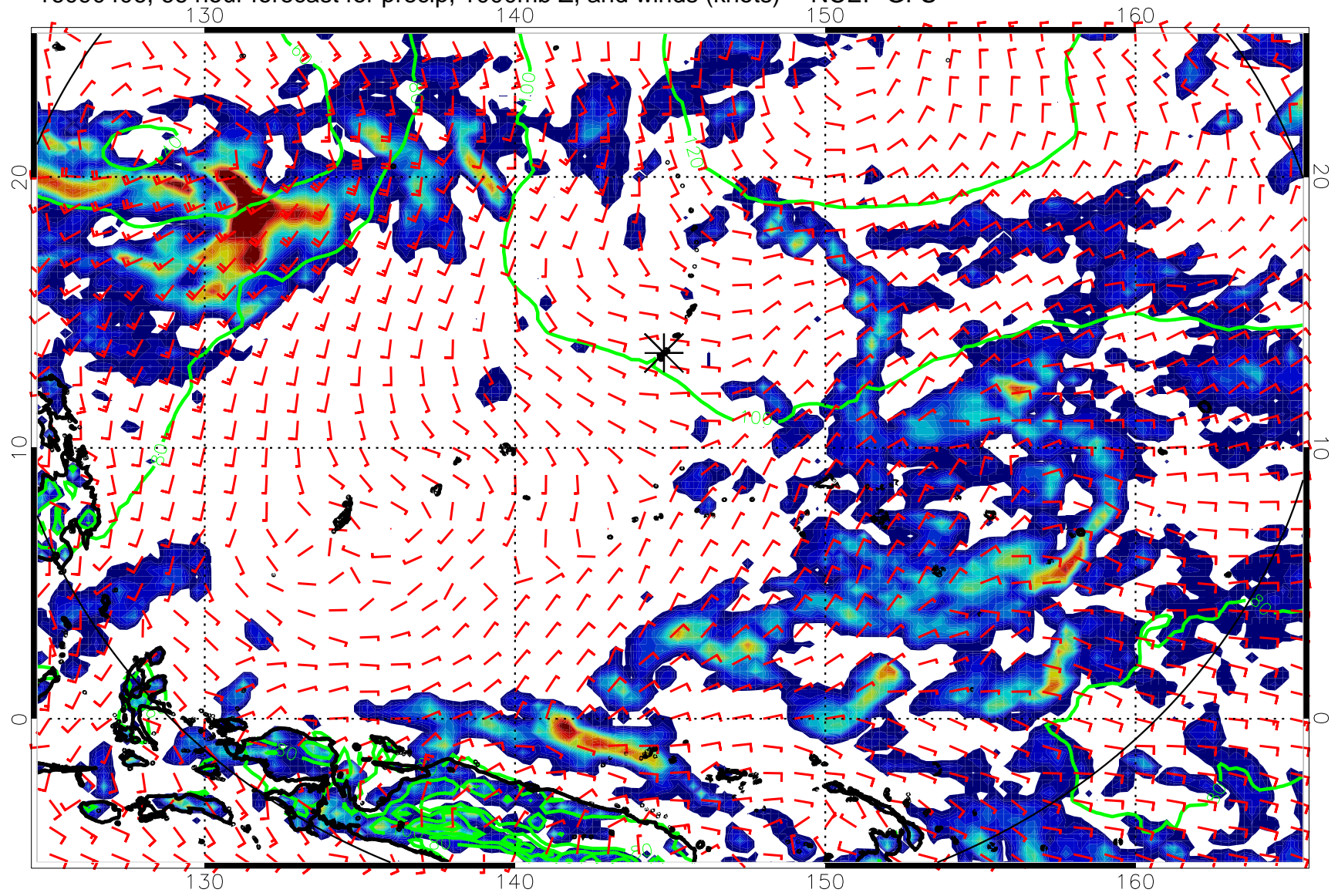
16090406, 66 hour forecast for precip, 1000mb Z, and winds (knots) -- NCEP GFS
