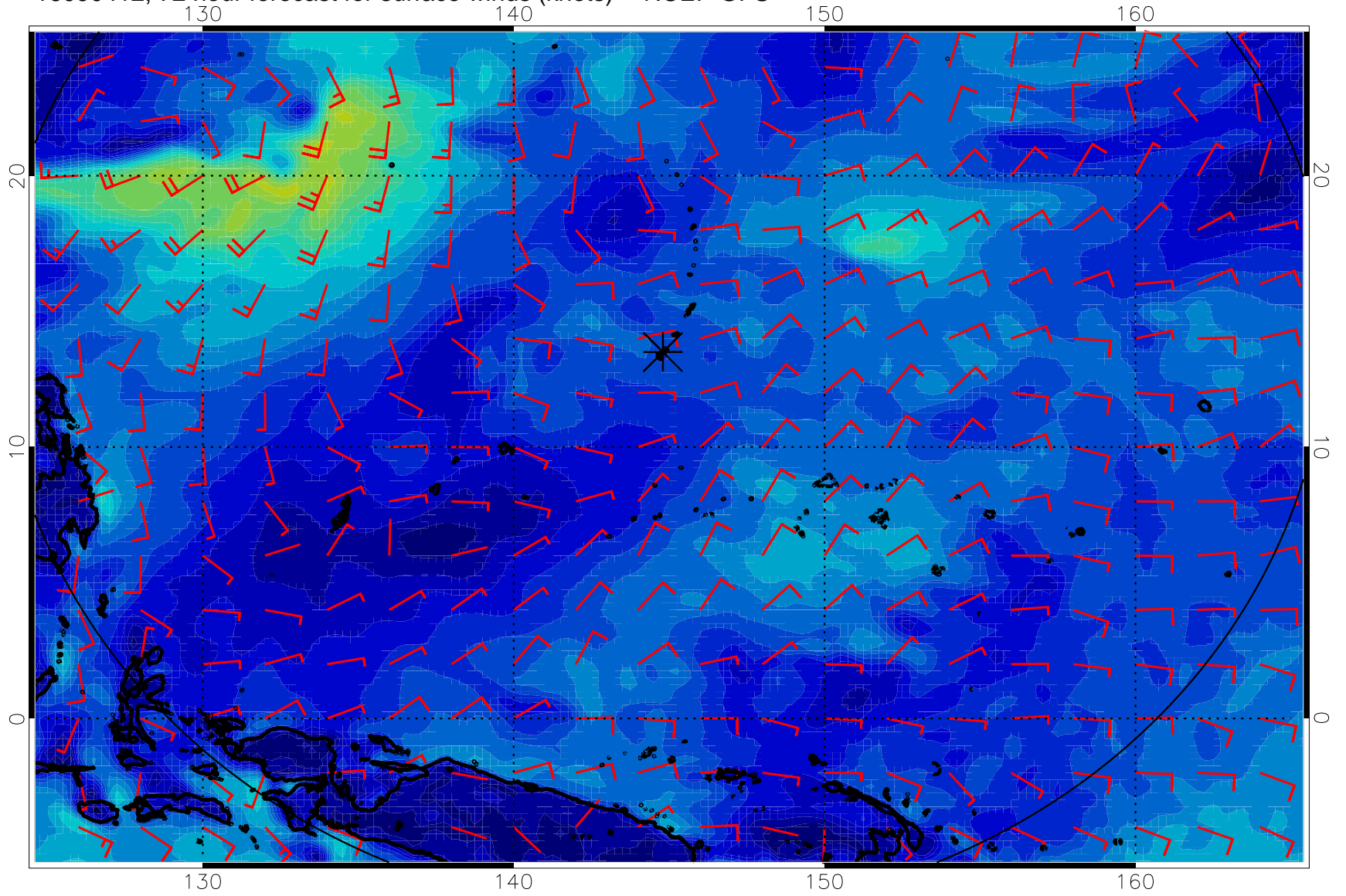
16090412, 72 hour forecast for surface winds (knots) -- NCEP GFS
