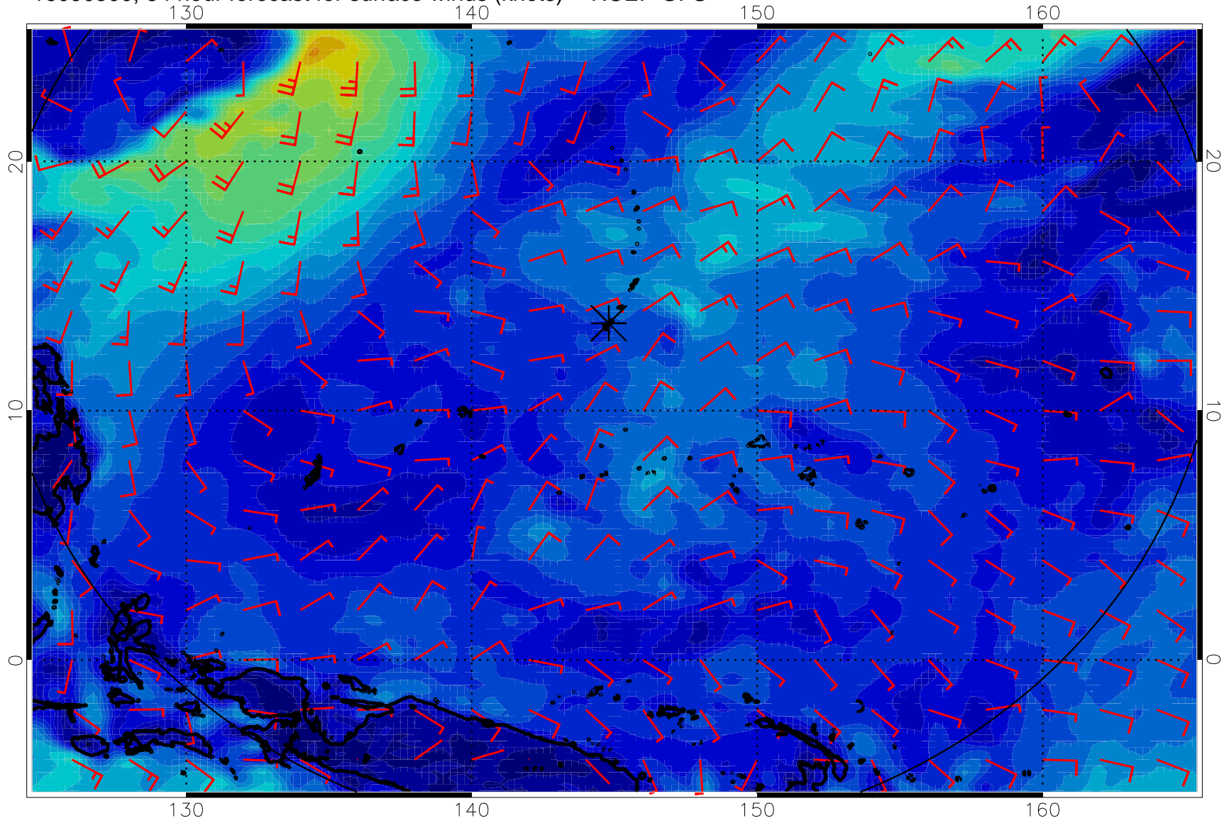
16090500, 84 hour forecast for surface winds (knots) -- NCEP GFS
