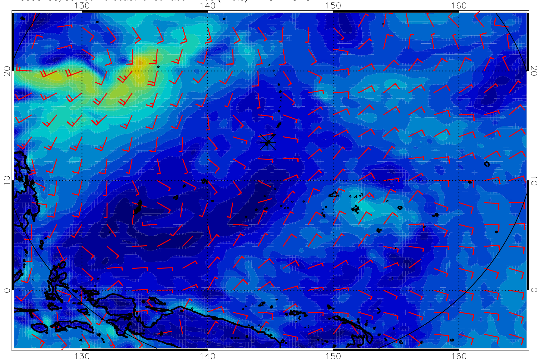
16090406, 66 hour forecast for surface winds (knots) -- NCEP GFS
