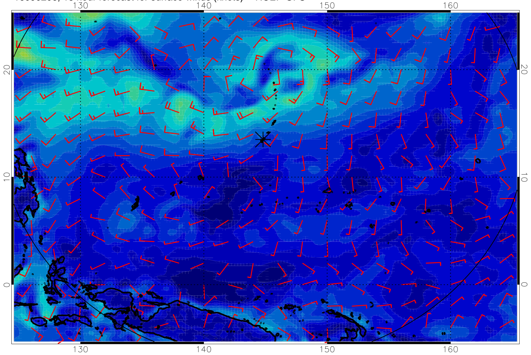
16090206, 18 hour forecast for surface winds (knots) -- NCEP GFS
