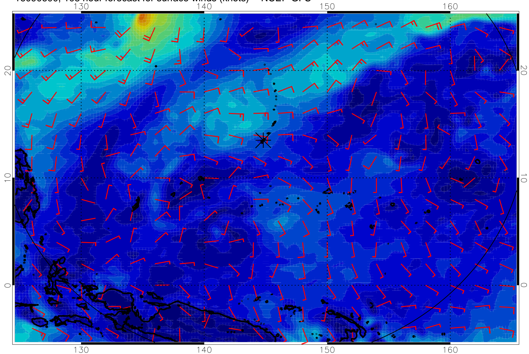
16090600, 108 hour forecast for surface winds (knots) -- NCEP GFS
