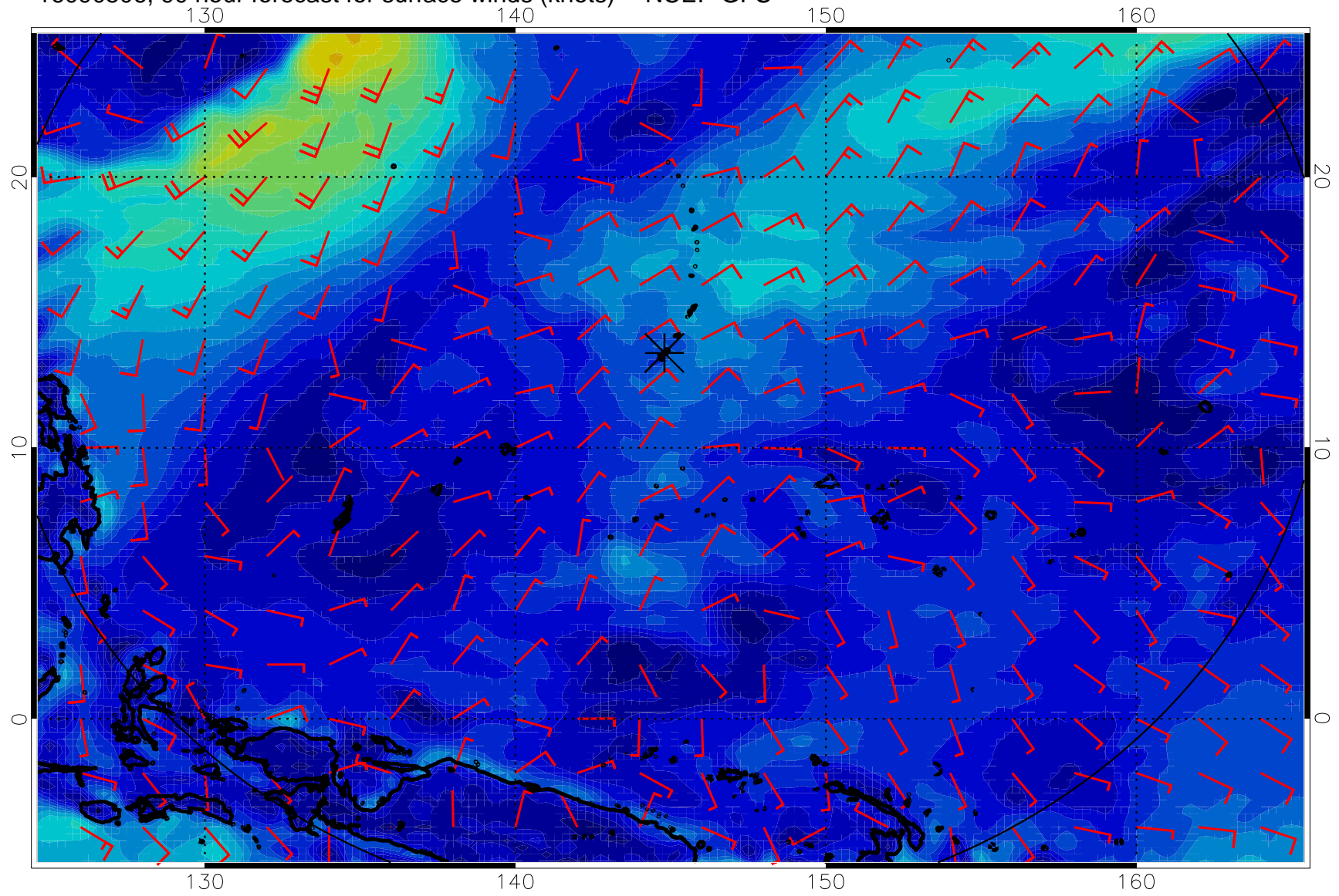
16090506, 90 hour forecast for surface winds (knots) -- NCEP GFS
