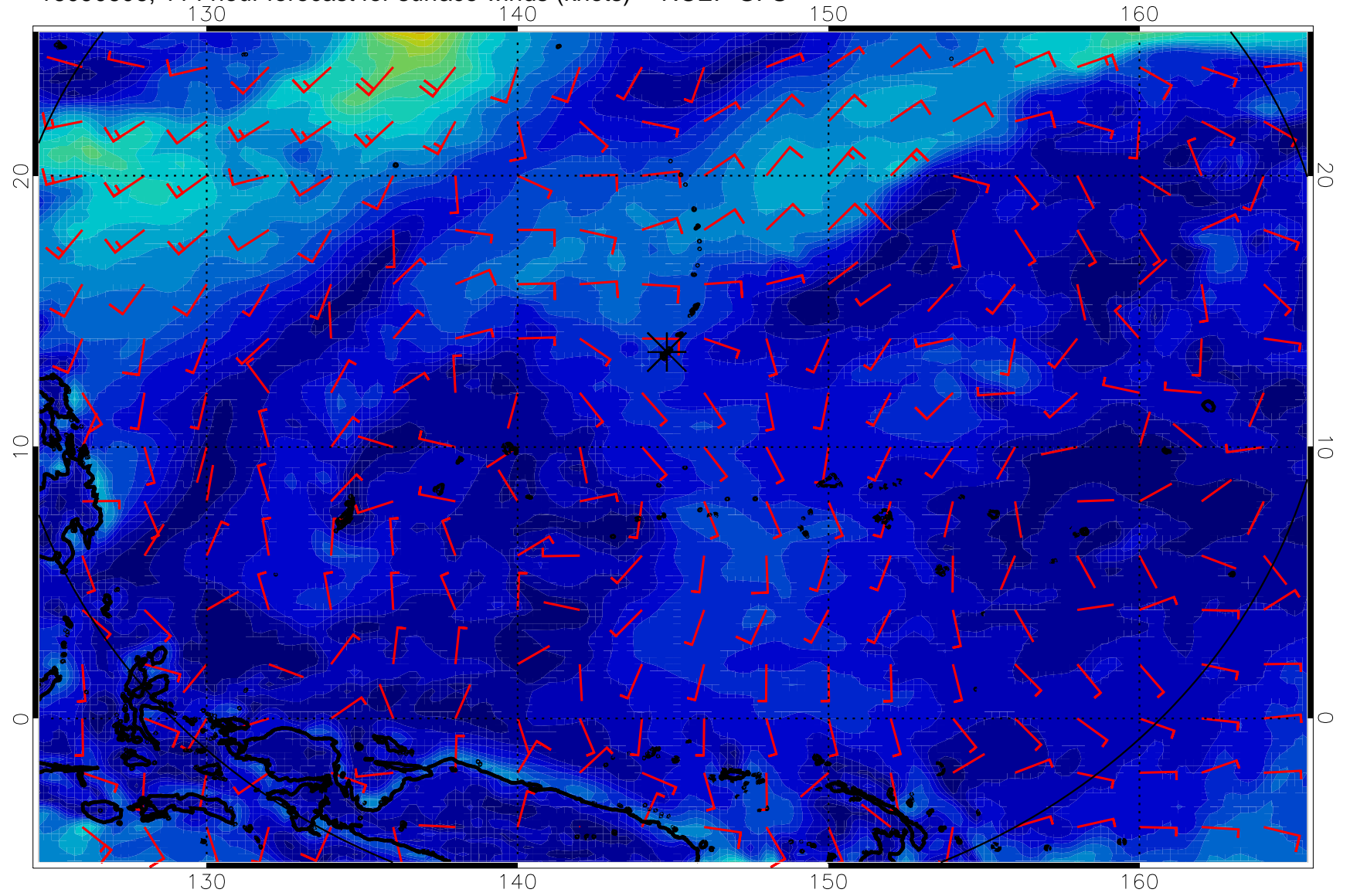
16090606, 114 hour forecast for surface winds (knots) -- NCEP GFS
