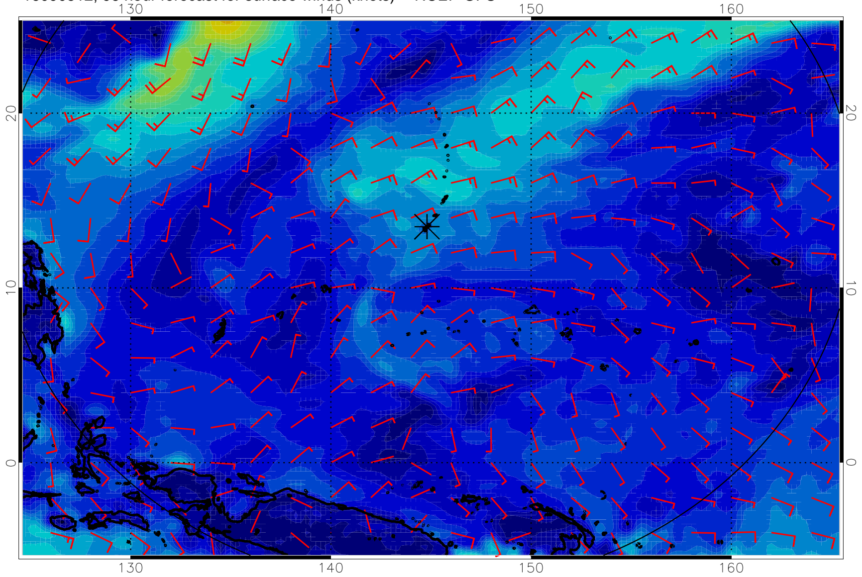
16090512, 96 hour forecast for surface winds (knots) -- NCEP GFS
