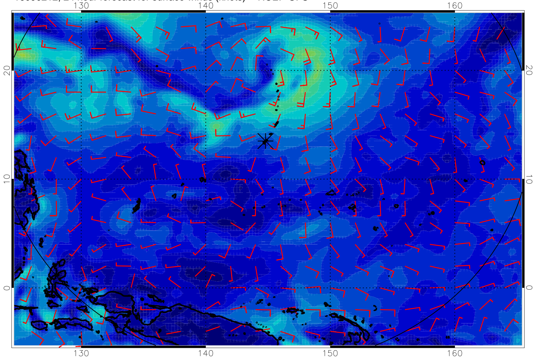
16090212, 24 hour forecast for surface winds (knots) -- NCEP GFS
