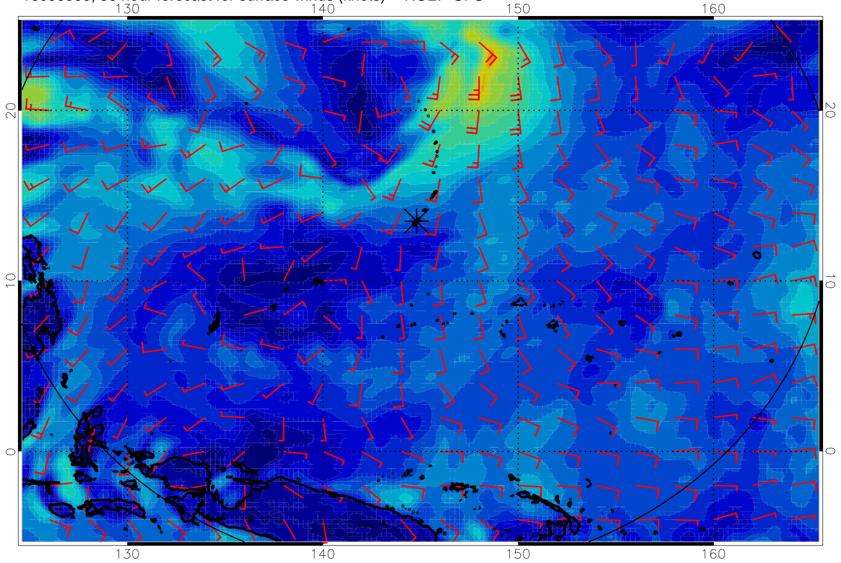
16090300, 36 hour forecast for surface winds (knots) -- NCEP GFS
