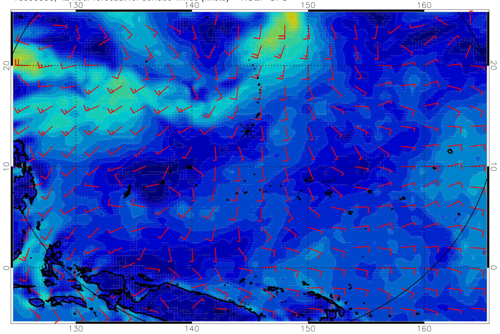
16090306, 42 hour forecast for surface winds (knots) -- NCEP GFS
