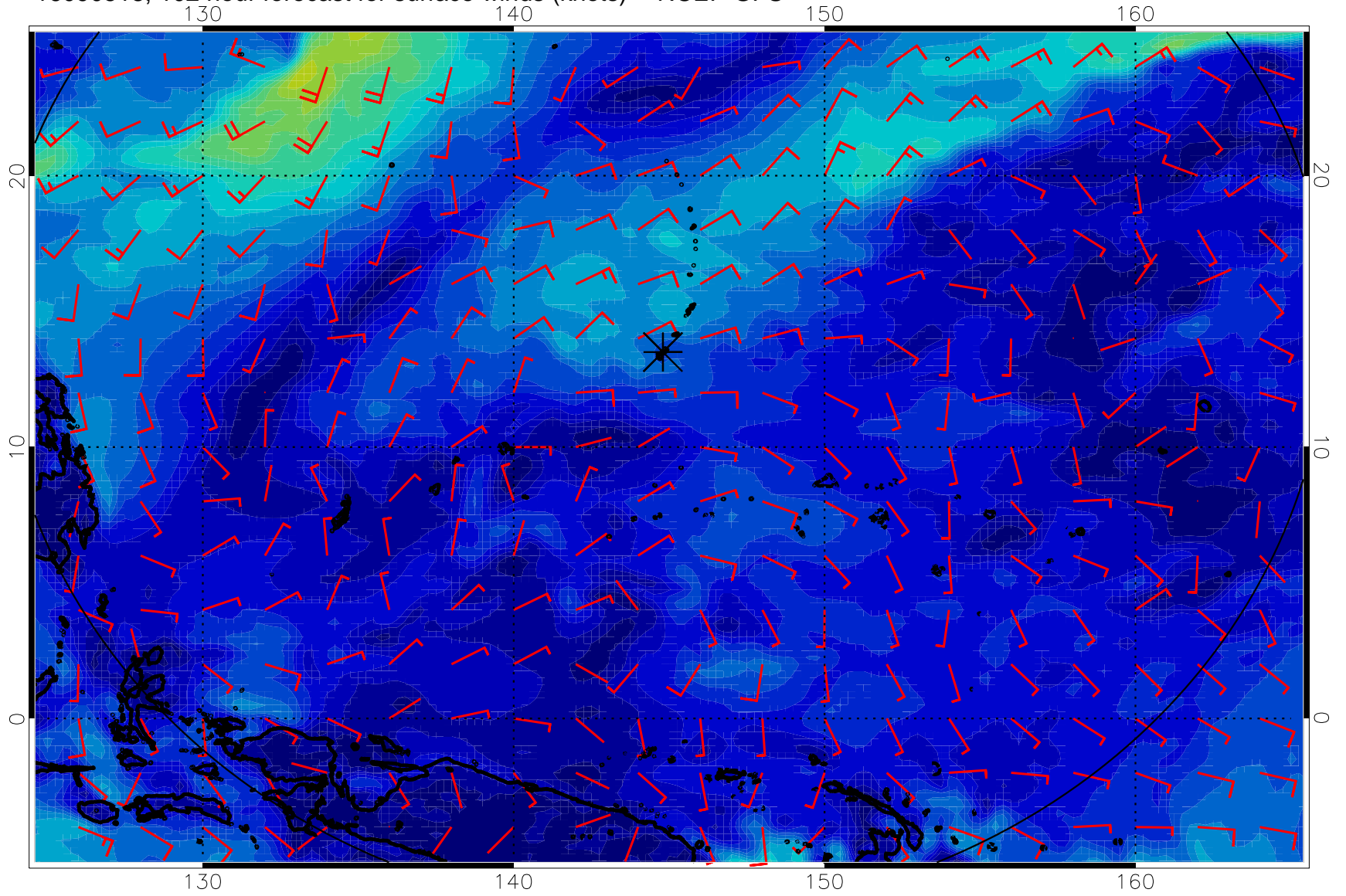
16090518, 102 hour forecast for surface winds (knots) -- NCEP GFS
