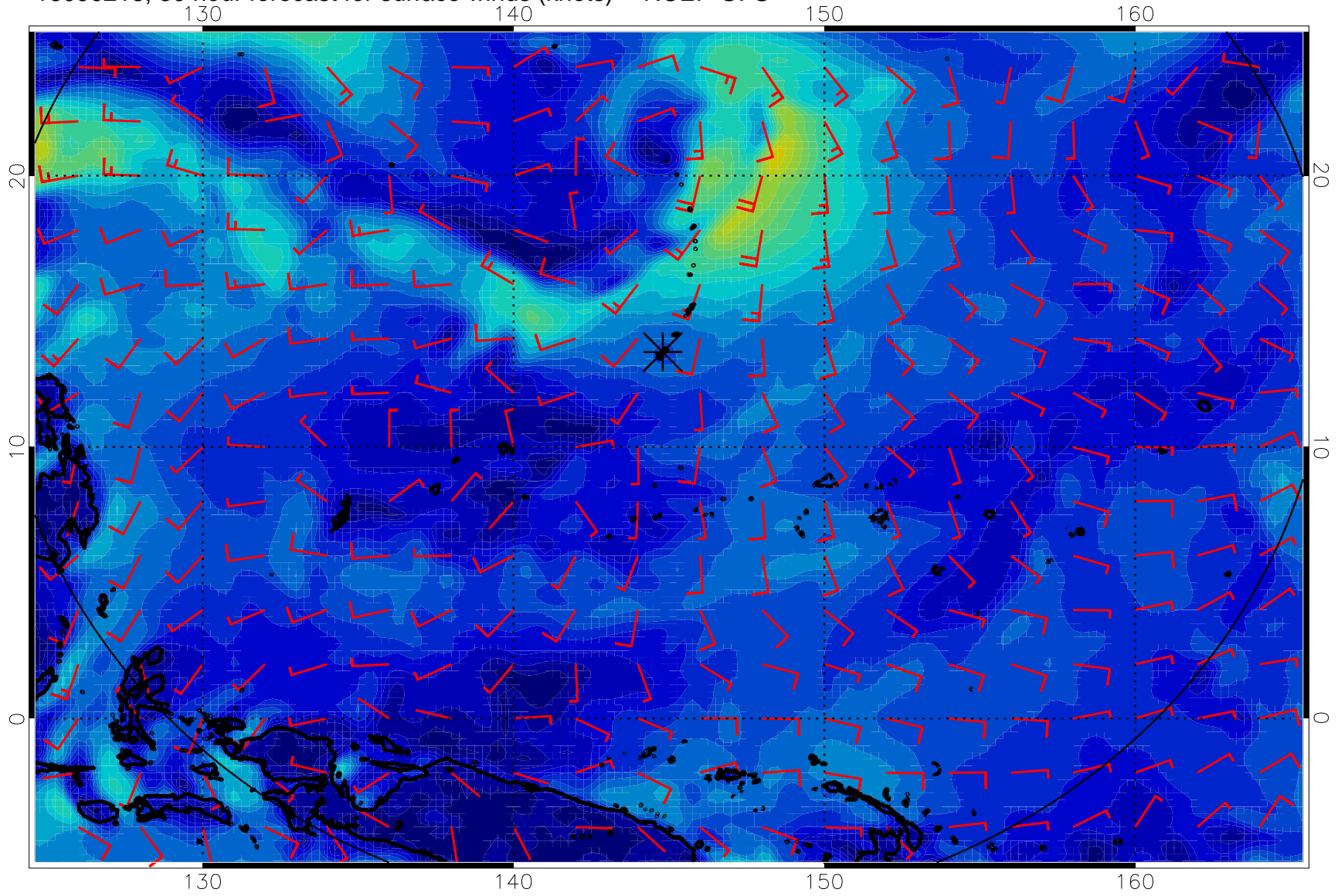
16090218, 30 hour forecast for surface winds (knots) -- NCEP GFS
