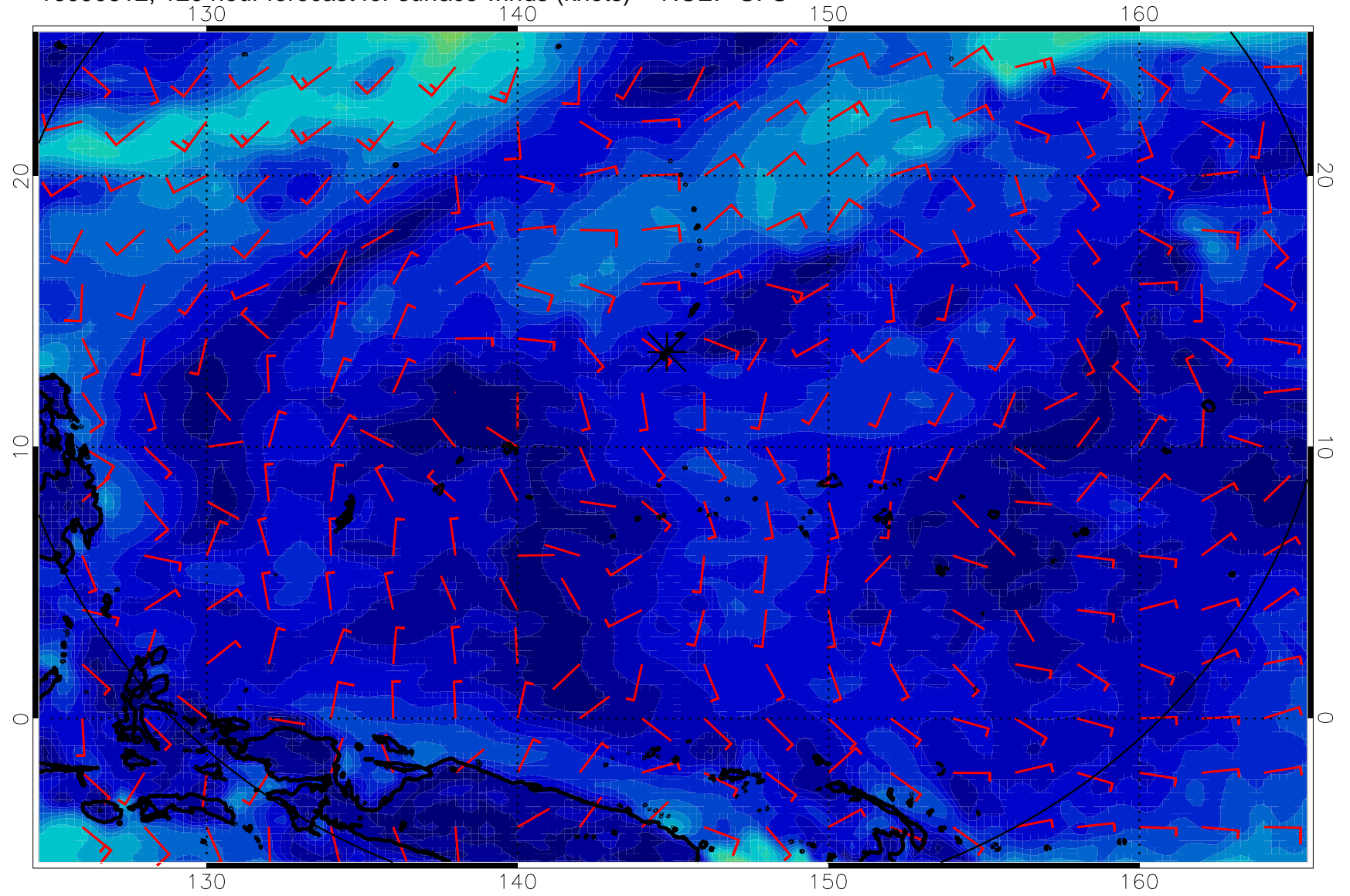
16090612, 120 hour forecast for surface winds (knots) -- NCEP GFS
