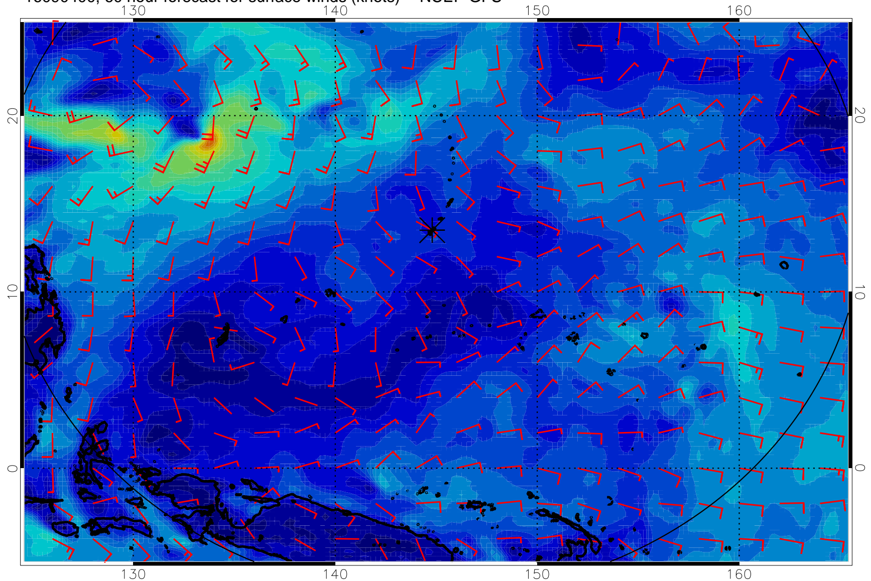
16090400, 60 hour forecast for surface winds (knots) -- NCEP GFS
