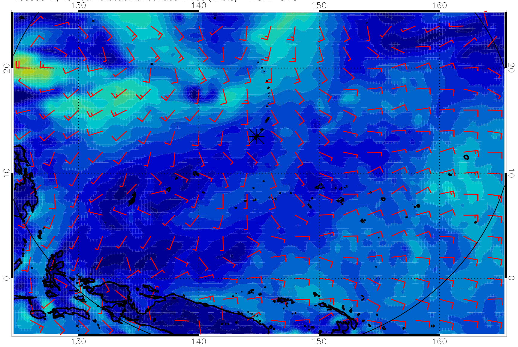
16090312, 48 hour forecast for surface winds (knots) -- NCEP GFS
