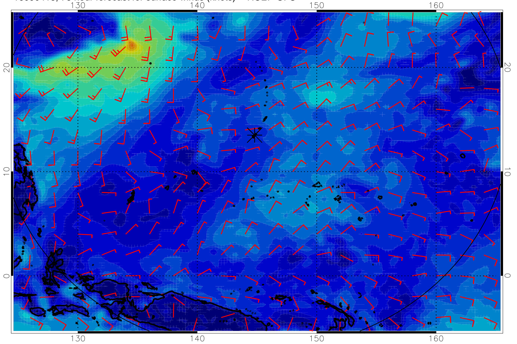
16090418, 78 hour forecast for surface winds (knots) -- NCEP GFS
