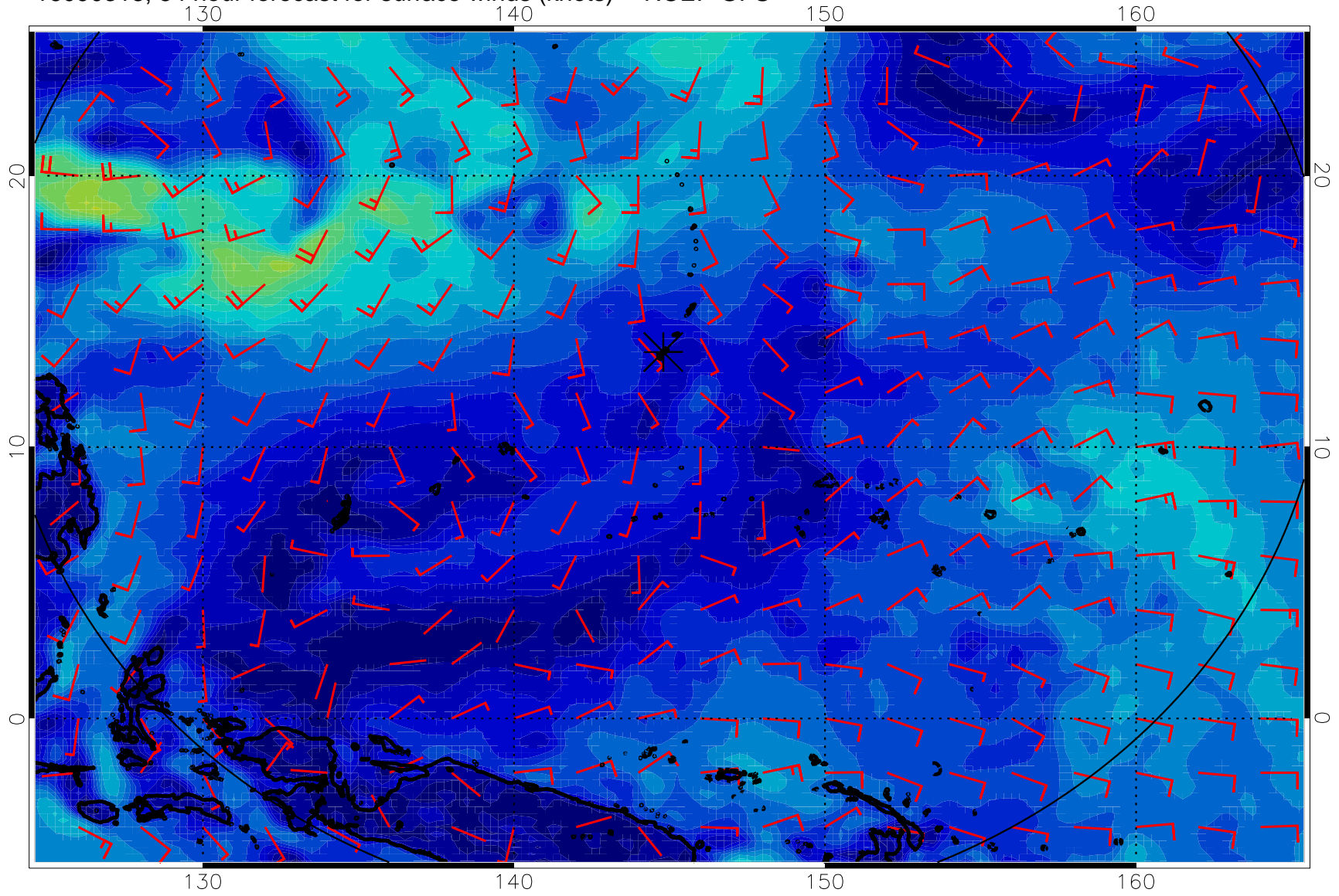
16090318, 54 hour forecast for surface winds (knots) -- NCEP GFS
