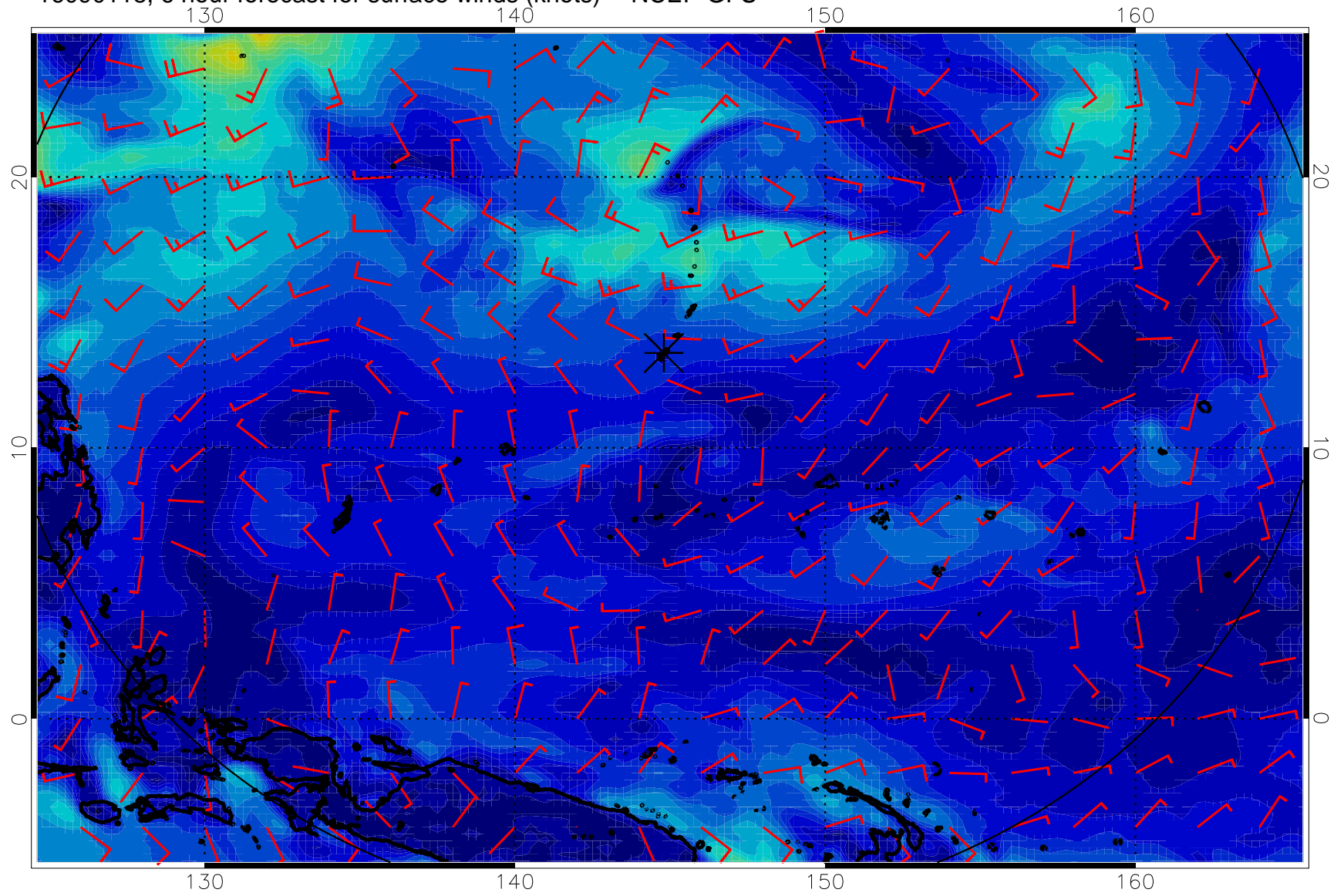
16090118, 6 hour forecast for surface winds (knots) -- NCEP GFS
