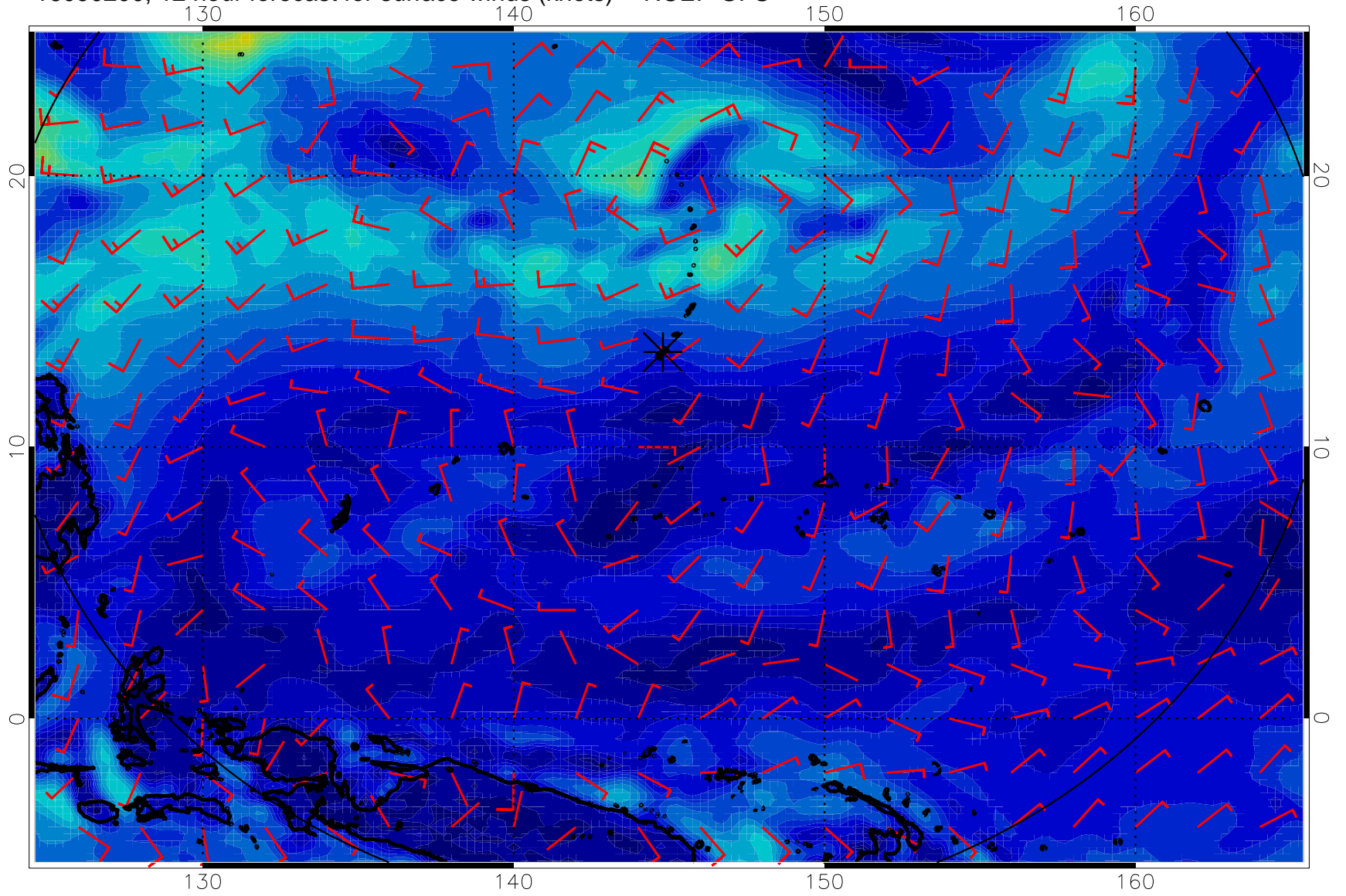
16090200, 12 hour forecast for surface winds (knots) -- NCEP GFS
