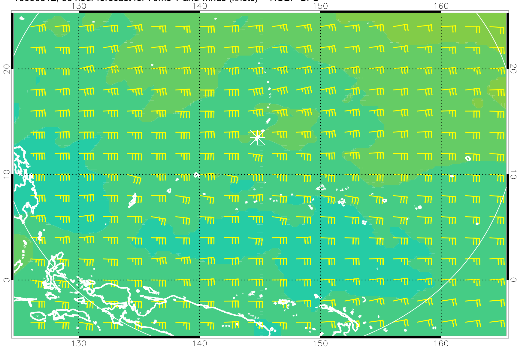
16090512, 96 hour forecast for 70mb T and winds (knots) -- NCEP GFS
