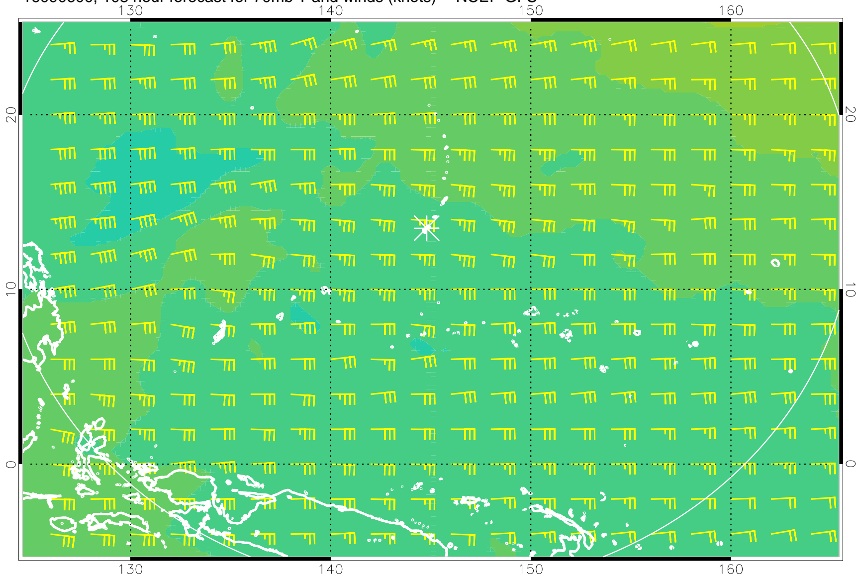
16090600, 108 hour forecast for 70mb T and winds (knots) -- NCEP GFS
