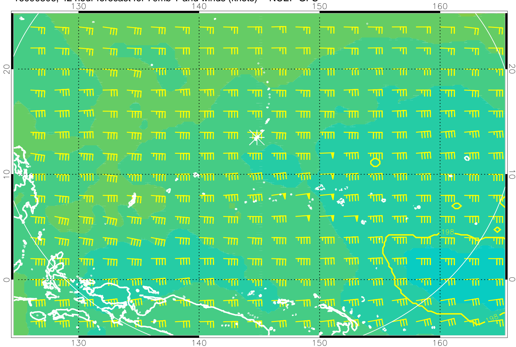
16090306, 42 hour forecast for 70mb T and winds (knots) -- NCEP GFS
