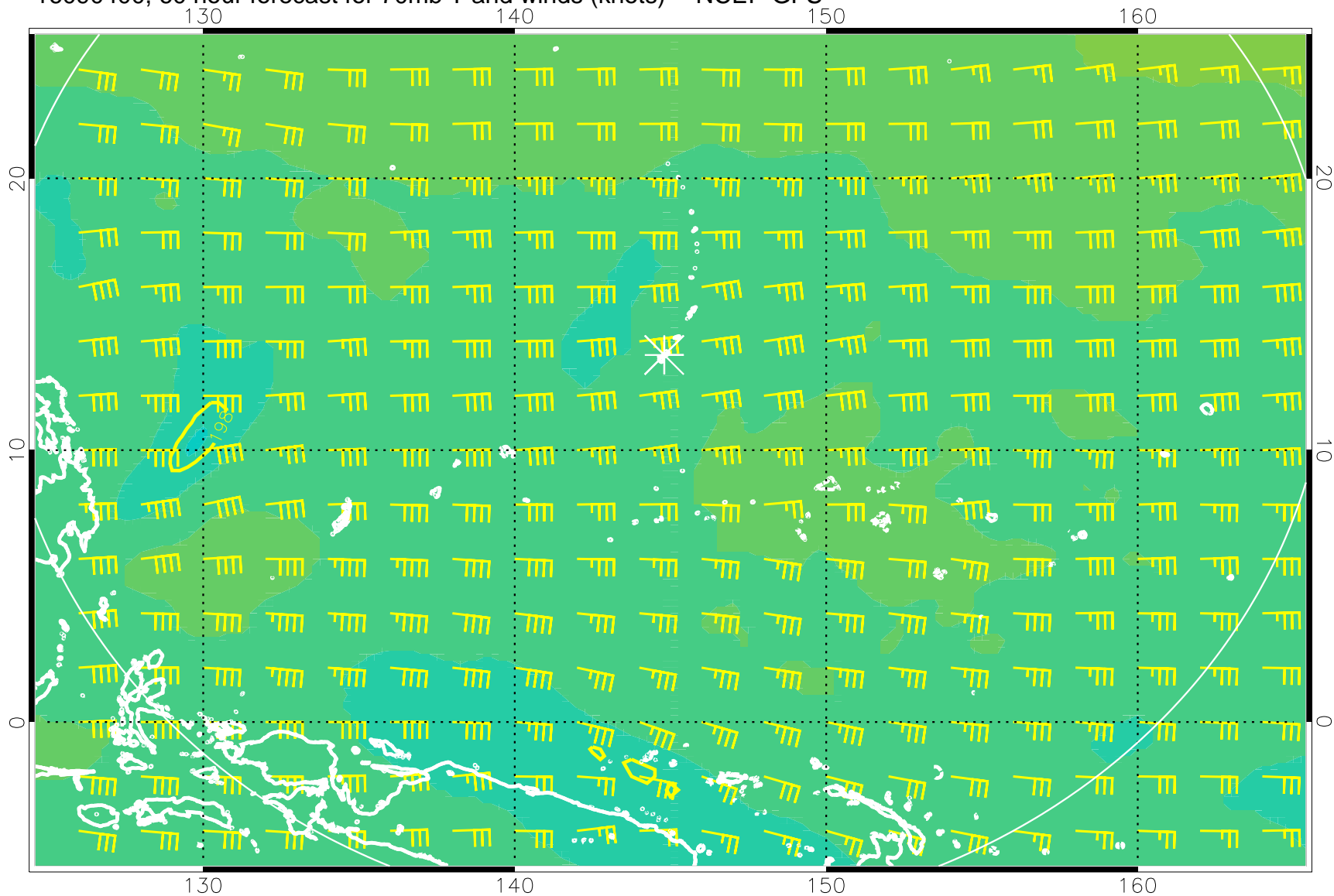
16090400, 60 hour forecast for 70mb T and winds (knots) -- NCEP GFS
