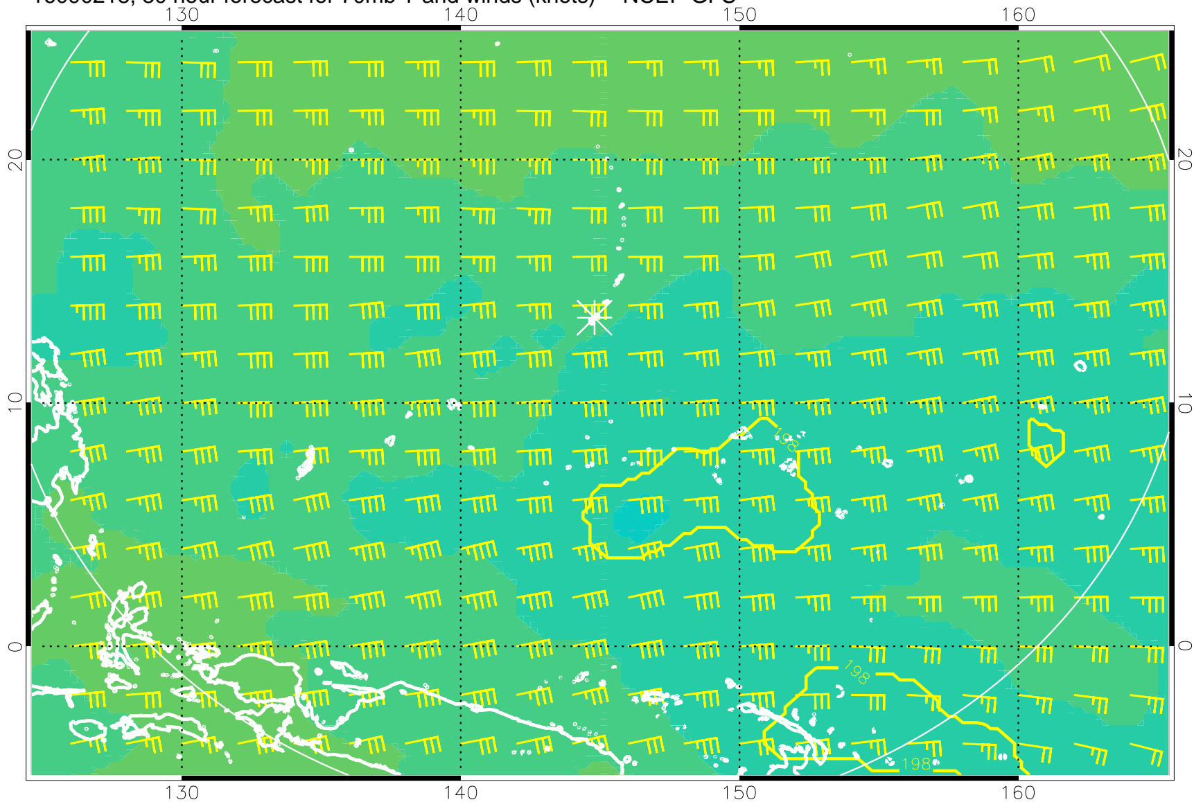
16090218, 30 hour forecast for 70mb T and winds (knots) -- NCEP GFS
