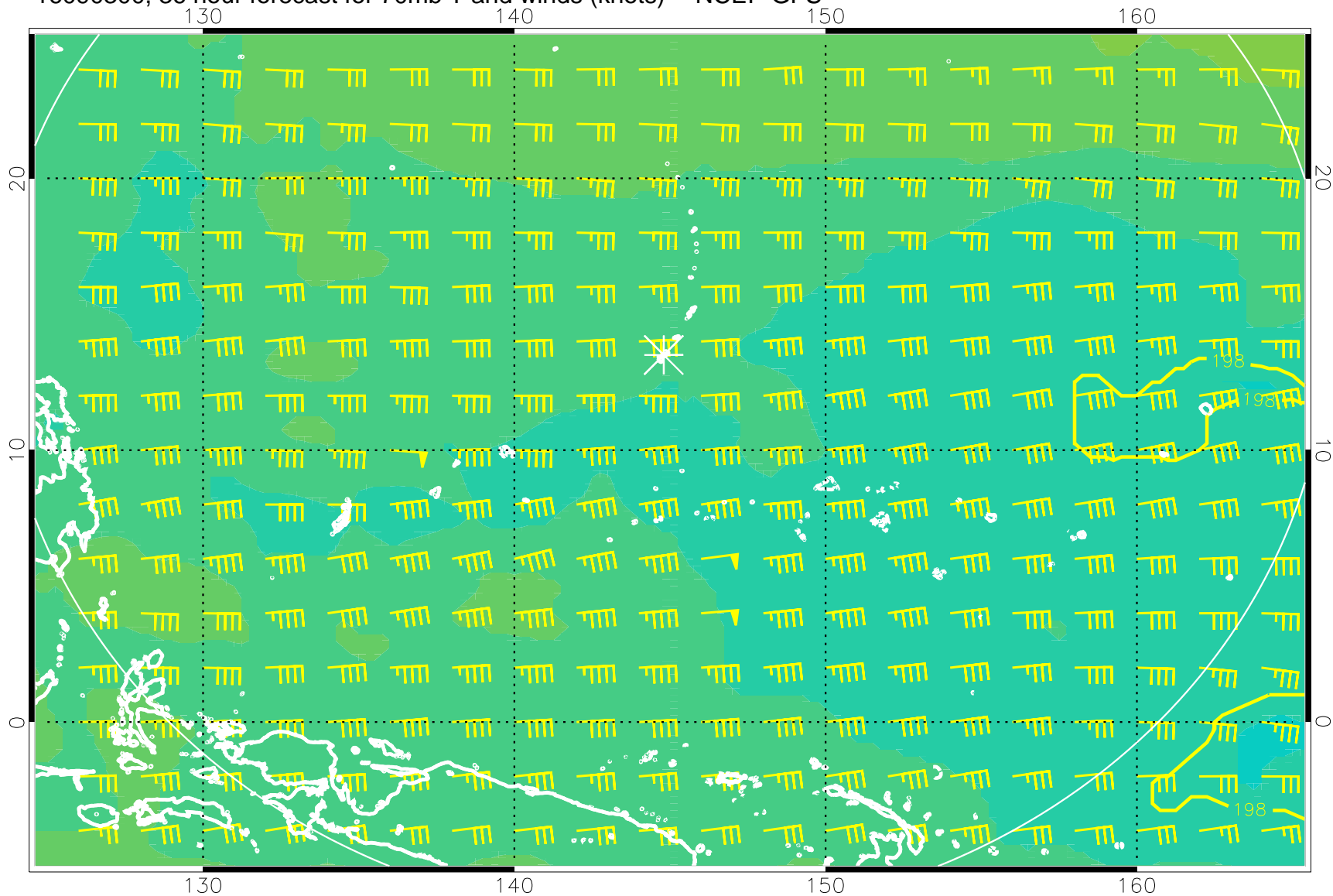
16090300, 36 hour forecast for 70mb T and winds (knots) -- NCEP GFS
