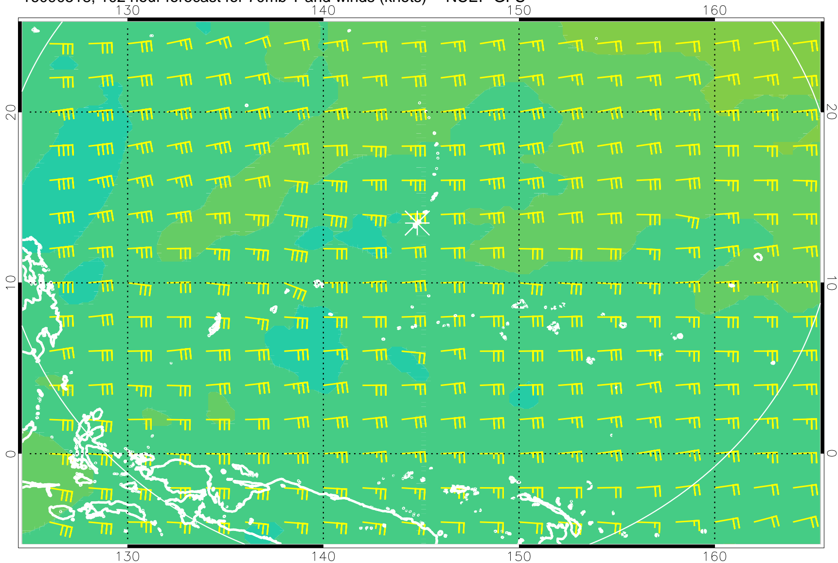
16090518, 102 hour forecast for 70mb T and winds (knots) -- NCEP GFS
