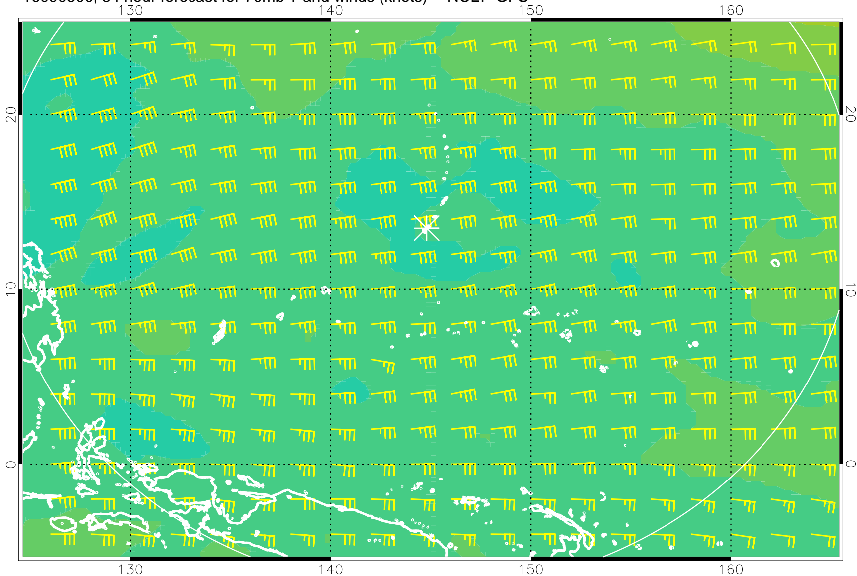
16090500, 84 hour forecast for 70mb T and winds (knots) -- NCEP GFS
