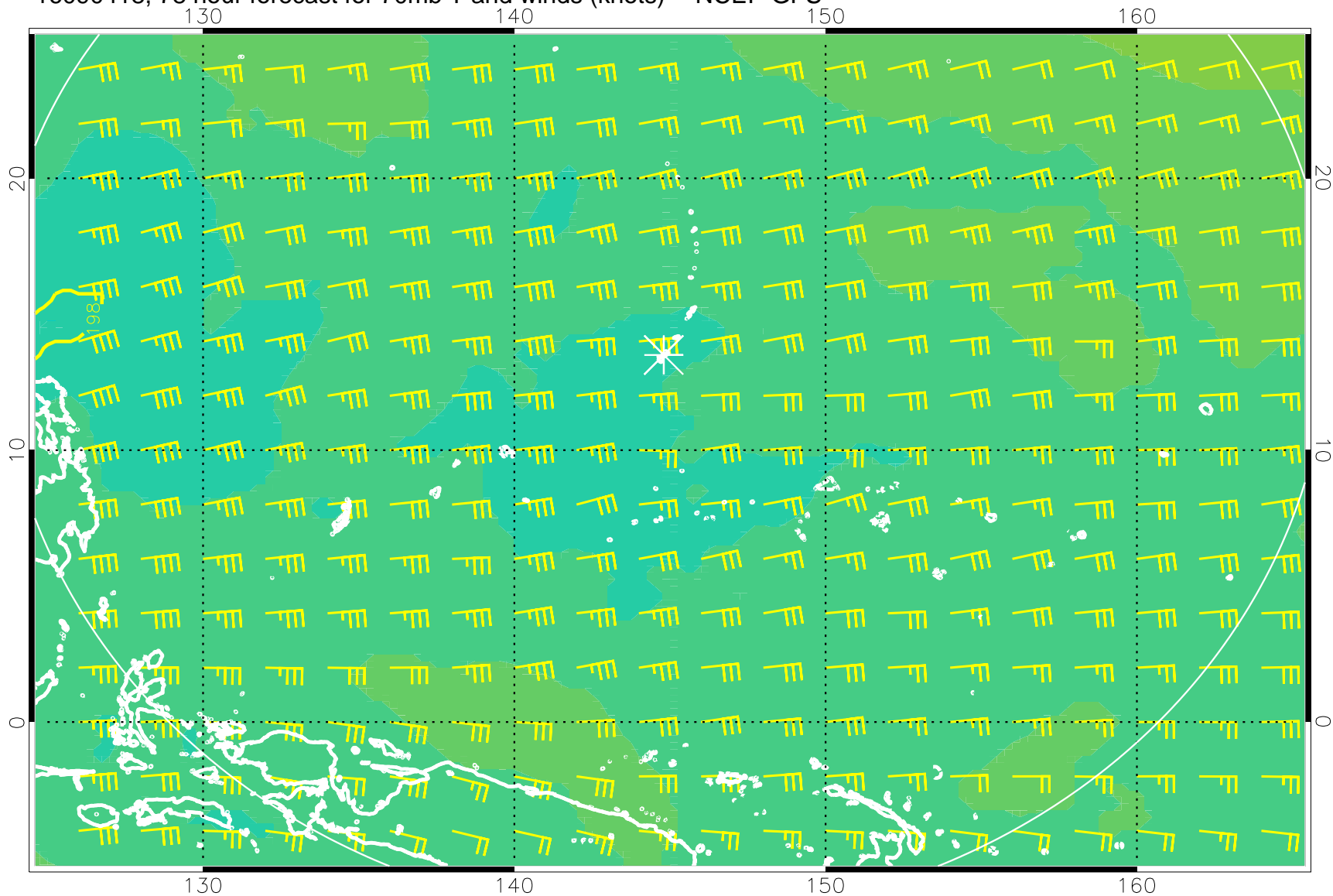
16090418, 78 hour forecast for 70mb T and winds (knots) -- NCEP GFS
