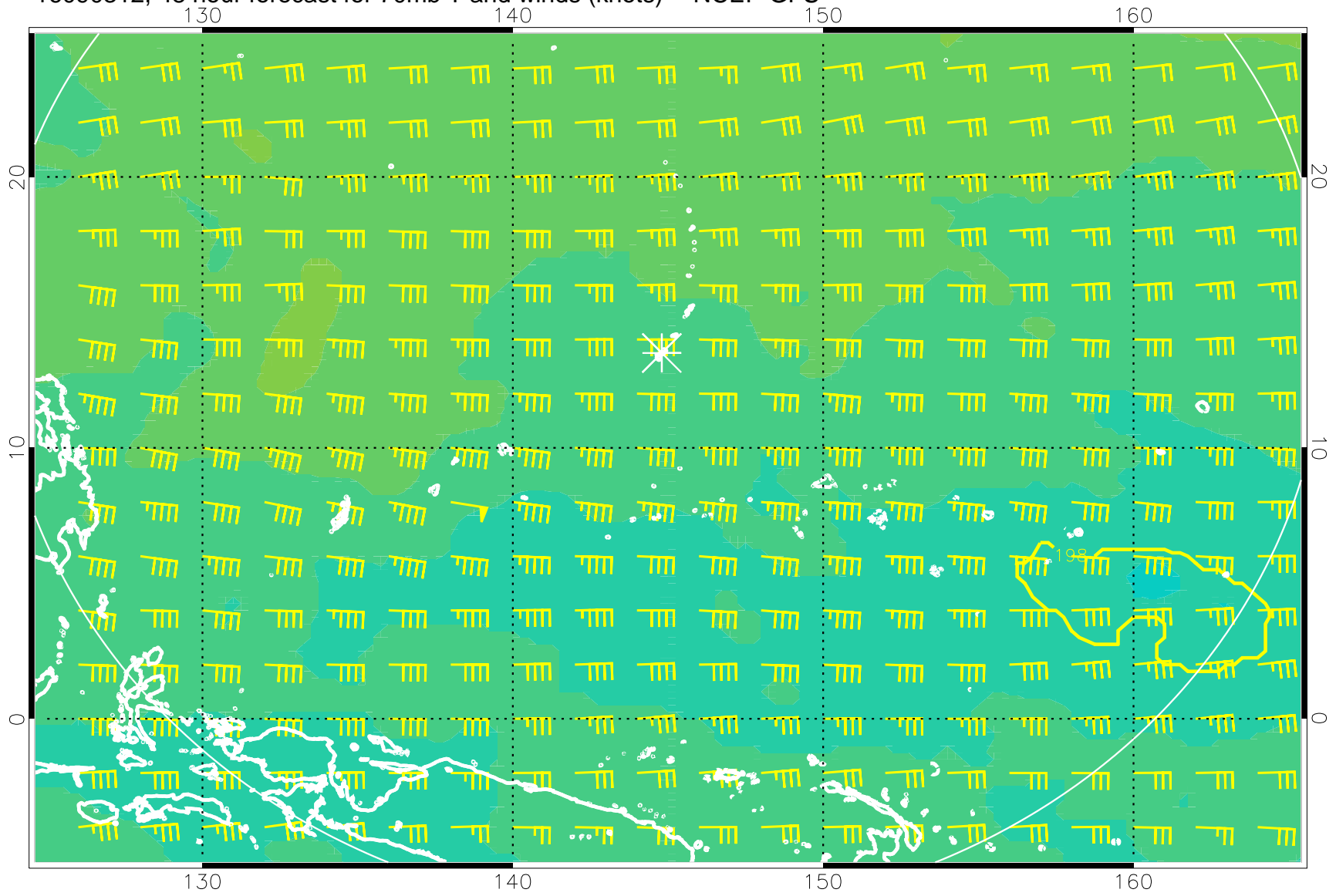
16090312, 48 hour forecast for 70mb T and winds (knots) -- NCEP GFS
