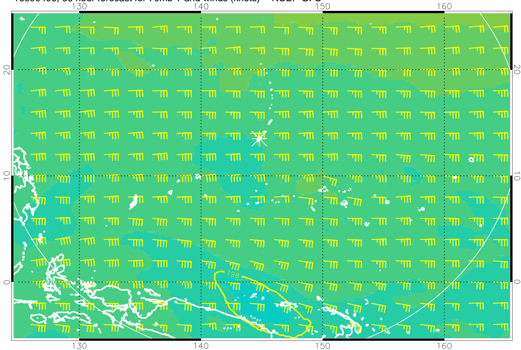
16090406, 66 hour forecast for 70mb T and winds (knots) -- NCEP GFS
