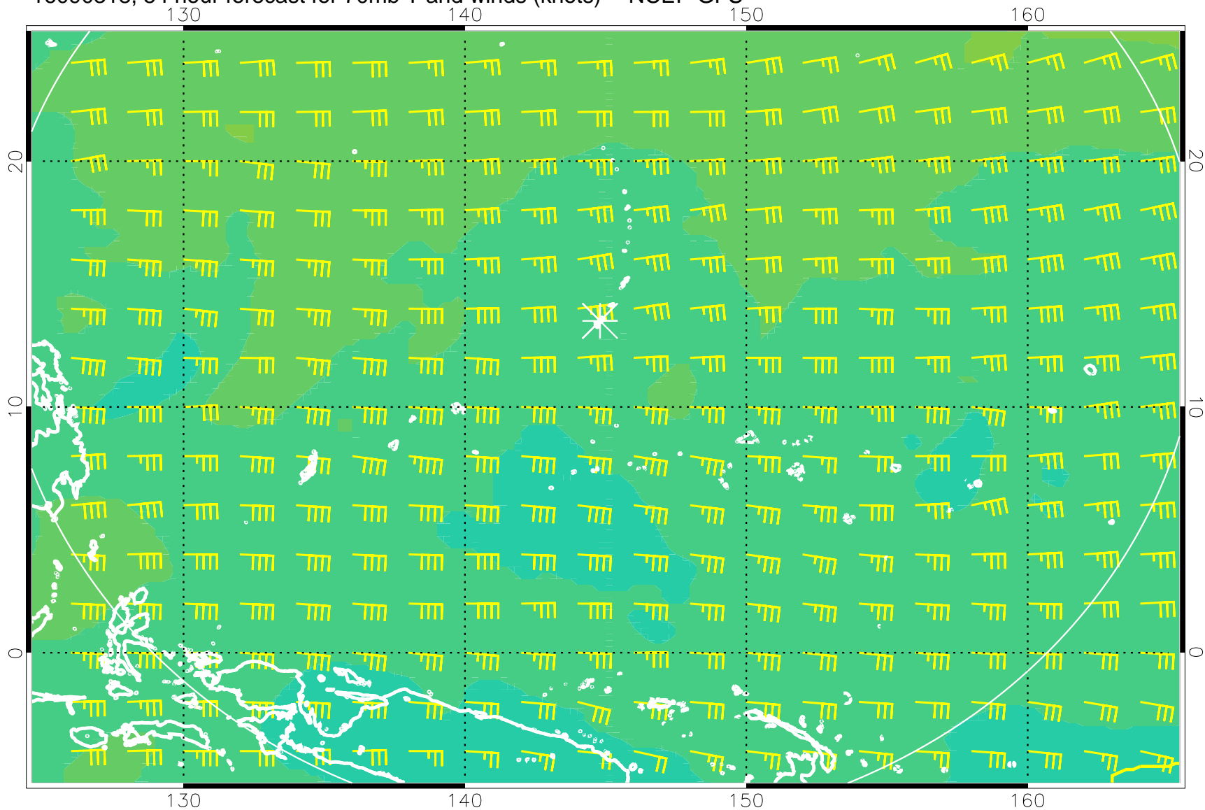
16090318, 54 hour forecast for 70mb T and winds (knots) -- NCEP GFS
