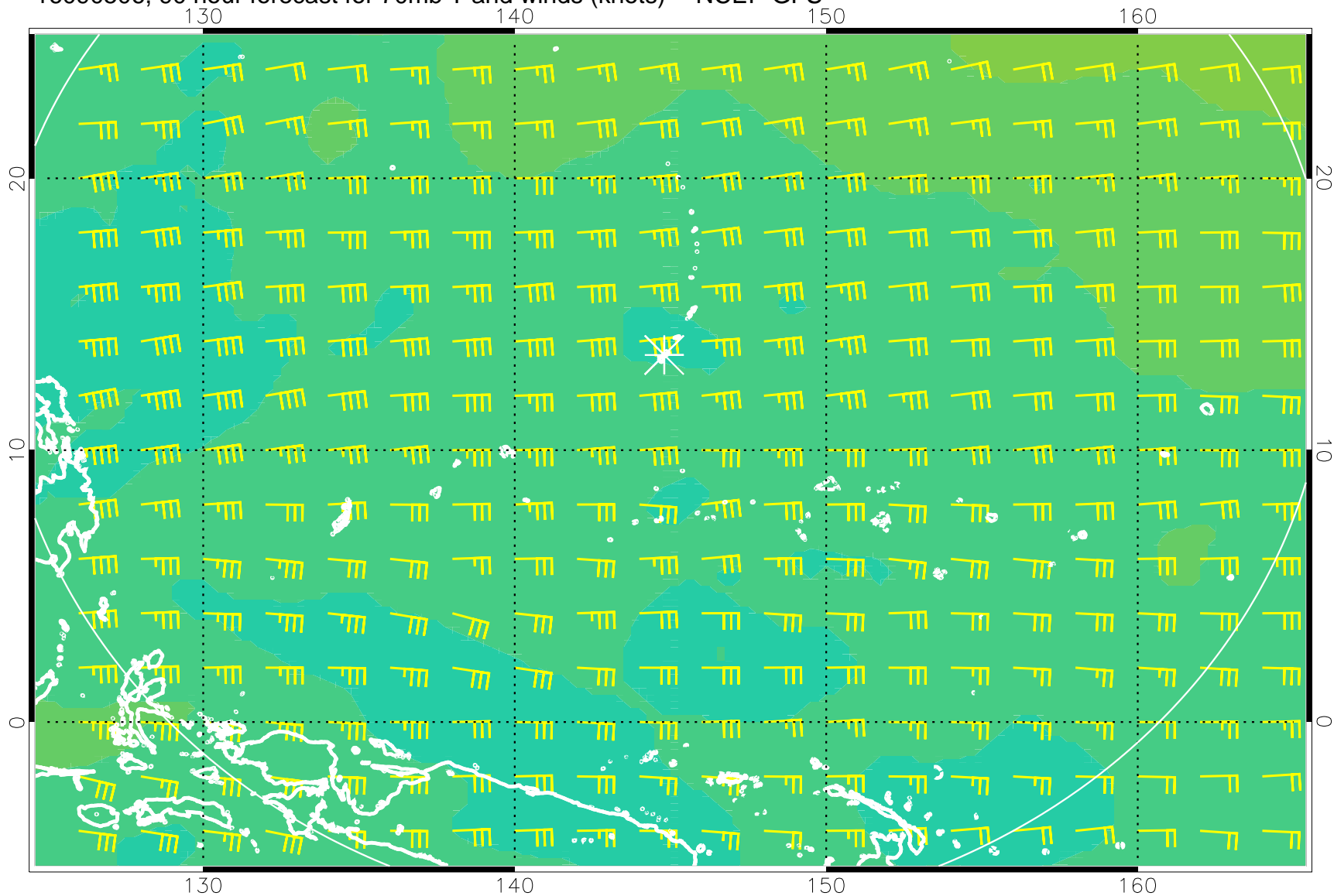
16090506, 90 hour forecast for 70mb T and winds (knots) -- NCEP GFS
