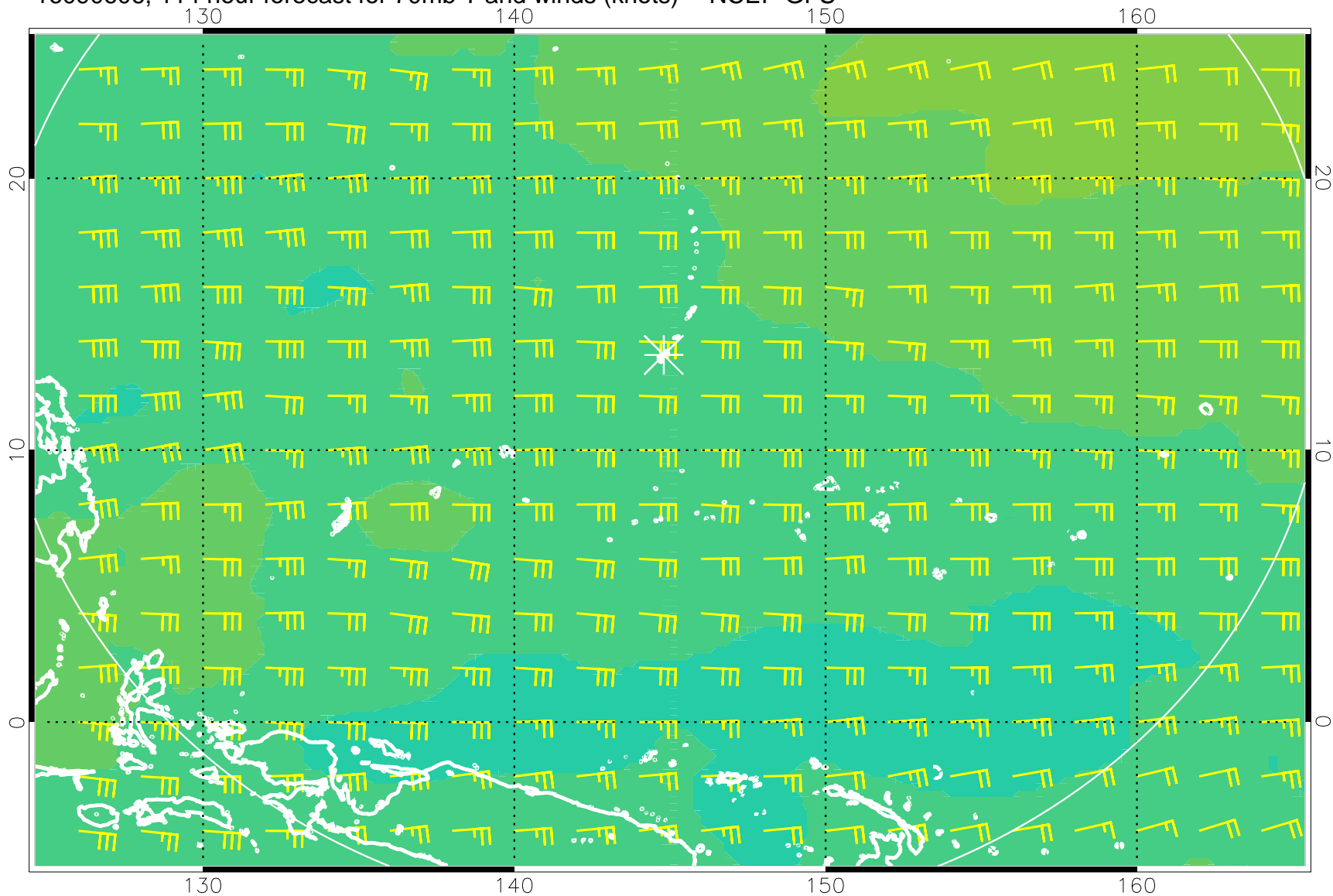
16090606, 114 hour forecast for 70mb T and winds (knots) -- NCEP GFS
