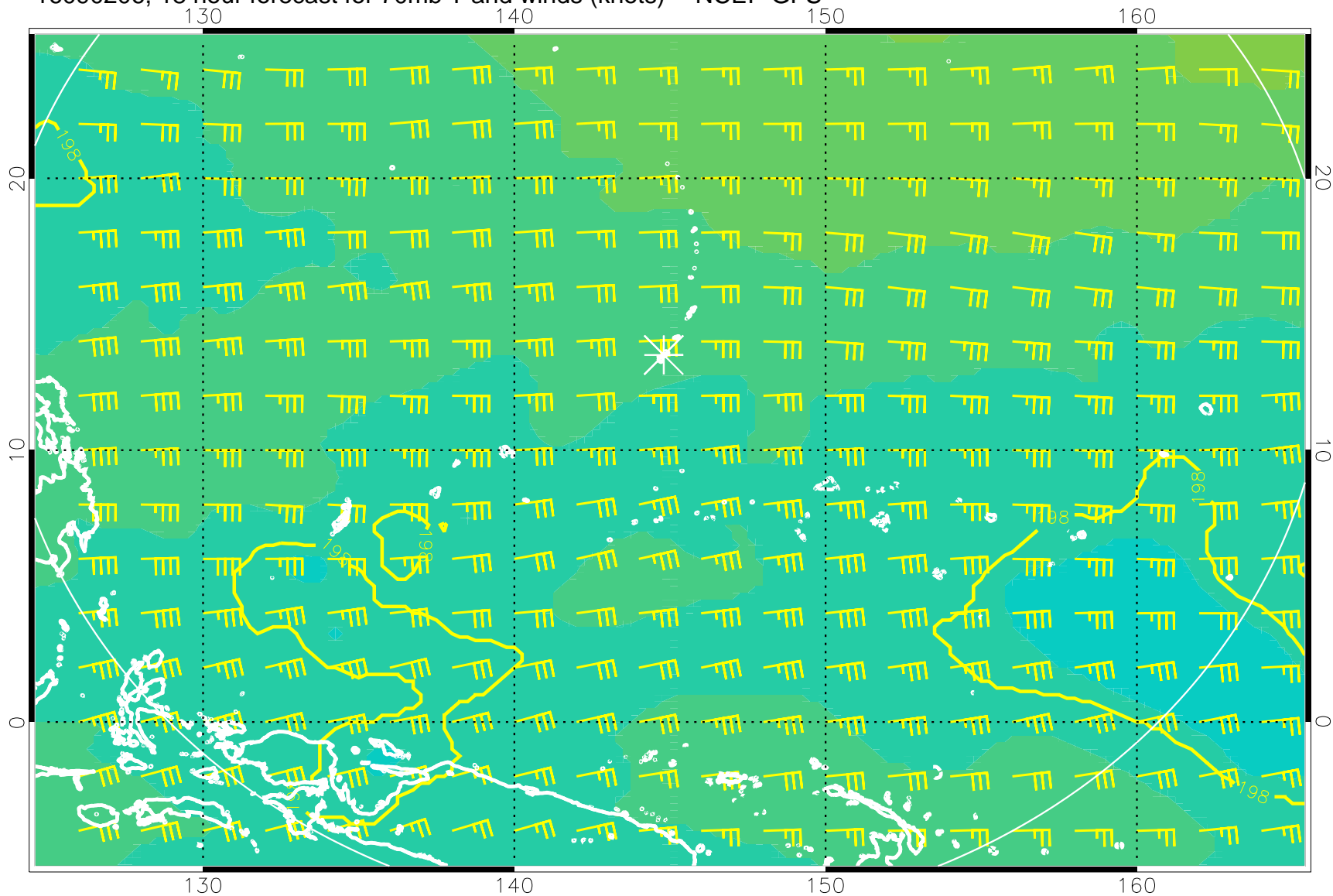
16090206, 18 hour forecast for 70mb T and winds (knots) -- NCEP GFS
