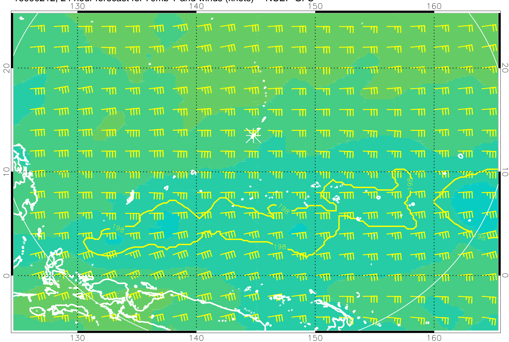
16090212, 24 hour forecast for 70mb T and winds (knots) -- NCEP GFS
