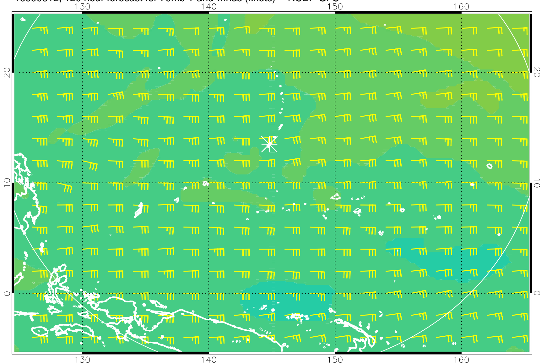
16090612, 120 hour forecast for 70mb T and winds (knots) -- NCEP GFS
