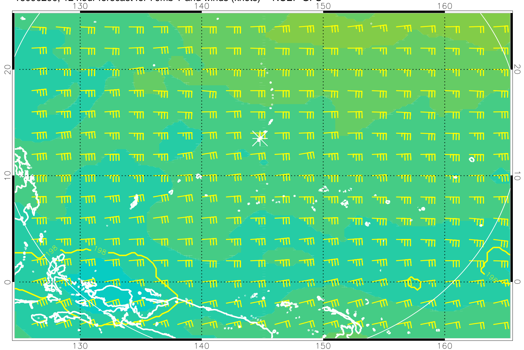
16090200, 12 hour forecast for 70mb T and winds (knots) -- NCEP GFS
