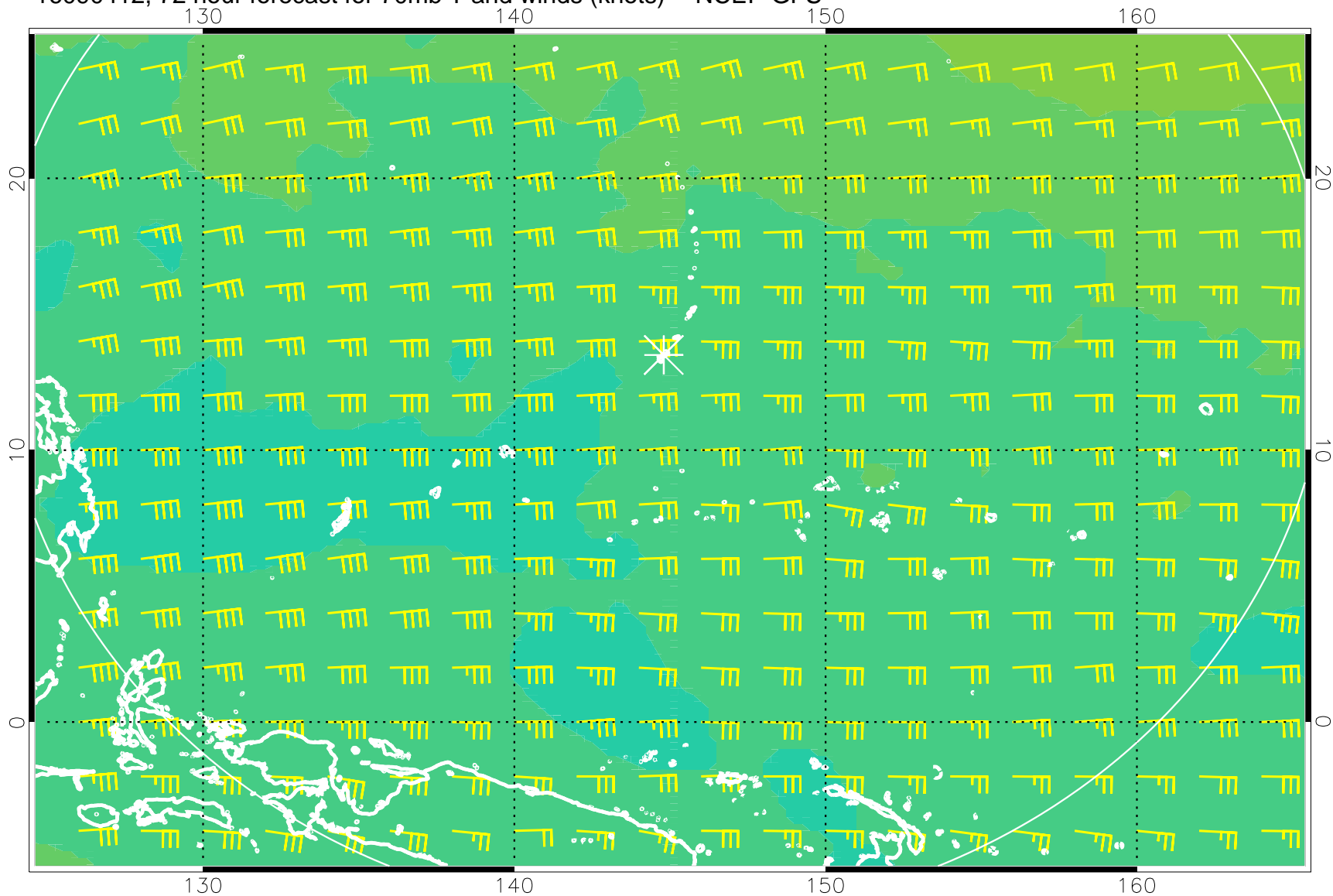
16090412, 72 hour forecast for 70mb T and winds (knots) -- NCEP GFS
