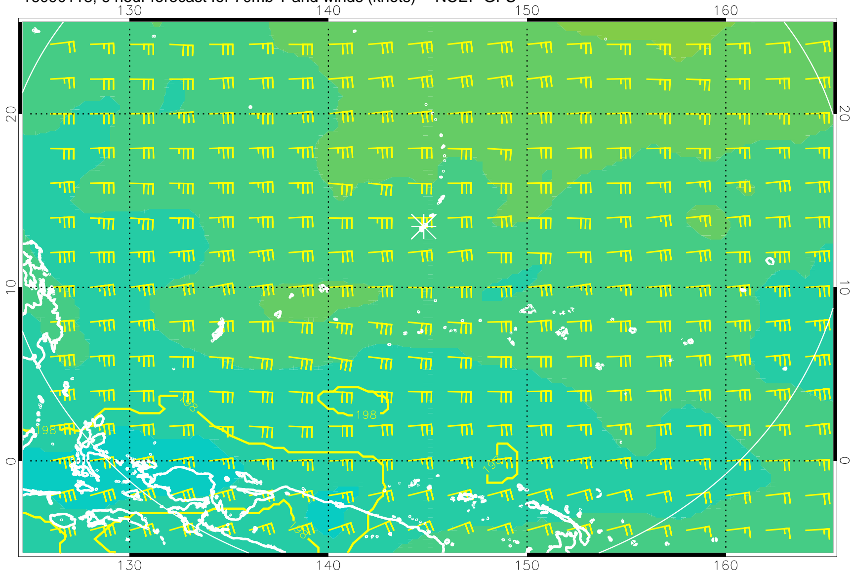
16090118, 6 hour forecast for 70mb T and winds (knots) -- NCEP GFS
