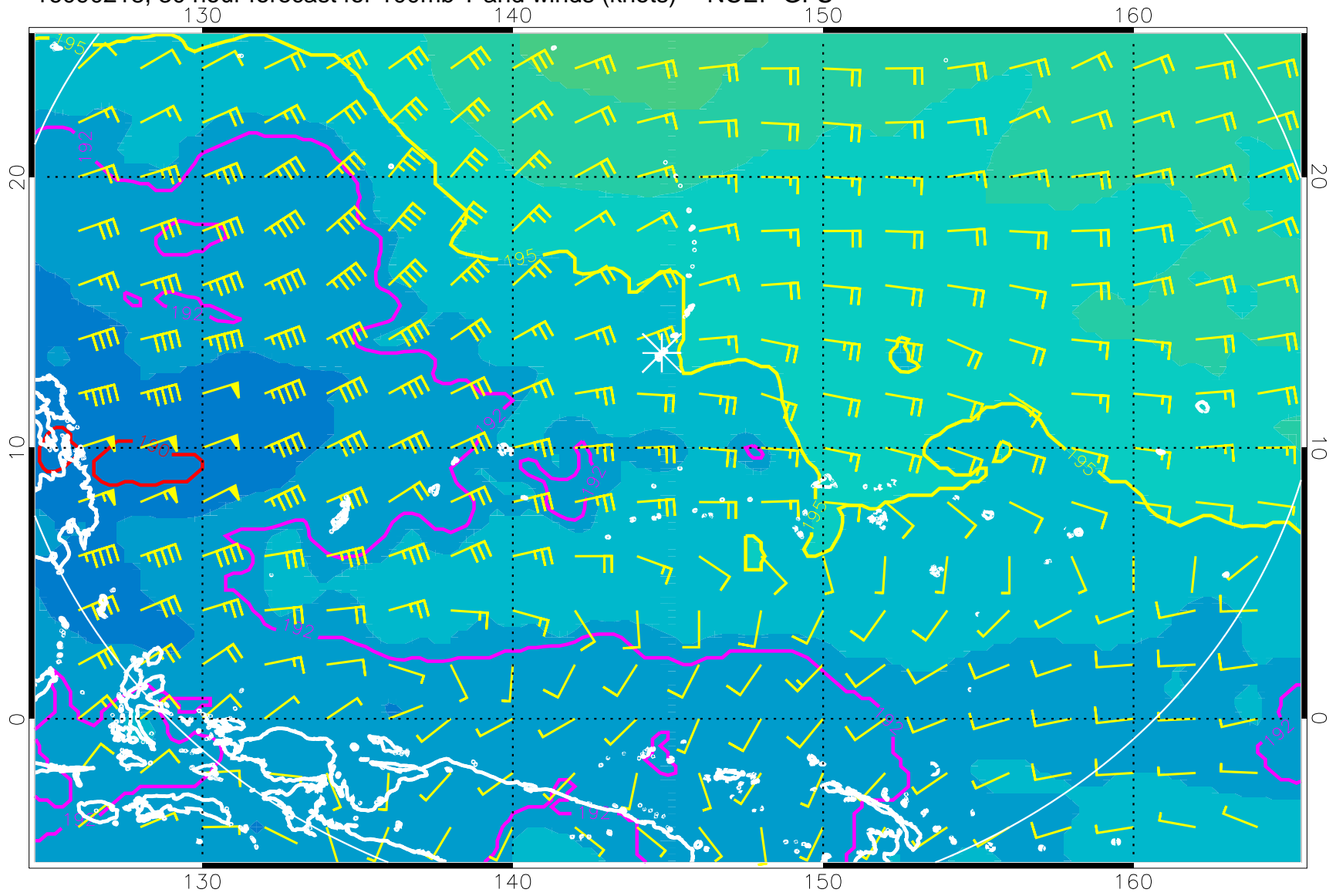
16090218, 30 hour forecast for 100mb T and winds (knots) -- NCEP GFS
