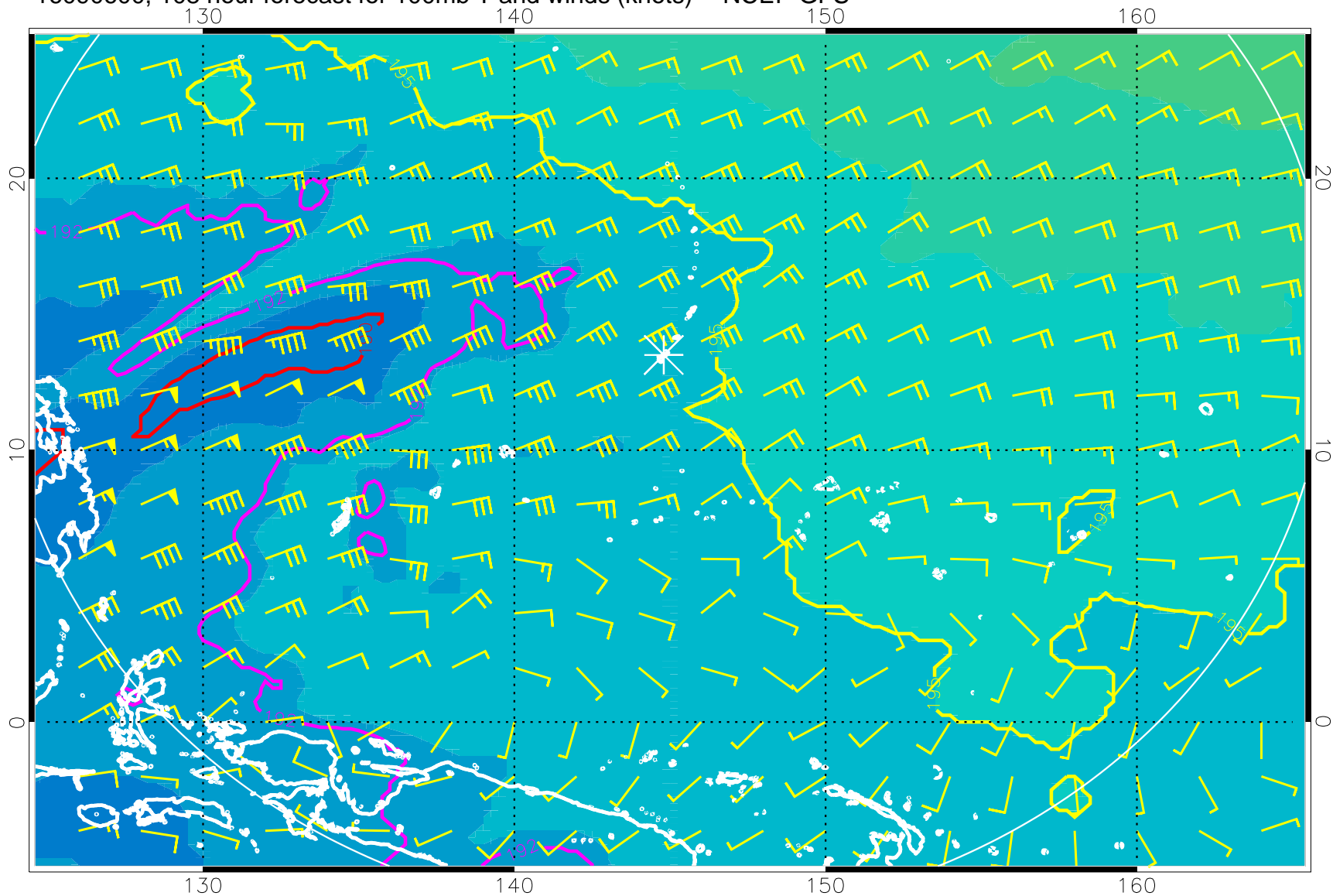
16090600, 108 hour forecast for 100mb T and winds (knots) -- NCEP GFS
