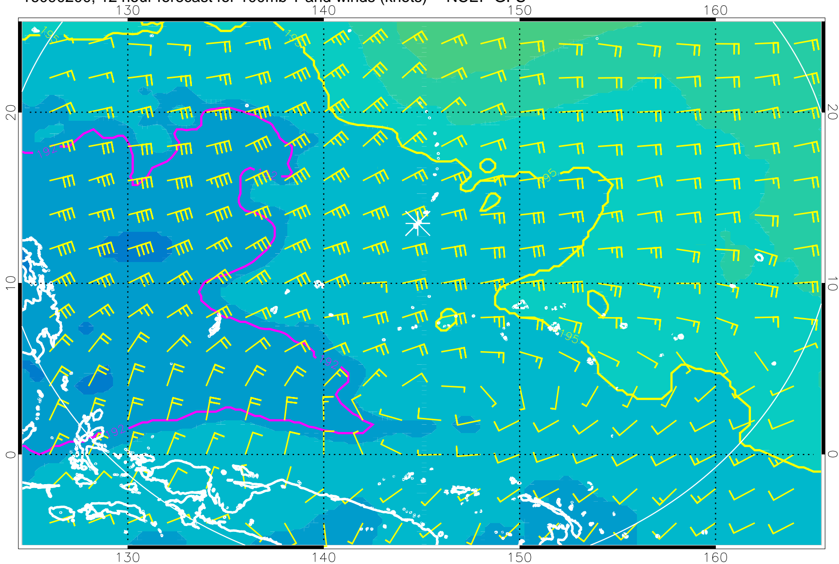
16090200, 12 hour forecast for 100mb T and winds (knots) -- NCEP GFS
