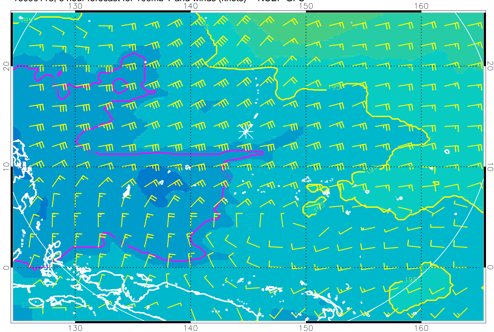
16090118, 6 hour forecast for 100mb T and winds (knots) -- NCEP GFS
