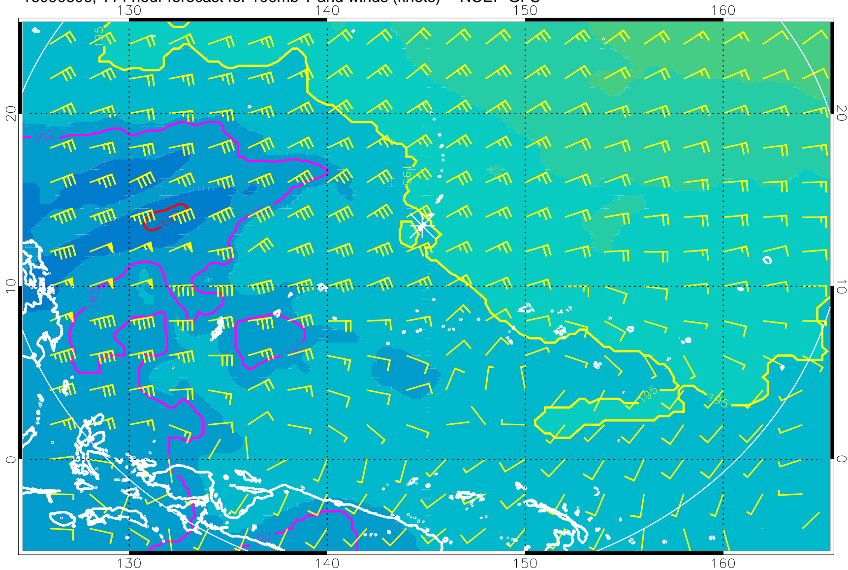
16090606, 114 hour forecast for 100mb T and winds (knots) -- NCEP GFS
