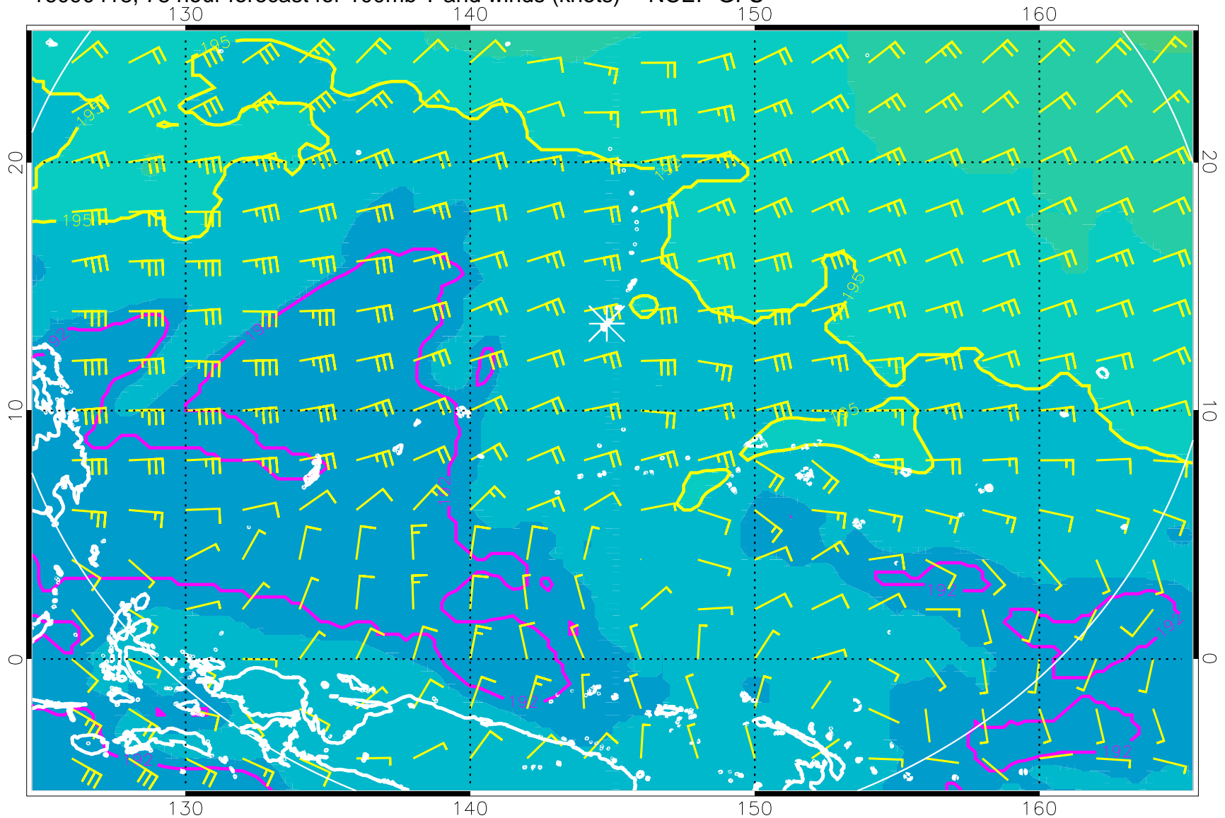
16090418, 78 hour forecast for 100mb T and winds (knots) -- NCEP GFS
