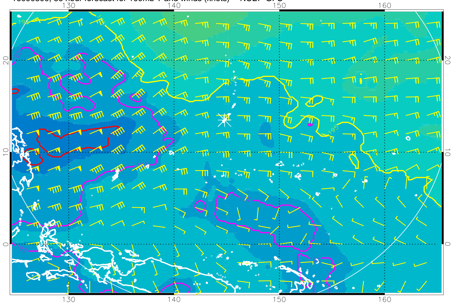
16090300, 36 hour forecast for 100mb T and winds (knots) -- NCEP GFS
