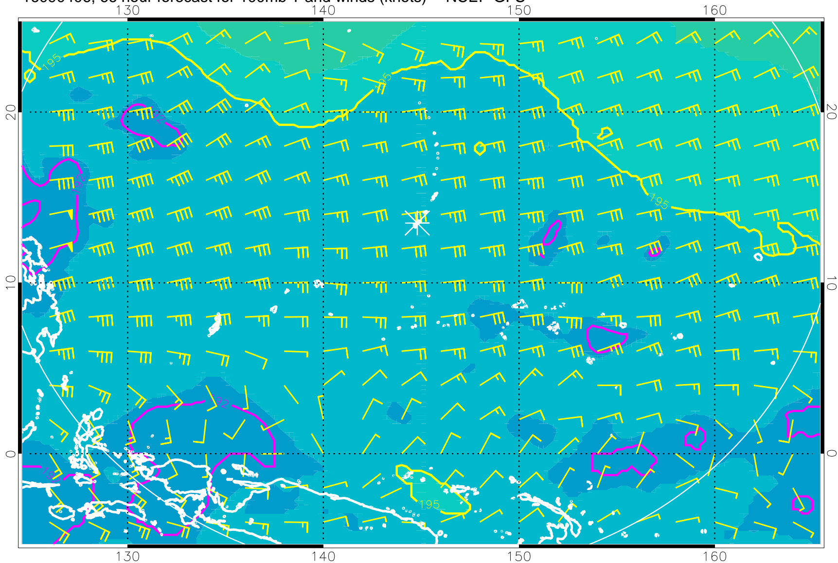
16090406, 66 hour forecast for 100mb T and winds (knots) -- NCEP GFS
