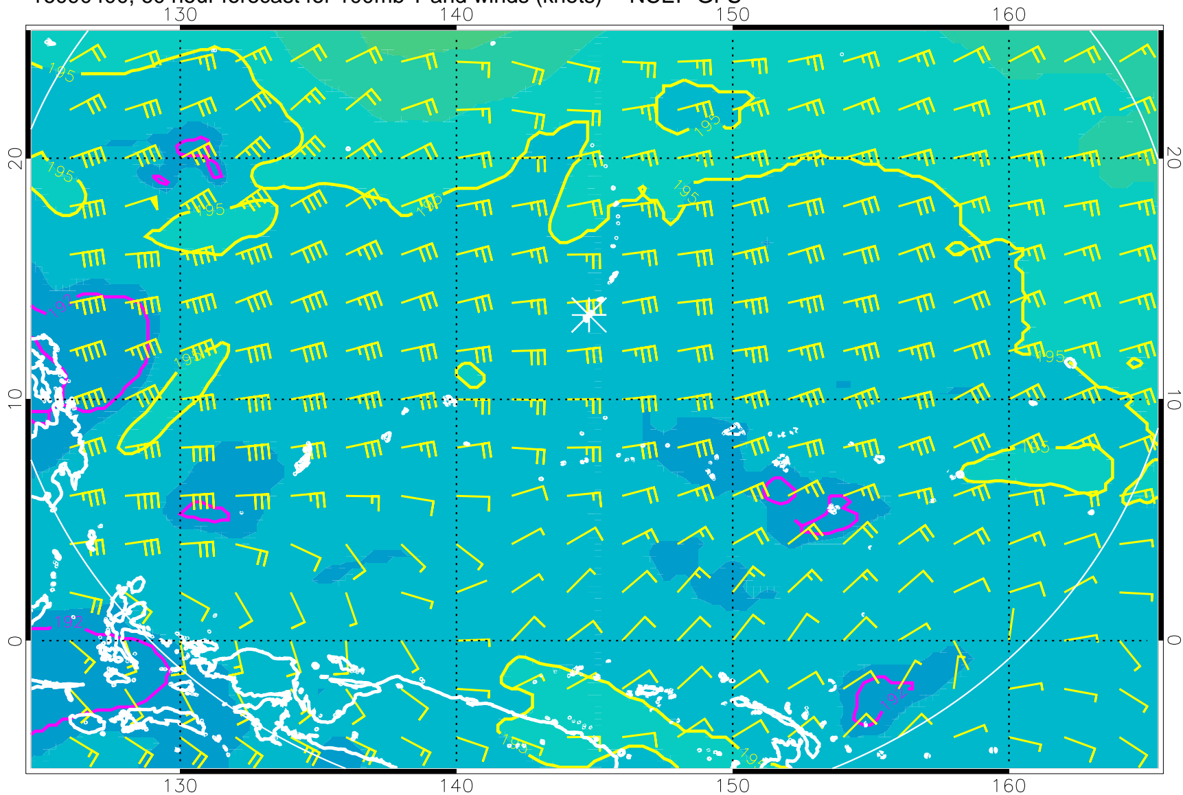
16090400, 60 hour forecast for 100mb T and winds (knots) -- NCEP GFS
