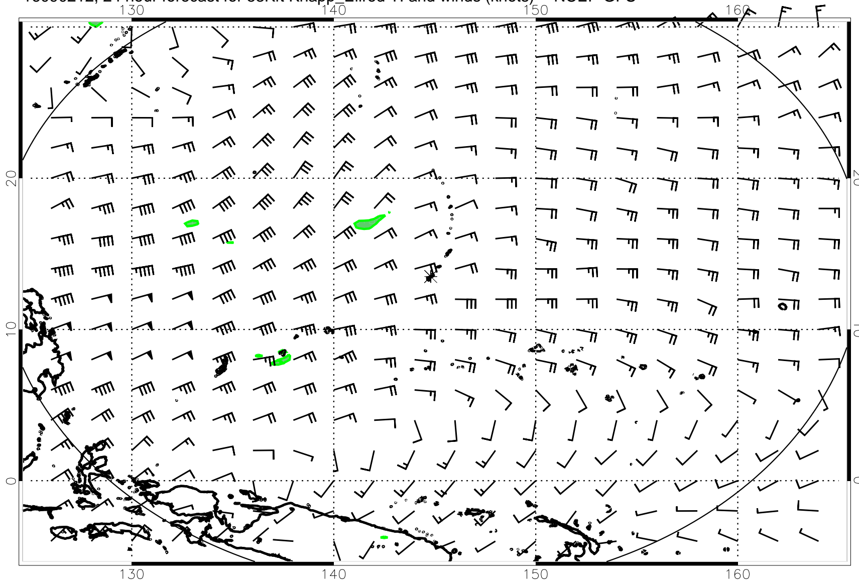
16090212, 24 hour forecast for 53Kft Knapp_Ellrod TI and winds (knots) -- NCEP GFS
