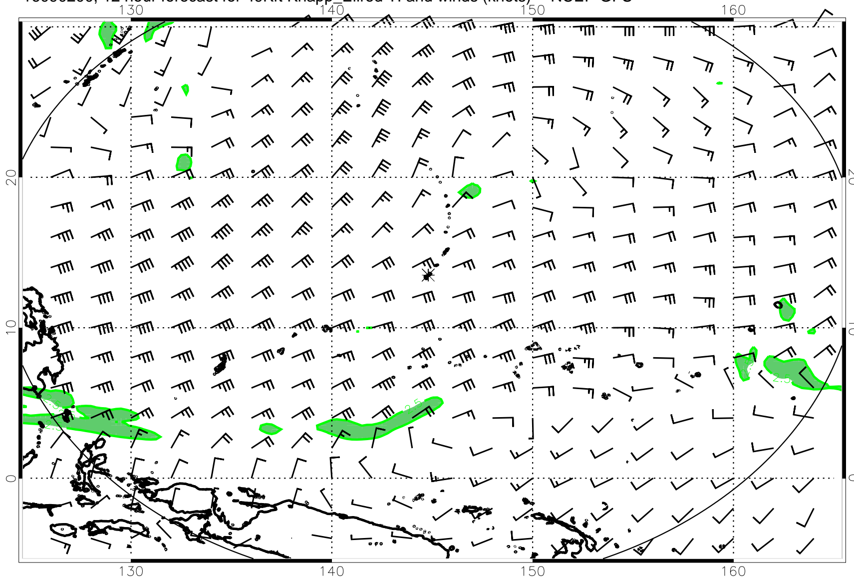
16090200, 12 hour forecast for 49Kft Knapp_Ellrod TI and winds (knots) -- NCEP GFS
