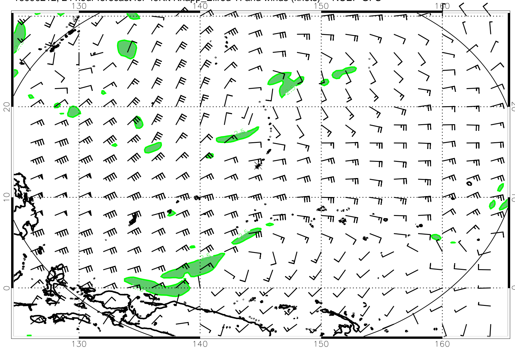
16090212, 24 hour forecast for 49Kft Knapp_Ellrod TI and winds (knots) -- NCEP GFS
