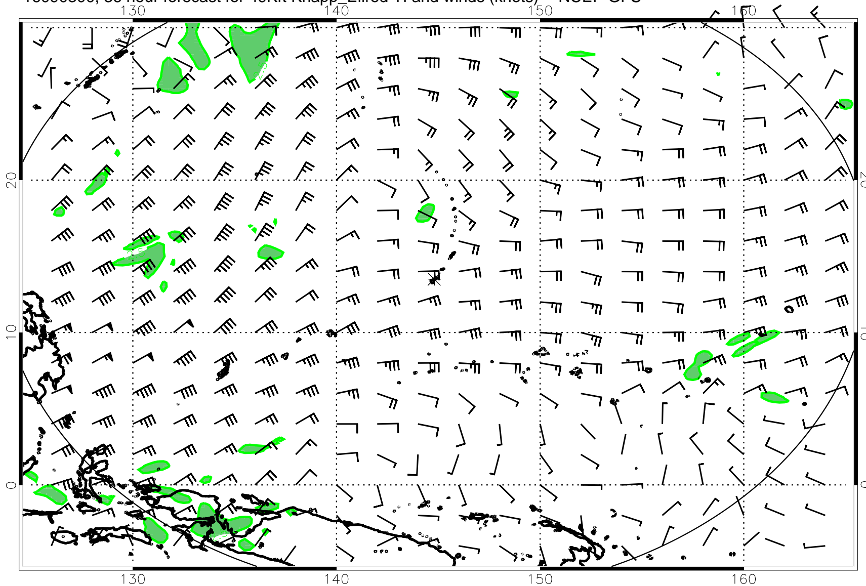
16090300, 36 hour forecast for 49Kft Knapp_Ellrod TI and winds (knots) -- NCEP GFS
