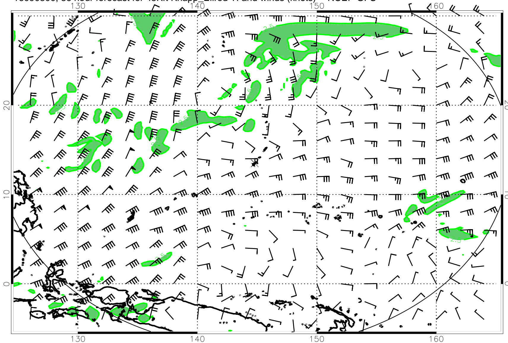
16090300, 36 hour forecast for 45Kft Knapp_Ellrod TI and winds (knots) -- NCEP GFS
