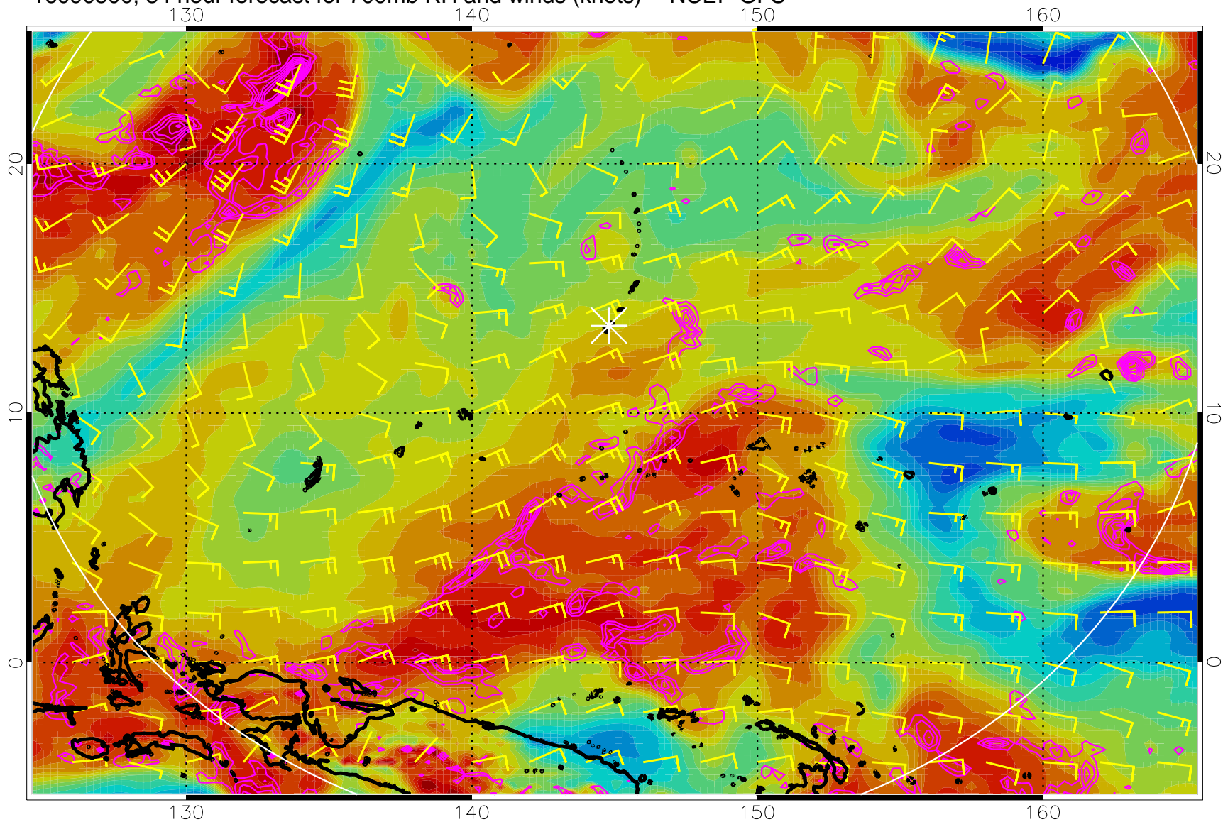
16090500, 84 hour forecast for 700mb RH and winds (knots) -- NCEP GFS
