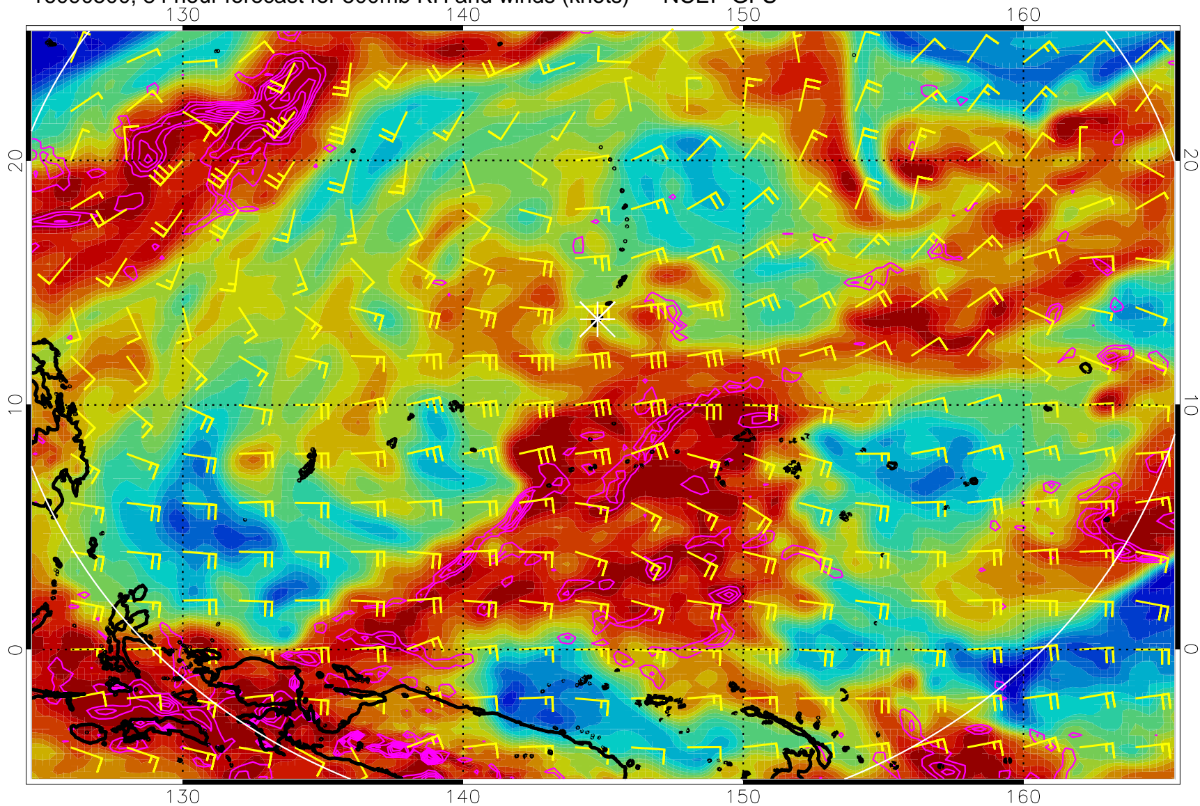
16090500, 84 hour forecast for 500mb RH and winds (knots) -- NCEP GFS
