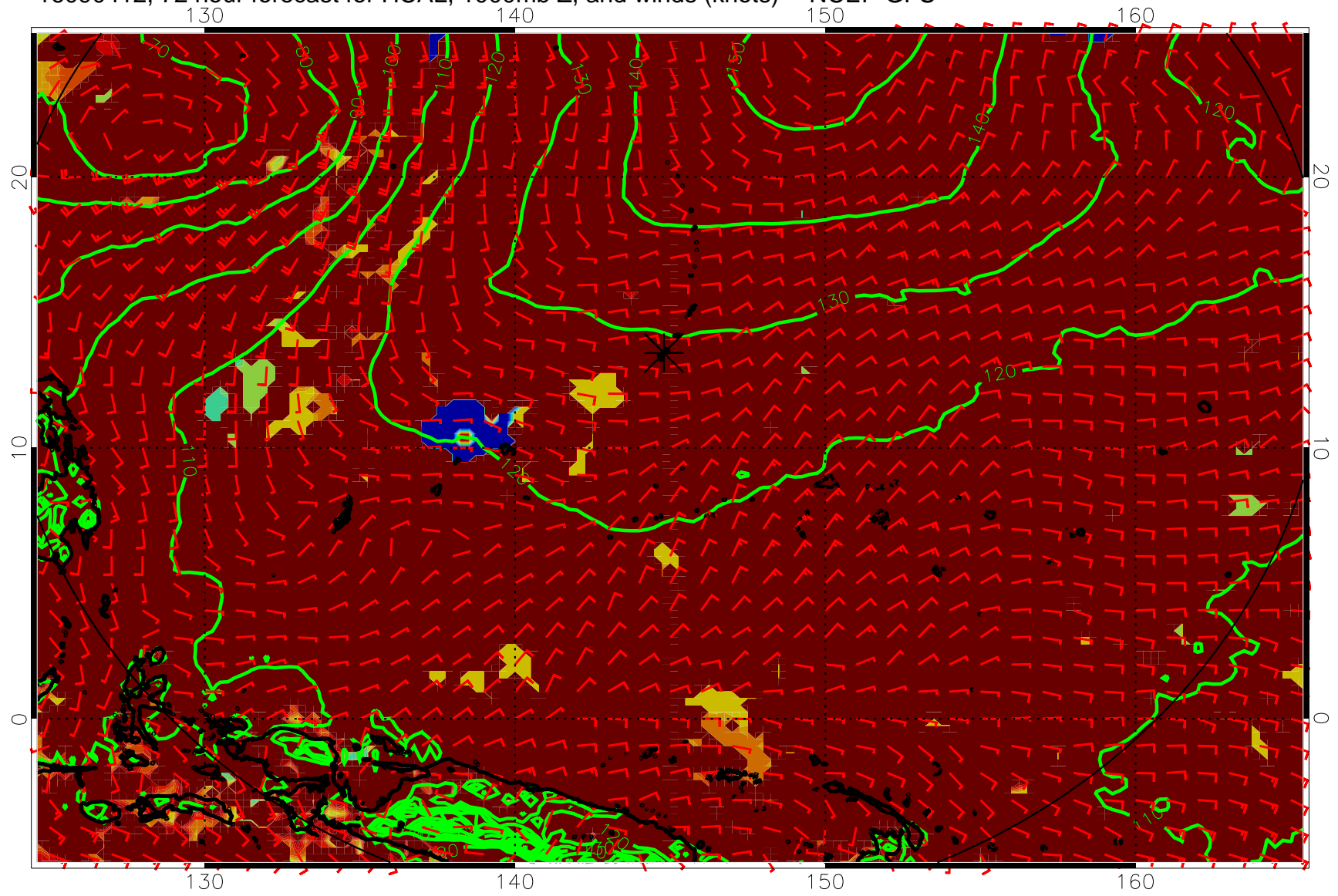
16090412, 72 hour forecast for HCAL, 1000mb Z, and winds (knots) -- NCEP GFS
