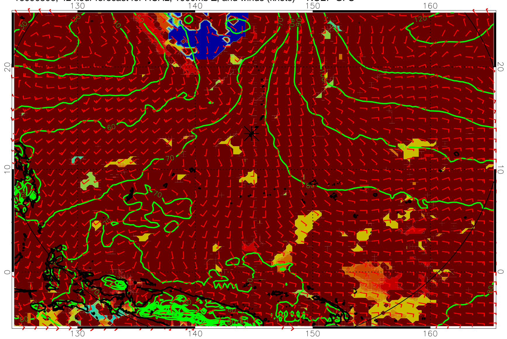
16090306, 42 hour forecast for HCAL, 1000mb Z, and winds (knots) -- NCEP GFS
