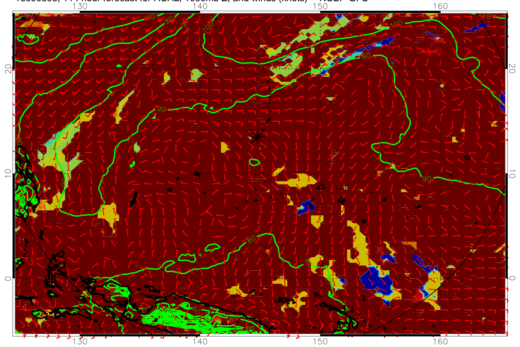
16090606, 114 hour forecast for HCAL, 1000mb Z, and winds (knots) -- NCEP GFS
