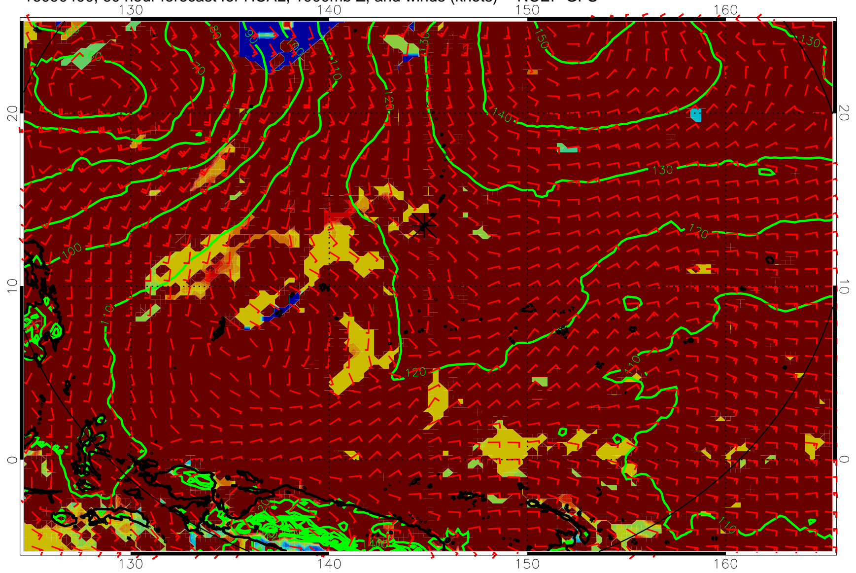
16090400, 60 hour forecast for HCAL, 1000mb Z, and winds (knots) -- NCEP GFS
