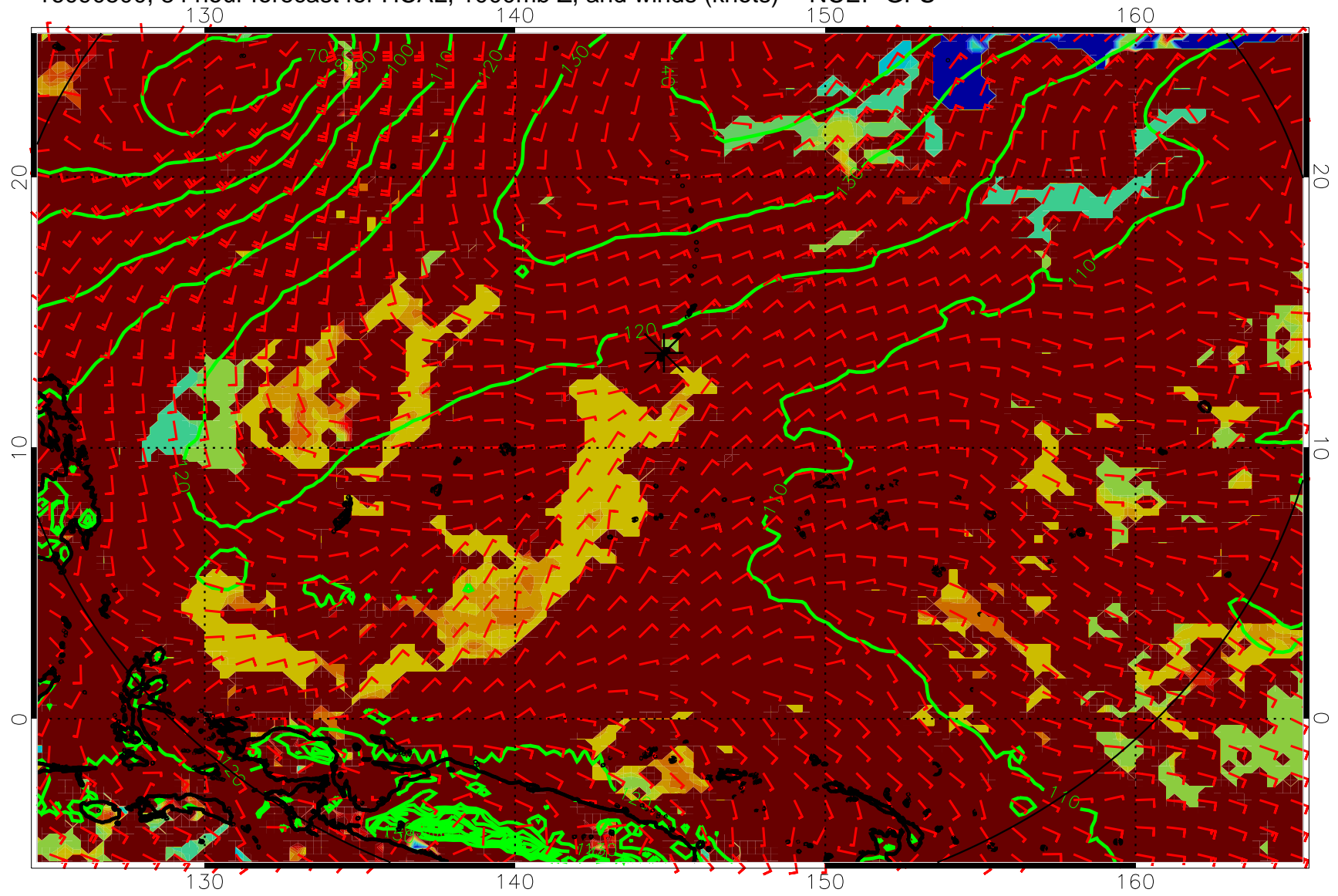
16090500, 84 hour forecast for HCAL, 1000mb Z, and winds (knots) -- NCEP GFS
