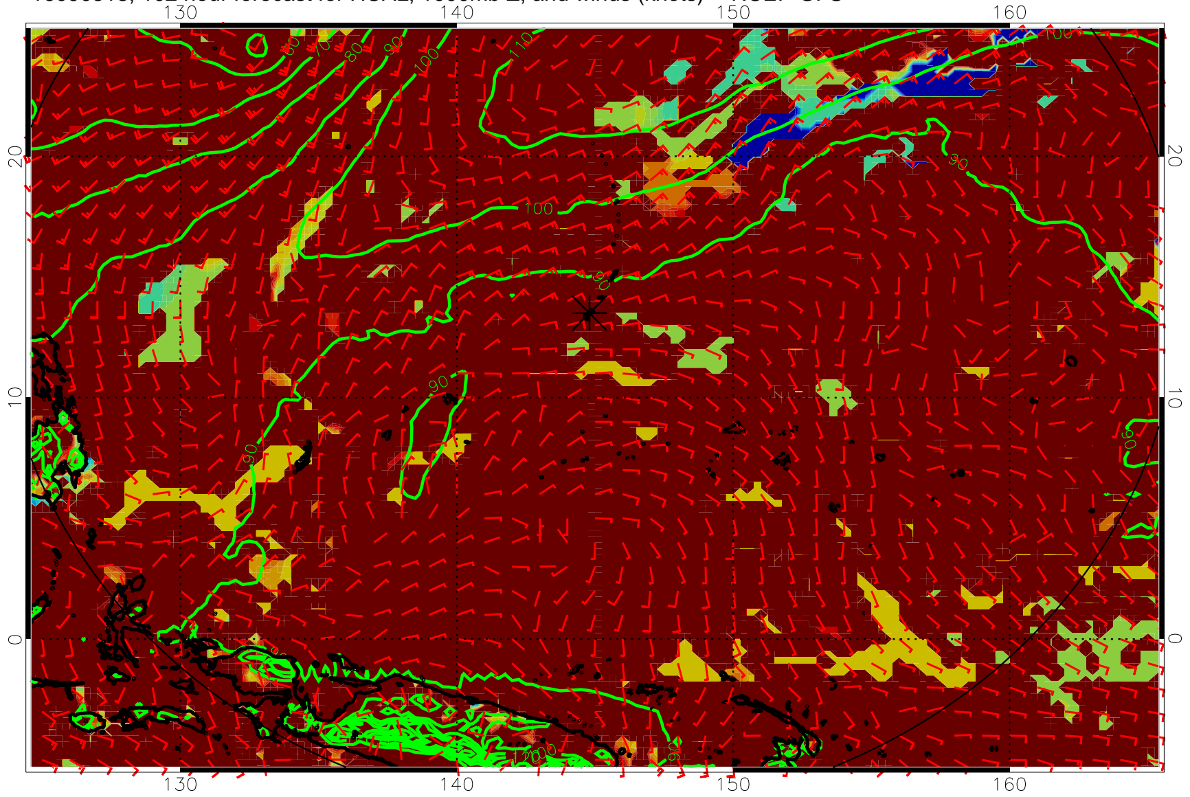
16090518, 102 hour forecast for HCAL, 1000mb Z, and winds (knots) -- NCEP GFS
