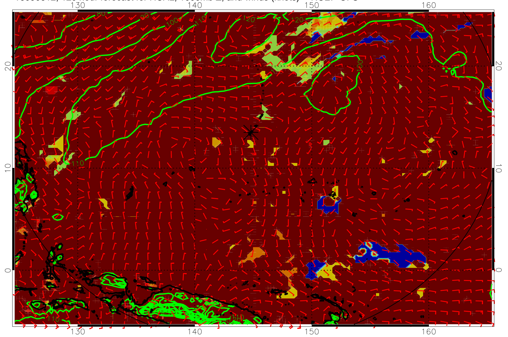
16090612, 120 hour forecast for HCAL, 1000mb Z, and winds (knots) -- NCEP GFS
