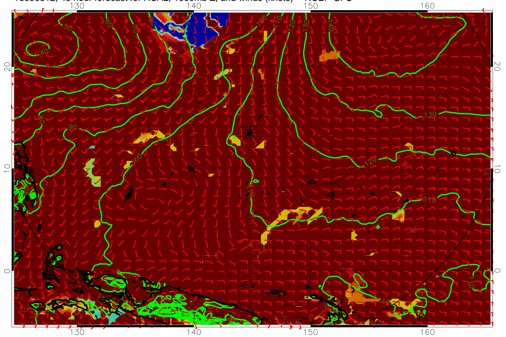
16090312, 48 hour forecast for HCAL, 1000mb Z, and winds (knots) -- NCEP GFS
