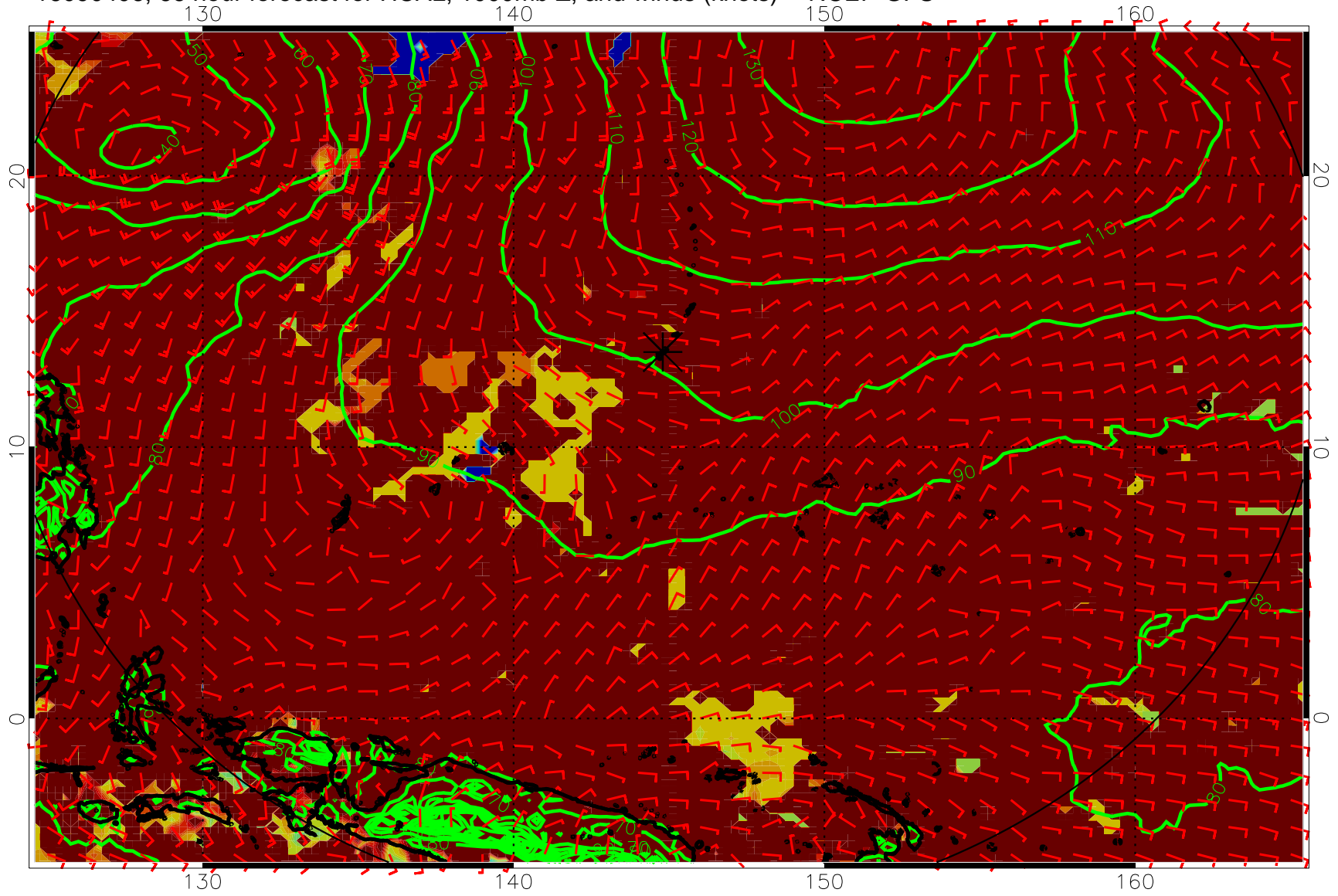
16090406, 66 hour forecast for HCAL, 1000mb Z, and winds (knots) -- NCEP GFS
