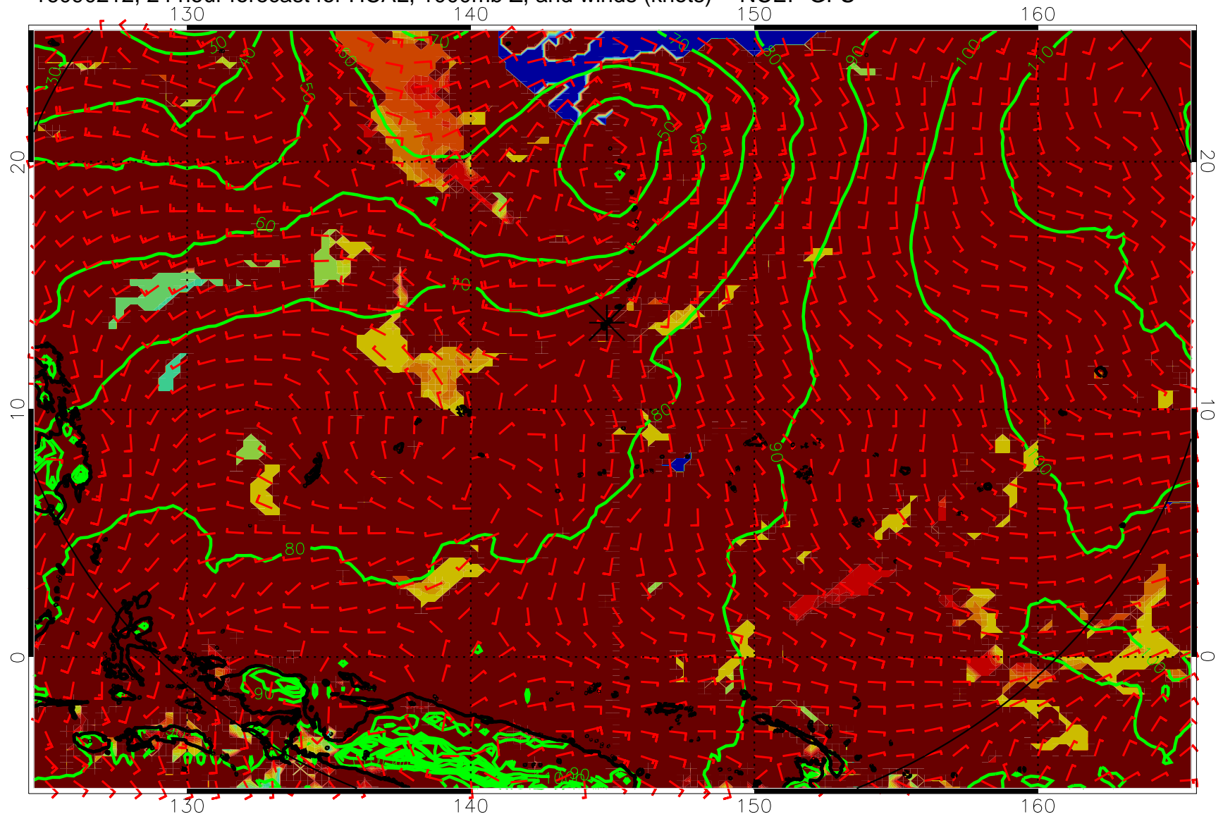
16090212, 24 hour forecast for HCAL, 1000mb Z, and winds (knots) -- NCEP GFS
