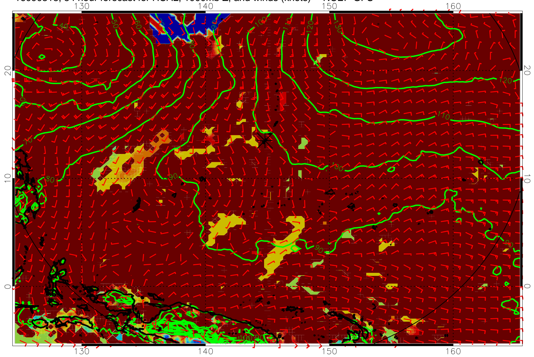
16090318, 54 hour forecast for HCAL, 1000mb Z, and winds (knots) -- NCEP GFS
