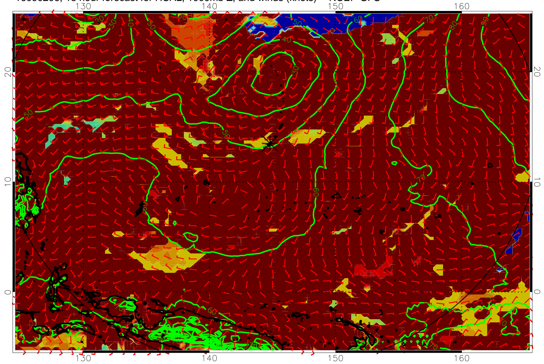
16090206, 18 hour forecast for HCAL, 1000mb Z, and winds (knots) -- NCEP GFS
