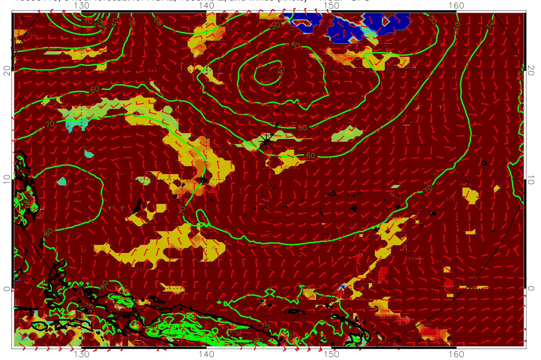
16090118, 6 hour forecast for HCAL, 1000mb Z, and winds (knots) -- NCEP GFS
