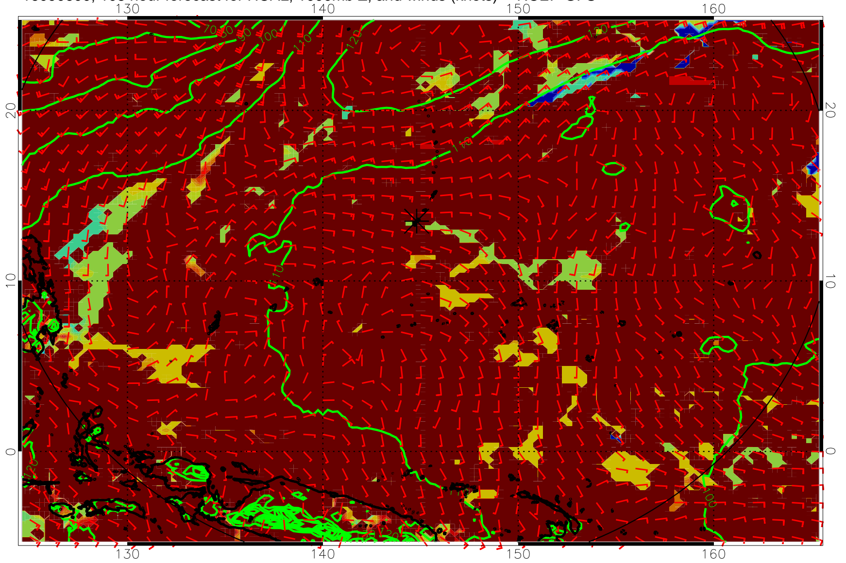
16090600, 108 hour forecast for HCAL, 1000mb Z, and winds (knots) -- NCEP GFS
