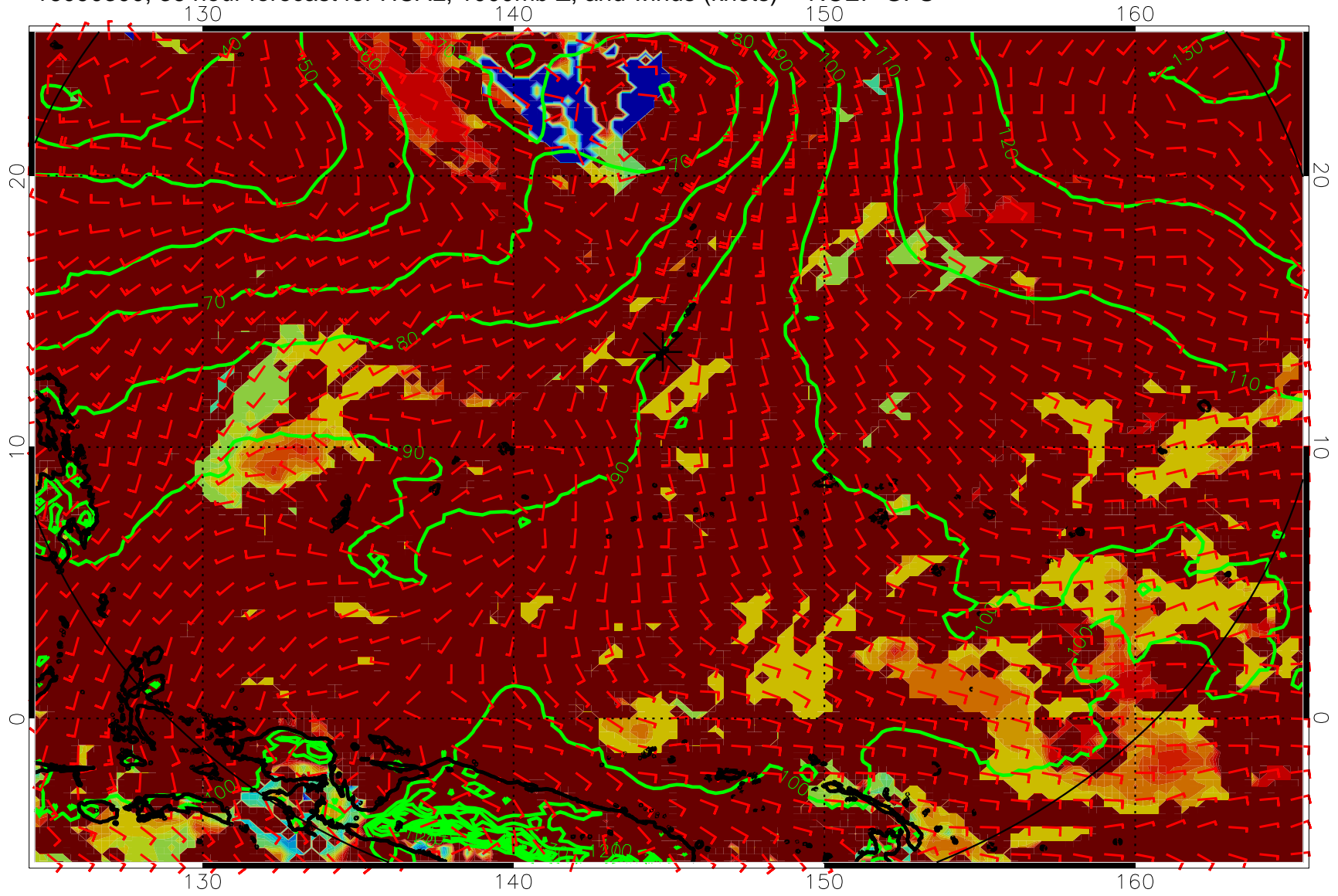
16090300, 36 hour forecast for HCAL, 1000mb Z, and winds (knots) -- NCEP GFS
