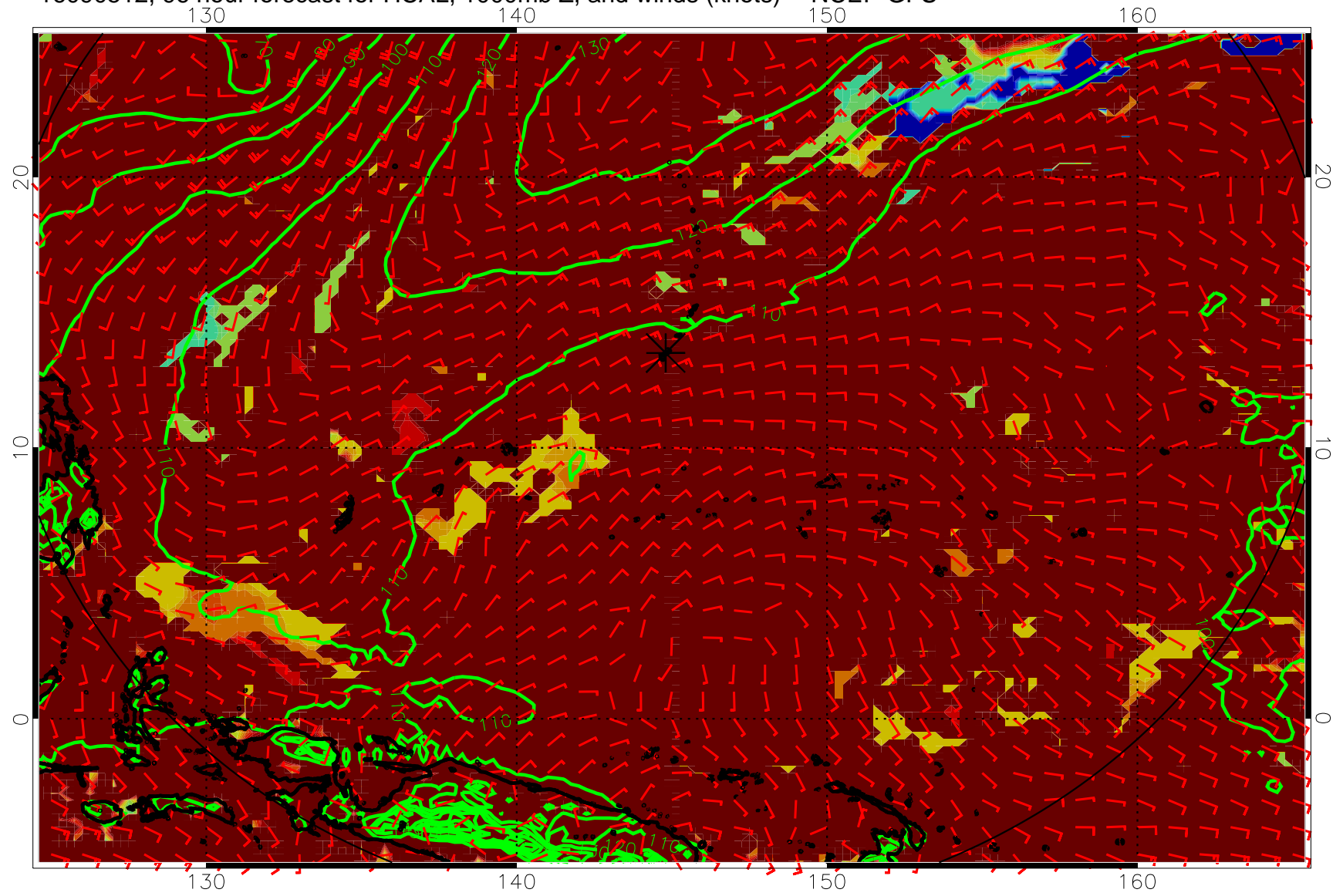
16090512, 96 hour forecast for HCAL, 1000mb Z, and winds (knots) -- NCEP GFS
