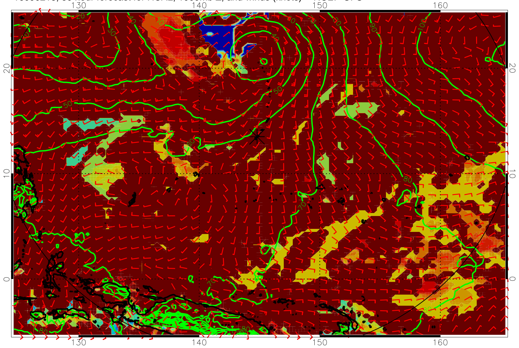
16090218, 30 hour forecast for HCAL, 1000mb Z, and winds (knots) -- NCEP GFS
