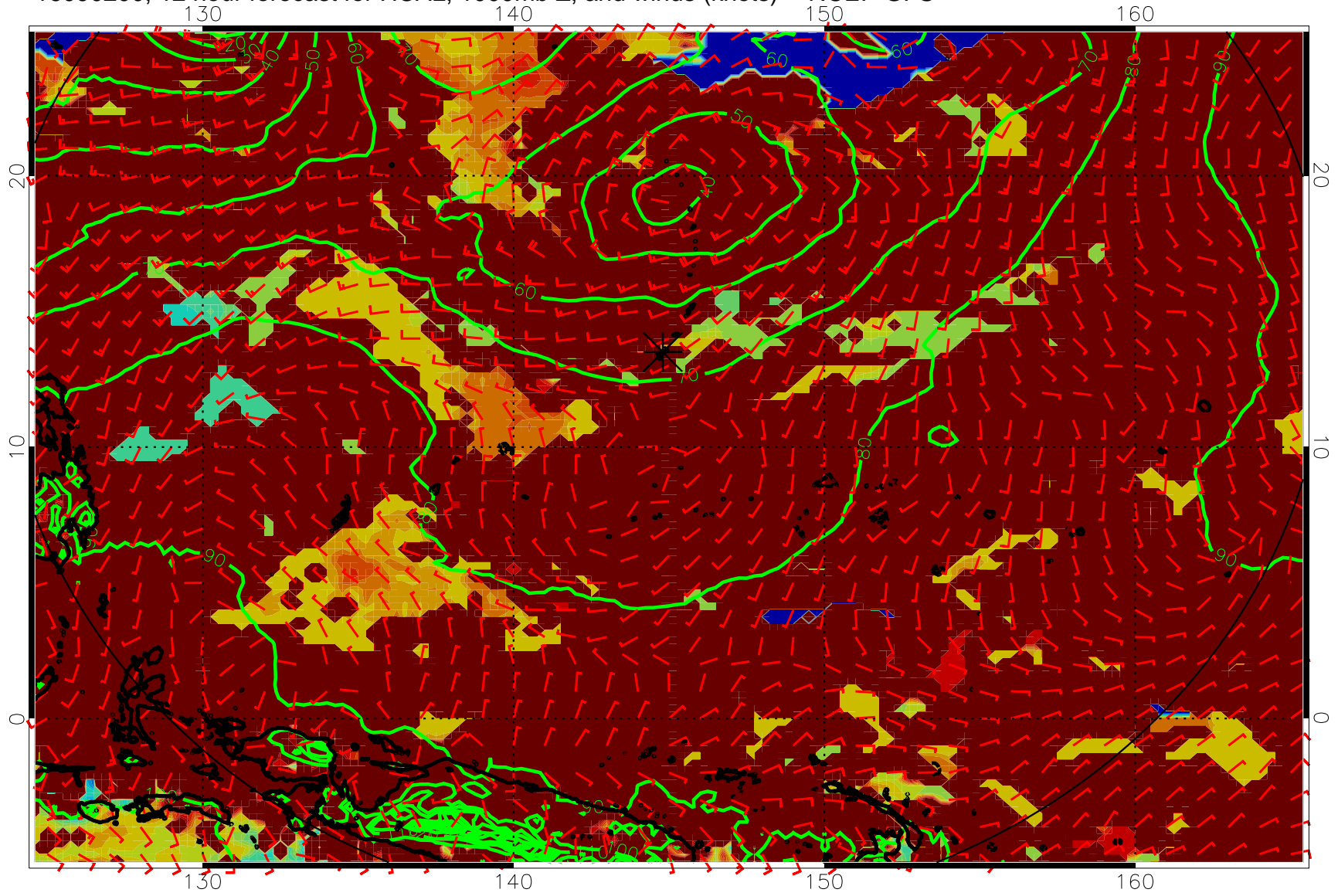
16090200, 12 hour forecast for HCAL, 1000mb Z, and winds (knots) -- NCEP GFS
