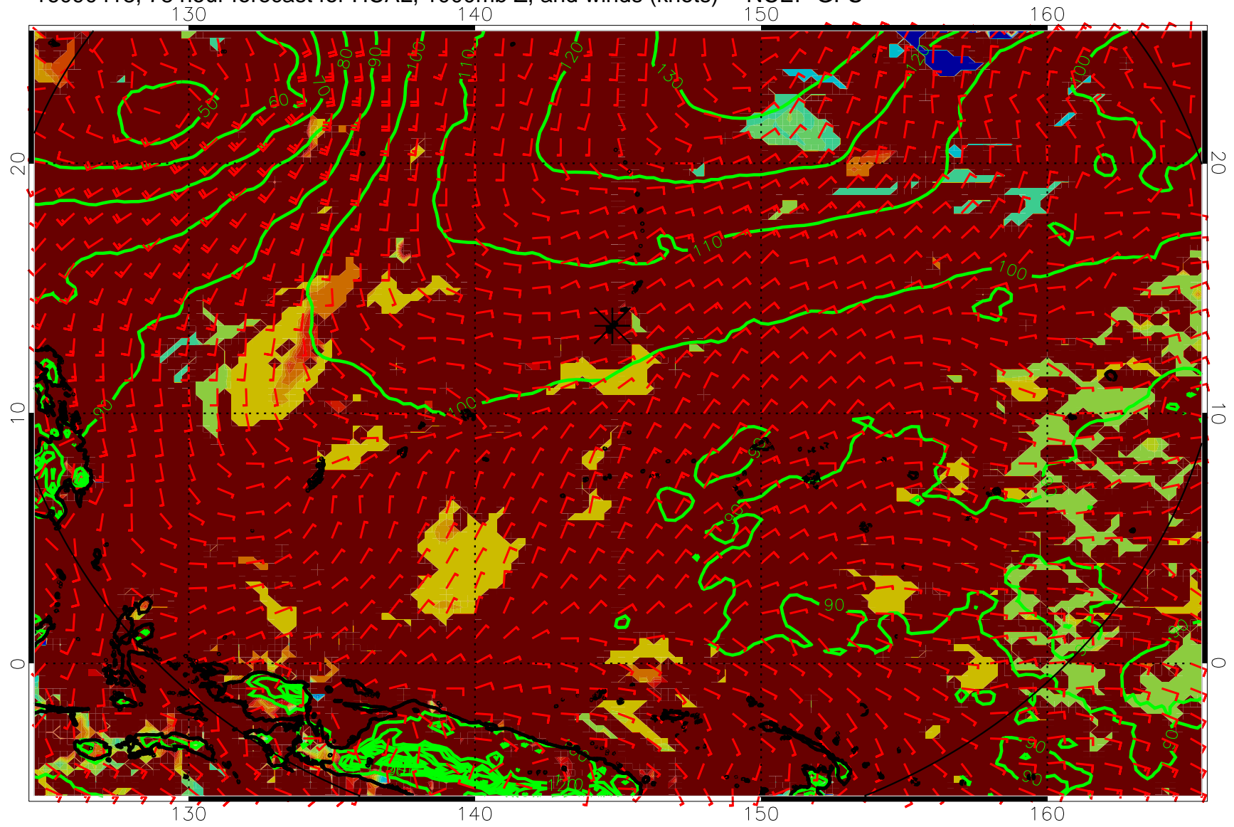
16090418, 78 hour forecast for HCAL, 1000mb Z, and winds (knots) -- NCEP GFS
