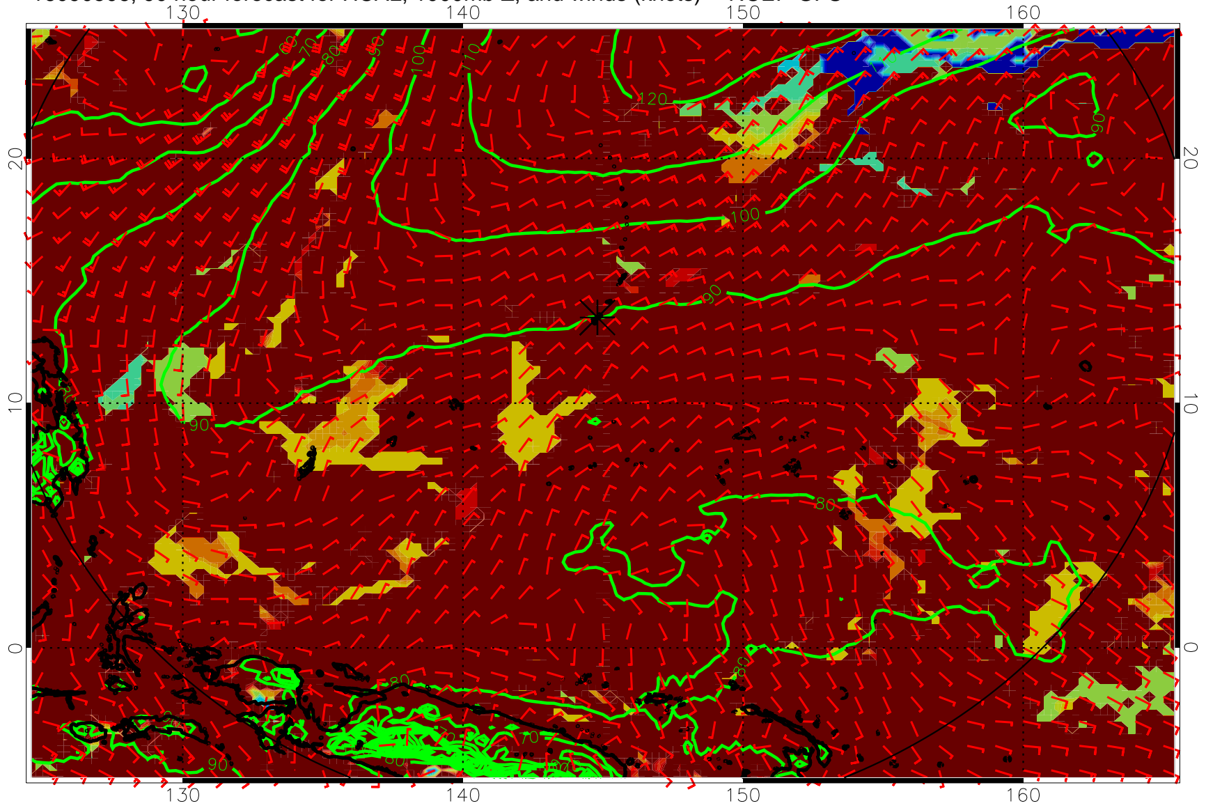
16090506, 90 hour forecast for HCAL, 1000mb Z, and winds (knots) -- NCEP GFS
