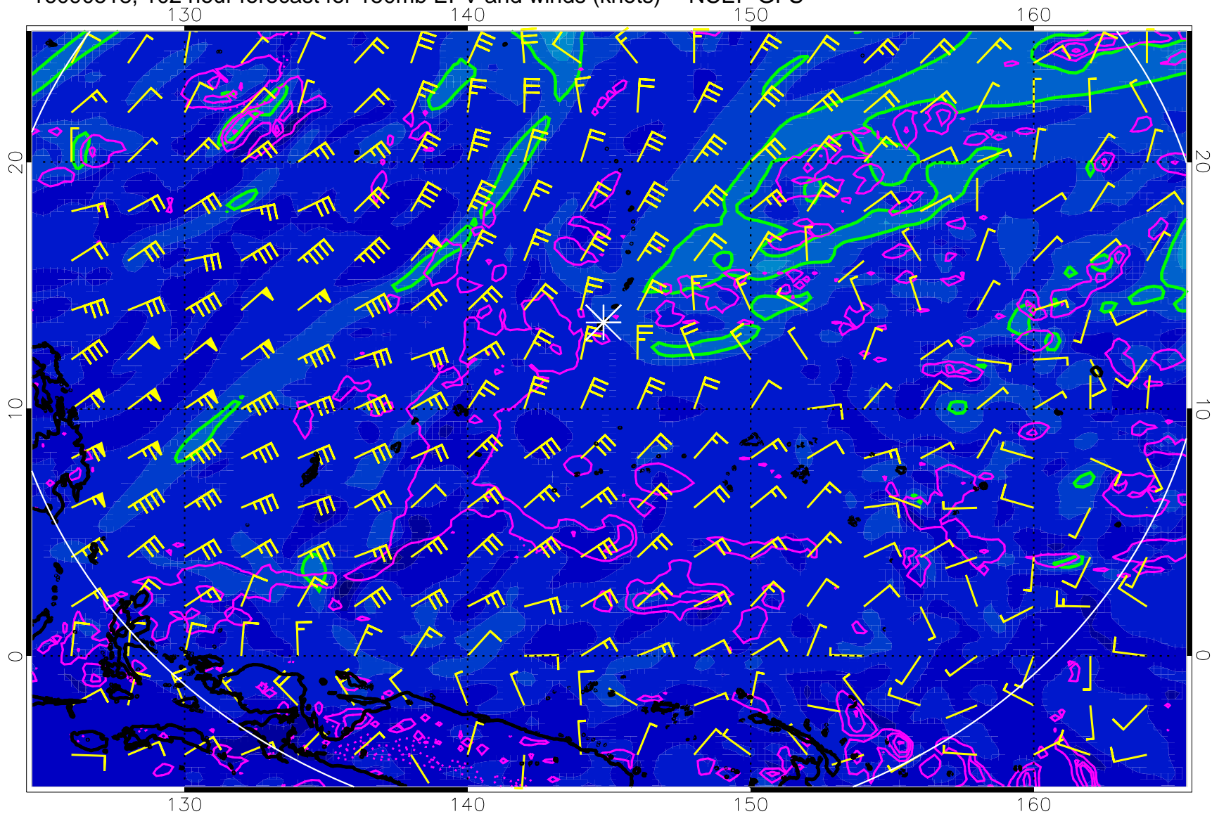
16090518, 102 hour forecast for 150mb EPV and winds (knots) -- NCEP GFS
