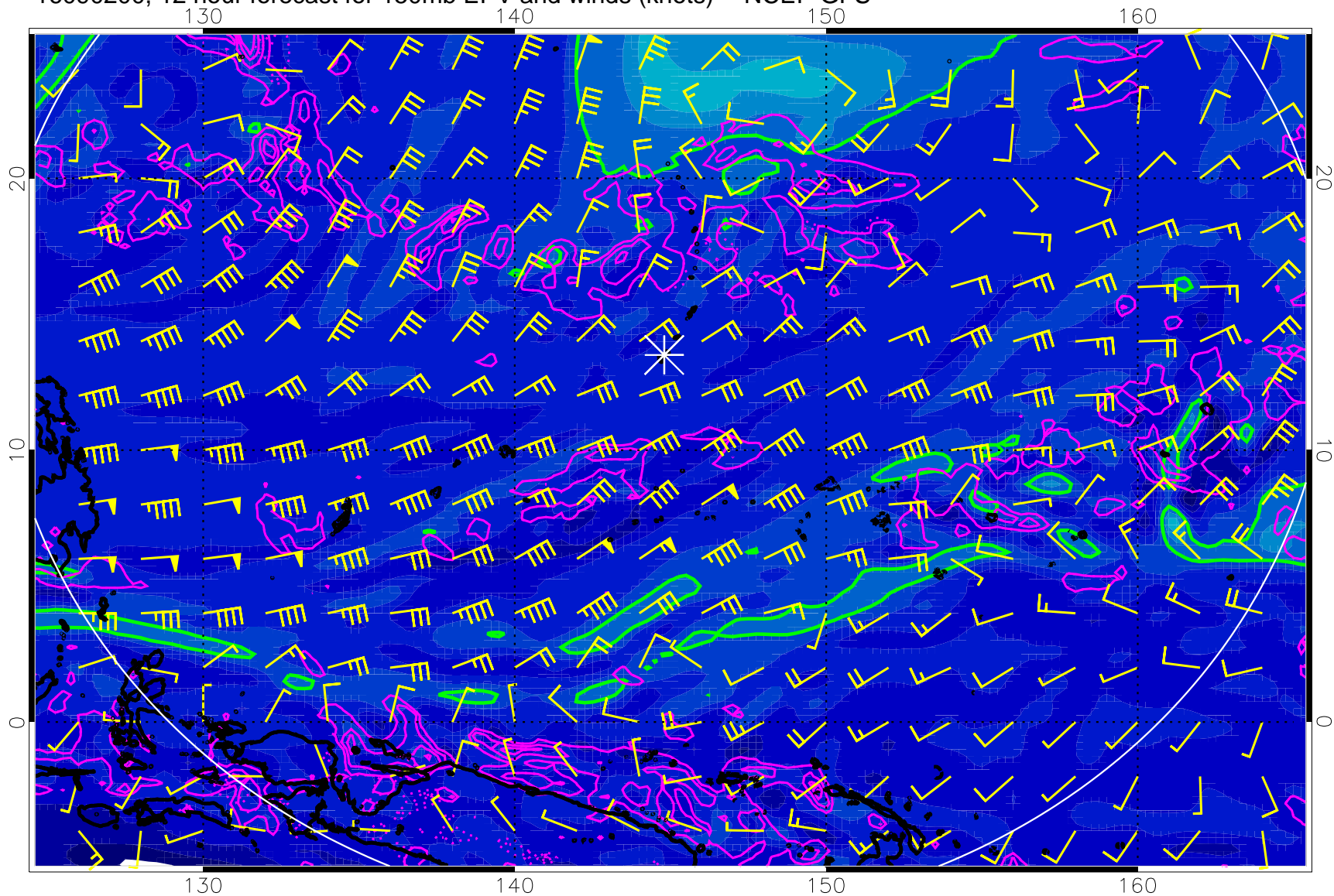
16090200, 12 hour forecast for 150mb EPV and winds (knots) -- NCEP GFS
