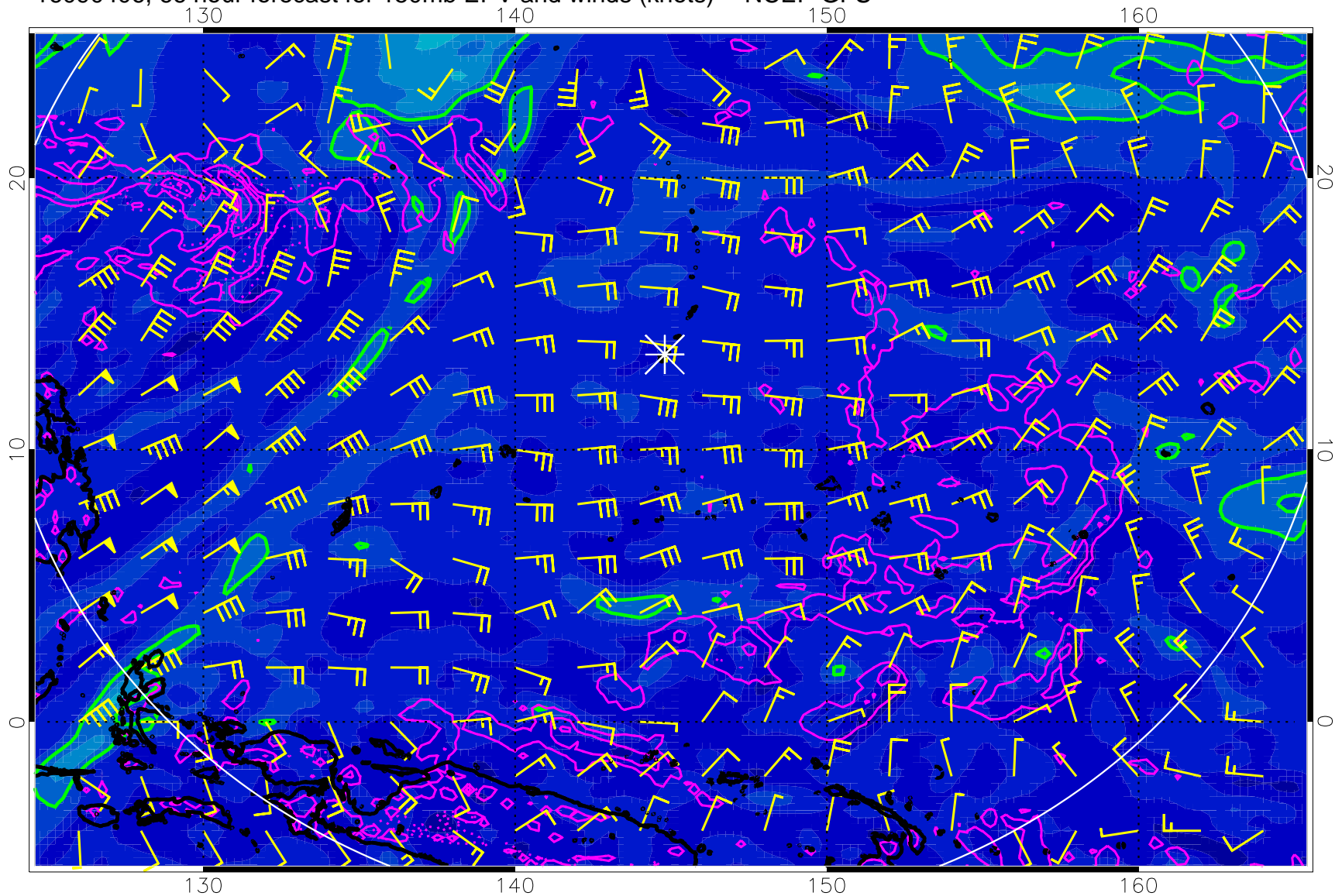
16090406, 66 hour forecast for 150mb EPV and winds (knots) -- NCEP GFS
