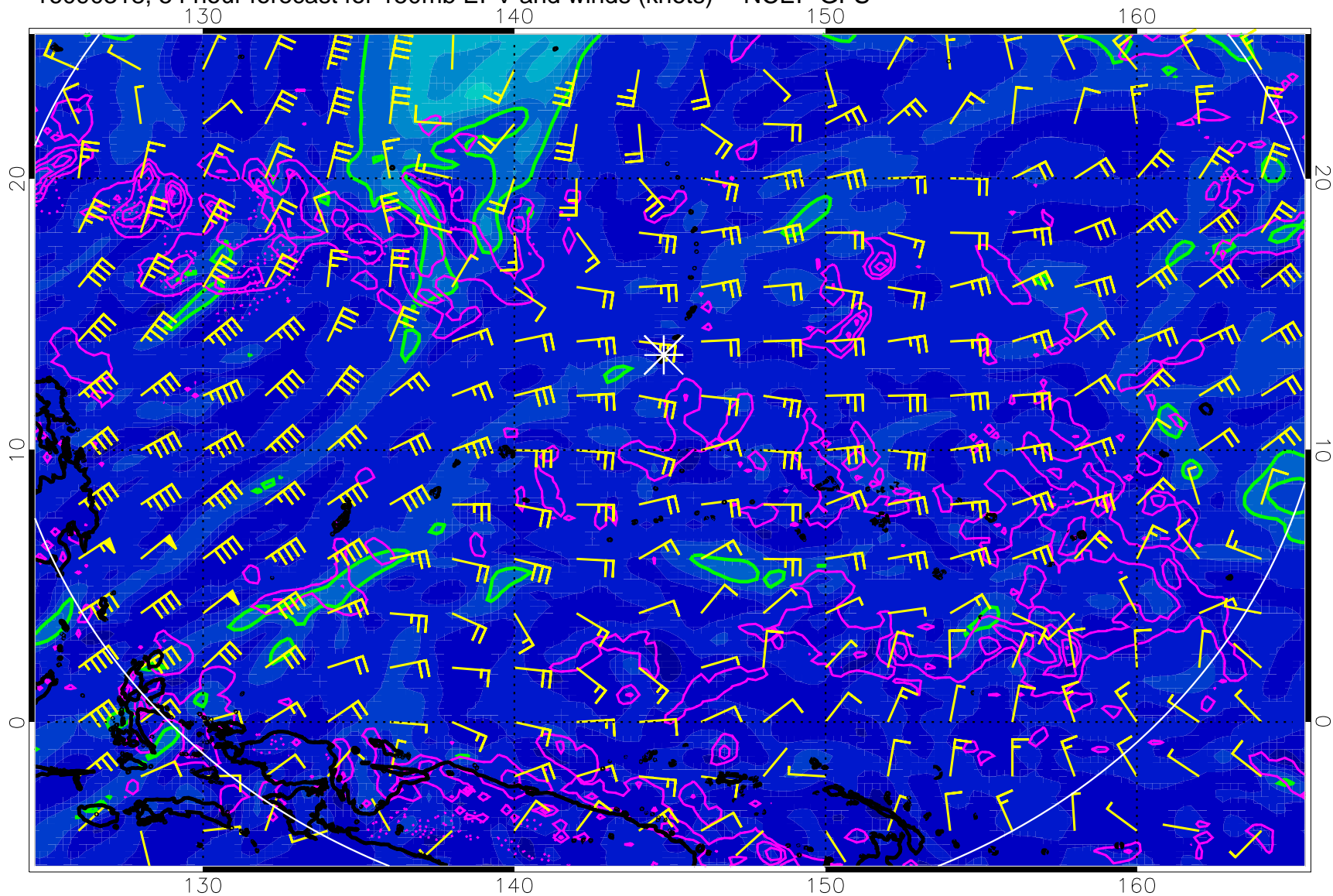
16090318, 54 hour forecast for 150mb EPV and winds (knots) -- NCEP GFS
