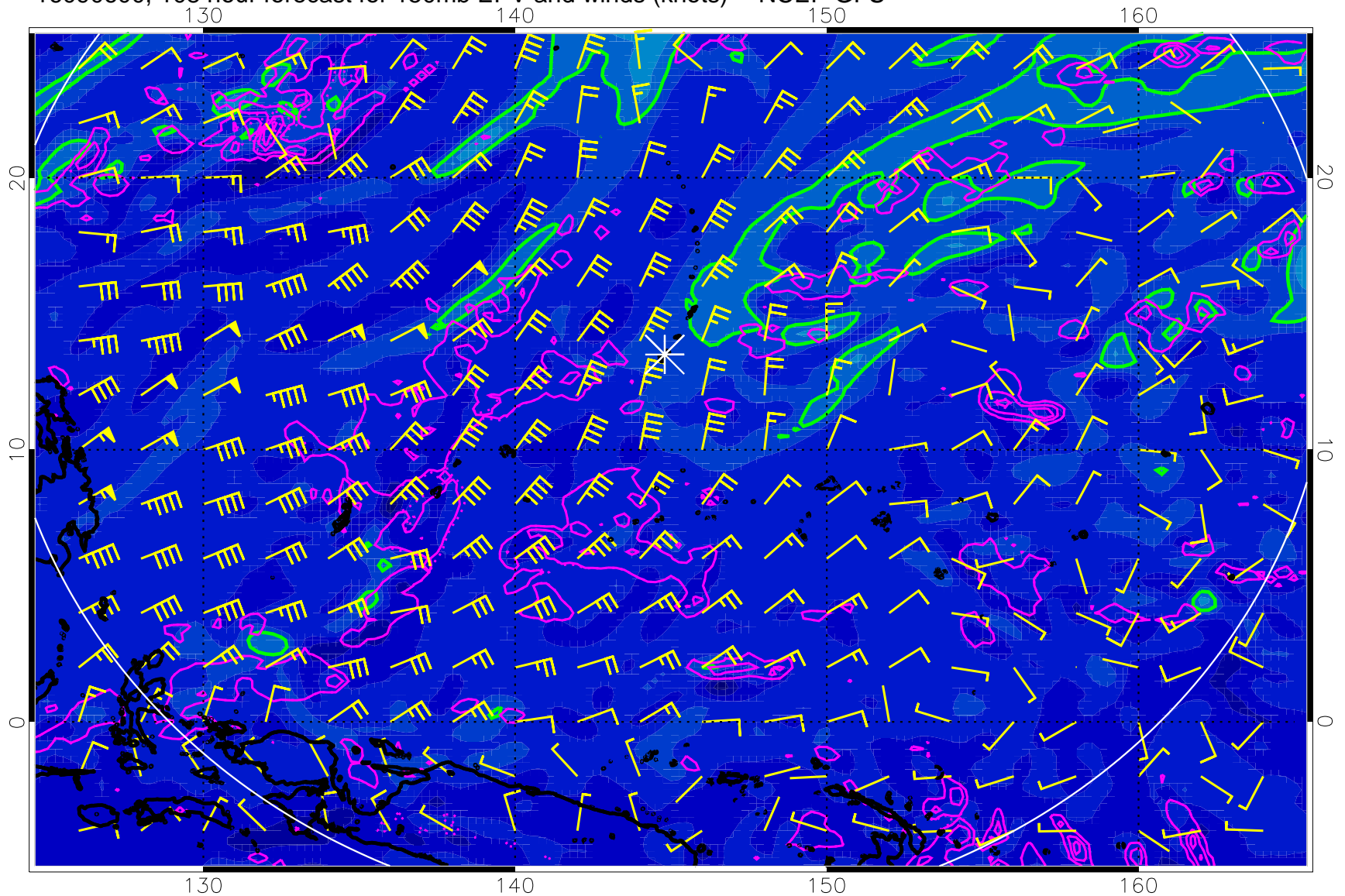
16090600, 108 hour forecast for 150mb EPV and winds (knots) -- NCEP GFS
