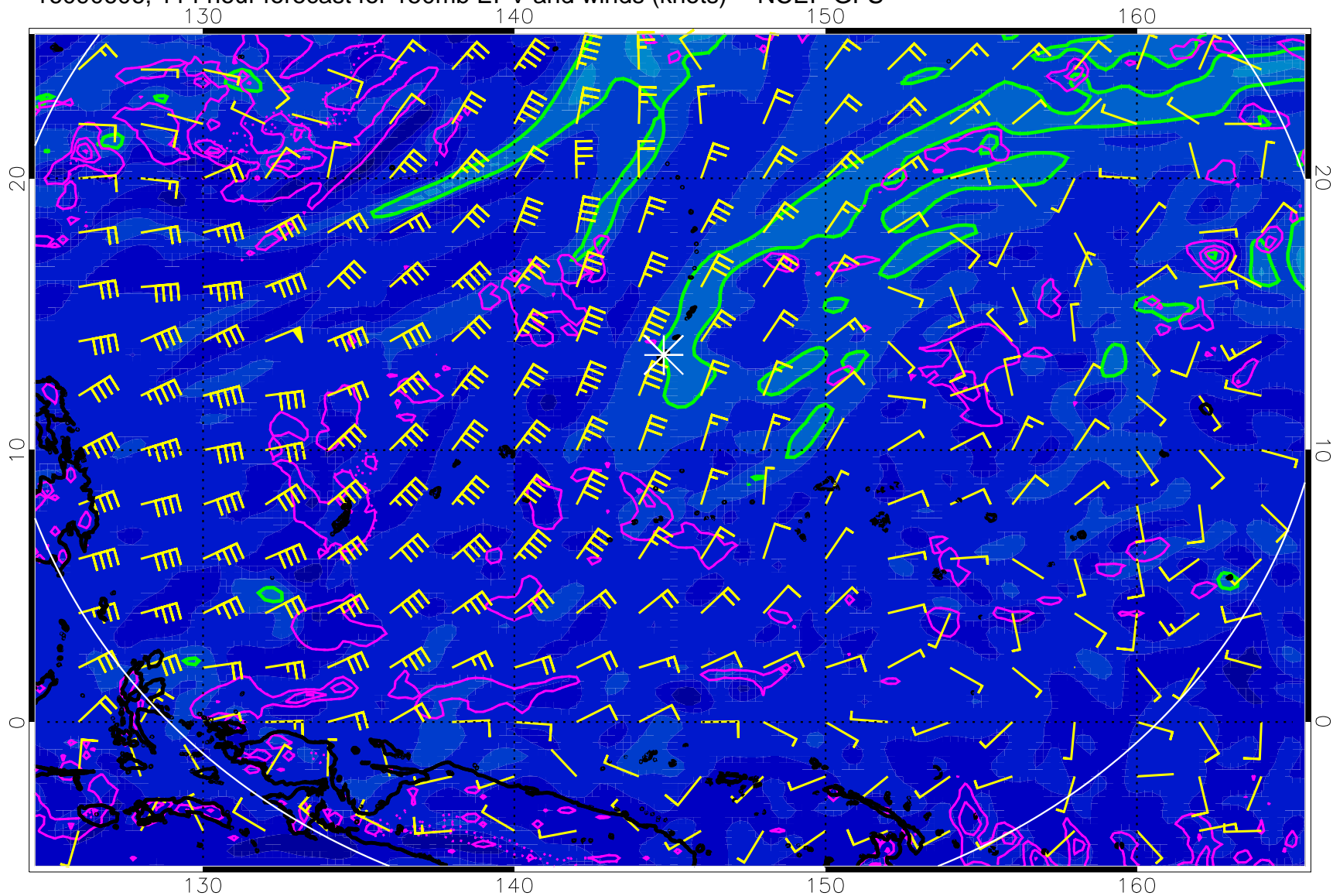
16090606, 114 hour forecast for 150mb EPV and winds (knots) -- NCEP GFS
