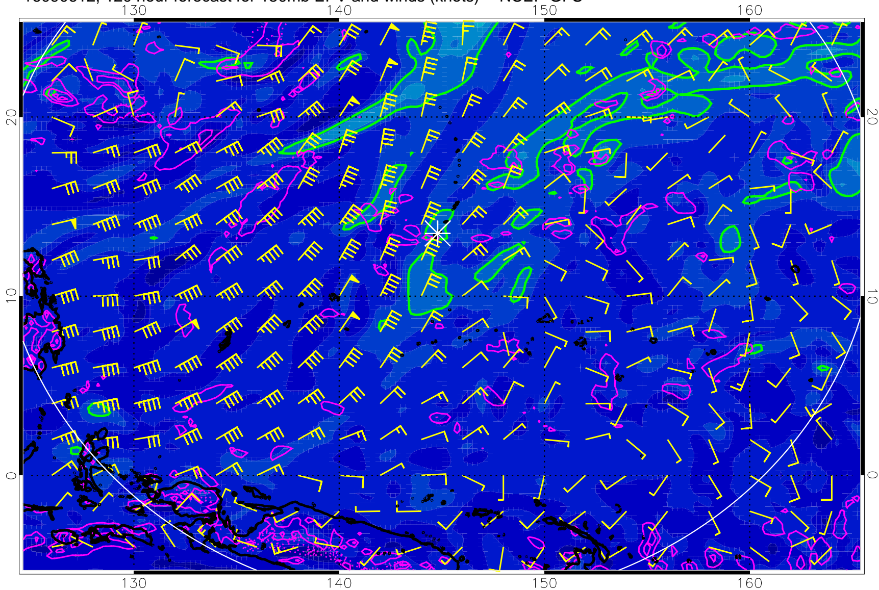
16090612, 120 hour forecast for 150mb EPV and winds (knots) -- NCEP GFS
