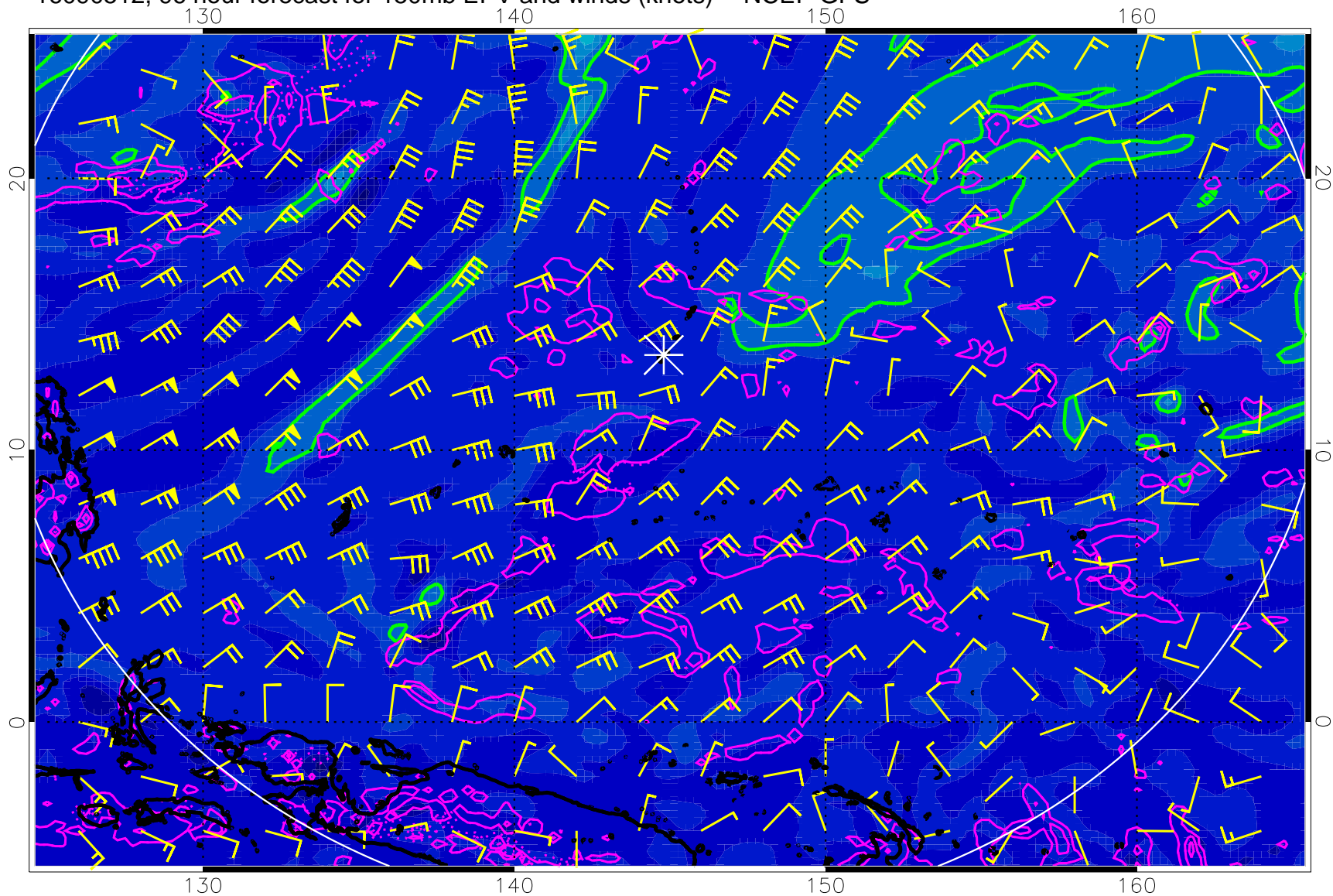
16090512, 96 hour forecast for 150mb EPV and winds (knots) -- NCEP GFS
