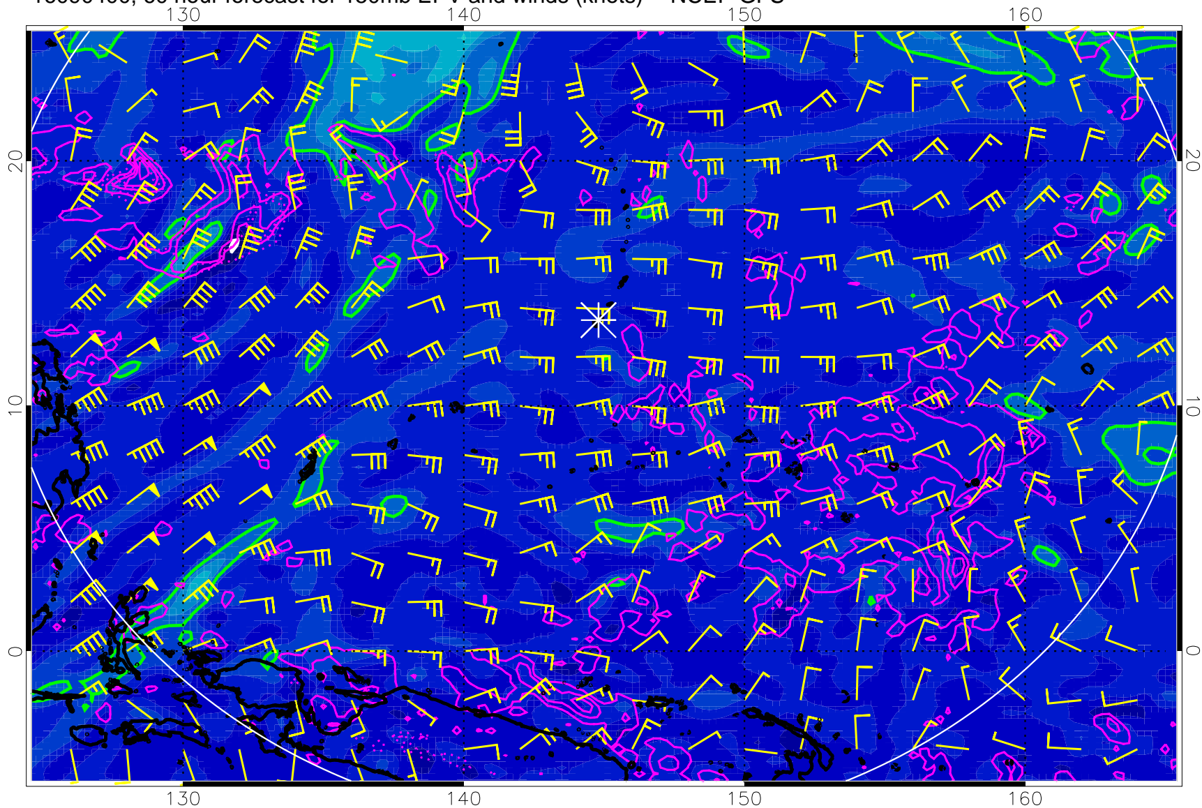
16090400, 60 hour forecast for 150mb EPV and winds (knots) -- NCEP GFS
