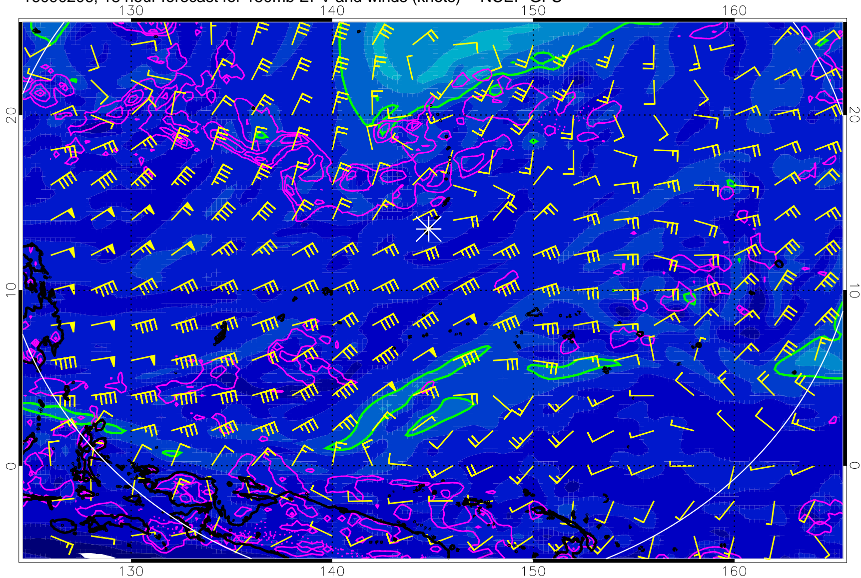
16090206, 18 hour forecast for 150mb EPV and winds (knots) -- NCEP GFS
