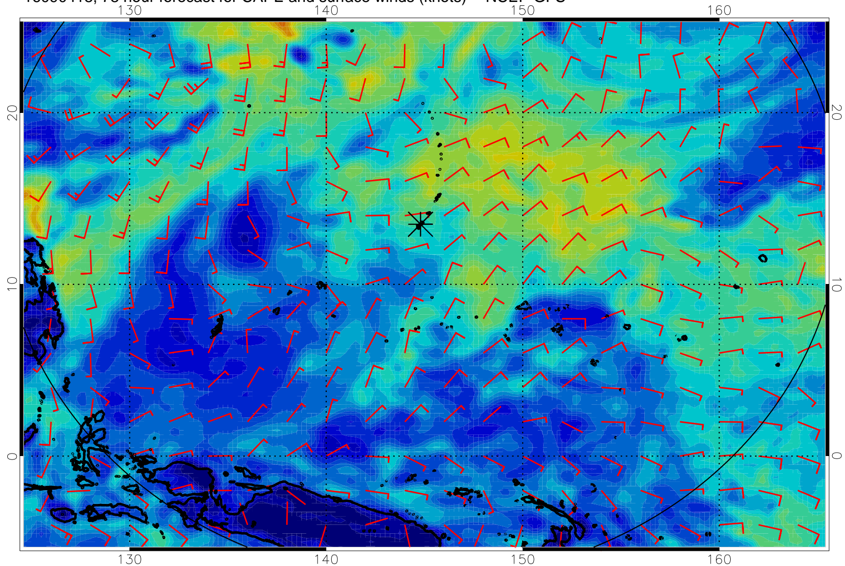
16090418, 78 hour forecast for CAPE and surface winds (knots) -- NCEP GFS
