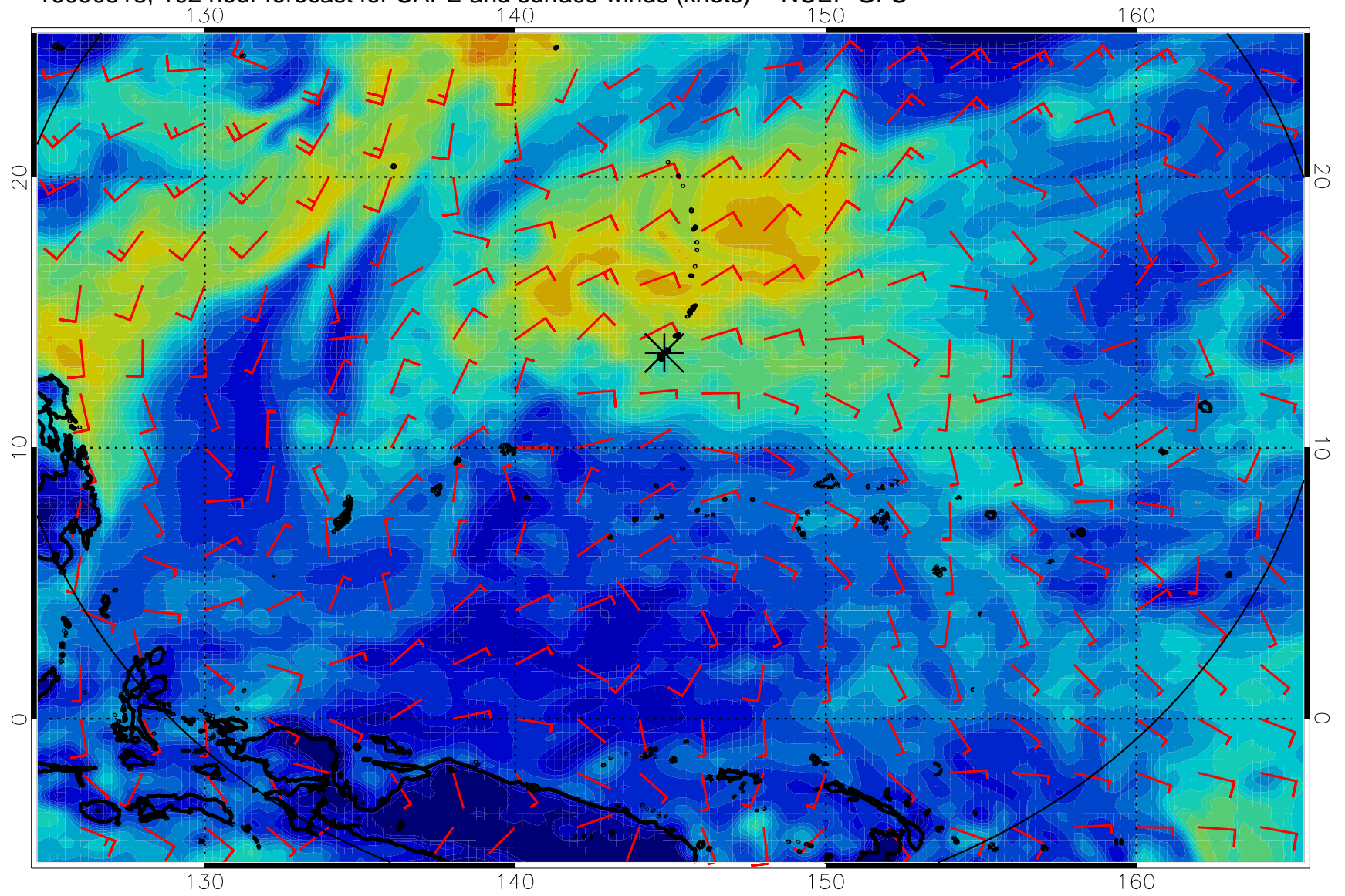
16090518, 102 hour forecast for CAPE and surface winds (knots) -- NCEP GFS
