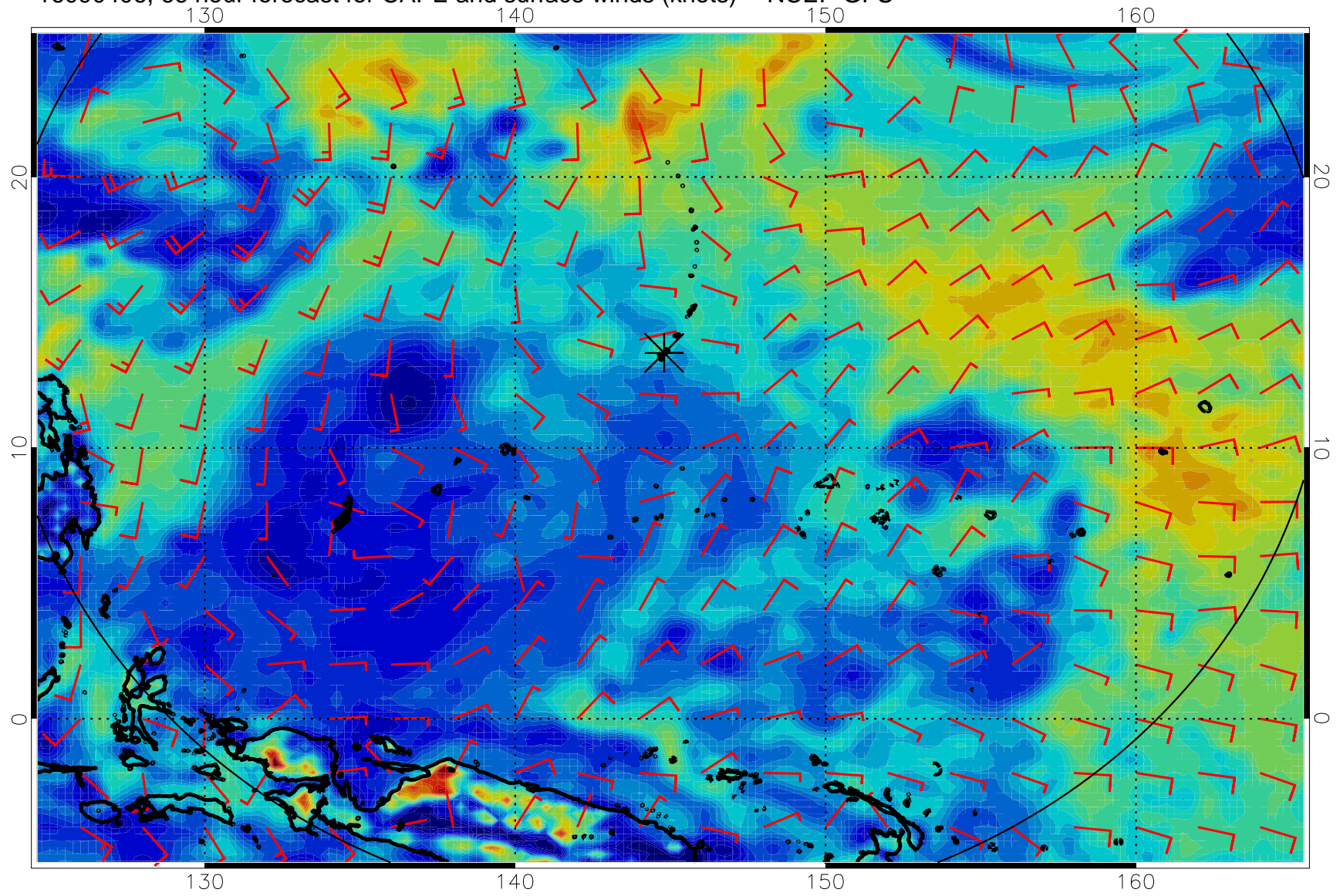
16090406, 66 hour forecast for CAPE and surface winds (knots) -- NCEP GFS
