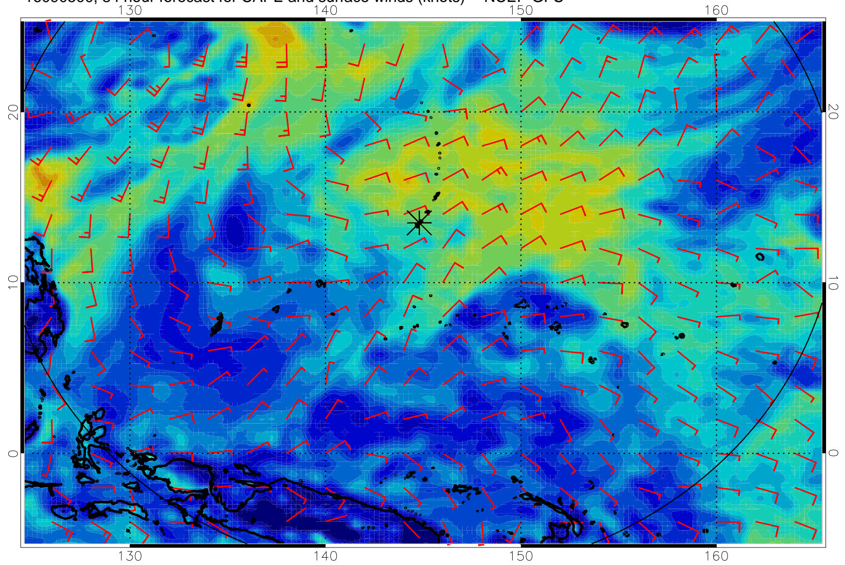
16090500, 84 hour forecast for CAPE and surface winds (knots) -- NCEP GFS
