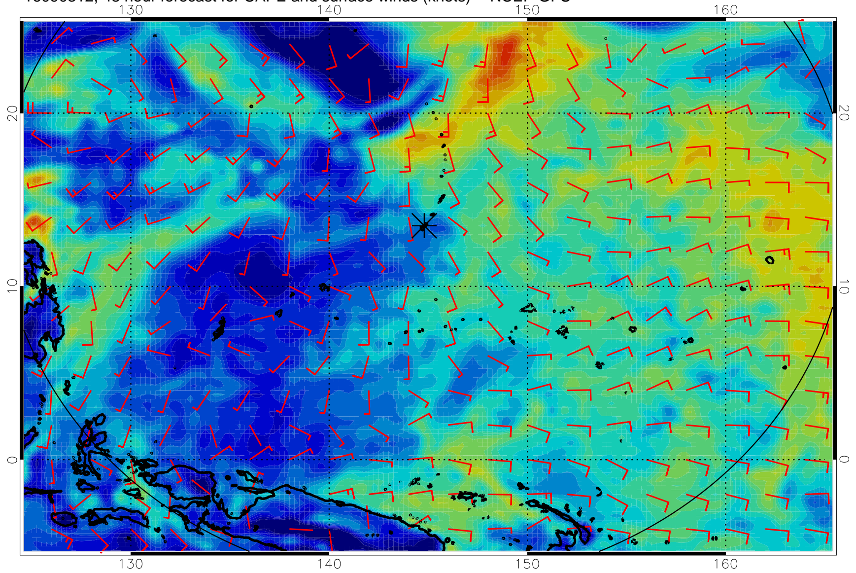
16090312, 48 hour forecast for CAPE and surface winds (knots) -- NCEP GFS
