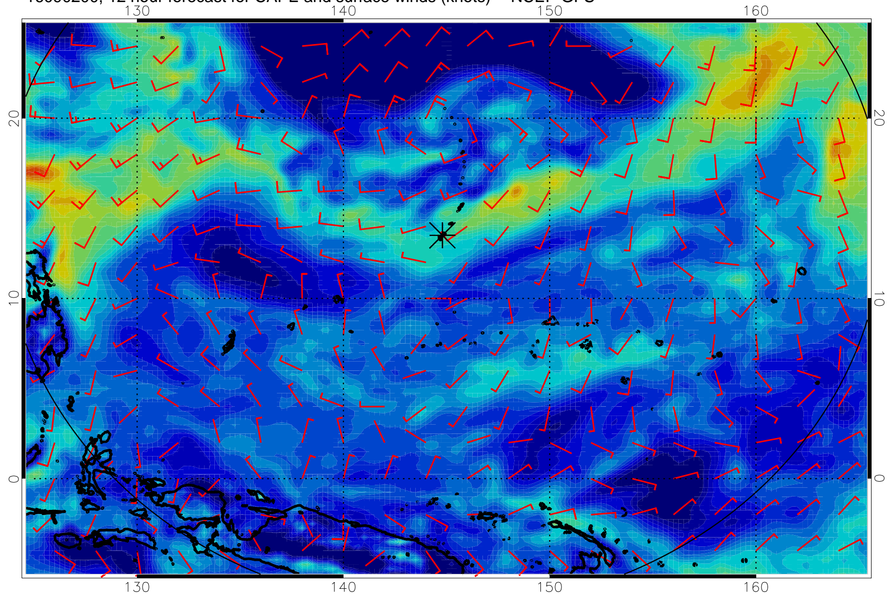
16090200, 12 hour forecast for CAPE and surface winds (knots) -- NCEP GFS
