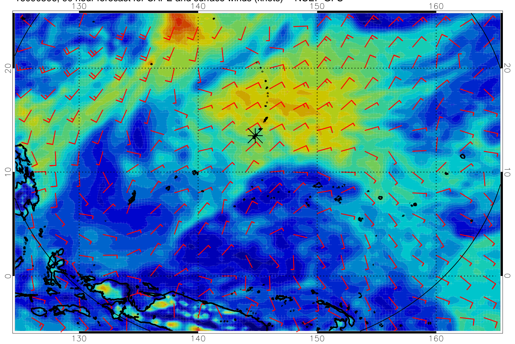
16090506, 90 hour forecast for CAPE and surface winds (knots) -- NCEP GFS
