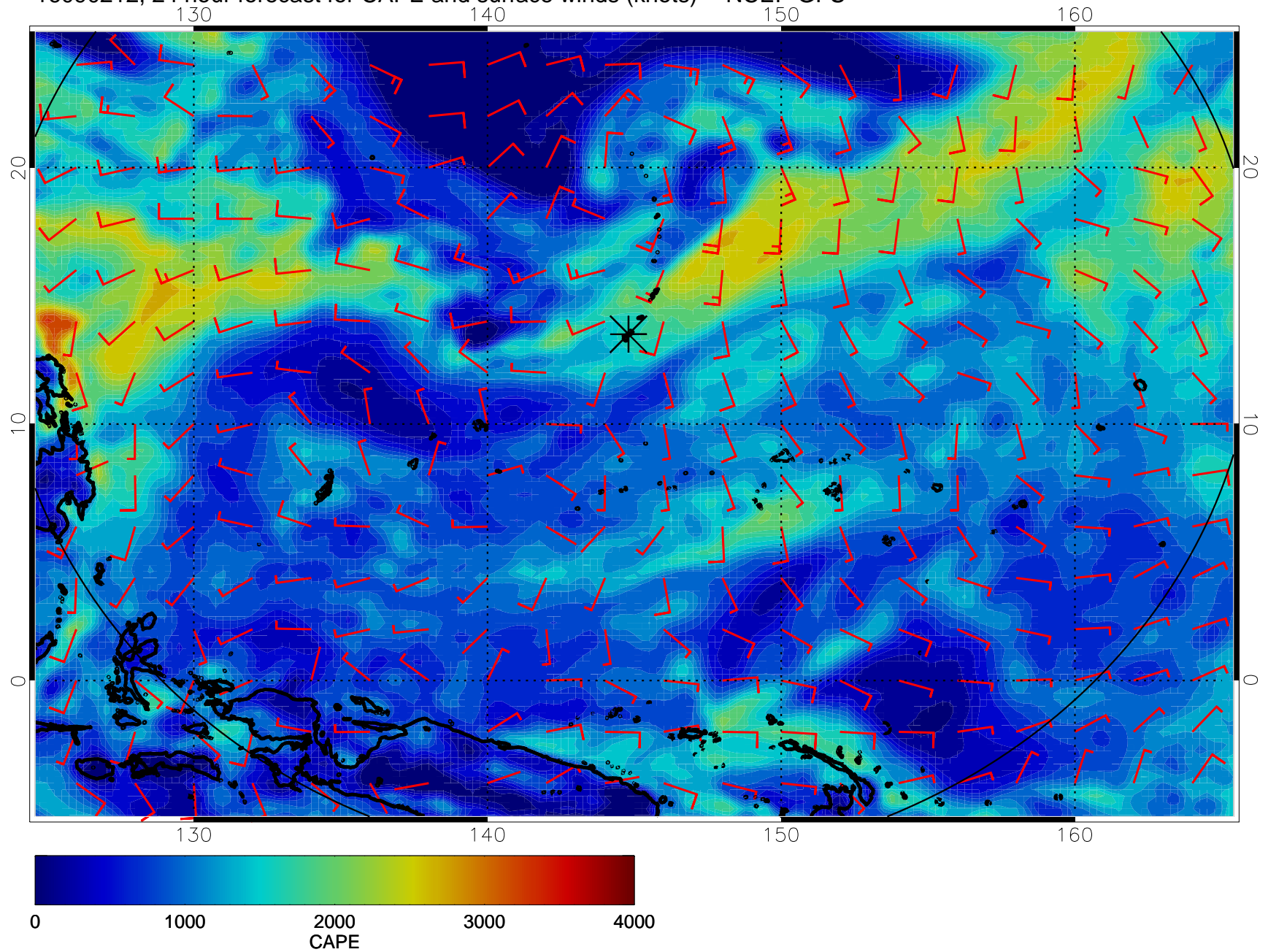
16090212, 24 hour forecast for CAPE and surface winds (knots) -- NCEP GFS
