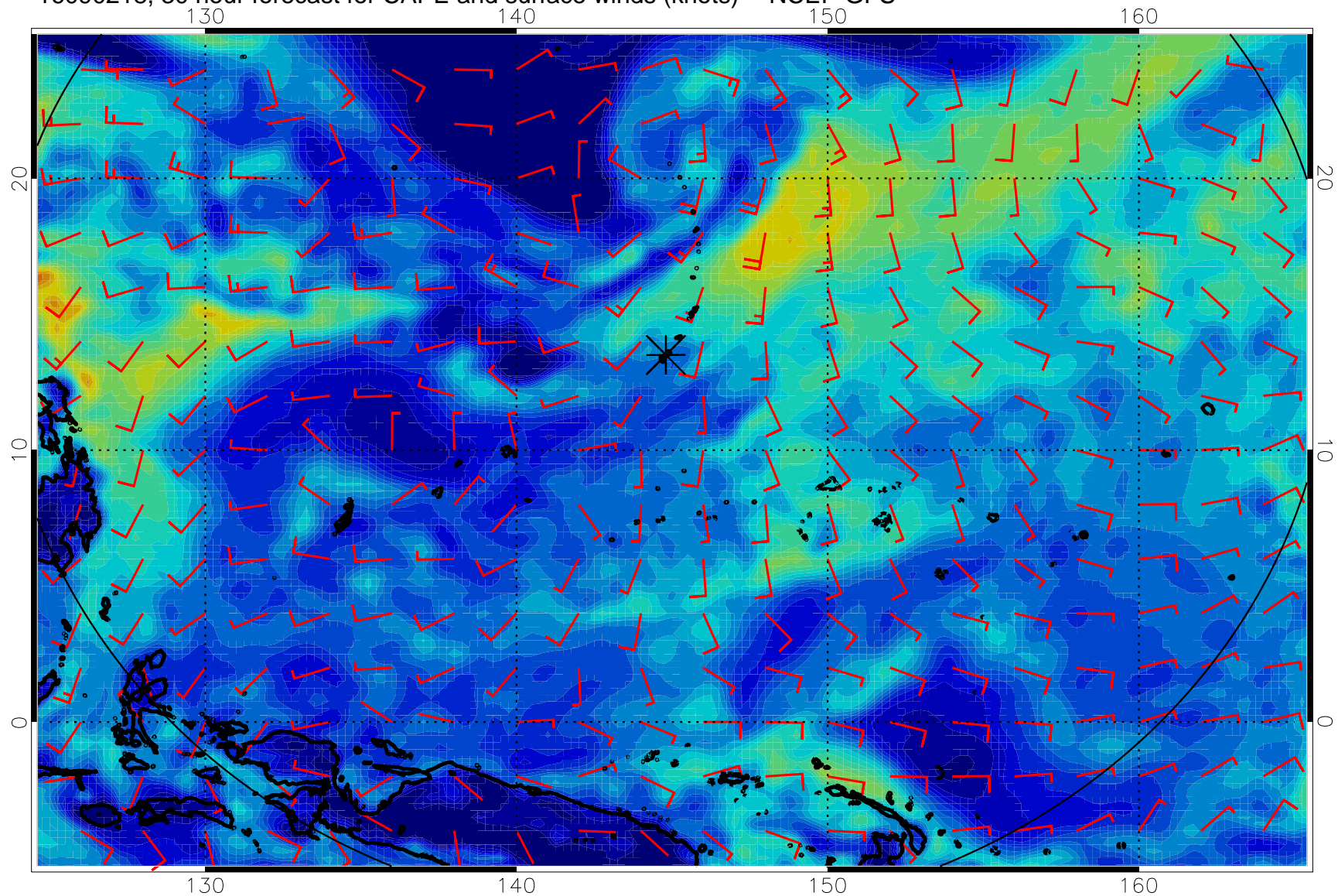
16090218, 30 hour forecast for CAPE and surface winds (knots) -- NCEP GFS
