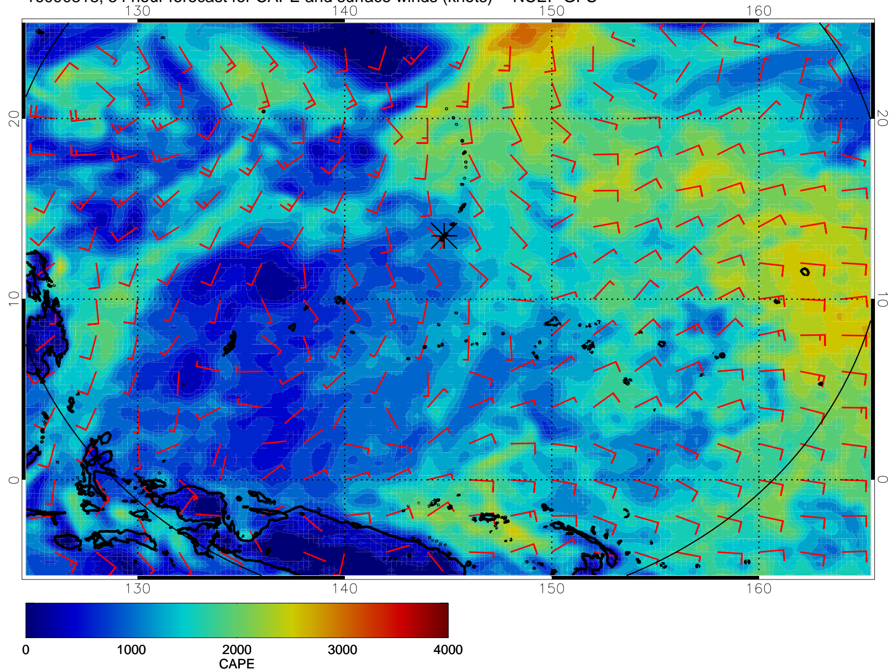
16090318, 54 hour forecast for CAPE and surface winds (knots) -- NCEP GFS
