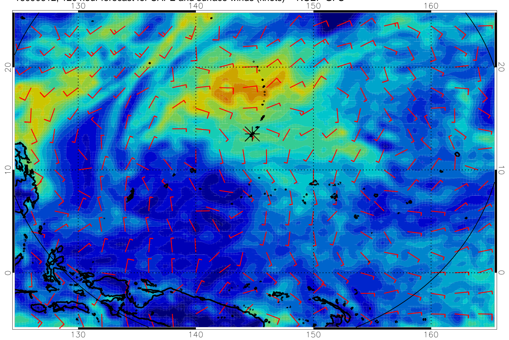
16090612, 120 hour forecast for CAPE and surface winds (knots) -- NCEP GFS
