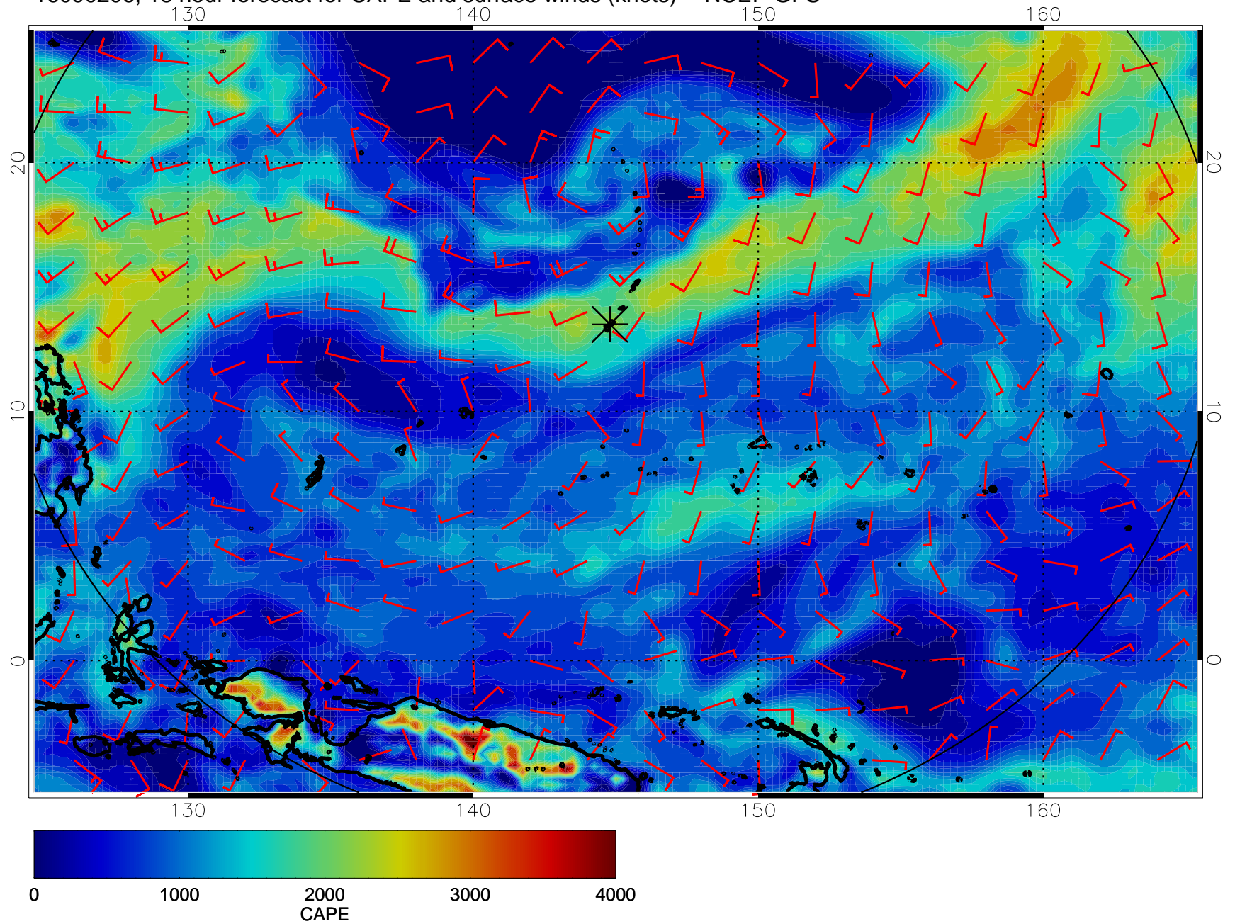
16090206, 18 hour forecast for CAPE and surface winds (knots) -- NCEP GFS
