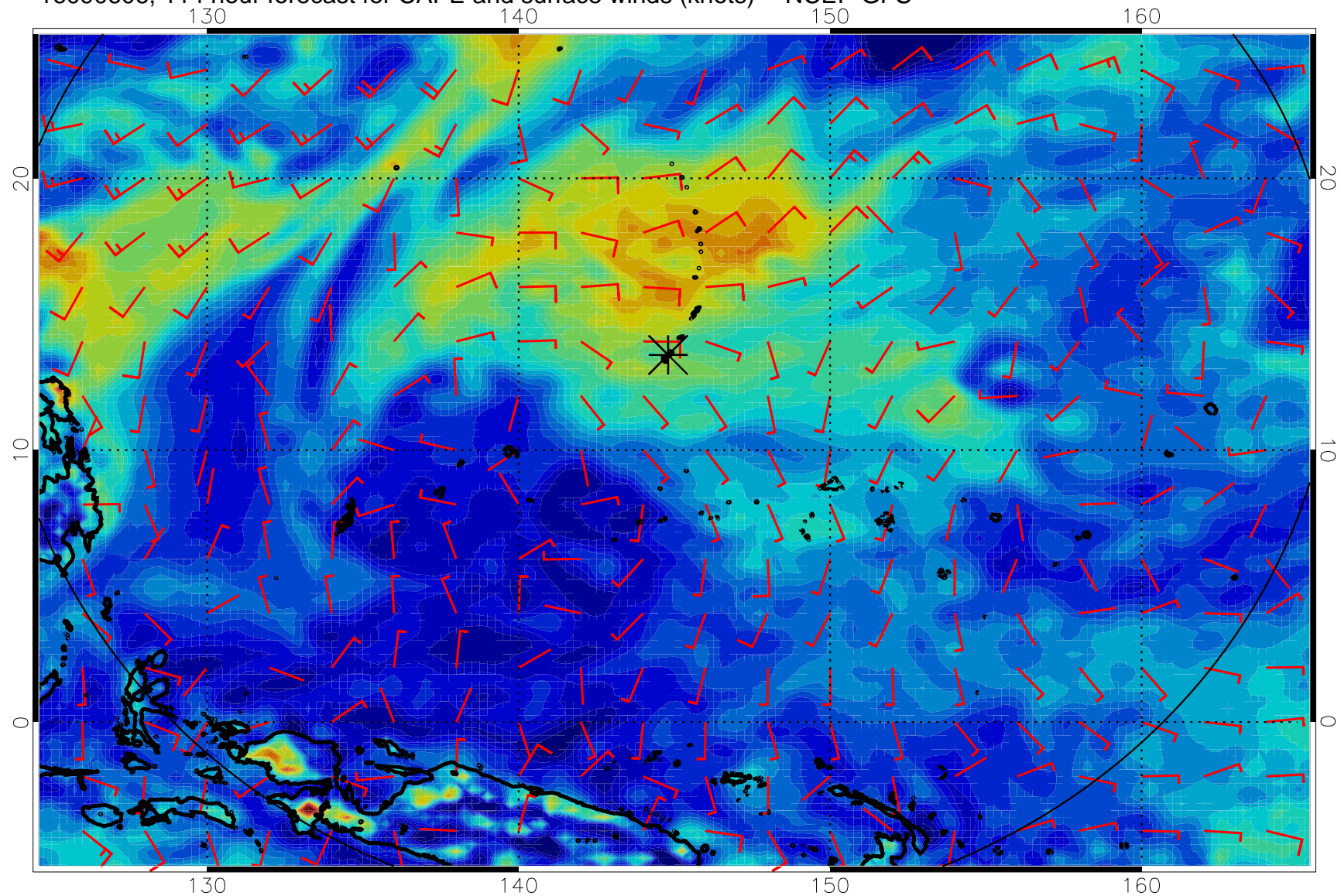
16090606, 114 hour forecast for CAPE and surface winds (knots) -- NCEP GFS
