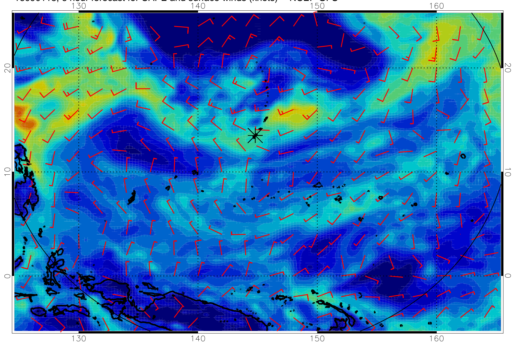
16090118, 6 hour forecast for CAPE and surface winds (knots) -- NCEP GFS
