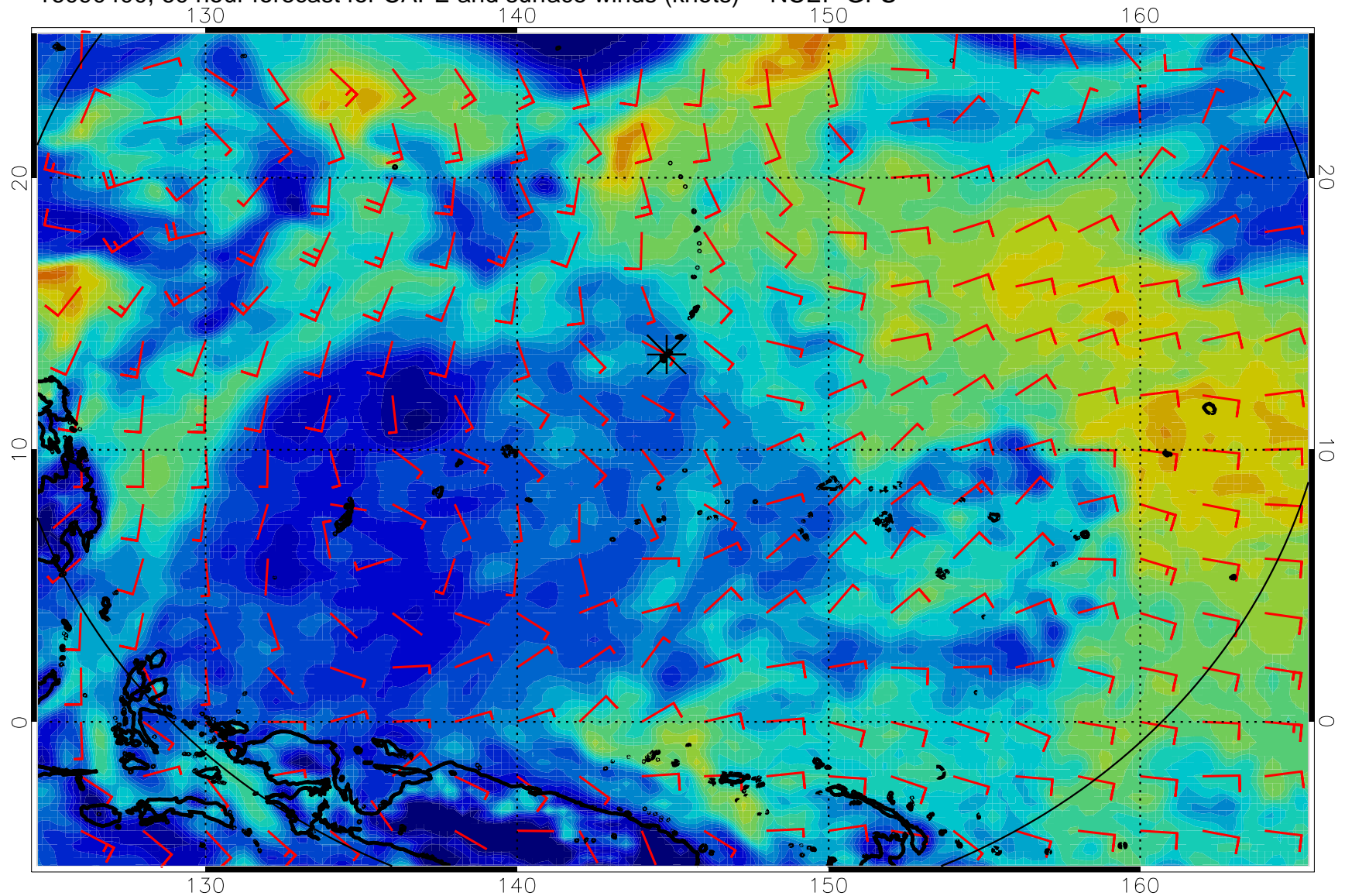
16090400, 60 hour forecast for CAPE and surface winds (knots) -- NCEP GFS
