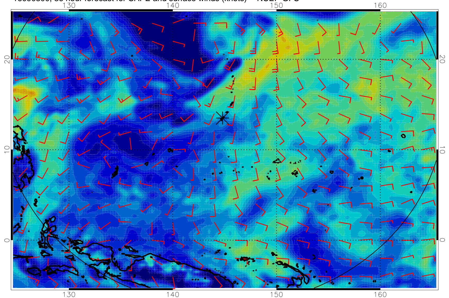
16090300, 36 hour forecast for CAPE and surface winds (knots) -- NCEP GFS
