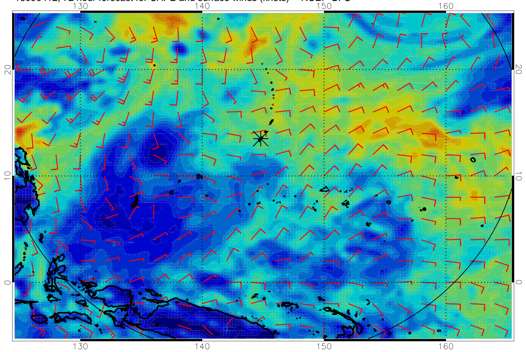
16090412, 72 hour forecast for CAPE and surface winds (knots) -- NCEP GFS
