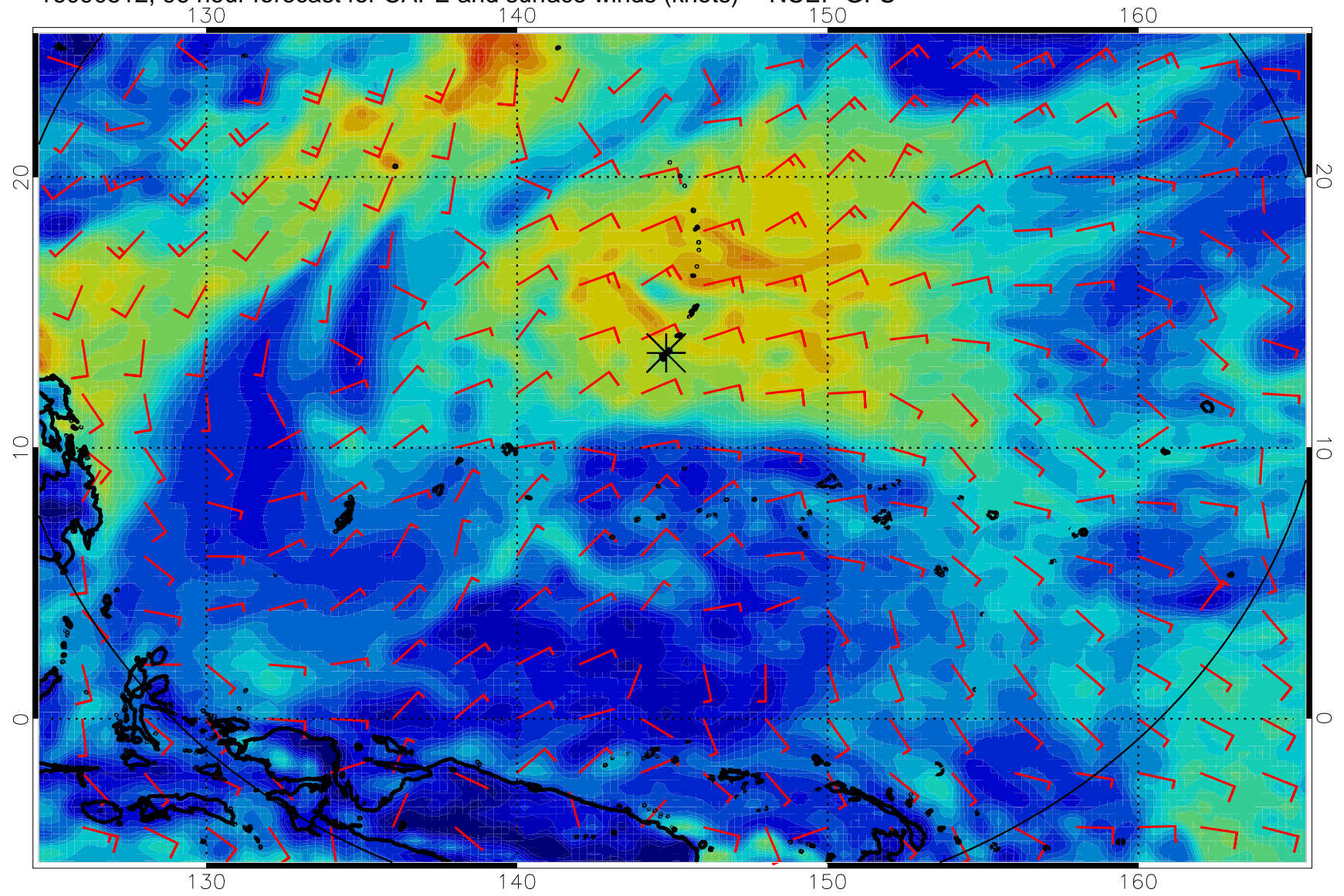
16090512, 96 hour forecast for CAPE and surface winds (knots) -- NCEP GFS
