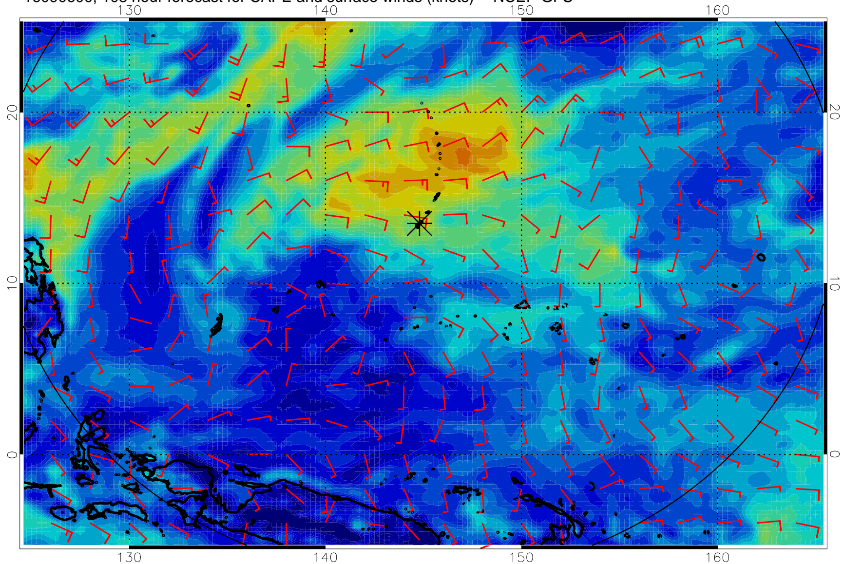
16090600, 108 hour forecast for CAPE and surface winds (knots) -- NCEP GFS
