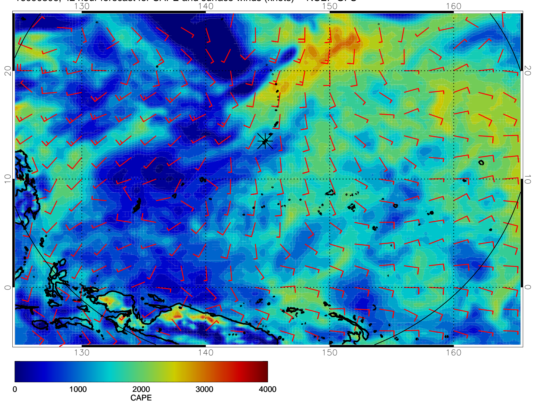
16090306, 42 hour forecast for CAPE and surface winds (knots) -- NCEP GFS
