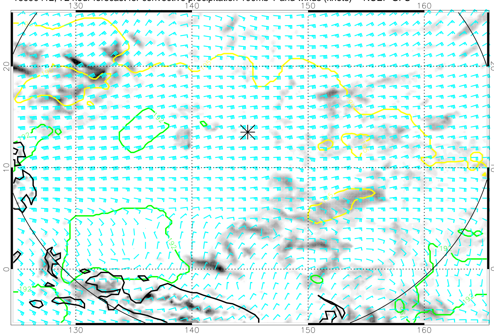
16090412, 72 hour forecast for convective precipitation 100mb T and winds (knots) -- NCEP GFS
