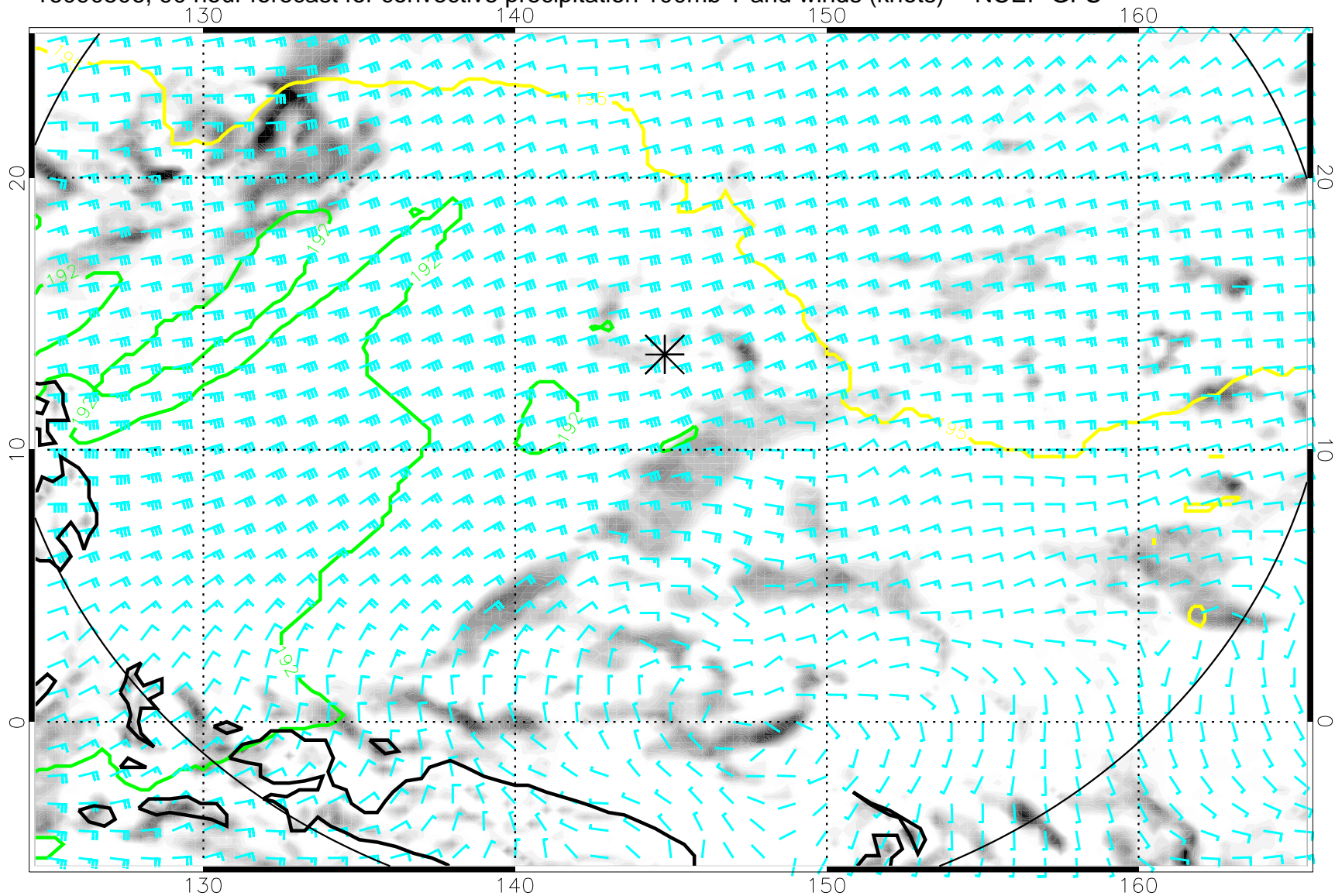
16090506, 90 hour forecast for convective precipitation 100mb T and winds (knots) -- NCEP GFS
