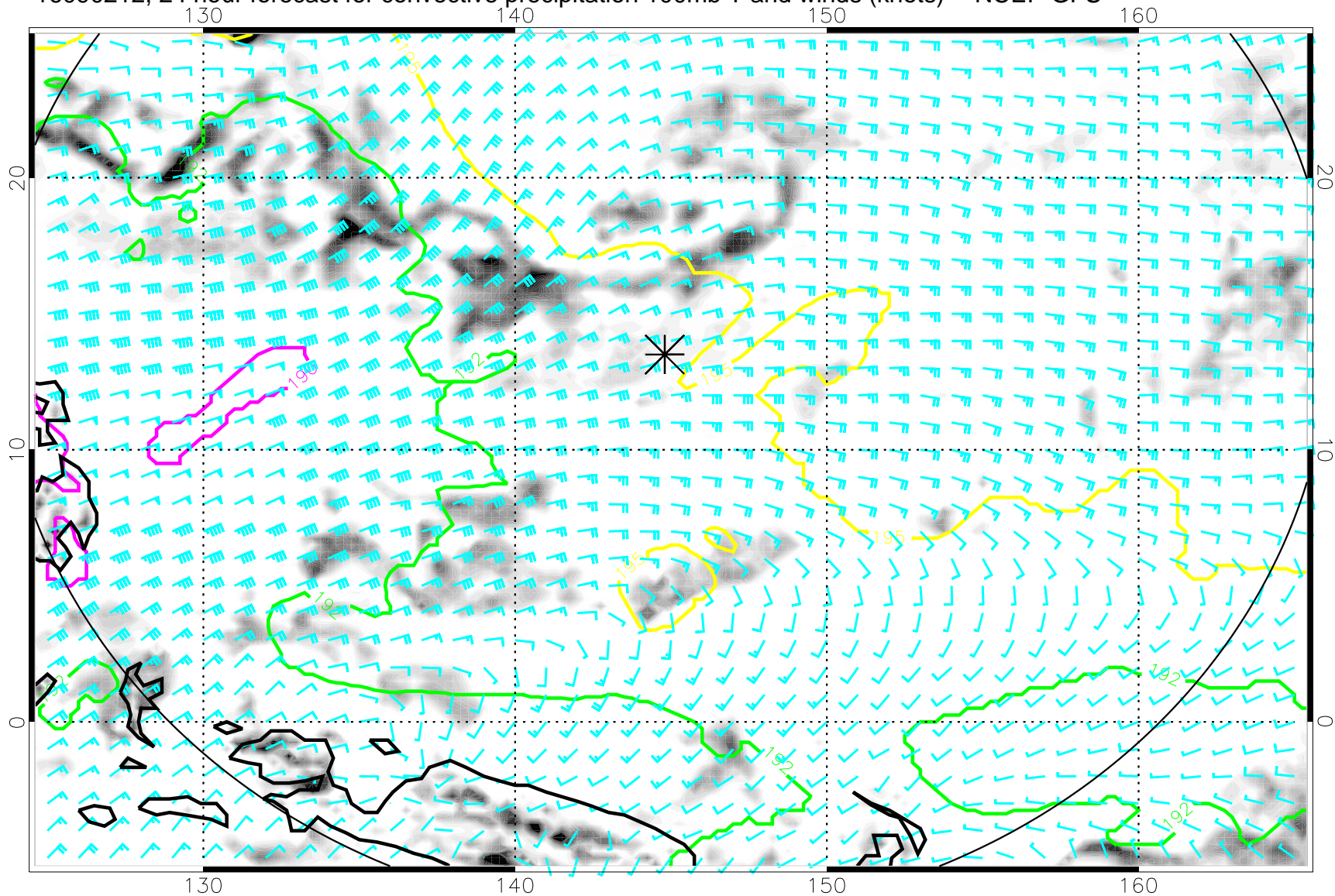
16090212, 24 hour forecast for convective precipitation 100mb T and winds (knots) -- NCEP GFS
