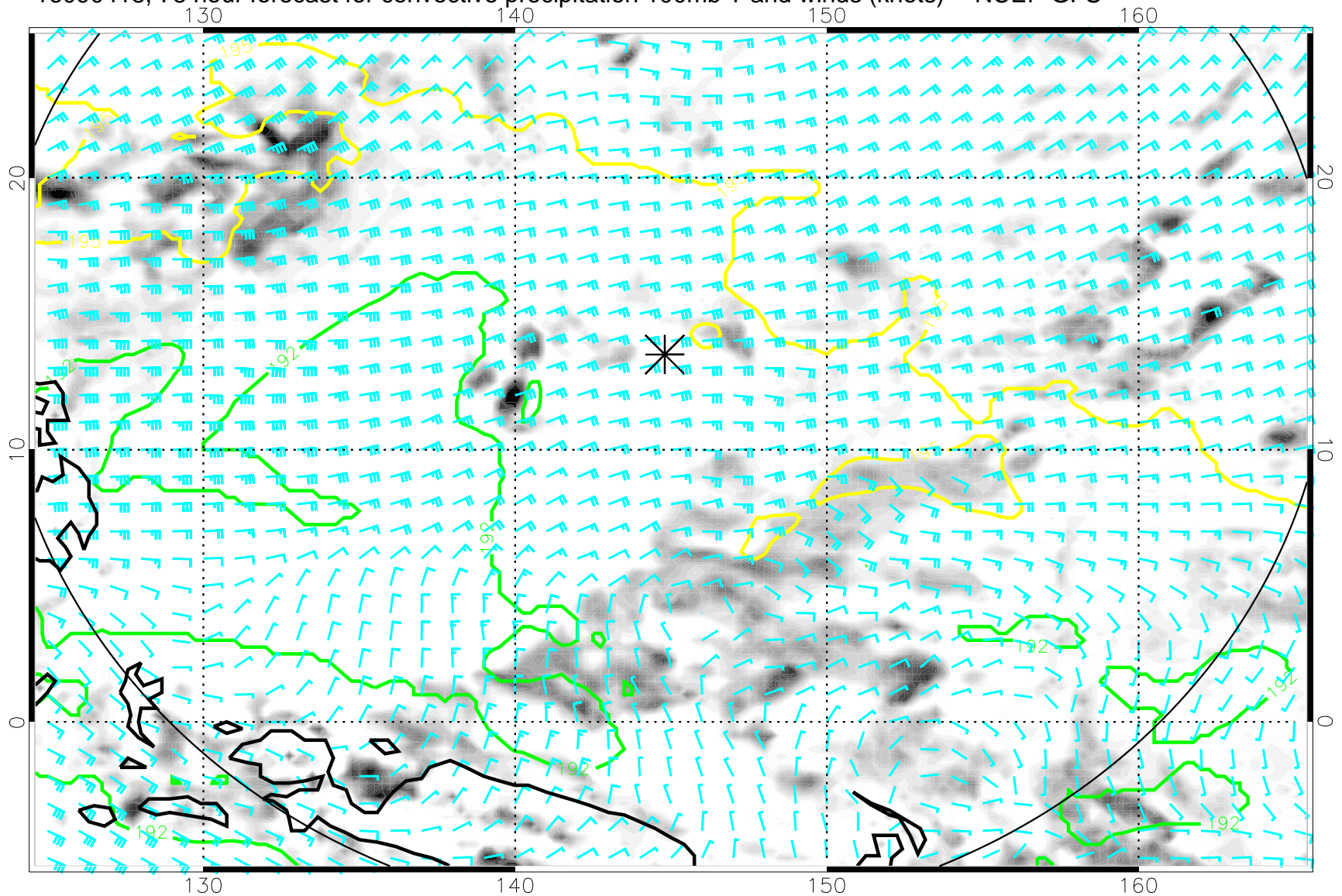
16090418, 78 hour forecast for convective precipitation 100mb T and winds (knots) -- NCEP GFS
