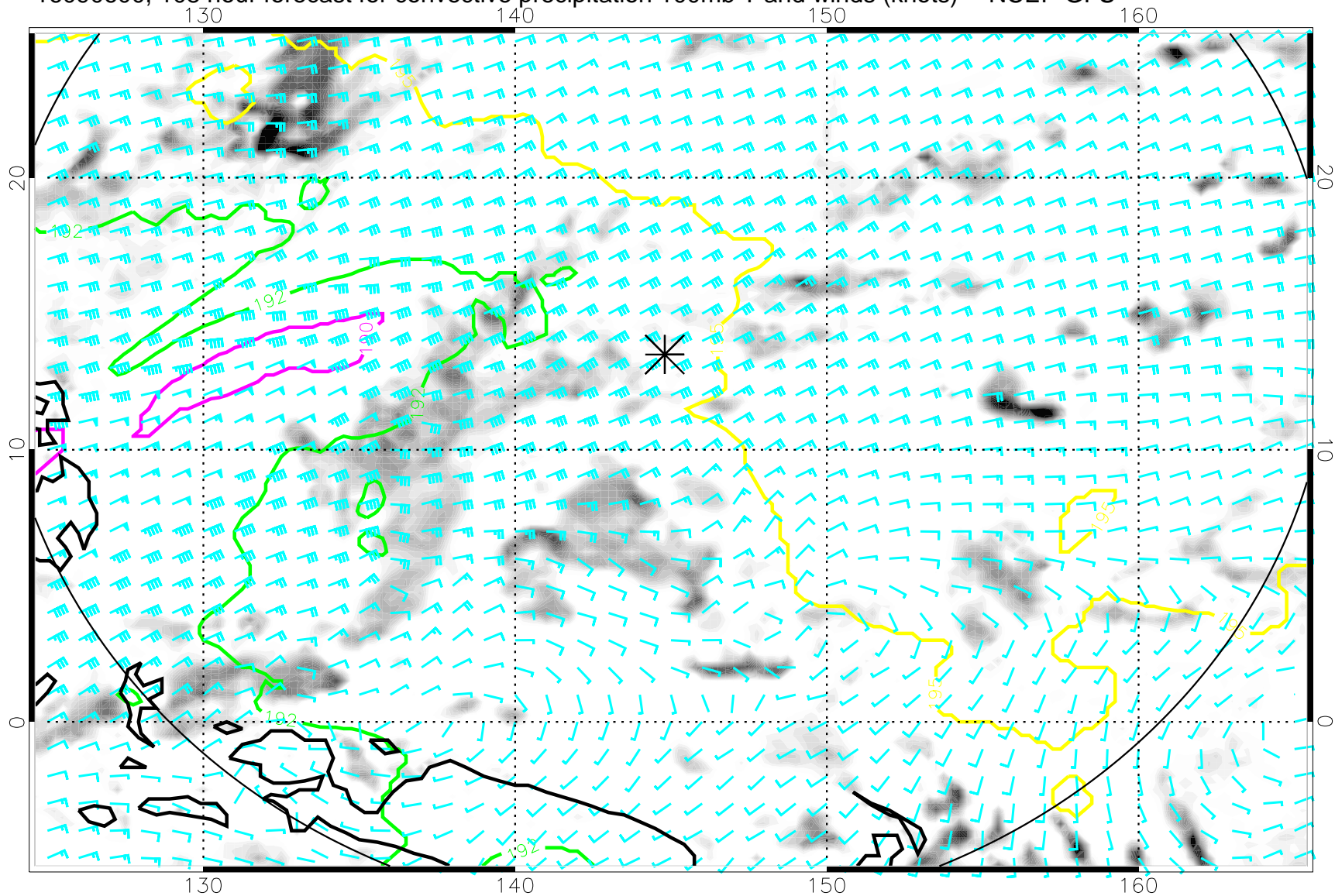
16090600, 108 hour forecast for convective precipitation 100mb T and winds (knots) -- NCEP GFS
