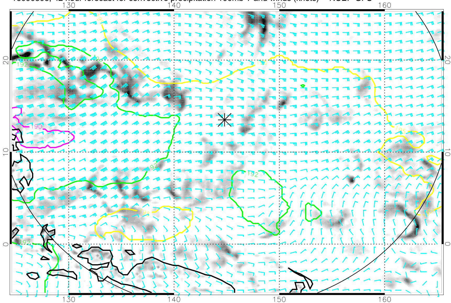
16090306, 42 hour forecast for convective precipitation 100mb T and winds (knots) -- NCEP GFS
