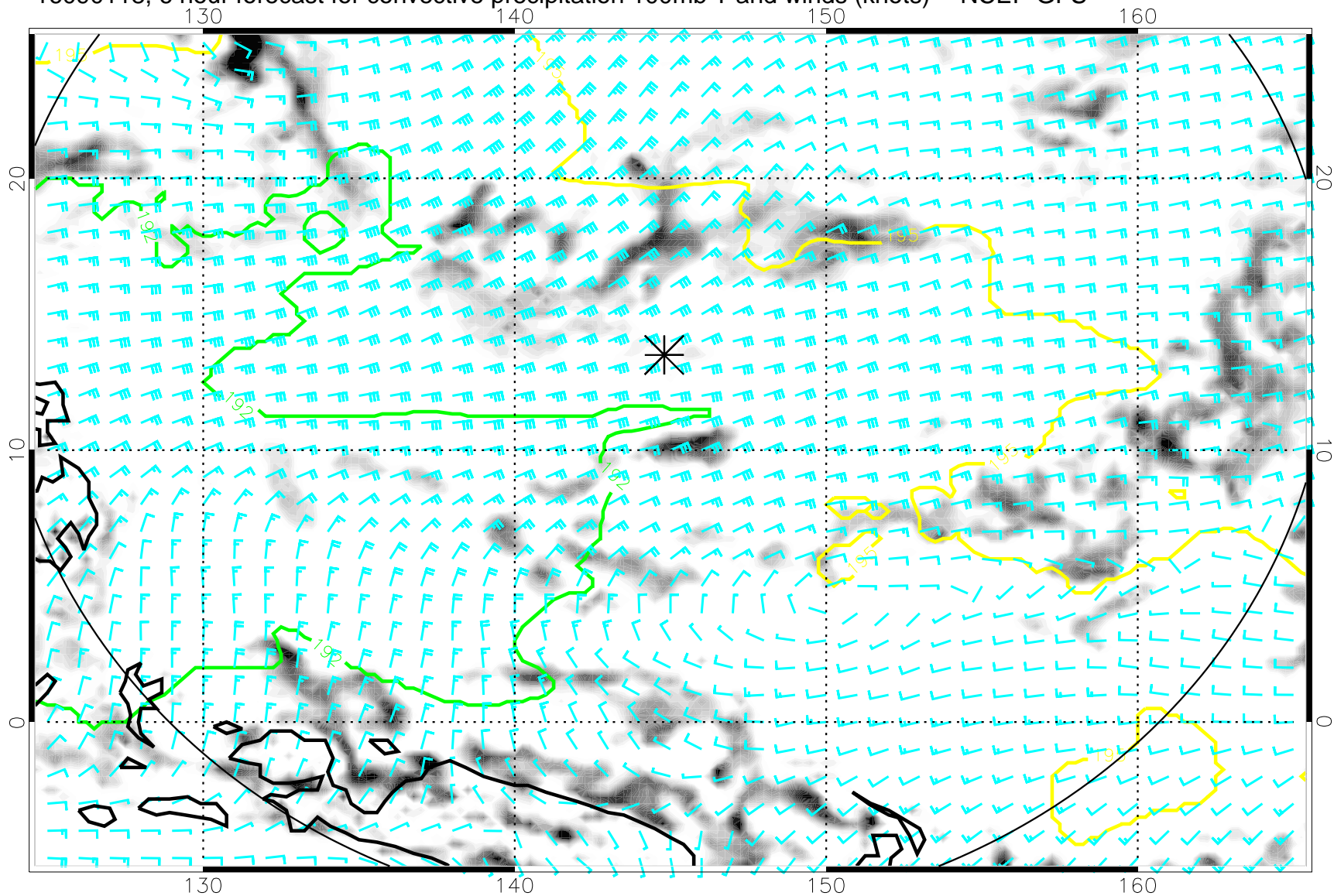
16090118, 6 hour forecast for convective precipitation 100mb T and winds (knots) -- NCEP GFS
