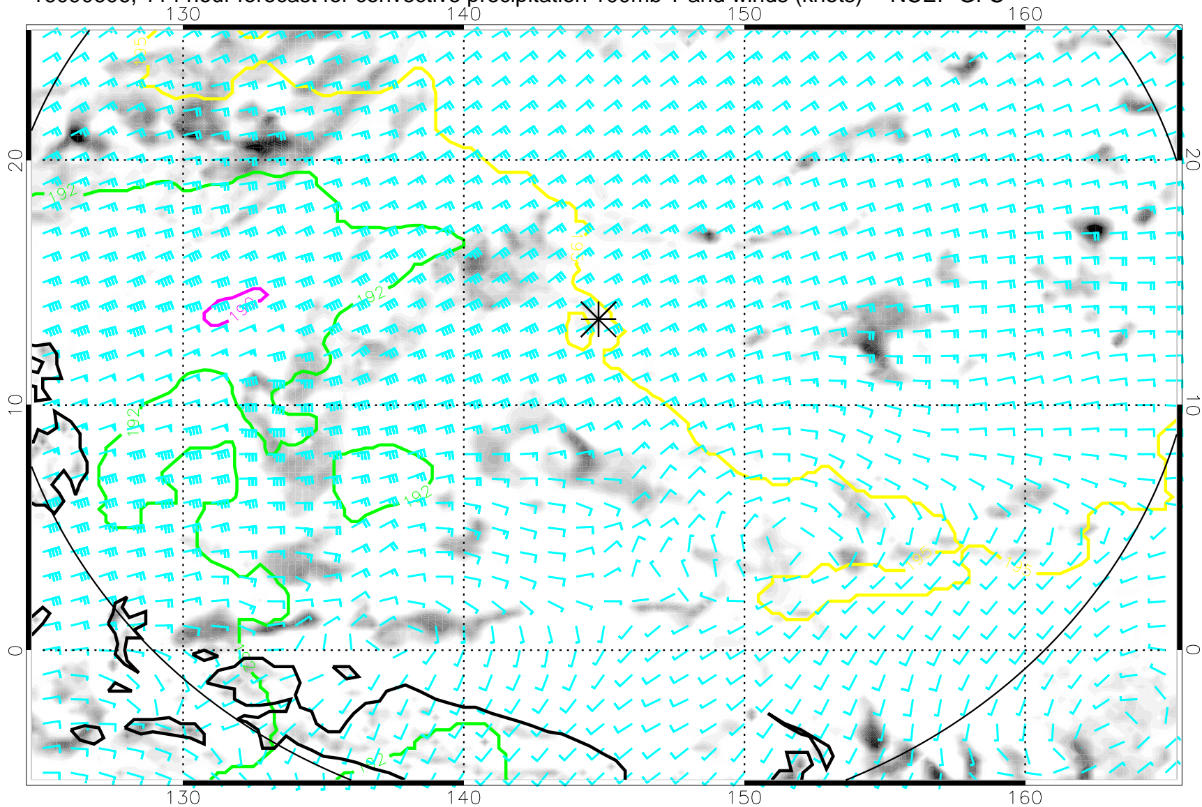
16090606, 114 hour forecast for convective precipitation 100mb T and winds (knots) -- NCEP GFS
