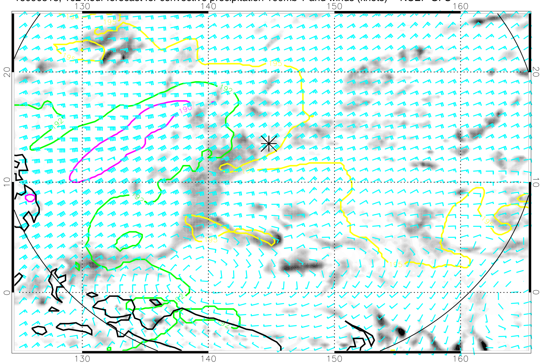
16090518, 102 hour forecast for convective precipitation 100mb T and winds (knots) -- NCEP GFS
