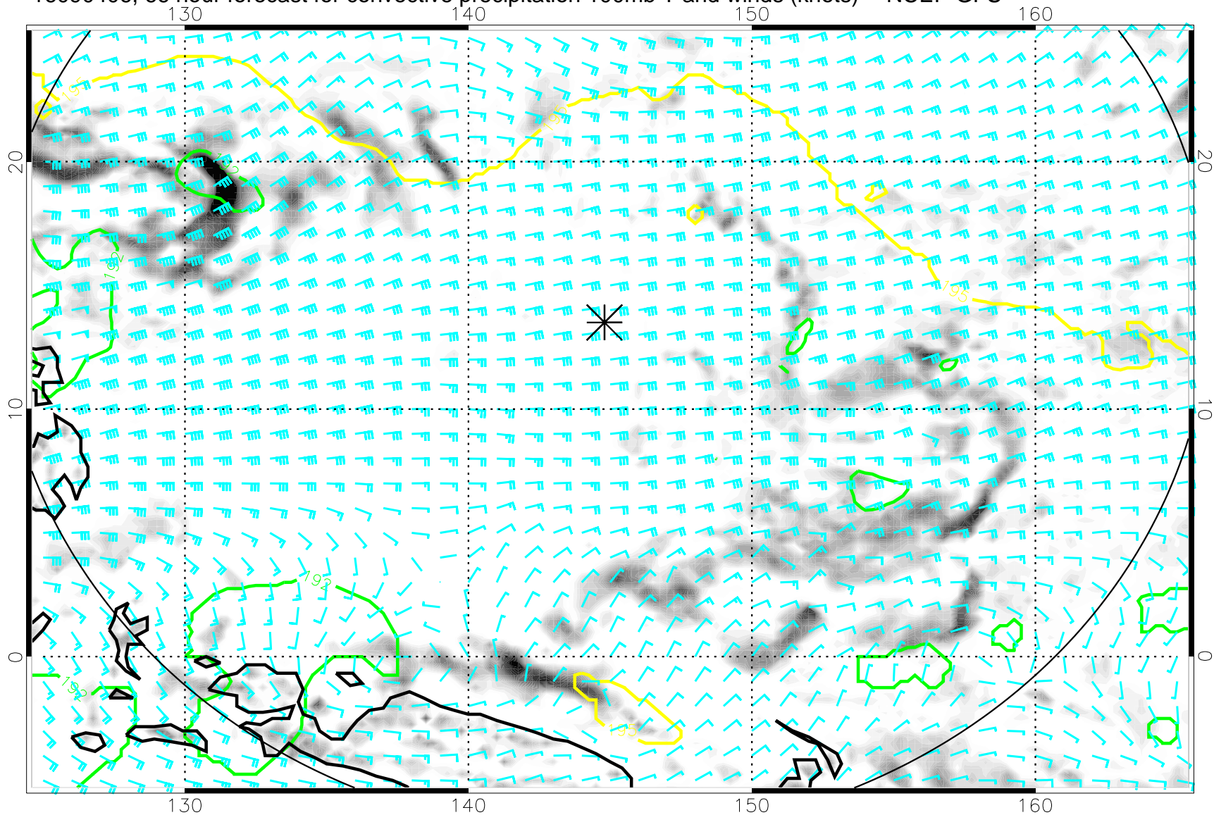
16090406, 66 hour forecast for convective precipitation 100mb T and winds (knots) -- NCEP GFS
