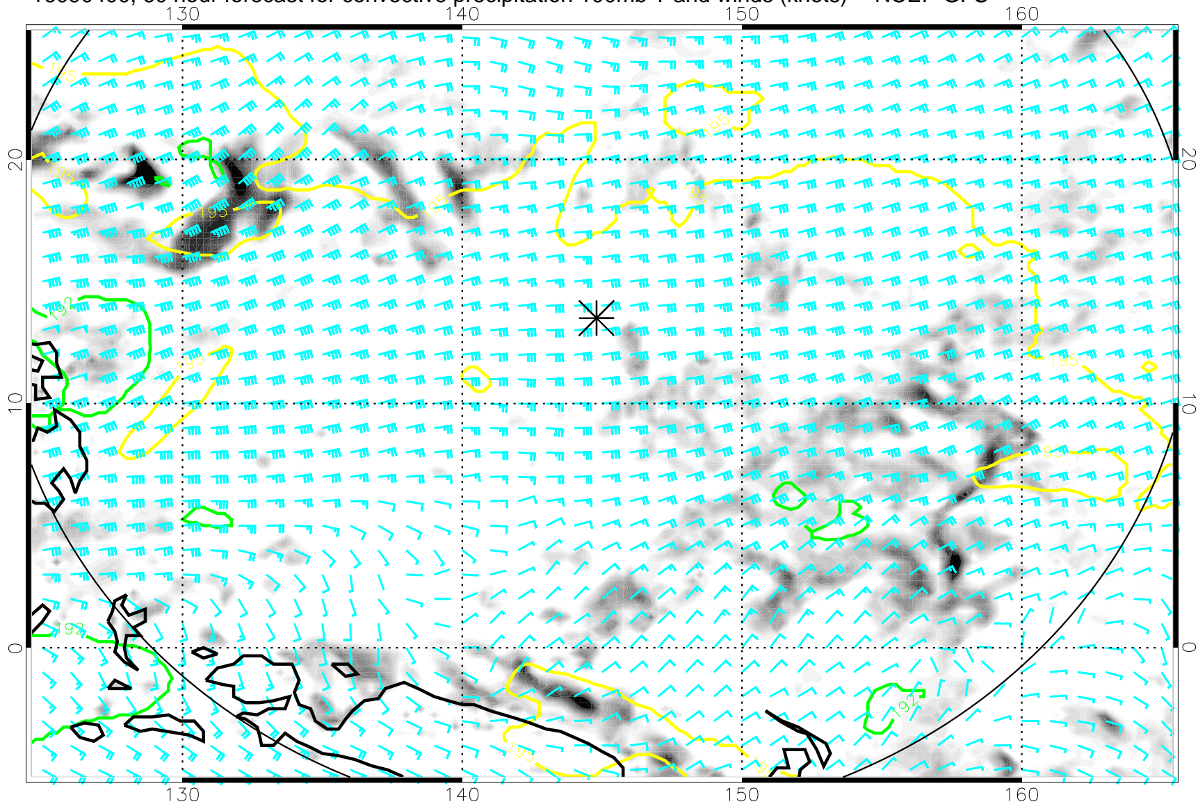
16090400, 60 hour forecast for convective precipitation 100mb T and winds (knots) -- NCEP GFS
