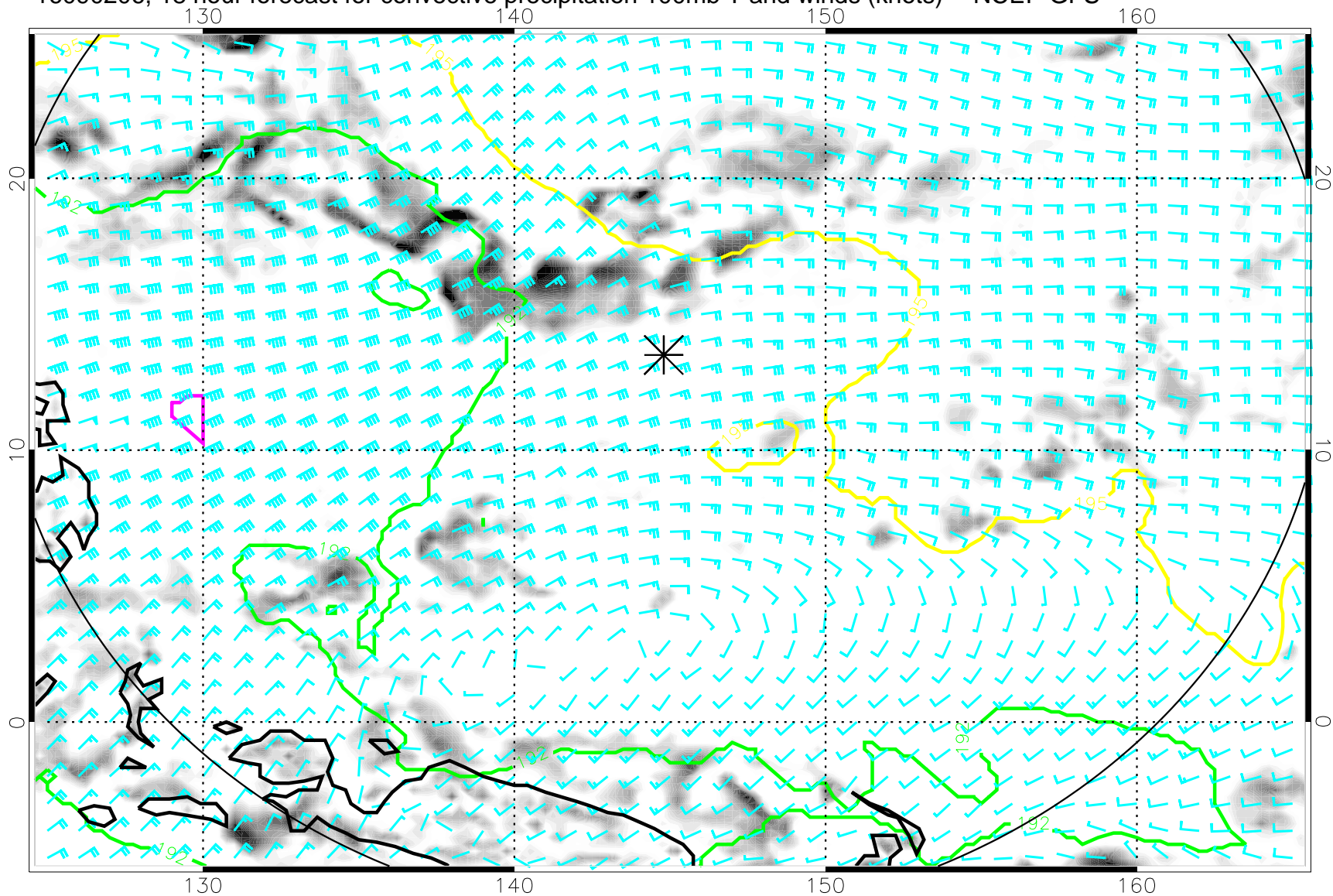
16090206, 18 hour forecast for convective precipitation 100mb T and winds (knots) -- NCEP GFS
