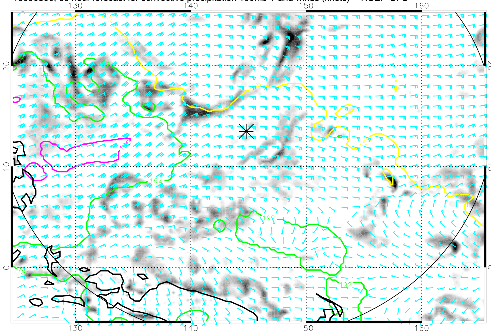
16090300, 36 hour forecast for convective precipitation 100mb T and winds (knots) -- NCEP GFS
