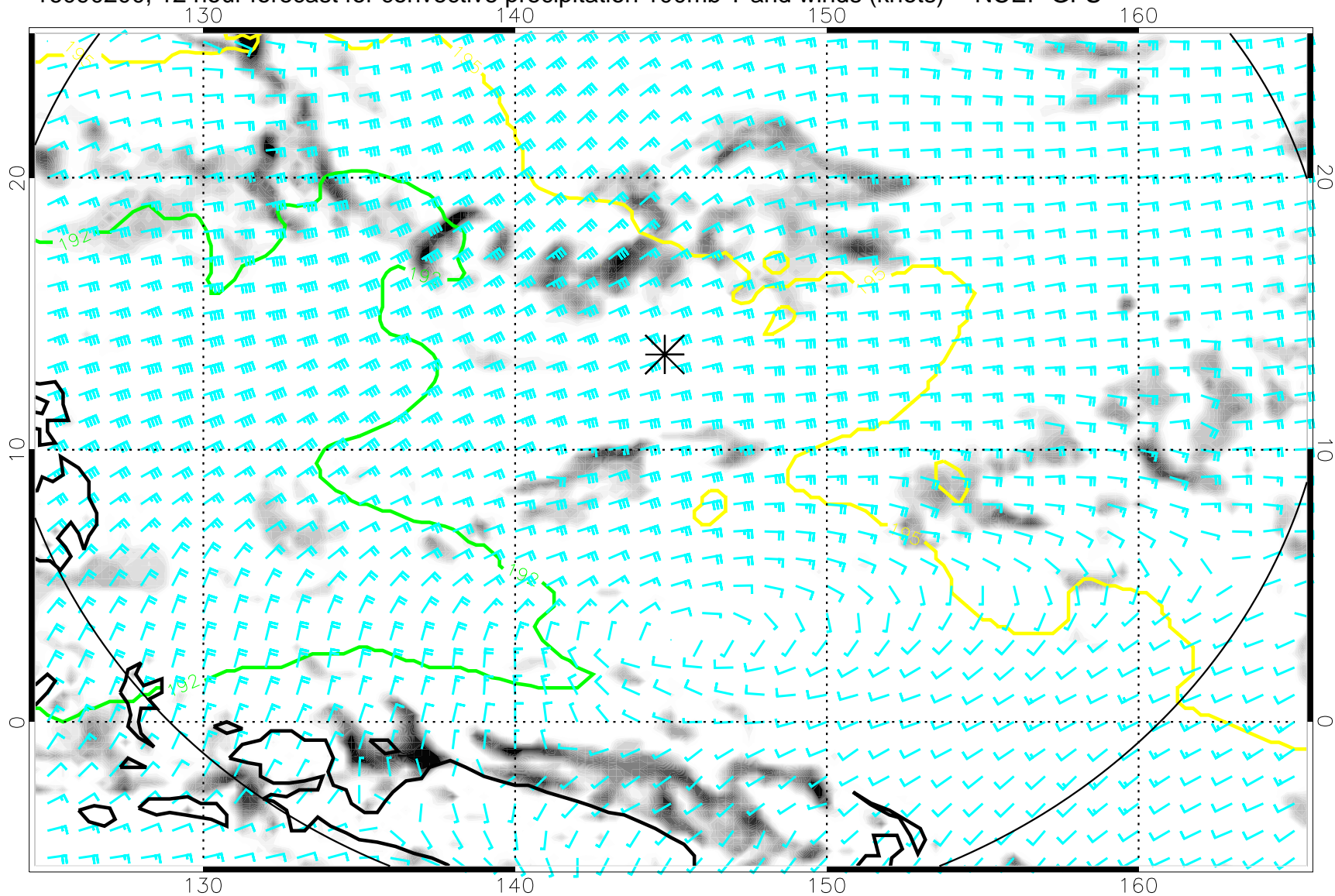
16090200, 12 hour forecast for convective precipitation 100mb T and winds (knots) -- NCEP GFS
