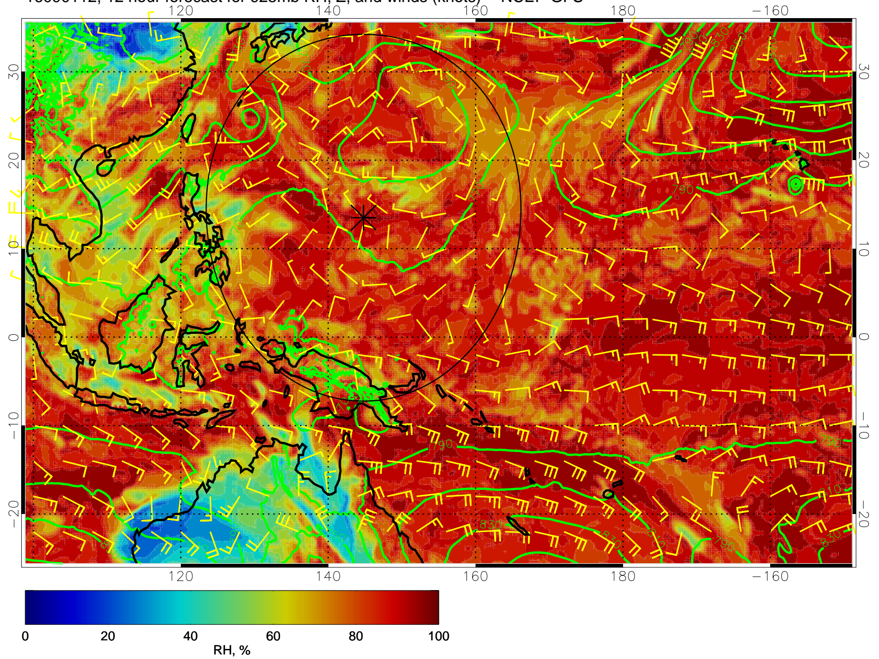
16090112, 12 hour forecast for 925mb RH, Z, and winds (knots) -- NCEP GFS
