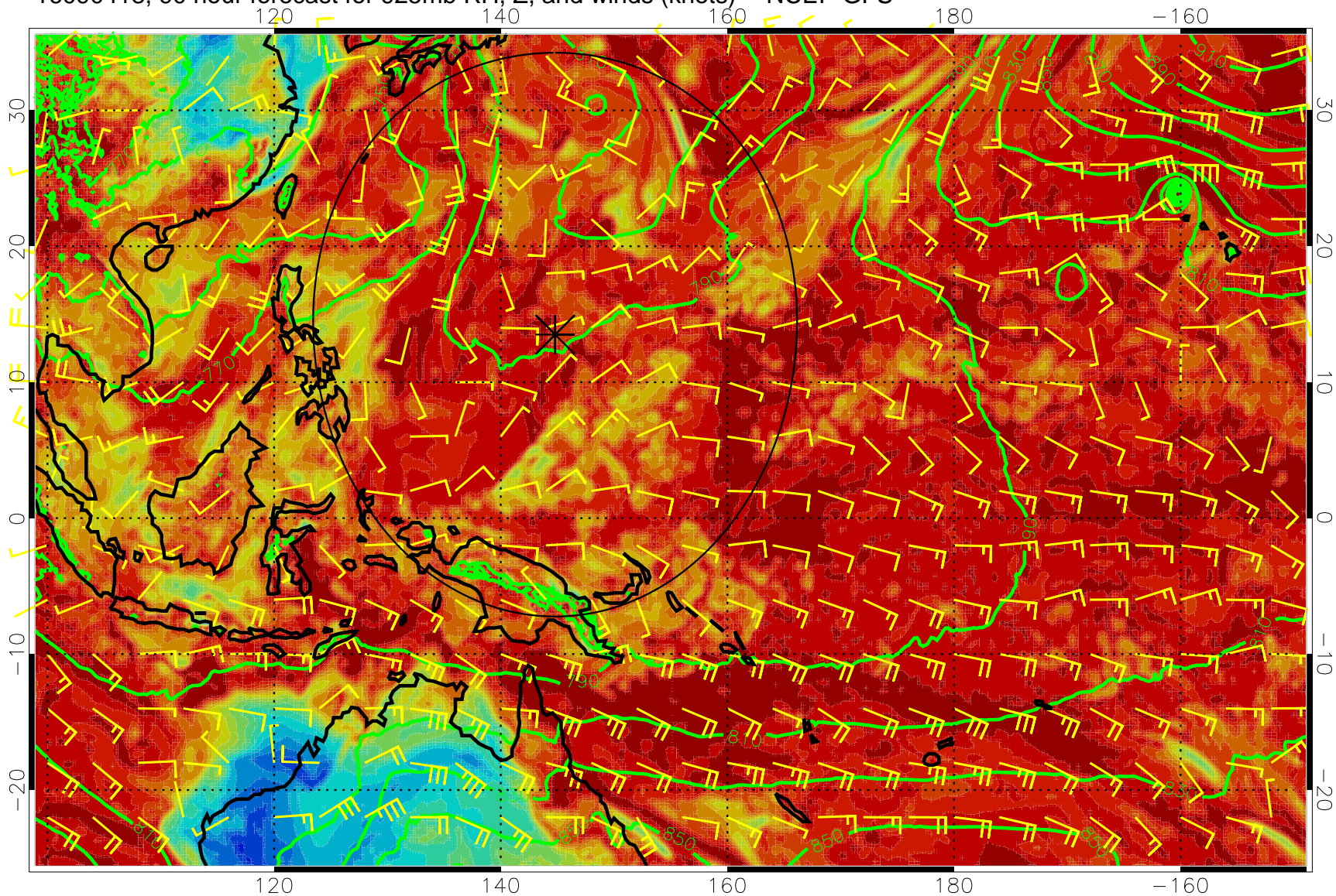
16090418, 90 hour forecast for 925mb RH, Z, and winds (knots) -- NCEP GFS
