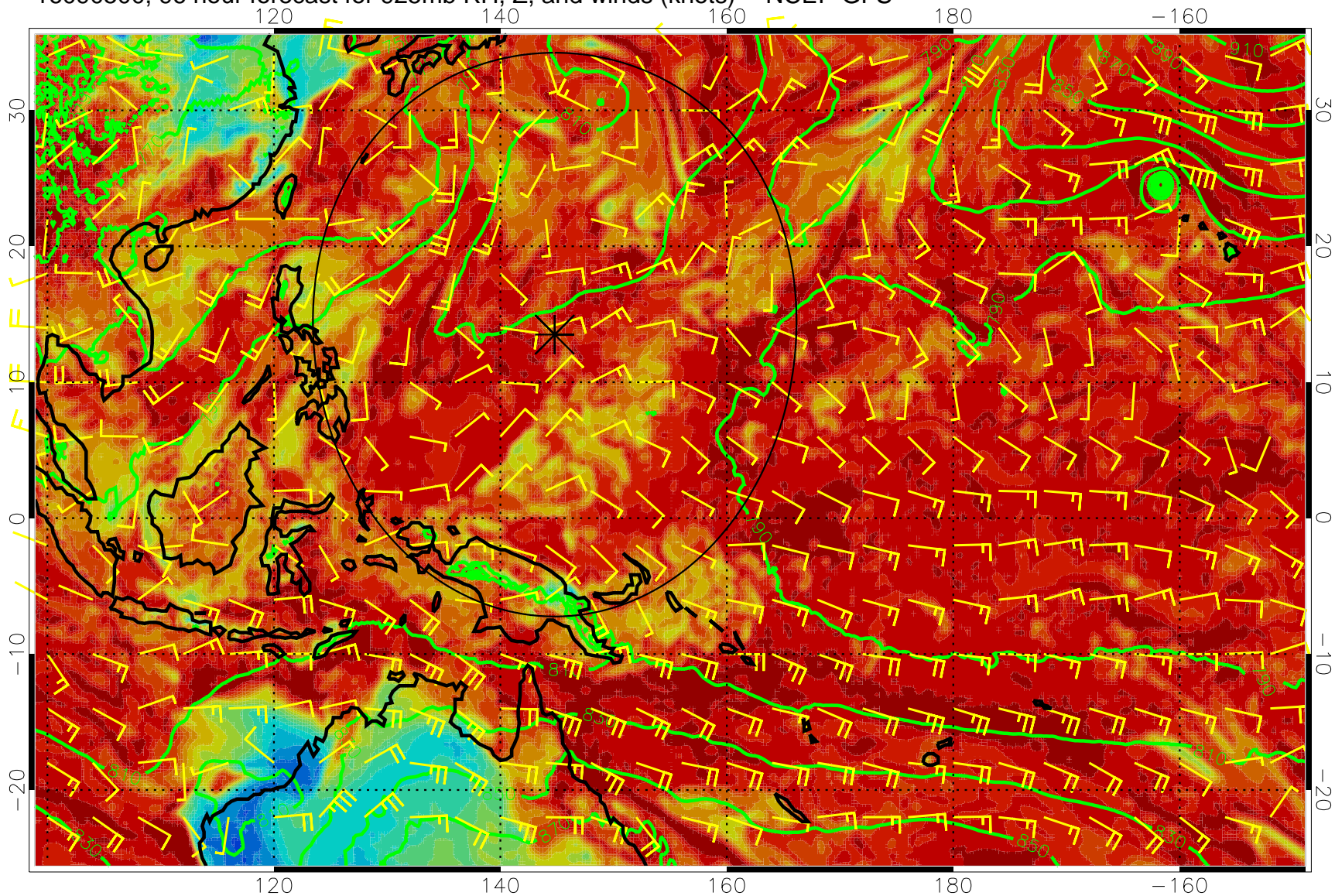
16090500, 96 hour forecast for 925mb RH, Z, and winds (knots) -- NCEP GFS
