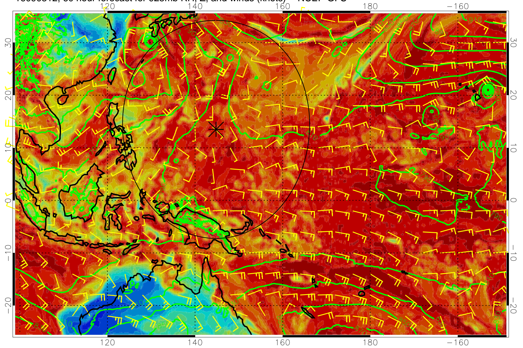
16090312, 60 hour forecast for 925mb RH, Z, and winds (knots) -- NCEP GFS
