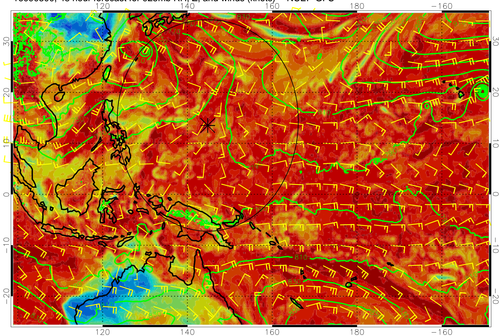
16090300, 48 hour forecast for 925mb RH, Z, and winds (knots) -- NCEP GFS
