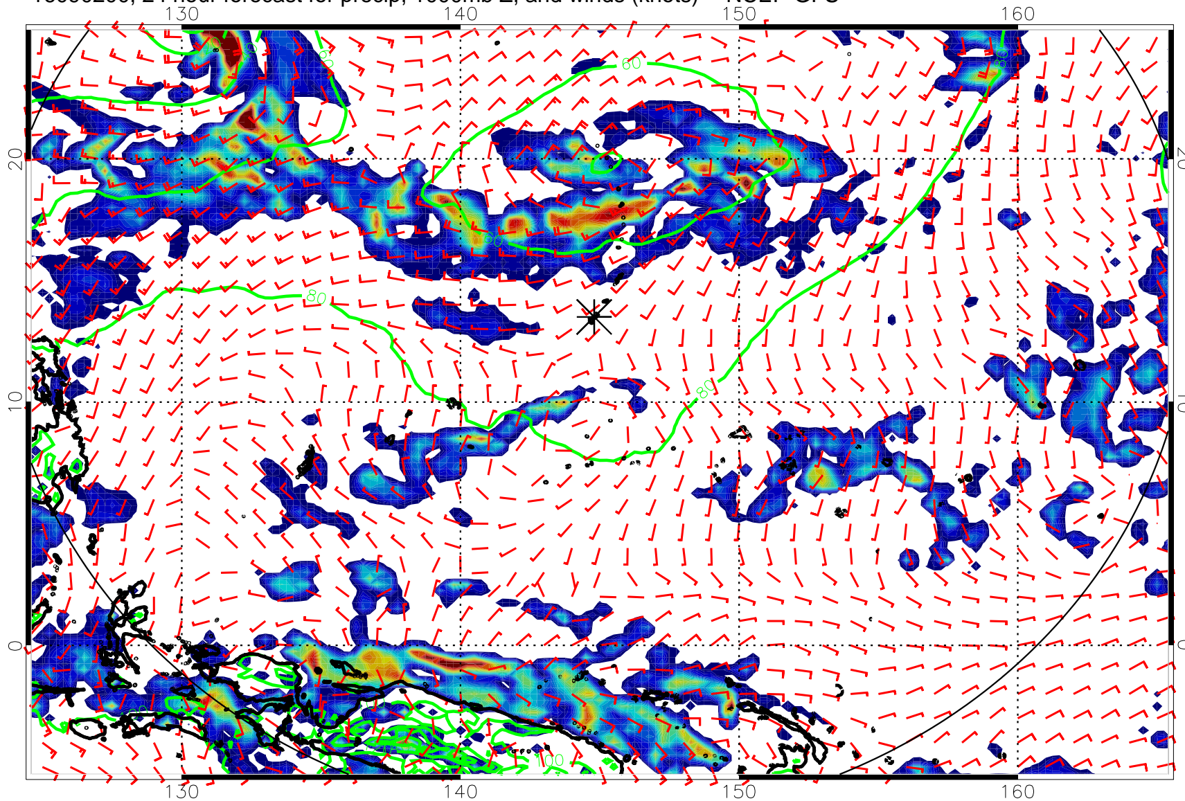
16090200, 24 hour forecast for precip, 1000mb Z, and winds (knots) -- NCEP GFS
