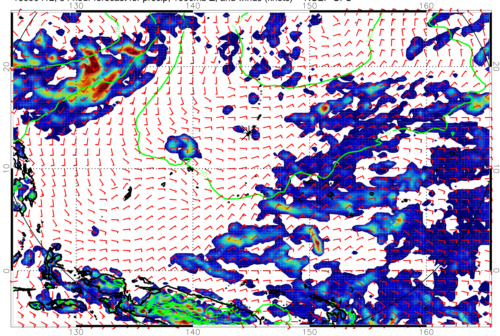
16090412, 84 hour forecast for precip, 1000mb Z, and winds (knots) -- NCEP GFS
