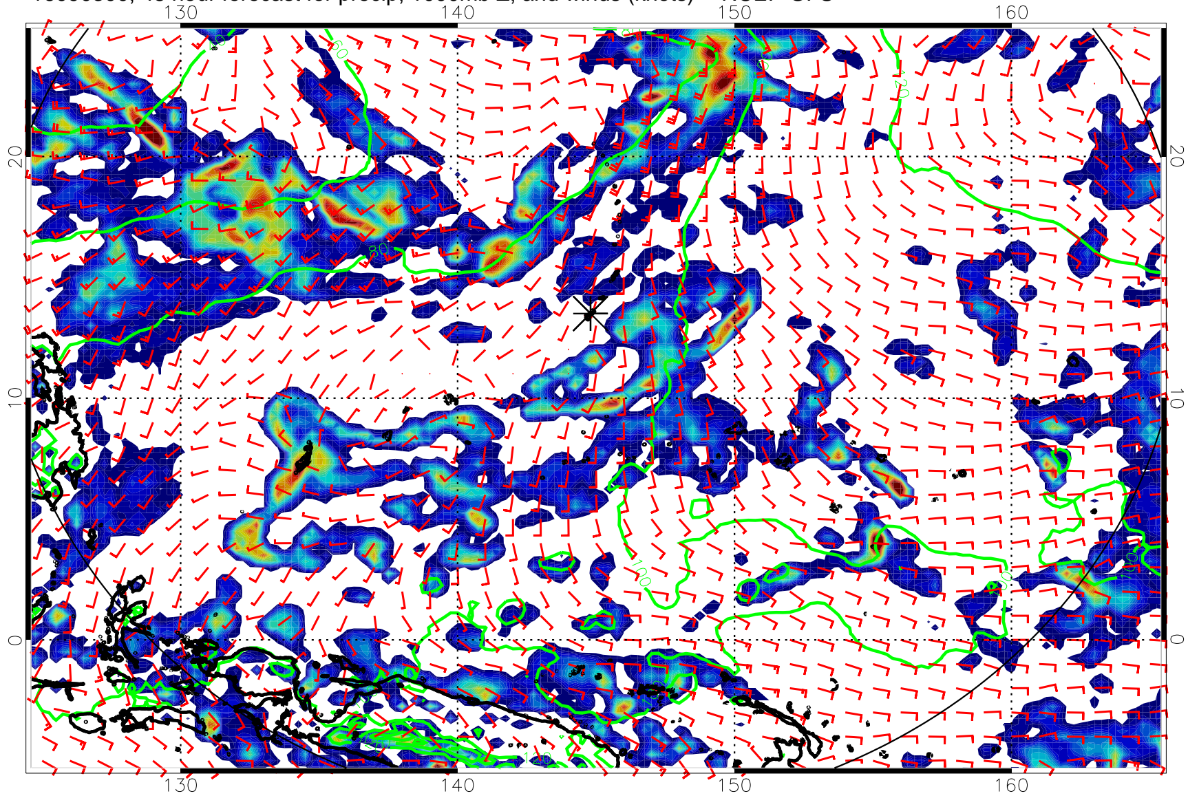
16090300, 48 hour forecast for precip, 1000mb Z, and winds (knots) -- NCEP GFS
