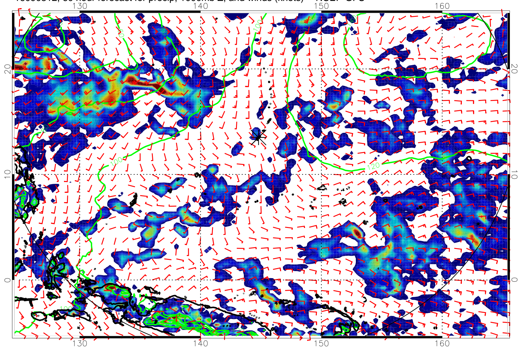
16090312, 60 hour forecast for precip, 1000mb Z, and winds (knots) -- NCEP GFS
