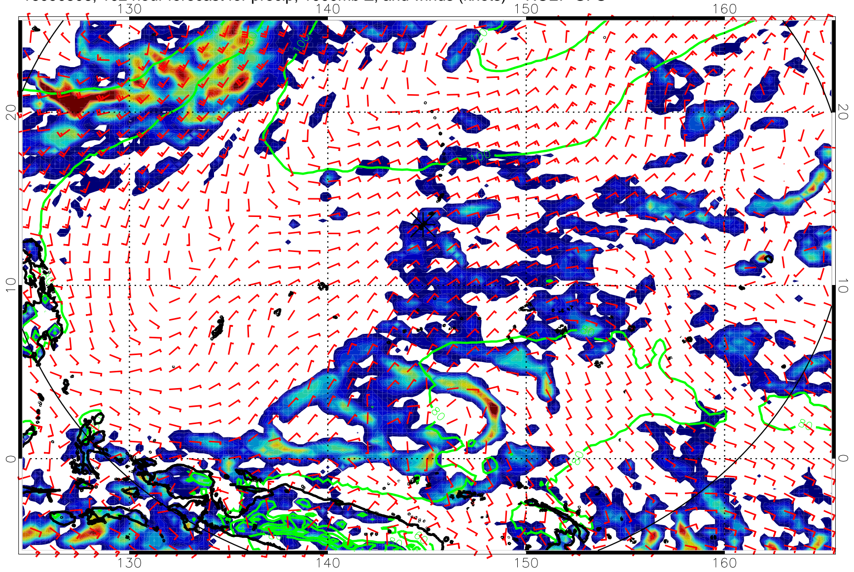
16090506, 102 hour forecast for precip, 1000mb Z, and winds (knots) -- NCEP GFS
