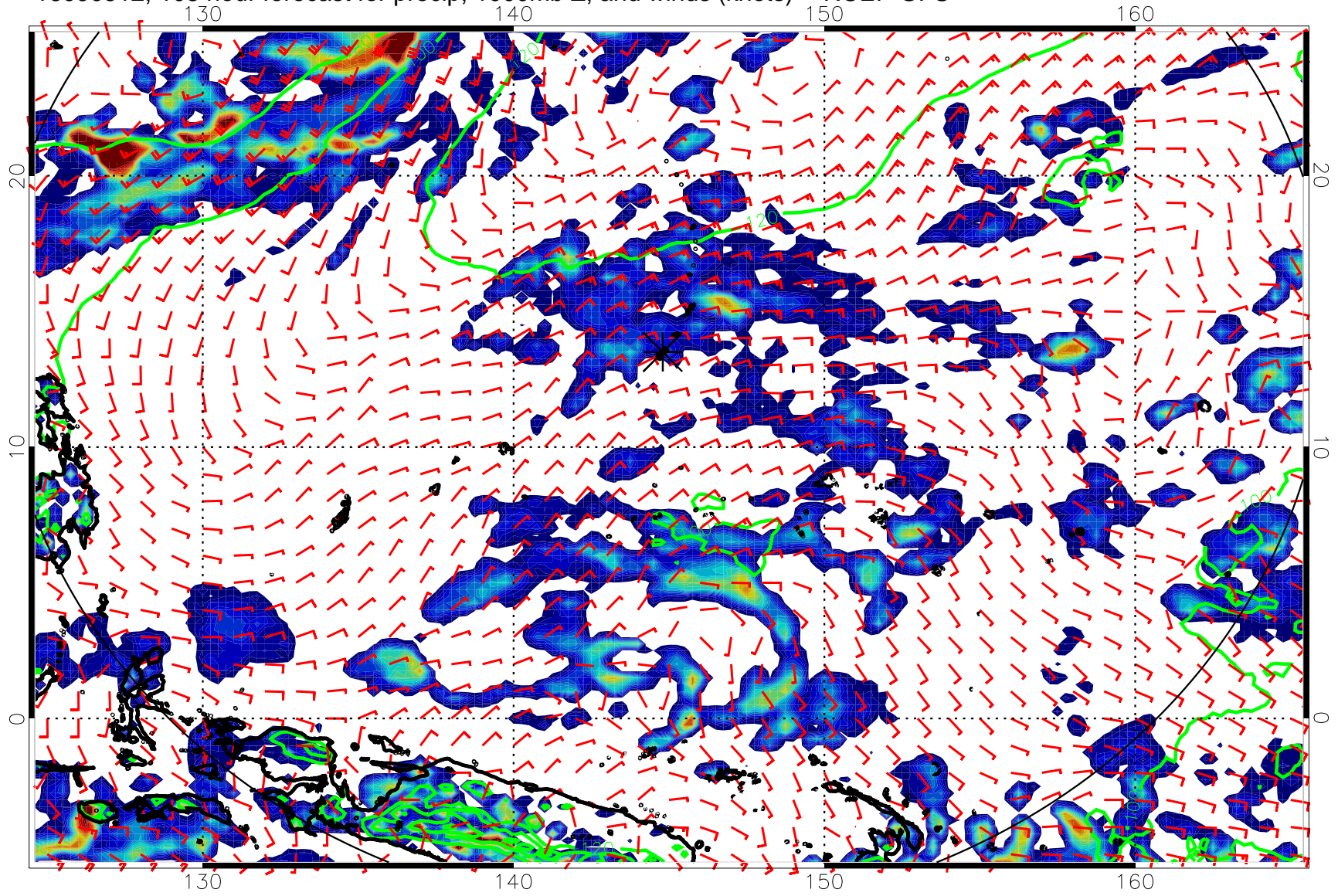
16090512, 108 hour forecast for precip, 1000mb Z, and winds (knots) -- NCEP GFS
