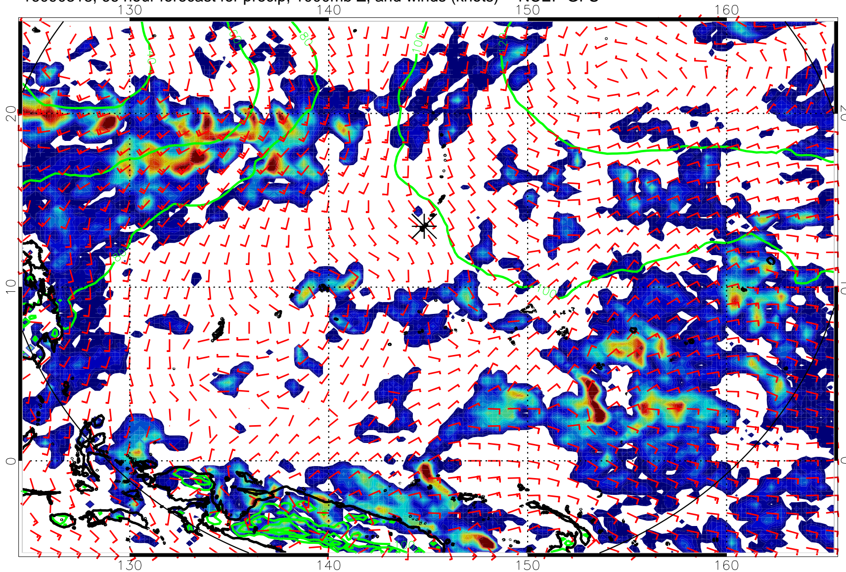
16090318, 66 hour forecast for precip, 1000mb Z, and winds (knots) -- NCEP GFS
