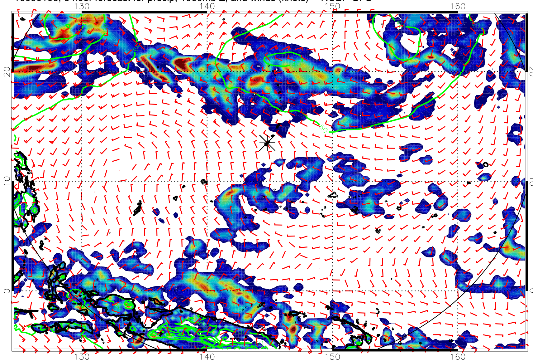
16090106, 6 hour forecast for precip, 1000mb Z, and winds (knots) -- NCEP GFS
