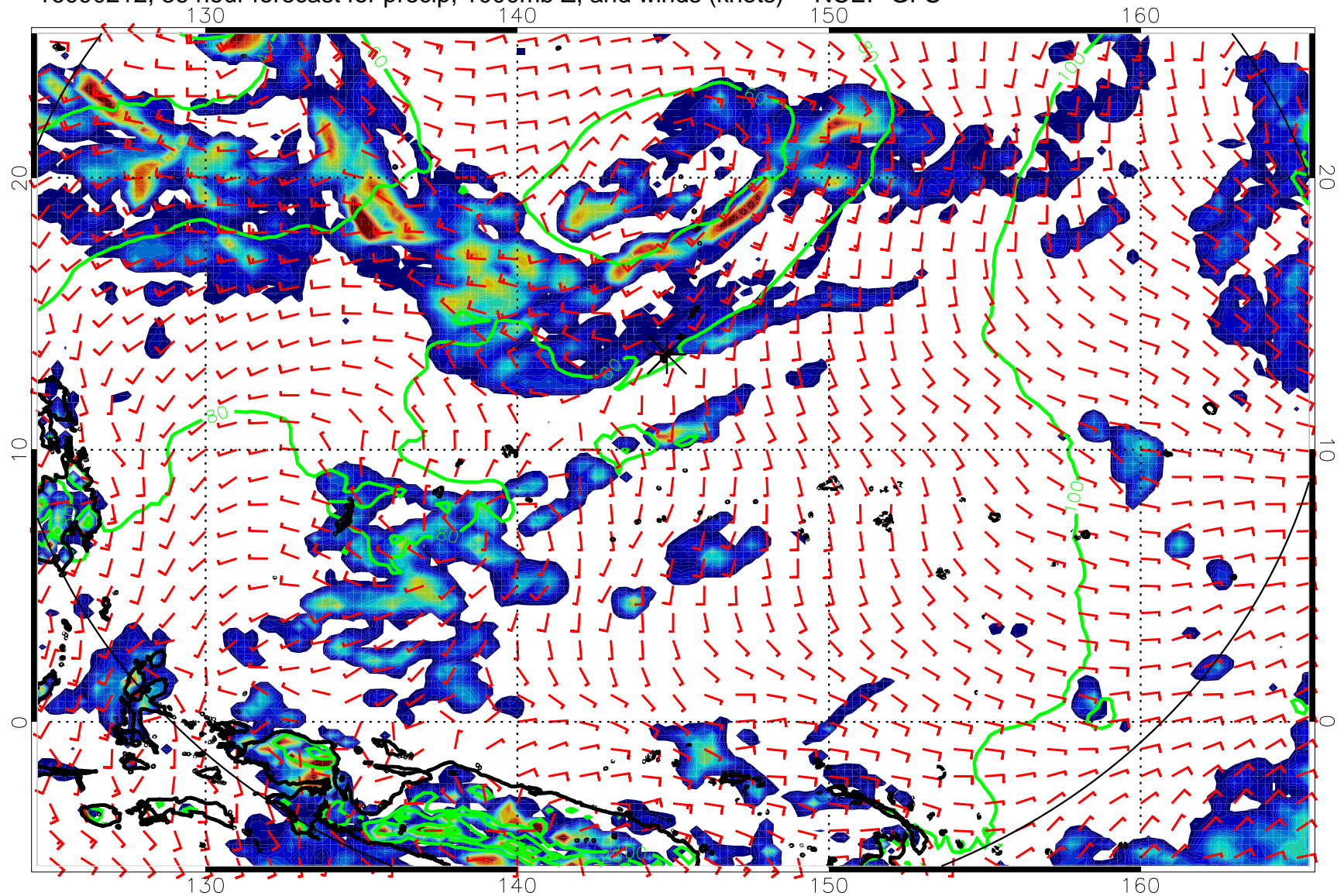
16090212, 36 hour forecast for precip, 1000mb Z, and winds (knots) -- NCEP GFS
