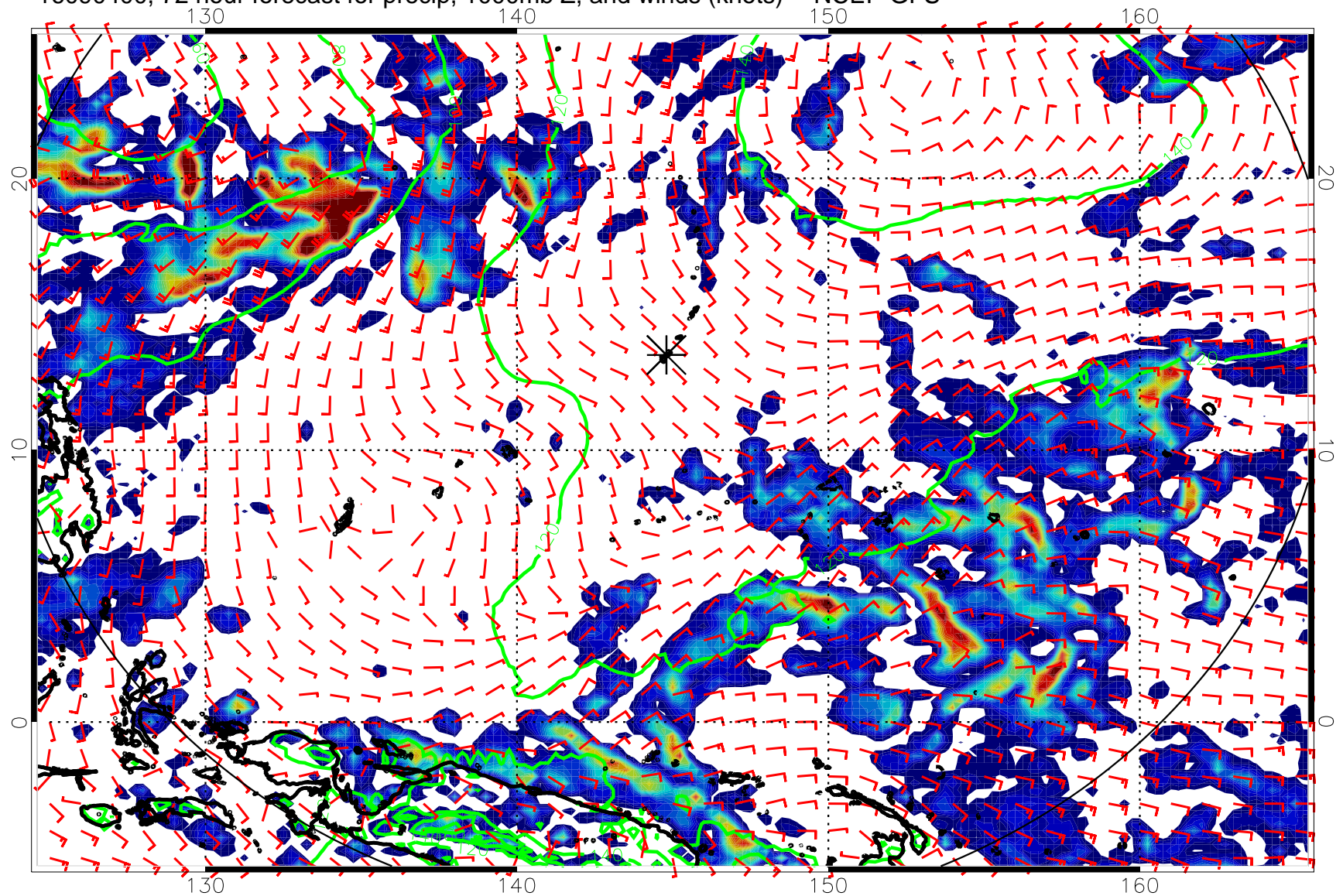
16090400, 72 hour forecast for precip, 1000mb Z, and winds (knots) -- NCEP GFS
