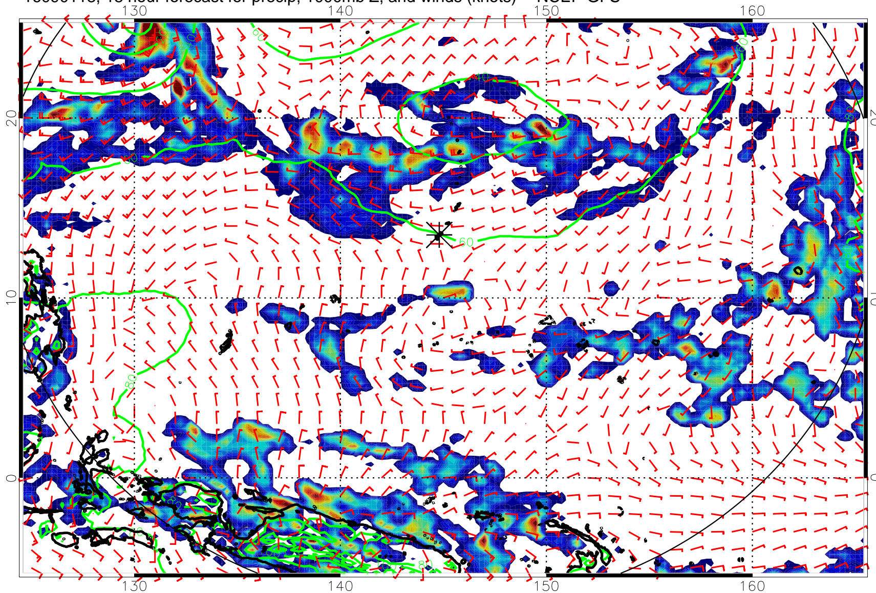
16090118, 18 hour forecast for precip, 1000mb Z, and winds (knots) -- NCEP GFS
