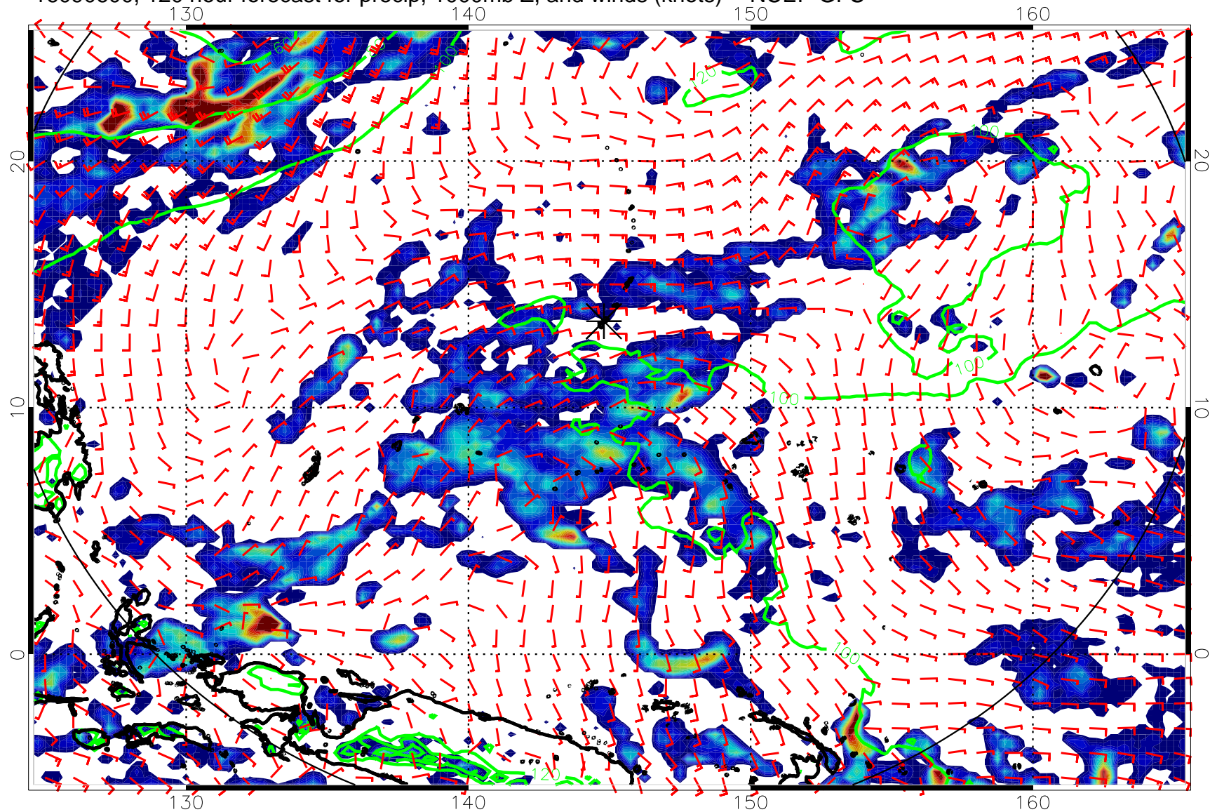
16090600, 120 hour forecast for precip, 1000mb Z, and winds (knots) -- NCEP GFS
