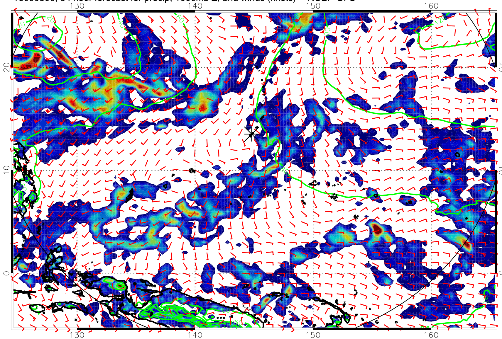
16090306, 54 hour forecast for precip, 1000mb Z, and winds (knots) -- NCEP GFS
