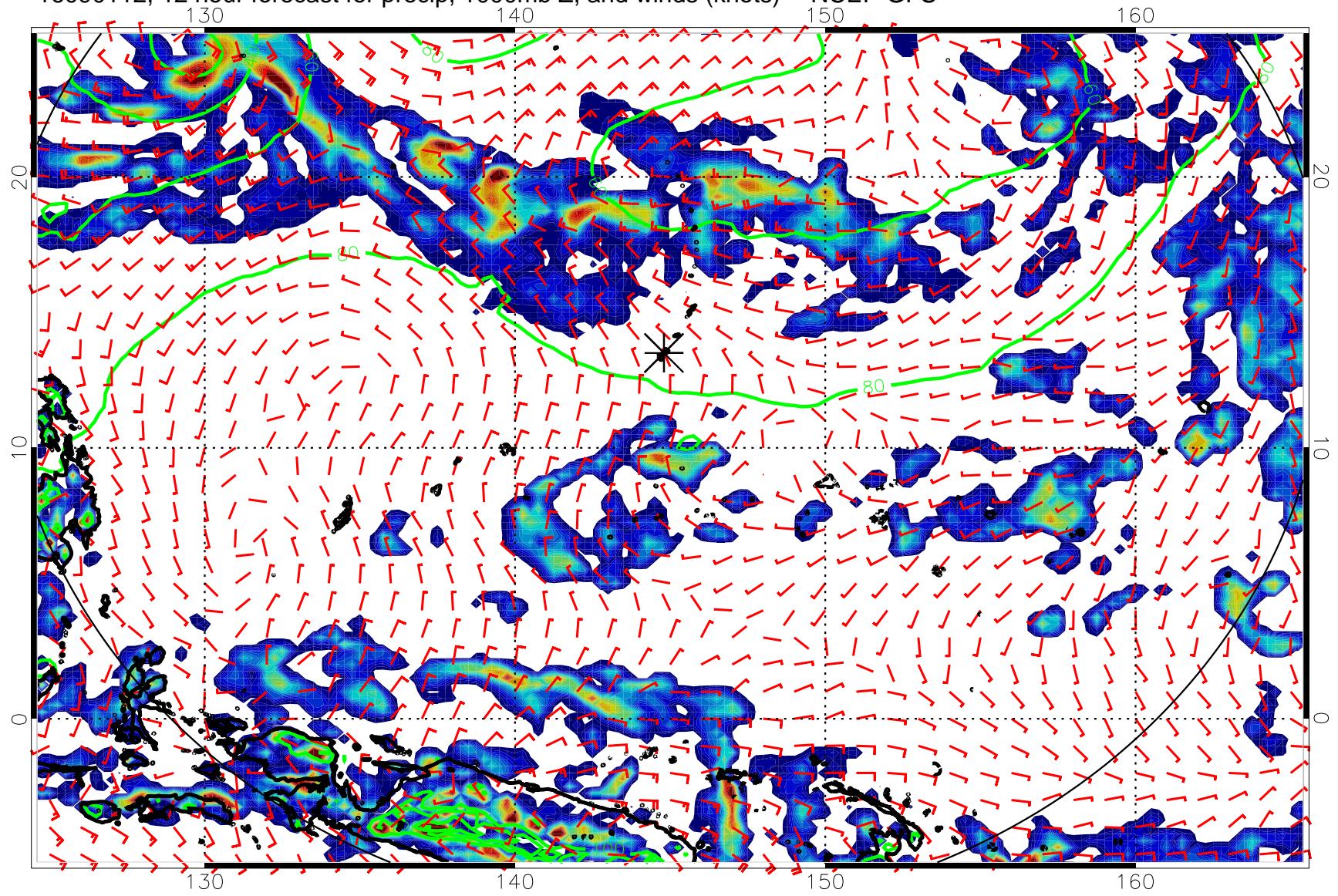
16090112, 12 hour forecast for precip, 1000mb Z, and winds (knots) -- NCEP GFS
