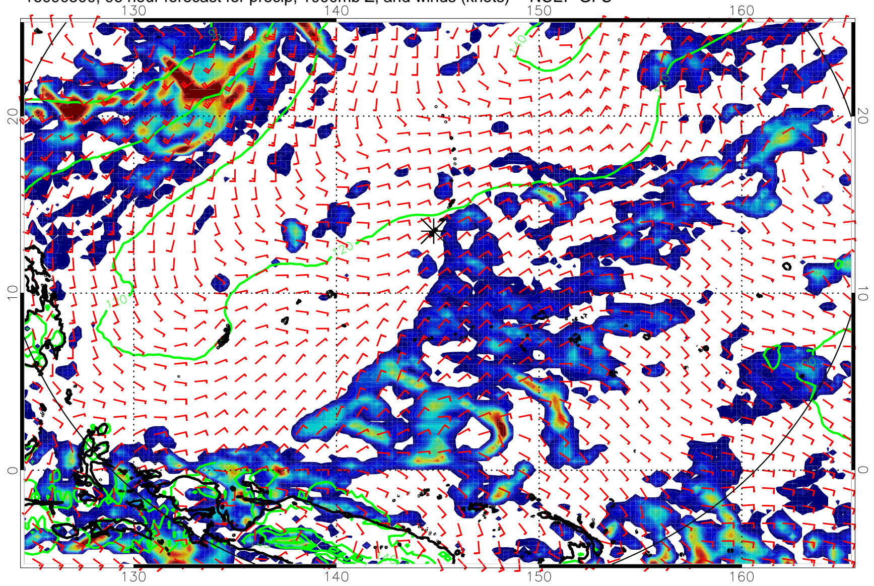
16090500, 96 hour forecast for precip, 1000mb Z, and winds (knots) -- NCEP GFS
