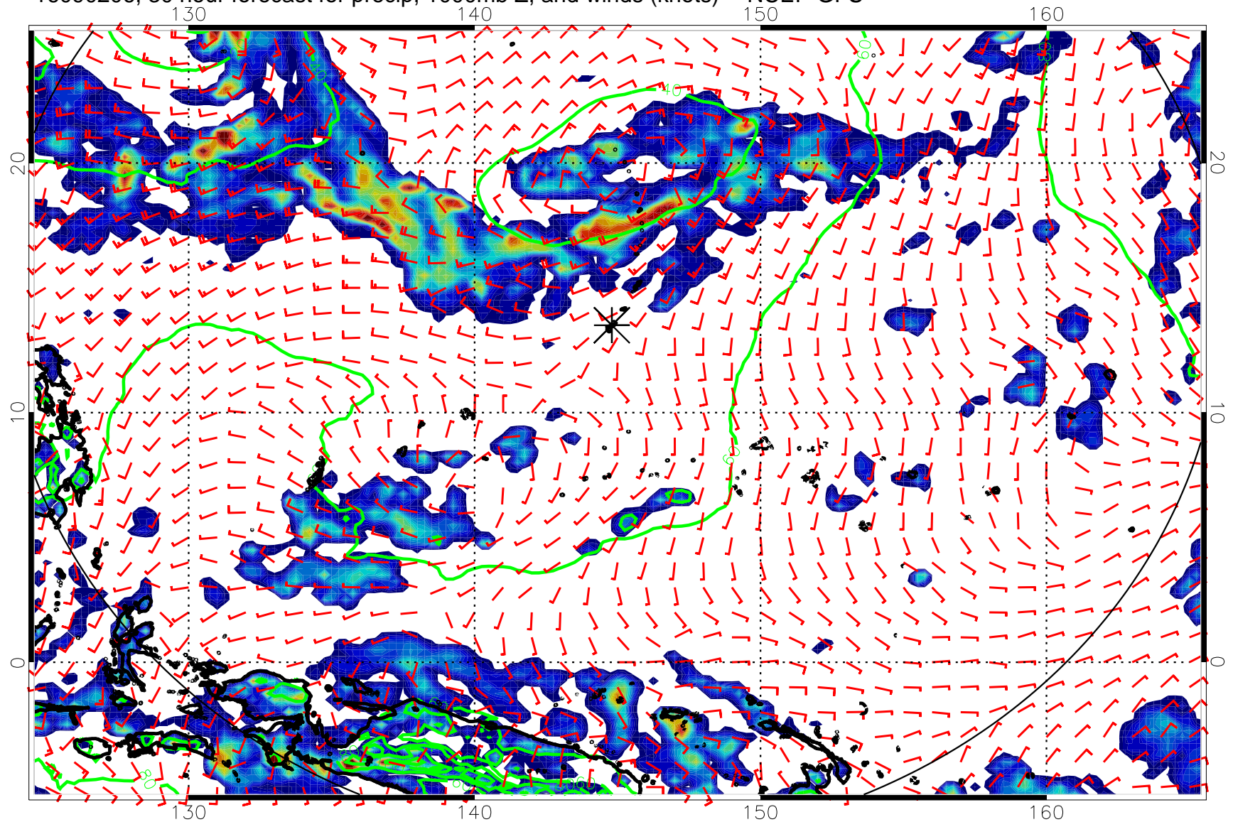
16090206, 30 hour forecast for precip, 1000mb Z, and winds (knots) -- NCEP GFS
