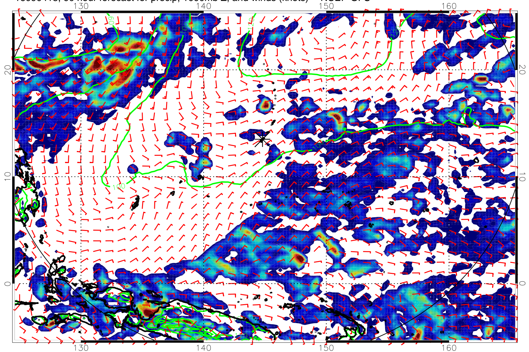
16090418, 90 hour forecast for precip, 1000mb Z, and winds (knots) -- NCEP GFS
