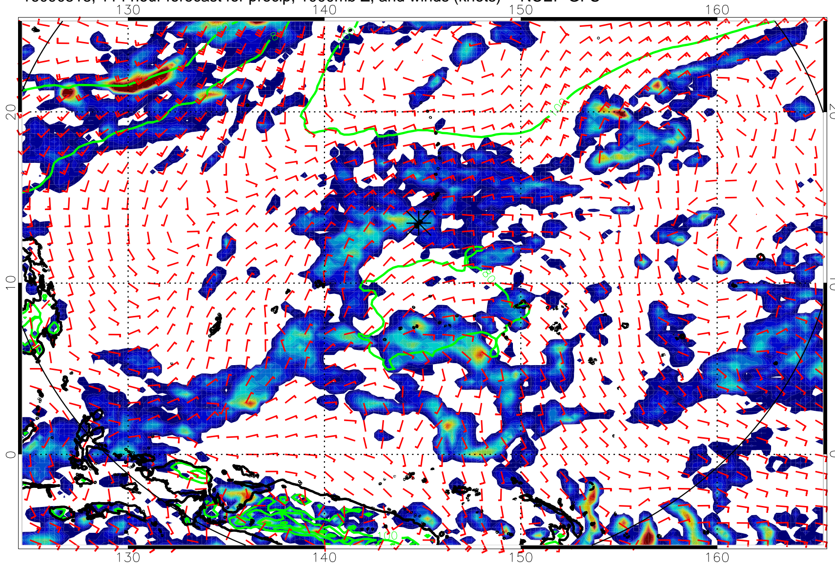
16090518, 114 hour forecast for precip, 1000mb Z, and winds (knots) -- NCEP GFS
