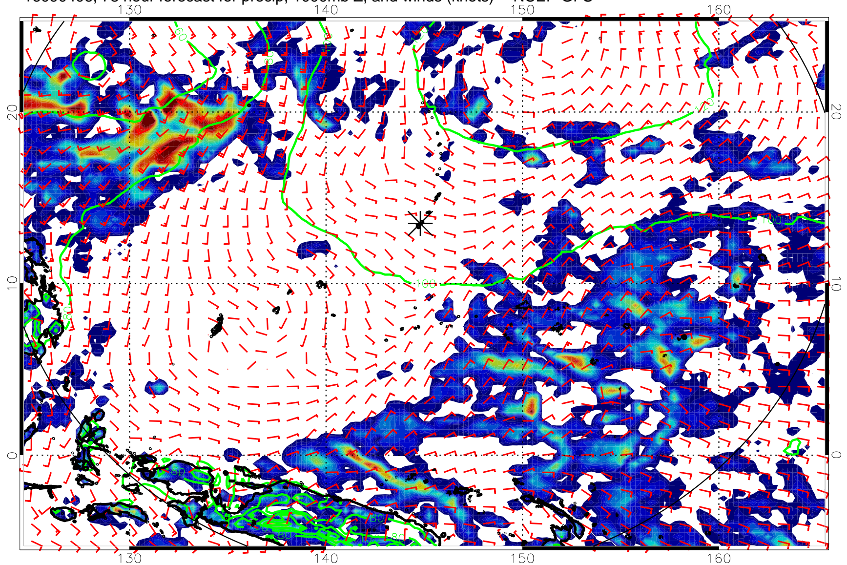
16090406, 78 hour forecast for precip, 1000mb Z, and winds (knots) -- NCEP GFS
