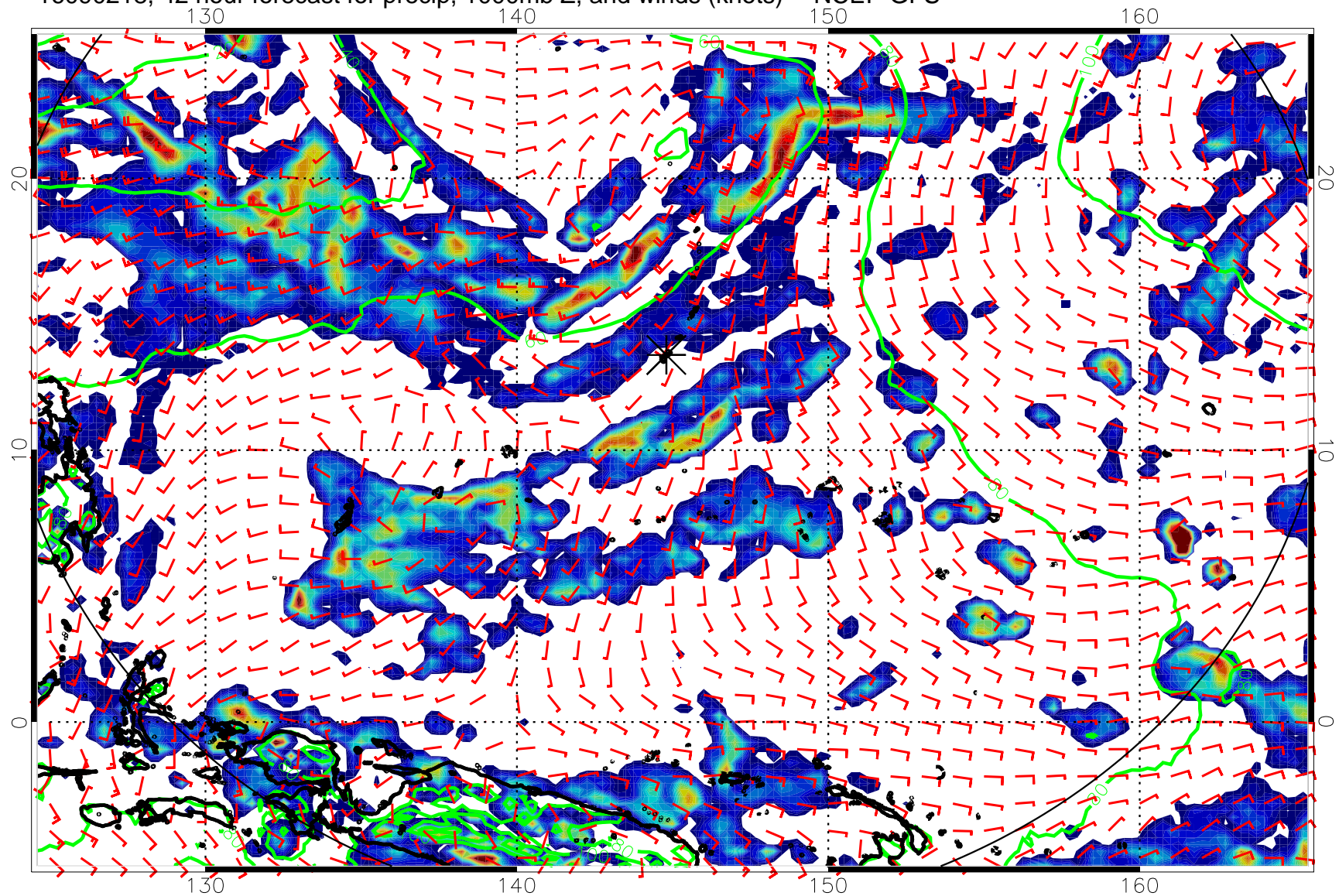
16090218, 42 hour forecast for precip, 1000mb Z, and winds (knots) -- NCEP GFS
