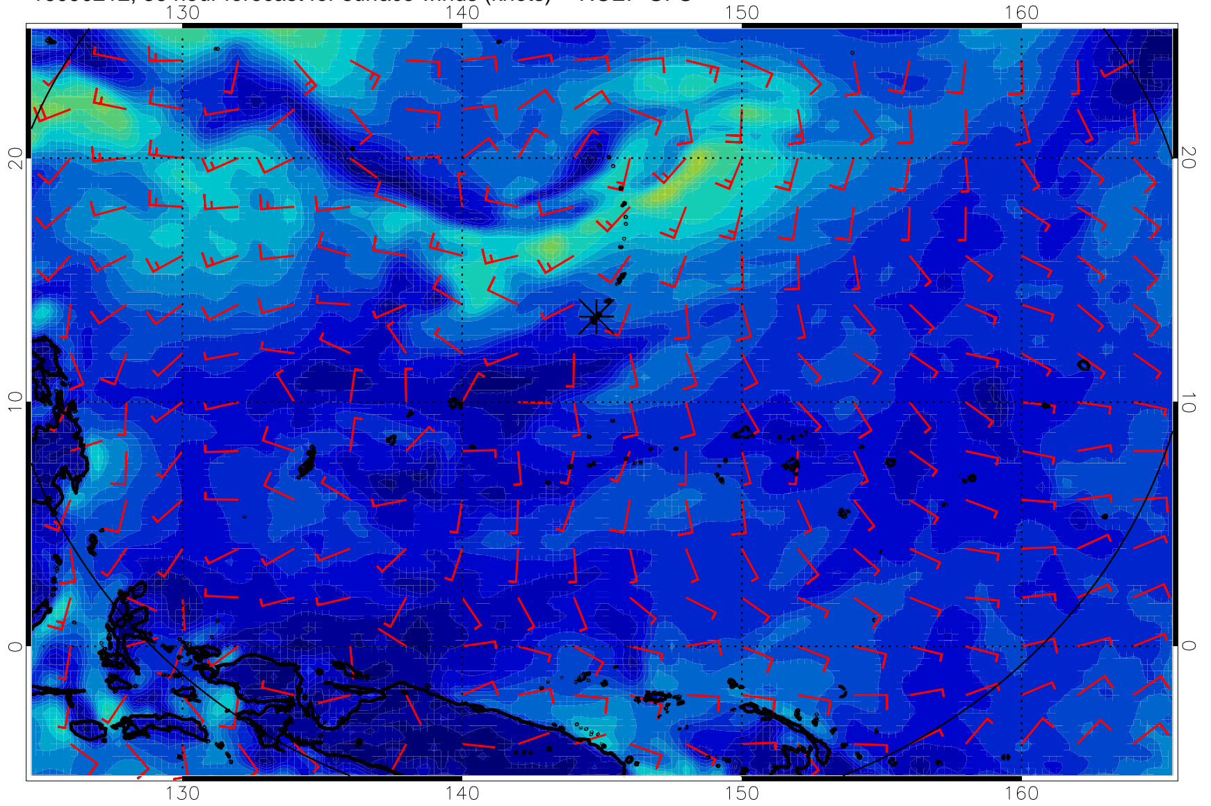
16090212, 36 hour forecast for surface winds (knots) -- NCEP GFS
