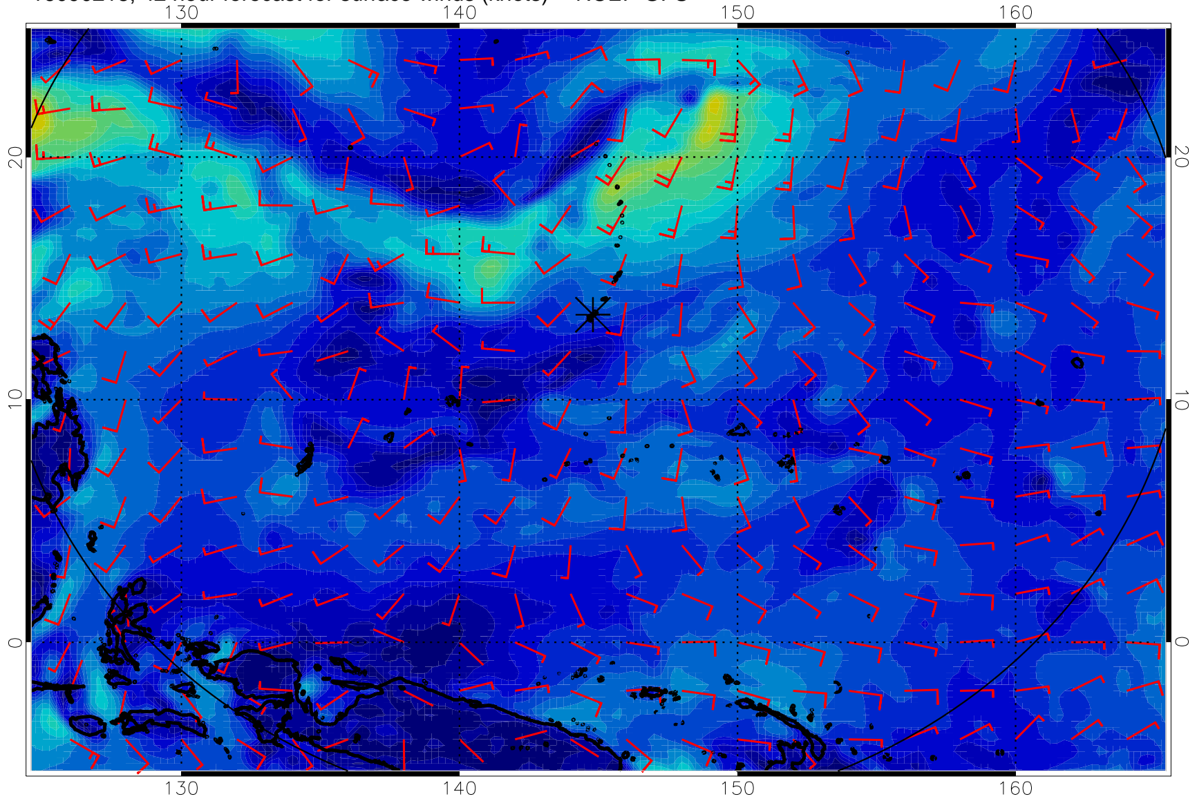
16090218, 42 hour forecast for surface winds (knots) -- NCEP GFS
