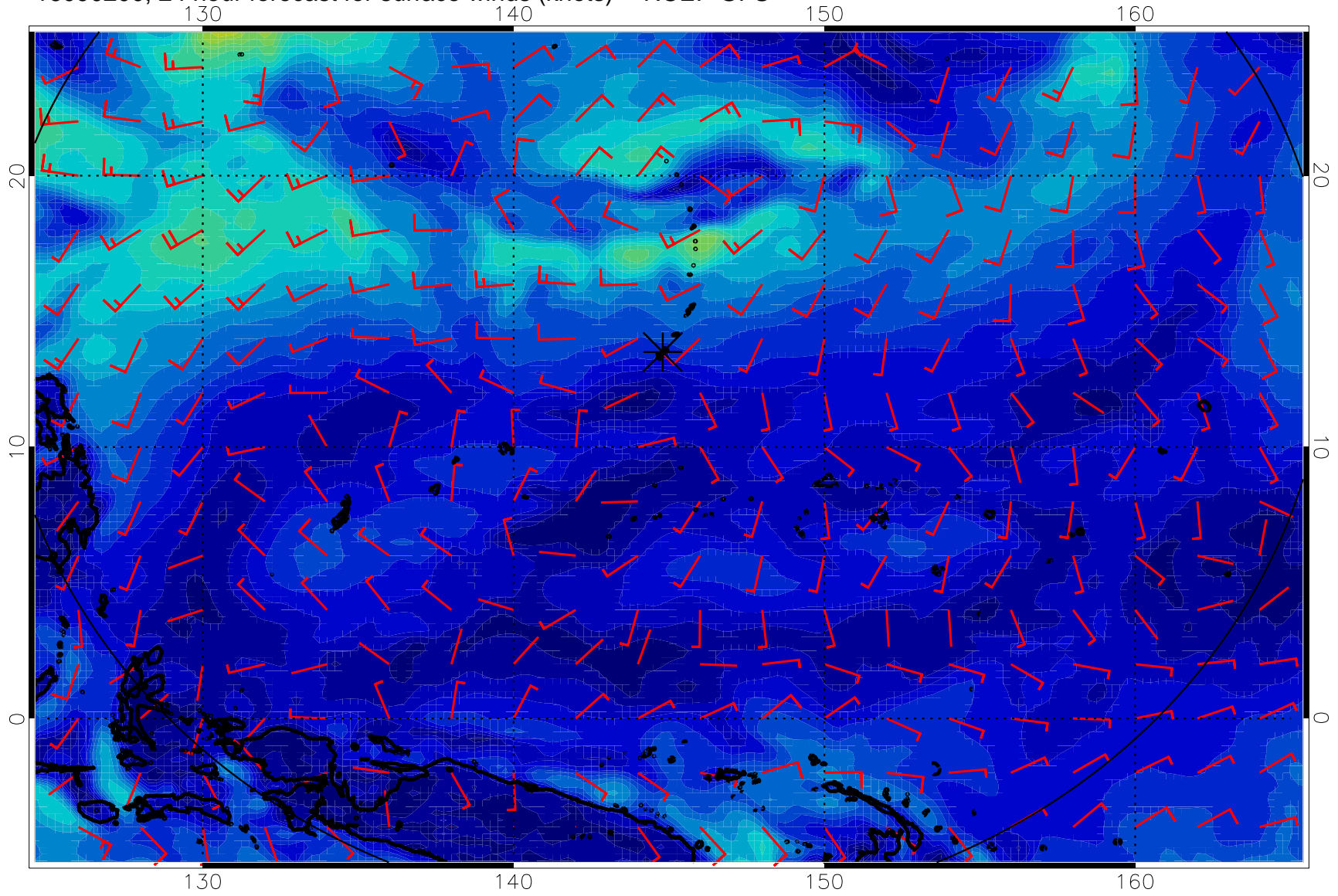
16090200, 24 hour forecast for surface winds (knots) -- NCEP GFS
