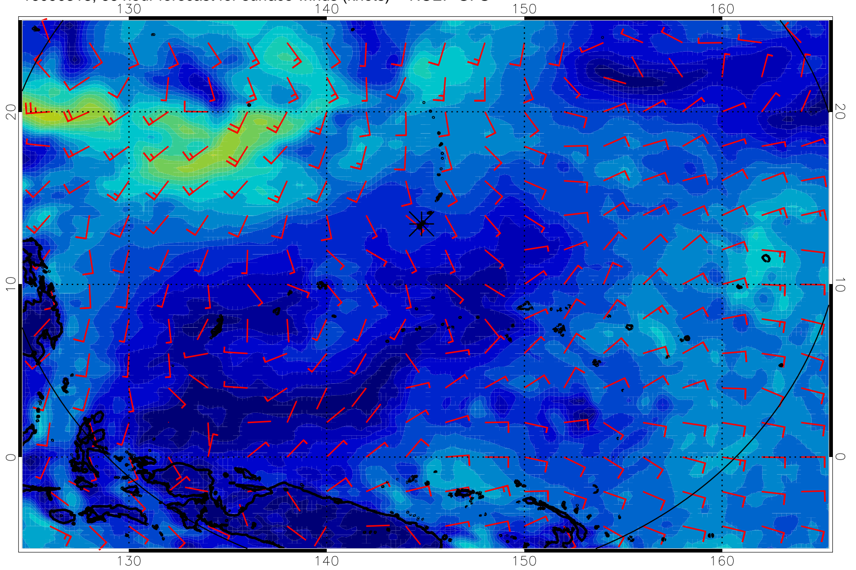
16090318, 66 hour forecast for surface winds (knots) -- NCEP GFS
