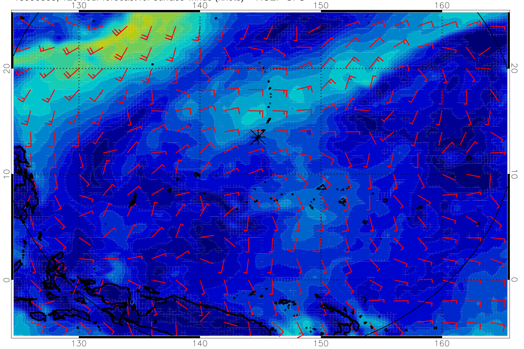
16090600, 120 hour forecast for surface winds (knots) -- NCEP GFS
