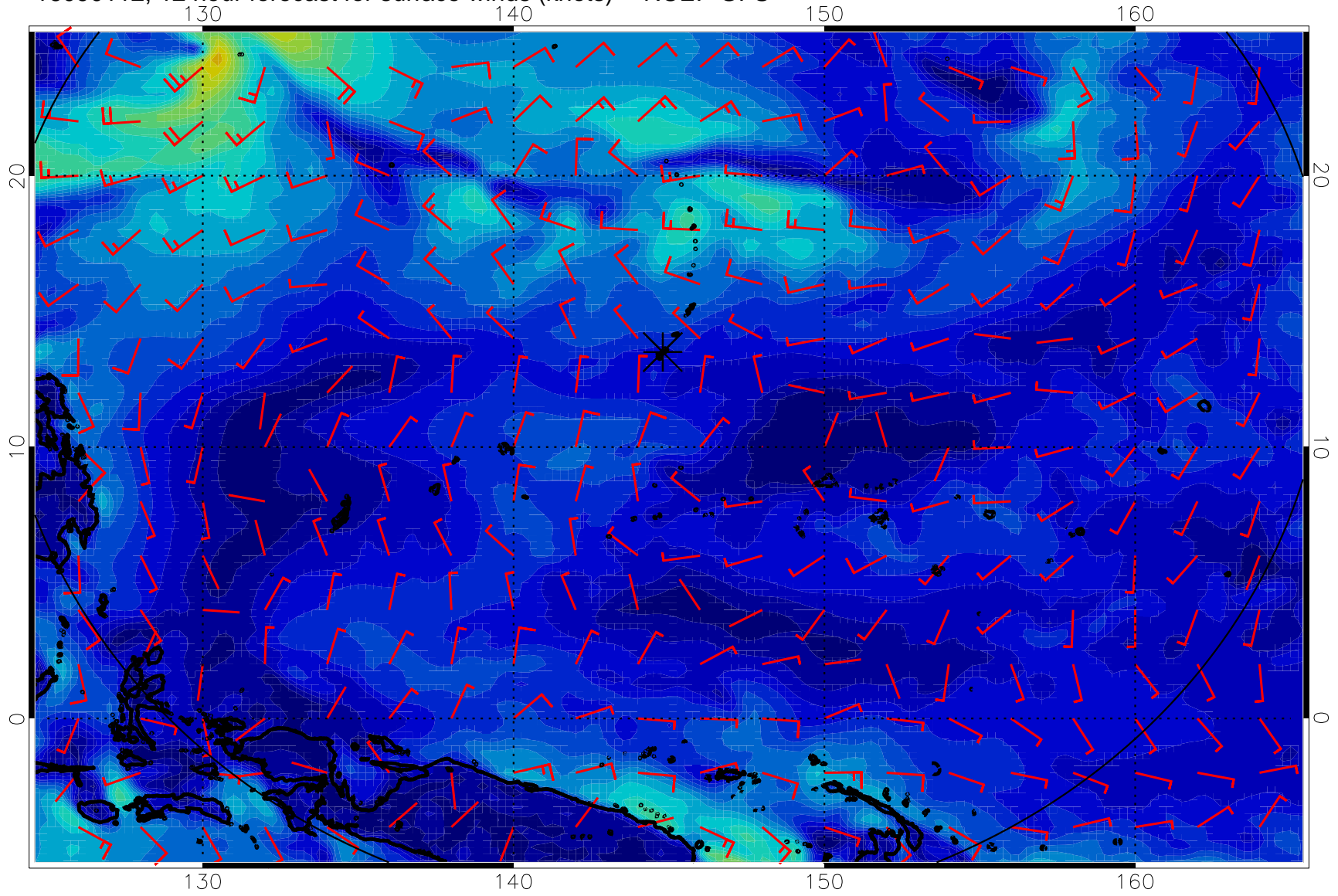
16090112, 12 hour forecast for surface winds (knots) -- NCEP GFS
