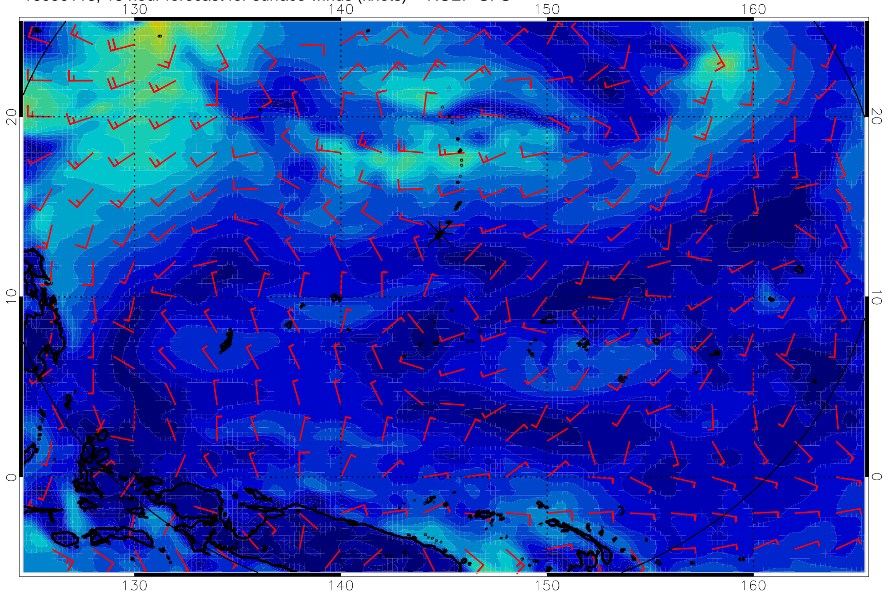
16090118, 18 hour forecast for surface winds (knots) -- NCEP GFS
