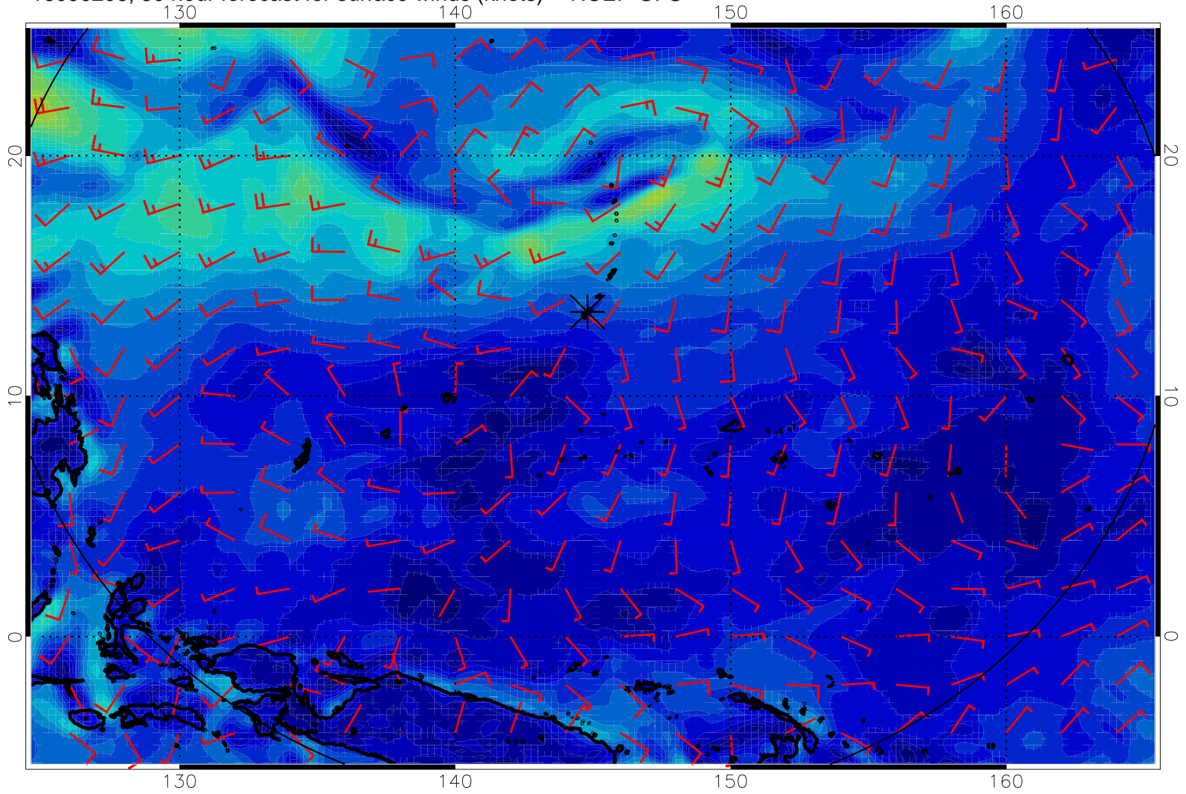
16090206, 30 hour forecast for surface winds (knots) -- NCEP GFS
