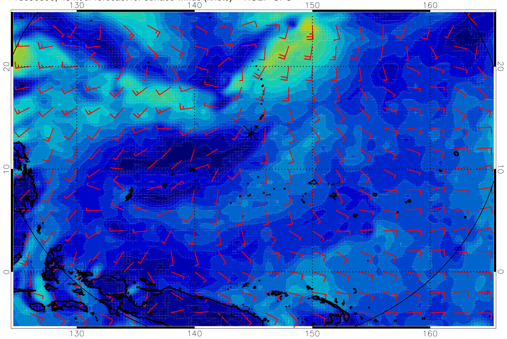
16090300, 48 hour forecast for surface winds (knots) -- NCEP GFS
