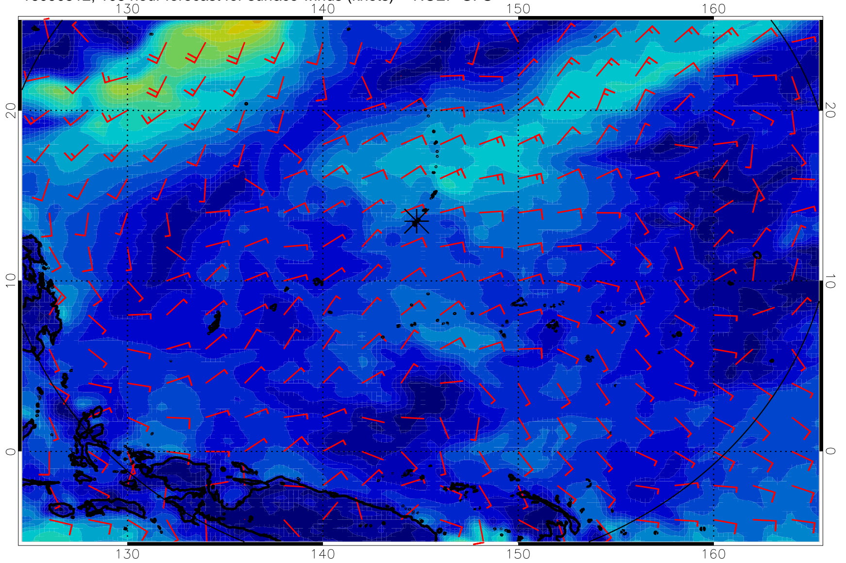
16090512, 108 hour forecast for surface winds (knots) -- NCEP GFS
