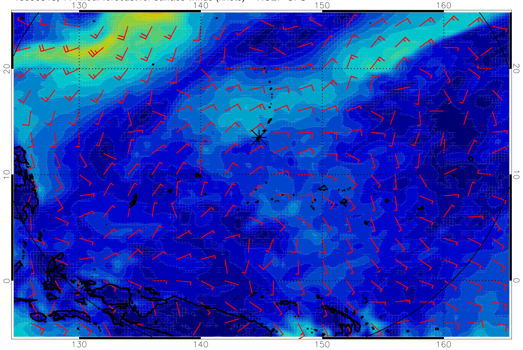
16090518, 114 hour forecast for surface winds (knots) -- NCEP GFS
