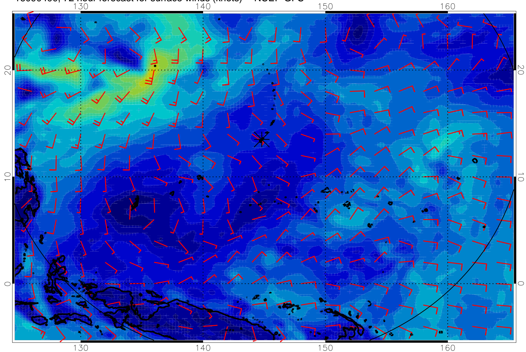
16090400, 72 hour forecast for surface winds (knots) -- NCEP GFS
