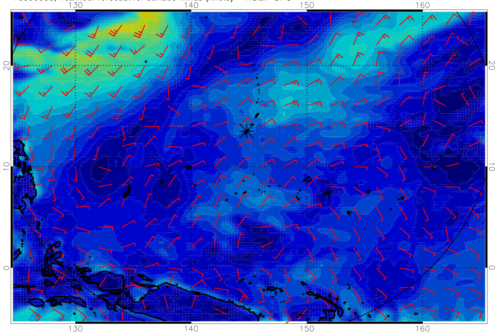
16090506, 102 hour forecast for surface winds (knots) -- NCEP GFS
