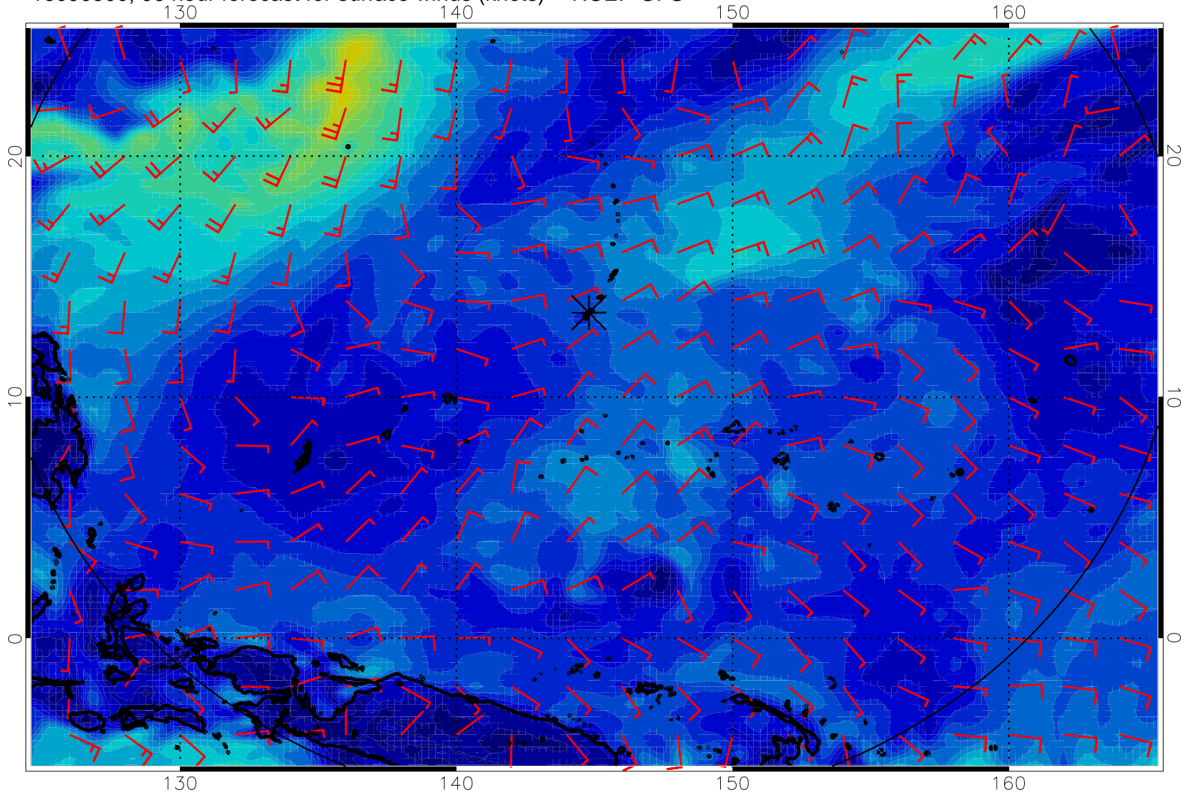
16090500, 96 hour forecast for surface winds (knots) -- NCEP GFS
