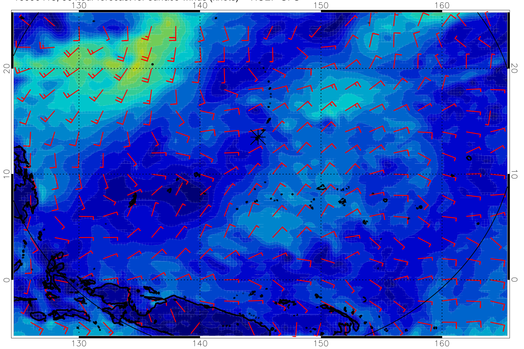
16090418, 90 hour forecast for surface winds (knots) -- NCEP GFS
