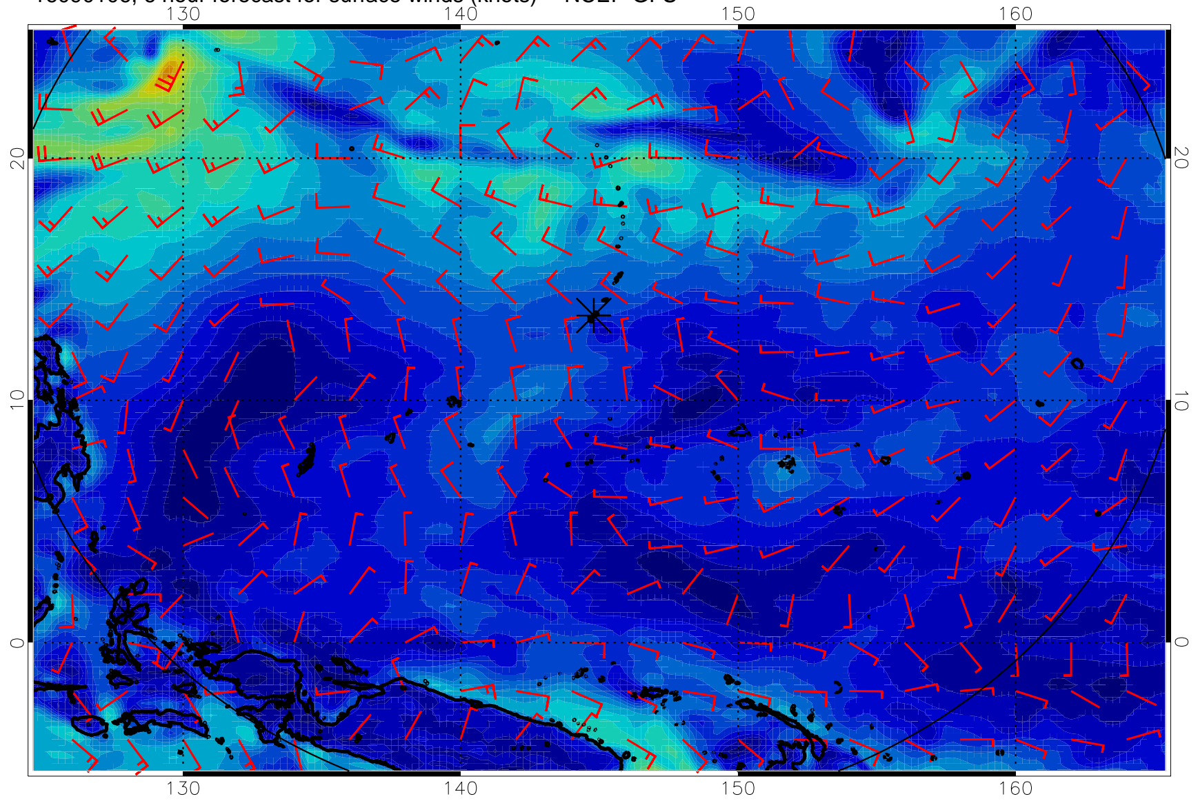
16090106, 6 hour forecast for surface winds (knots) -- NCEP GFS
