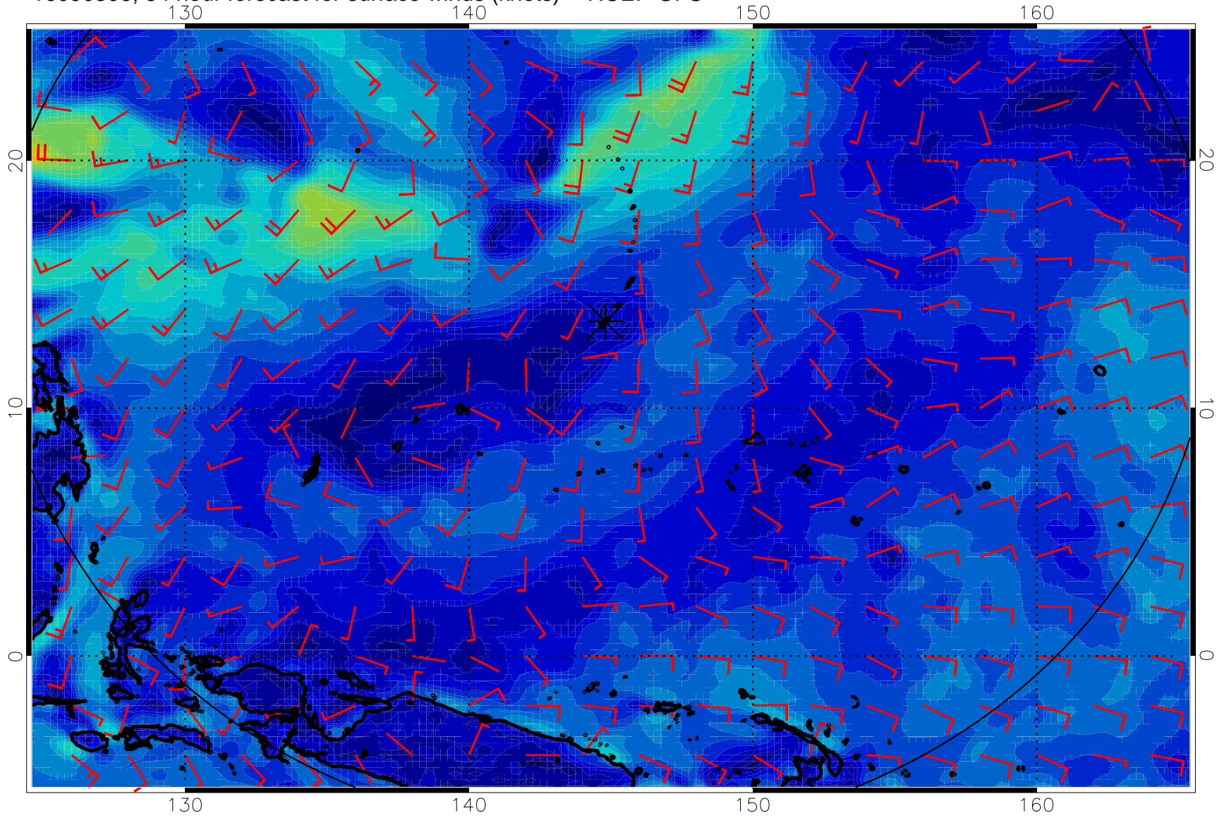
16090306, 54 hour forecast for surface winds (knots) -- NCEP GFS
