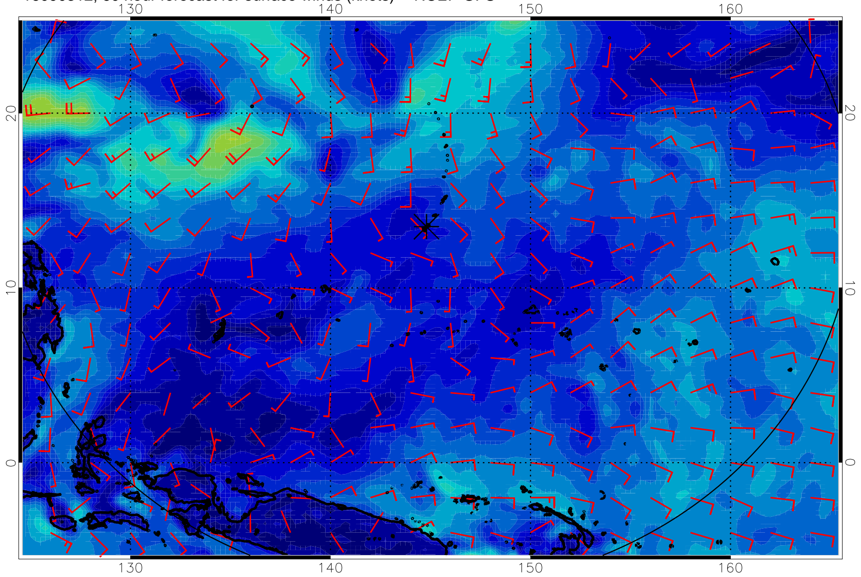
16090312, 60 hour forecast for surface winds (knots) -- NCEP GFS
