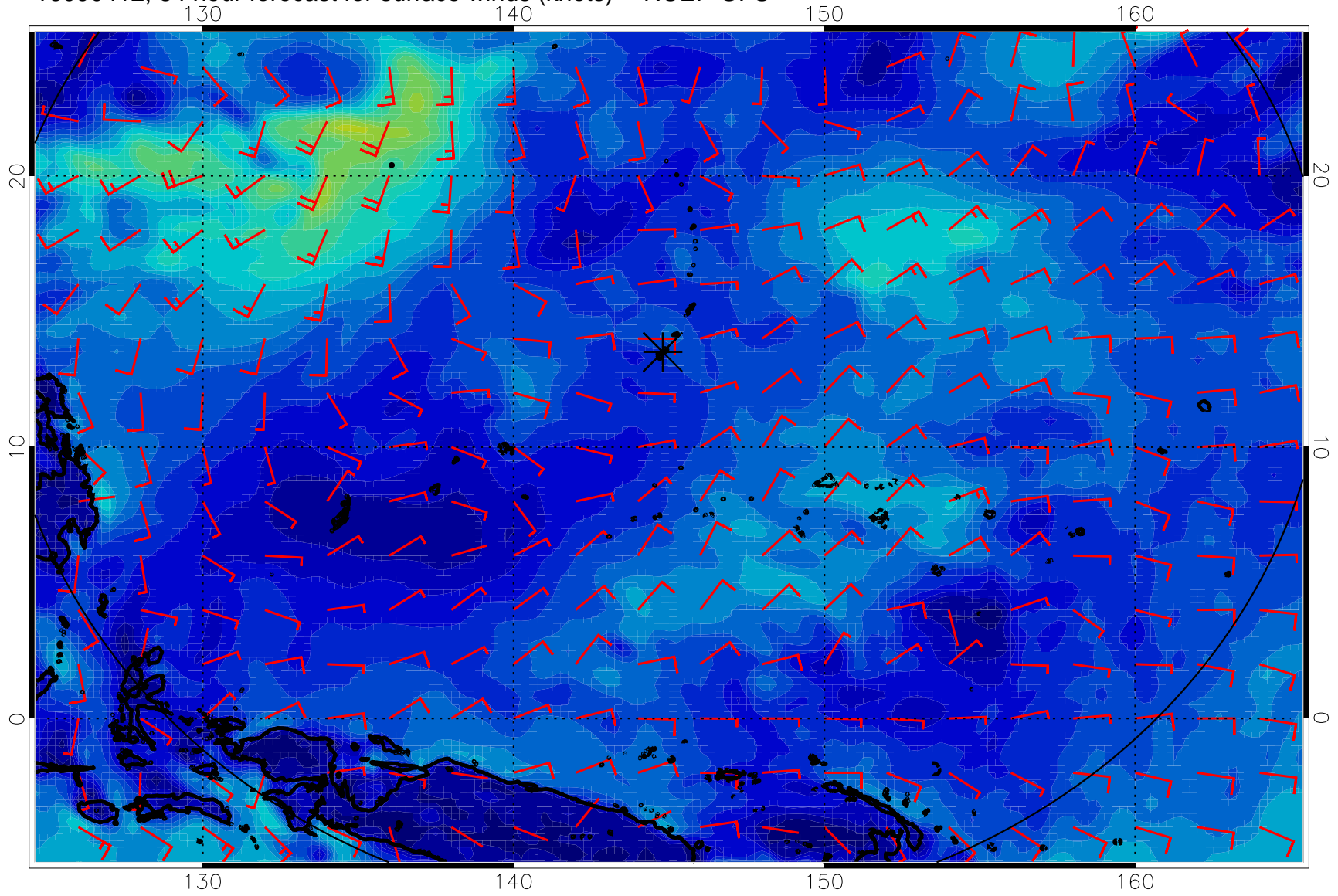
16090412, 84 hour forecast for surface winds (knots) -- NCEP GFS
