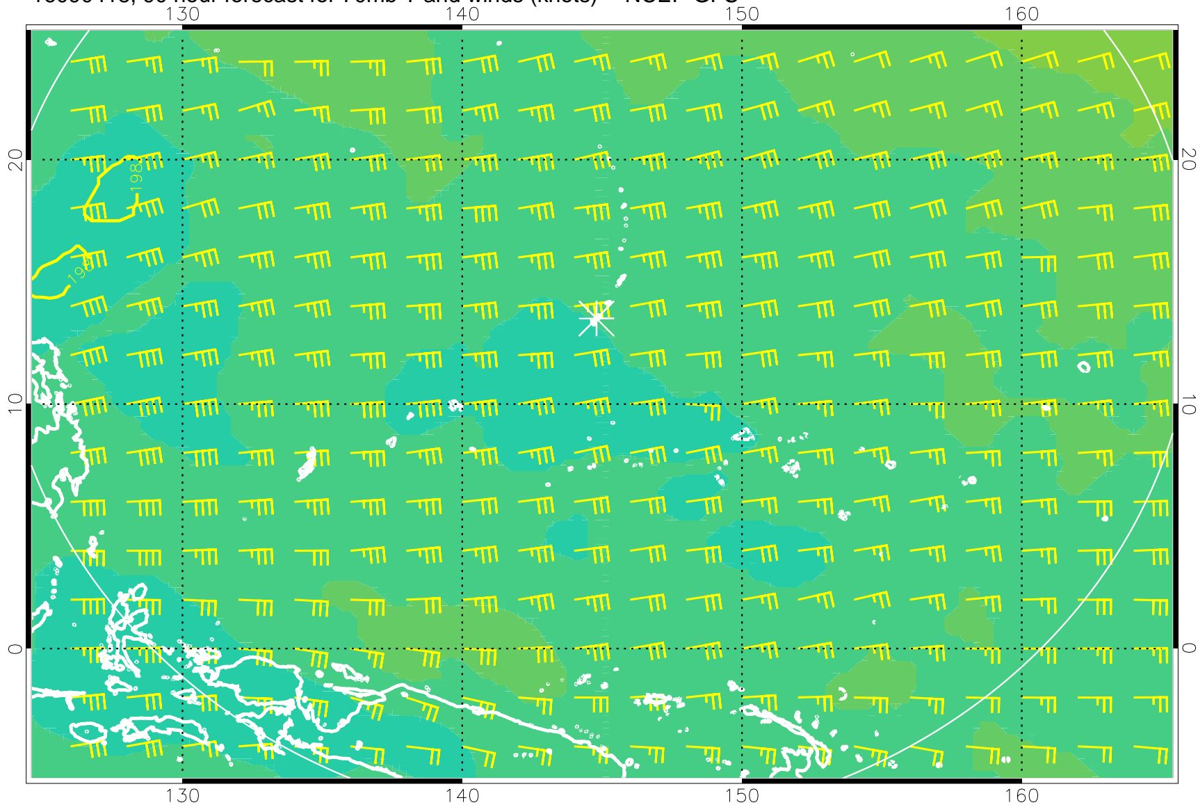
16090418, 90 hour forecast for 70mb T and winds (knots) -- NCEP GFS
