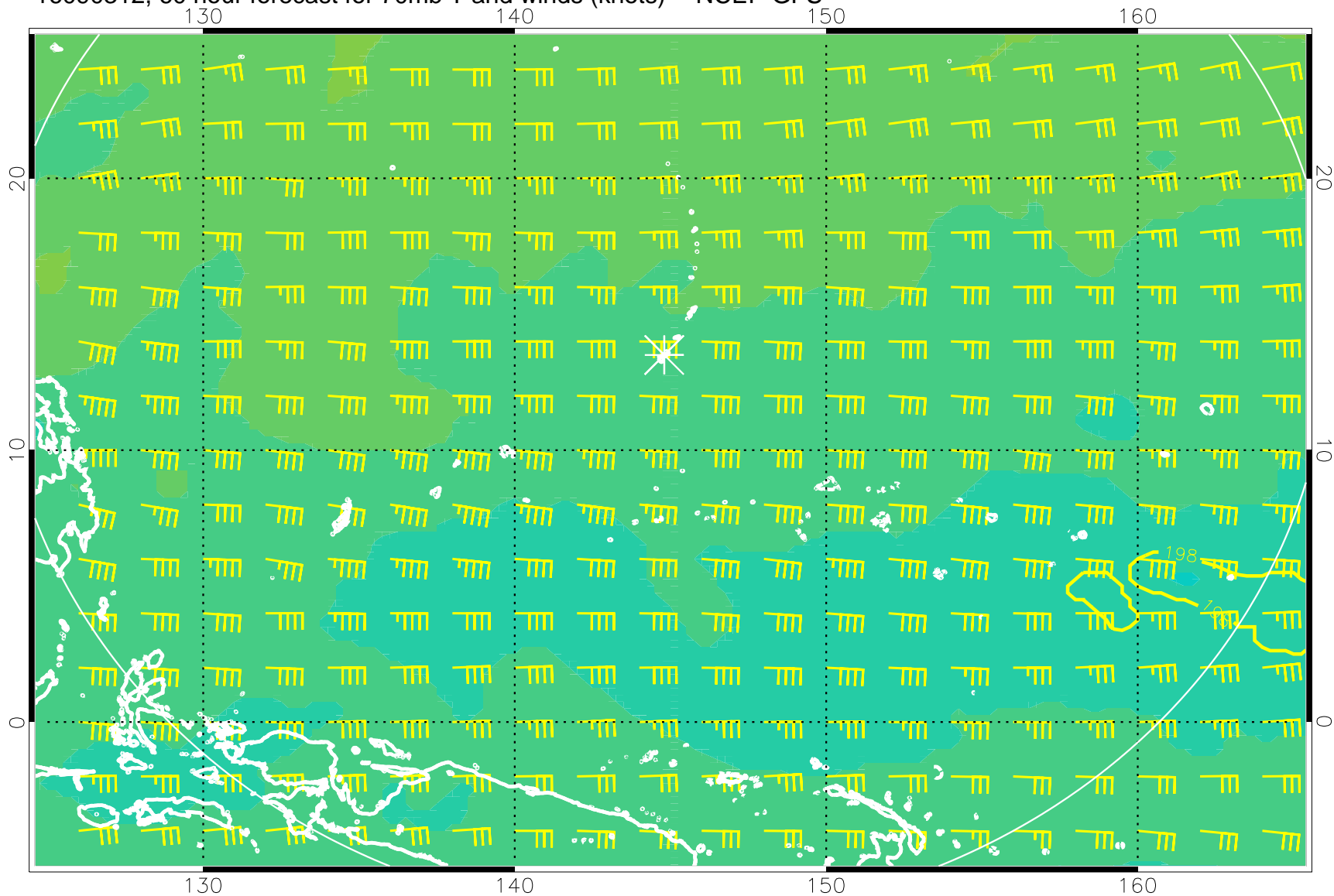
16090312, 60 hour forecast for 70mb T and winds (knots) -- NCEP GFS
