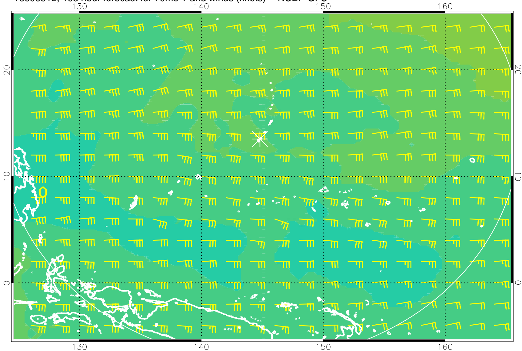
16090512, 108 hour forecast for 70mb T and winds (knots) -- NCEP GFS
