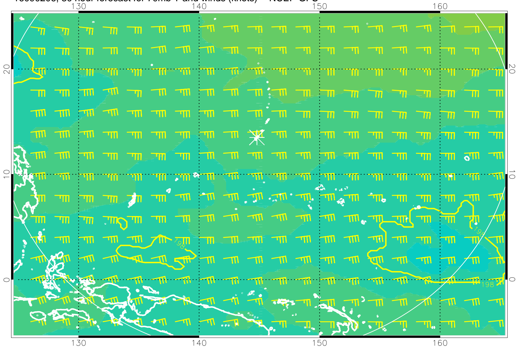
16090206, 30 hour forecast for 70mb T and winds (knots) -- NCEP GFS
