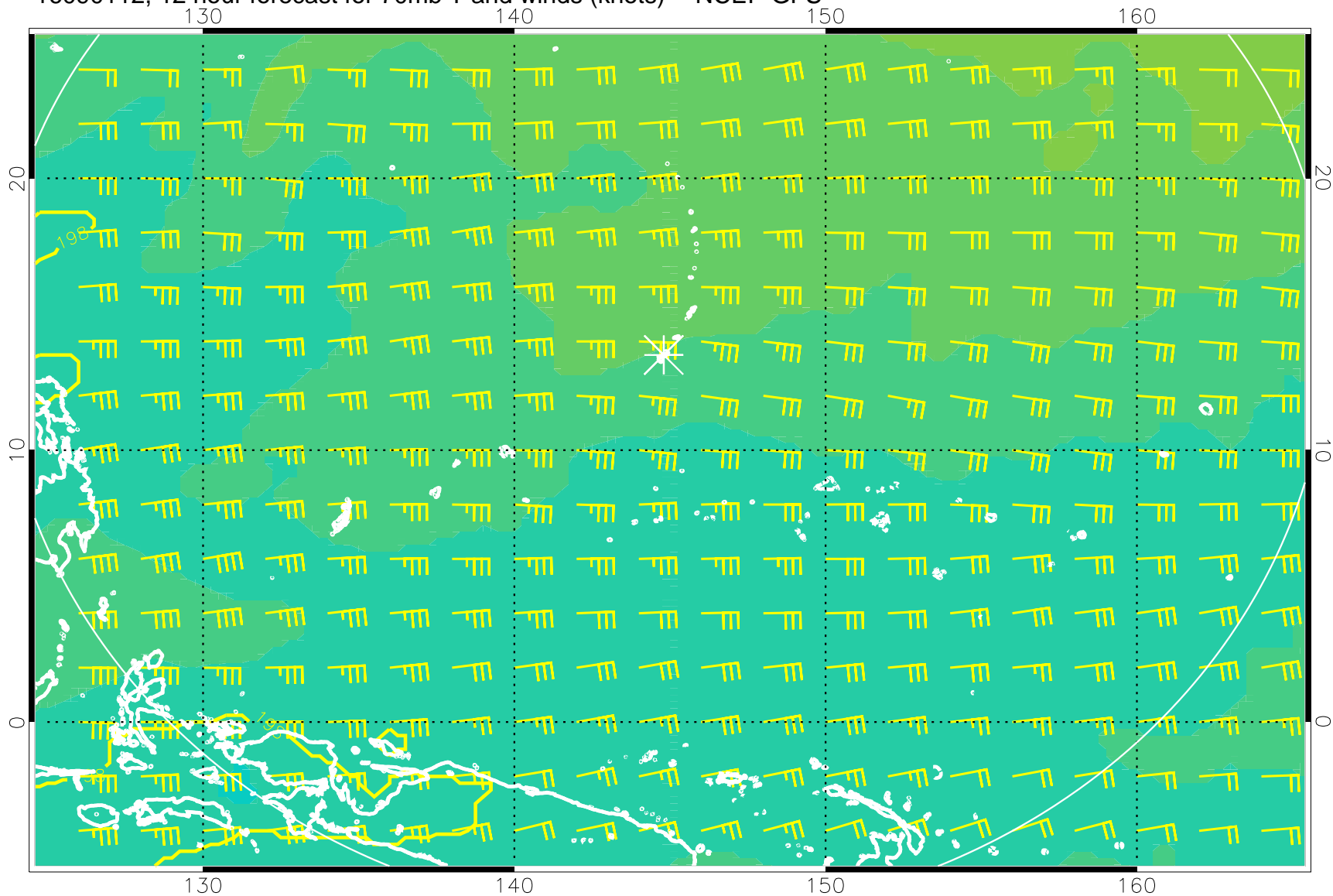
16090112, 12 hour forecast for 70mb T and winds (knots) -- NCEP GFS
