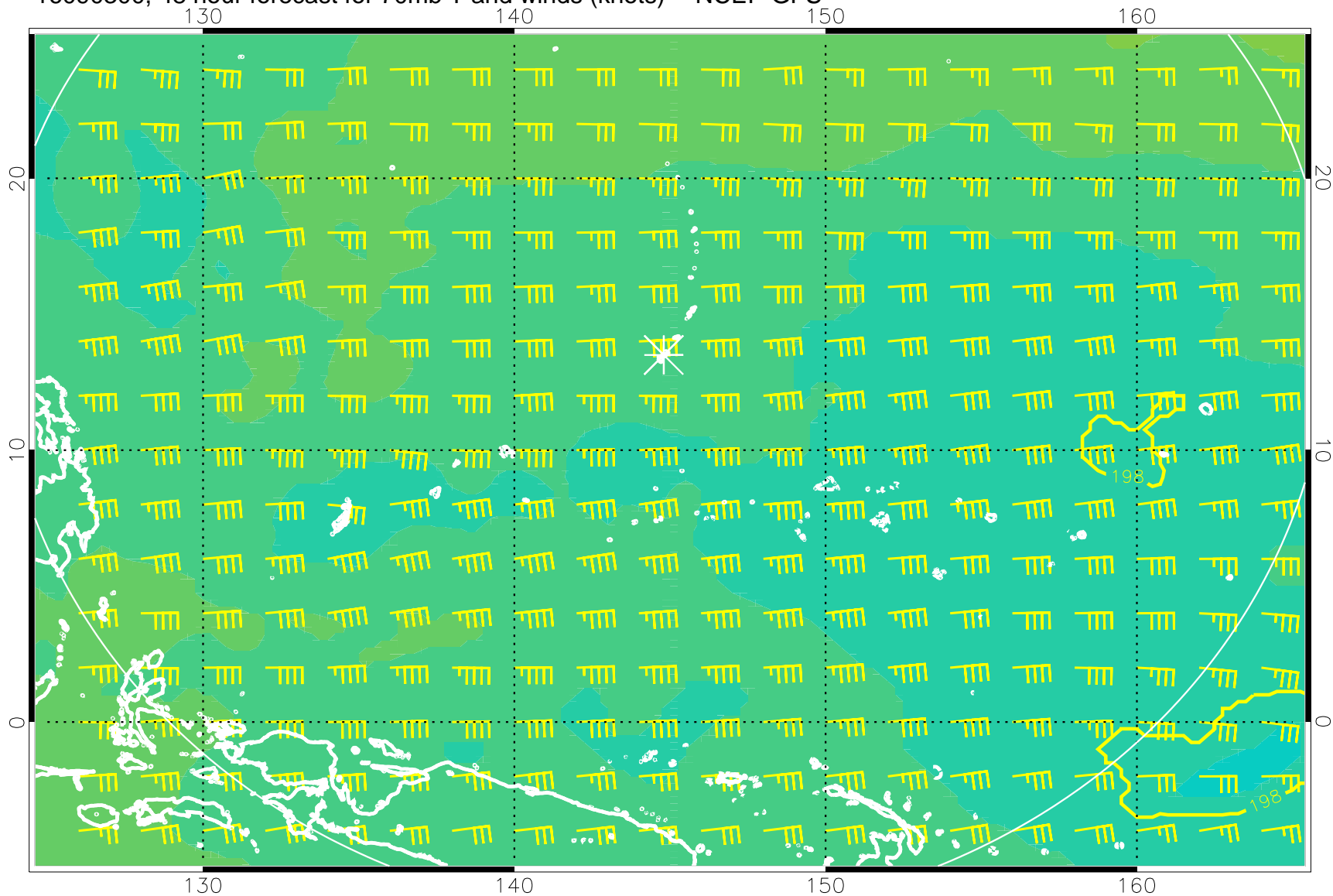
16090300, 48 hour forecast for 70mb T and winds (knots) -- NCEP GFS
