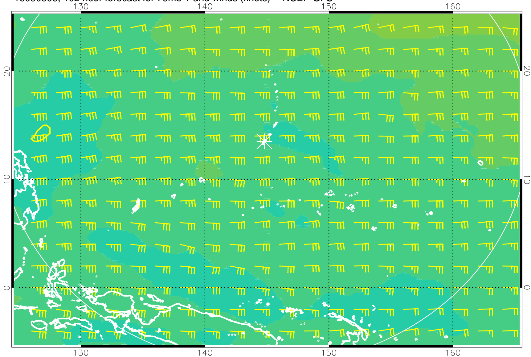
16090506, 102 hour forecast for 70mb T and winds (knots) -- NCEP GFS
