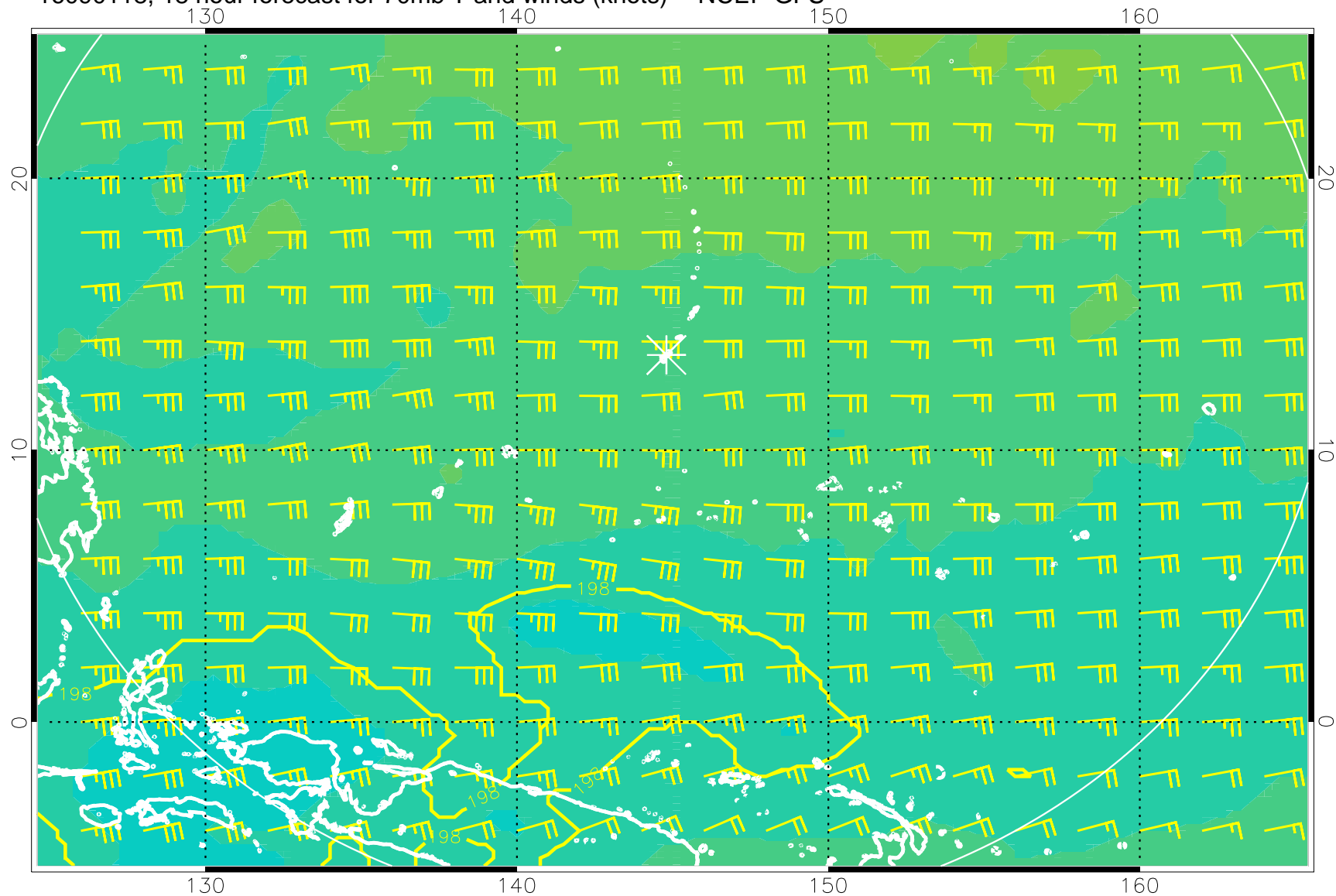
16090118, 18 hour forecast for 70mb T and winds (knots) -- NCEP GFS
