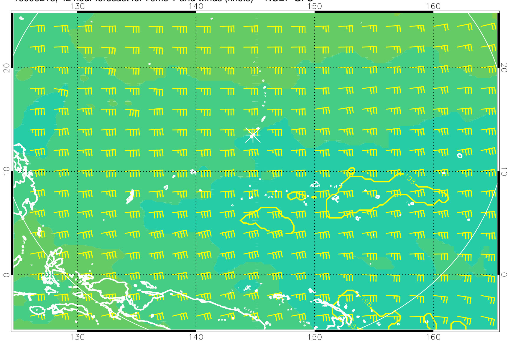
16090218, 42 hour forecast for 70mb T and winds (knots) -- NCEP GFS
