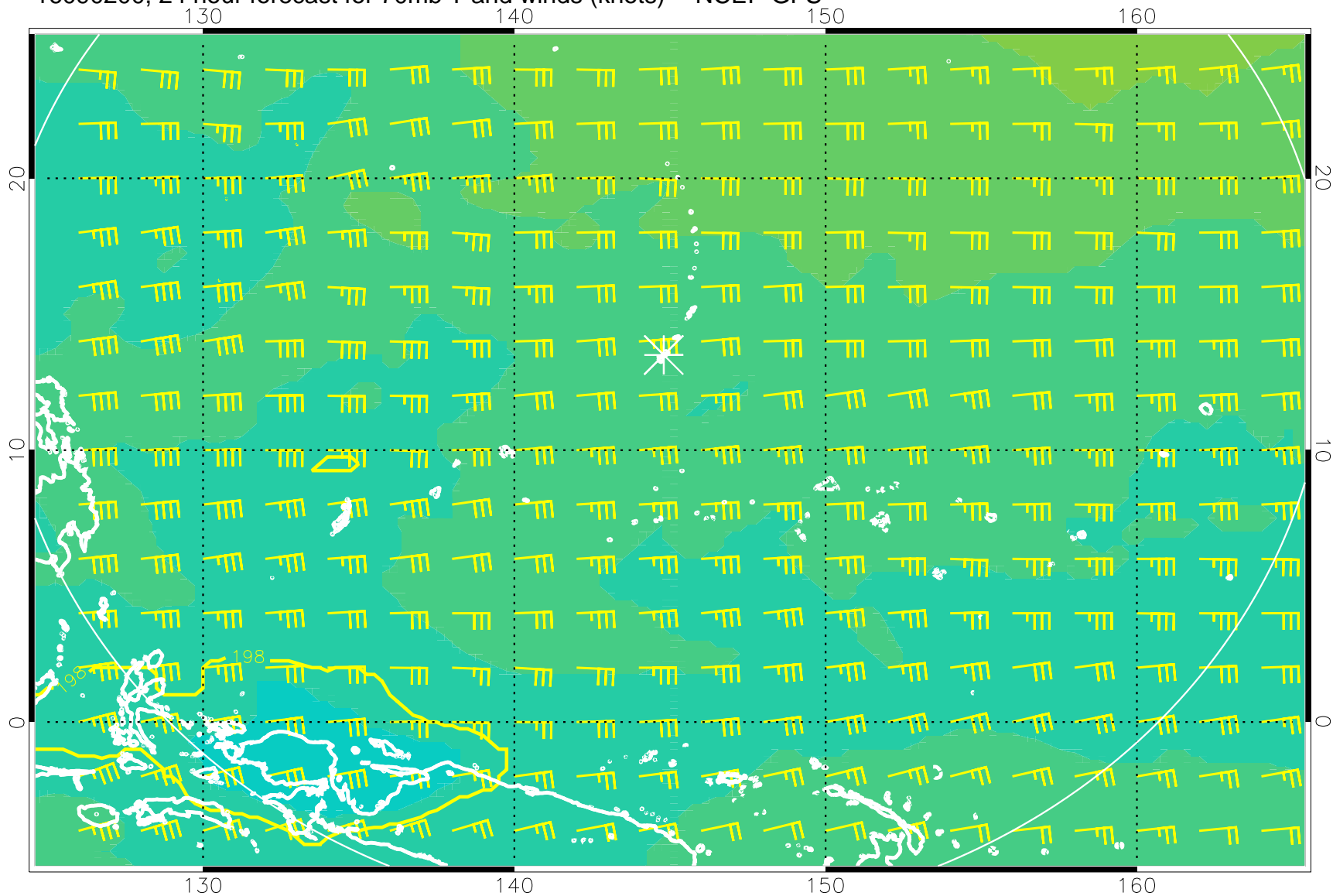
16090200, 24 hour forecast for 70mb T and winds (knots) -- NCEP GFS
