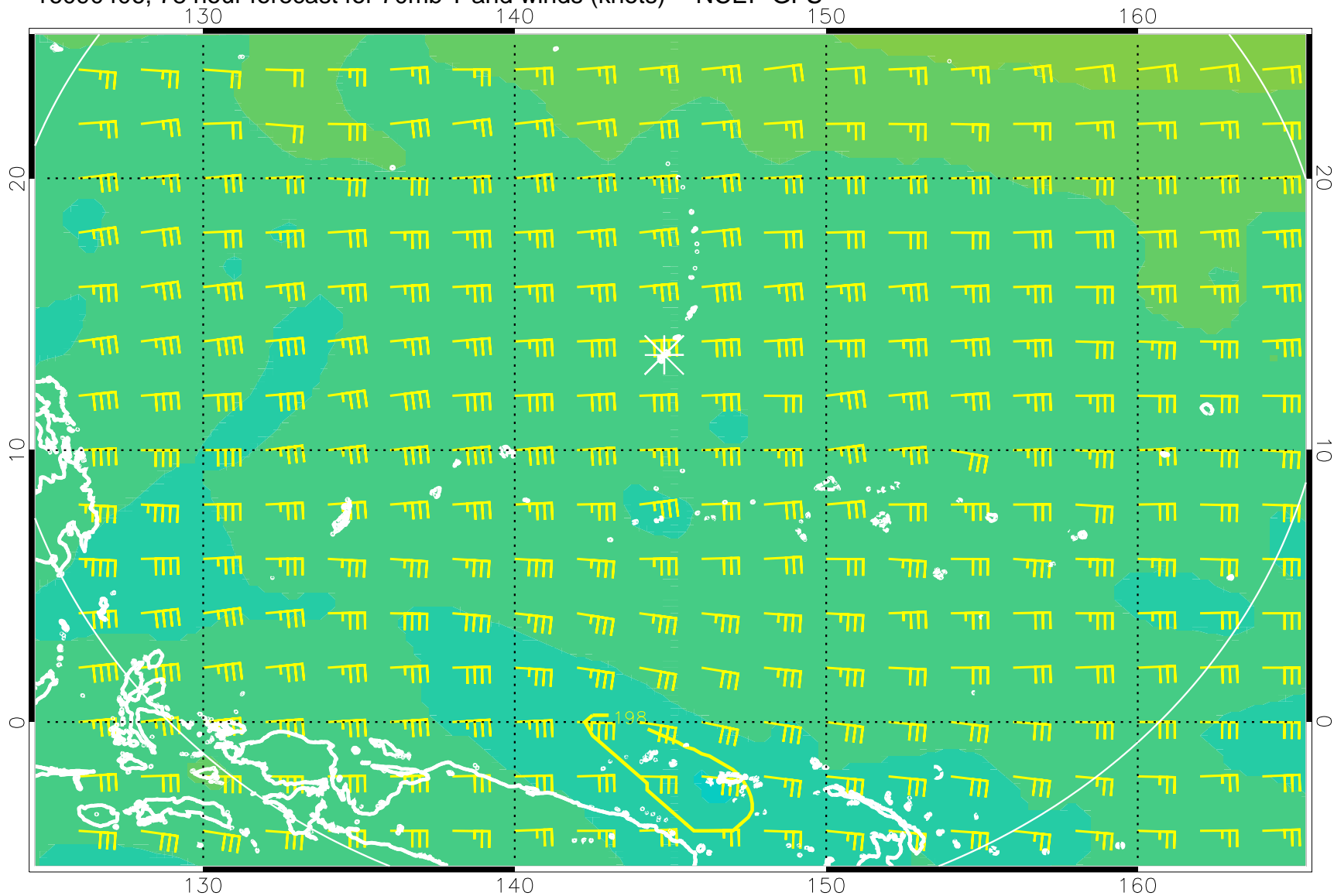
16090406, 78 hour forecast for 70mb T and winds (knots) -- NCEP GFS
