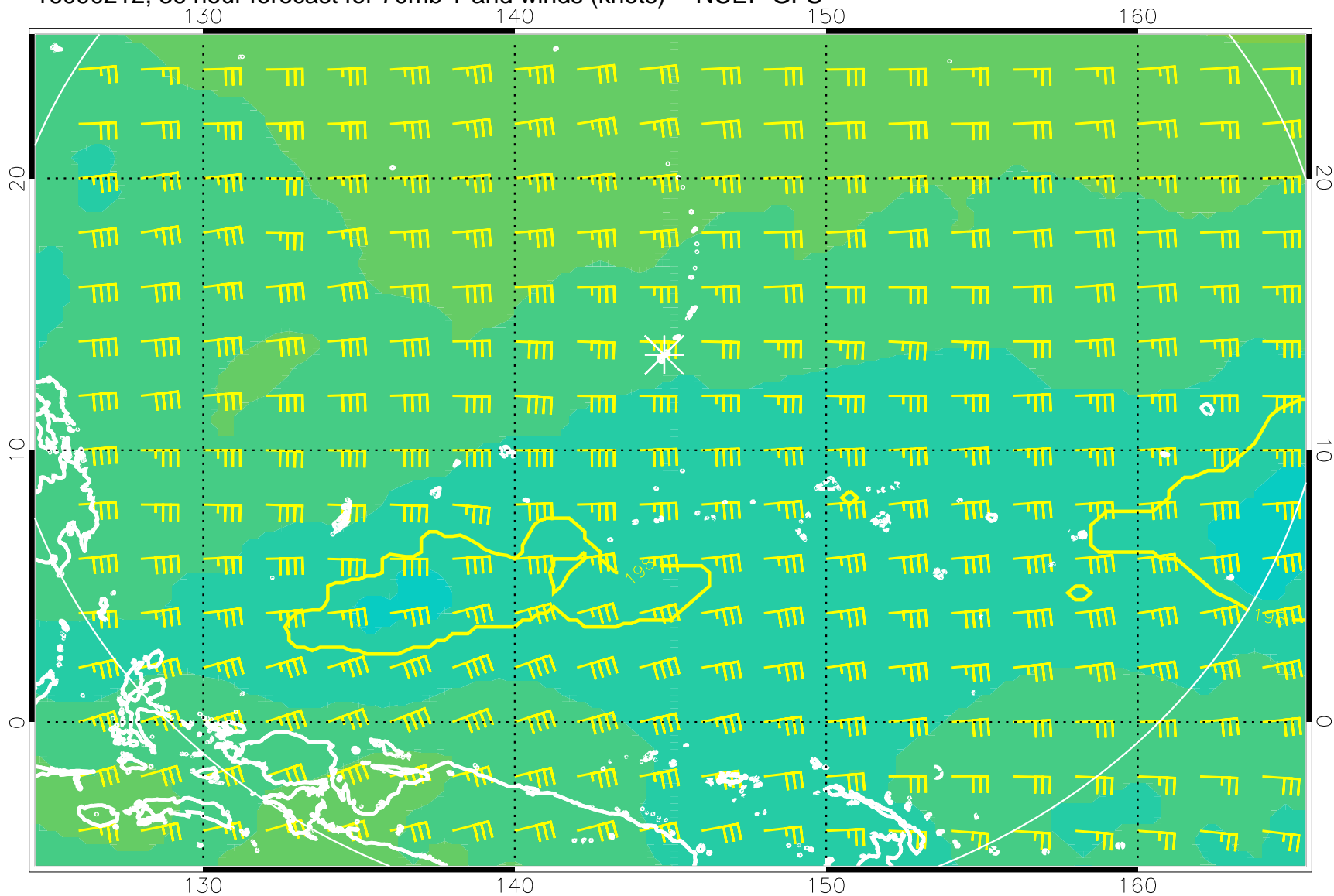
16090212, 36 hour forecast for 70mb T and winds (knots) -- NCEP GFS
