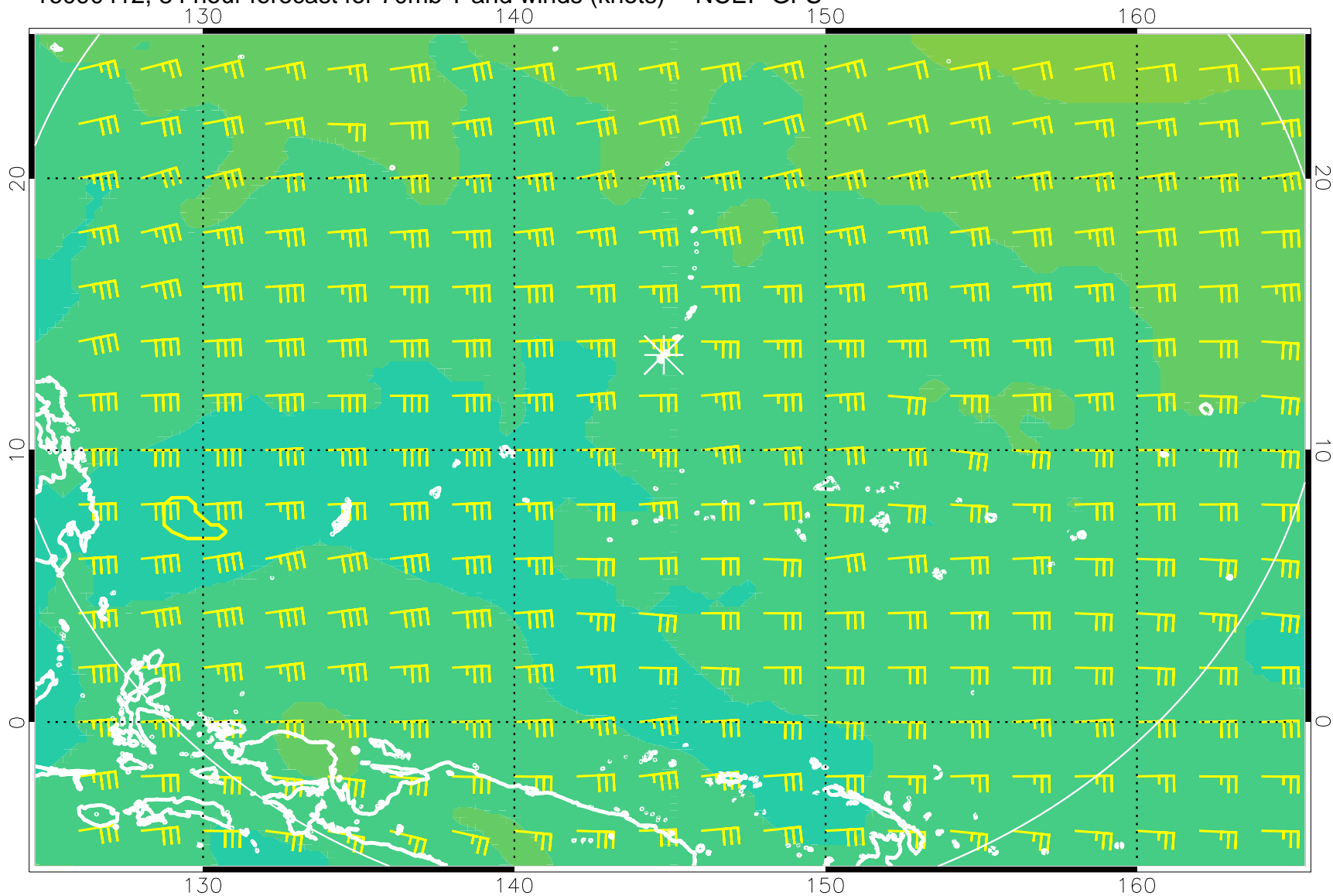
16090412, 84 hour forecast for 70mb T and winds (knots) -- NCEP GFS
