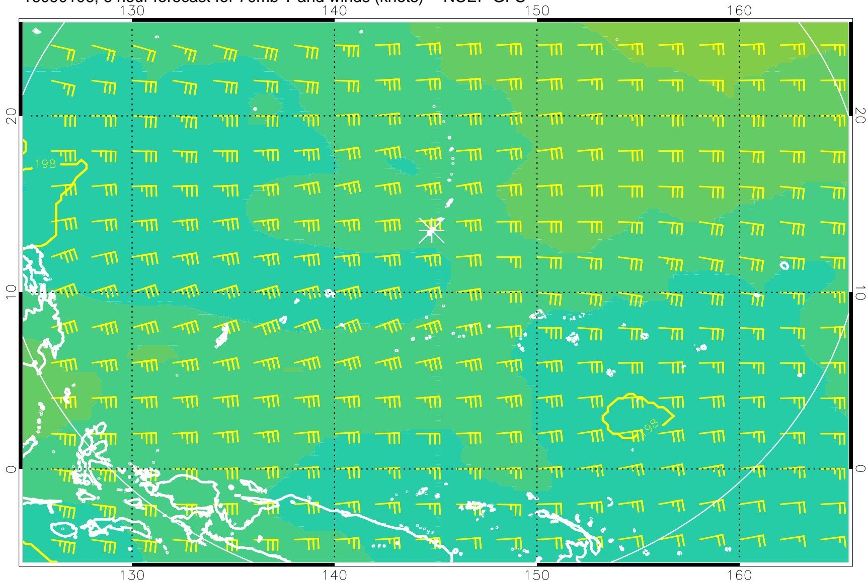
16090106, 6 hour forecast for 70mb T and winds (knots) -- NCEP GFS
