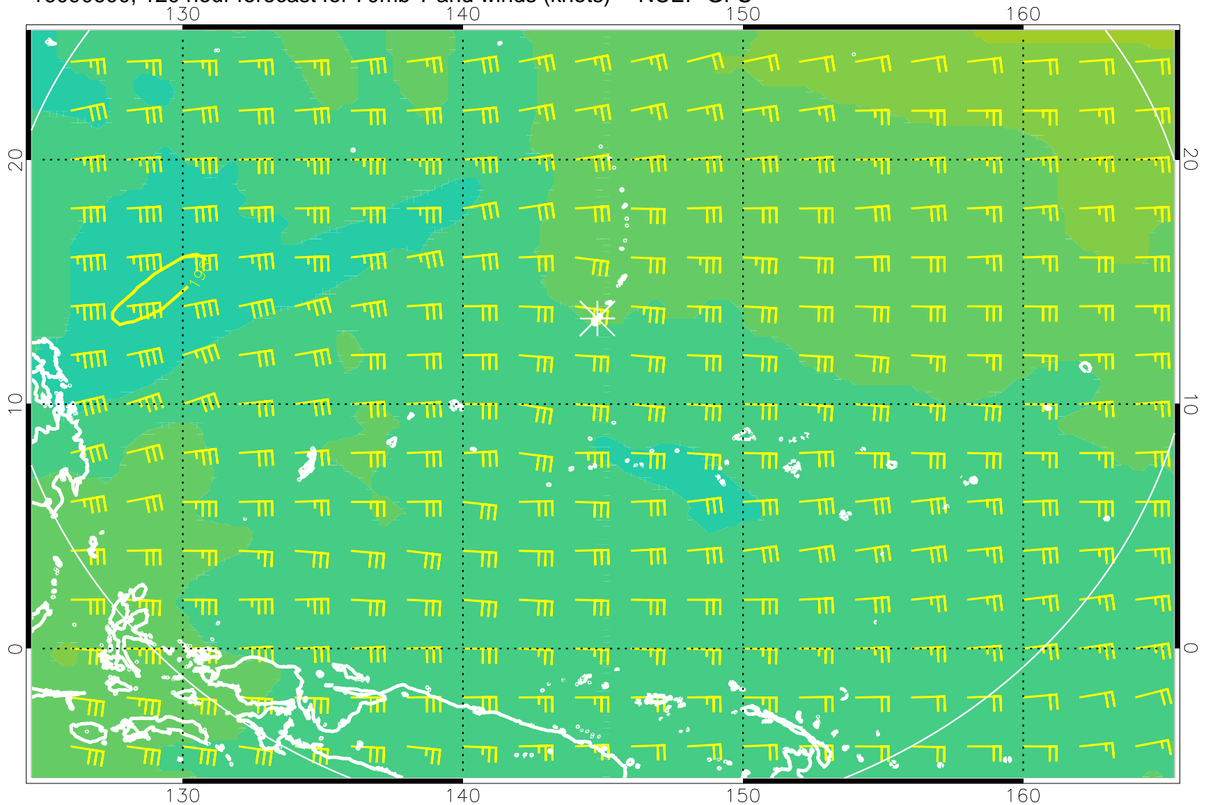
16090600, 120 hour forecast for 70mb T and winds (knots) -- NCEP GFS
