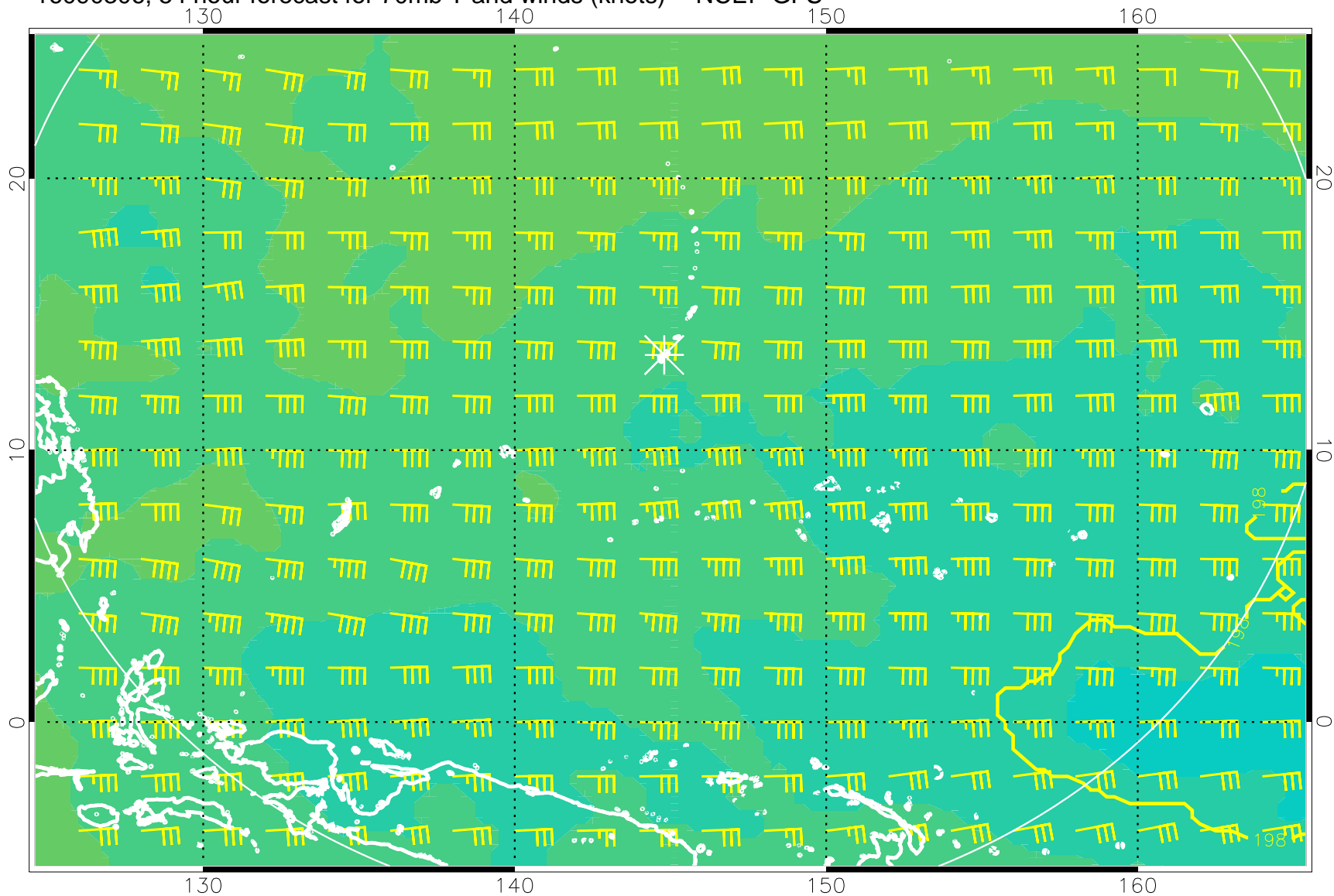
16090306, 54 hour forecast for 70mb T and winds (knots) -- NCEP GFS
