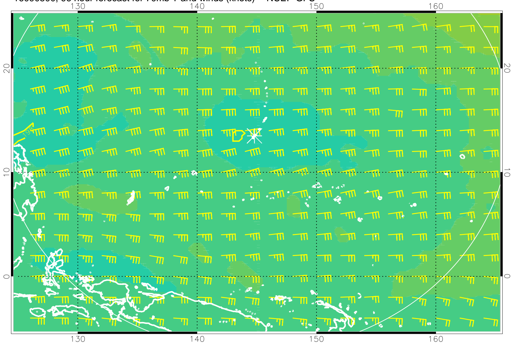
16090500, 96 hour forecast for 70mb T and winds (knots) -- NCEP GFS
