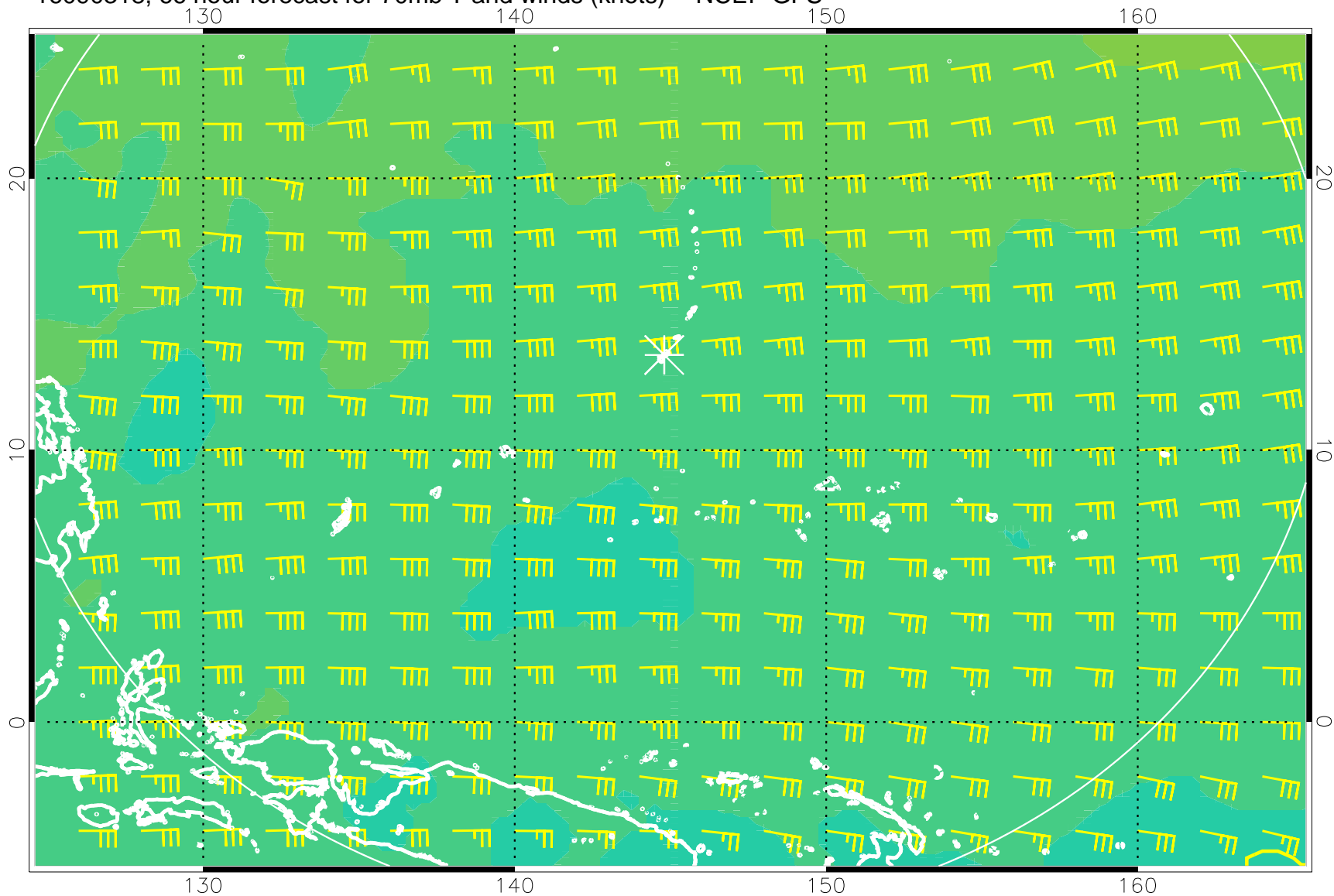
16090318, 66 hour forecast for 70mb T and winds (knots) -- NCEP GFS
