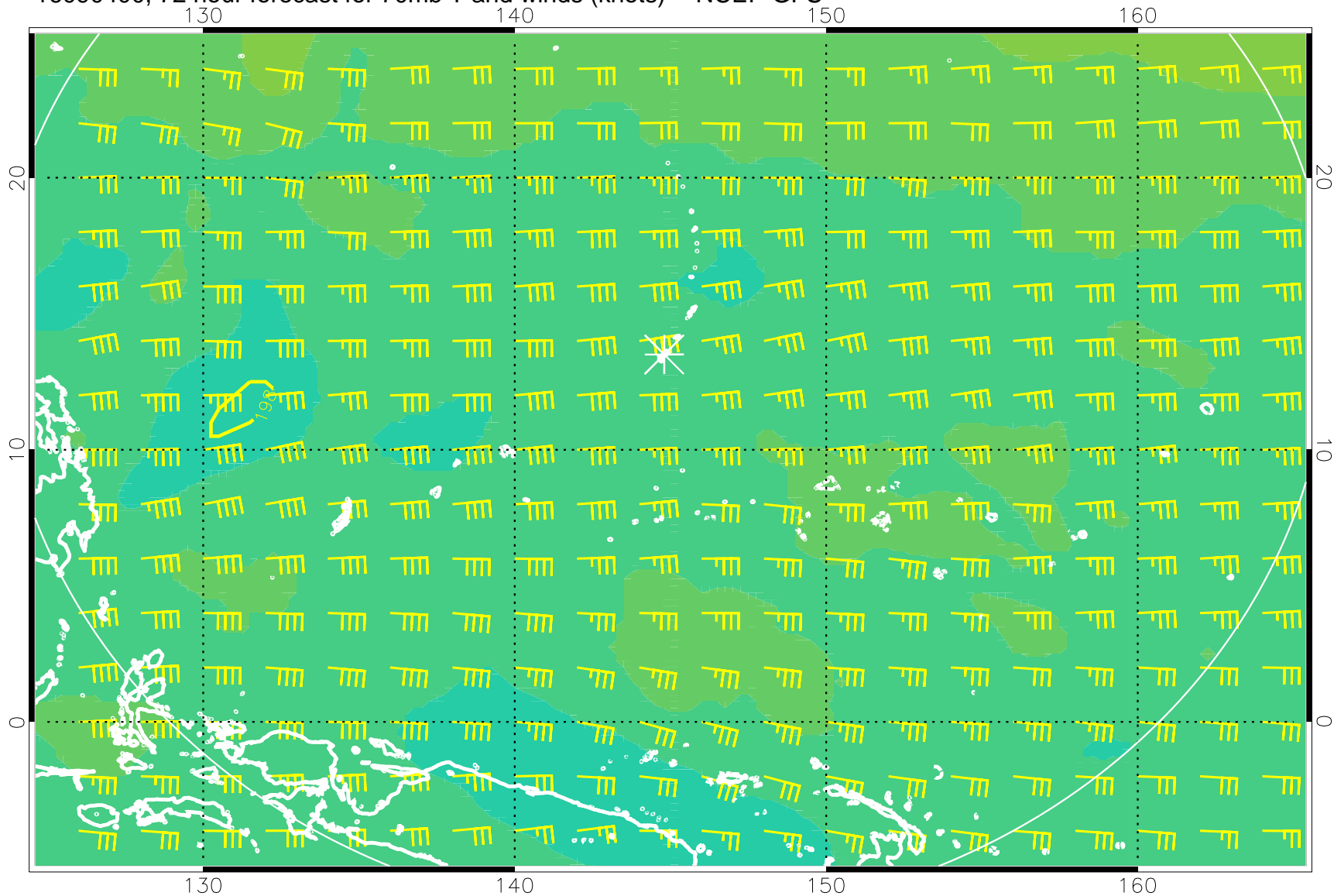
16090400, 72 hour forecast for 70mb T and winds (knots) -- NCEP GFS
