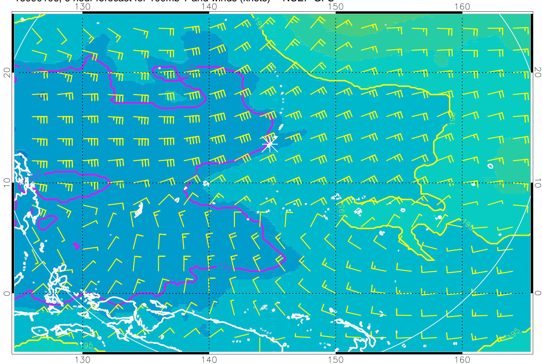
16090106, 6 hour forecast for 100mb T and winds (knots) -- NCEP GFS
