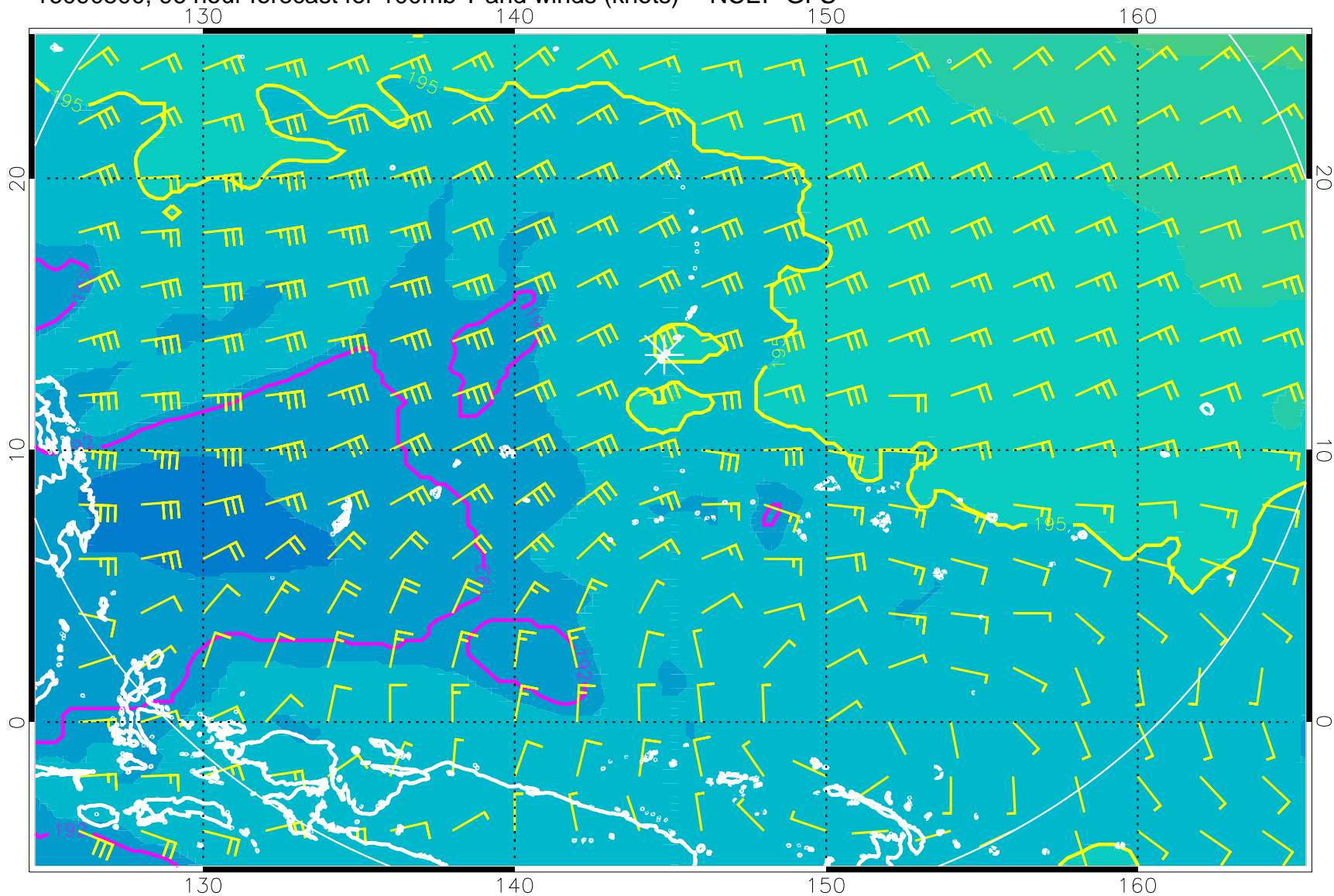
16090500, 96 hour forecast for 100mb T and winds (knots) -- NCEP GFS
