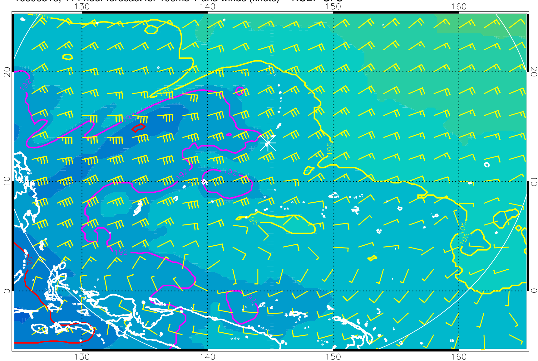
16090518, 114 hour forecast for 100mb T and winds (knots) -- NCEP GFS
