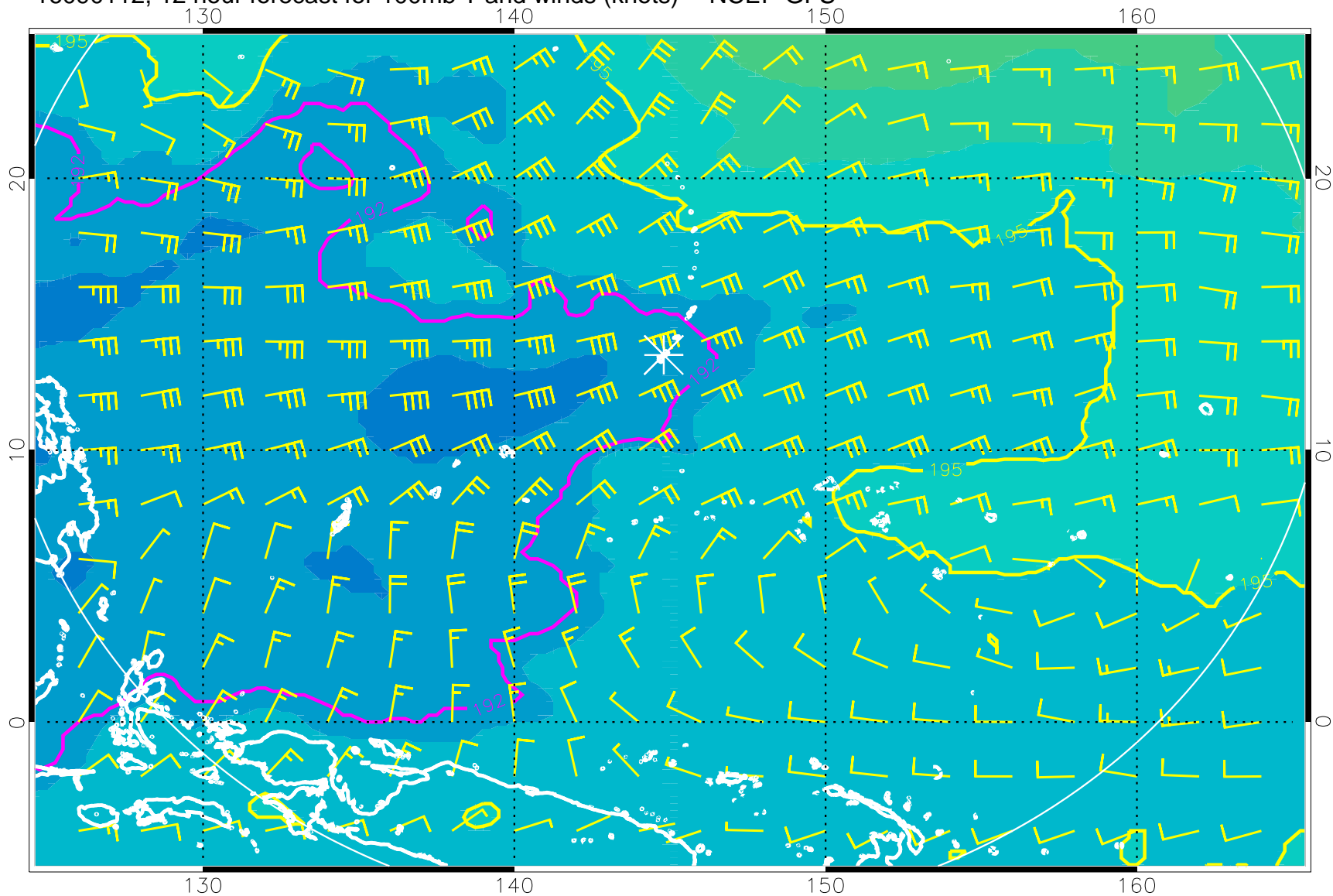
16090112, 12 hour forecast for 100mb T and winds (knots) -- NCEP GFS
