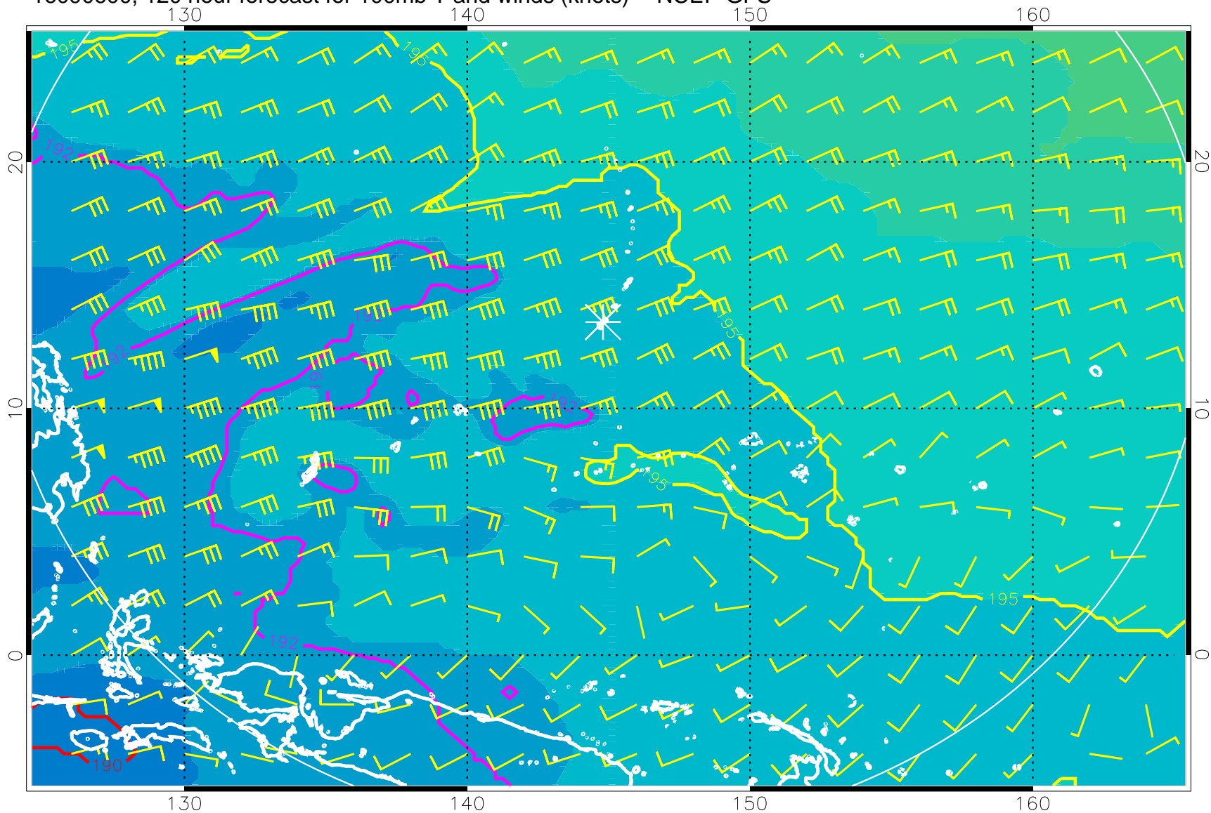
16090600, 120 hour forecast for 100mb T and winds (knots) -- NCEP GFS
