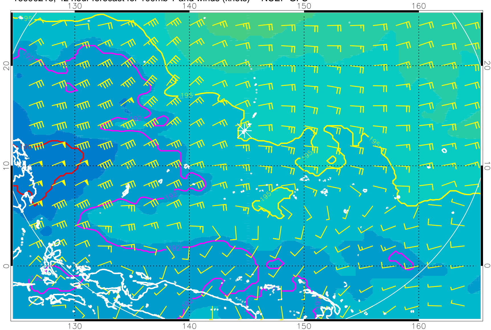
16090218, 42 hour forecast for 100mb T and winds (knots) -- NCEP GFS
