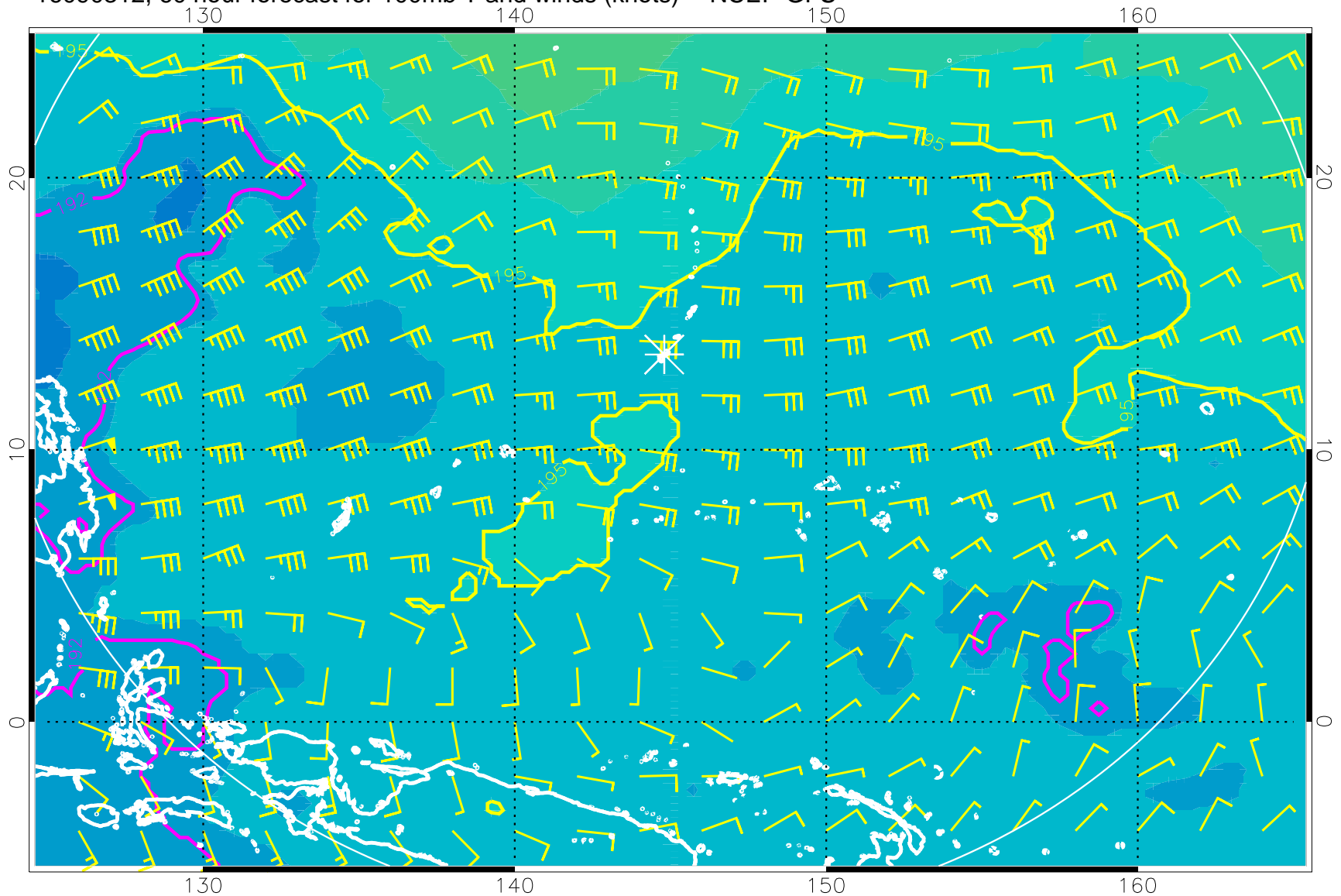
16090312, 60 hour forecast for 100mb T and winds (knots) -- NCEP GFS
