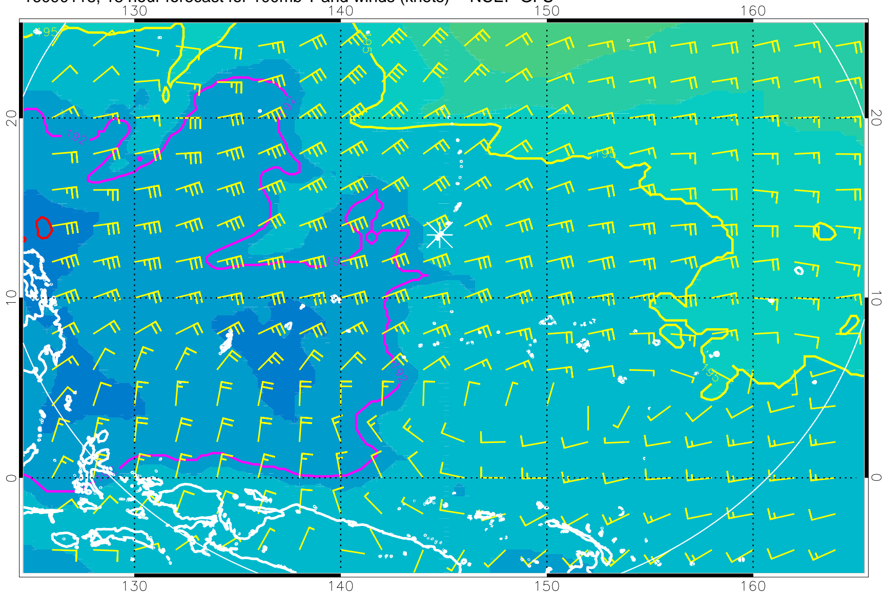
16090118, 18 hour forecast for 100mb T and winds (knots) -- NCEP GFS
