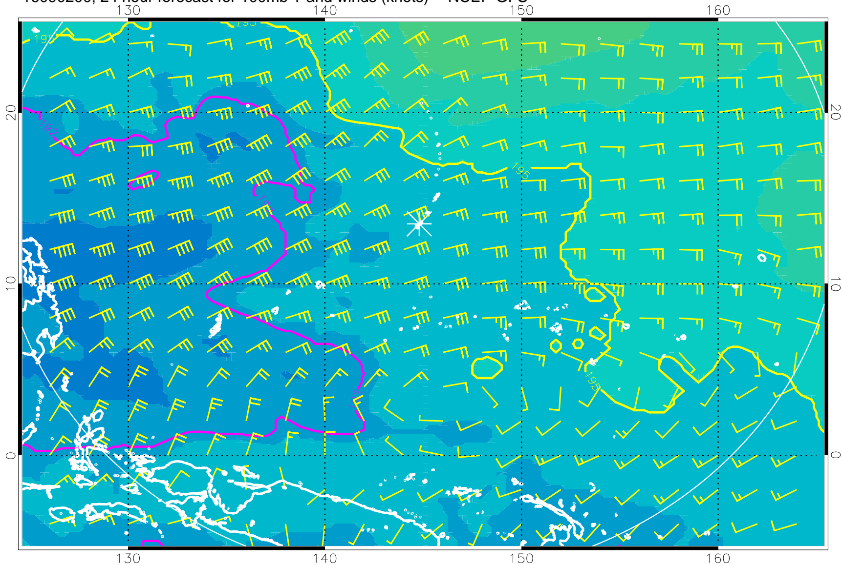
16090200, 24 hour forecast for 100mb T and winds (knots) -- NCEP GFS
