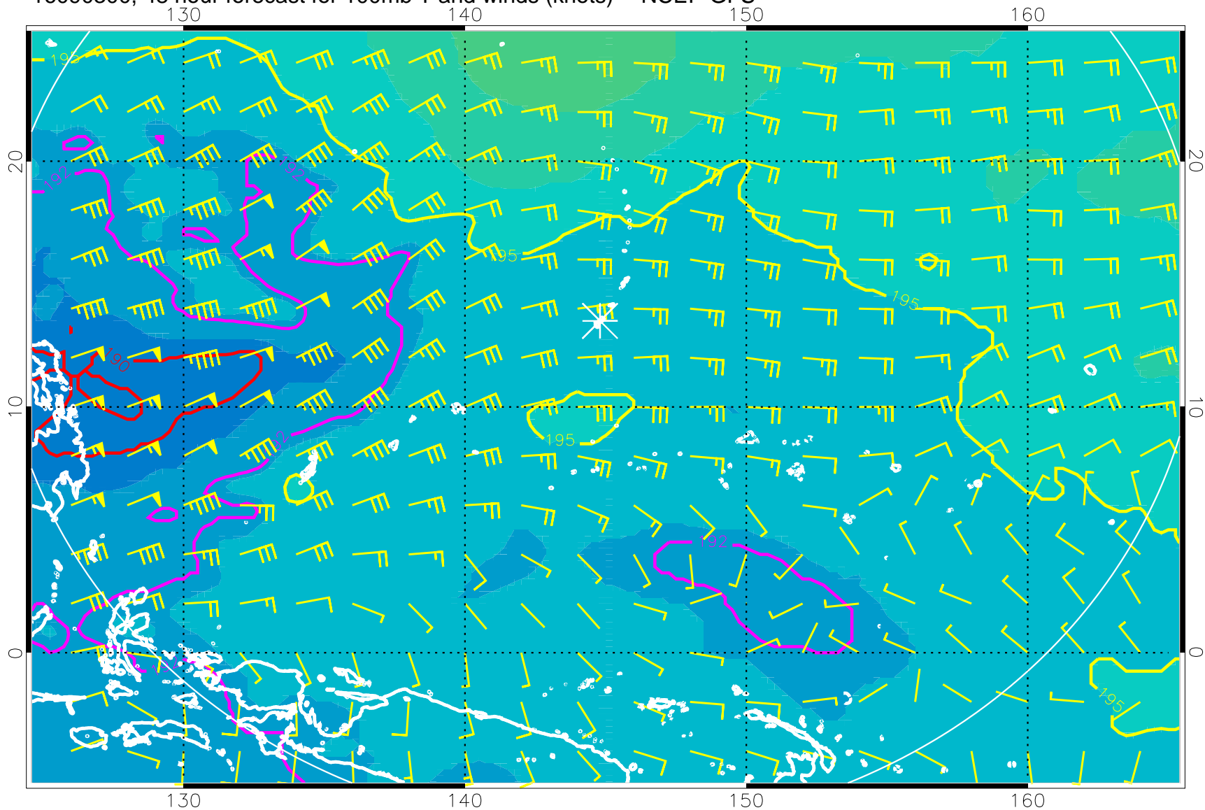
16090300, 48 hour forecast for 100mb T and winds (knots) -- NCEP GFS
