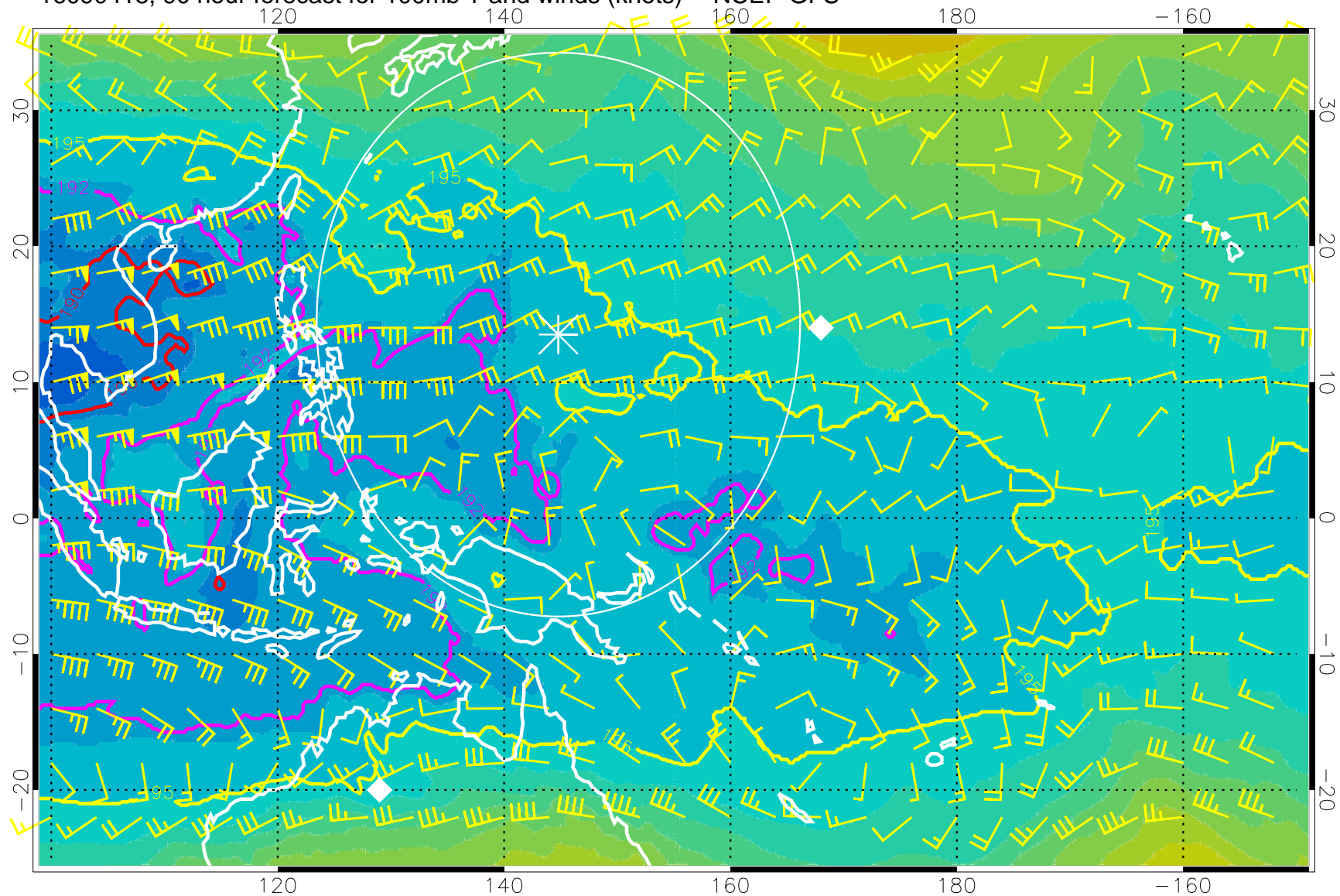
16090418, 90 hour forecast for 100mb T and winds (knots) -- NCEP GFS
