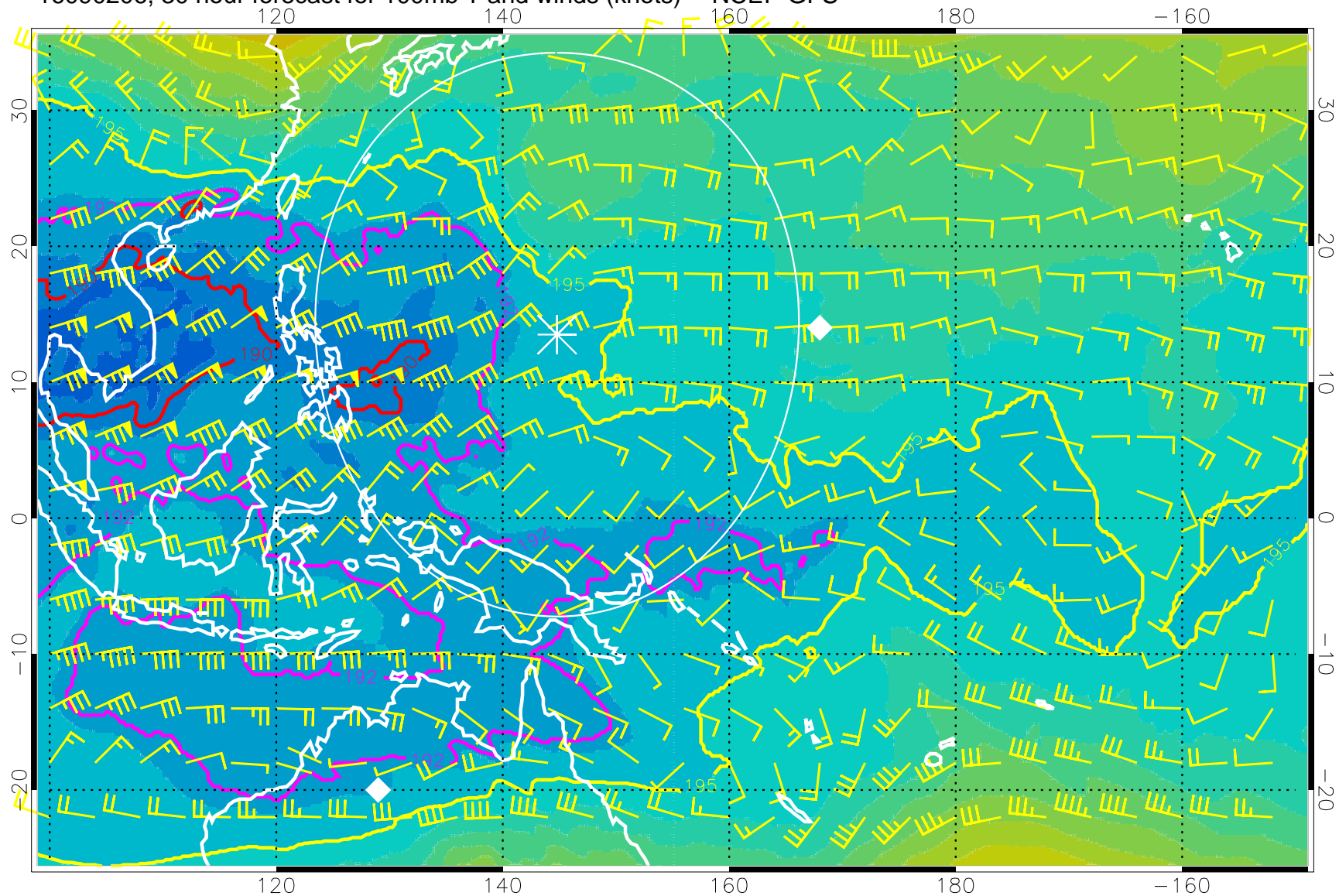
16090206, 30 hour forecast for 100mb T and winds (knots) -- NCEP GFS
