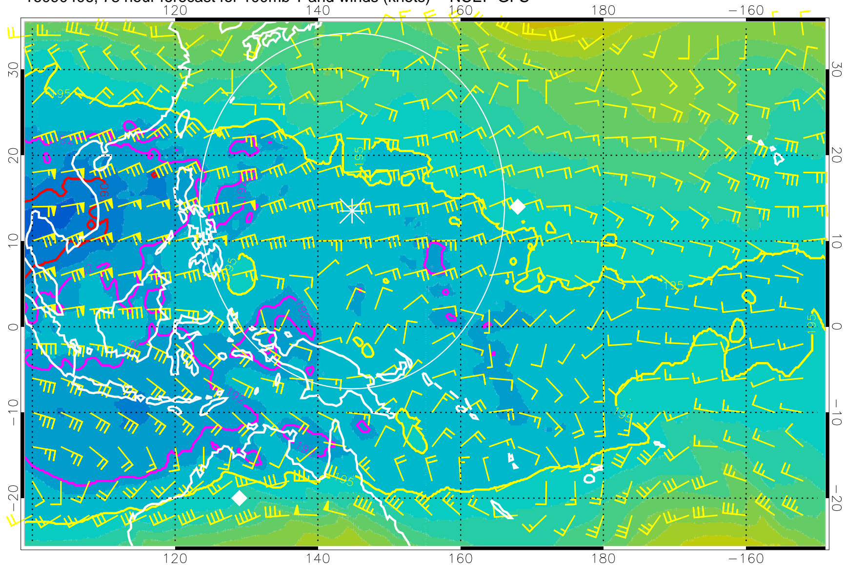
16090406, 78 hour forecast for 100mb T and winds (knots) -- NCEP GFS
