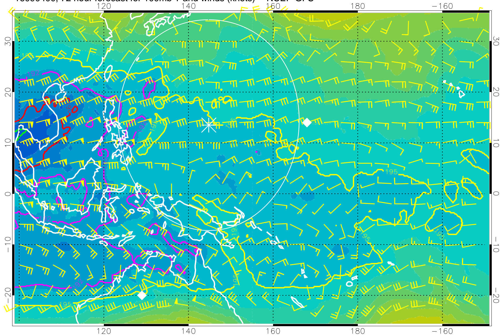
16090400, 72 hour forecast for 100mb T and winds (knots) -- NCEP GFS
