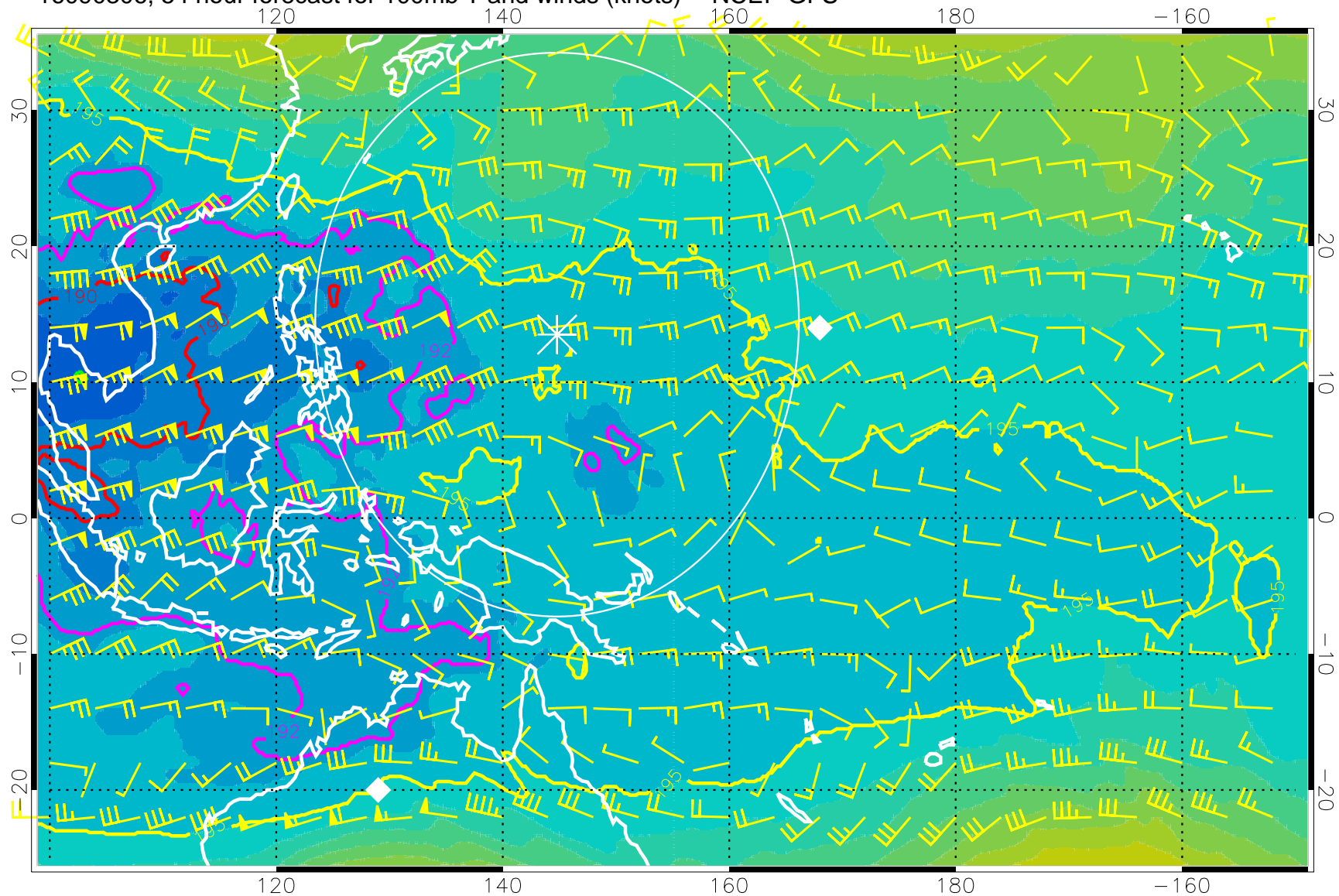
16090306, 54 hour forecast for 100mb T and winds (knots) -- NCEP GFS
