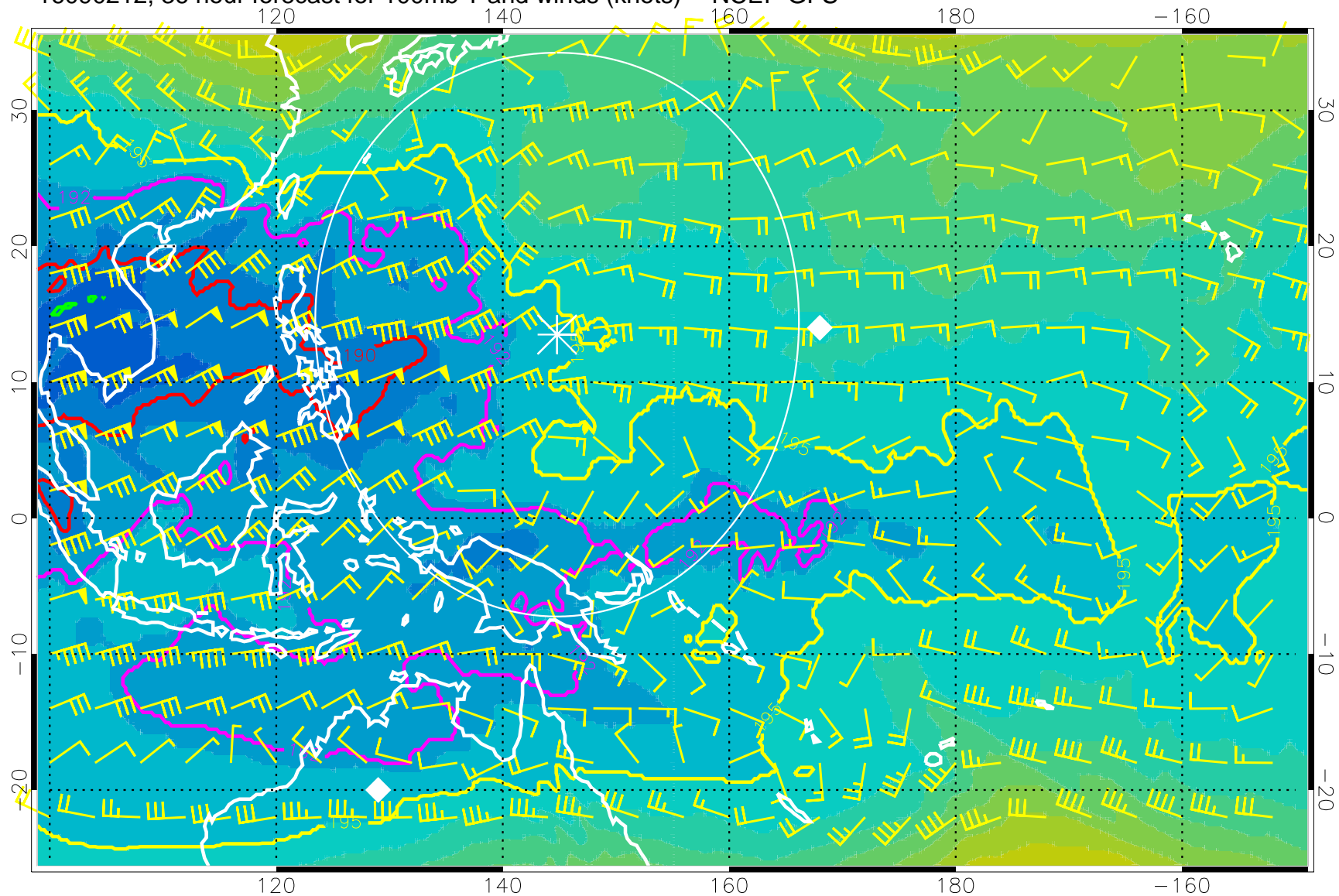
16090212, 36 hour forecast for 100mb T and winds (knots) -- NCEP GFS
