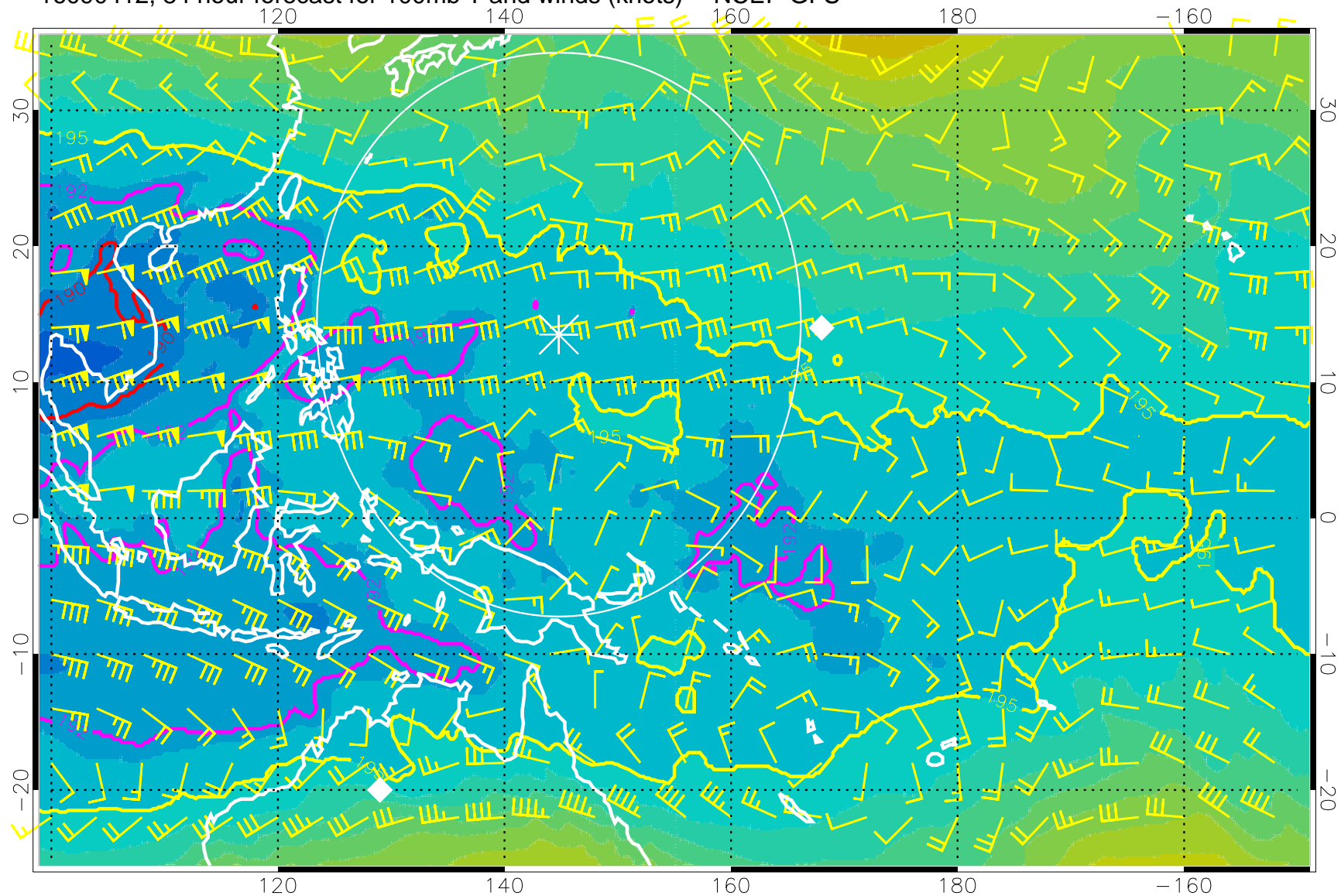
16090412, 84 hour forecast for 100mb T and winds (knots) -- NCEP GFS
