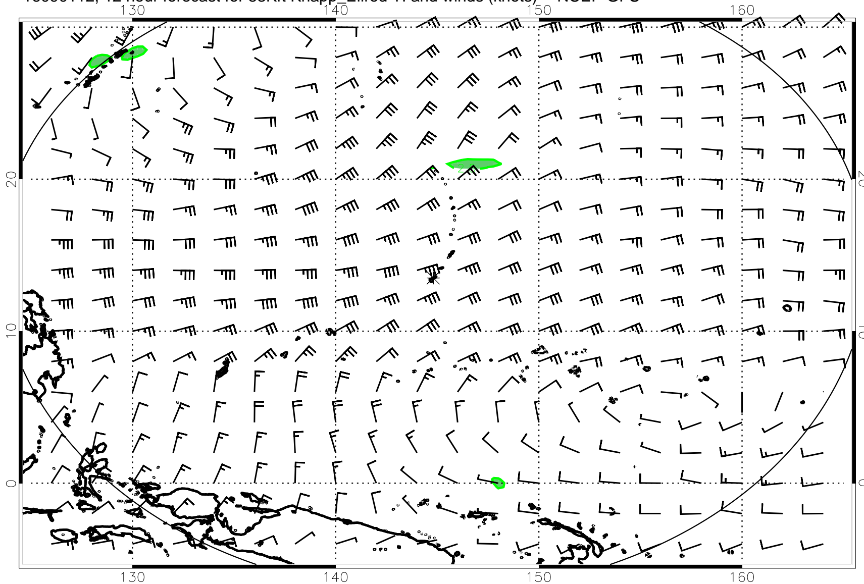
16090112, 12 hour forecast for 53Kft Knapp_Ellrod TI and winds (knots) -- NCEP GFS
