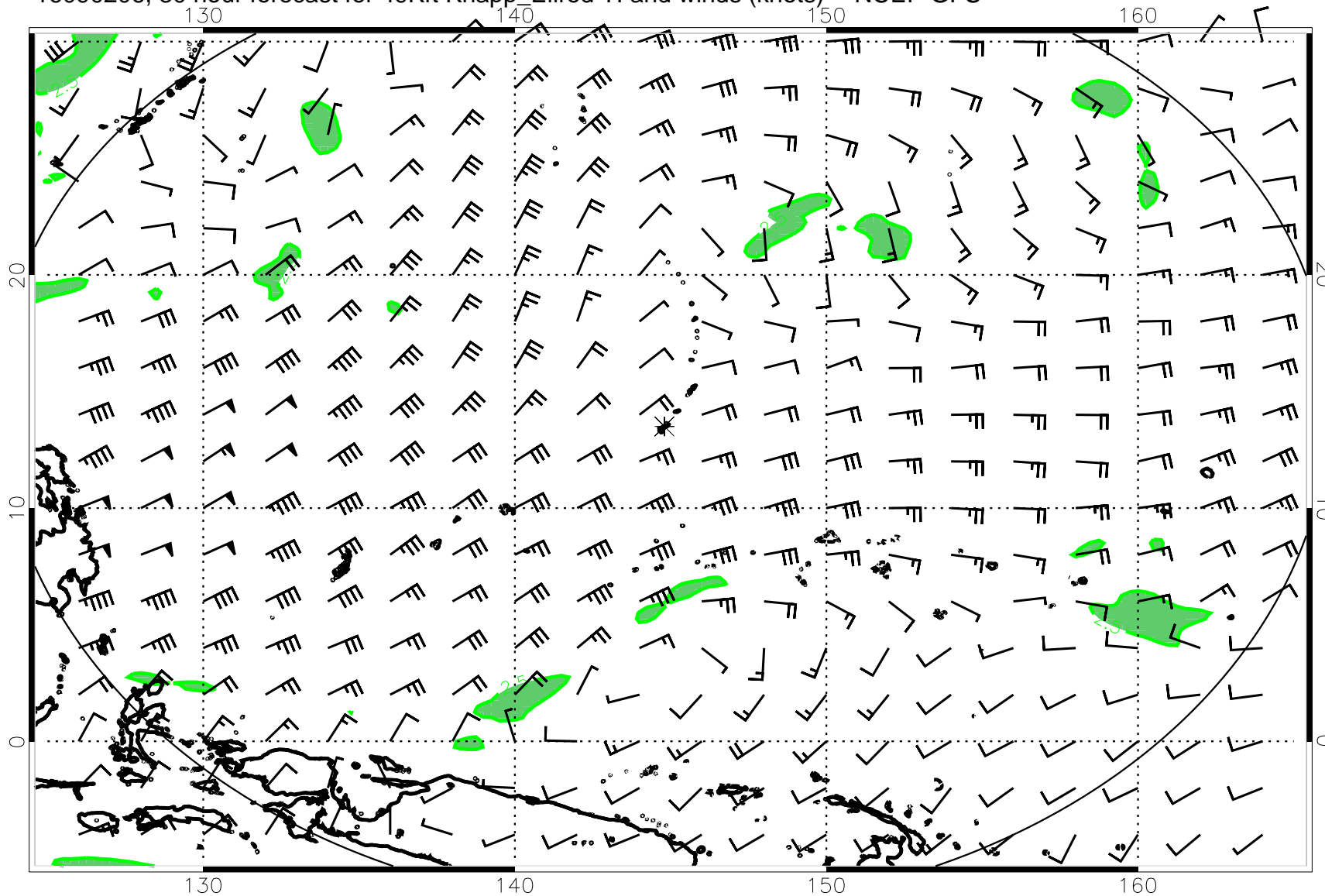
16090206, 30 hour forecast for 49Kft Knapp_Ellrod TI and winds (knots) -- NCEP GFS
