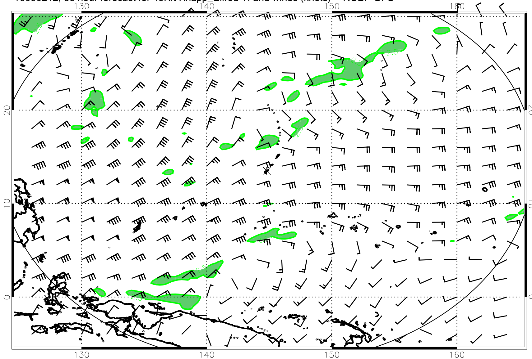
16090212, 36 hour forecast for 49Kft Knapp_Ellrod TI and winds (knots) -- NCEP GFS
