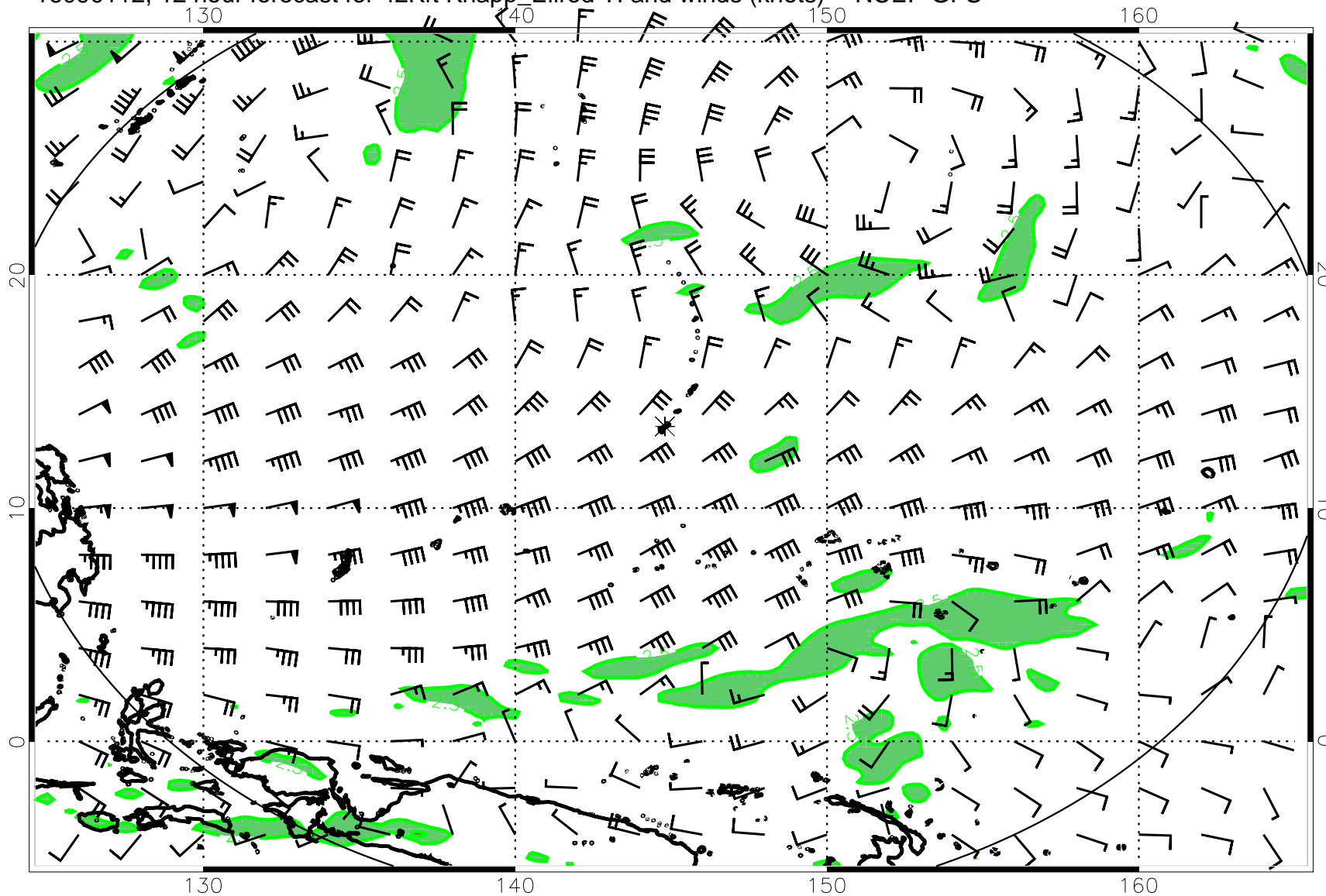
16090112, 12 hour forecast for 42Kft Knapp_Ellrod TI and winds (knots) -- NCEP GFS
