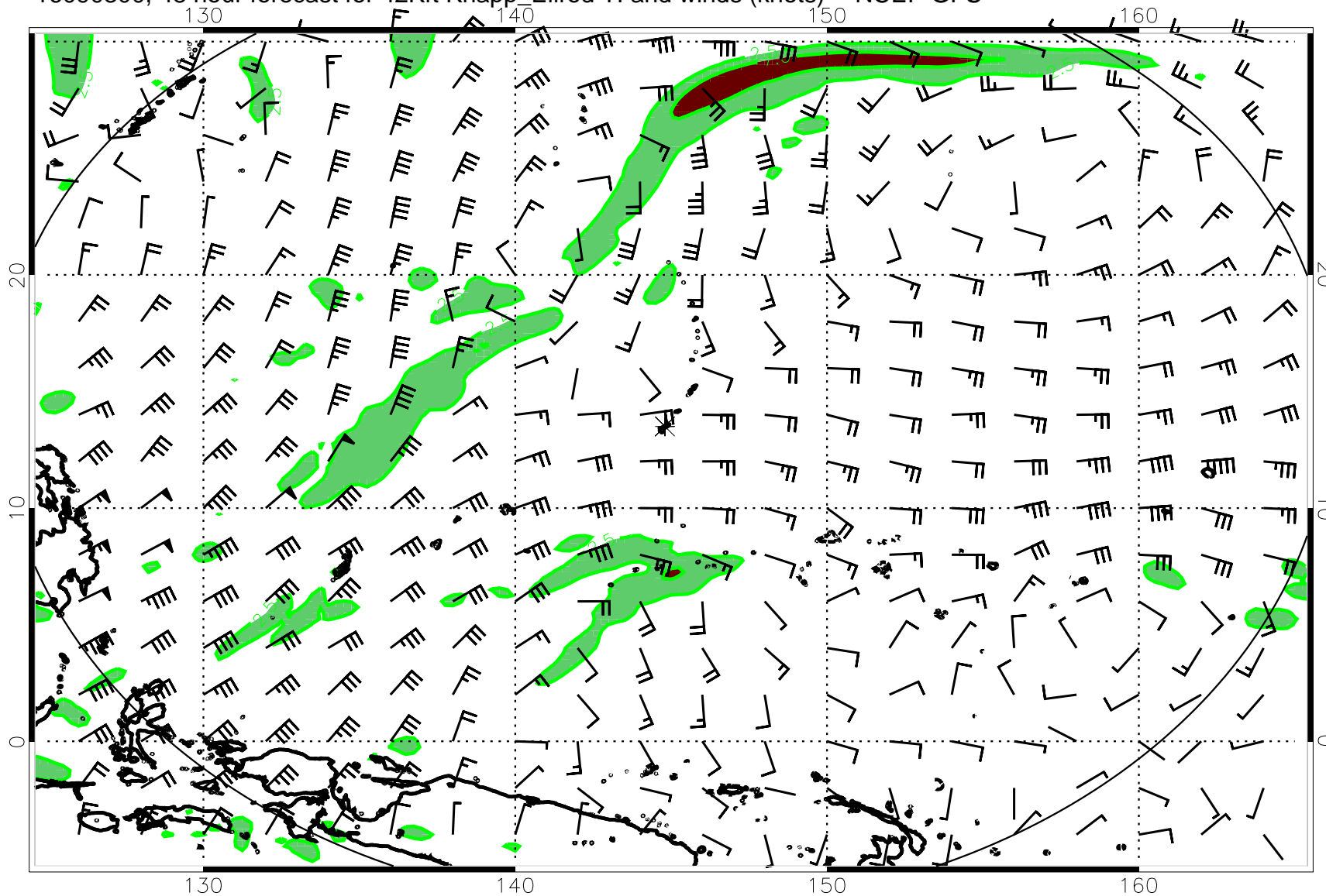
16090300, 48 hour forecast for 42Kft Knapp_Ellrod TI and winds (knots) -- NCEP GFS
