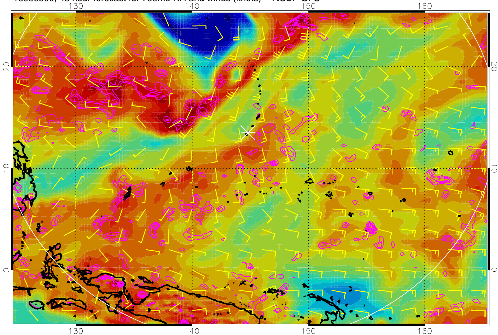
16090300, 48 hour forecast for 700mb RH and winds (knots) -- NCEP GFS
