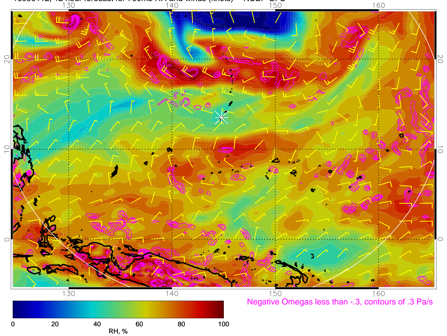
16090112, 12 hour forecast for 700mb RH and winds (knots) -- NCEP GFS
