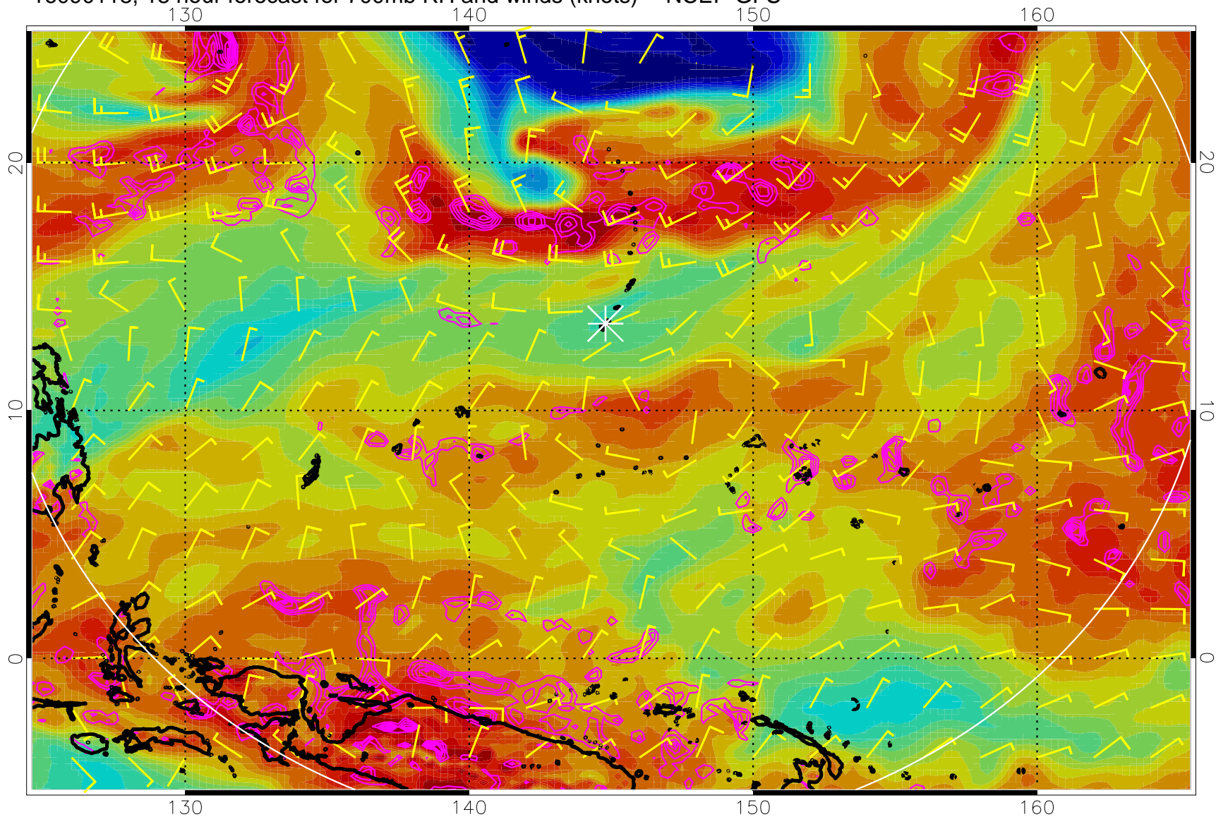
16090118, 18 hour forecast for 700mb RH and winds (knots) -- NCEP GFS
