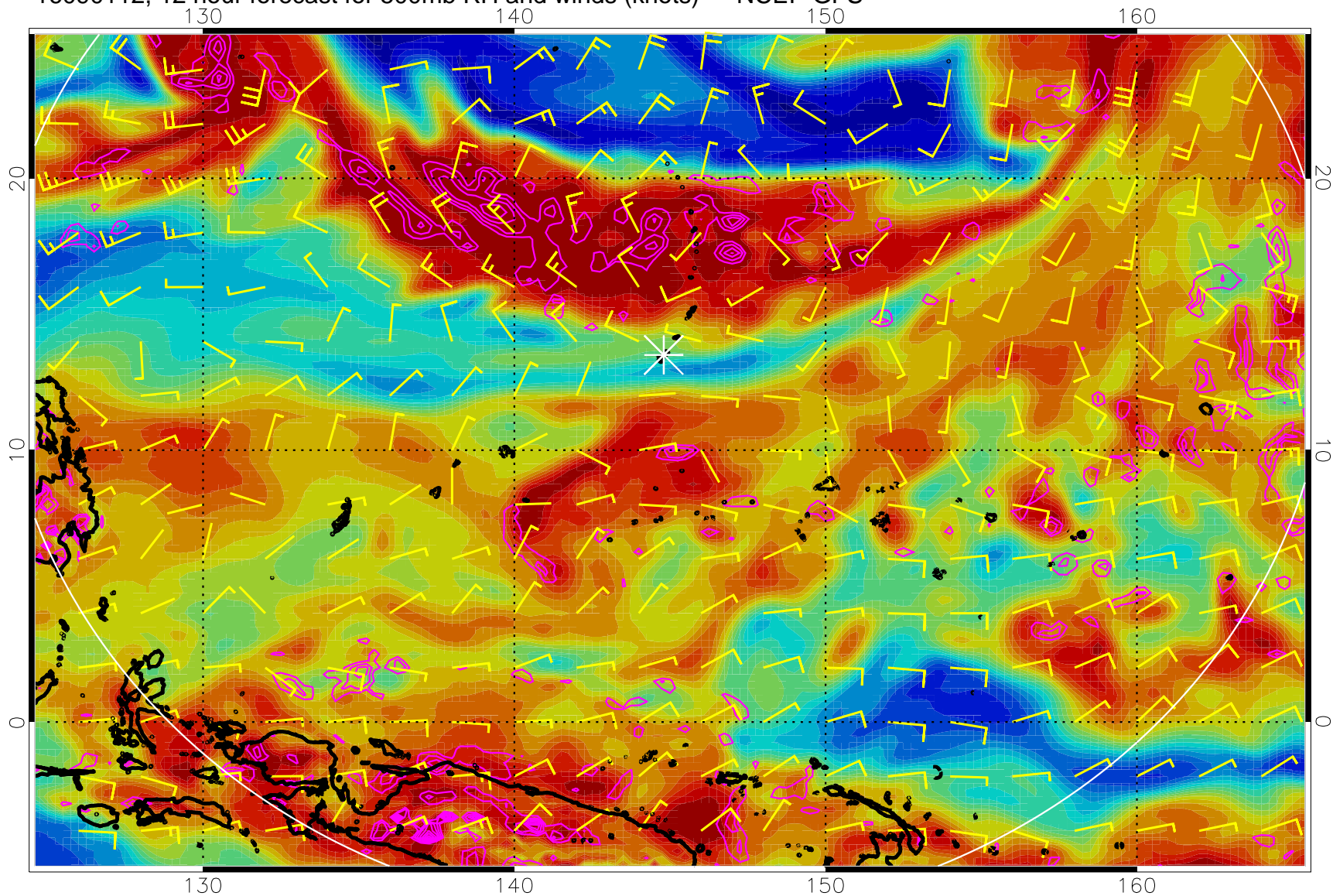
16090112, 12 hour forecast for 500mb RH and winds (knots) -- NCEP GFS
