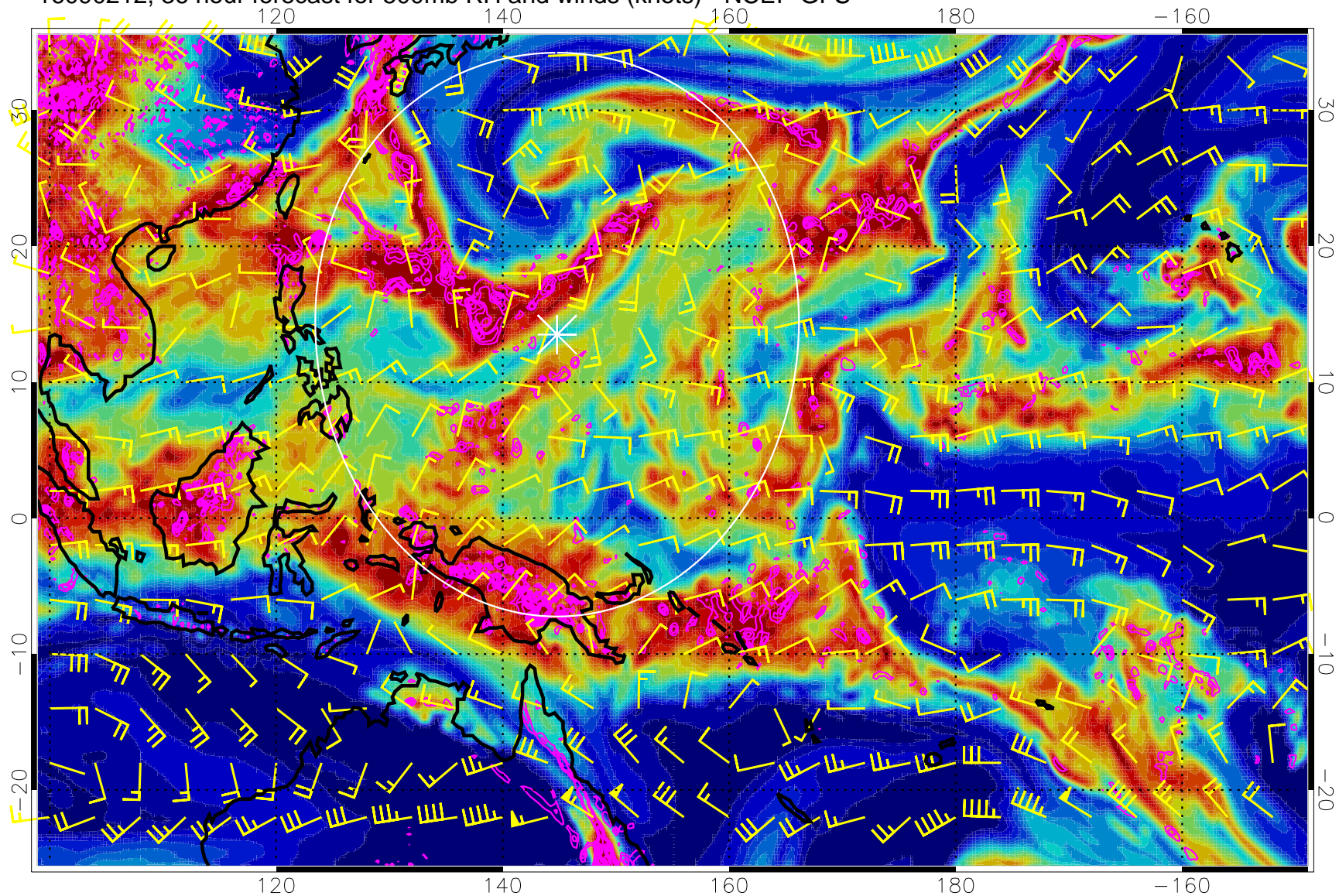
16090212, 36 hour forecast for 500mb RH and winds (knots) - NCEP GFS
