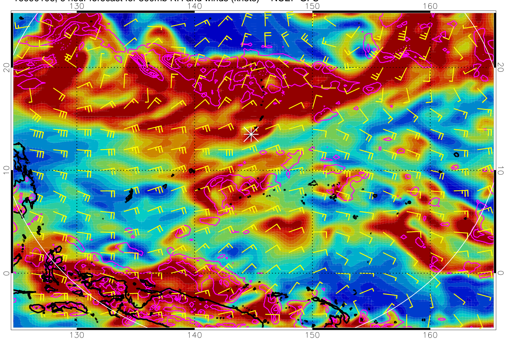
16090106, 6 hour forecast for 300mb RH and winds (knots) -- NCEP GFS
