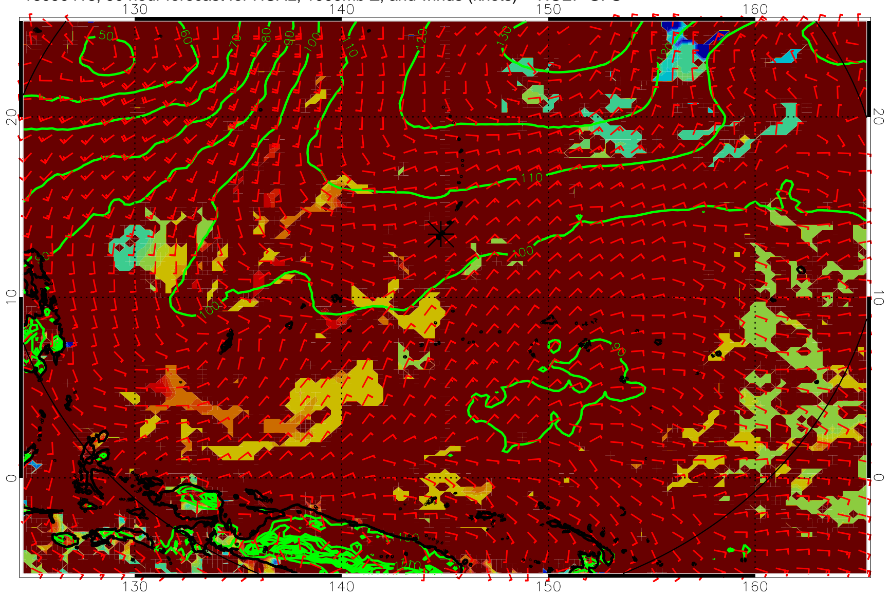
16090418, 90 hour forecast for HCAL, 1000mb Z, and winds (knots) -- NCEP GFS
