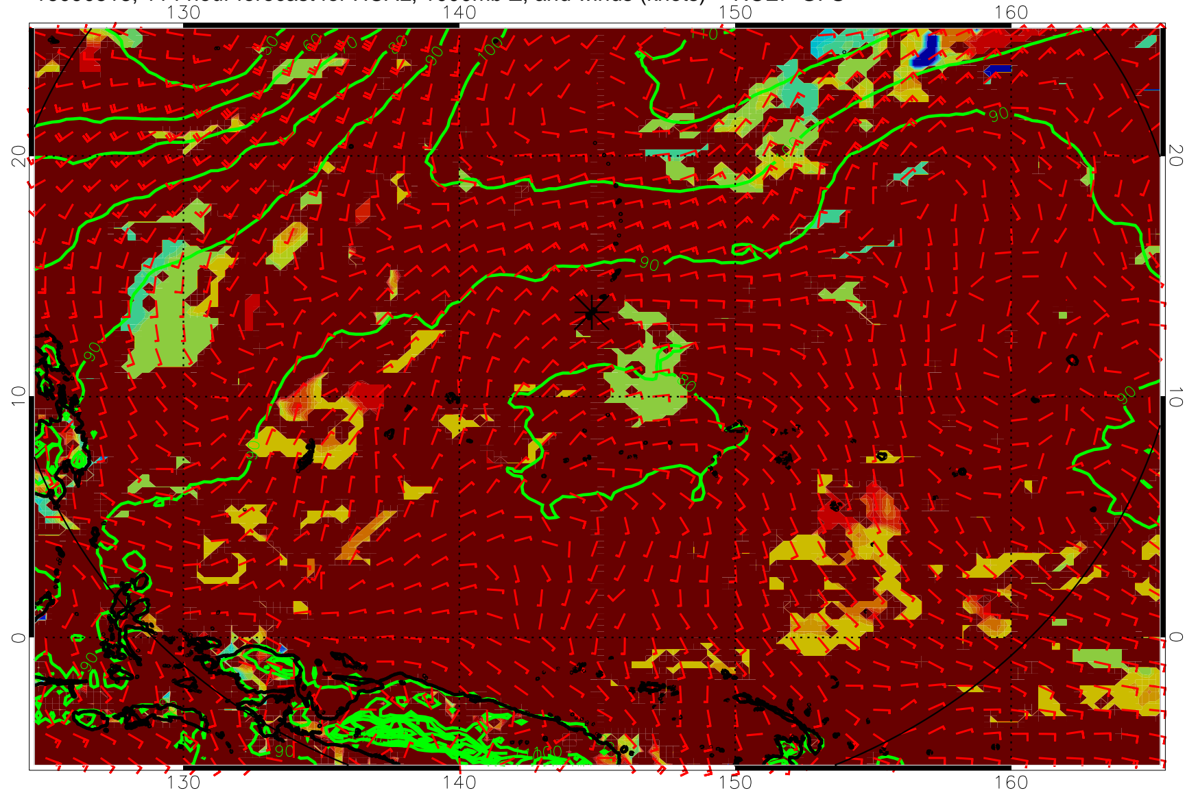
16090518, 114 hour forecast for HCAL, 1000mb Z, and winds (knots) -- NCEP GFS
