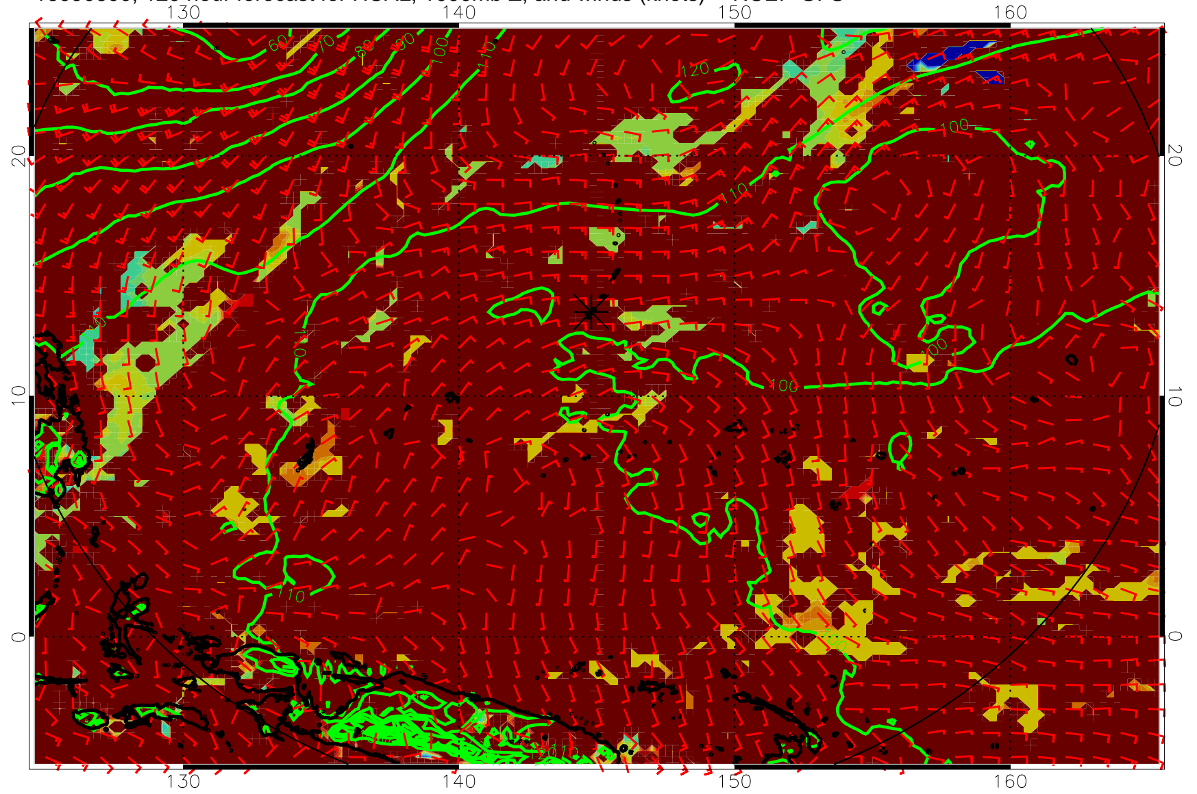
16090600, 120 hour forecast for HCAL, 1000mb Z, and winds (knots) -- NCEP GFS
