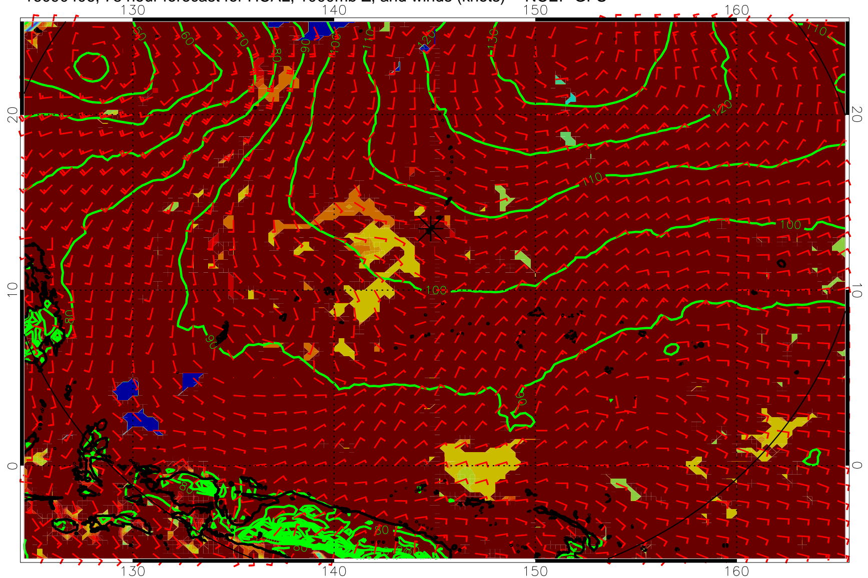
16090406, 78 hour forecast for HCAL, 1000mb Z, and winds (knots) -- NCEP GFS
