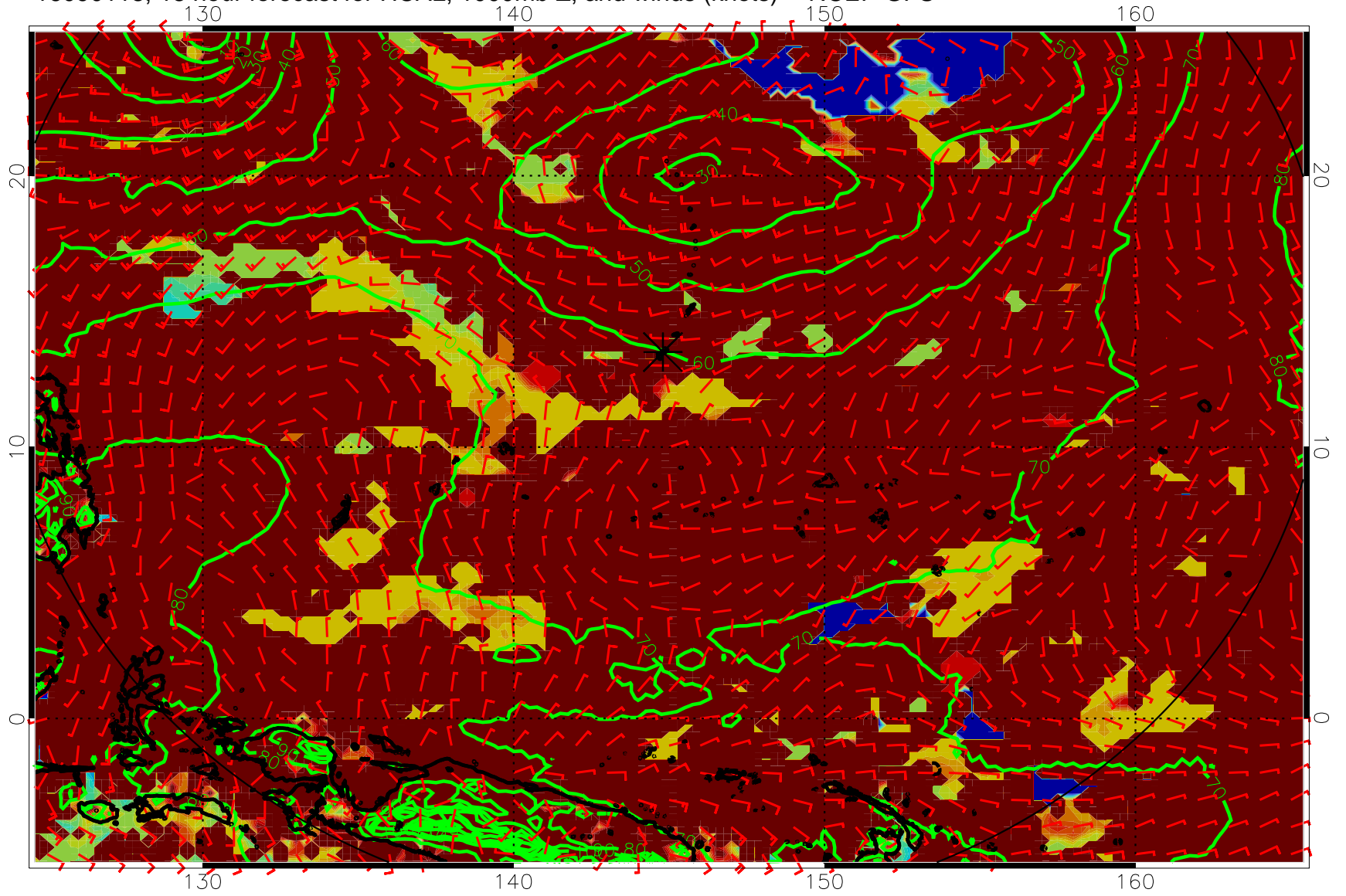
16090118, 18 hour forecast for HCAL, 1000mb Z, and winds (knots) -- NCEP GFS
