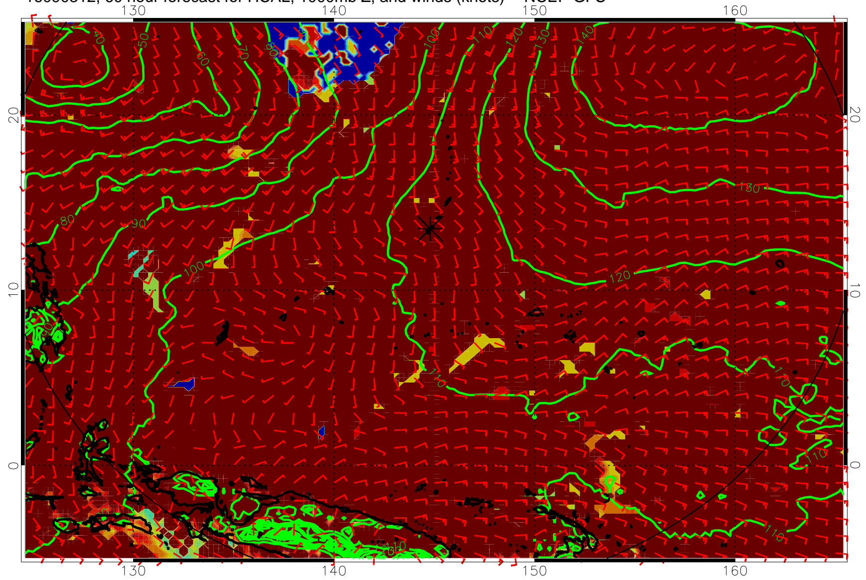
16090312, 60 hour forecast for HCAL, 1000mb Z, and winds (knots) -- NCEP GFS
