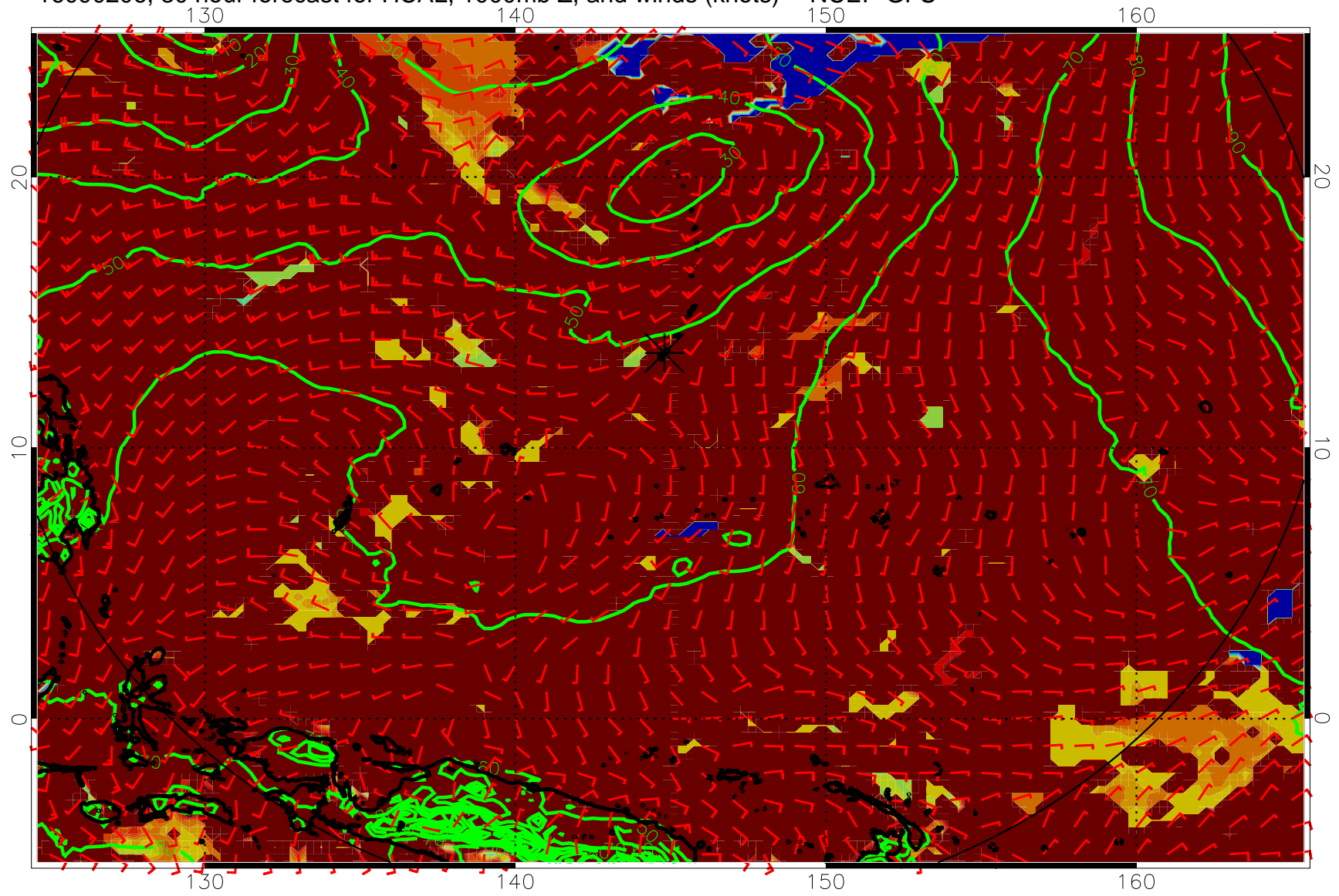
16090206, 30 hour forecast for HCAL, 1000mb Z, and winds (knots) -- NCEP GFS
