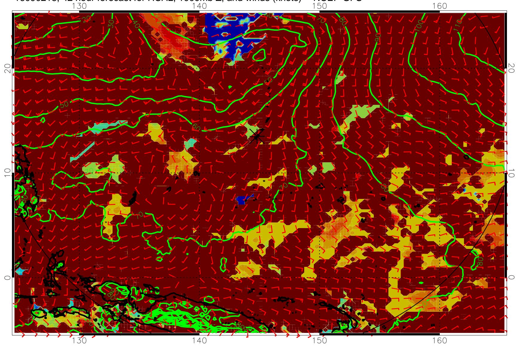
16090218, 42 hour forecast for HCAL, 1000mb Z, and winds (knots) -- NCEP GFS
