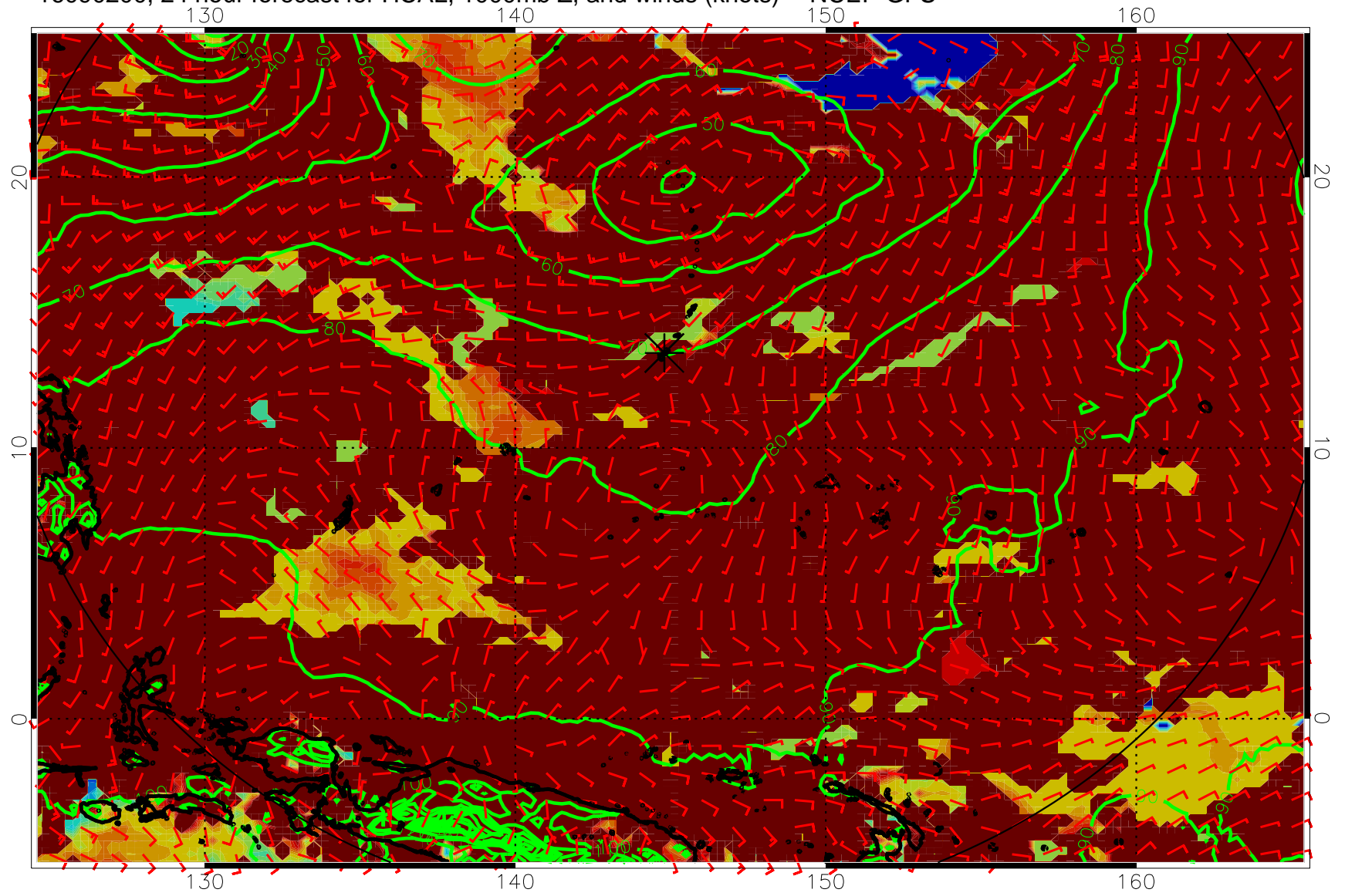
16090200, 24 hour forecast for HCAL, 1000mb Z, and winds (knots) -- NCEP GFS
