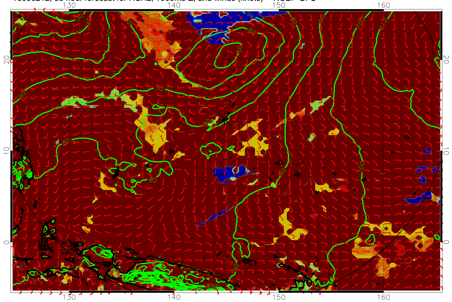
16090212, 36 hour forecast for HCAL, 1000mb Z, and winds (knots) -- NCEP GFS
