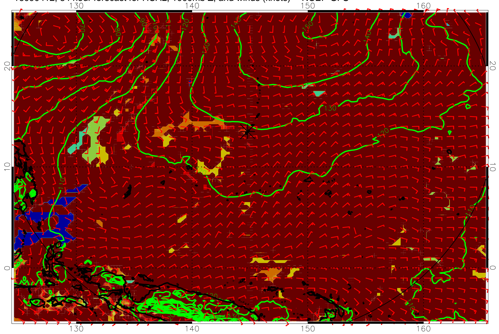
16090412, 84 hour forecast for HCAL, 1000mb Z, and winds (knots) -- NCEP GFS
