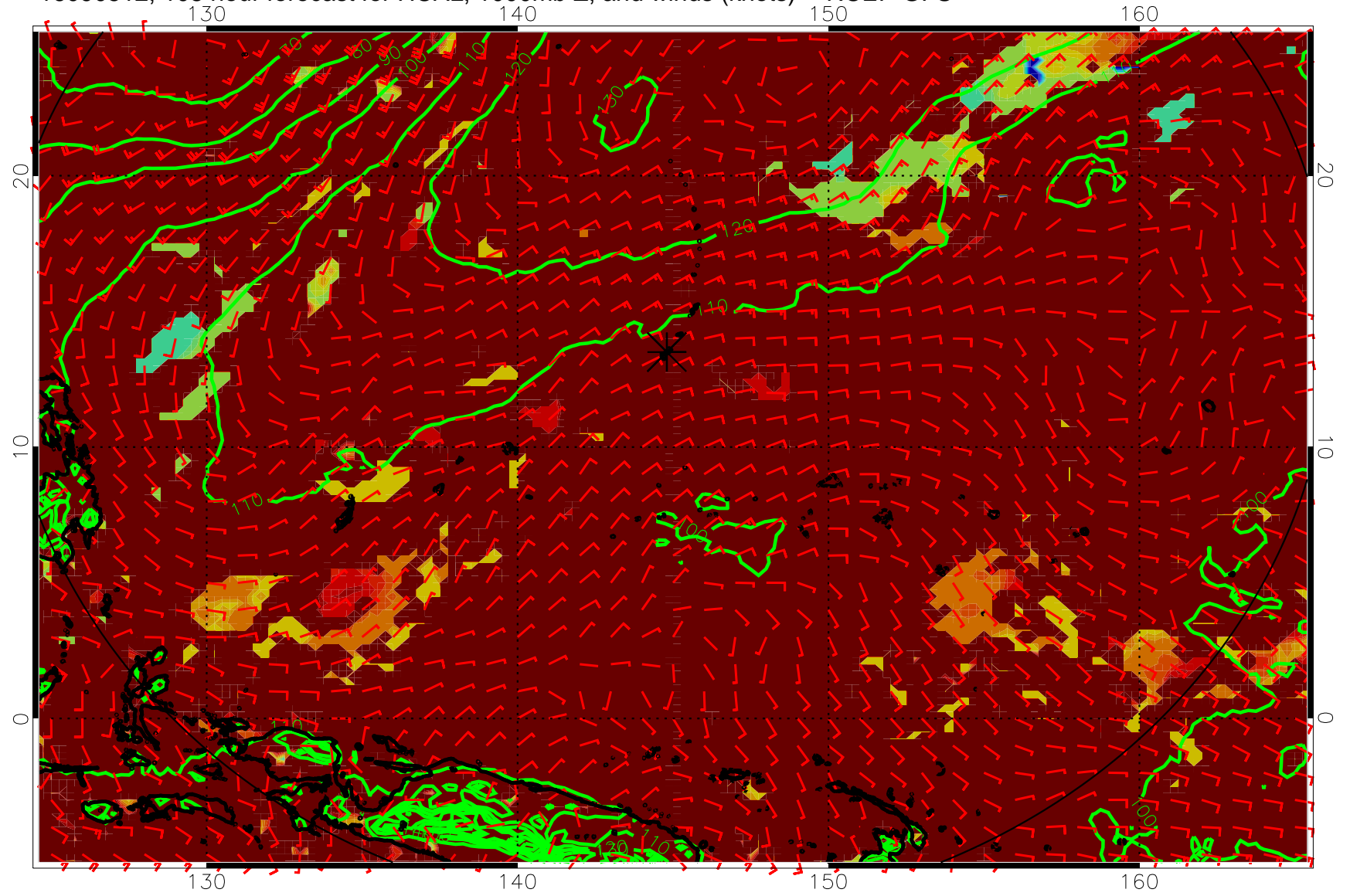
16090512, 108 hour forecast for HCAL, 1000mb Z, and winds (knots) -- NCEP GFS
