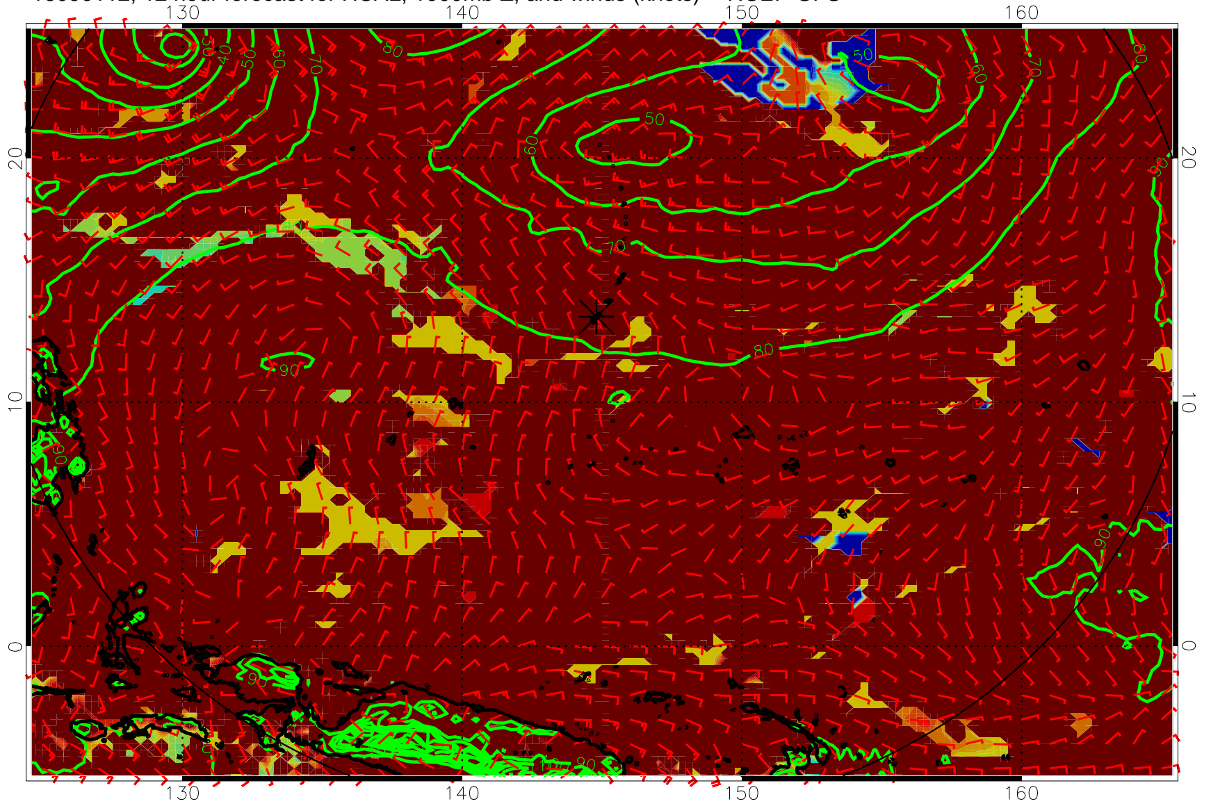
16090112, 12 hour forecast for HCAL, 1000mb Z, and winds (knots) -- NCEP GFS
