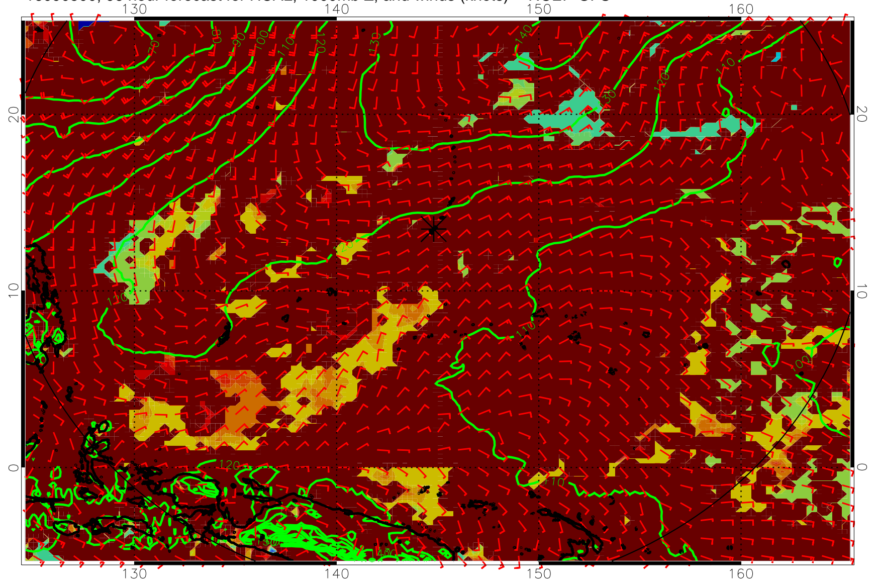
16090500, 96 hour forecast for HCAL, 1000mb Z, and winds (knots) -- NCEP GFS
