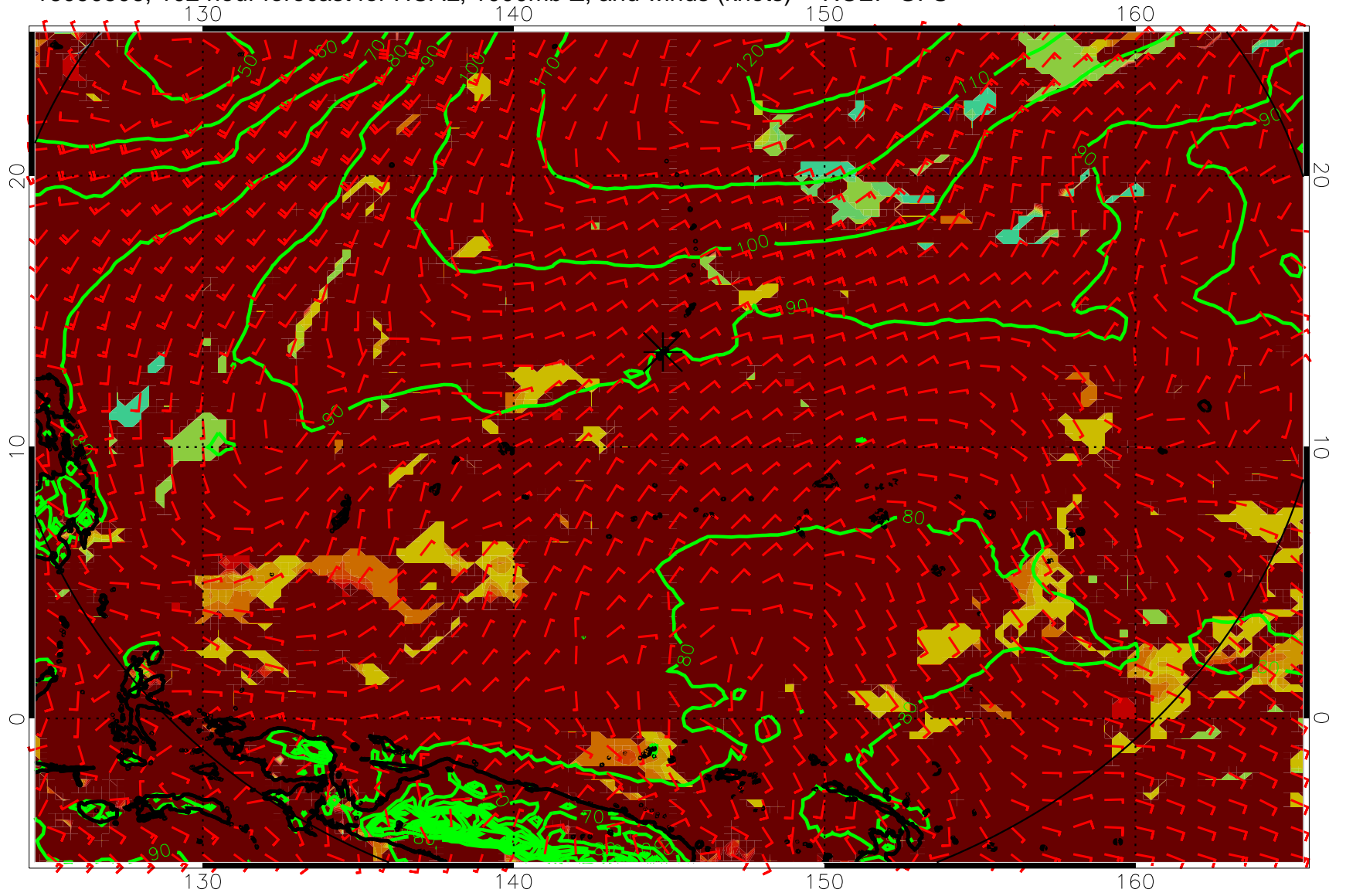
16090506, 102 hour forecast for HCAL, 1000mb Z, and winds (knots) -- NCEP GFS
