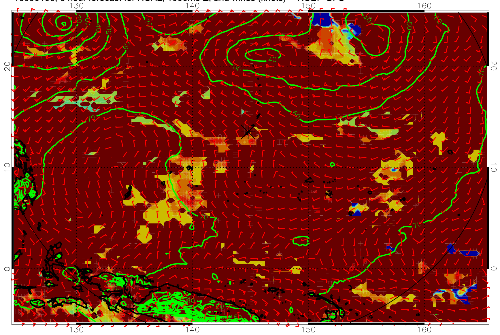
16090106, 6 hour forecast for HCAL, 1000mb Z, and winds (knots) -- NCEP GFS
