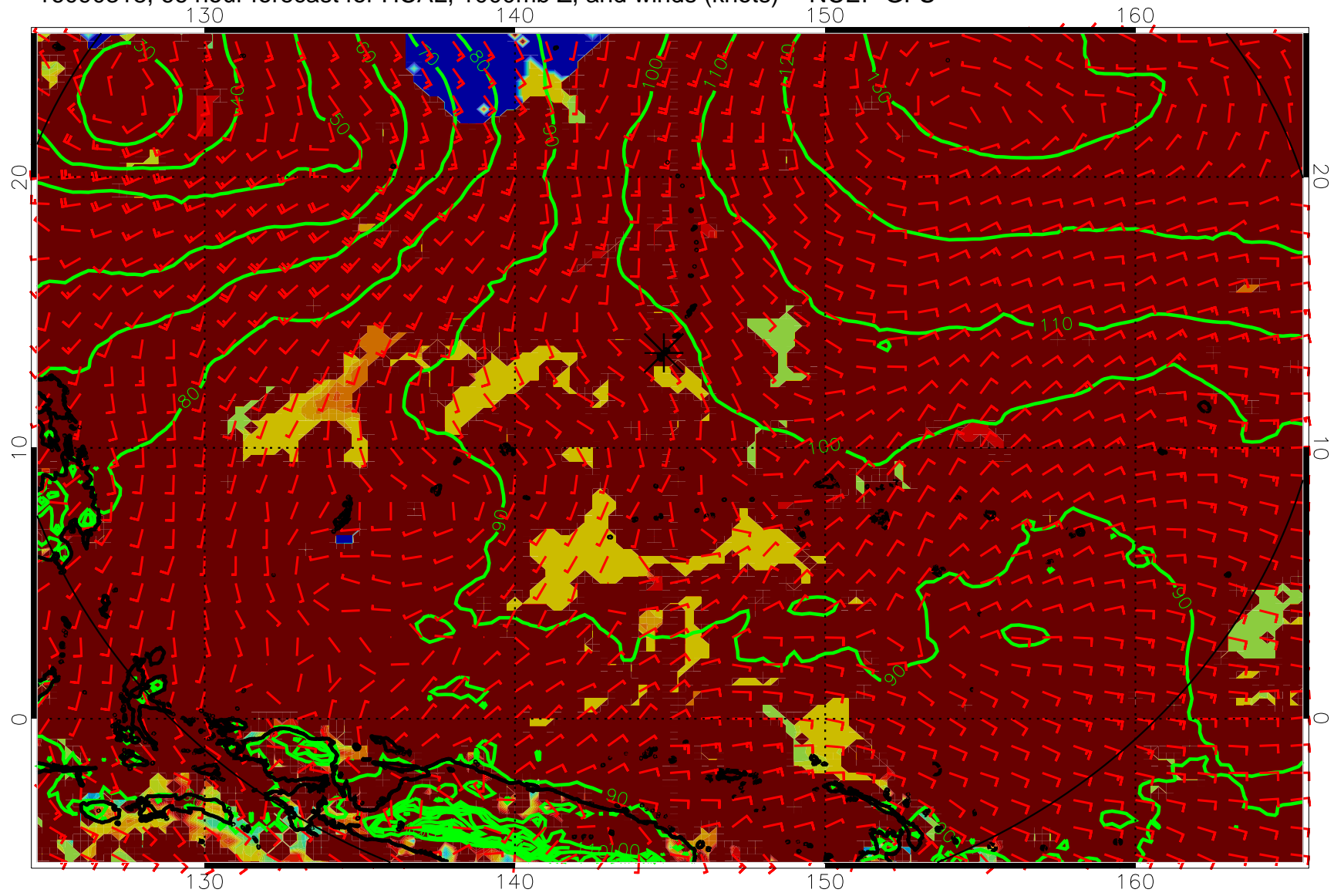
16090318, 66 hour forecast for HCAL, 1000mb Z, and winds (knots) -- NCEP GFS
