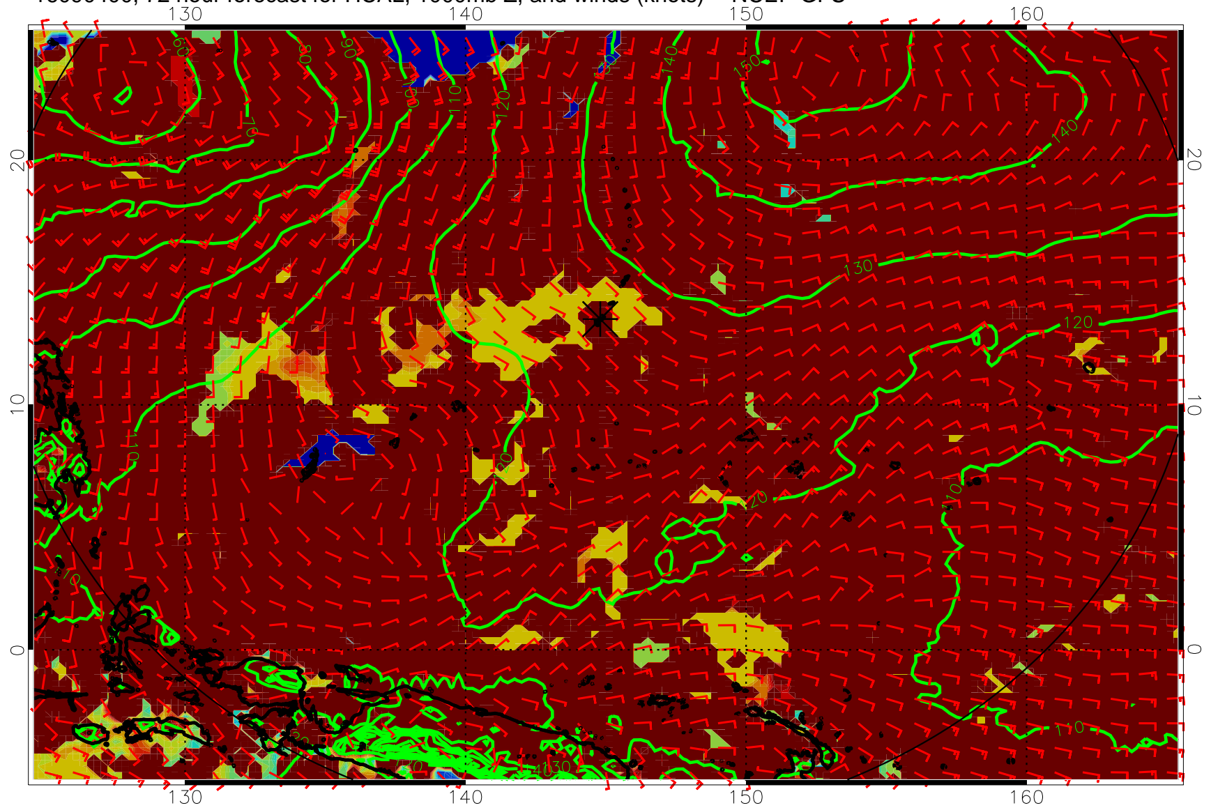
16090400, 72 hour forecast for HCAL, 1000mb Z, and winds (knots) -- NCEP GFS
