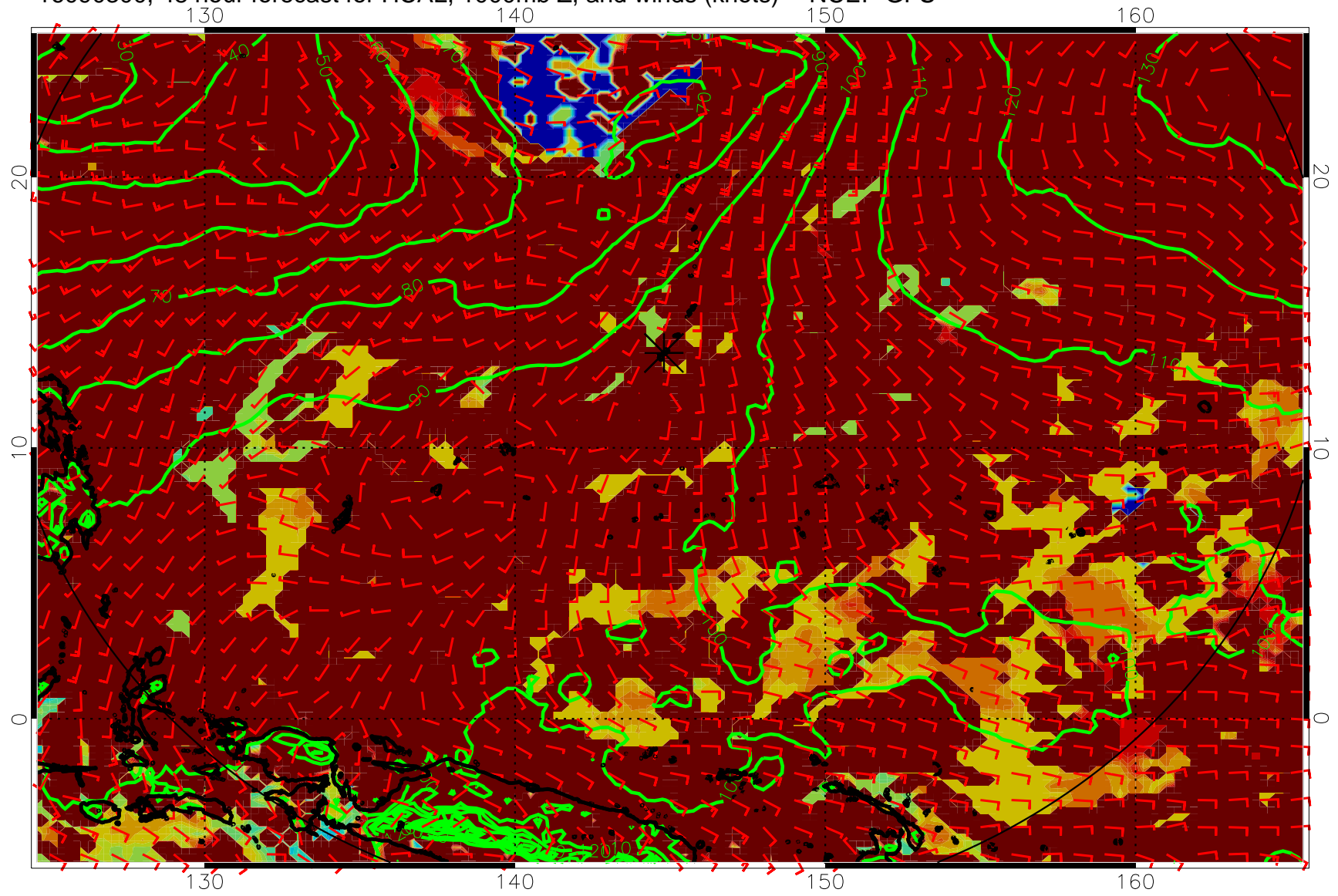
16090300, 48 hour forecast for HCAL, 1000mb Z, and winds (knots) -- NCEP GFS
