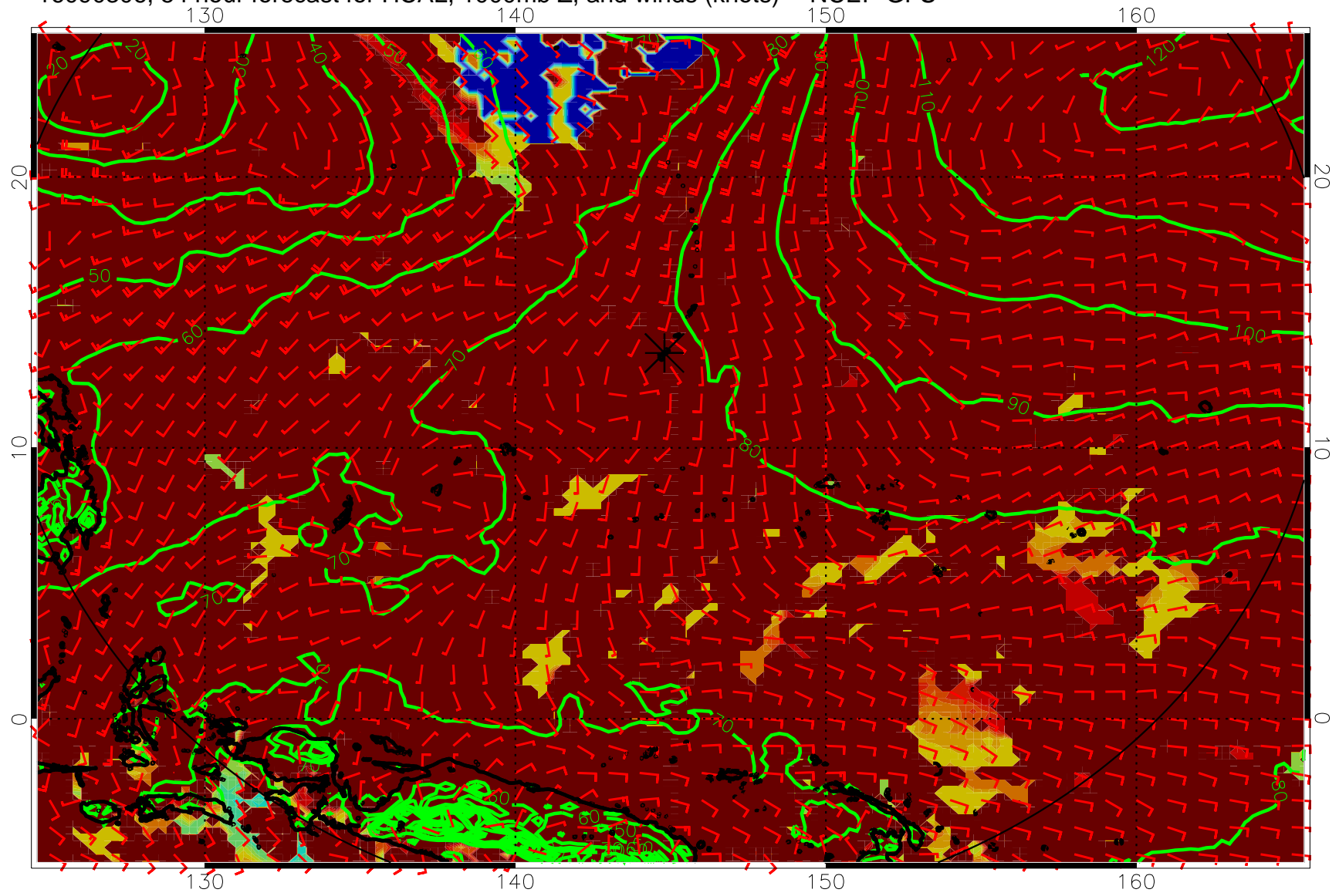
16090306, 54 hour forecast for HCAL, 1000mb Z, and winds (knots) -- NCEP GFS
