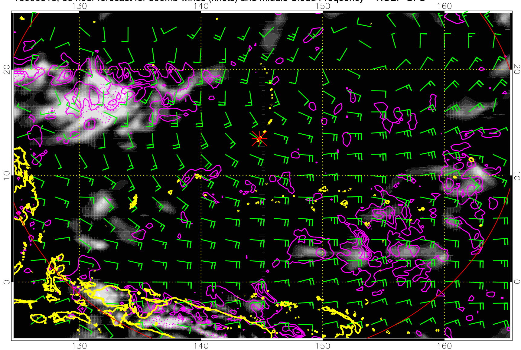
16090318, 66 hour forecast for 500mb winds (knots) and Middle Cloud Frequency -- NCEP GFS
