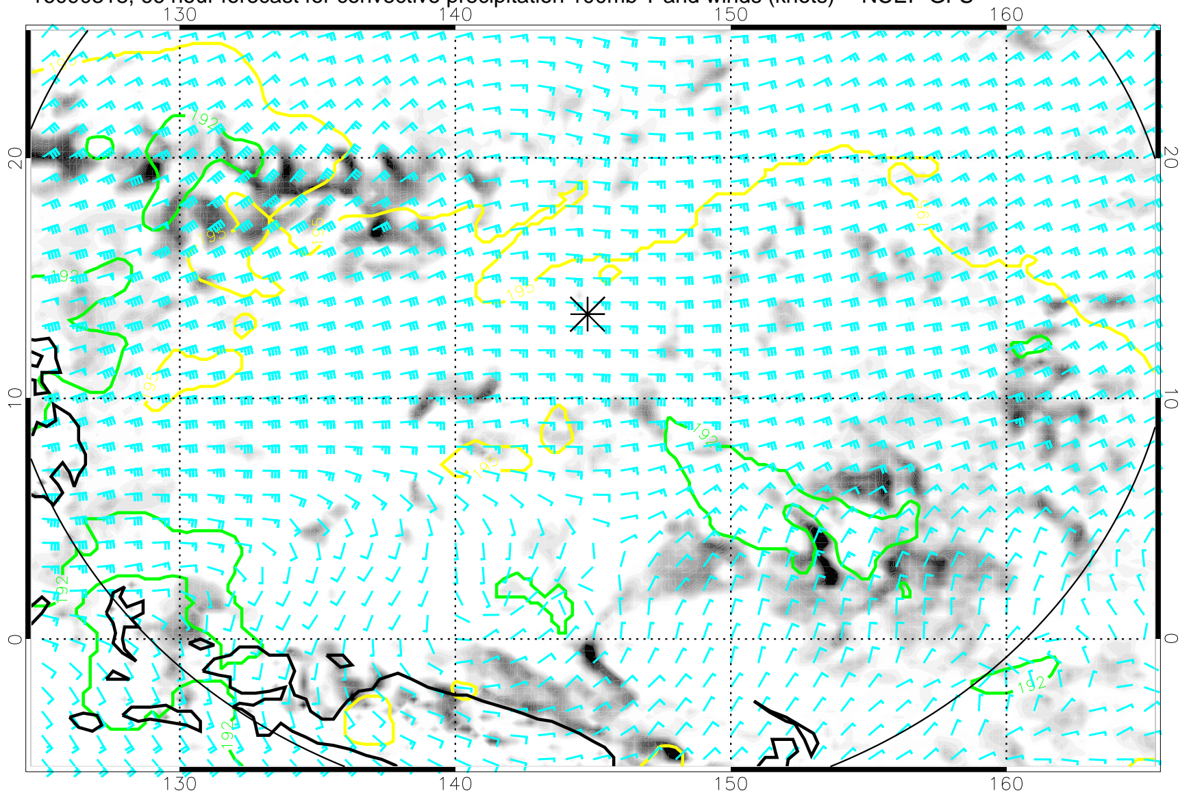
16090318, 66 hour forecast for convective precipitation 100mb T and winds (knots) -- NCEP GFS
