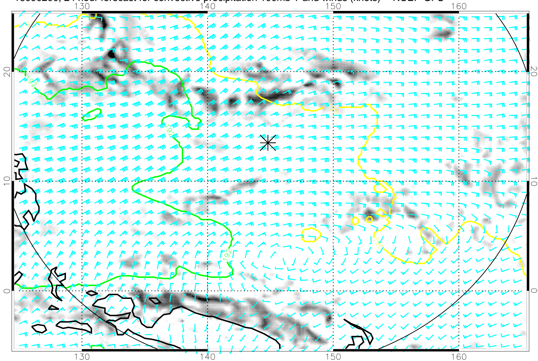
16090200, 24 hour forecast for convective precipitation 100mb T and winds (knots) -- NCEP GFS
