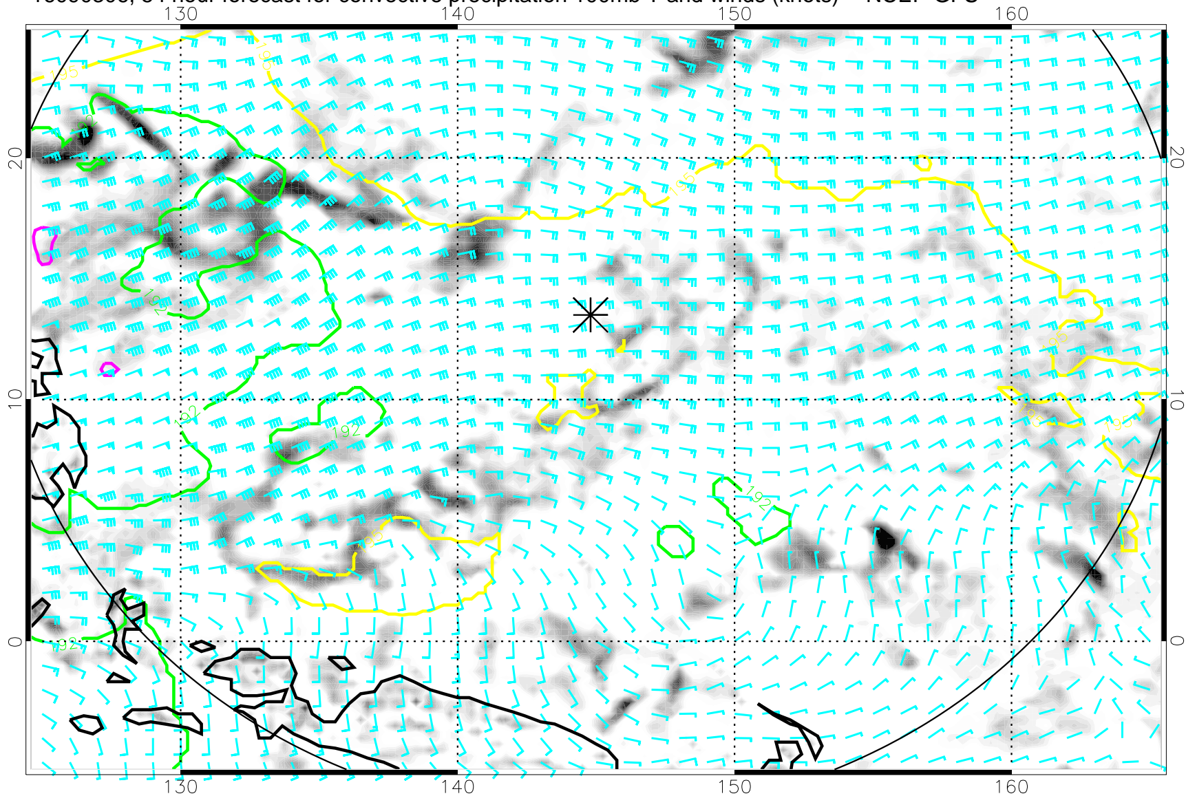
16090306, 54 hour forecast for convective precipitation 100mb T and winds (knots) -- NCEP GFS
