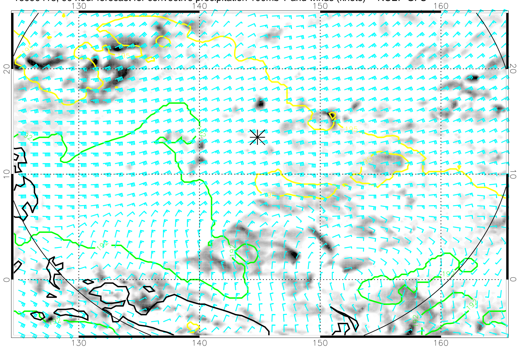
16090418, 90 hour forecast for convective precipitation 100mb T and winds (knots) -- NCEP GFS
