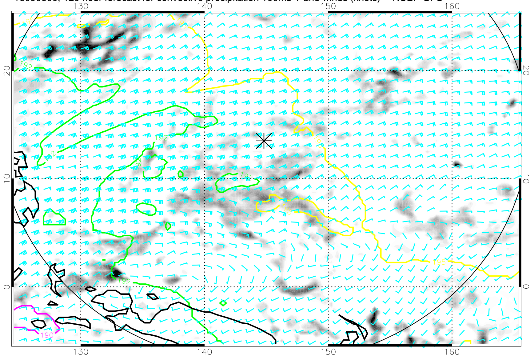
16090600, 120 hour forecast for convective precipitation 100mb T and winds (knots) -- NCEP GFS
