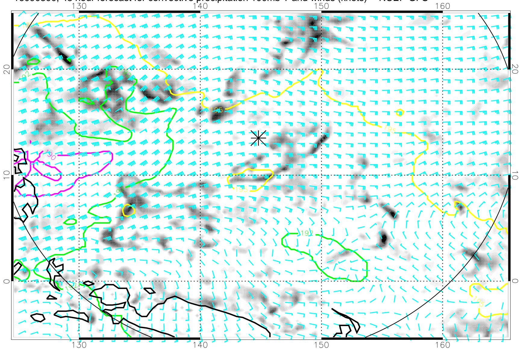
16090300, 48 hour forecast for convective precipitation 100mb T and winds (knots) -- NCEP GFS
