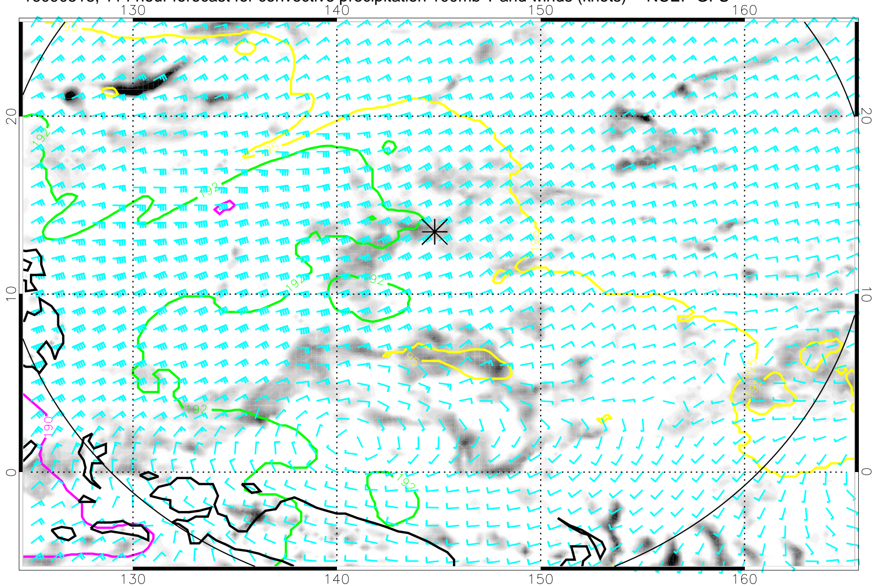
16090518, 114 hour forecast for convective precipitation 100mb T and winds (knots) -- NCEP GFS
