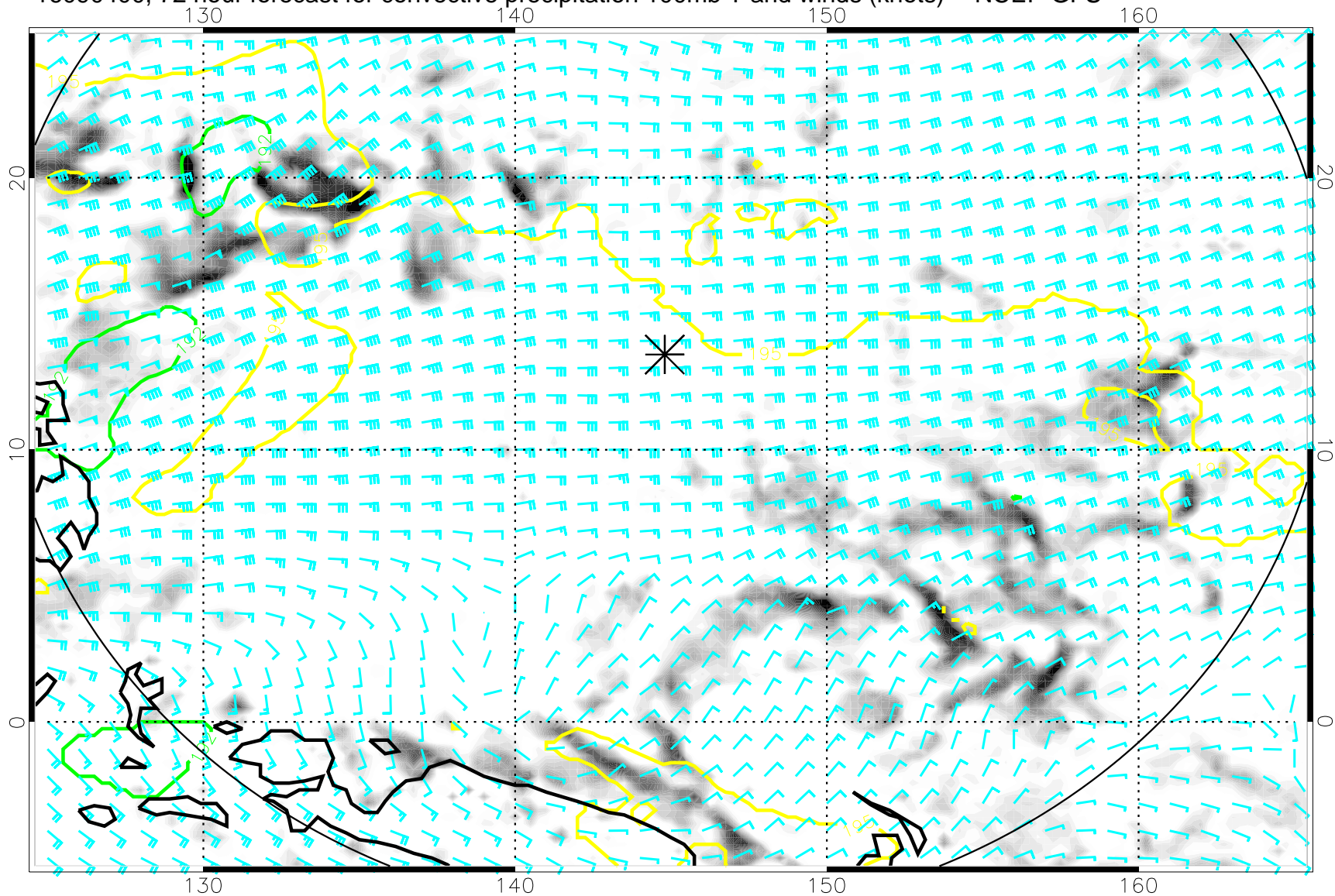
16090400, 72 hour forecast for convective precipitation 100mb T and winds (knots) -- NCEP GFS
