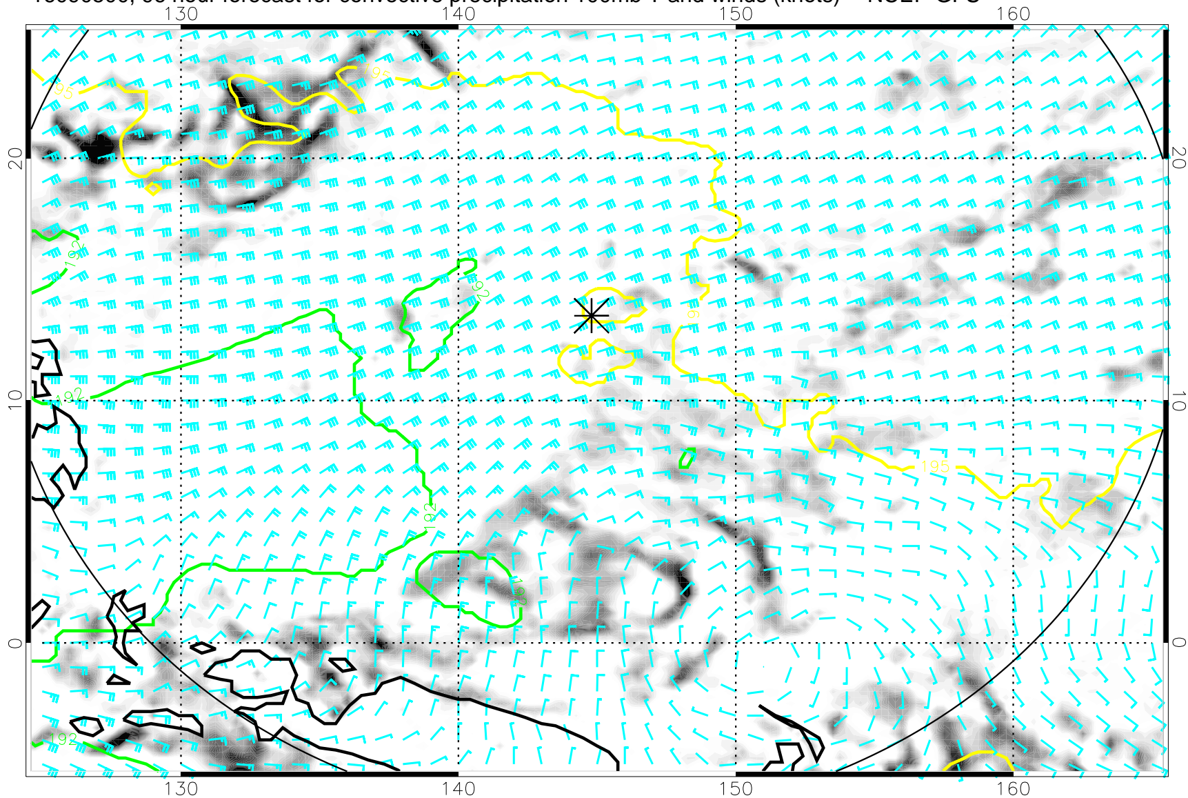
16090500, 96 hour forecast for convective precipitation 100mb T and winds (knots) -- NCEP GFS
