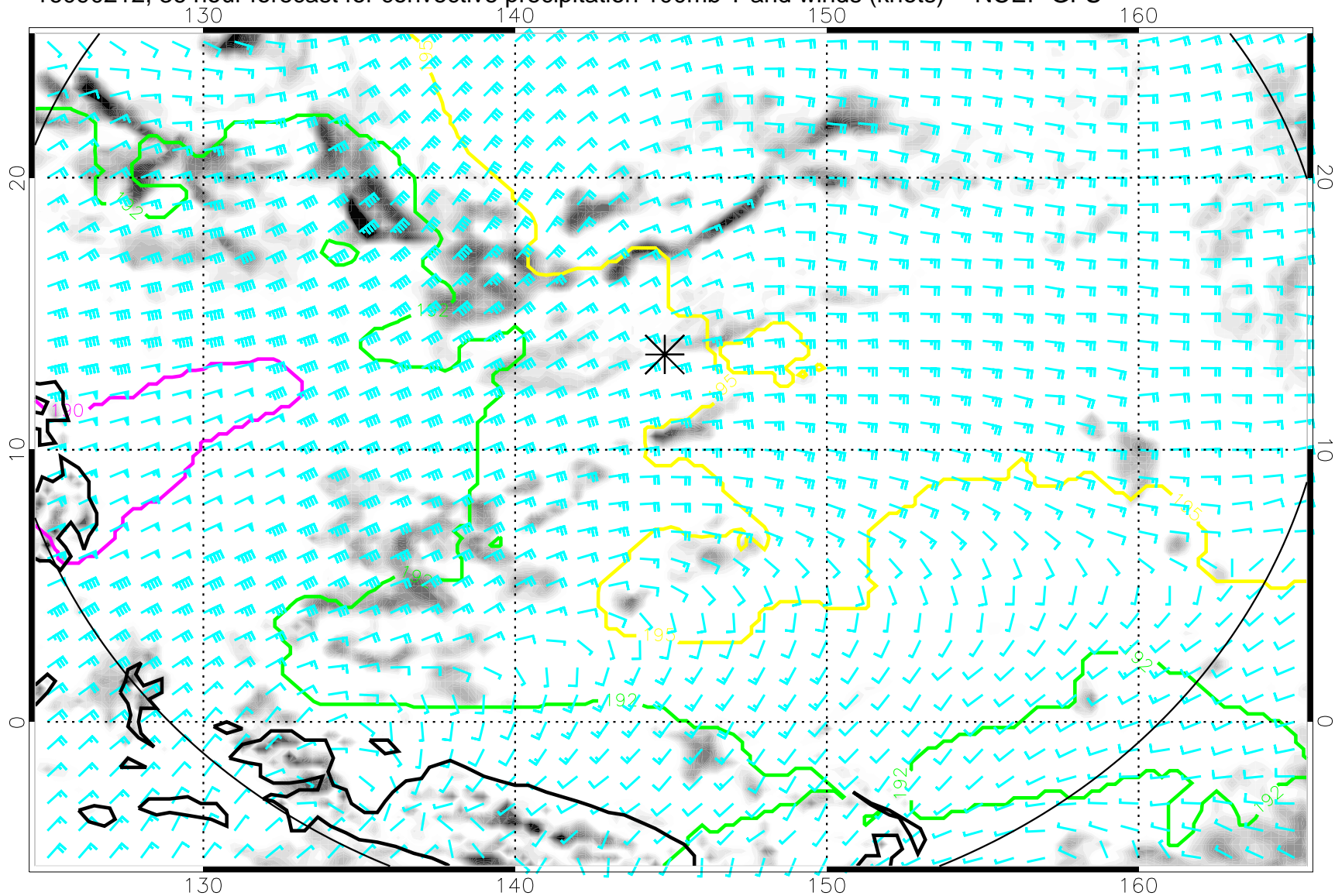
16090212, 36 hour forecast for convective precipitation 100mb T and winds (knots) -- NCEP GFS
