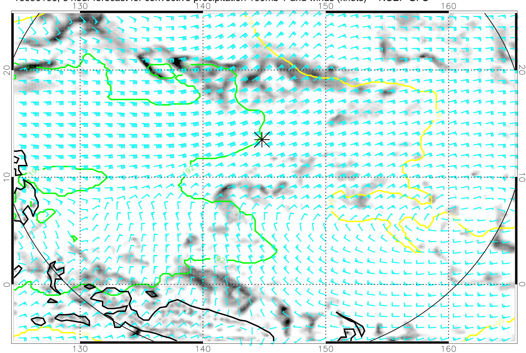
16090106, 6 hour forecast for convective precipitation 100mb T and winds (knots) -- NCEP GFS
