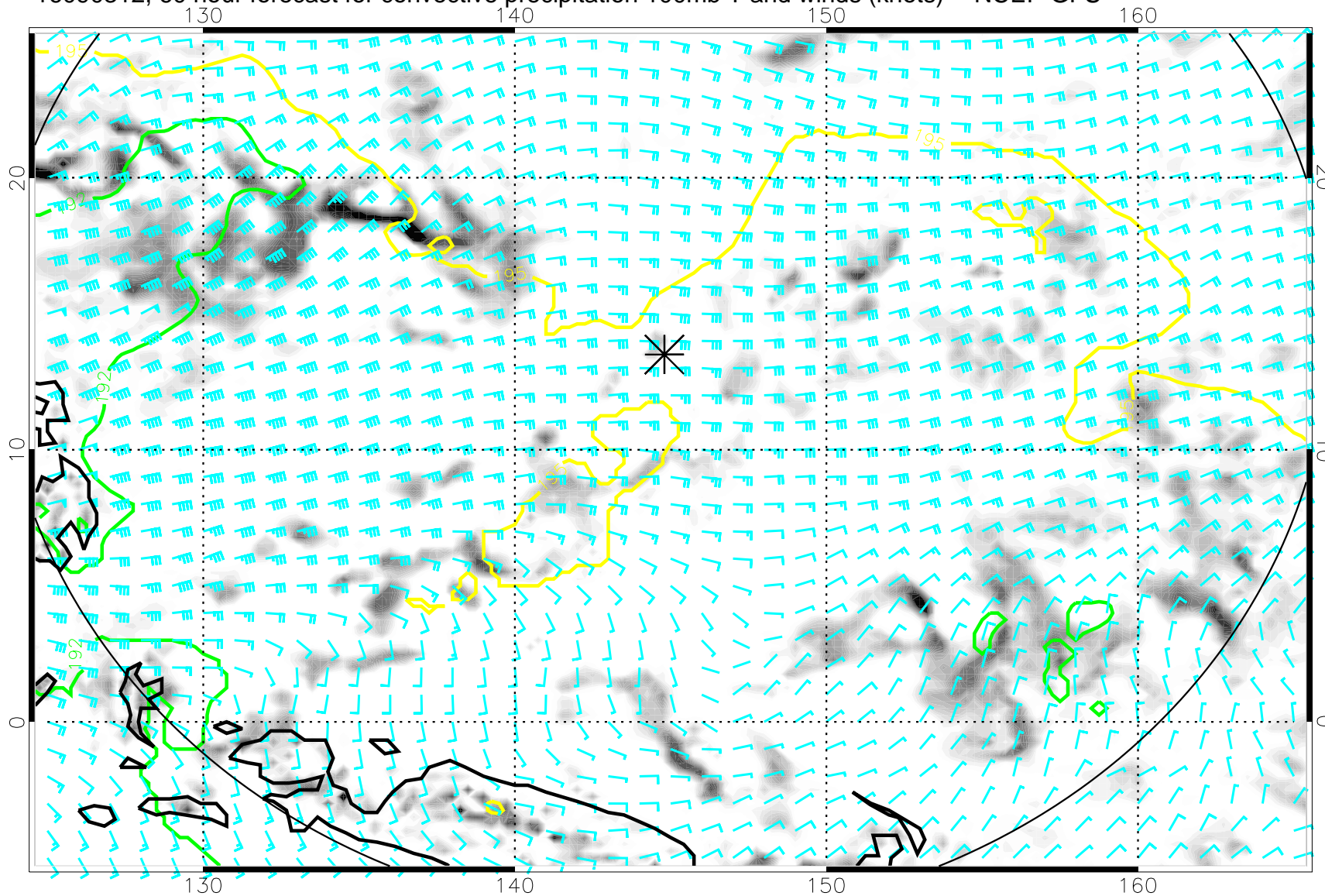
16090312, 60 hour forecast for convective precipitation 100mb T and winds (knots) -- NCEP GFS
