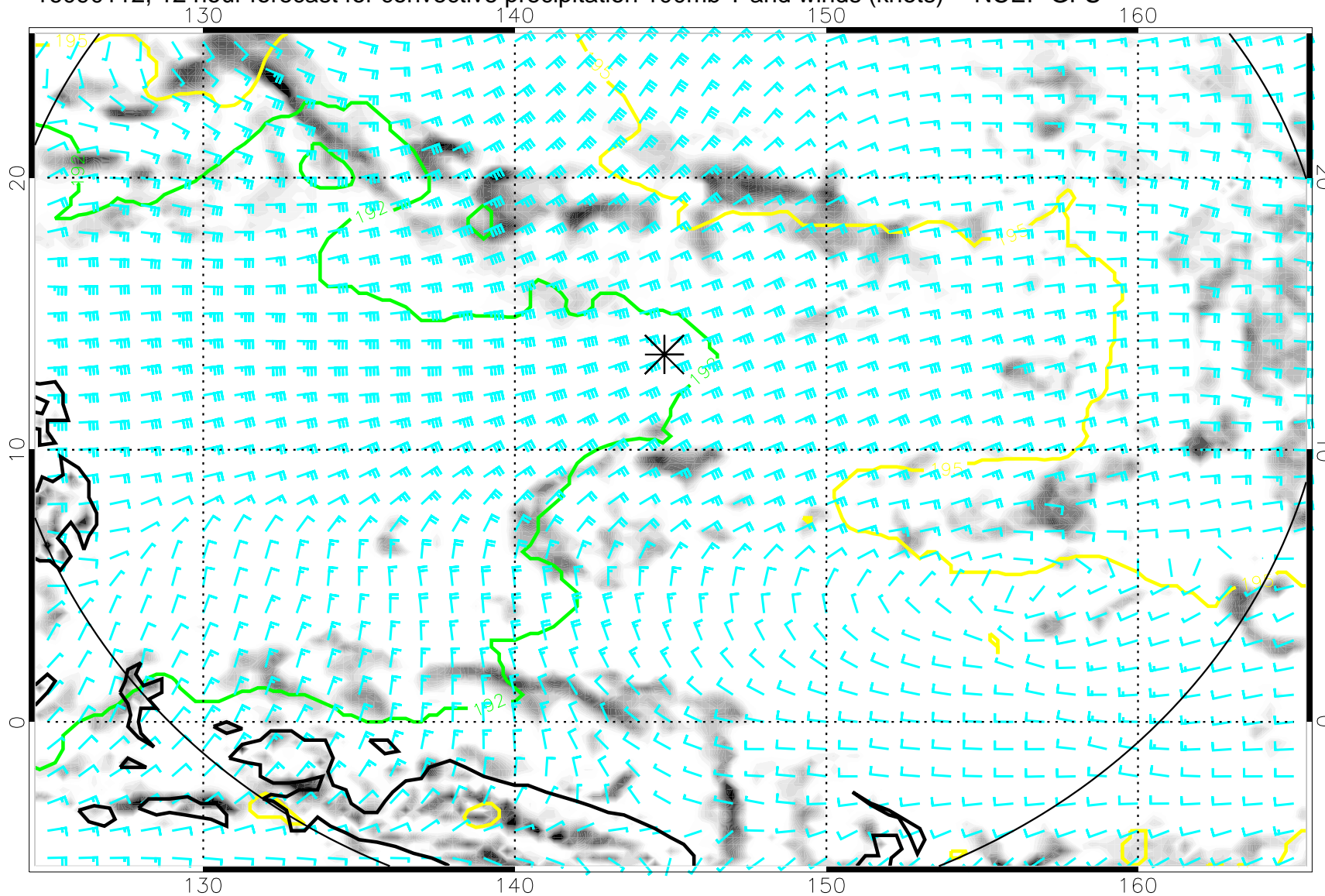
16090112, 12 hour forecast for convective precipitation 100mb T and winds (knots) -- NCEP GFS
