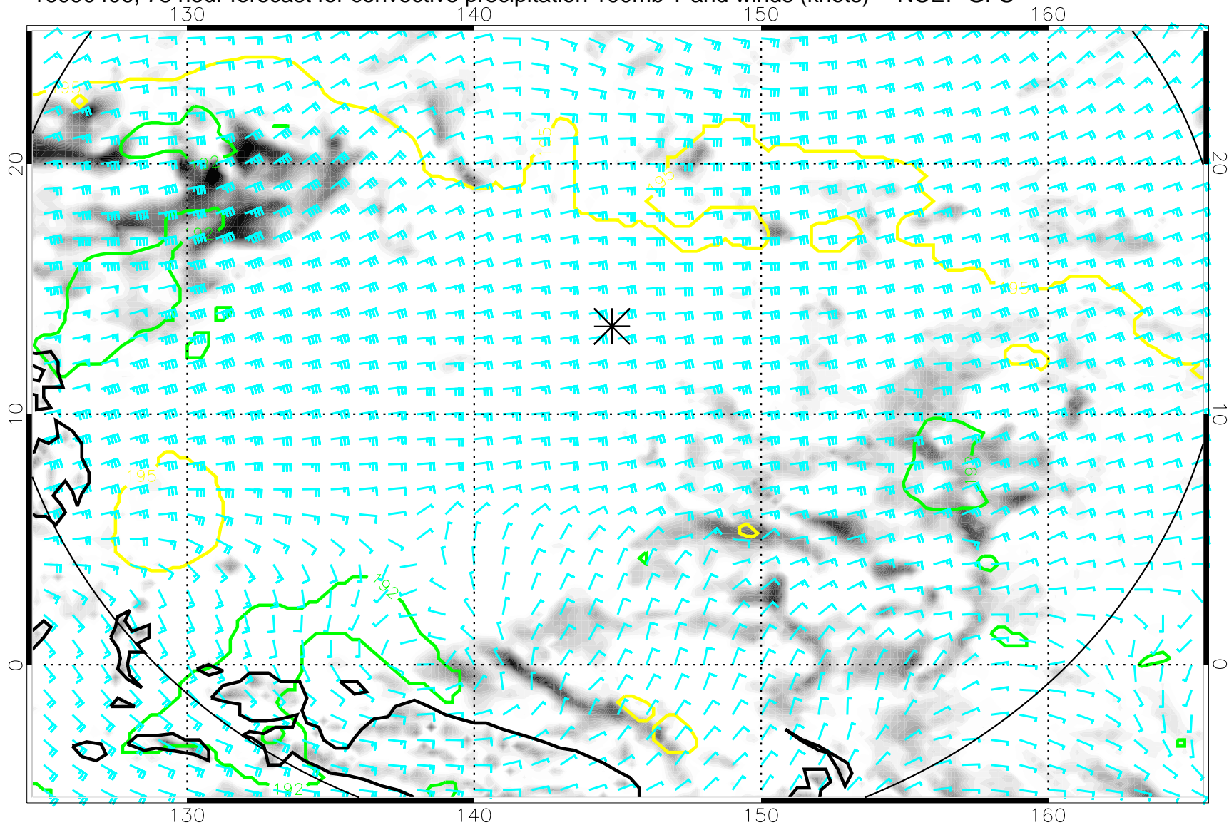
16090406, 78 hour forecast for convective precipitation 100mb T and winds (knots) -- NCEP GFS
