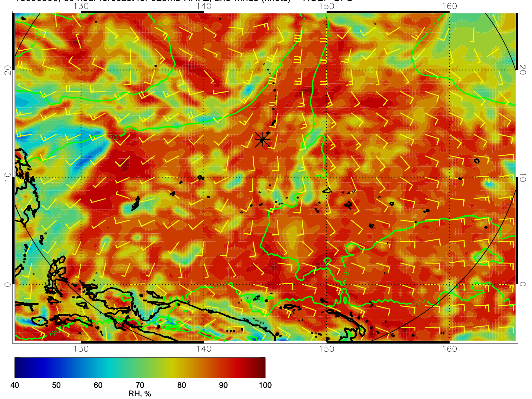
16090300, 60 hour forecast for 925mb RH, Z, and winds (knots) -- NCEP GFS
