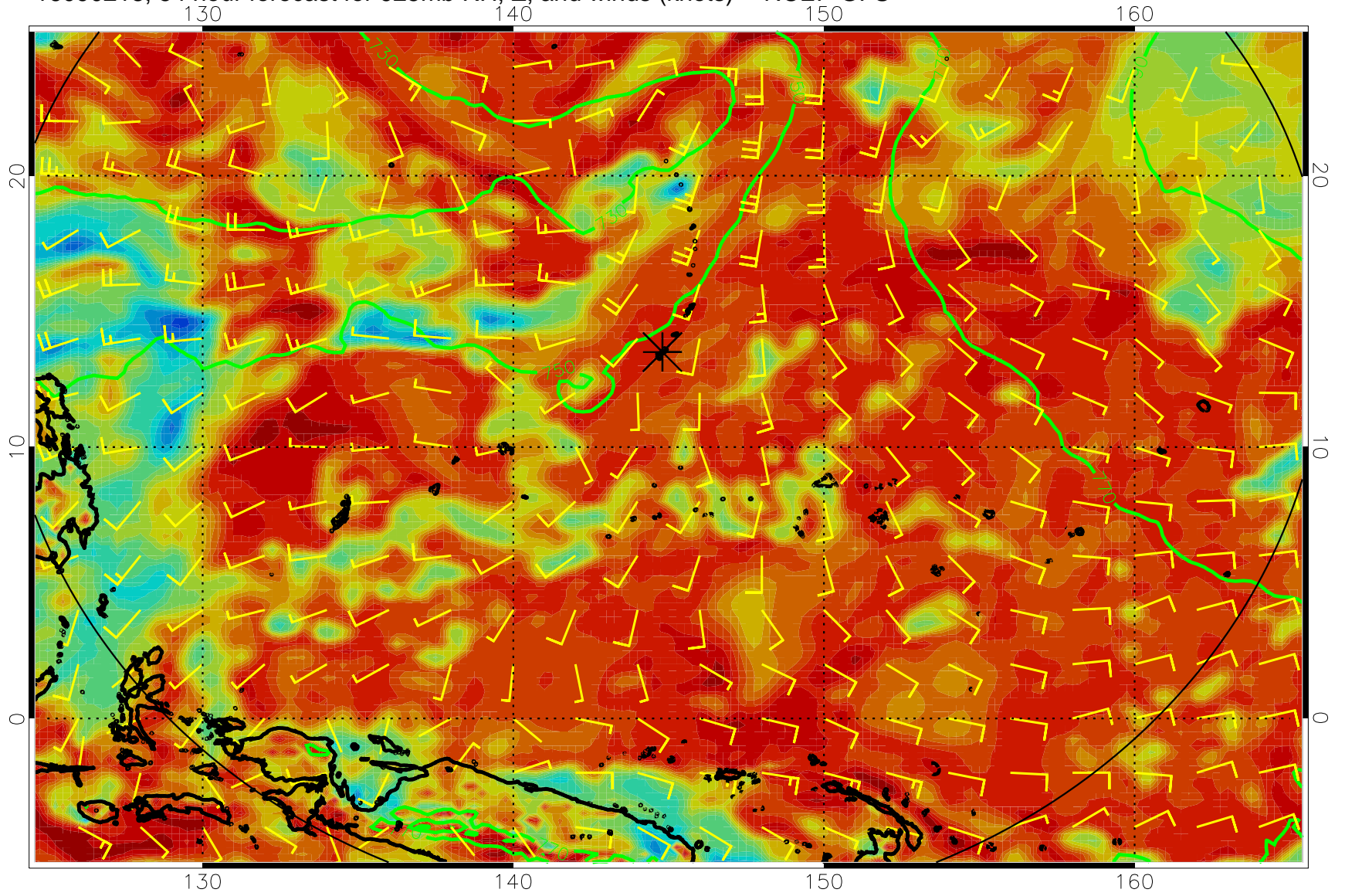
16090218, 54 hour forecast for 925mb RH, Z, and winds (knots) -- NCEP GFS
