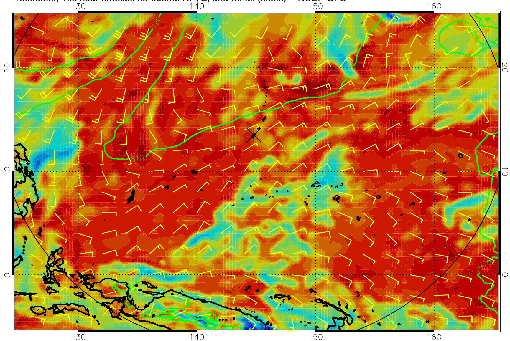
16090500, 108 hour forecast for 925mb RH, Z, and winds (knots) -- NCEP GFS
