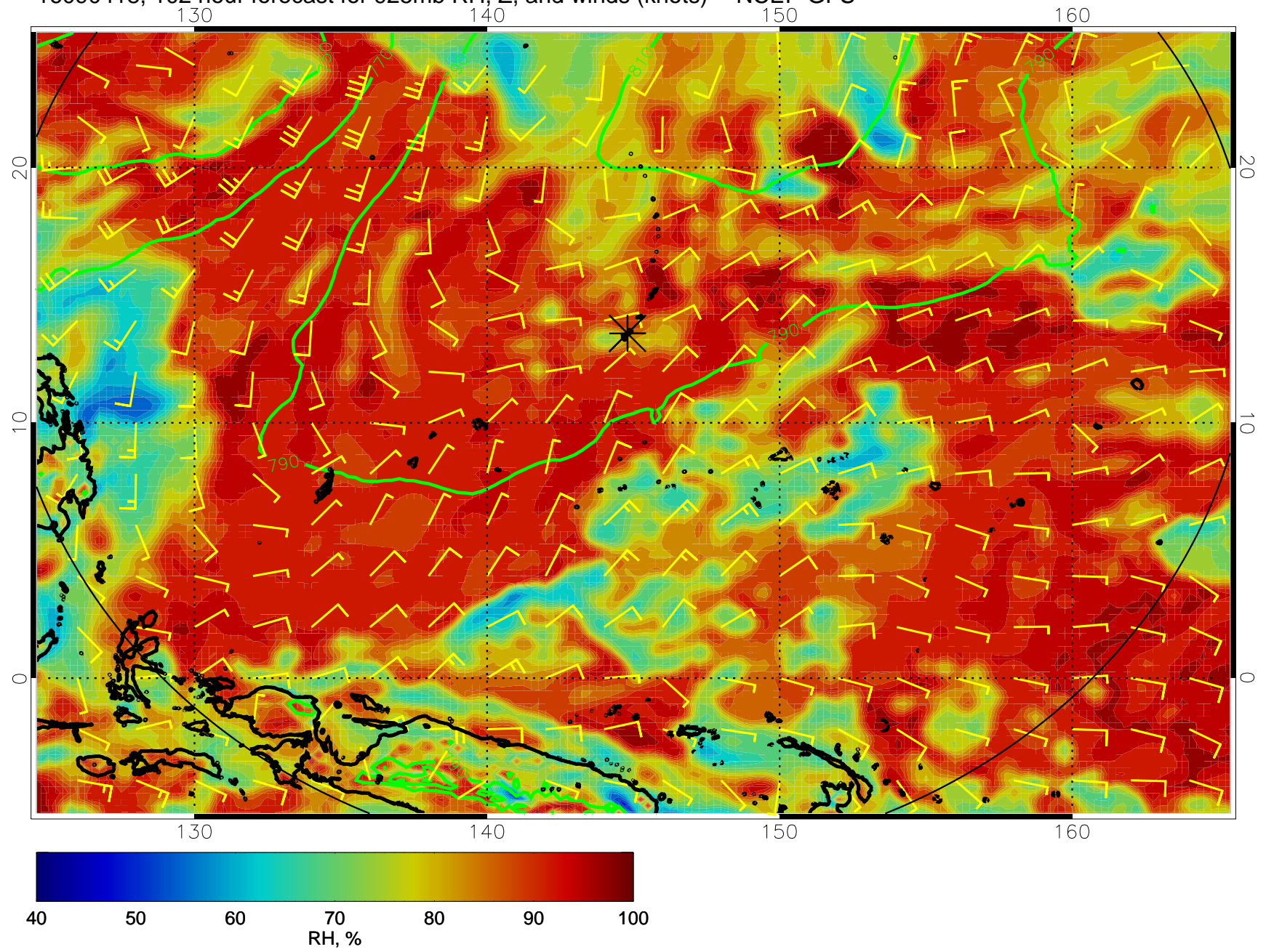
16090418, 102 hour forecast for 925mb RH, Z, and winds (knots) -- NCEP GFS
