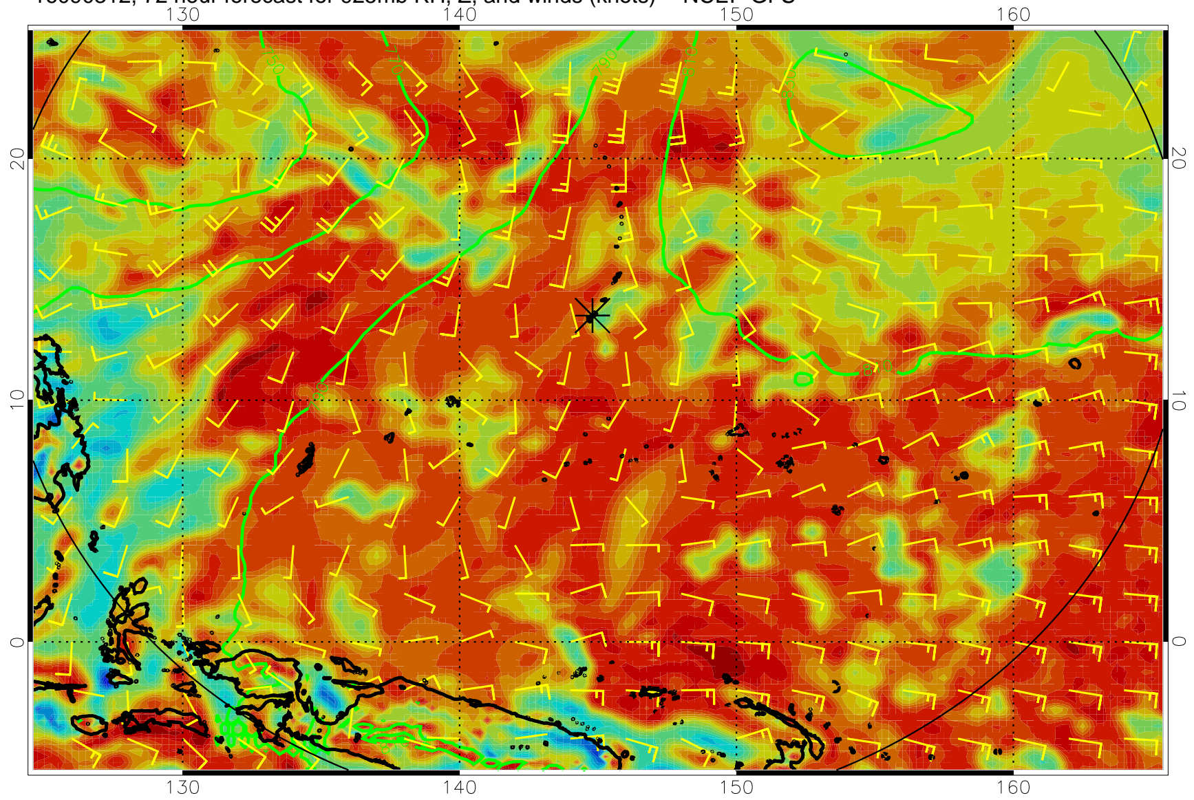
16090312, 72 hour forecast for 925mb RH, Z, and winds (knots) -- NCEP GFS
