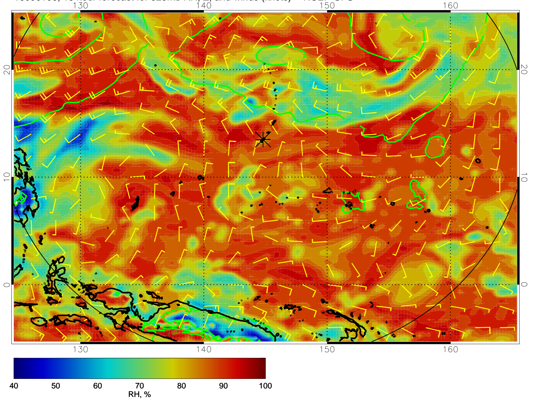
16090106, 18 hour forecast for 925mb RH, Z, and winds (knots) -- NCEP GFS
