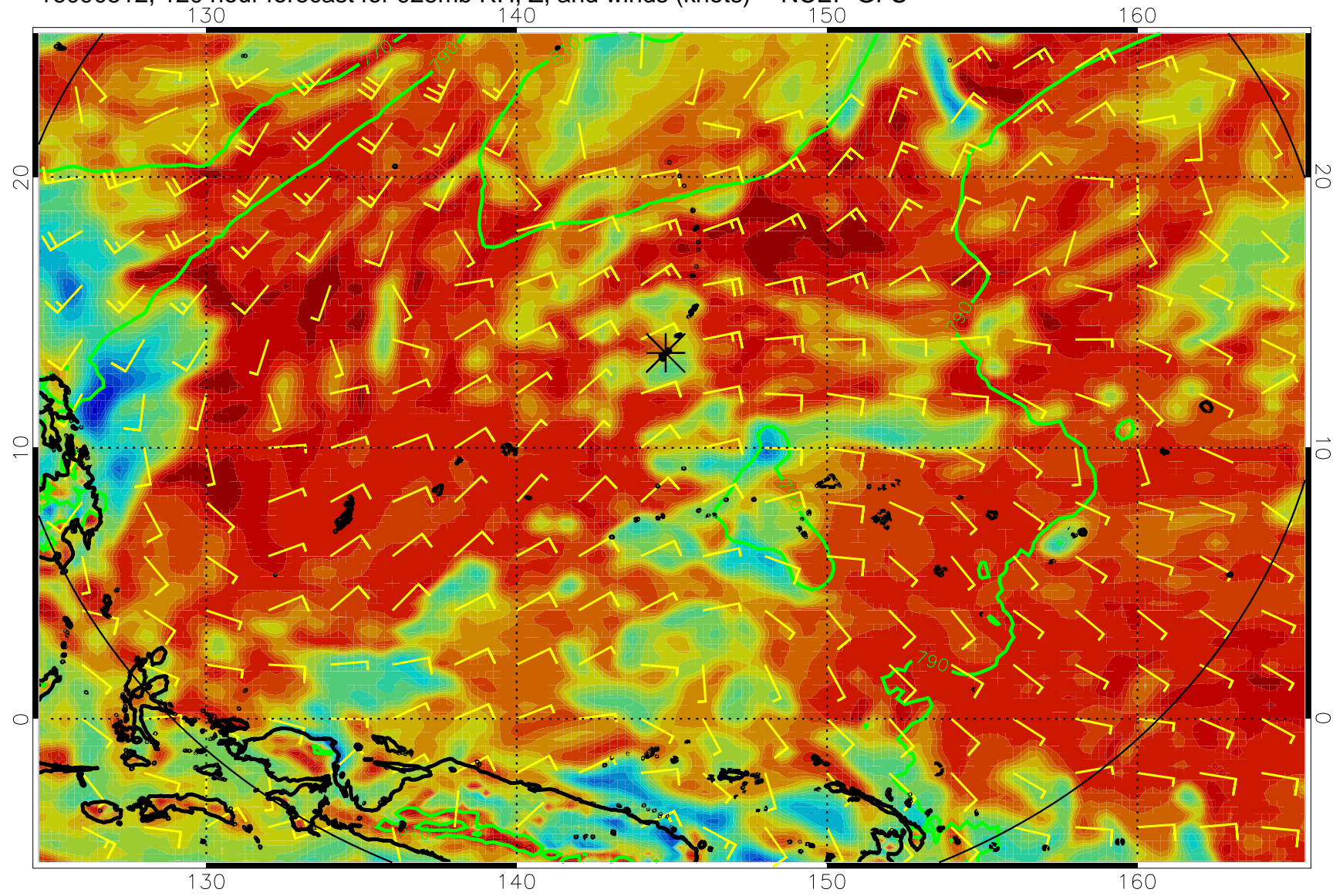
16090512, 120 hour forecast for 925mb RH, Z, and winds (knots) -- NCEP GFS
