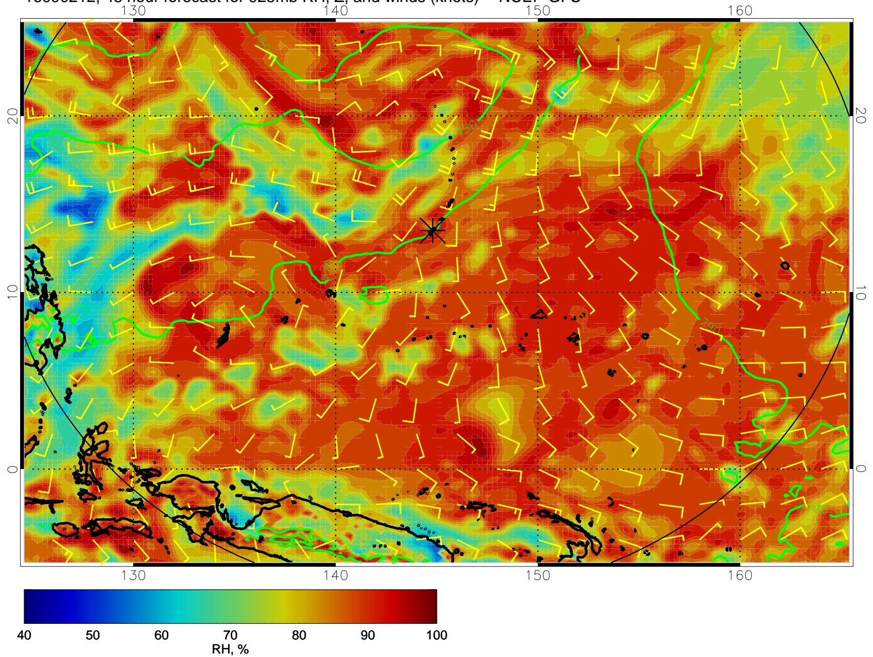
16090212, 48 hour forecast for 925mb RH, Z, and winds (knots) -- NCEP GFS
