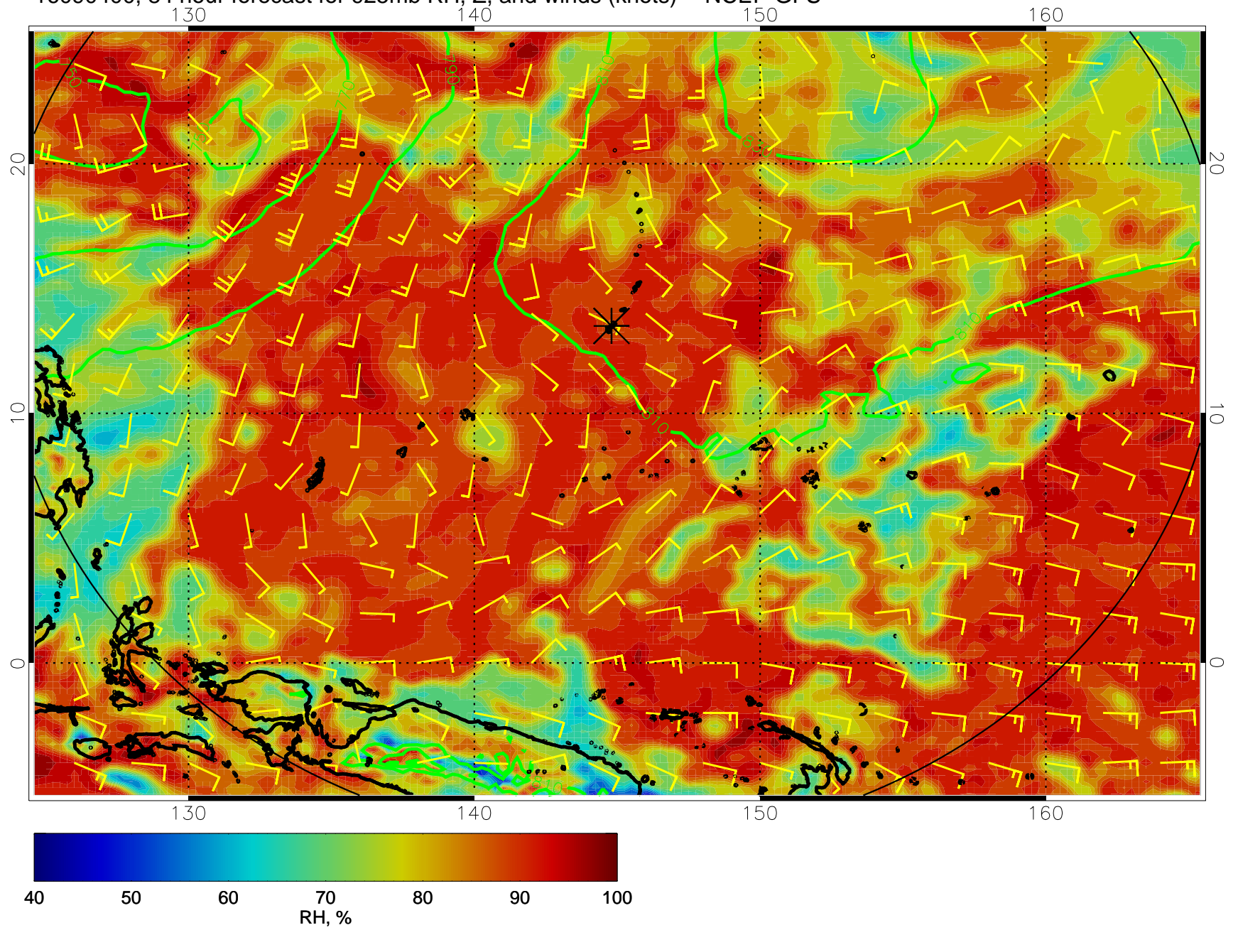
16090400, 84 hour forecast for 925mb RH, Z, and winds (knots) -- NCEP GFS
