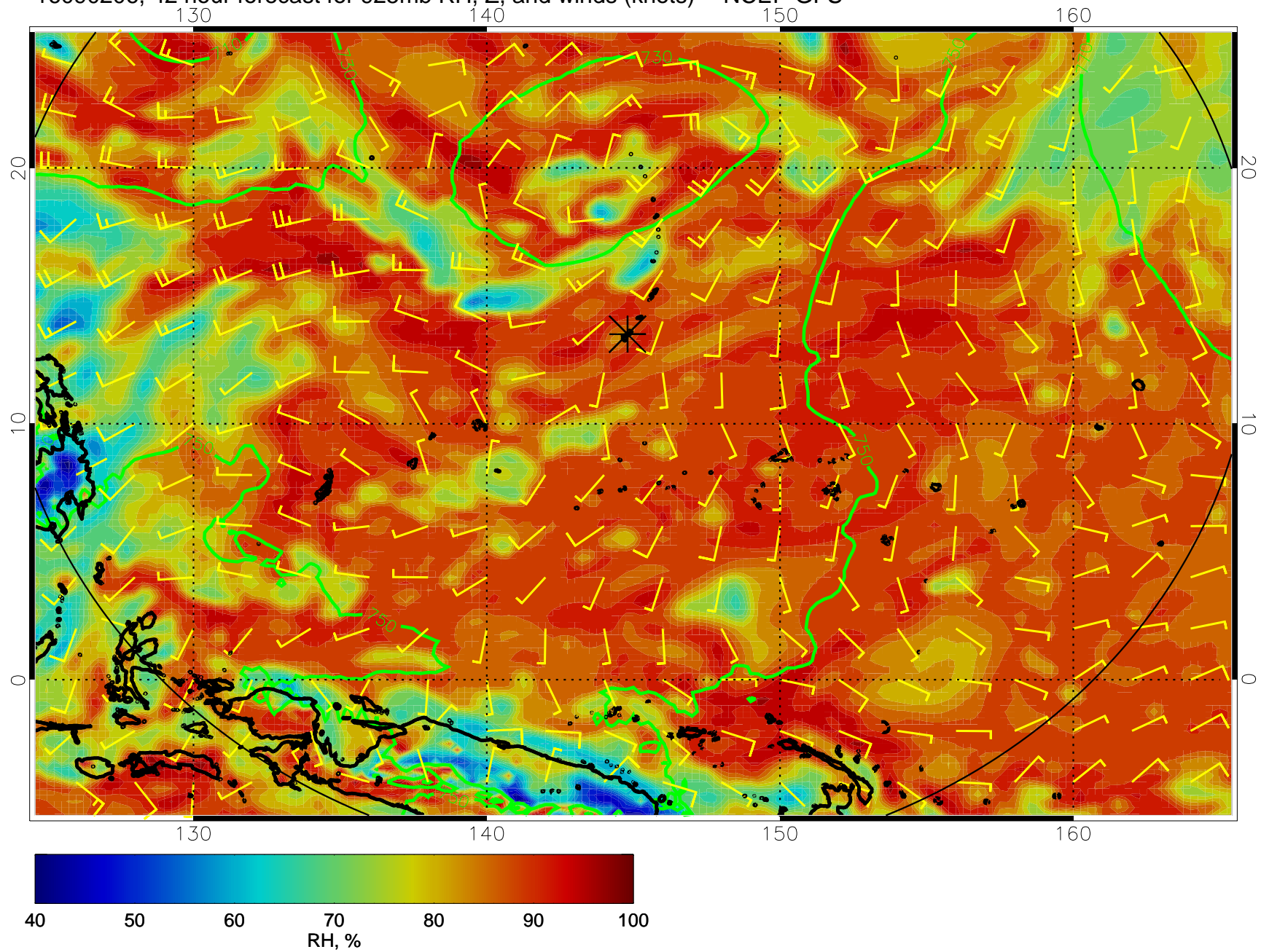
16090206, 42 hour forecast for 925mb RH, Z, and winds (knots) -- NCEP GFS
