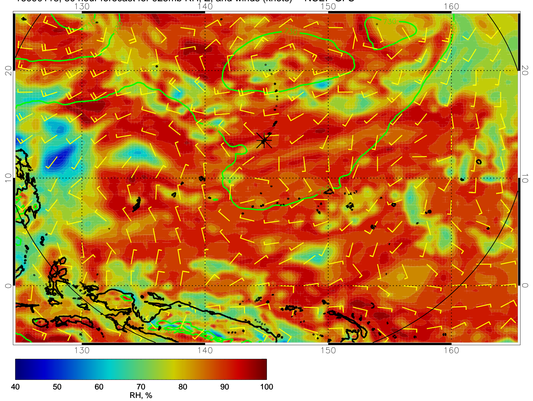
16090118, 30 hour forecast for 925mb RH, Z, and winds (knots) -- NCEP GFS
