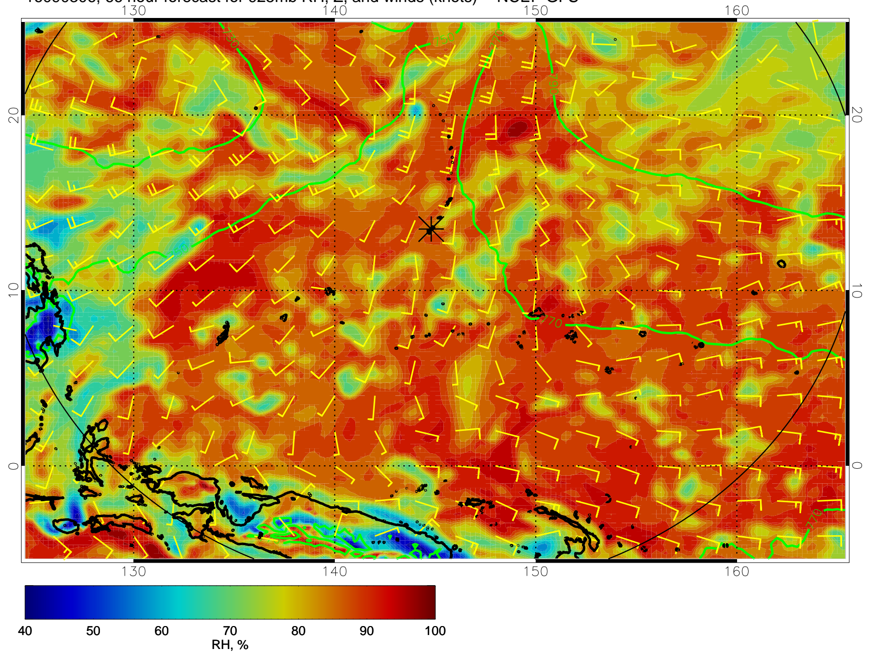
16090306, 66 hour forecast for 925mb RH, Z, and winds (knots) -- NCEP GFS
