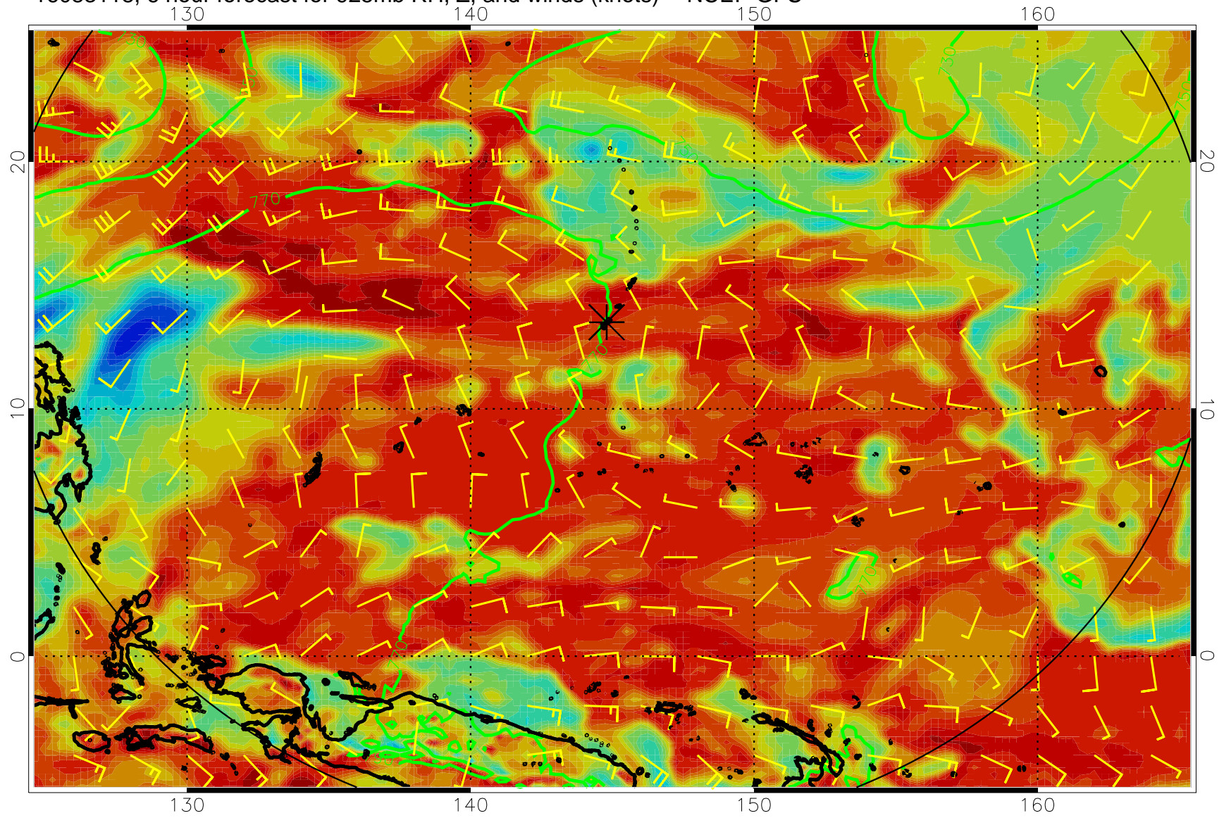
16083118, 6 hour forecast for 925mb RH, Z, and winds (knots) -- NCEP GFS
