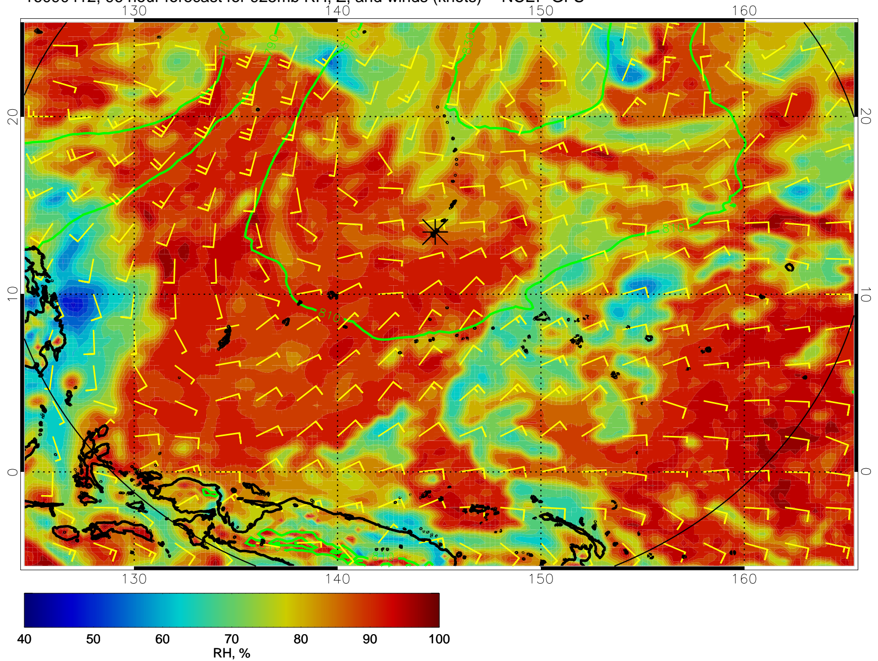
16090412, 96 hour forecast for 925mb RH, Z, and winds (knots) -- NCEP GFS
