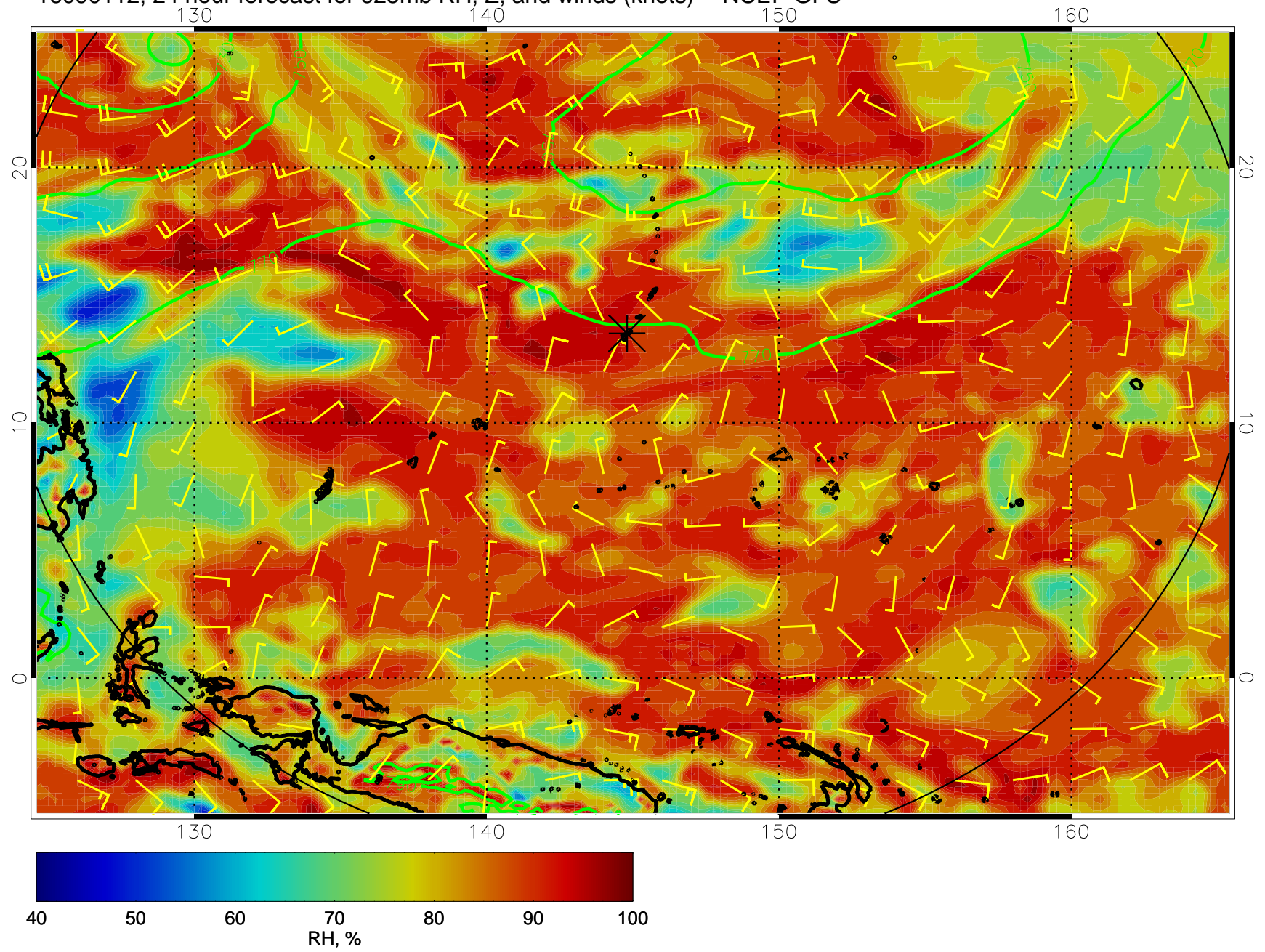
16090112, 24 hour forecast for 925mb RH, Z, and winds (knots) -- NCEP GFS
