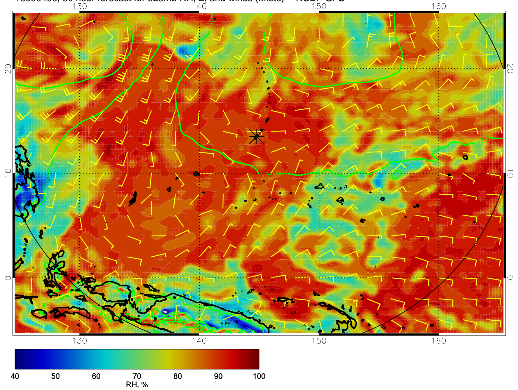
16090406, 90 hour forecast for 925mb RH, Z, and winds (knots) -- NCEP GFS
