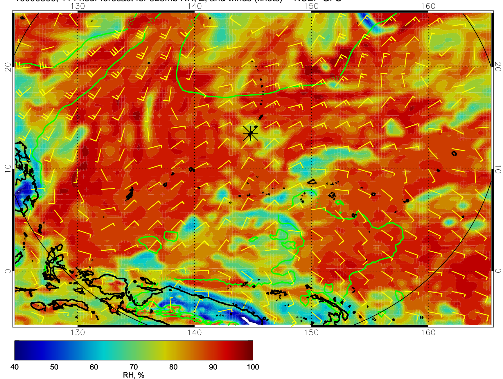
16090506, 114 hour forecast for 925mb RH, Z, and winds (knots) -- NCEP GFS
