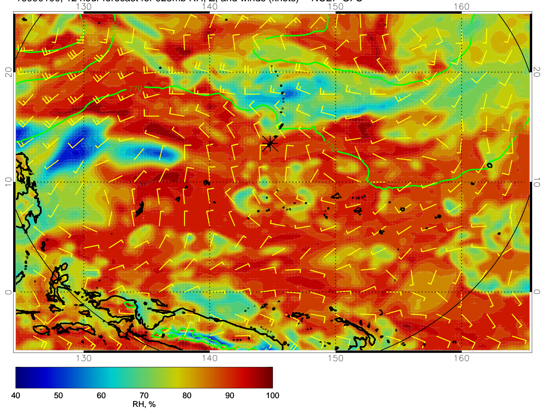
16090100, 12 hour forecast for 925mb RH, Z, and winds (knots) -- NCEP GFS
